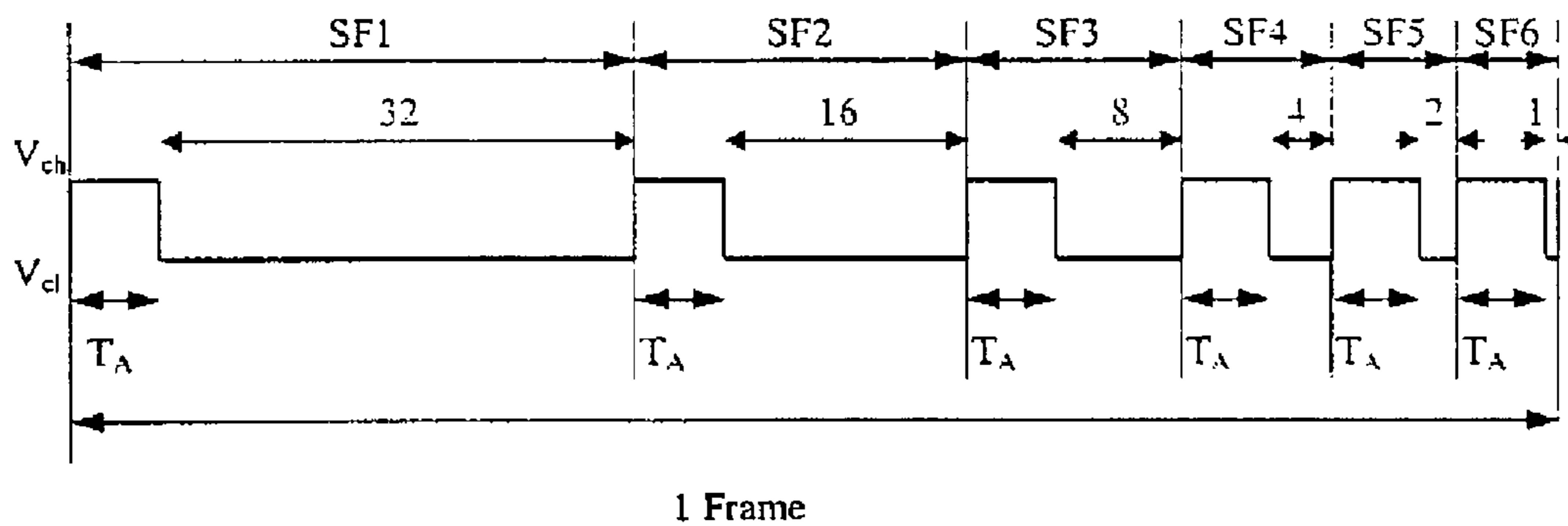
SF1-SF6:sub-frame, TA: write in time
