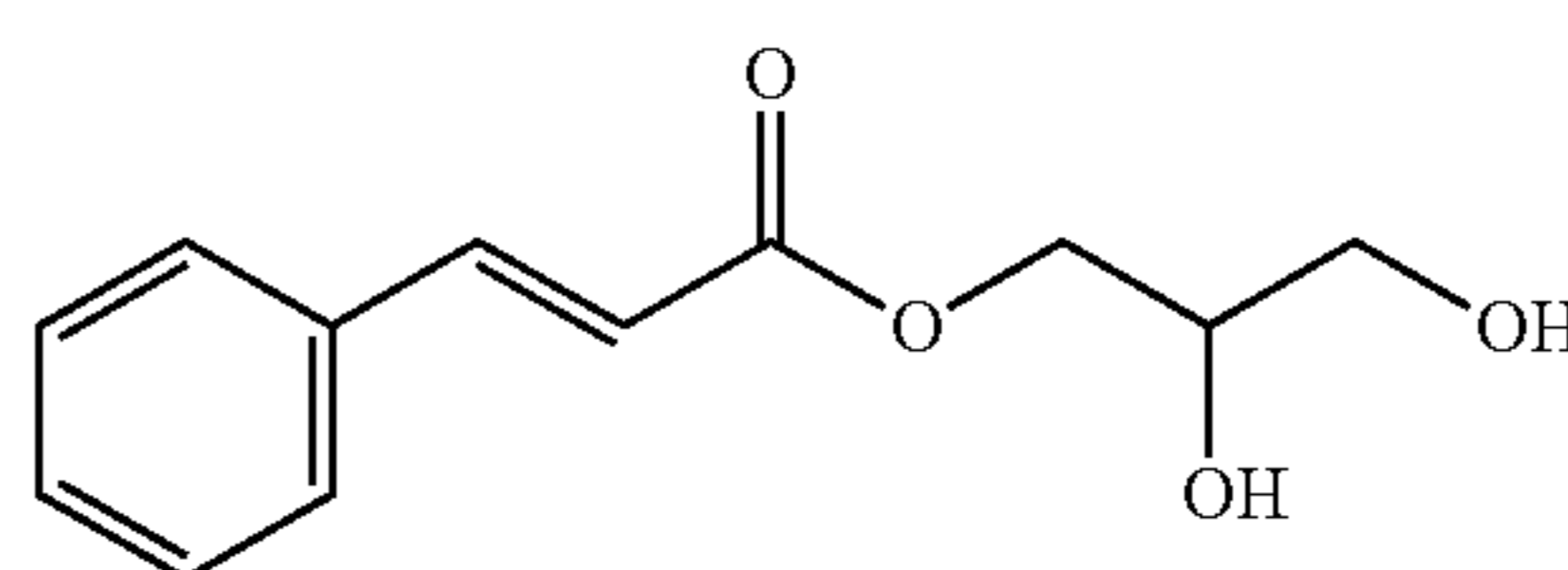
Glycerol Mono-Cinnamate
