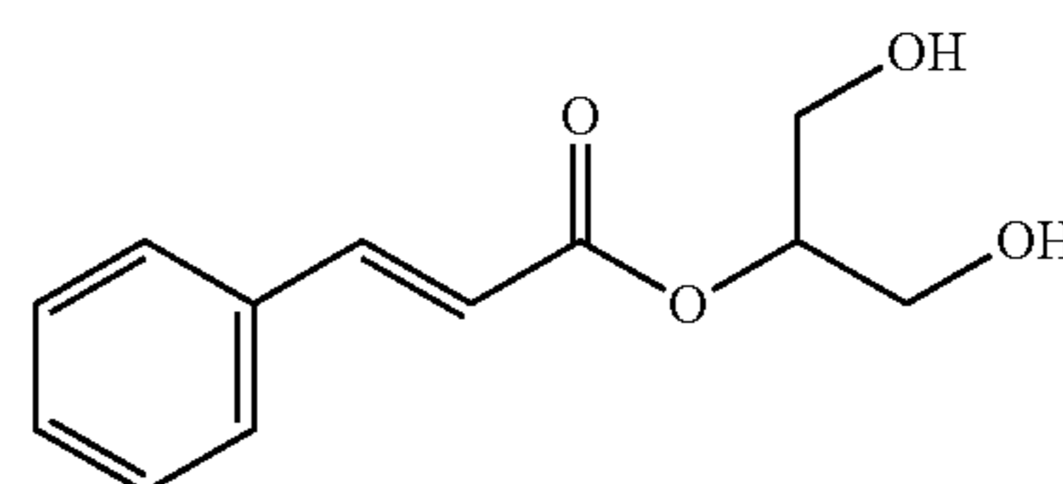
Glycerol Mono-Cinnamate
