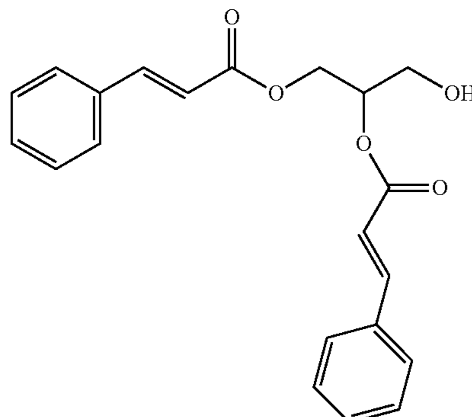
Glycerol Di-Cinnamate
