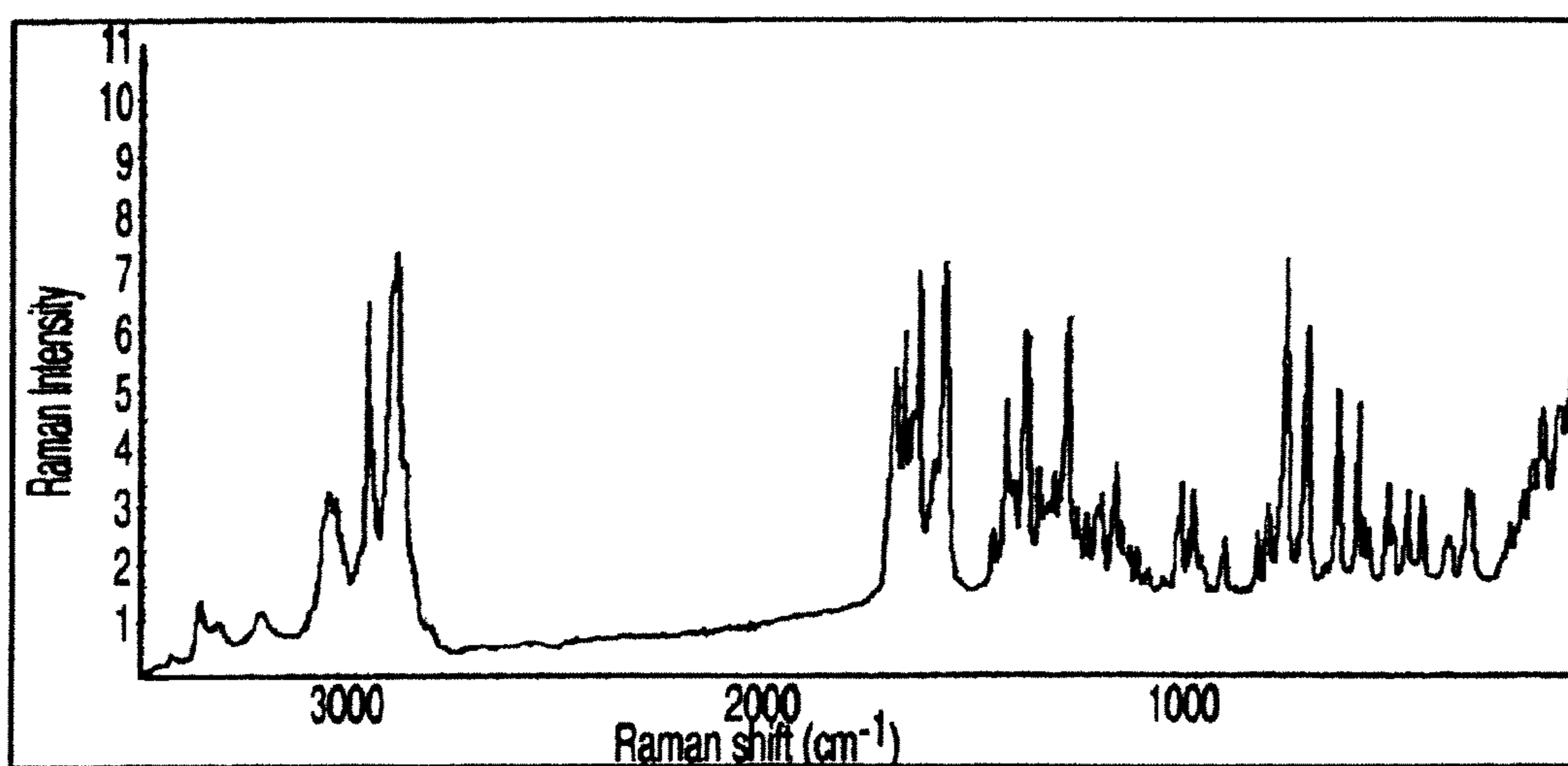
RAMAN SPECTRUM OF FORM C
