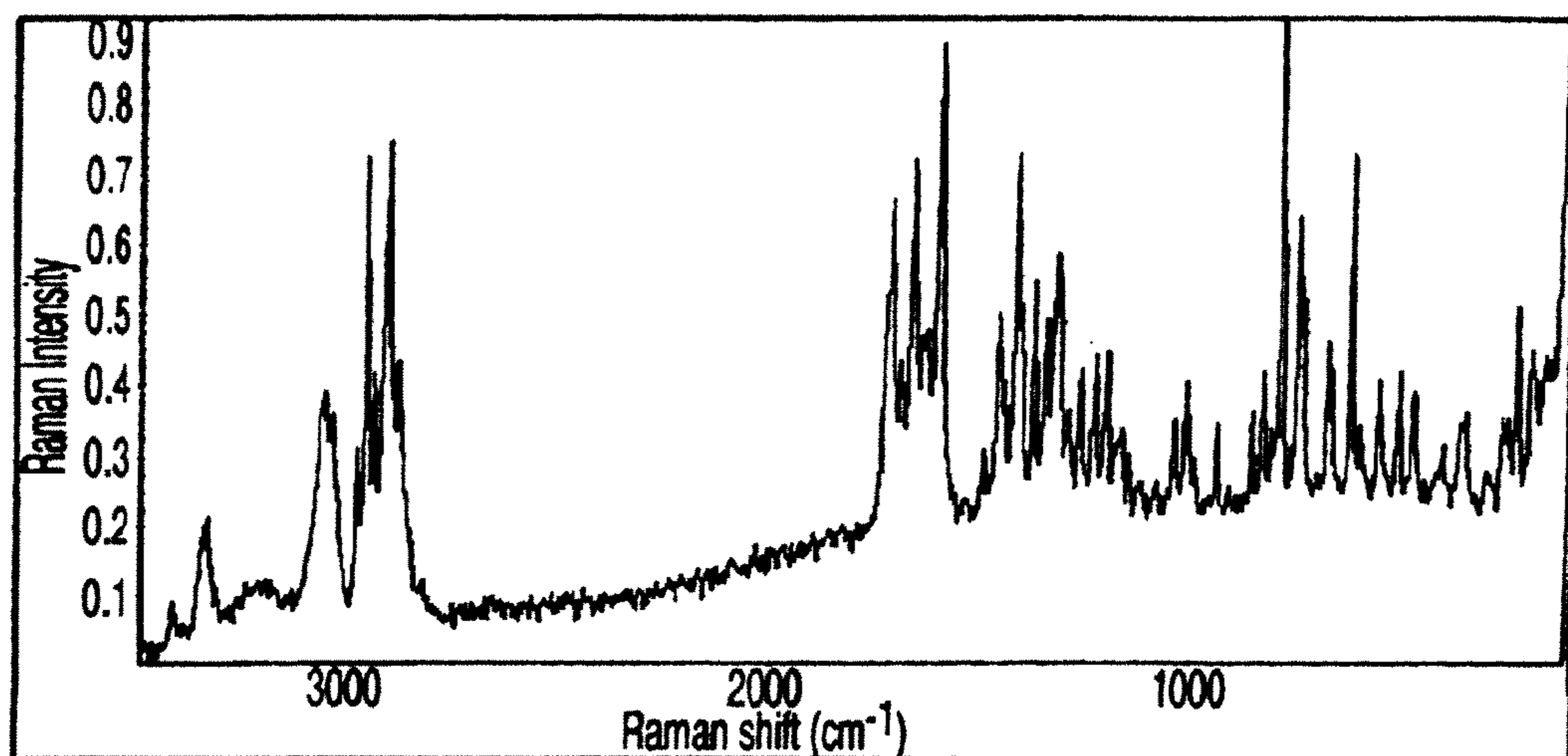
RAMAN SPECTRUM OF FORM B
