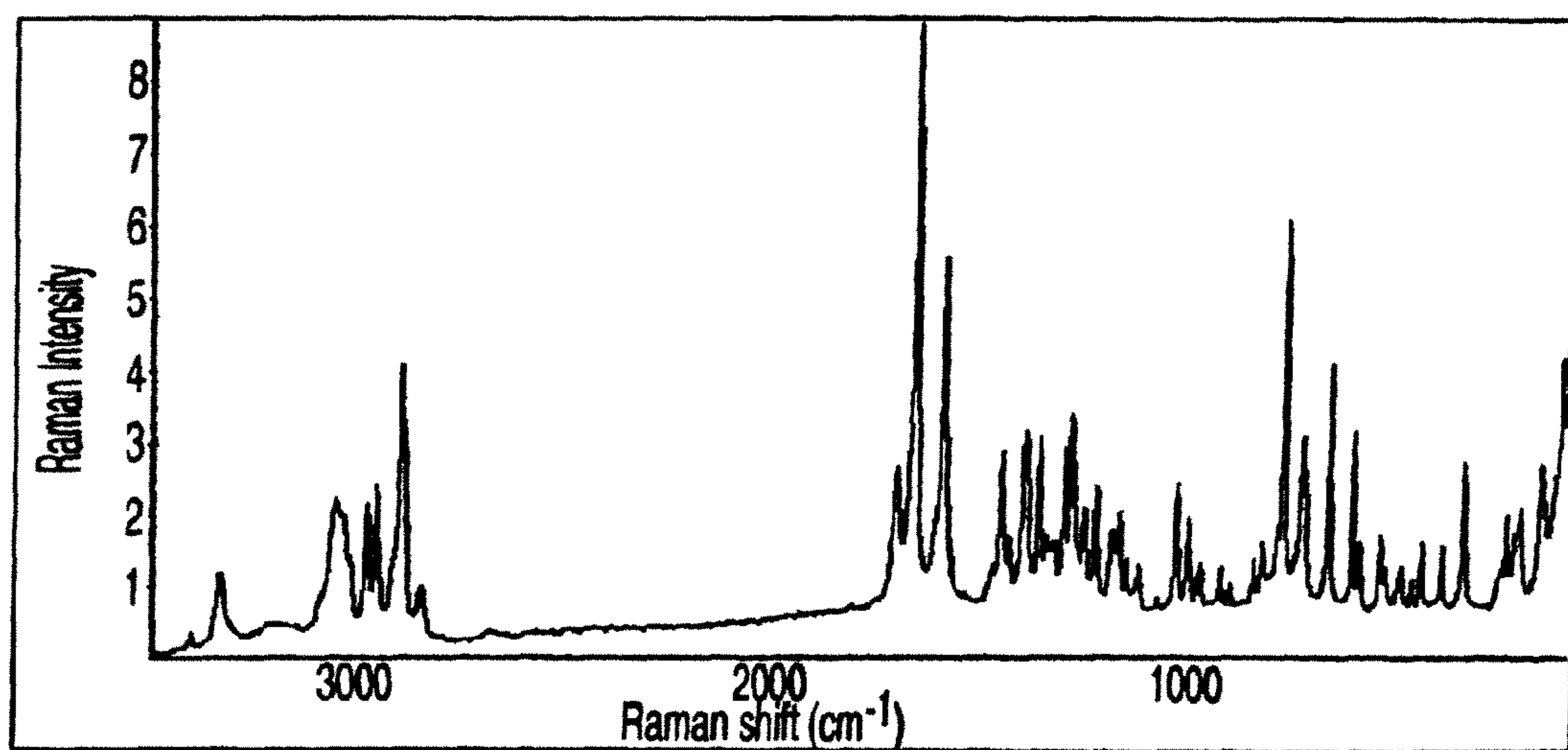
RAMAN SPECTRUM OF FORM A
