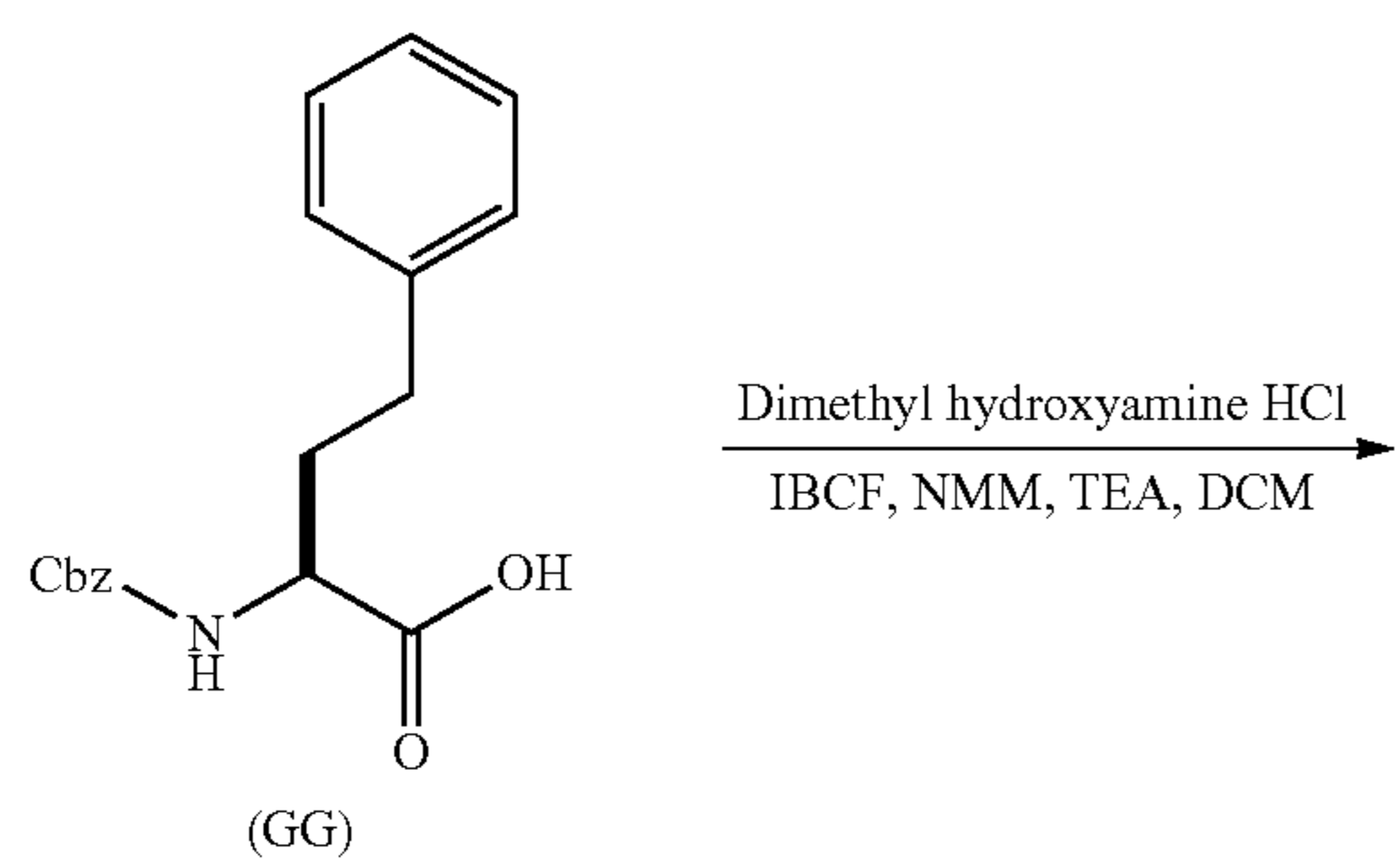
Scheme 8: Synthesis of Example 8
