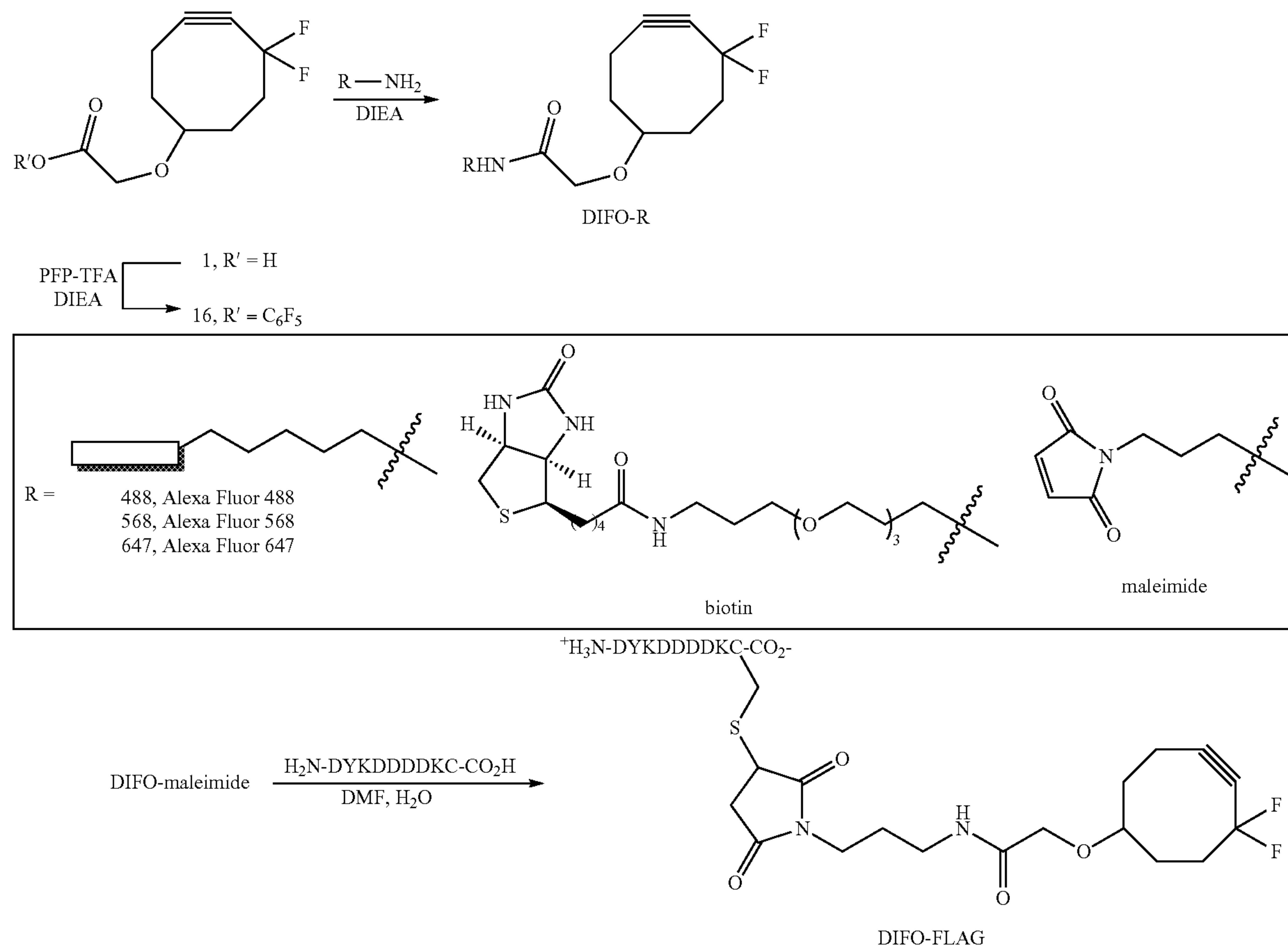
Scheme 7. Synthesis of conjugates of DIFO (biotin, Alexa Fluor 488, 568, and 647, and FLAG peptide)
