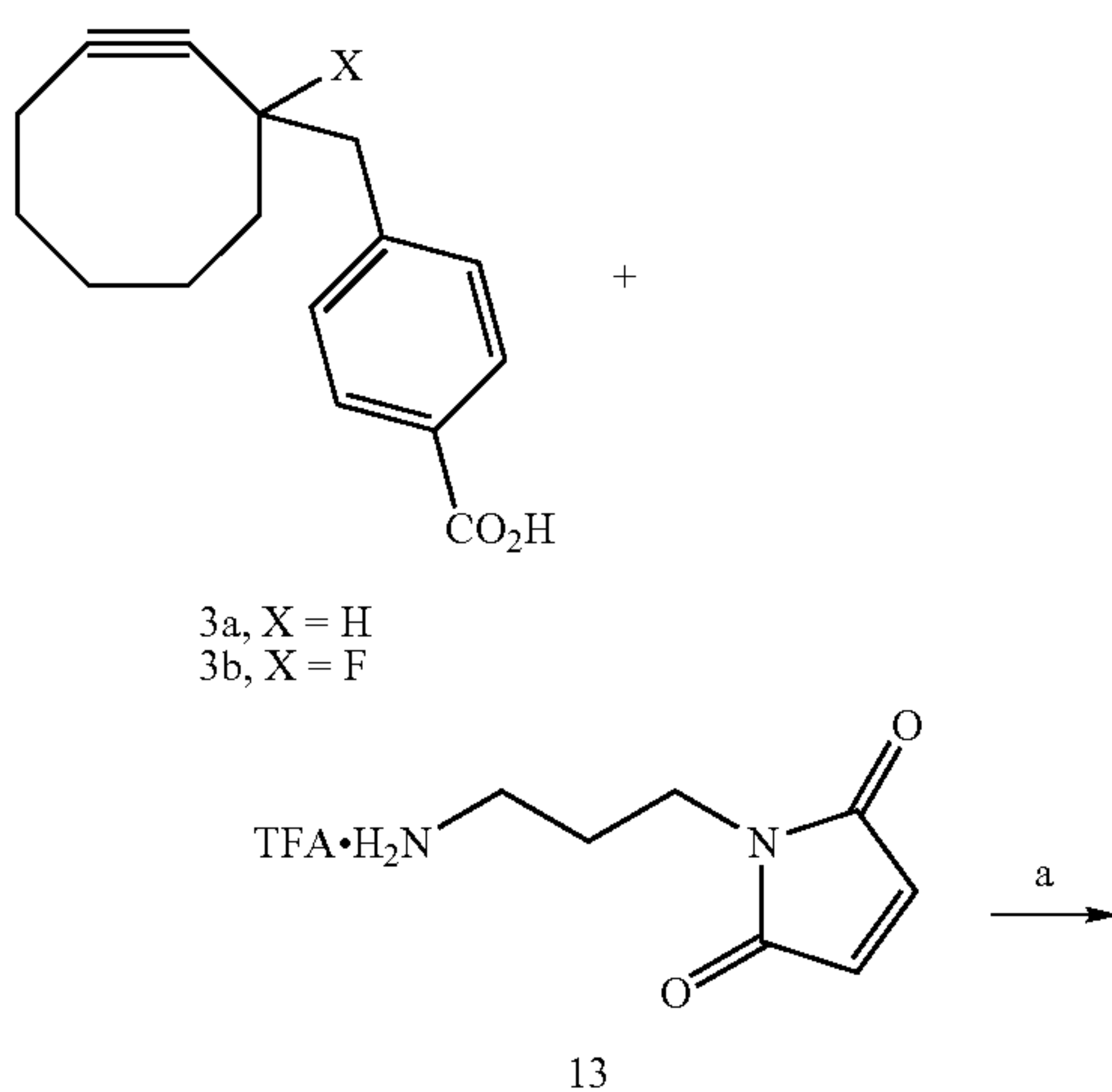
Scheme 2
