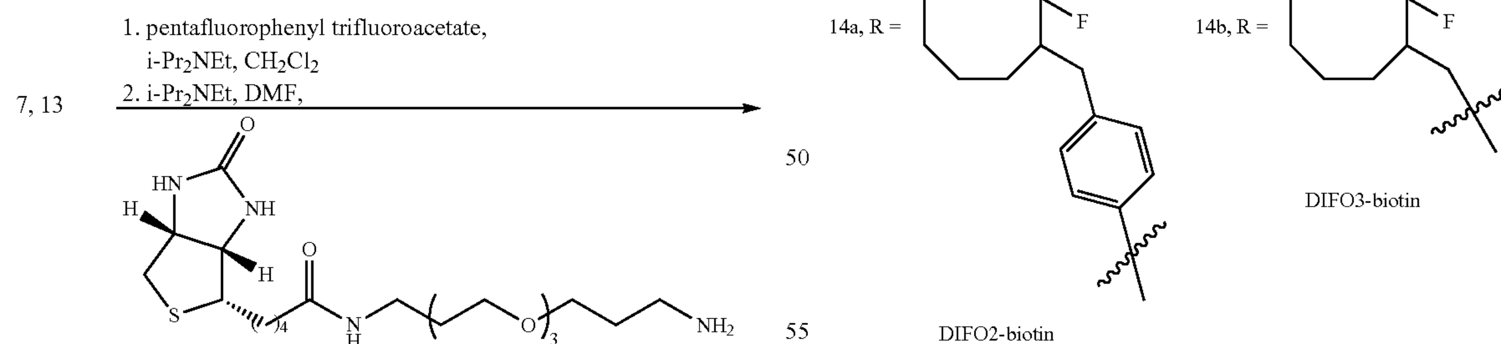
Scheme 10. Synthesis of biotin conjugates of DIFO2 and DIFO3.
