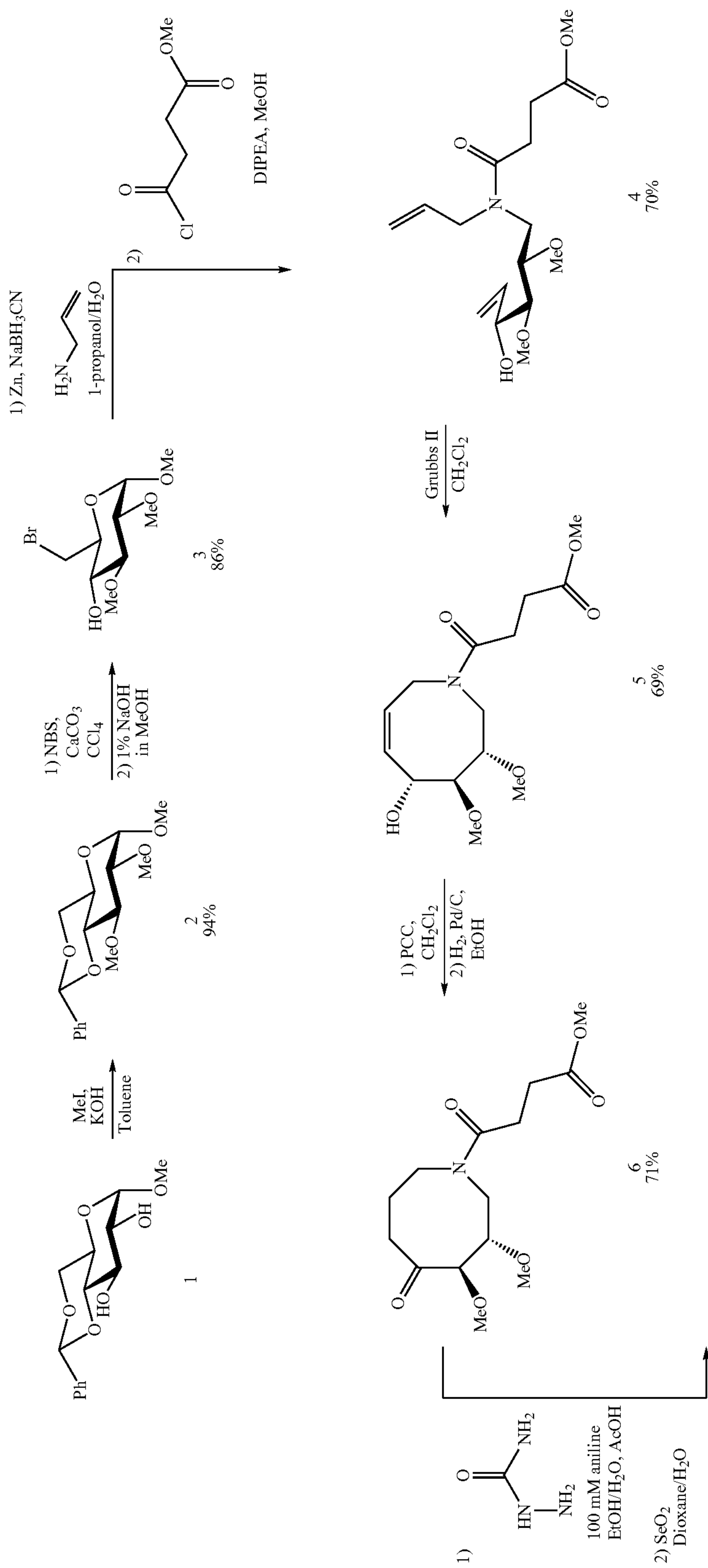
Scheme 3
