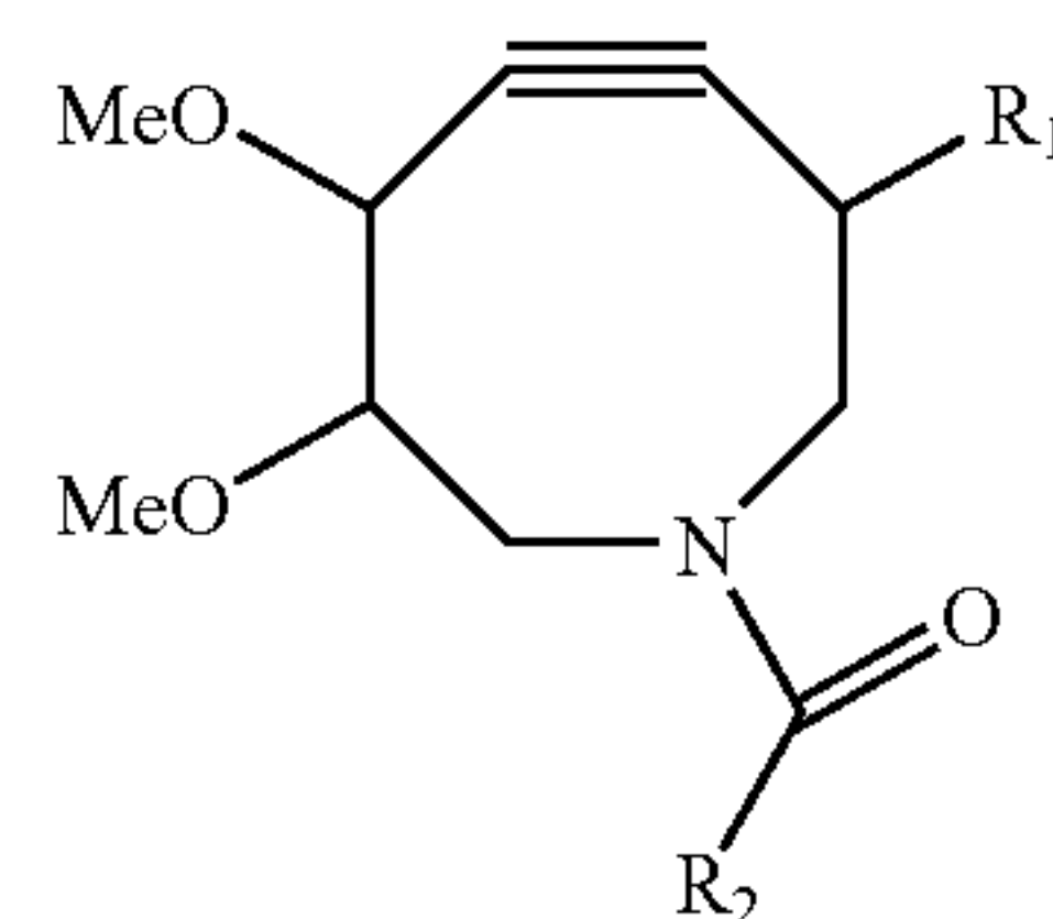
Formula XI
