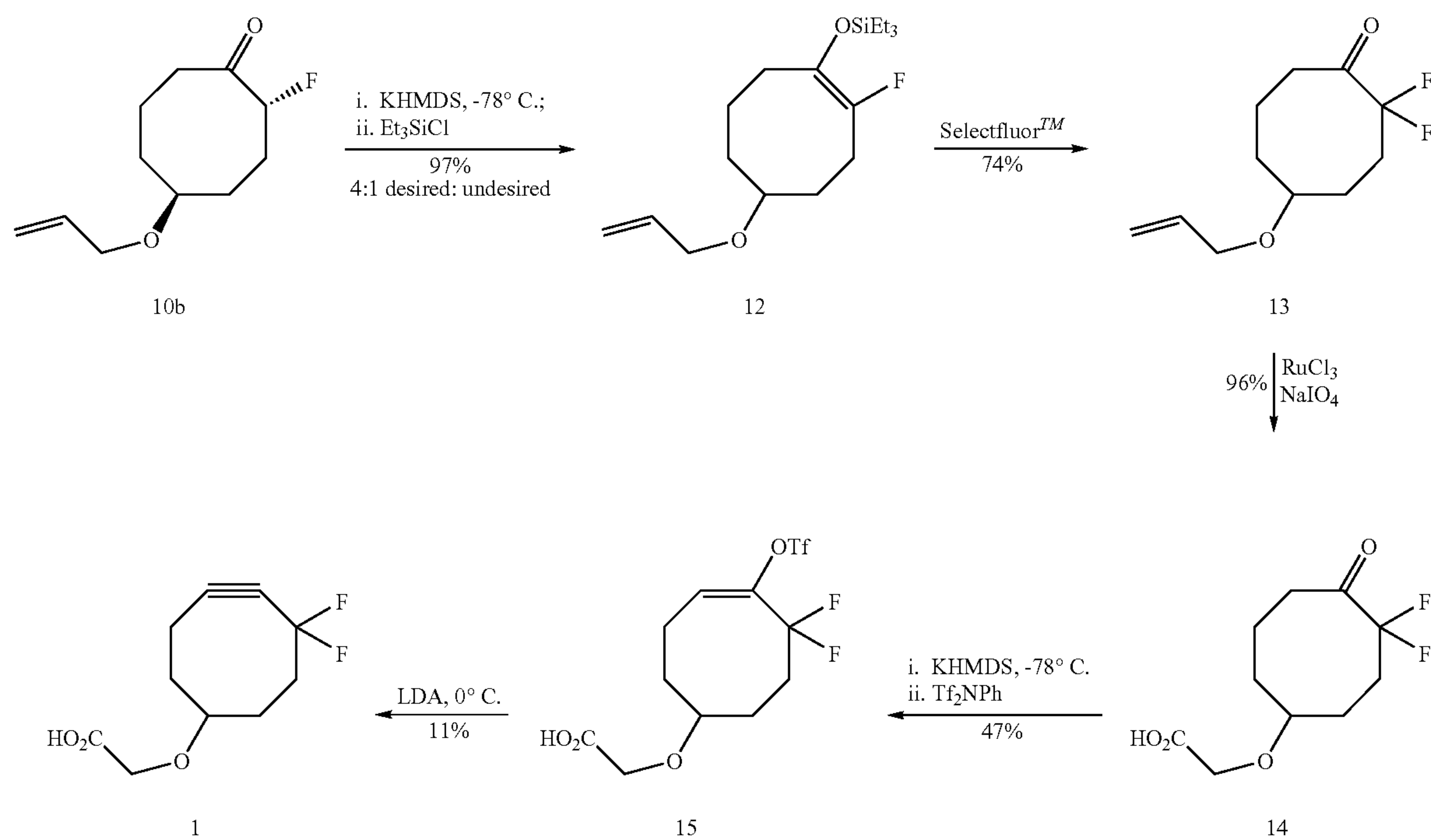
Scheme 6. Synthesis of DIFO (1), part II
