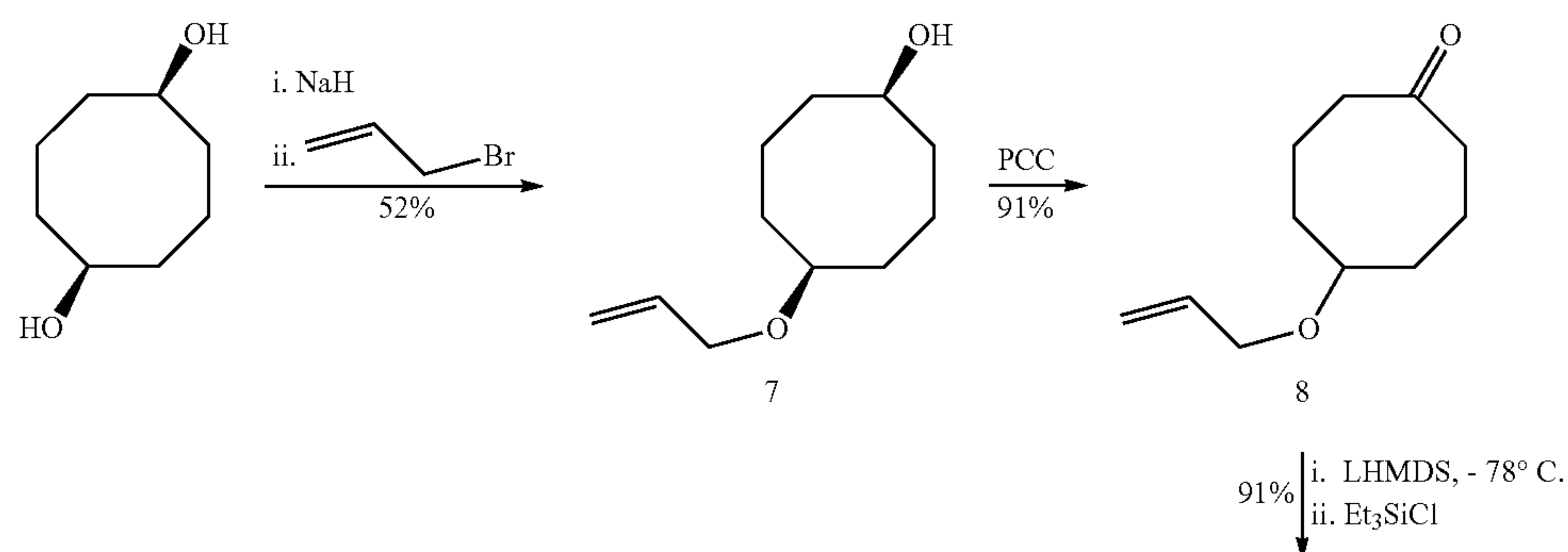
Scheme 5 Synthesis of DIFO (1), part I.
