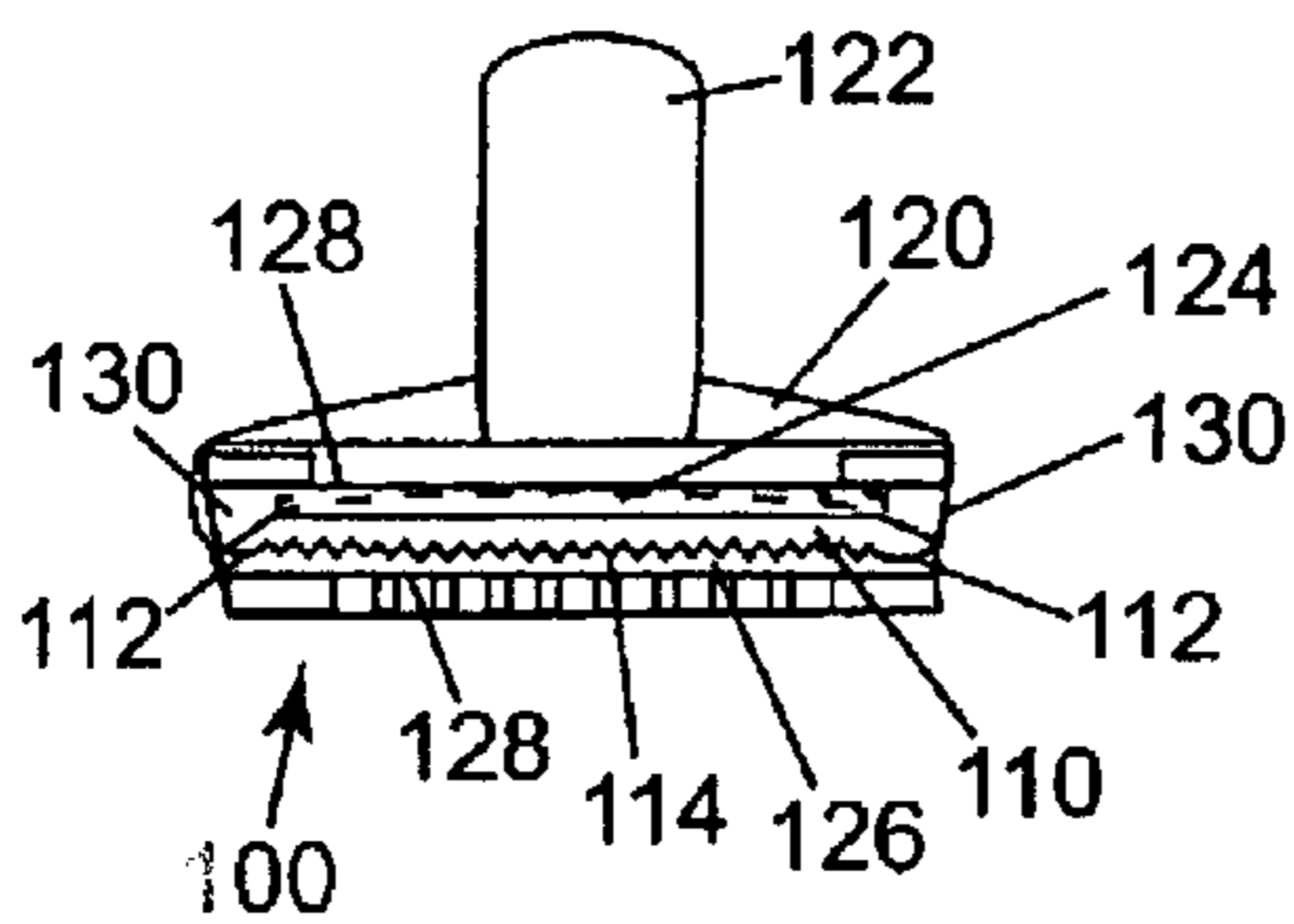
Fig. 1D
