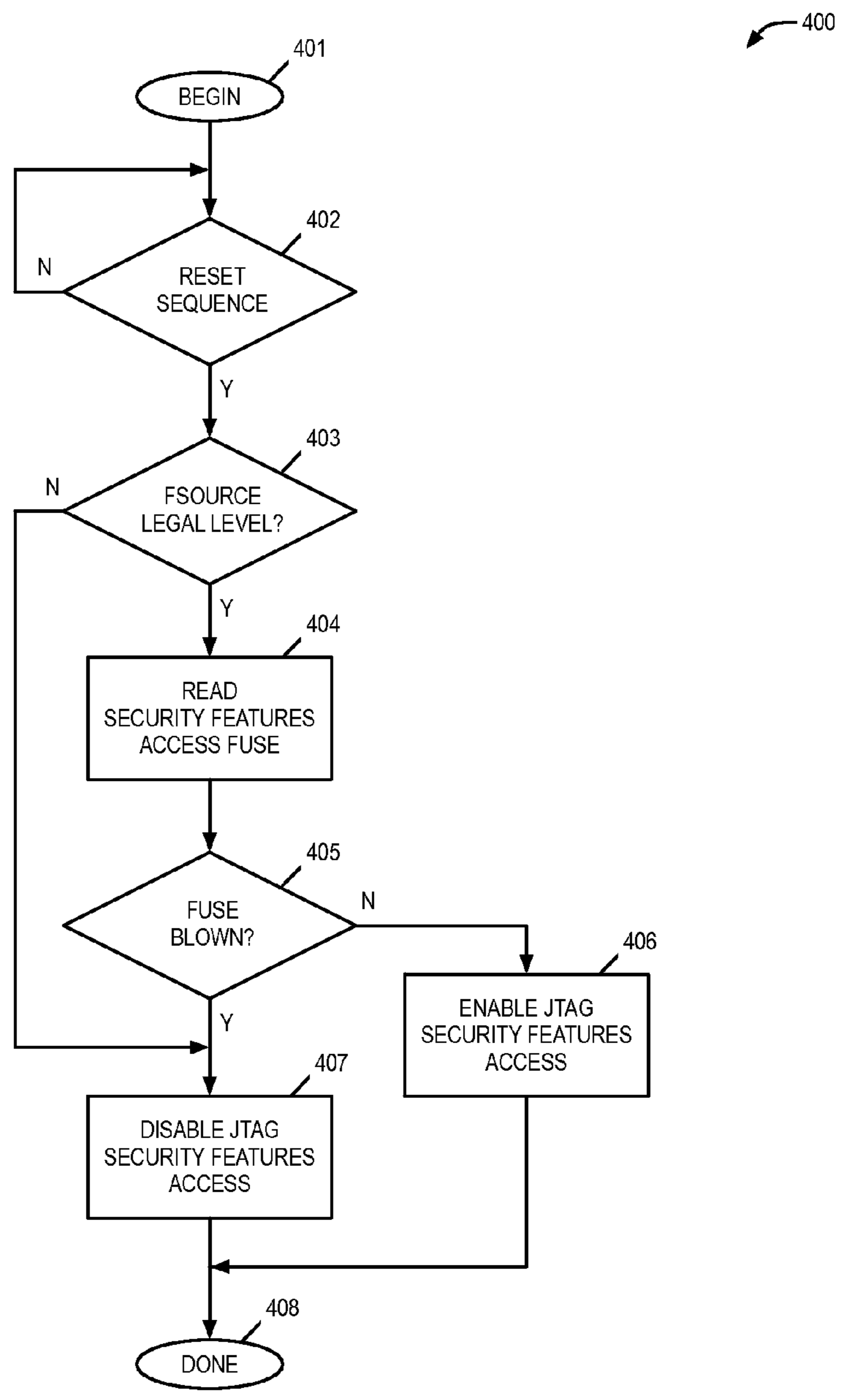
METHOD FOR FUSE ARRAY TAMPER PROTECTION
