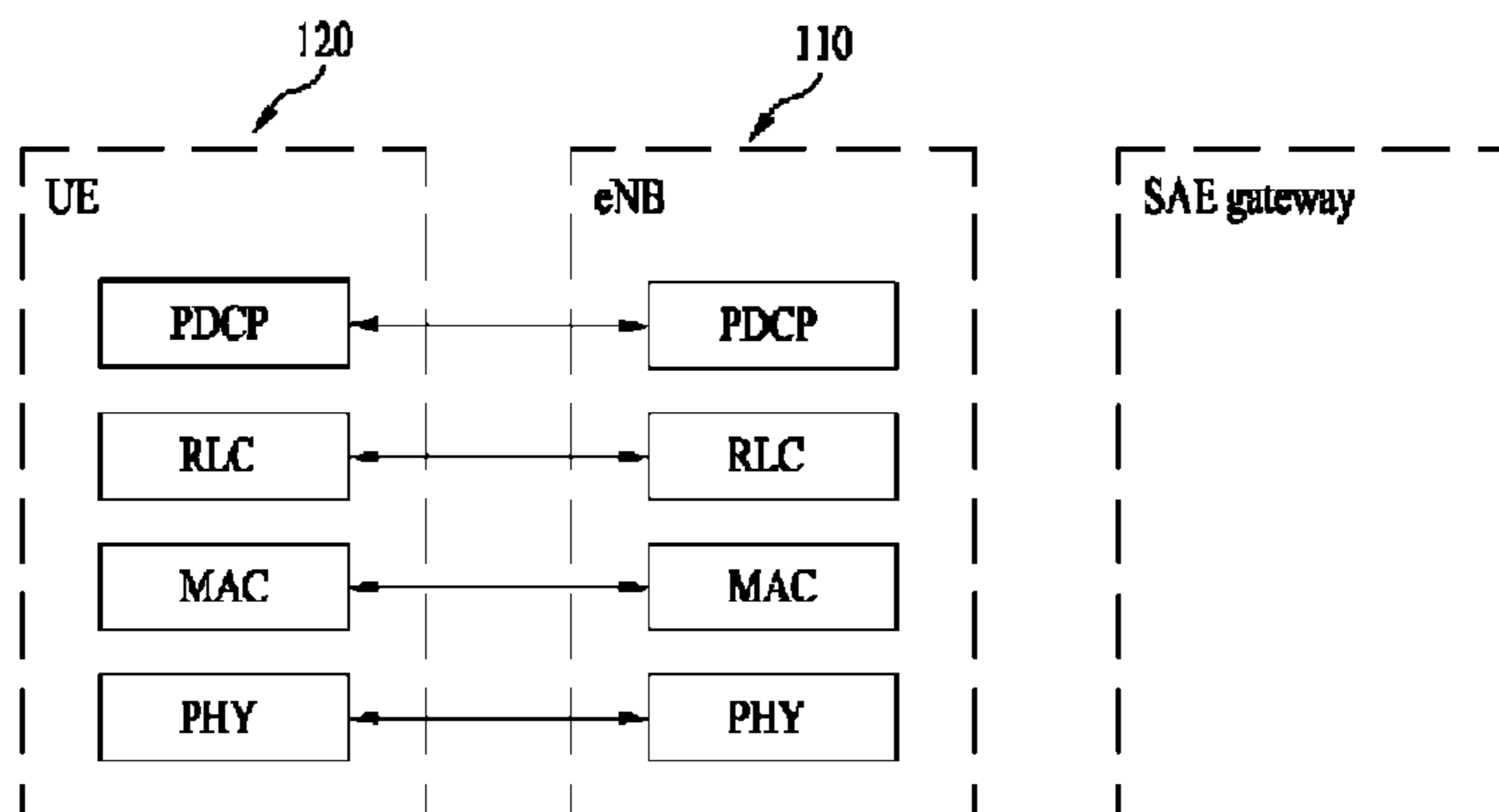
(b) user-plane protocol stack
