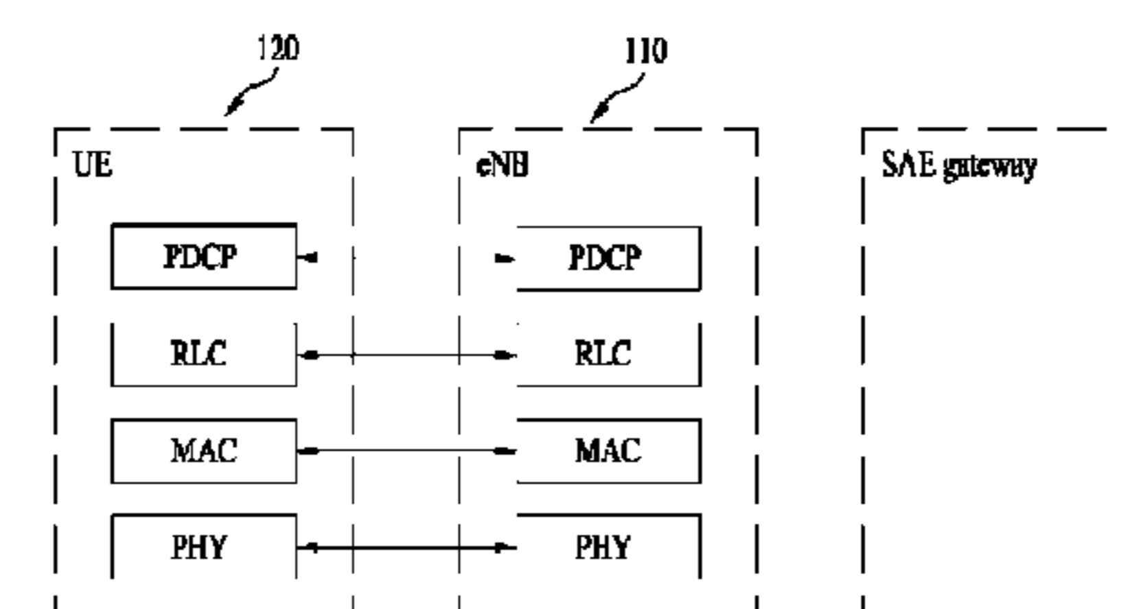
(b) user-plane protocol stack
