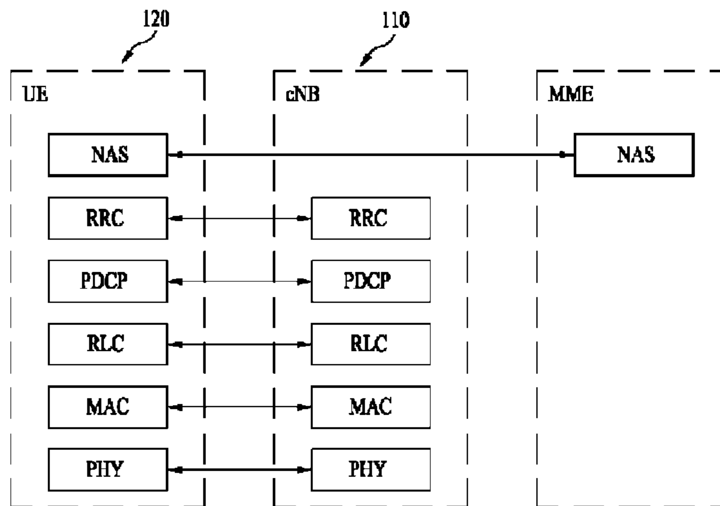
(a) control-plane protocol stack
