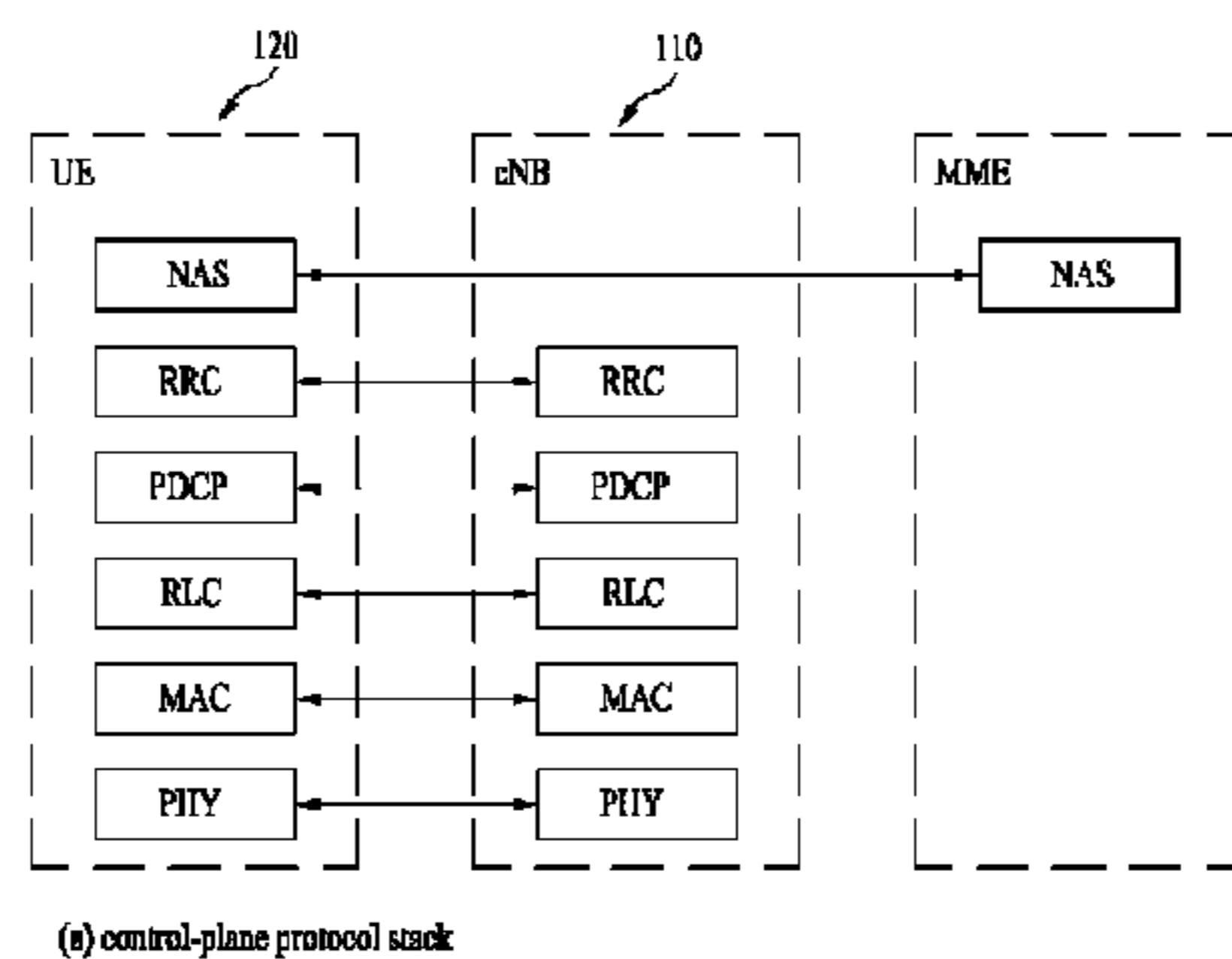
(a) control-plane protocol stack
