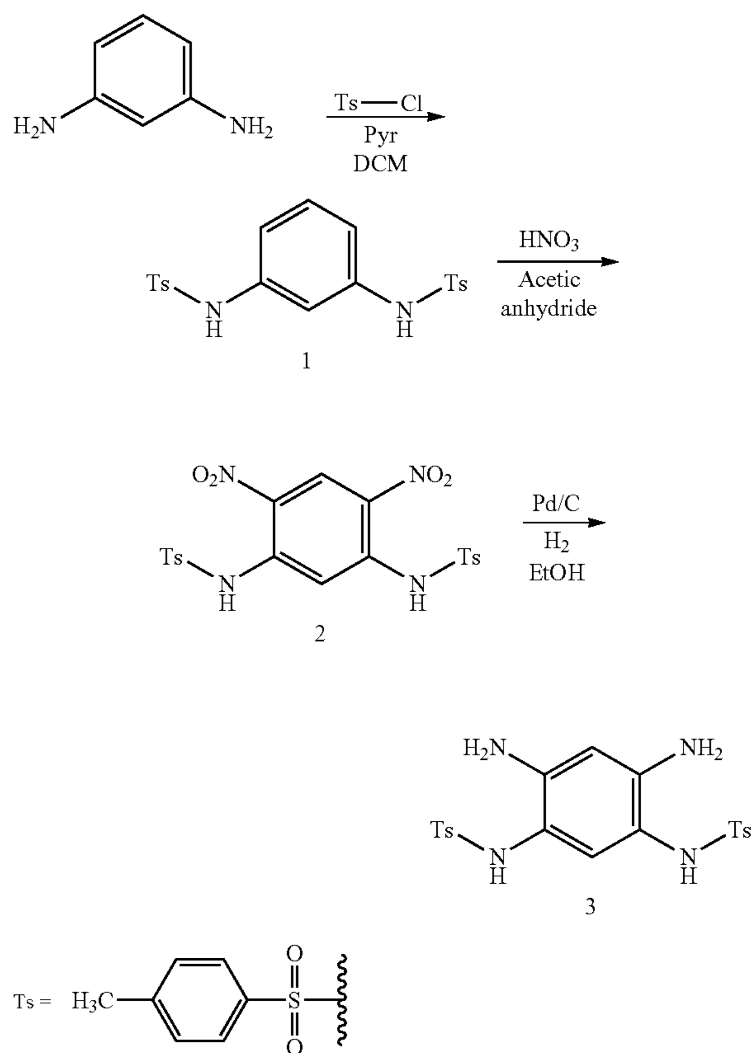
Scheme 1. Synthesis of 1,3-diamino-4,6-bis(p-toluenesulfonamido)benzene.
