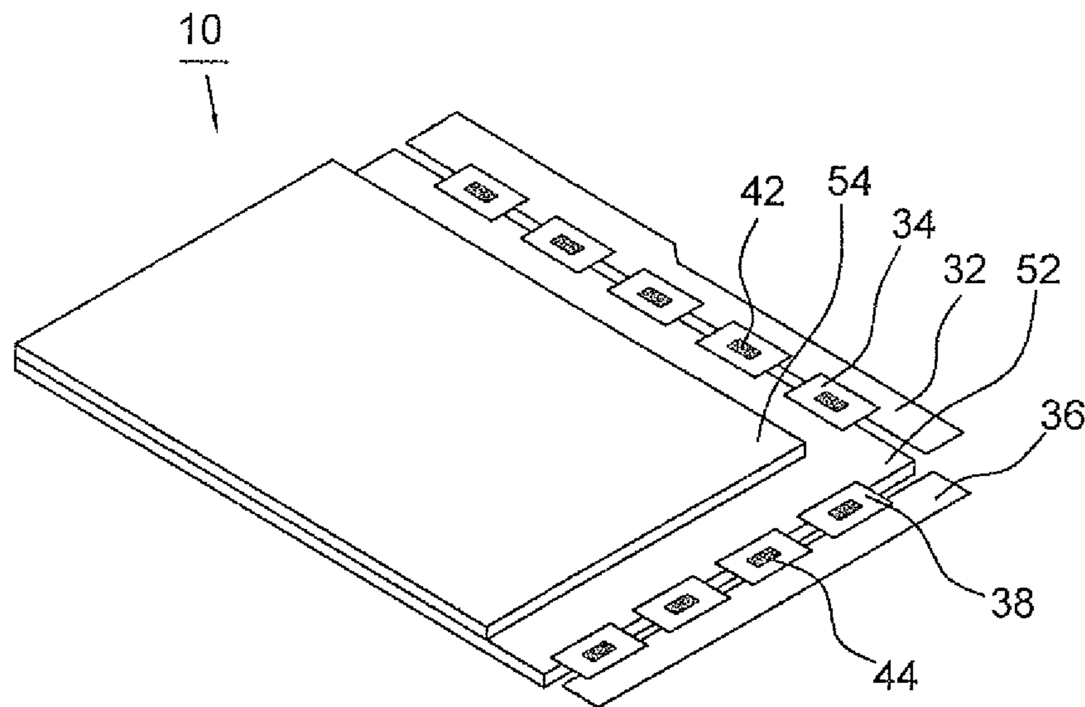
FIG.1 (PRIOR ART)
