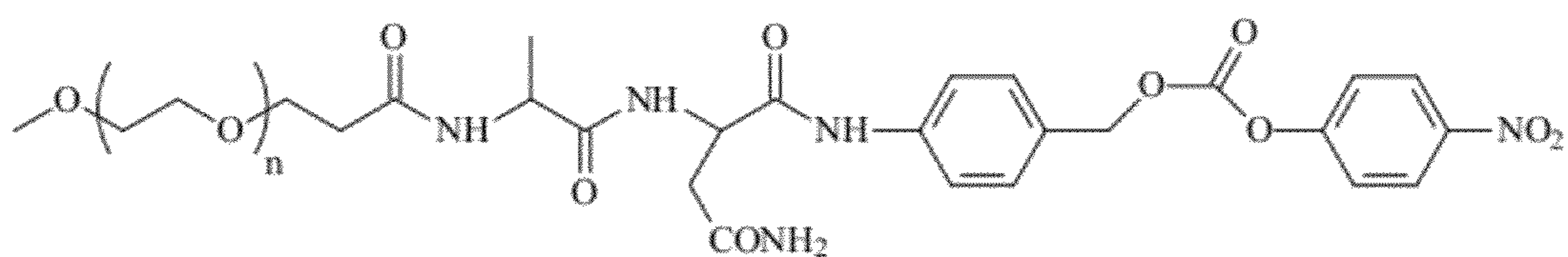
PEG-AlaAsn-PABC-PNP
