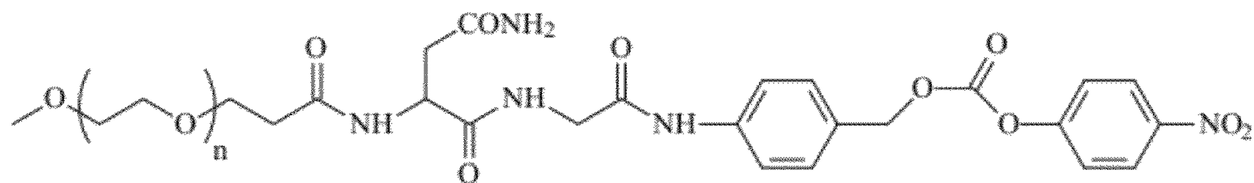
PEG-AsnGly-PABC-PNP
