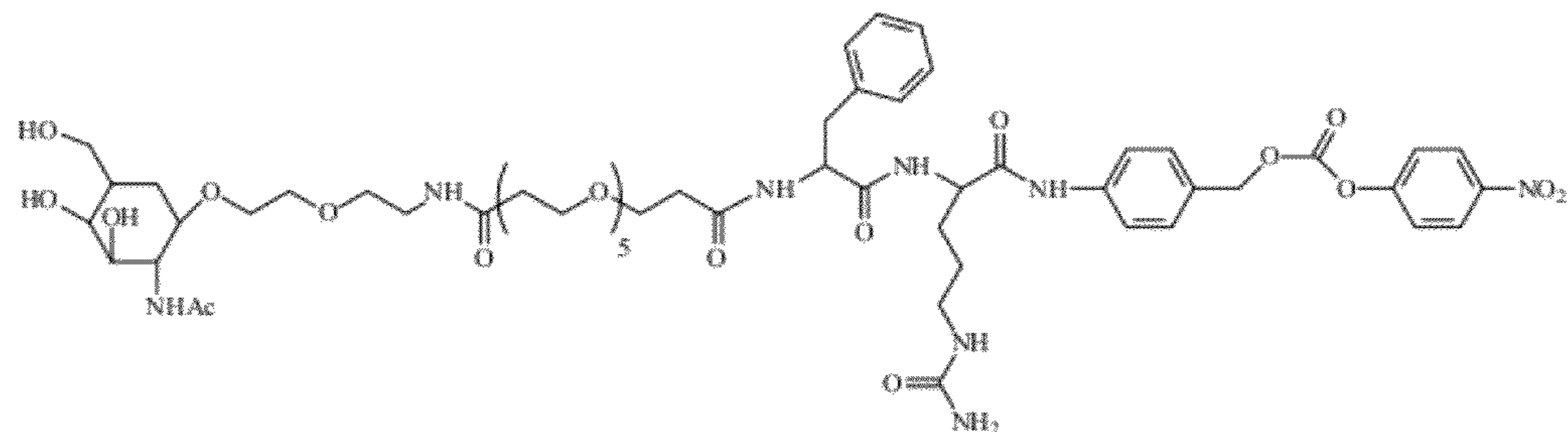
NAG-PEG7-PheCit-PABC-PNP
