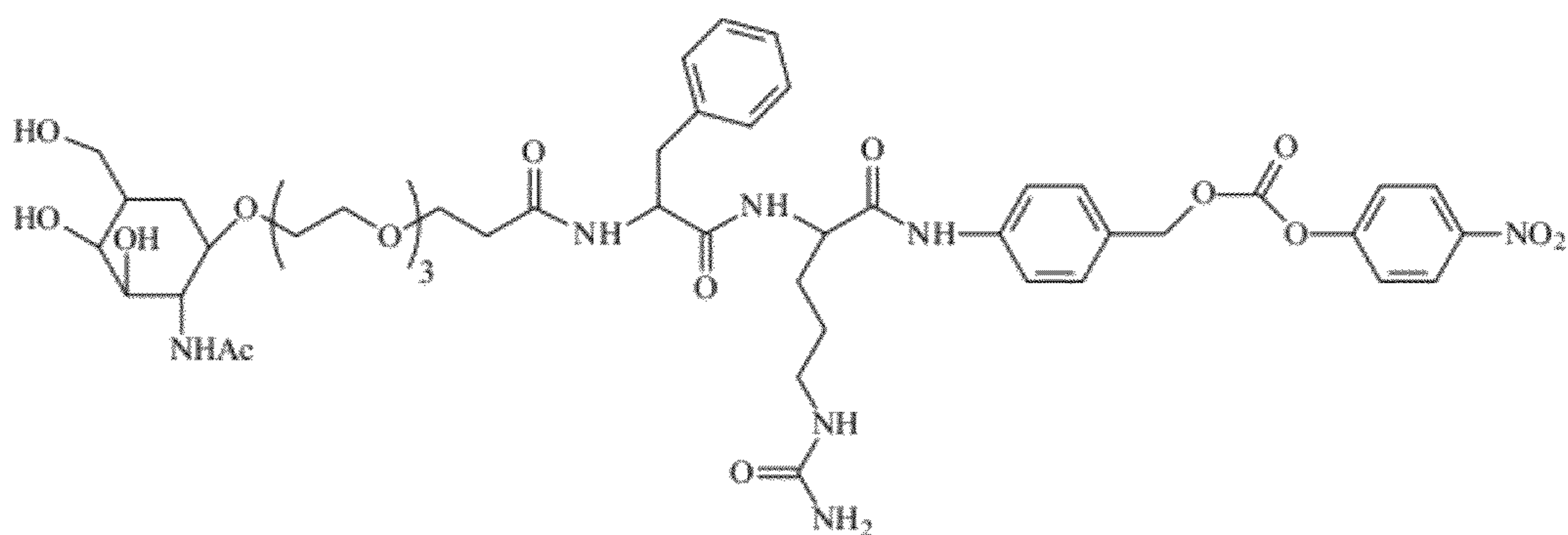
NAG-PEG4-PheCit-PABC-PNP
