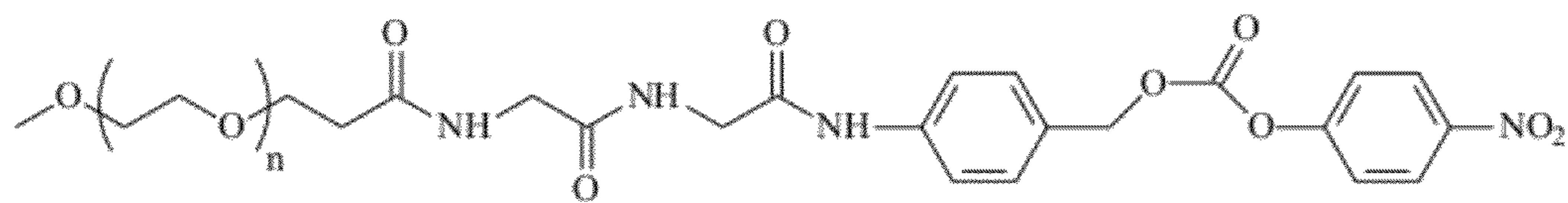
PEG-GlyGly-PABC-PNP
