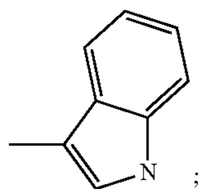
(tryptophan)
