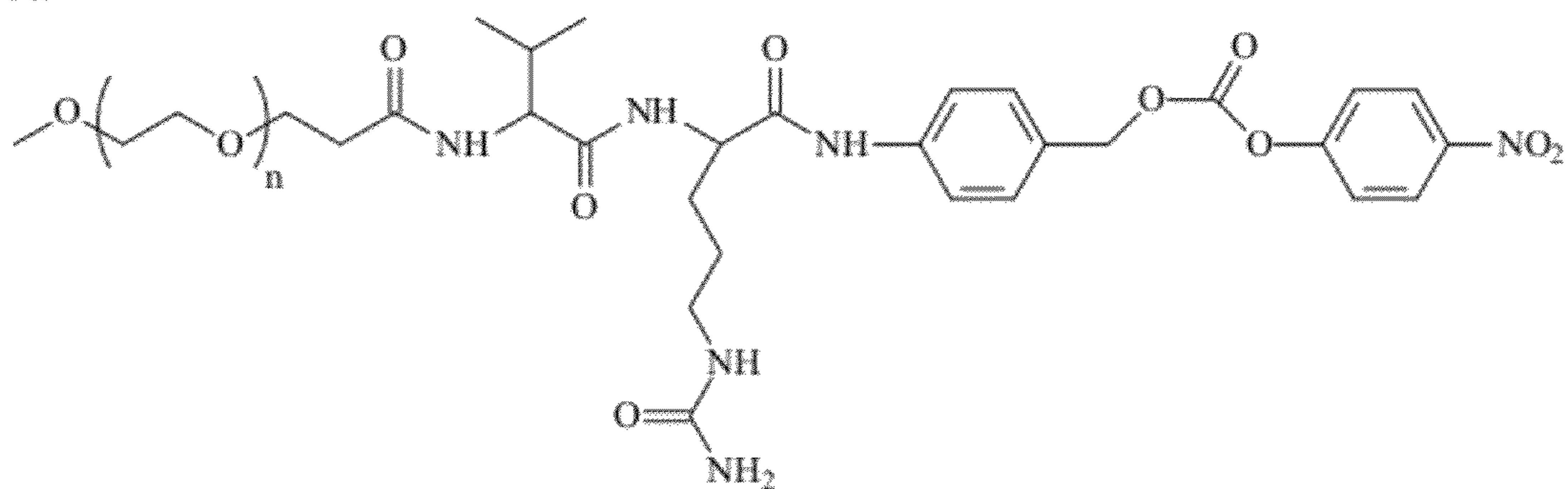
PEG-ValCit-PABC-PNP
