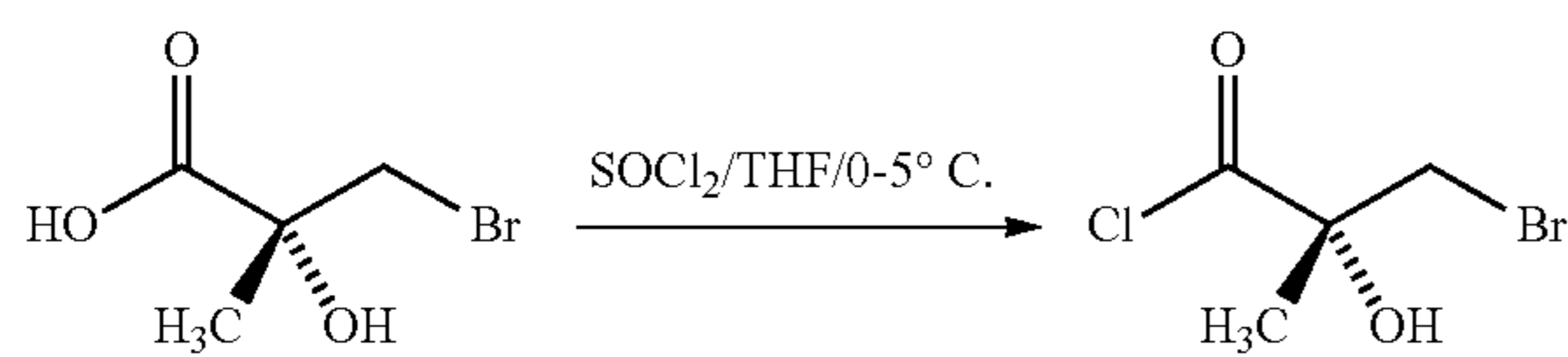
(R)-3-bromo-2-hydroxy-2-methylpropanoic acid
