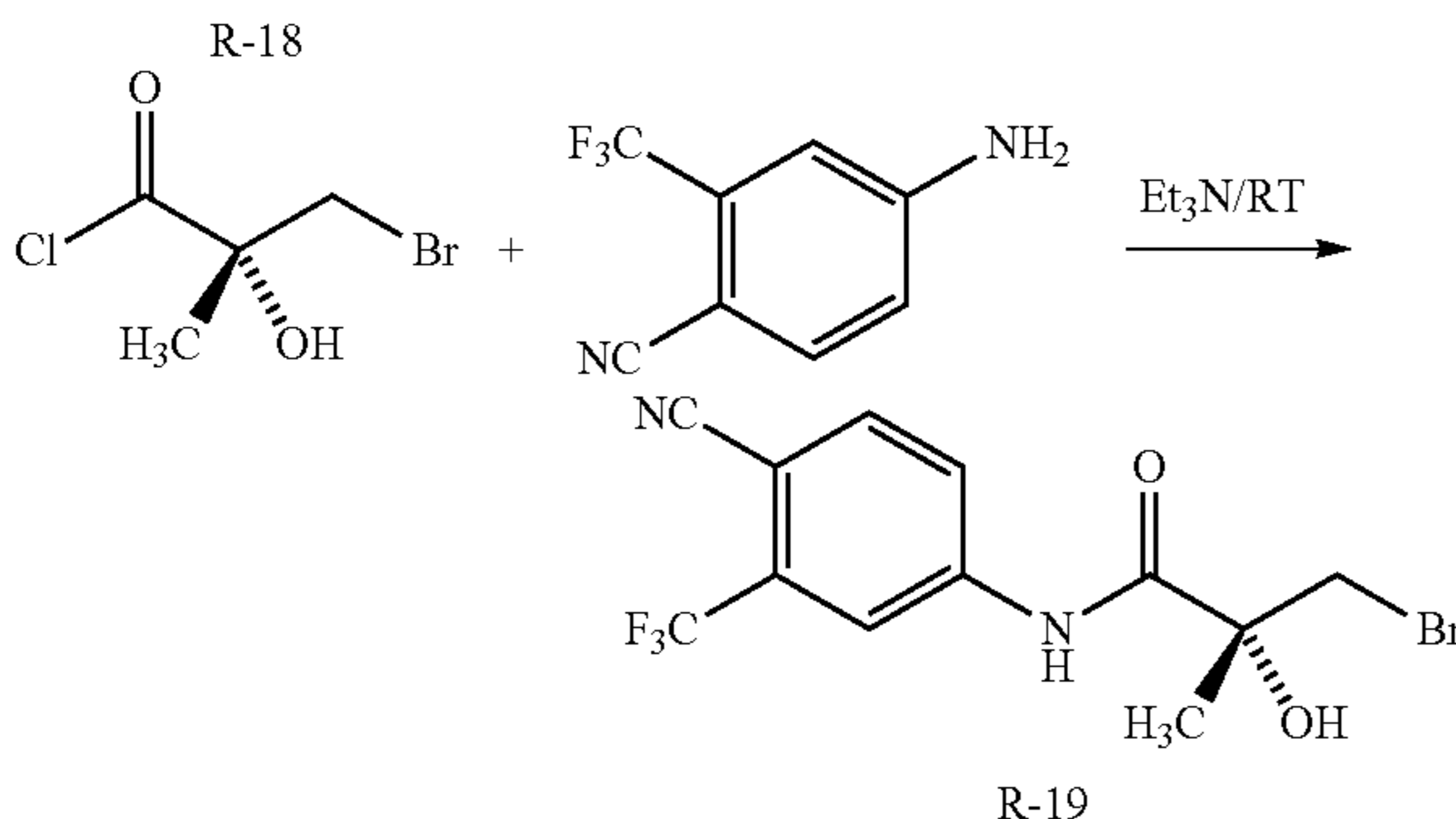
(R)-3-bromo-2-hydroxy-2-methylpropanoic acid
