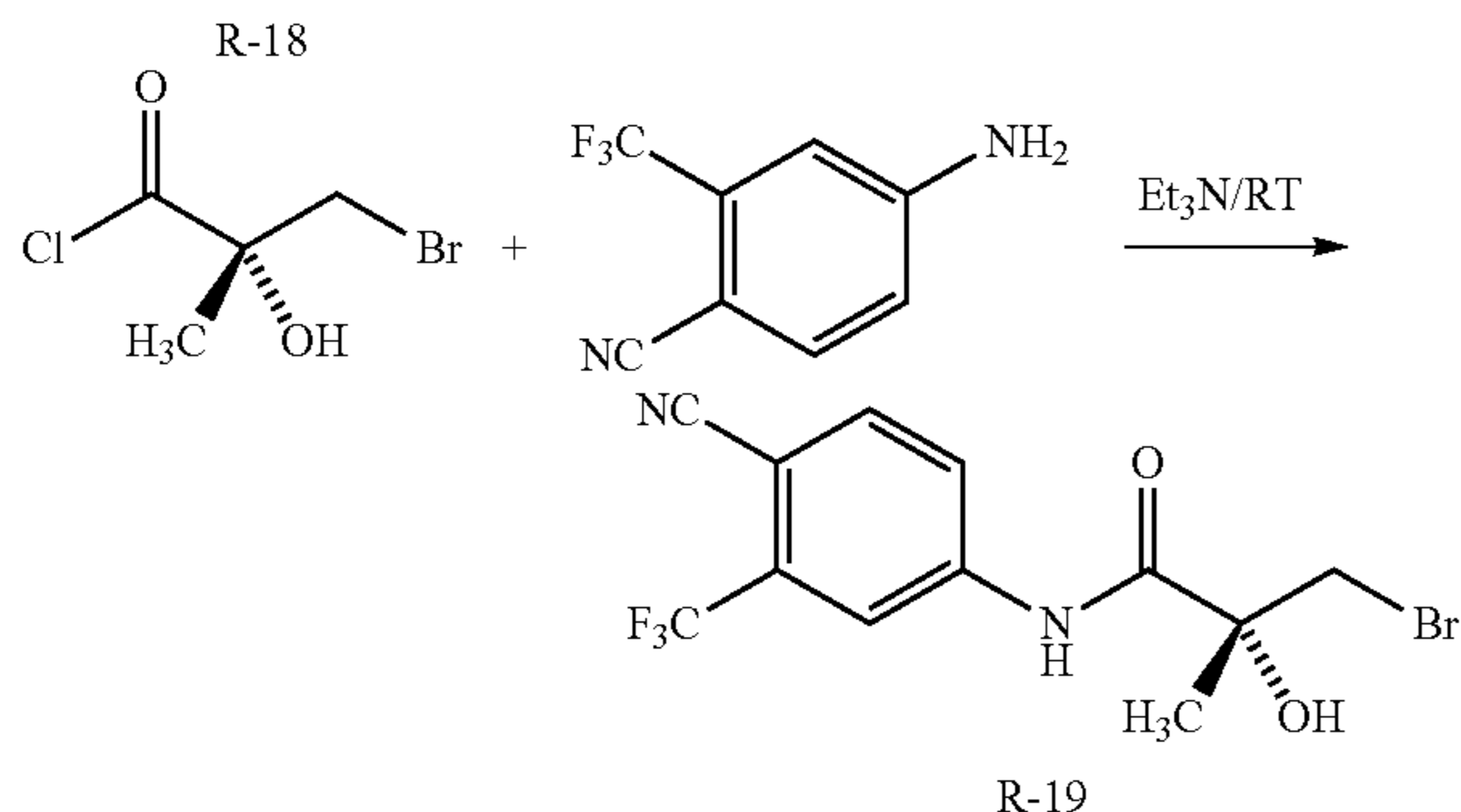
(R)-3-bromo-2-hydroxy-2-methylpropanoic acid
