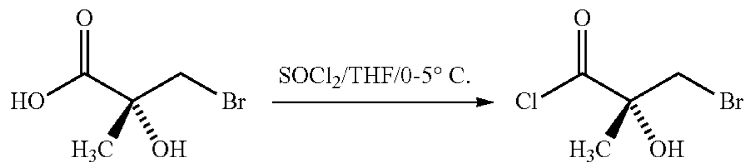
(R)-3-bromo-2-hydroxy-2-methylpropanoic acid
