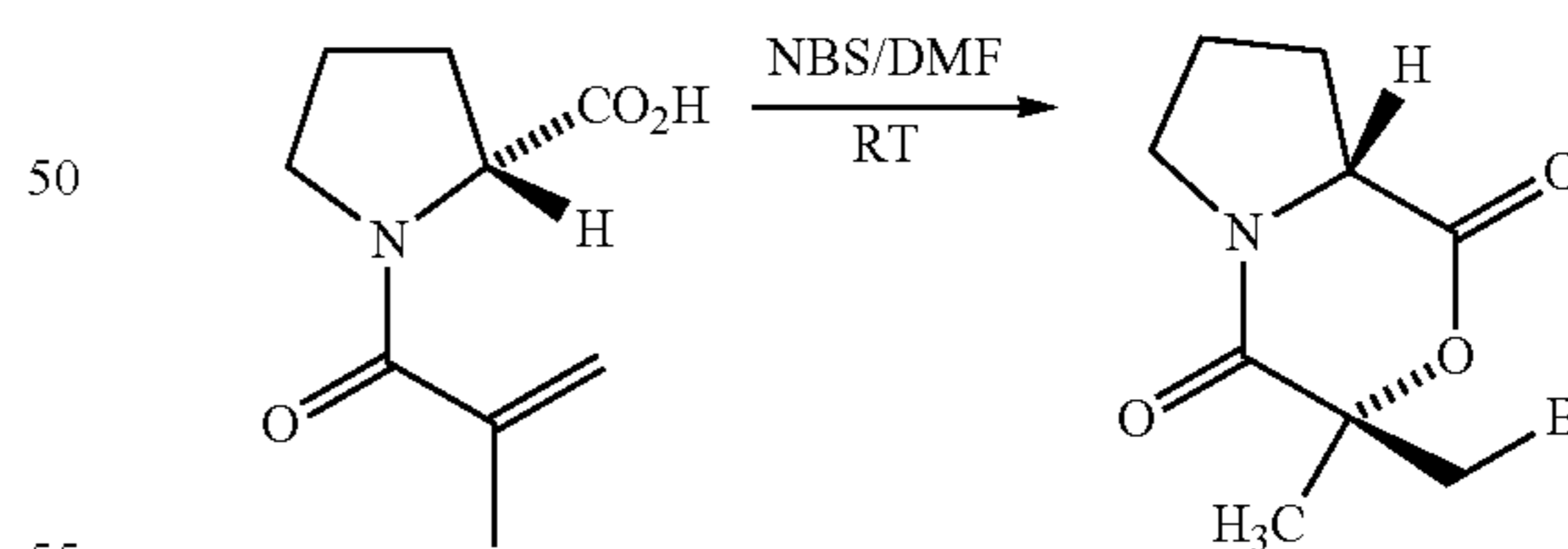
(3R,8aR)-3-Bromomethyl-3-methyl-tetrahydro-pyrrolo[2,1-c][1,4]oxazine-1,4-dione
