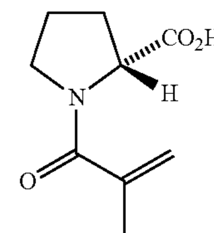
(2R)-1-Methacryloylpyrrolidin-2-carboxylic Acid
