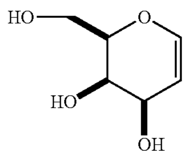
D-Galactal
