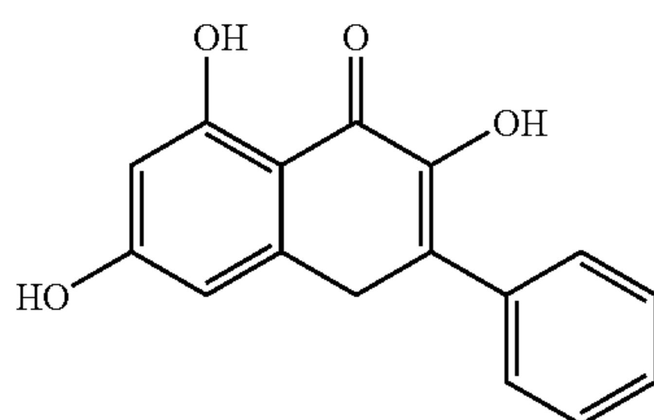
3,5,7-Trihydroxyflavone
