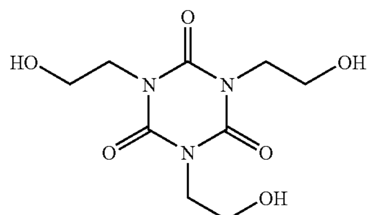
1,3,5-Tris(2-hydroxyethyl)-Cyanuric acid
