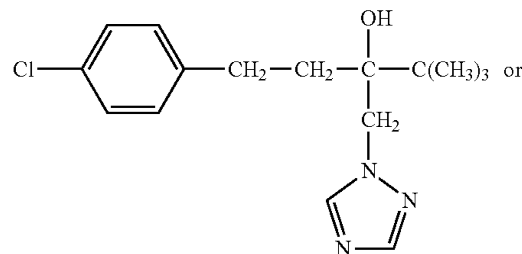
(tebuconazole)
