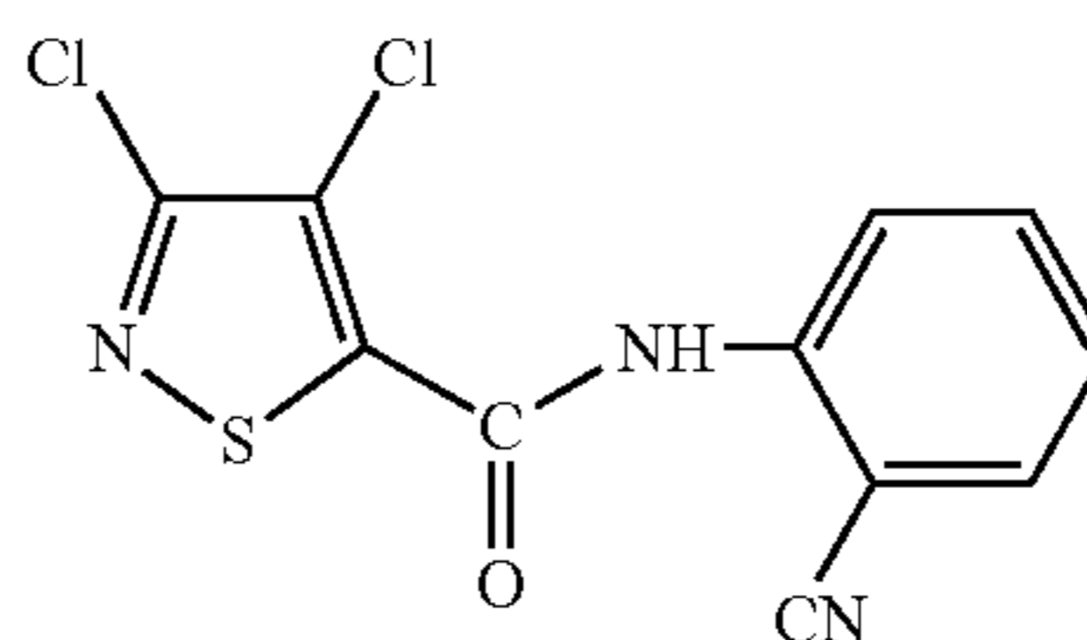
(I)
