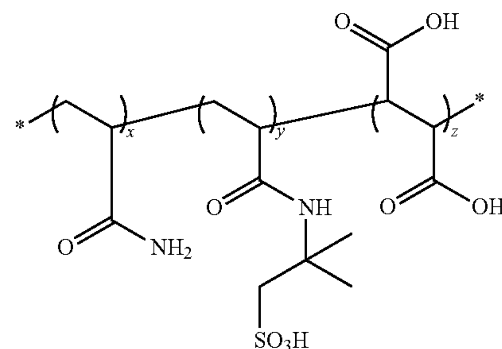
Poly(acrylamide-co-AMPS-co-maleic acid)
