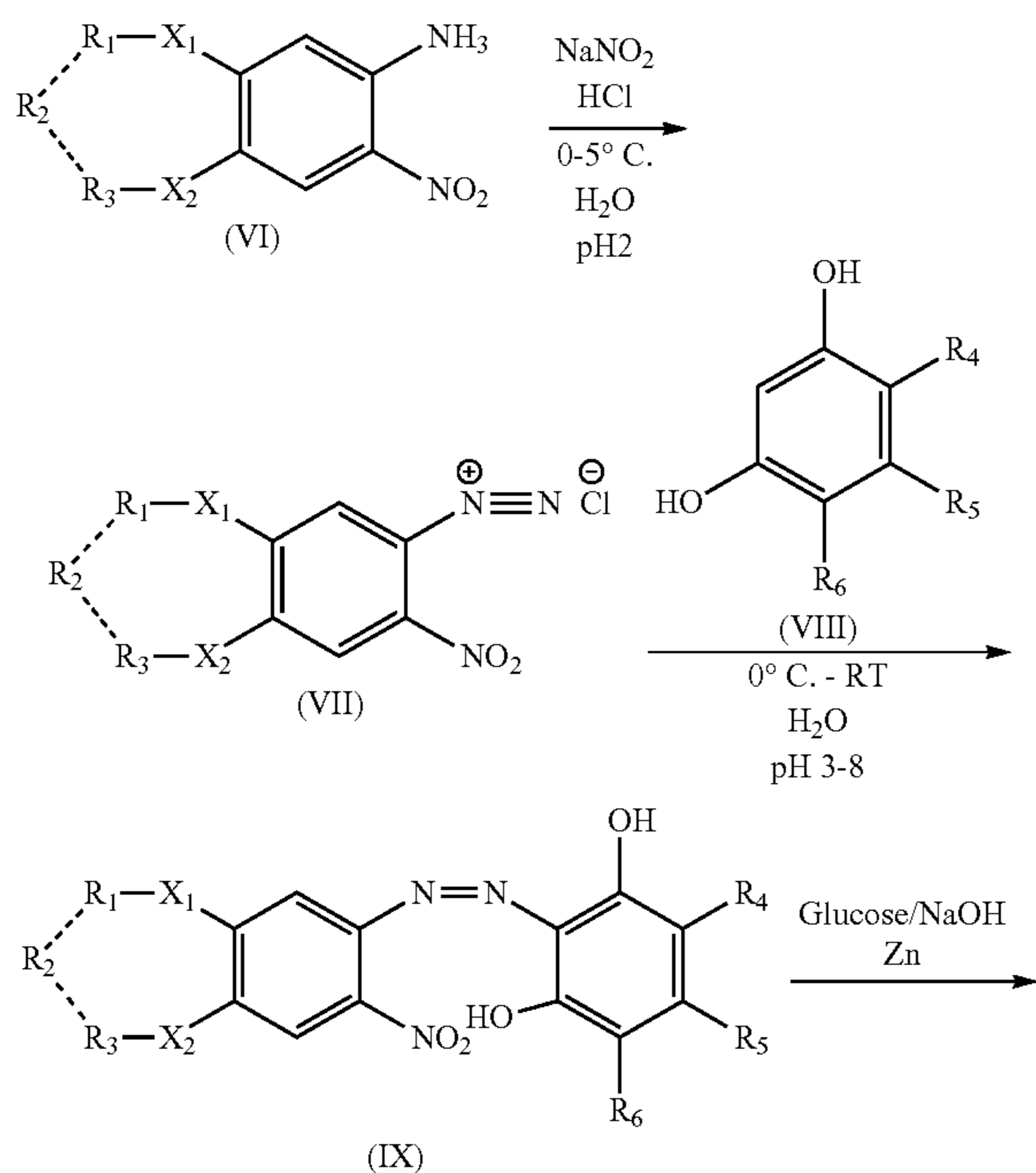
Scheme 1. Generic 2,6-dihydroxyphenyl-2H-benzotriazole synthesis
