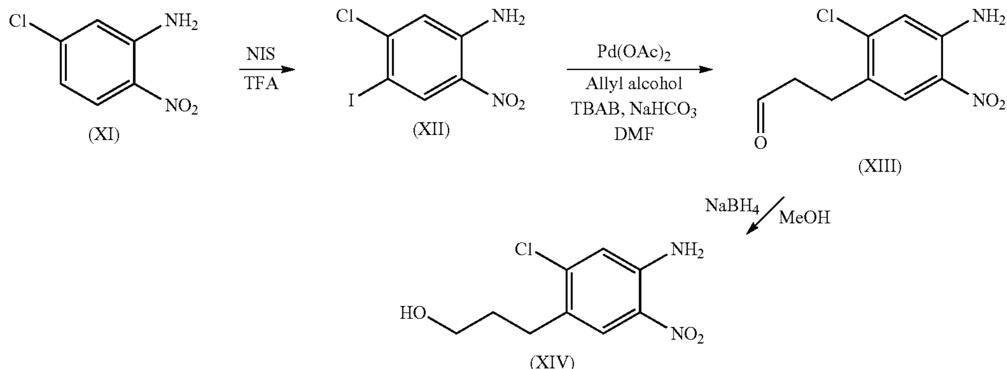
Scheme 2. Specific synthetic pathway to prepare 4-(3-hydroxypropyl)-5-chloro-2-nitroaniline starting material (XIV)
