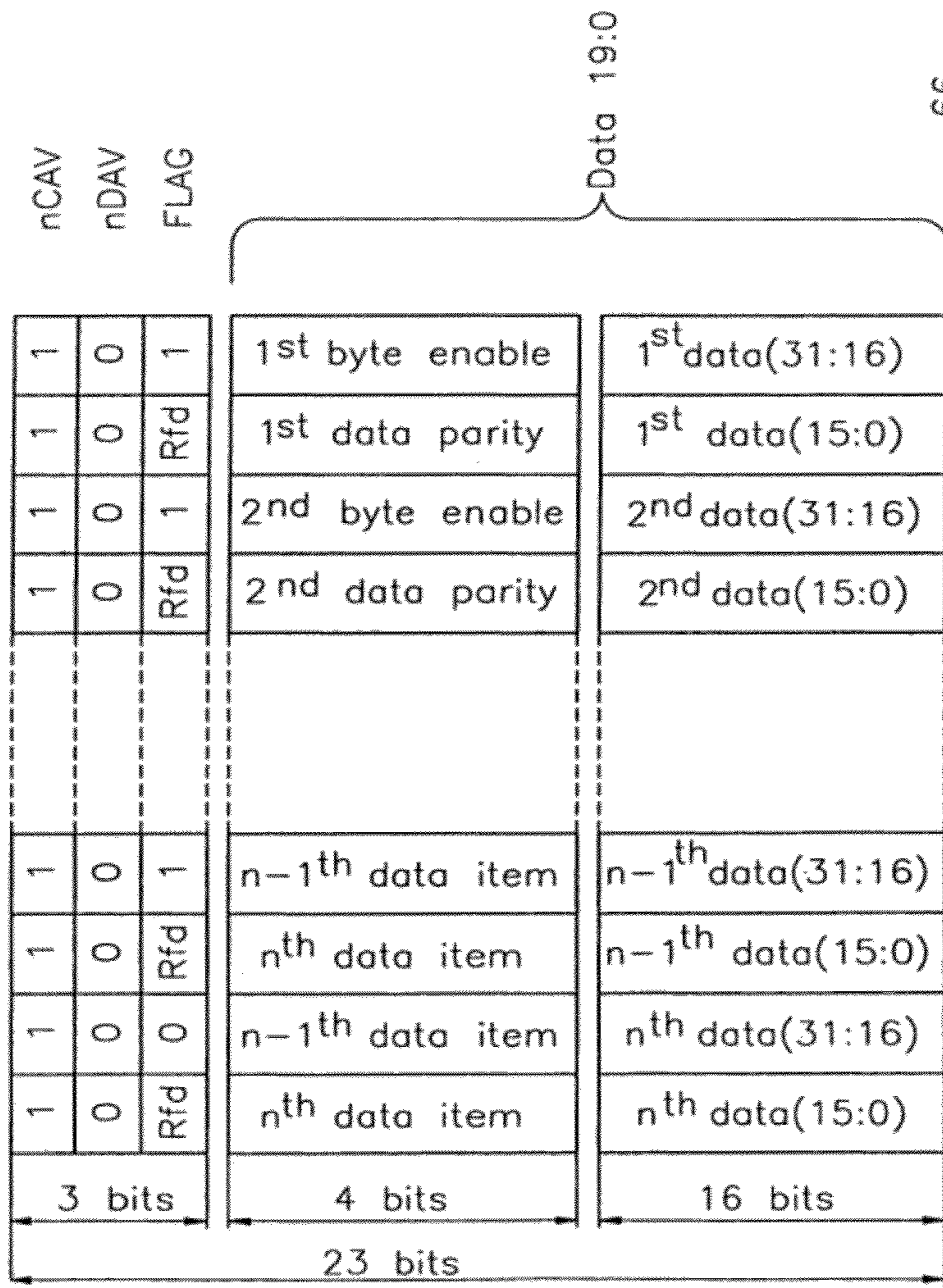
Example implementation showing: i960-style burst local bus protocol carried on HP-GLINK physical layer
