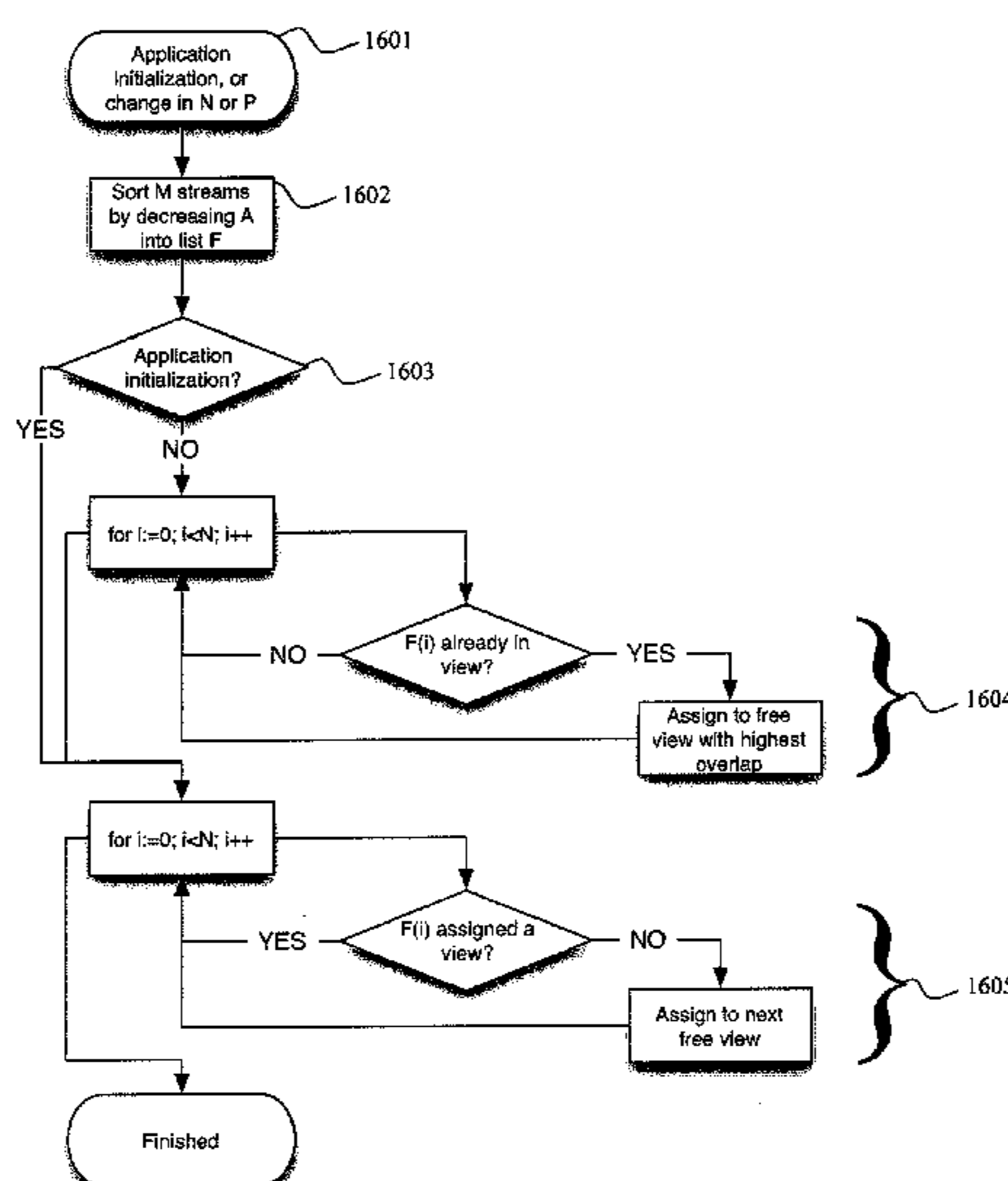
Block diagram of view allocation process – layout initialization
