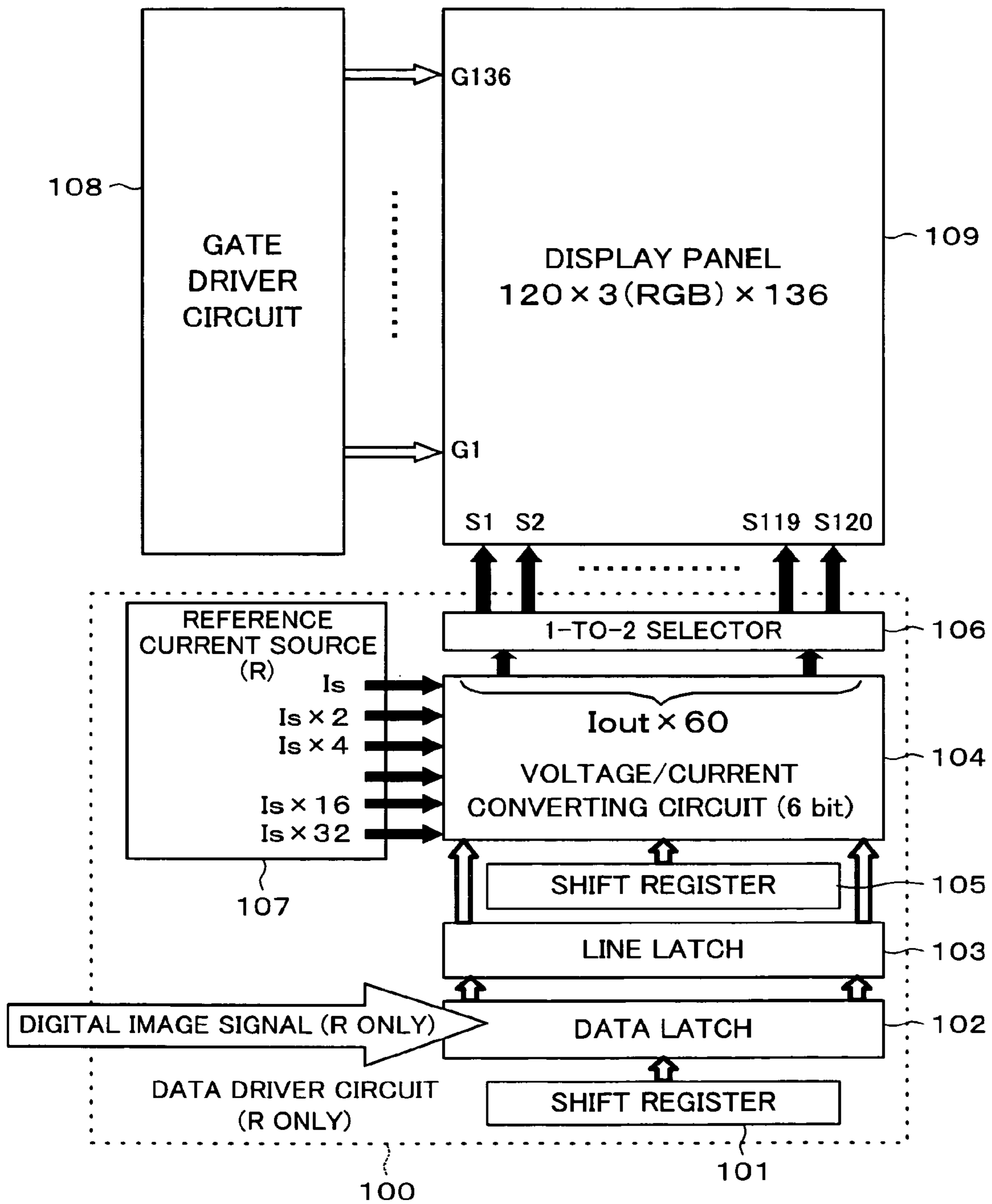
FIG. 19 (PRIOR ART)
