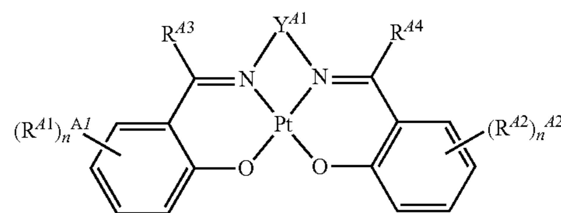
Formula (A)
