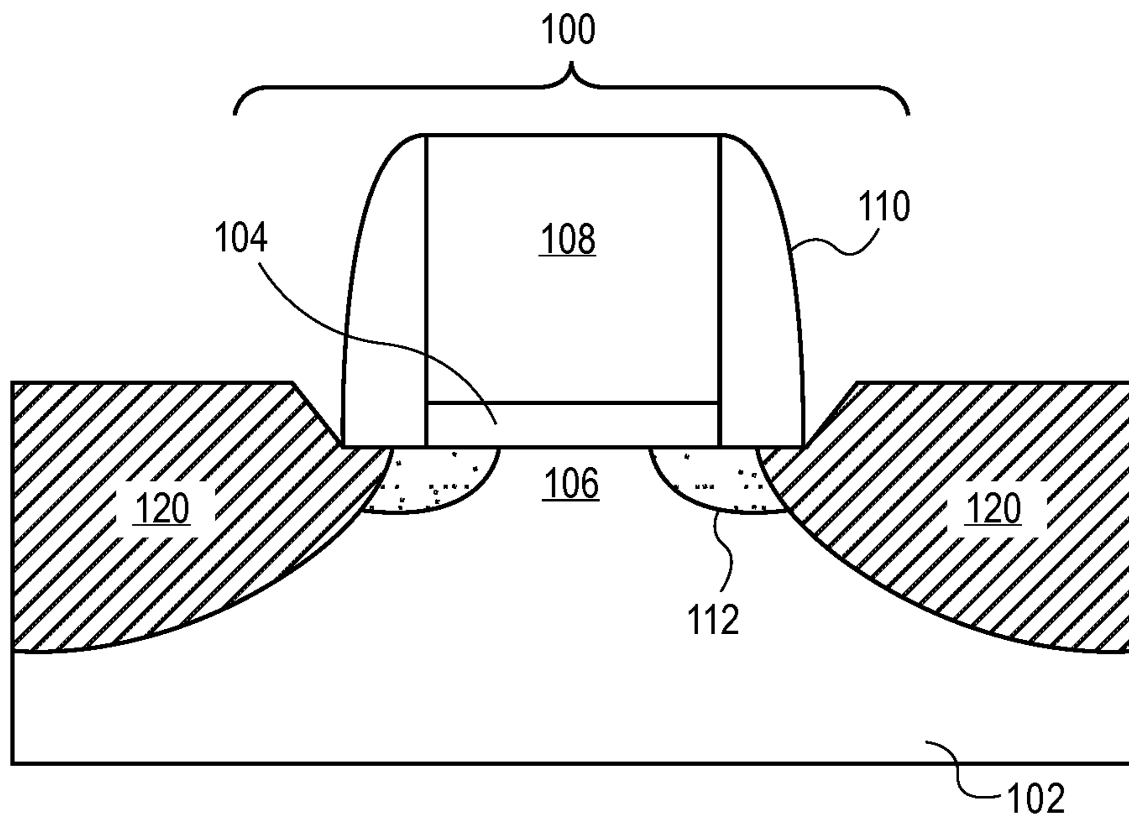
FIG. 1 (PRIOR ART)
