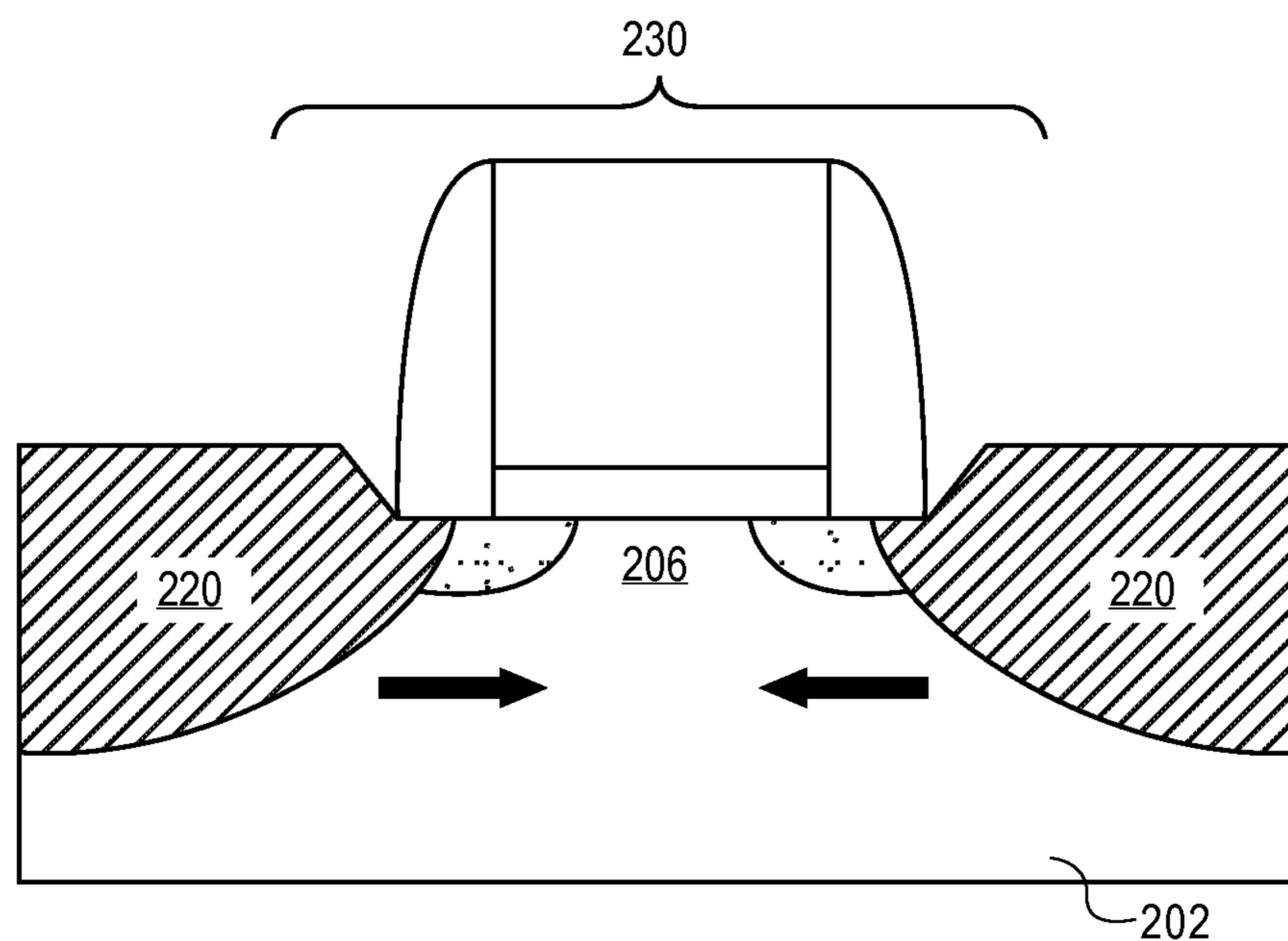
FIG. 2C (PRIOR ART)
