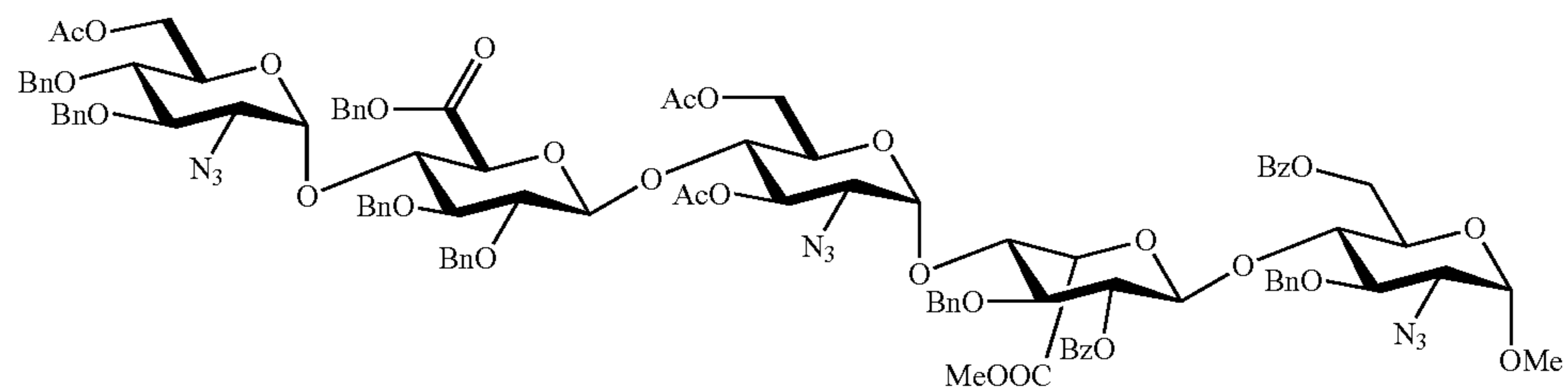
EDCBA Pentamer-CB \text{C}_{101}\text{H}_{105}\text{N}_9\text{O}_{30} Mol. Wt.: 1924.96
