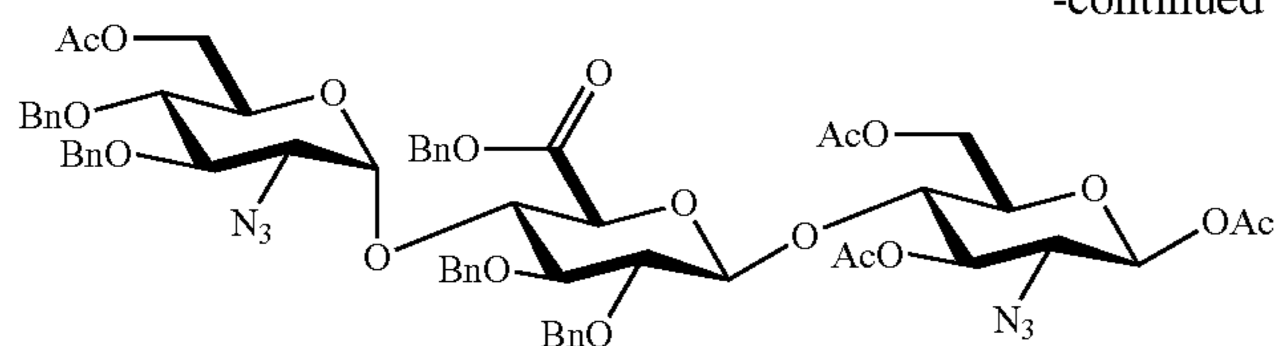
EDC-1-CB C_{59}H_{66}N_6O_{21} Mol. Wt.: 1195.18
