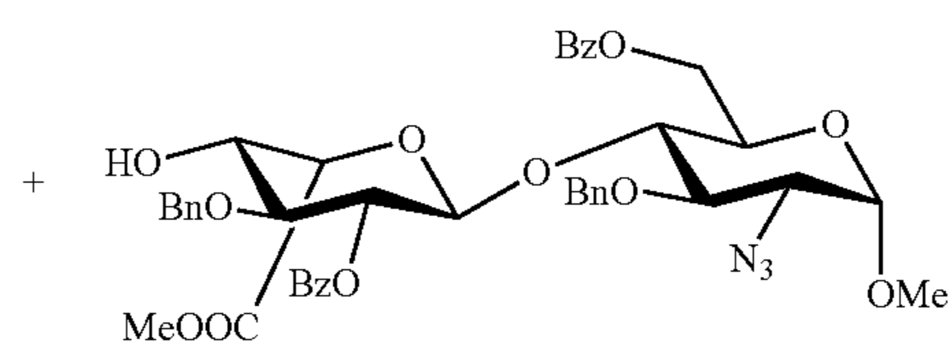
BA Dimer C_{42}H_{43}N_3O_{13} Mol. Wt.: 797.80
