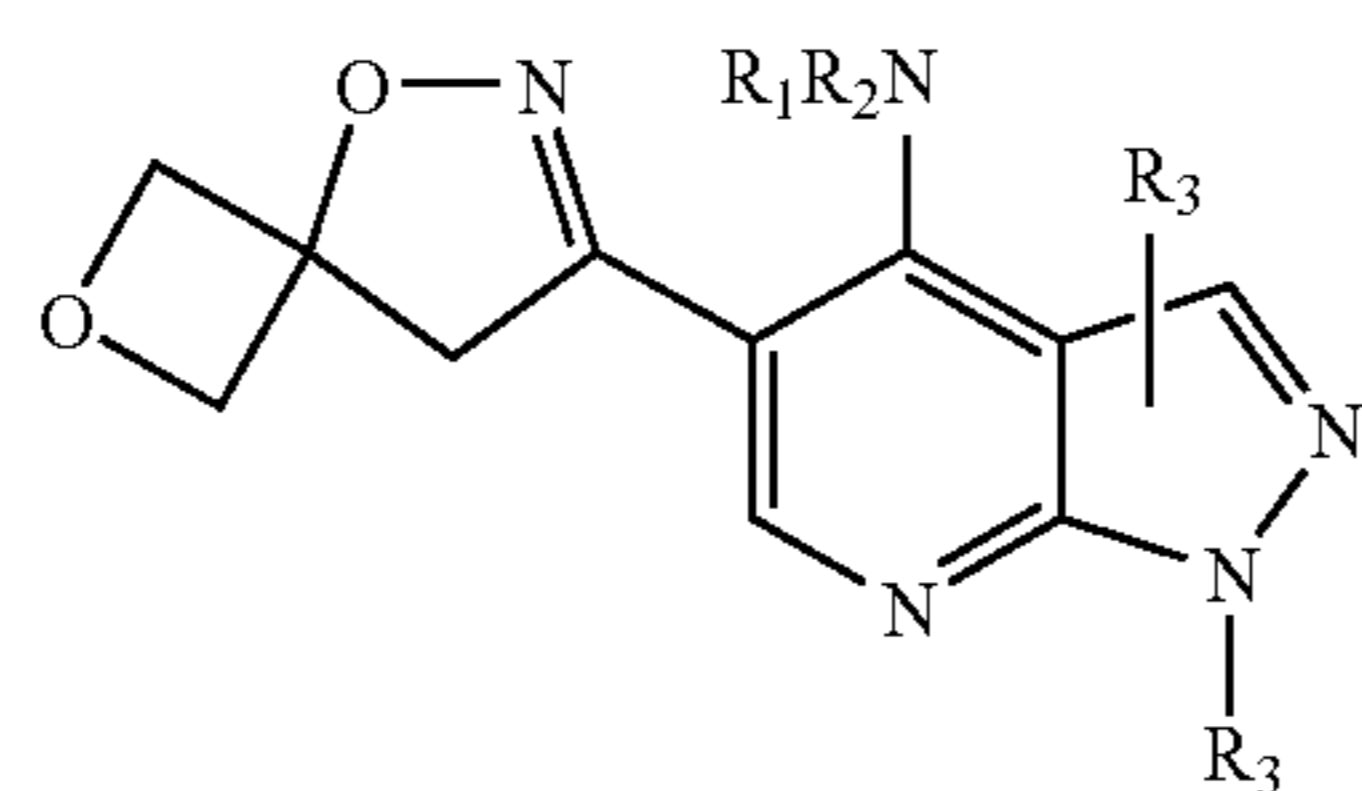
Formula XXVII
