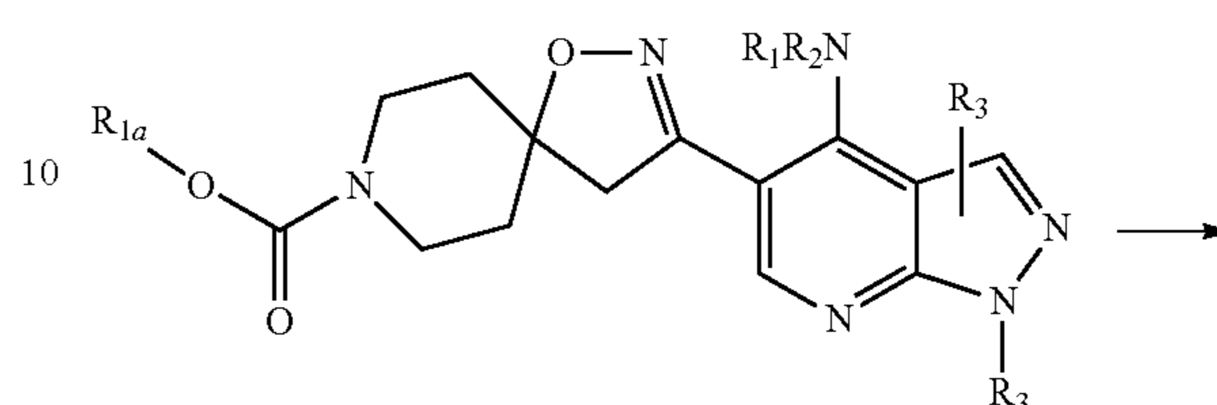
Formula XXVIII
