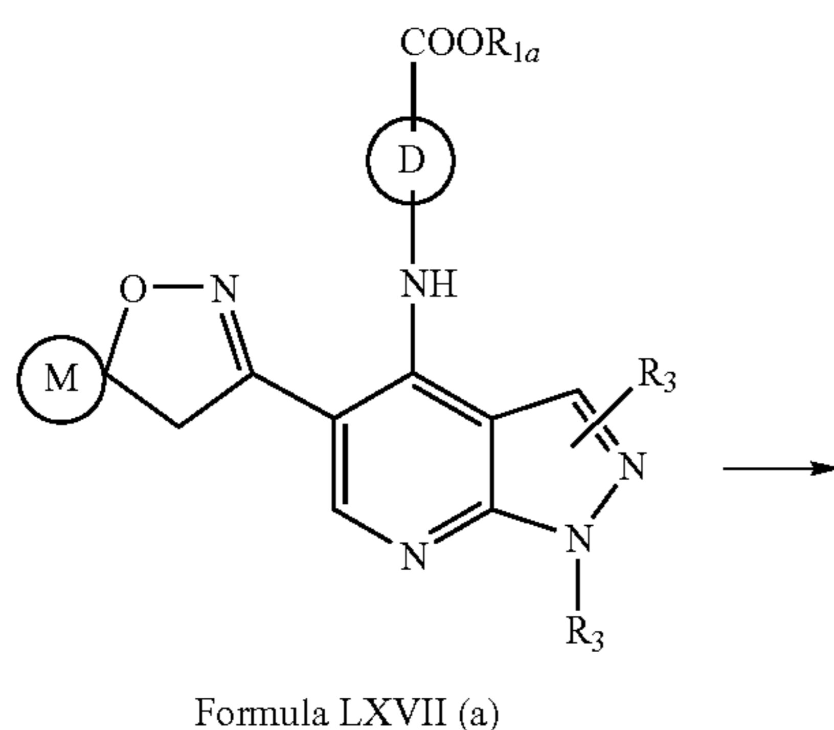
Scheme XII
