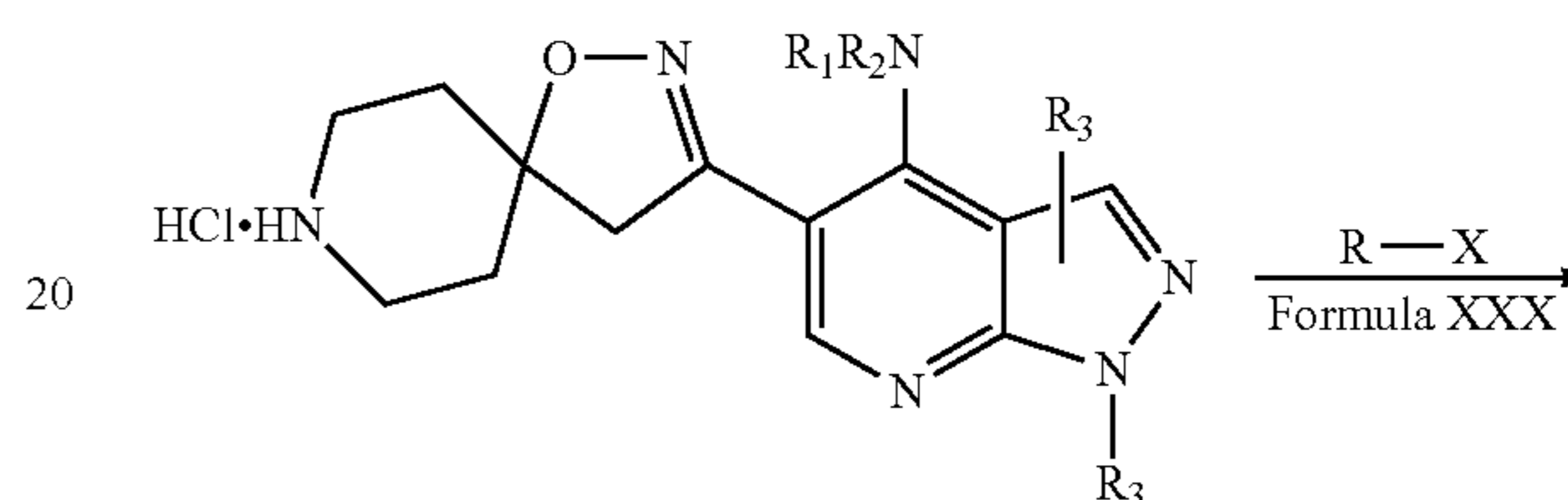
Formula XXIX
