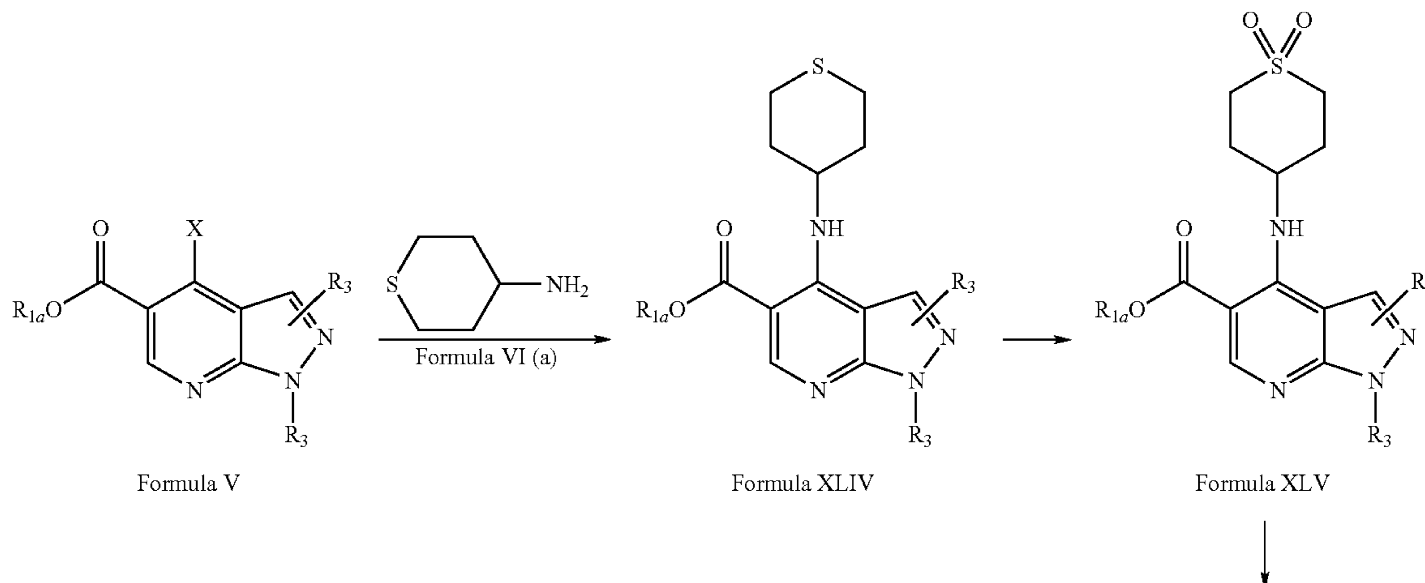
Scheme X
