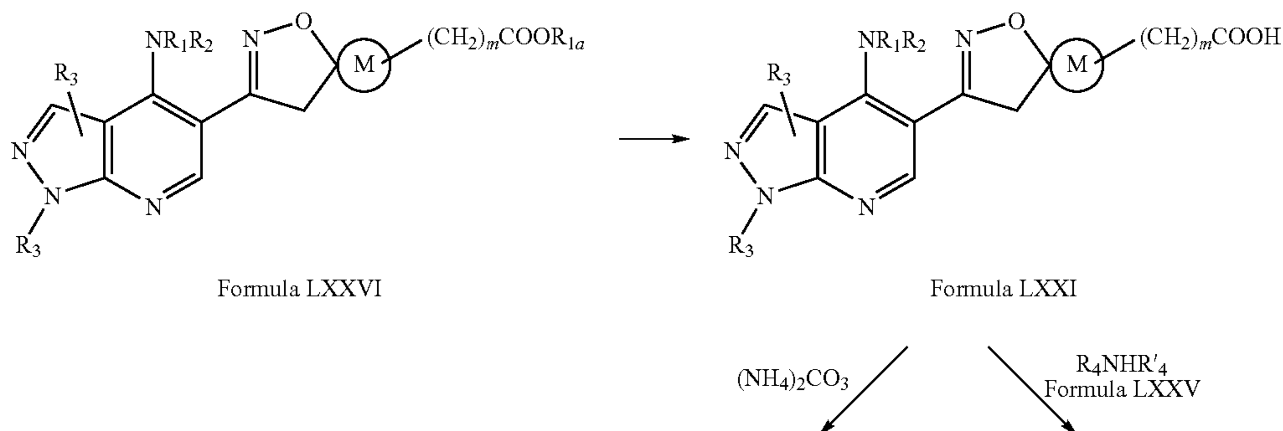
Scheme XIV
