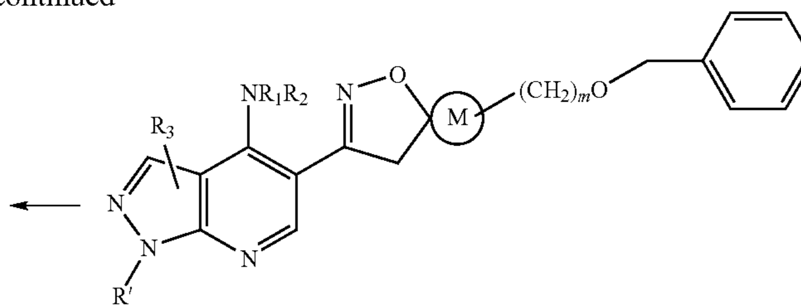
Formula XLII
