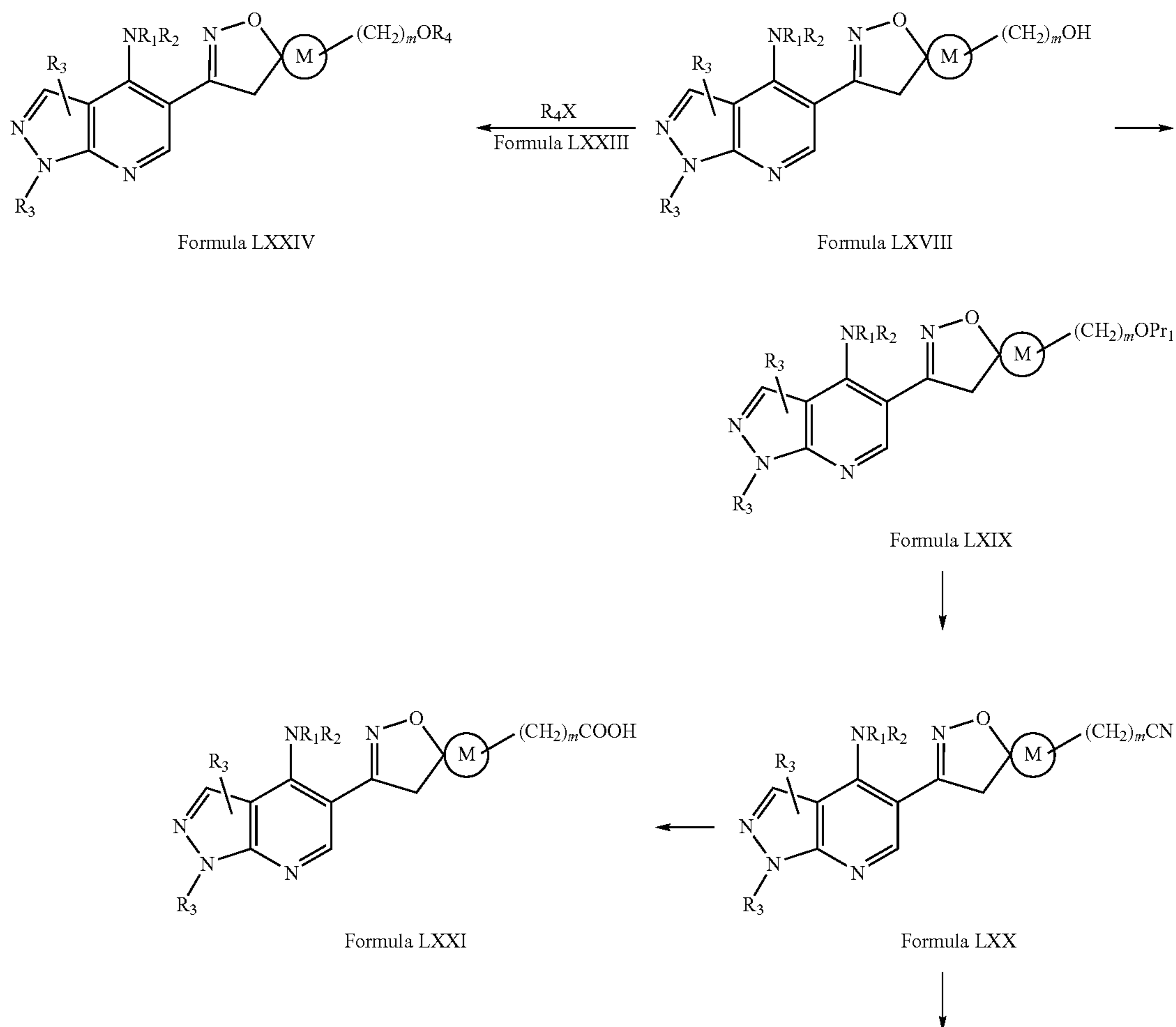
Scheme XIII
