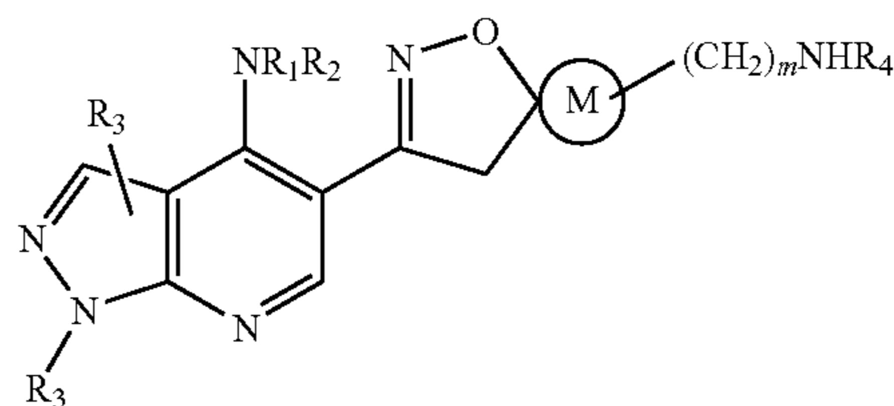
Formula LXXXI
