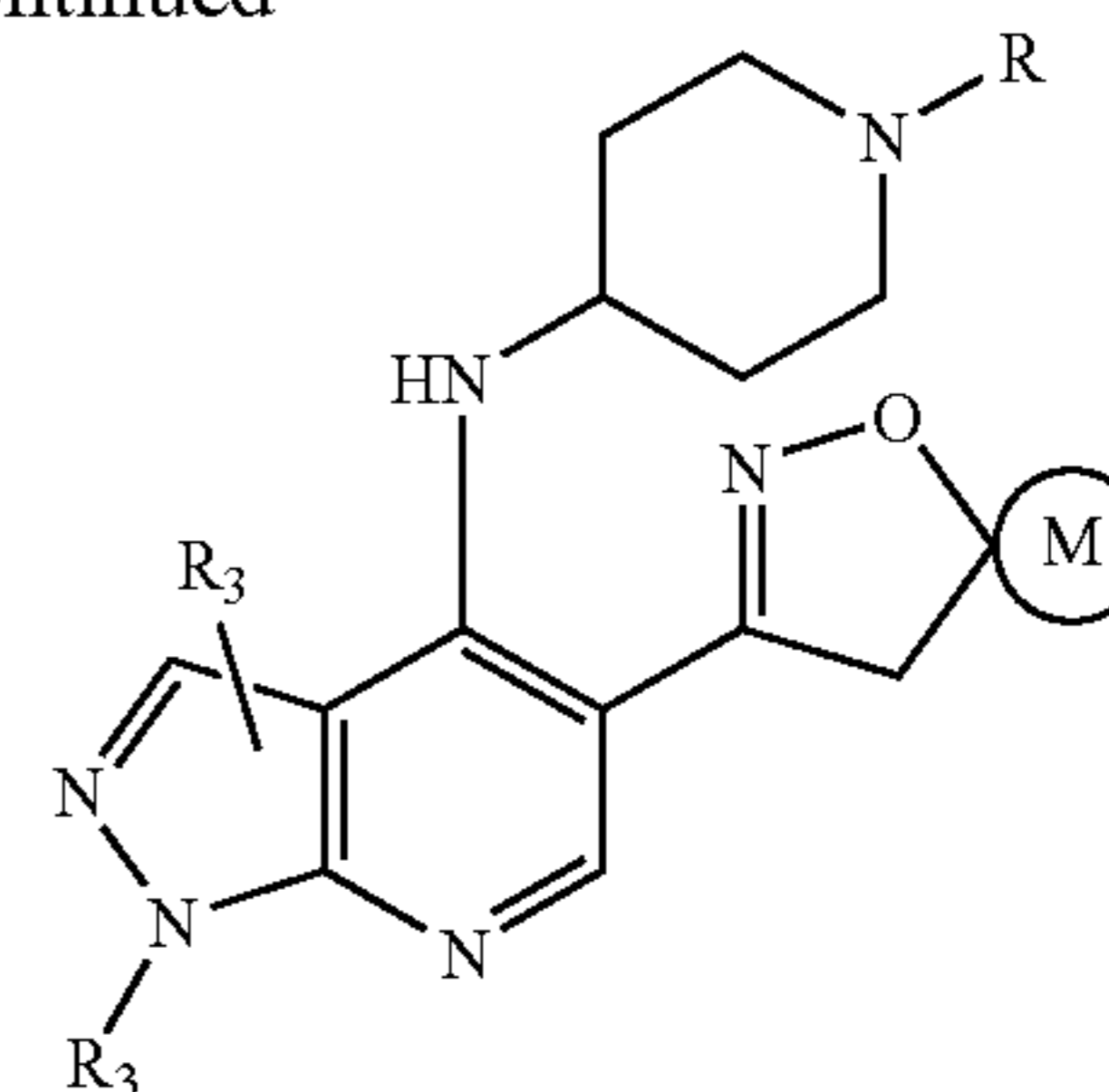
Formula XXXIX
