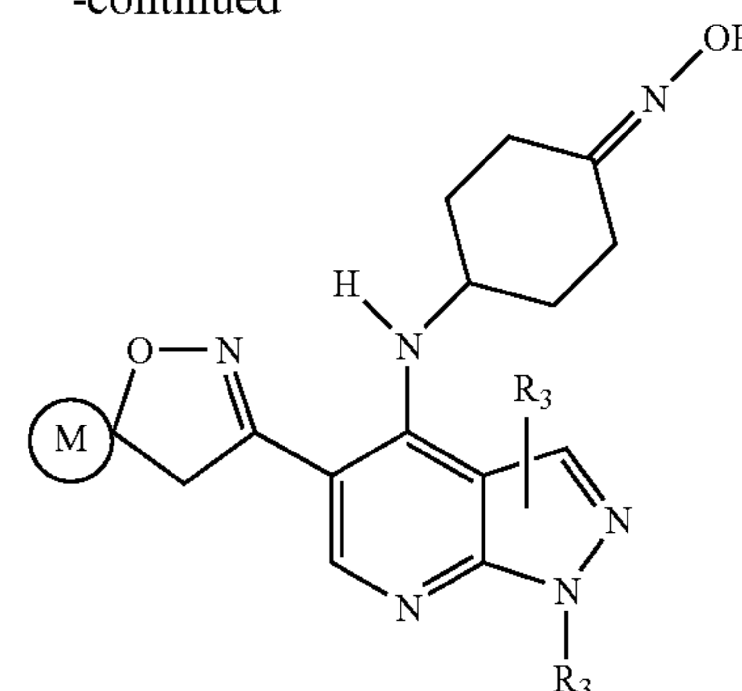
Formula XXIII
