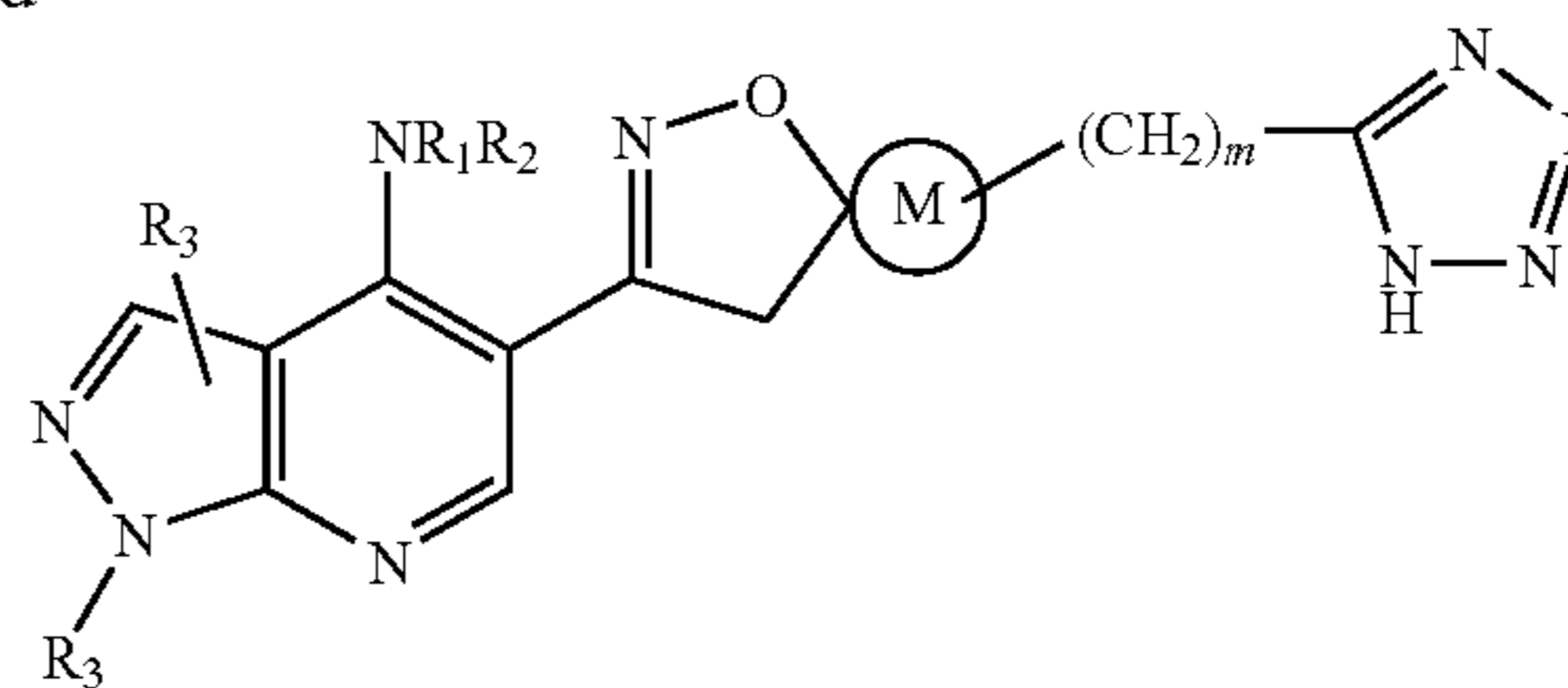
Formula LXXII
