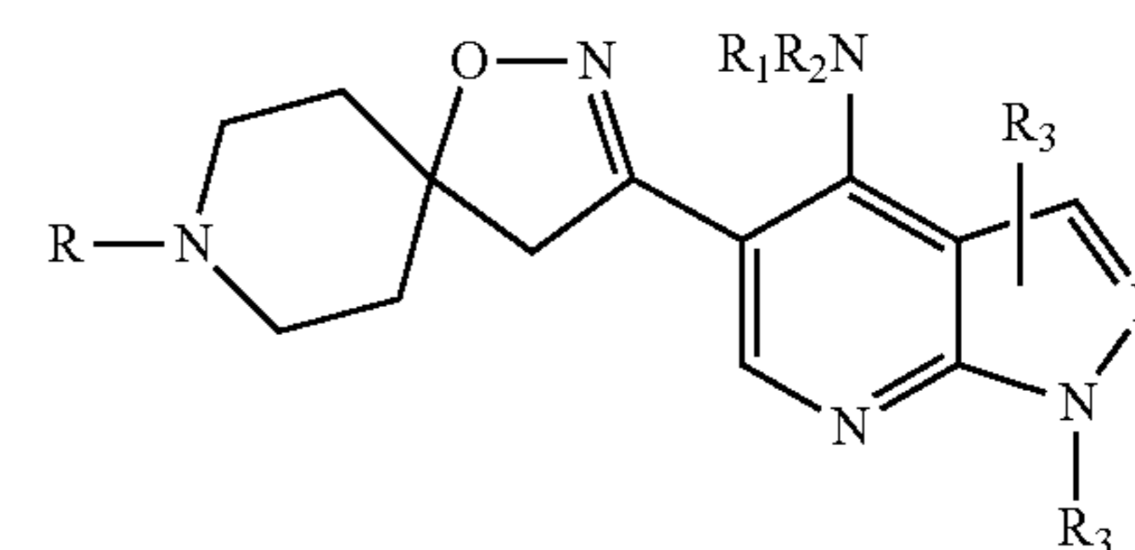
Formula XXXI
