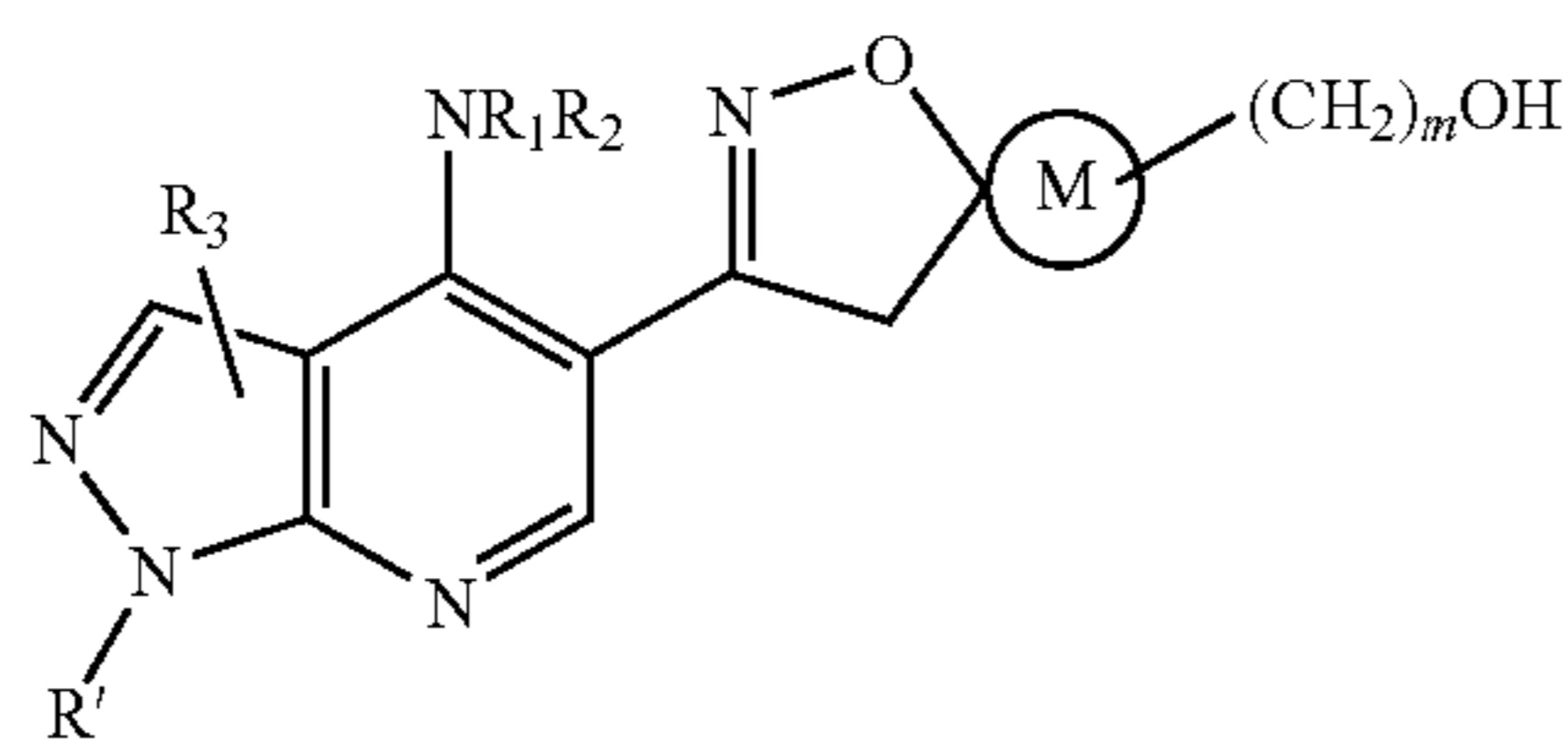
Formula XLIII
