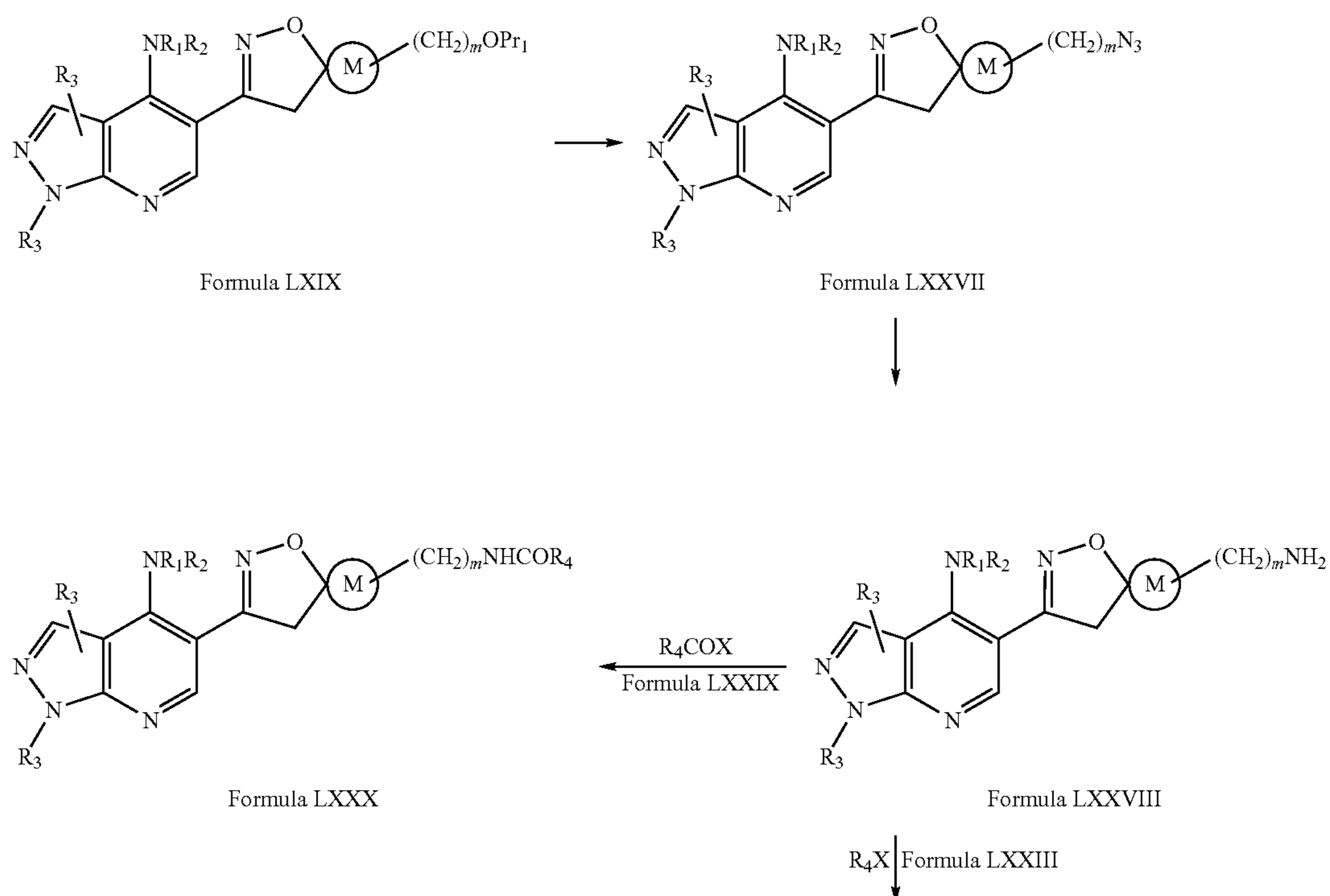
Scheme XV
