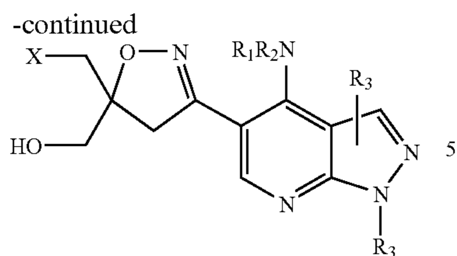
Formula XXVI
