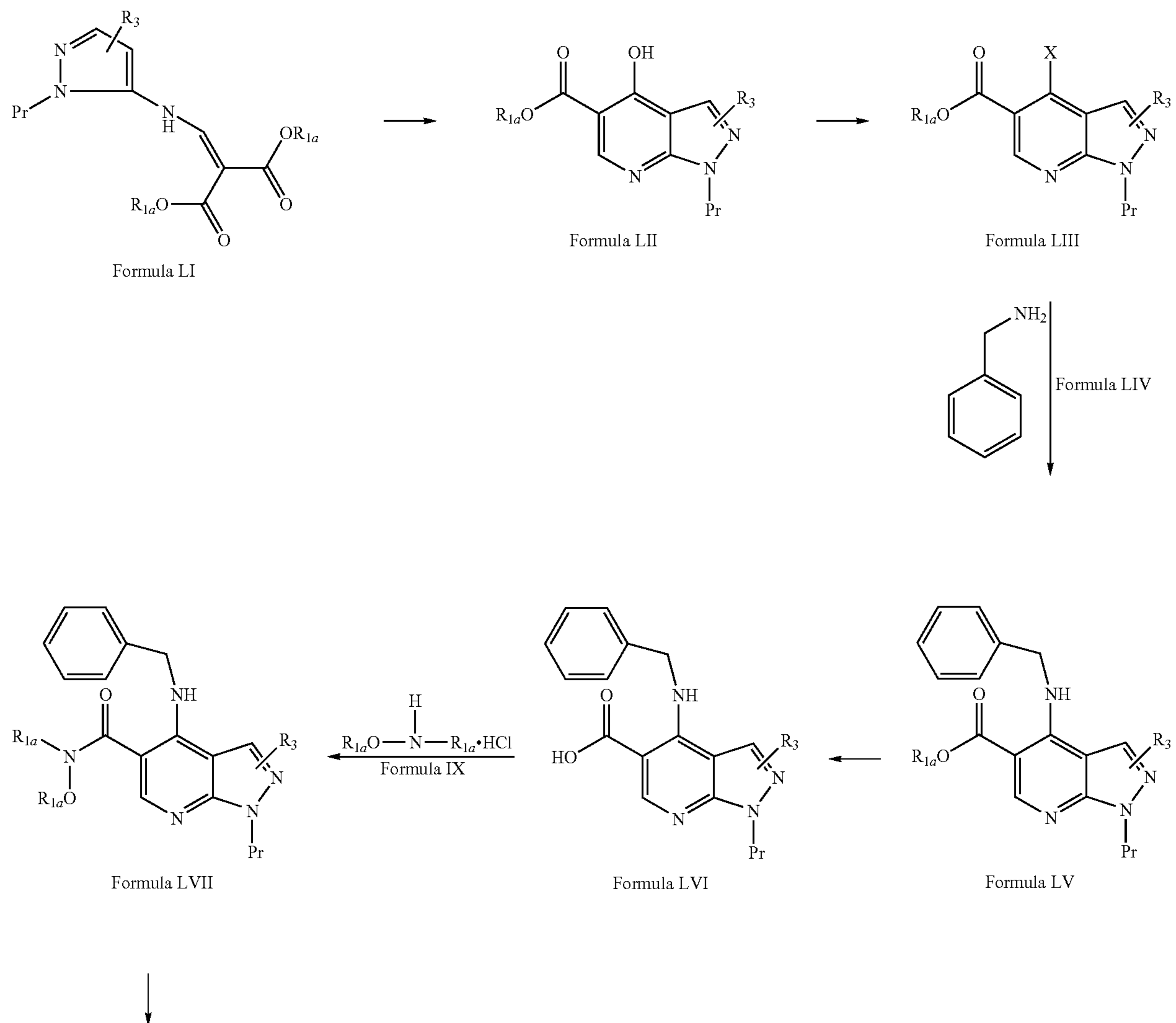
Scheme XI
