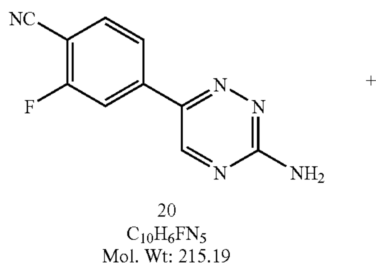
Scheme 5 (Example 26)
