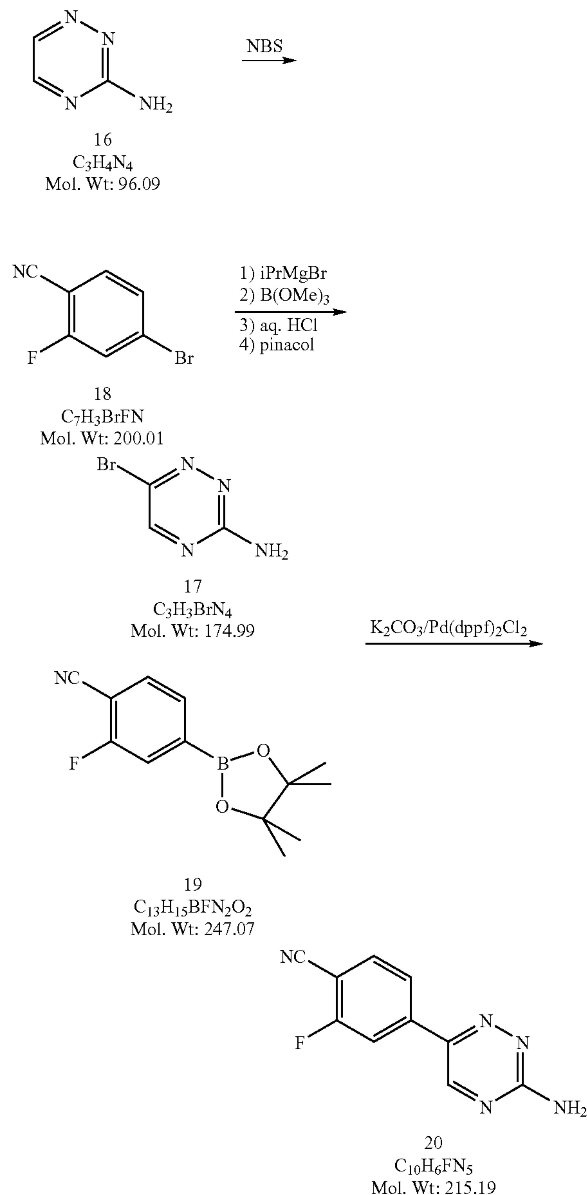
Scheme 4 (Examples 22-25)
