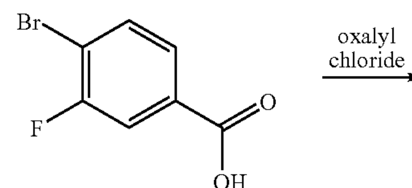
Scheme 1 (Examples 8-14)
