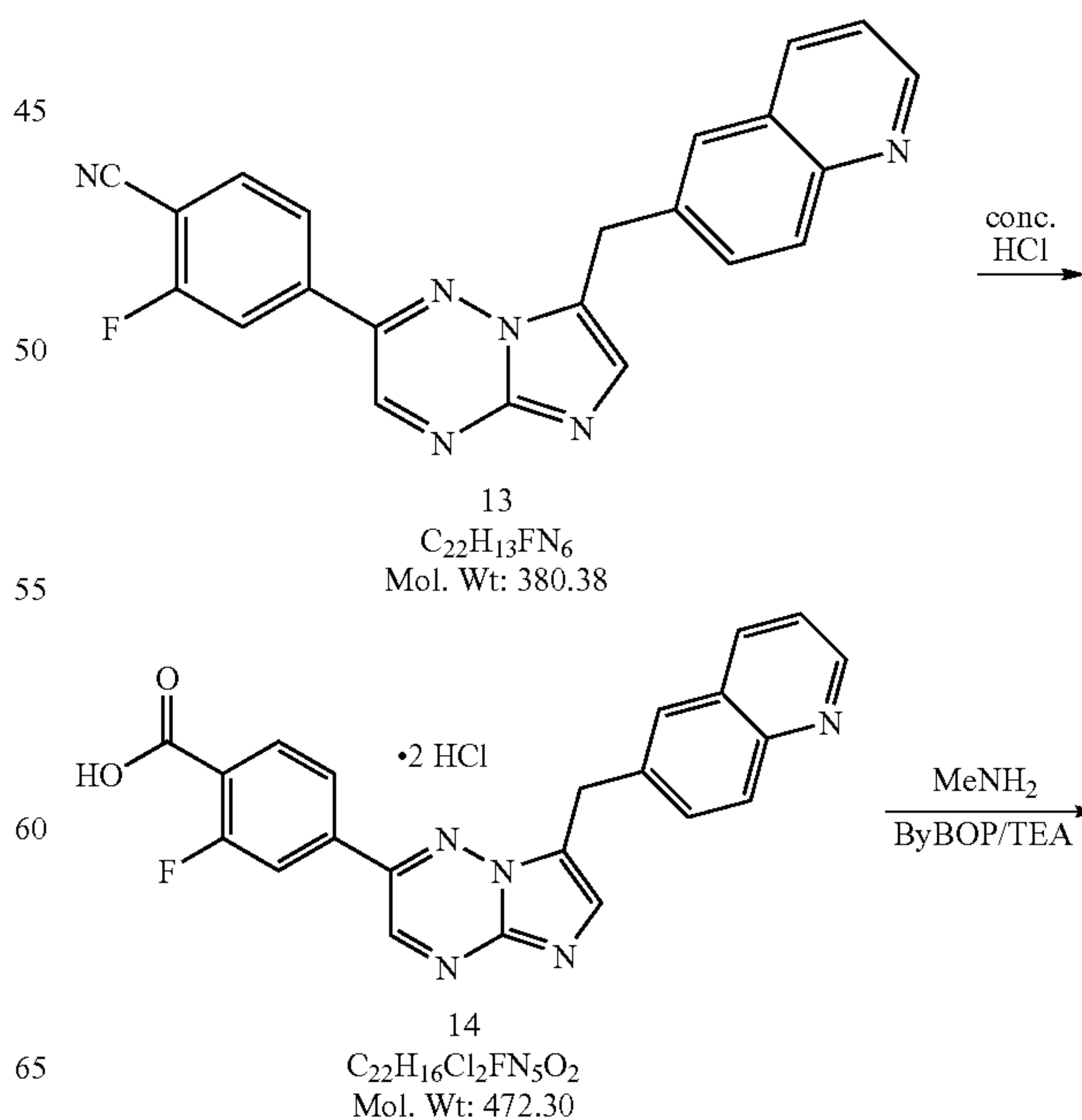
Scheme 3 (Examples 19-21)
