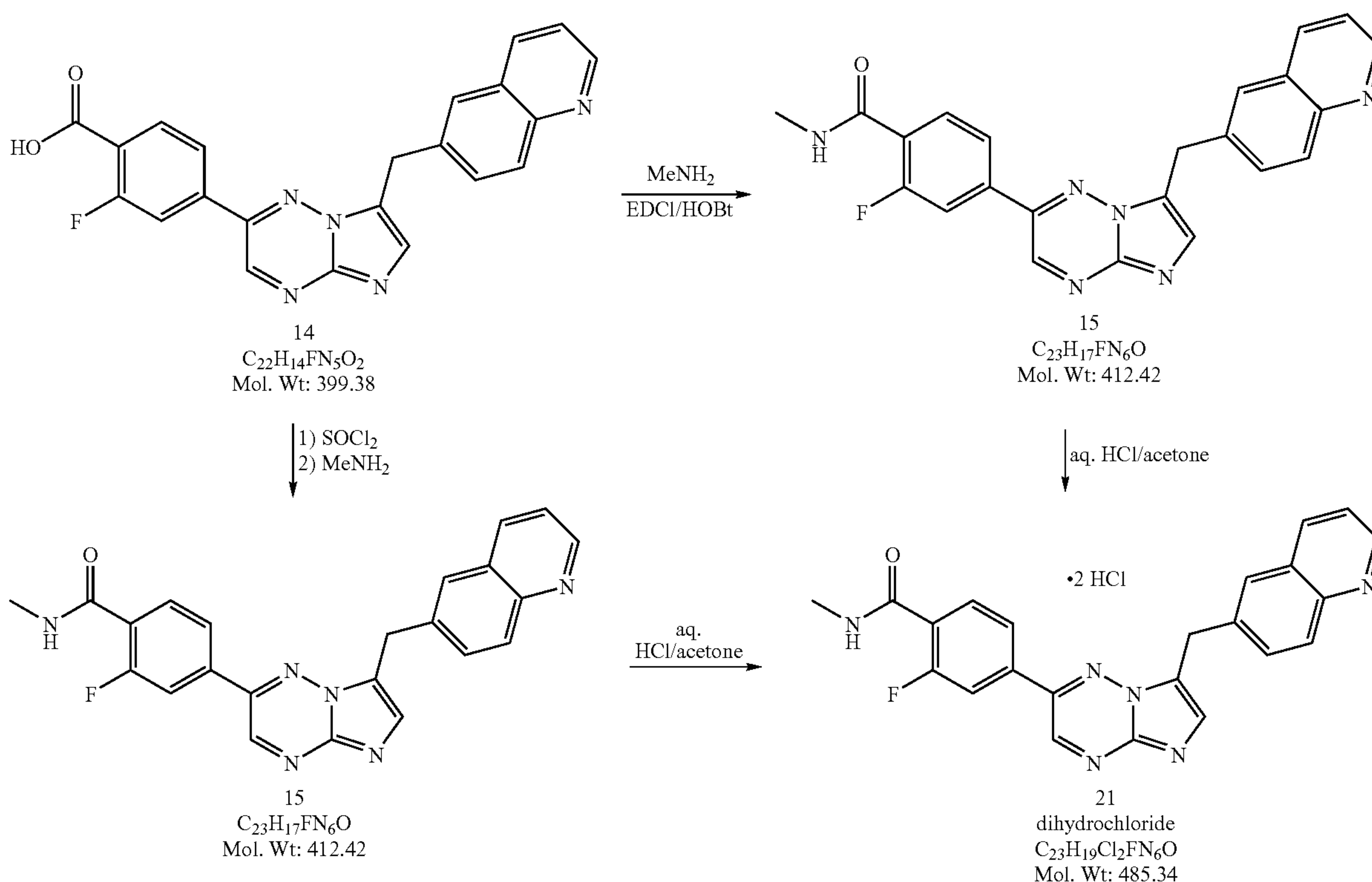
Scheme 6 (Examples 27-29)
