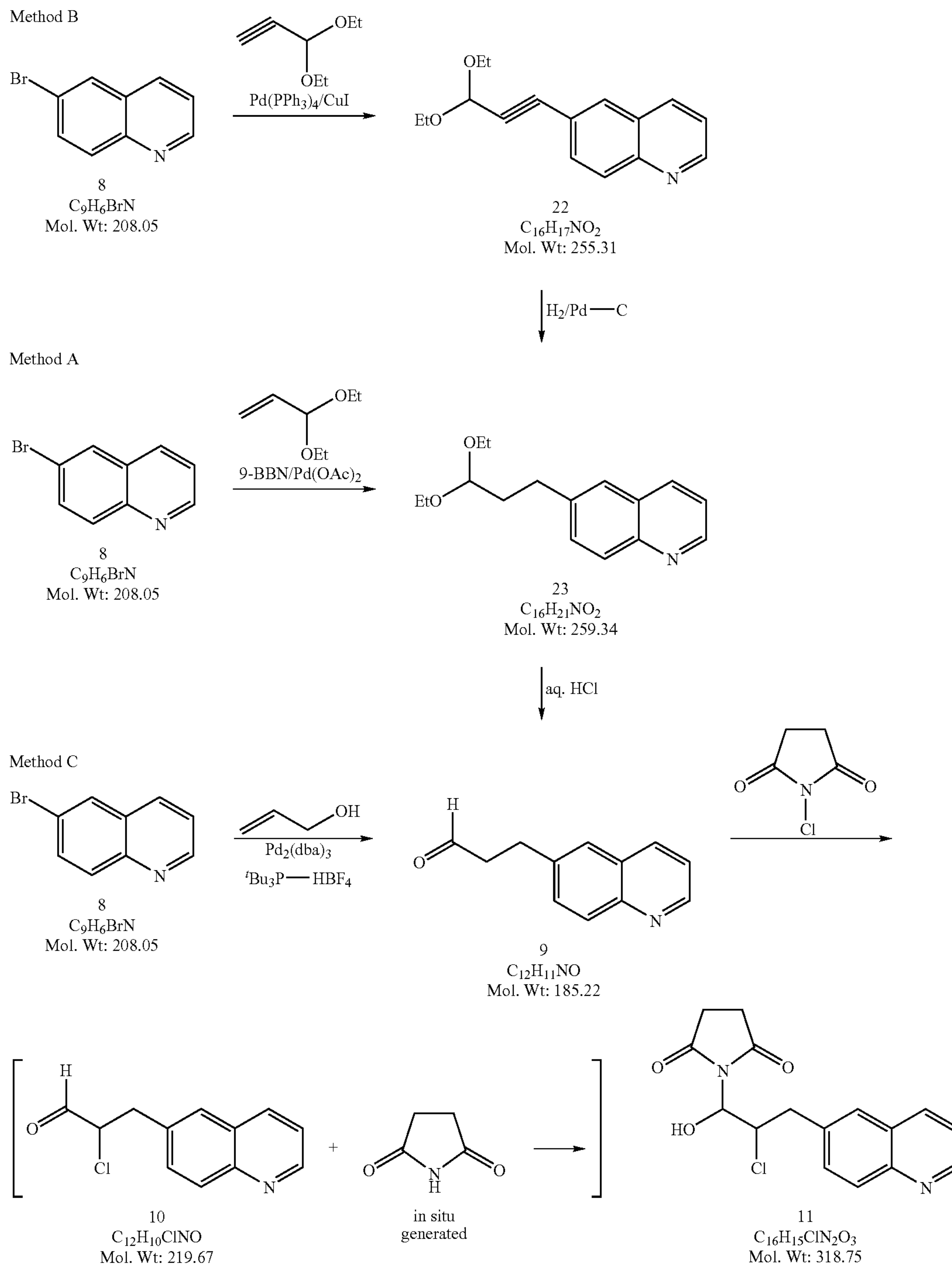
Scheme 2 (Examples 15-18)
