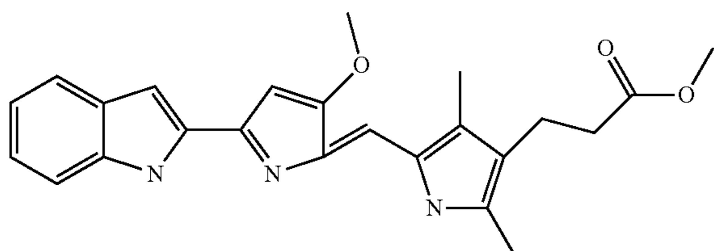
3-{5-[5-(1H-Indol-2-yl)-3-methoxy-pyrrol-2-ylidene-methyl]-2,4-dimethyl-1H-pyrrol-3-yl}-propionic acid methyl ester
