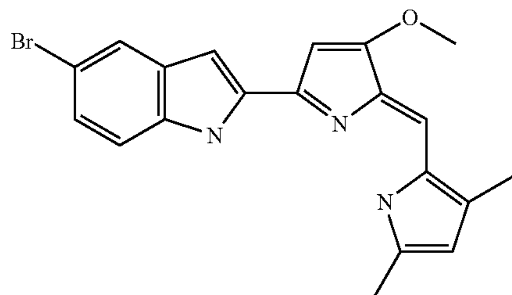
5-Bromo-2-[5-(3,5-dimethyl-1H-pyrrol-2-ylmethylene)-4-methoxy-5H-pyrrol-2-yl]-1H-indole
