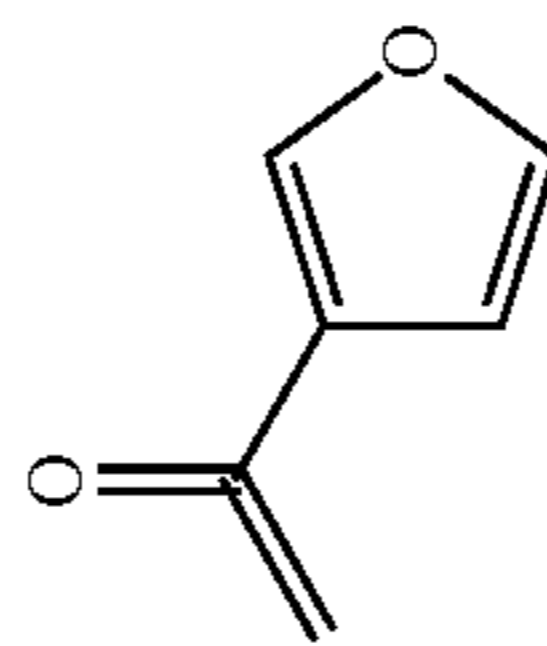
furan-3-yl-methanone
