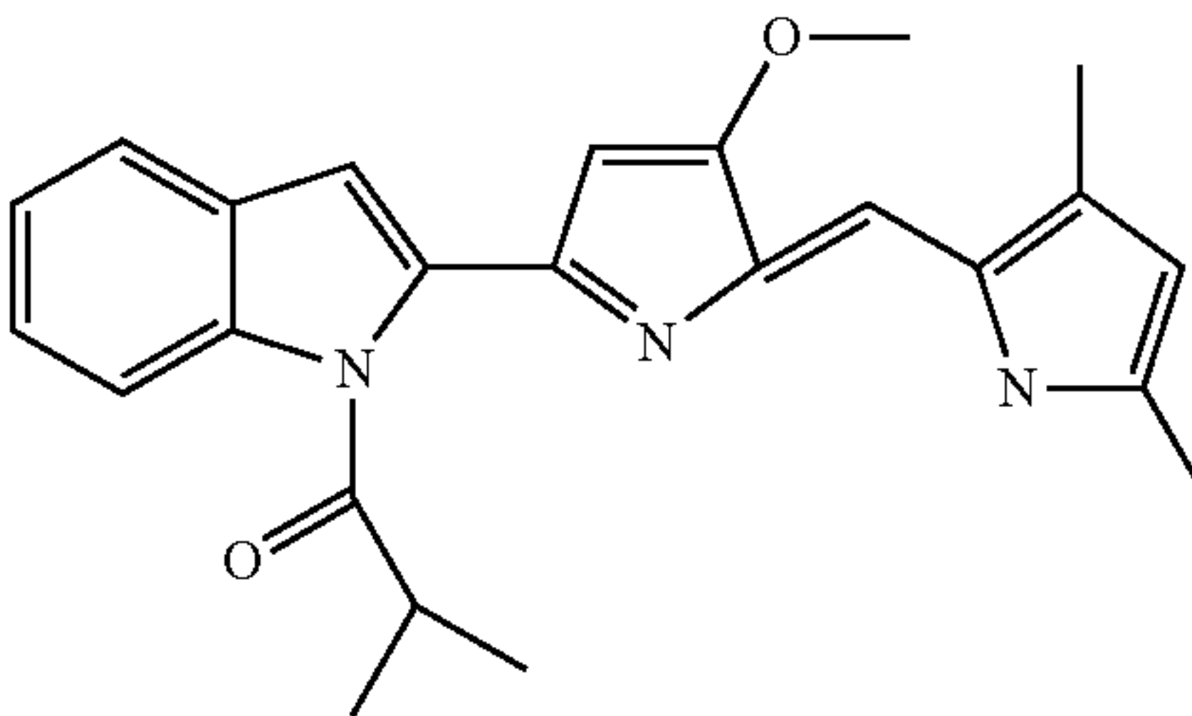
1-(2-[5-(3,5-Dimethyl-1H-pyrrol-2-ylmethylene)-4-methoxy-5H-pyrrol-2-yl]-indol-1-yl)-2-methyl-propan-1-one
