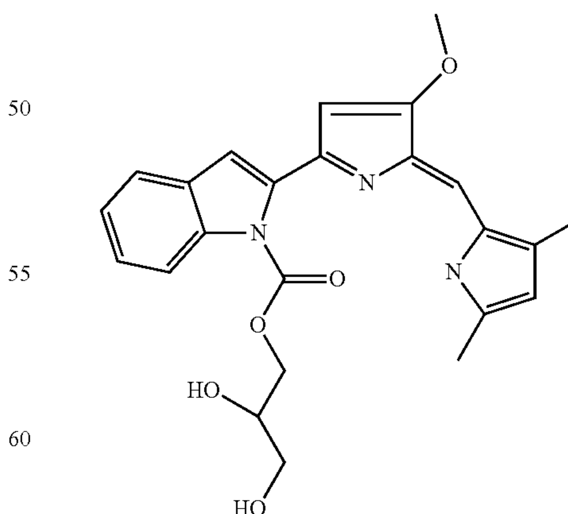
2-[5-(3,5-Dimethyl-1H-pyrrol-2-ylmethylene)-4-methoxy-5H-pyrrol-2-yl]-indole-1-carboxylic acid 2,3-dihydroxypropyl ester
