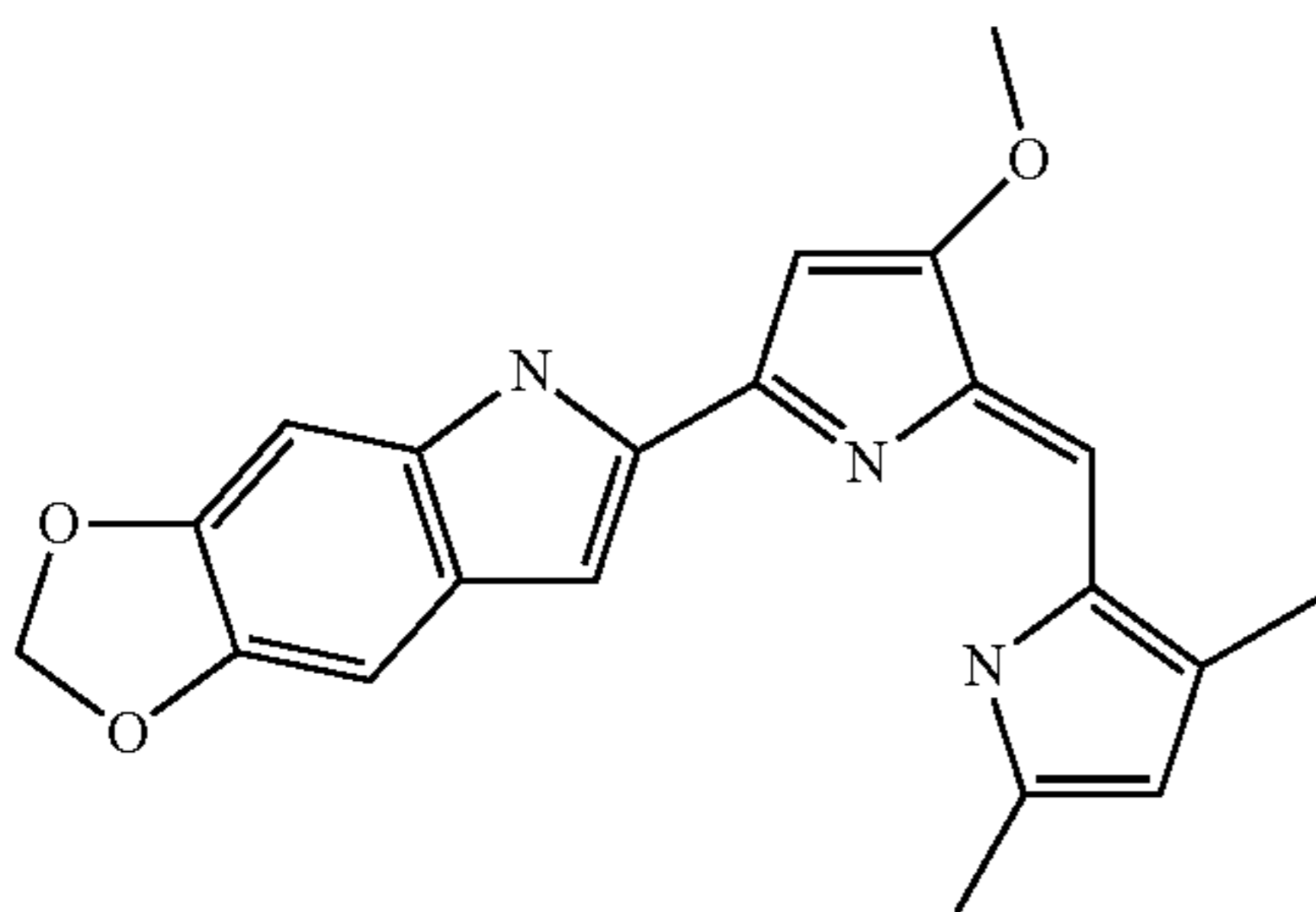
6-[5-(3,5-Dimethyl-1H-pyrrol-2-ylmethylene)-4-methoxy-5H-pyrrol-2-yl]-5H-[1,3]dioxolo[4,5-f]indole
