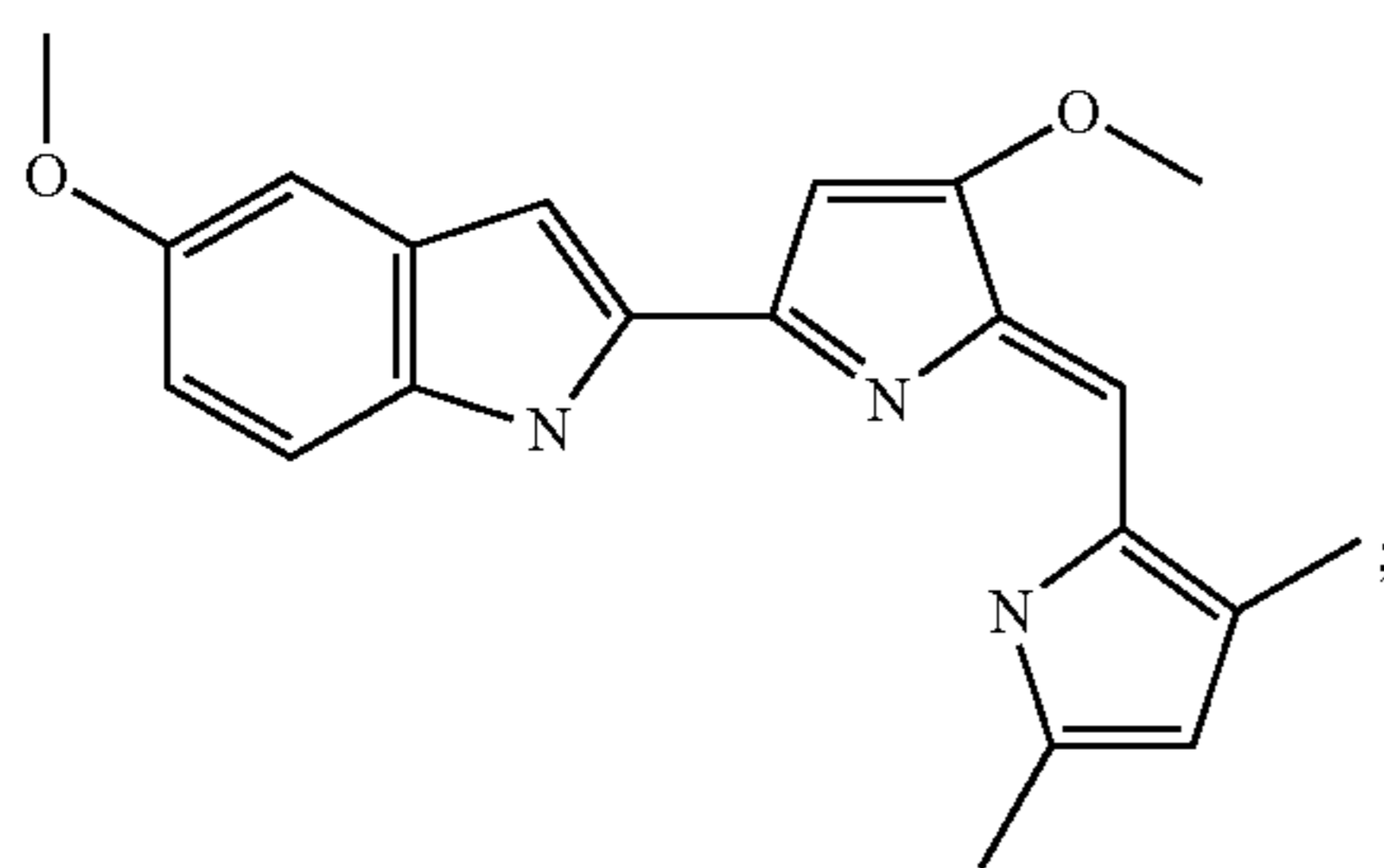
2-[5-(3,5-Dimethyl-1H-pyrrol-2-ylmethylene)-4-methoxy-5H-pyrrol-2-yl]-5-methoxy-1H-indole
