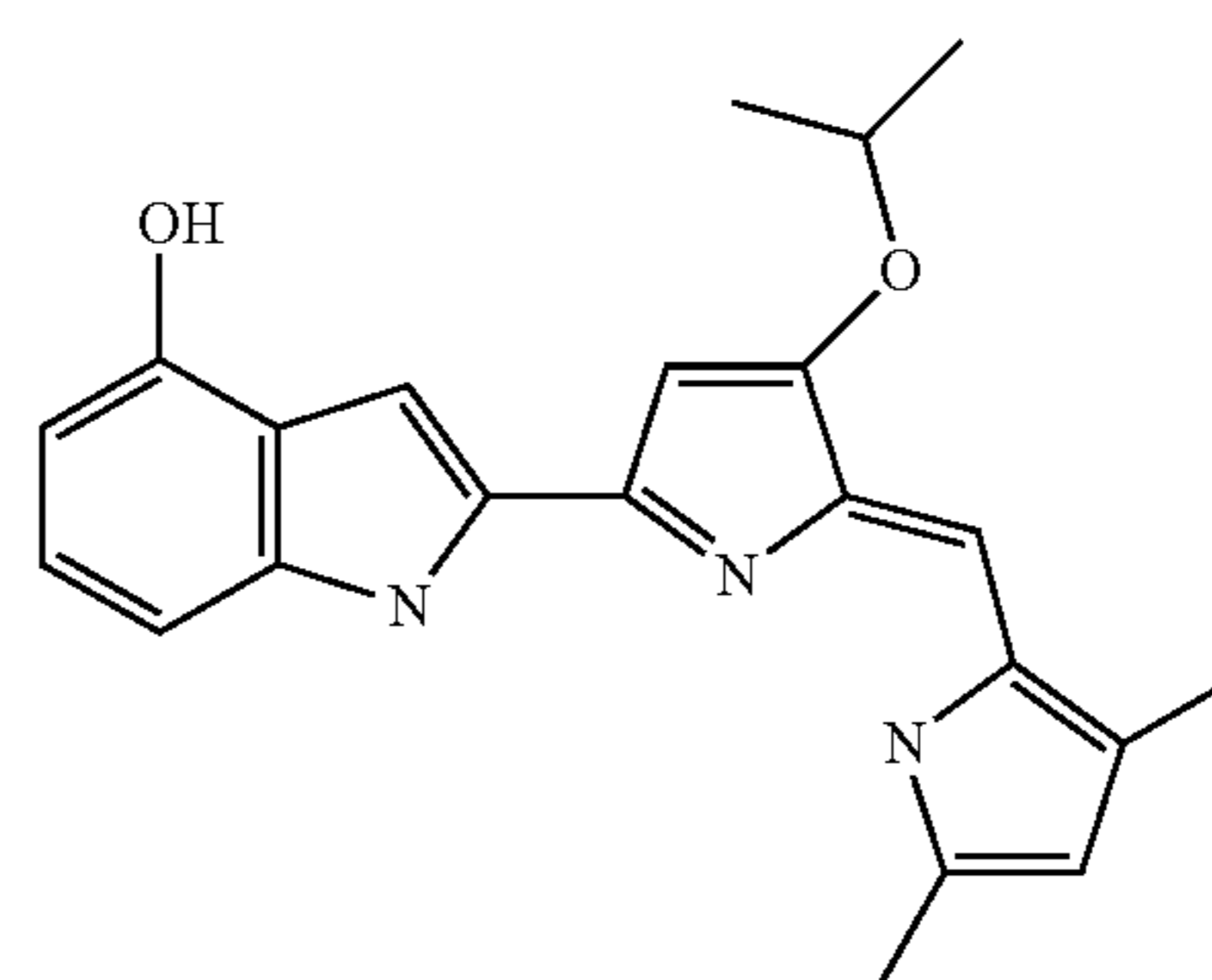
2-[5-(3,5-Dimethyl-1H-pyrrol-2-ylmethylene)-4-isopropoxy-5H-pyrrol-2-yl]-1H-indol-4-ol
