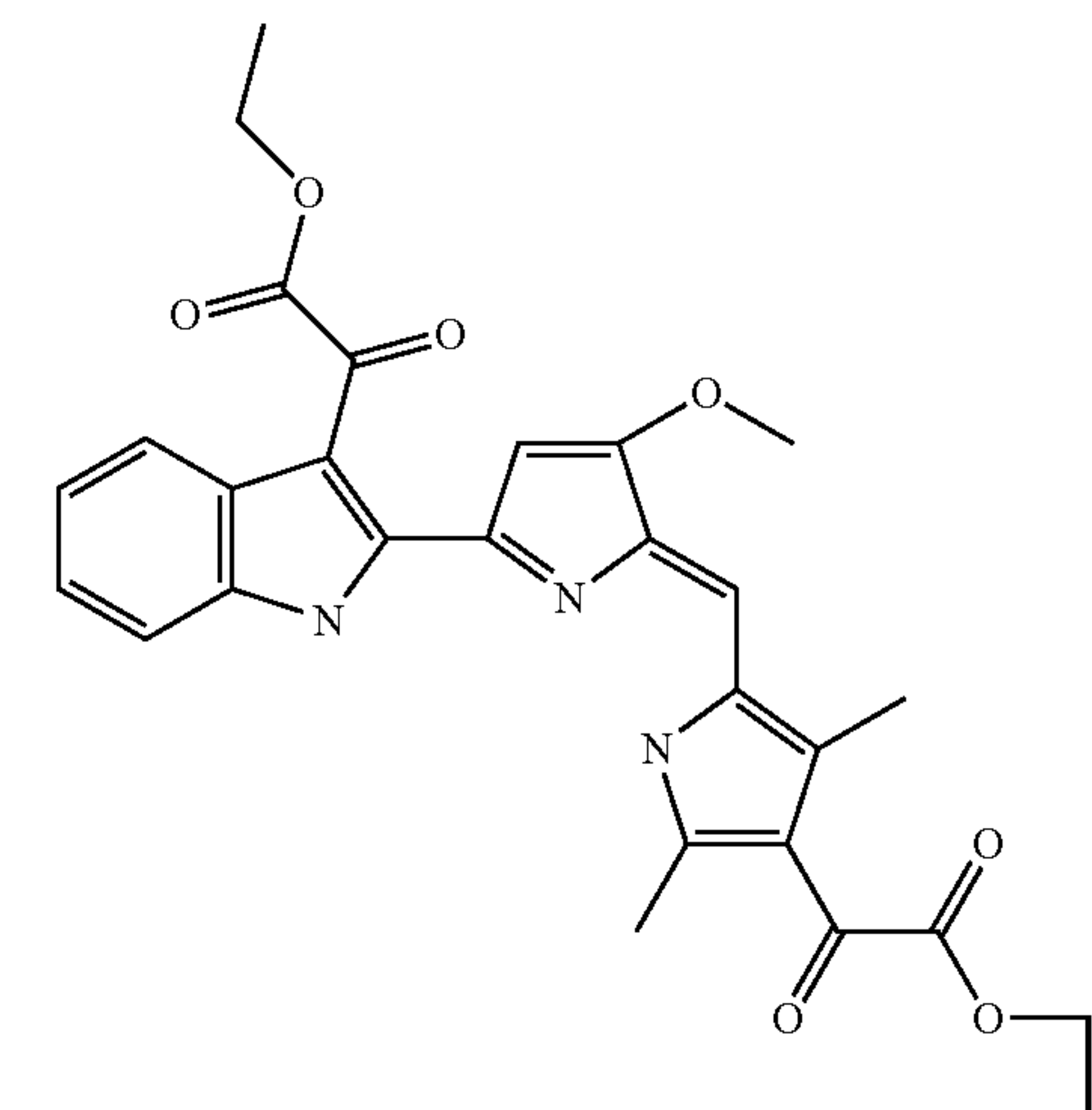
{2-[5-(4-Ethoxyoxalyl-3,5-dimethyl-1H-pyrrol-2-ylmethylene)-4-methoxy-5H-pyrrol-2-yl]-1H-indol-3-yl}-oxo-acetic acid ethyl ester
