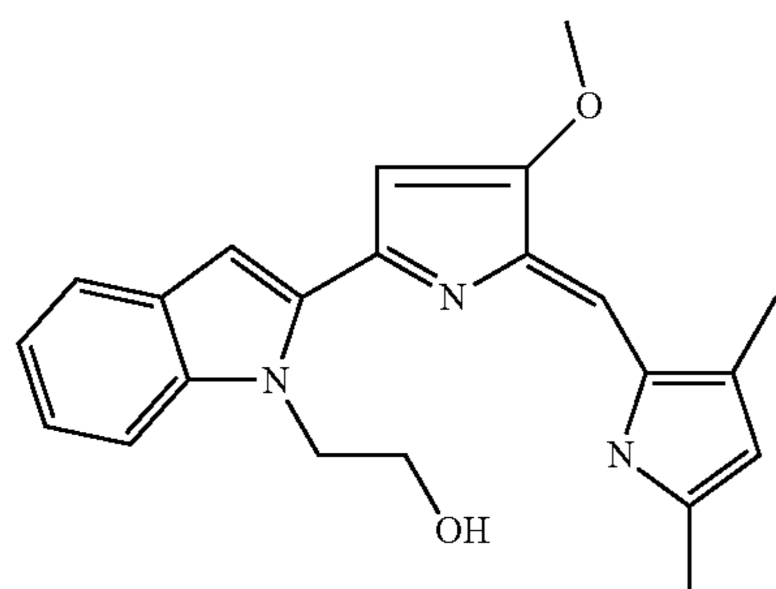
2-{2-[5-(3,5-Dimethyl-1H-pyrrol-2-ylmethylene)-4-methoxy-5H-pyrrol-2-yl]-indol-1-yl}-ethanol
