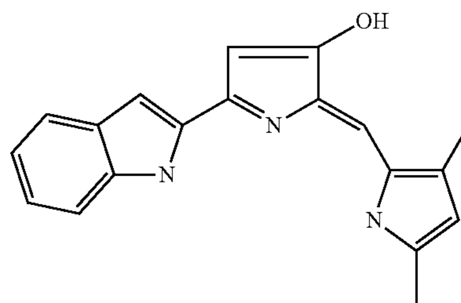
2-(3,5-Dimethyl-1H-pyrrol-2-ylmethylene)-5-(1H-indol-2-yl)-2H-pyrrol-3-ol
