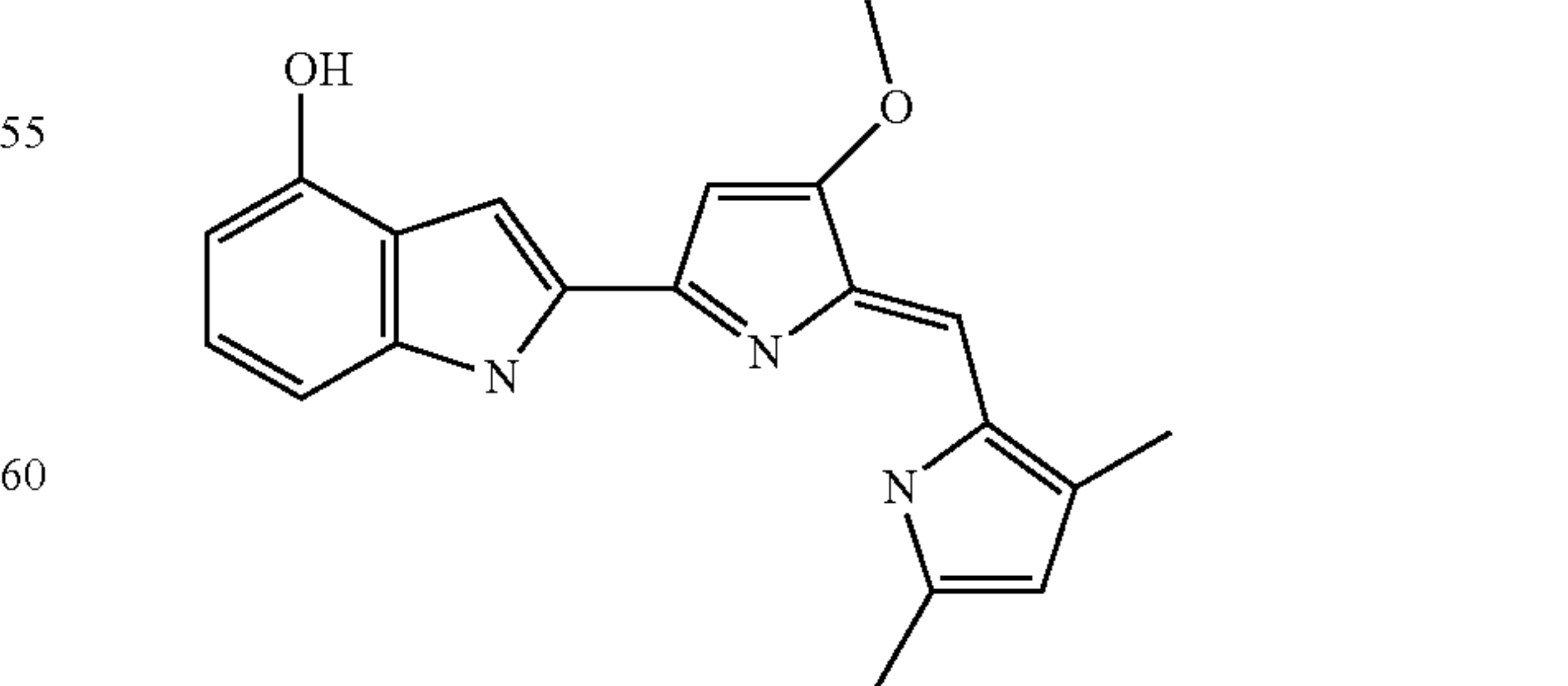
2-[5-(3,5-Dimethyl-1H-pyrrol-2-ylmethylene)-4-methoxy-5H-pyrrol-2-yl]-1H-indol-4-ol
