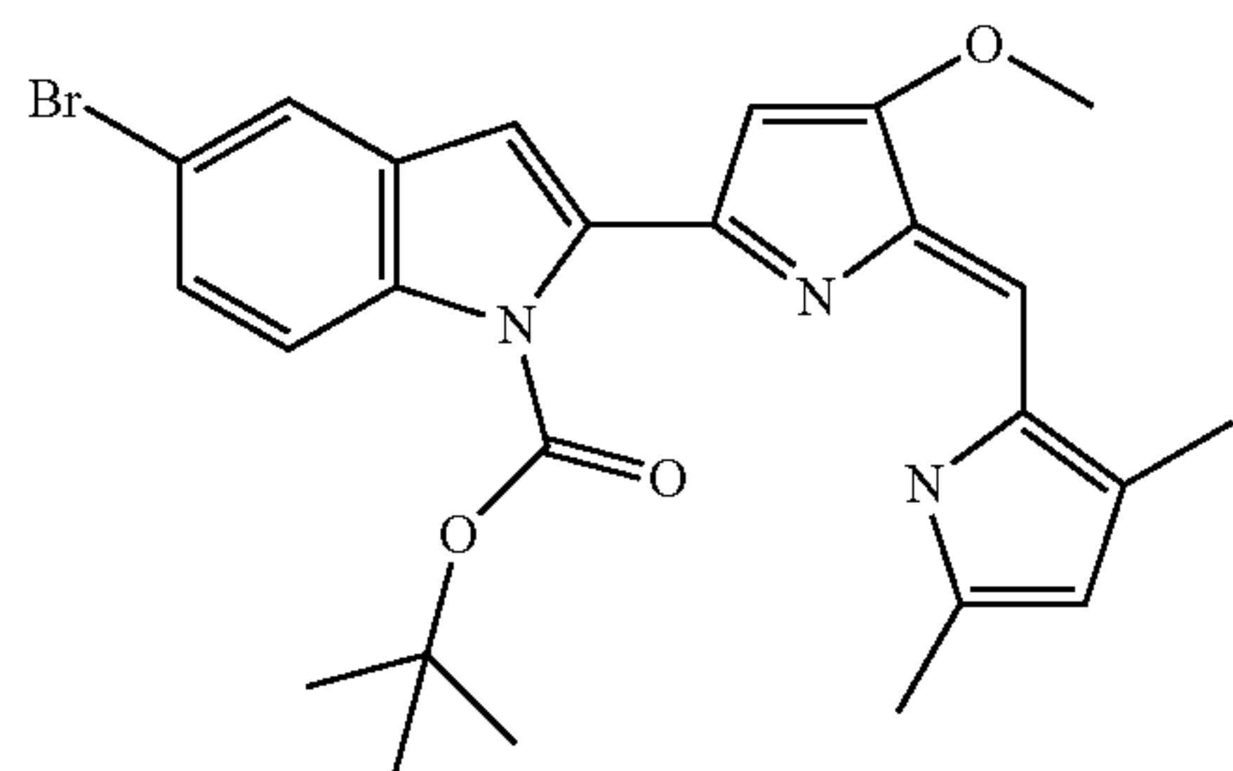
5-Bromo-2-[5-(3,5-dimethyl-1H-pyrrol-2-ylmethylene)-4-methoxy-5H-pyrrol-2-yl]-indole-1-carboxylic acid tert-butyl ester
