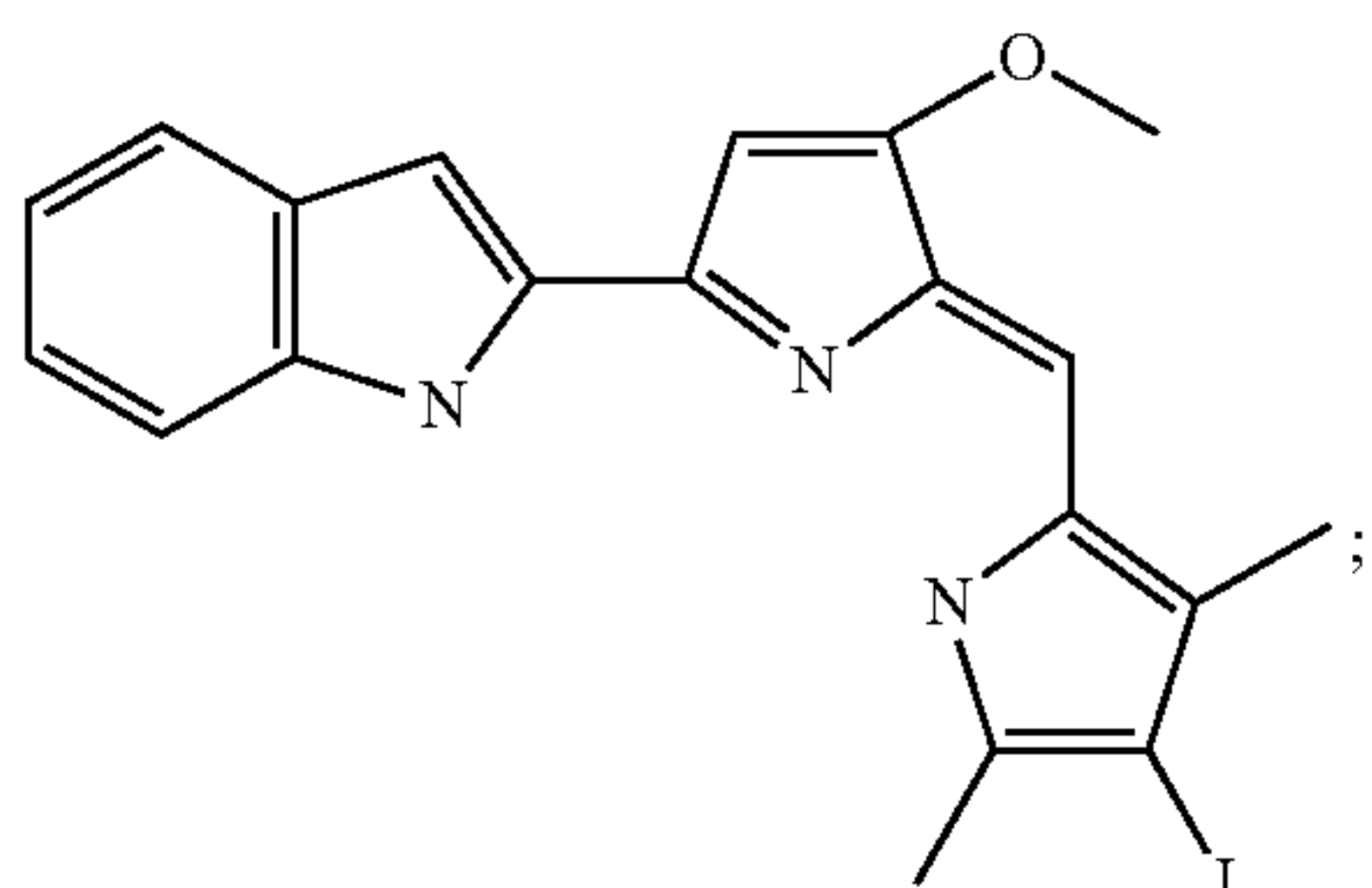
2-[5-(4-Iodo-3,5-dimethyl-1H-pyrrol-2-ylmethylene)-4-methoxy-5H-pyrrol-2-yl]-1H-indole
