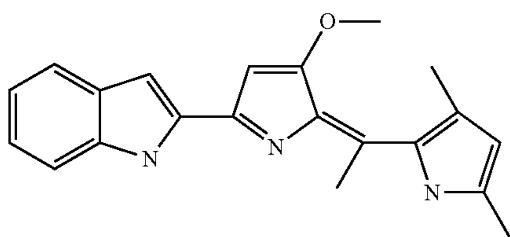
2-[5-[1-(3,5-Dimethyl-1H-pyrrol-2-yl)ethylidene]-4-methoxy-5H-pyrrol-2-yl]-1H-indole
