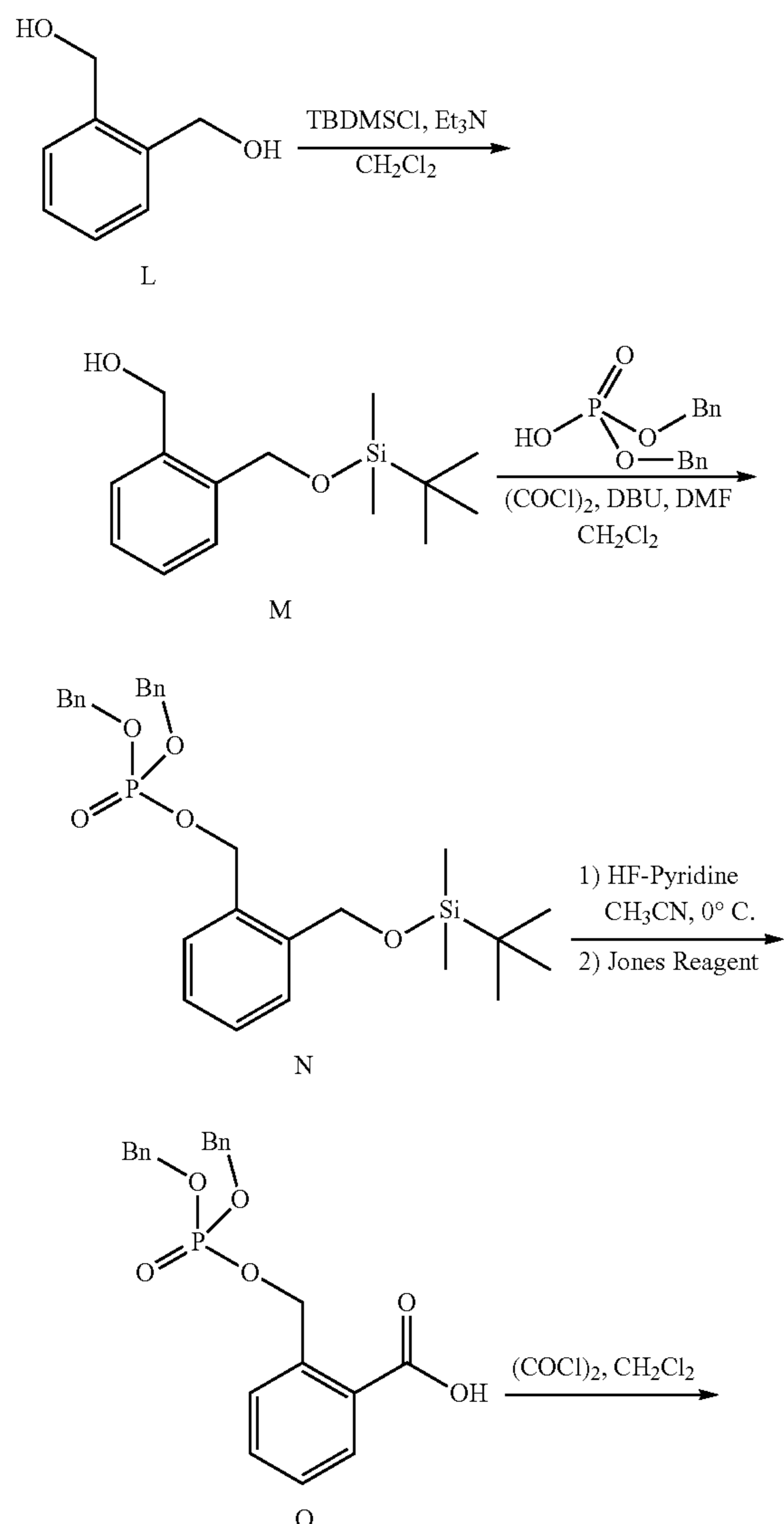
Scheme 4
