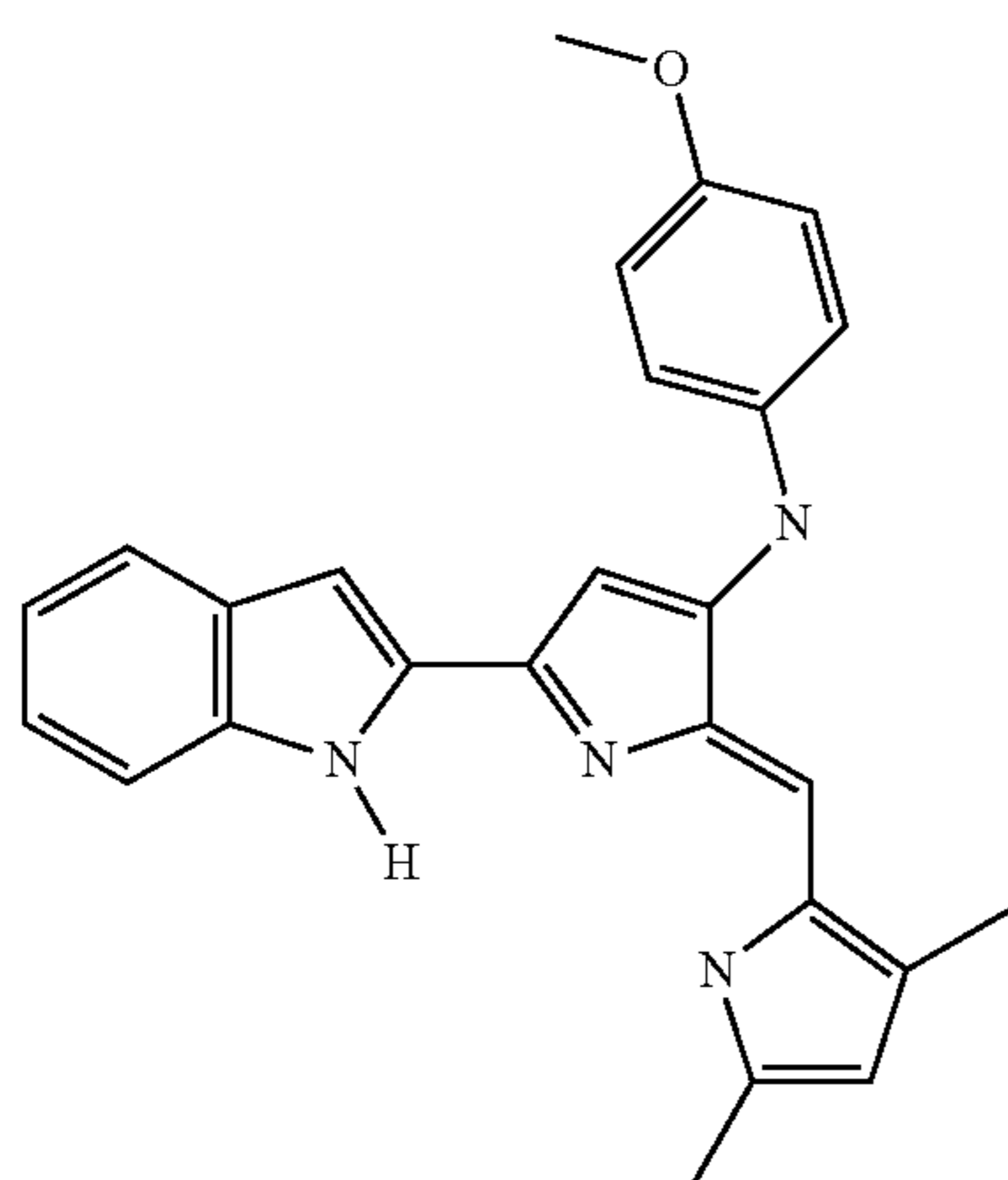
[2-(3,5-Dimethyl-1H-pyrrol-2-ylmethylene)-5-(1H-indol-2-yl)-2H-pyrrol-3-yl]-(4-methoxy-phenyl)-amine
