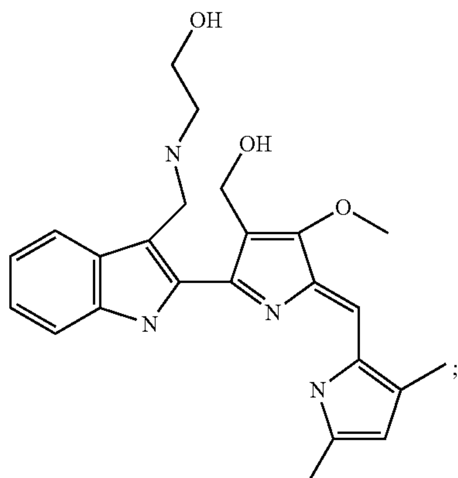
2-({2-[5-(3,5-Dimethyl-1H-pyrrol-2-ylmethylene)-3-hydroxymethyl-4-methoxy-5H-pyrrol-2-yl]-1H-indol-3-ylmethyl}-amino)-ethanol
