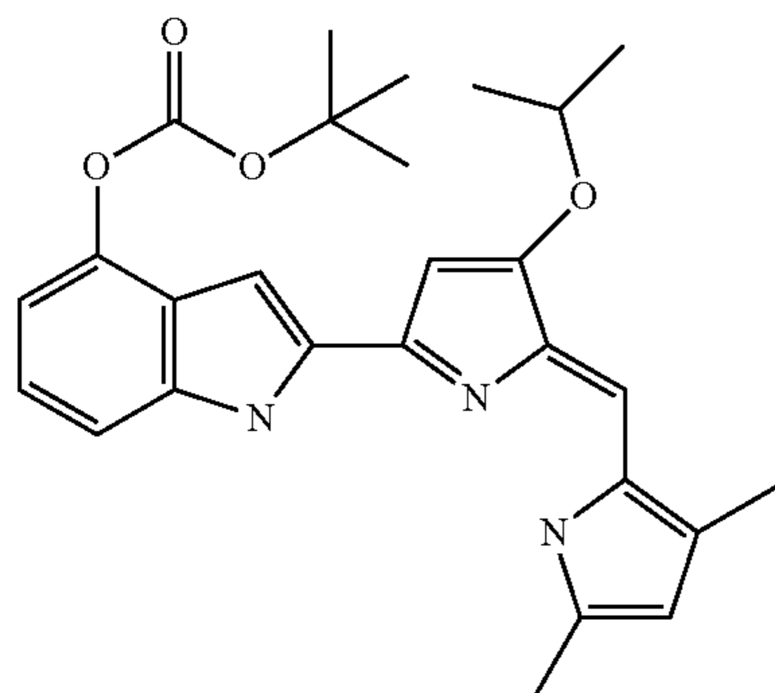
Carbonic acid tert-butyl ester 2-[5-(3,5-dimethyl-1H-pyrrol-2-ylmethylene)-4-isopropoxy-5H-pyrrol-2-yl]-1H-indol-4-yl ester
