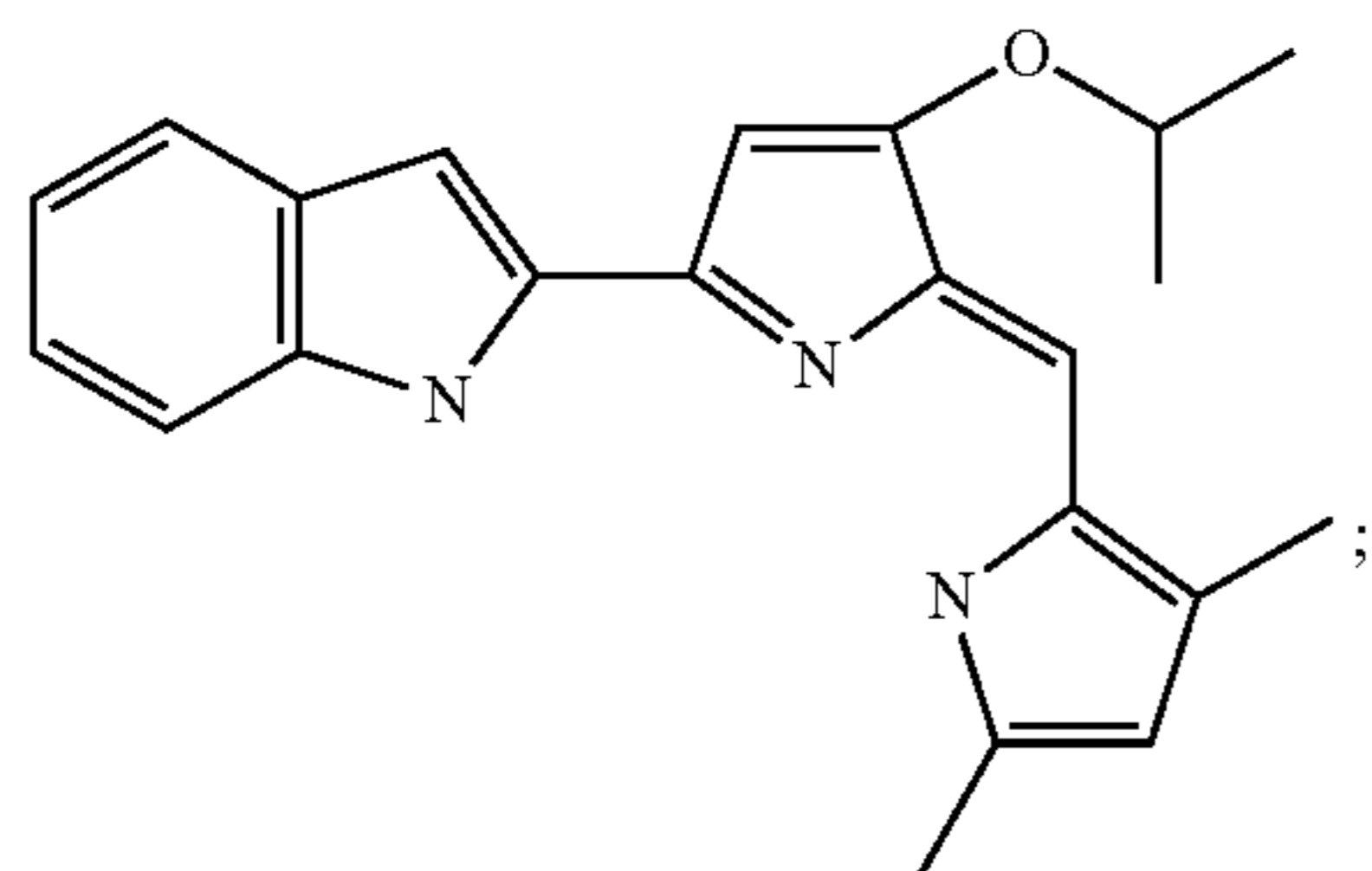
2-[5-(3,5-Dimethyl-1H-pyrrol-2-ylmethylene)-4-isopropoxy-5H-pyrrol-2-yl]-1H-indole
