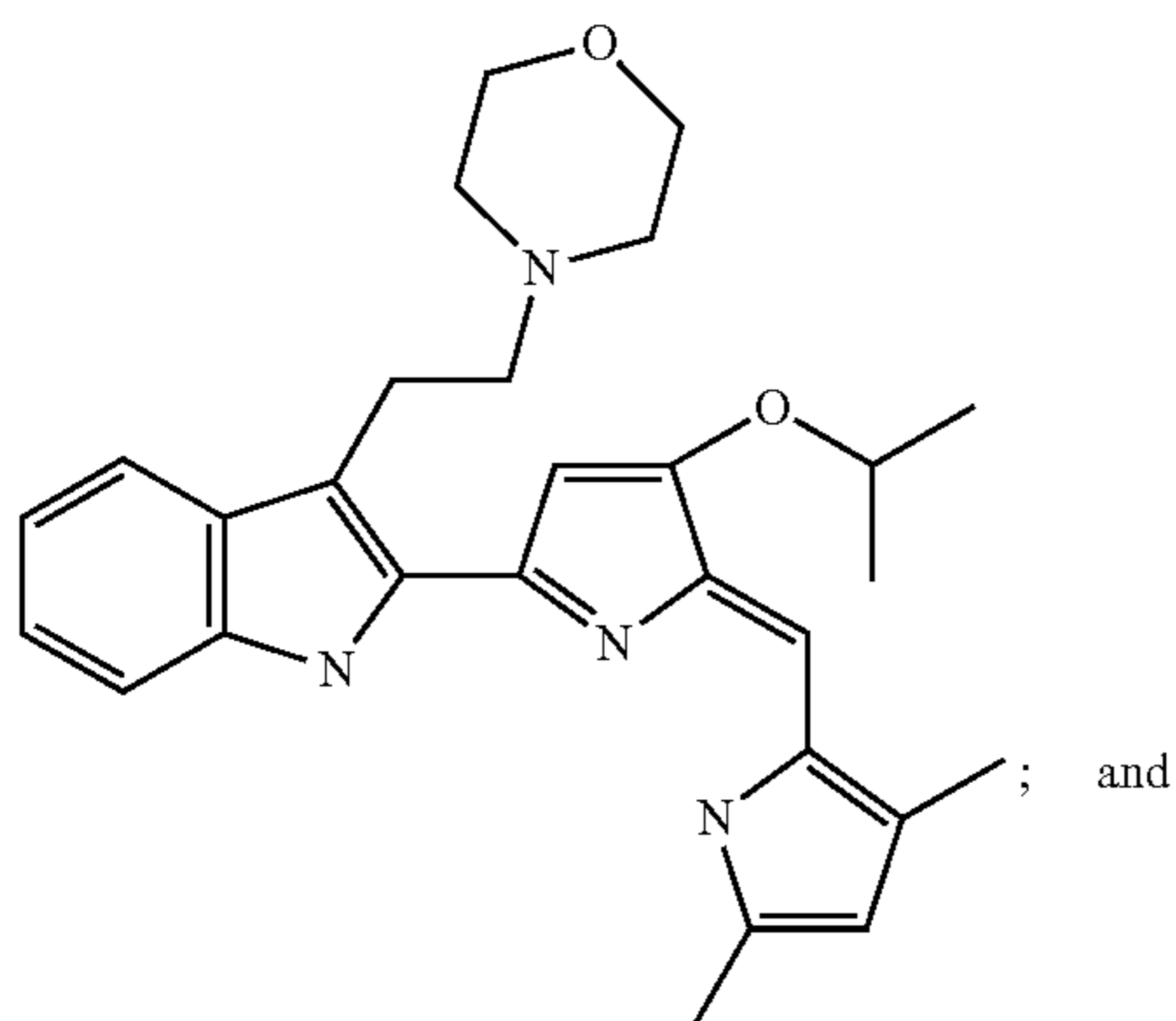
2-[5-(3,5-Dimethyl-1H-pyrrol-2-ylmethylene)-4-isopropoxy-5H-pyrrol-2-yl]-3-(2-morpholin-4-yl-ethyl)-1H-indole
