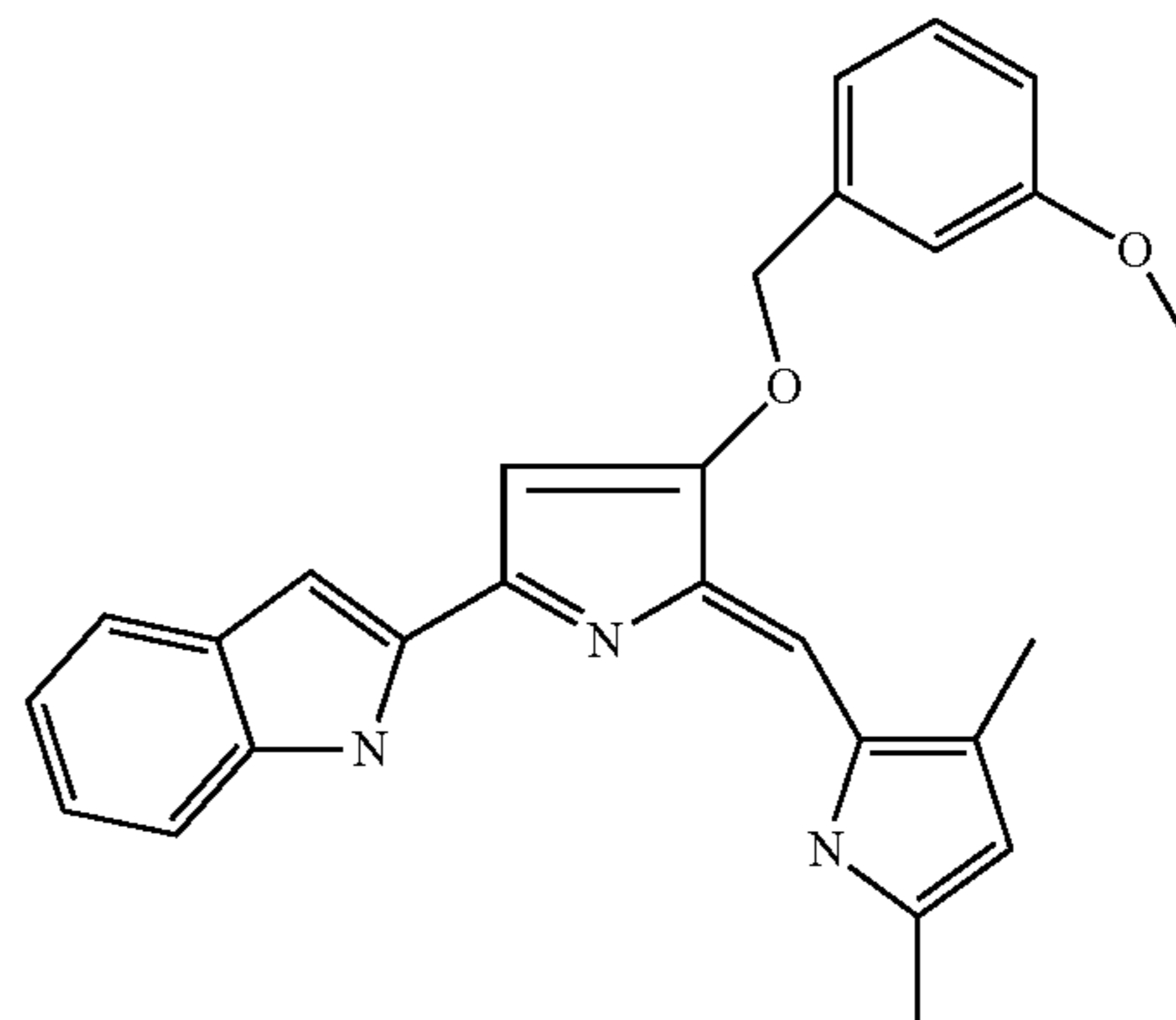
2-[5-(3,5-Dimethyl-1H-pyrrol-2-ylmethylene)-4-(3-methoxy-benzyloxy)-5H-pyrrol-2-yl]-1H-indole
