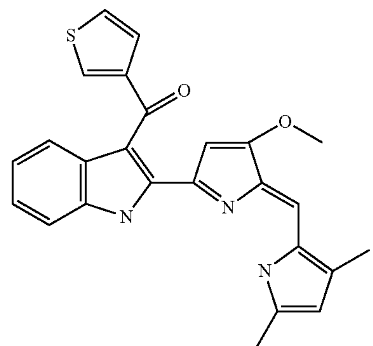
{2-[5-(3,5-Dimethyl-1H-pyrrol-2-ylmethylene)-4-methoxy-5H-pyrrol-2-yl]-1H-indol-3-yl}-thiophen-3-yl-methanone
