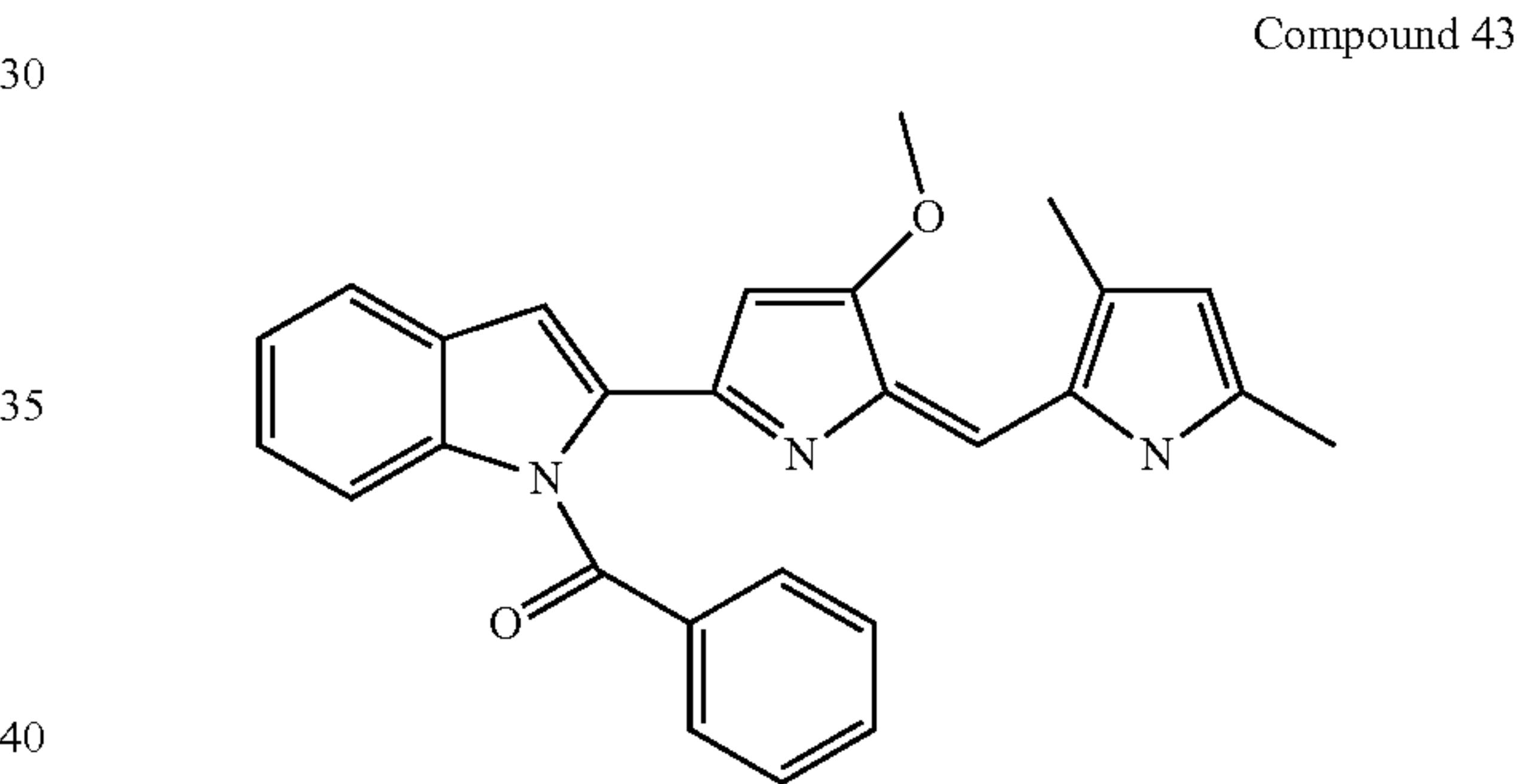
{2-[5-(3,5-Dimethyl-1H-pyrrol-2-ylmethylene)-4-methoxy-5H-pyrrol-2-yl]-indol-1-yl}-phenyl-methanone
