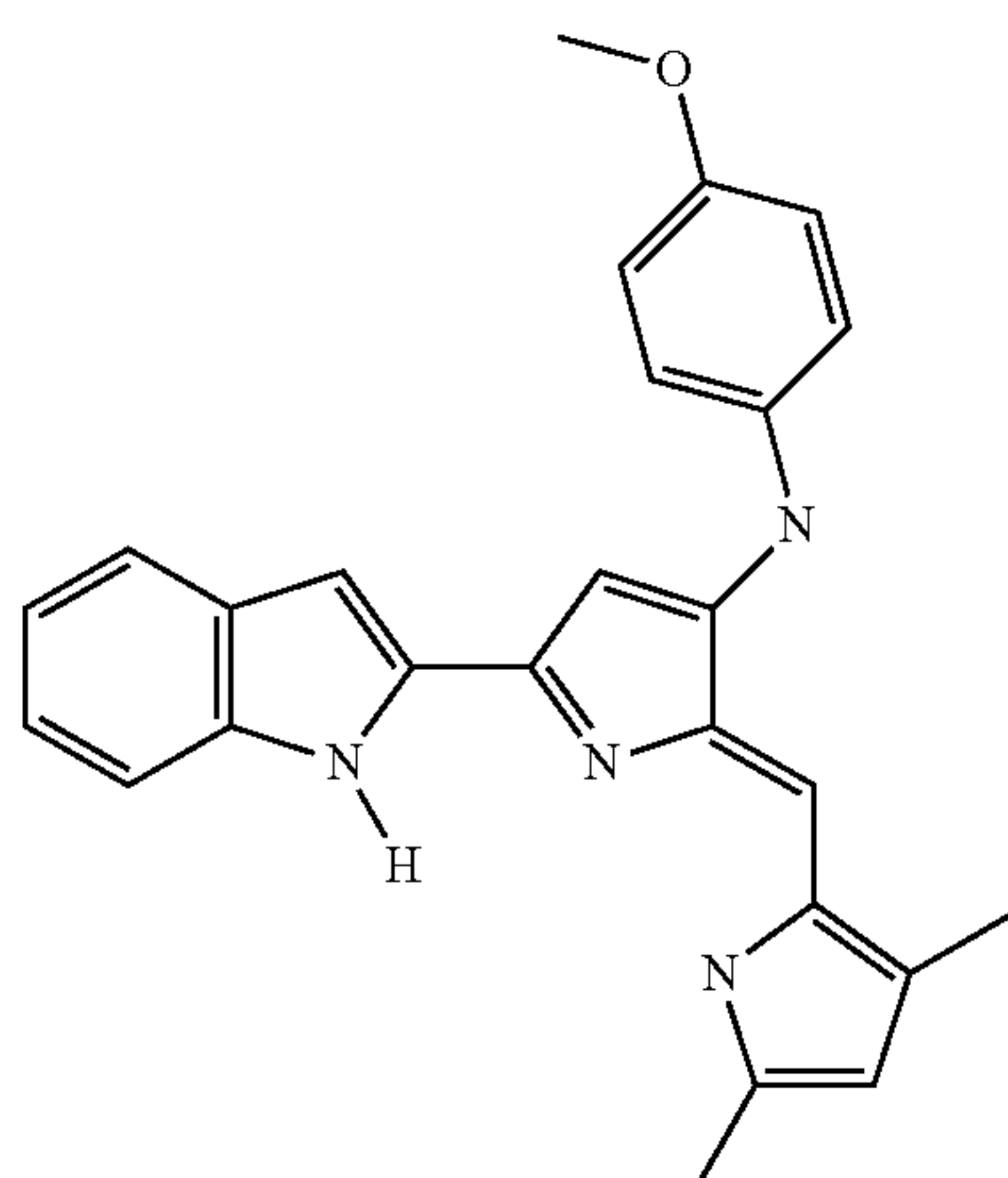
[2-(3,5-Dimethyl-1H-pyrrol-2-ylmethylene)-5-(1H-indol-2-yl)-2H-pyrrol-3-yl]-(4-methoxy-phenyl)-amine
