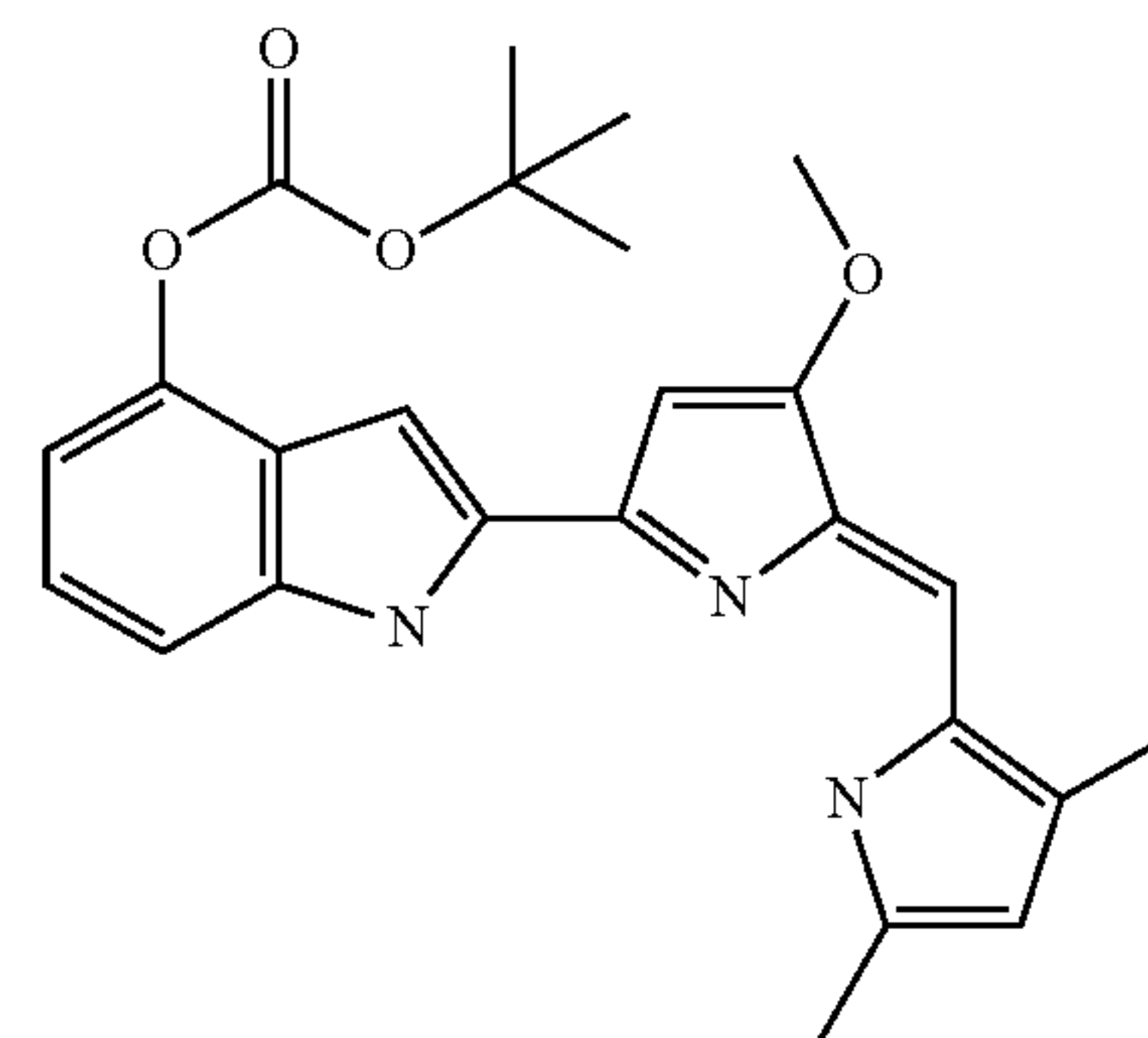
Carbonic acid tert-butyl ester 2-[5-(3,5-dimethyl-1H-pyrrol-2-ylmethylene)-4-methoxy-5H-pyrrol-2-yl]-1H-indol-4-yl ester
