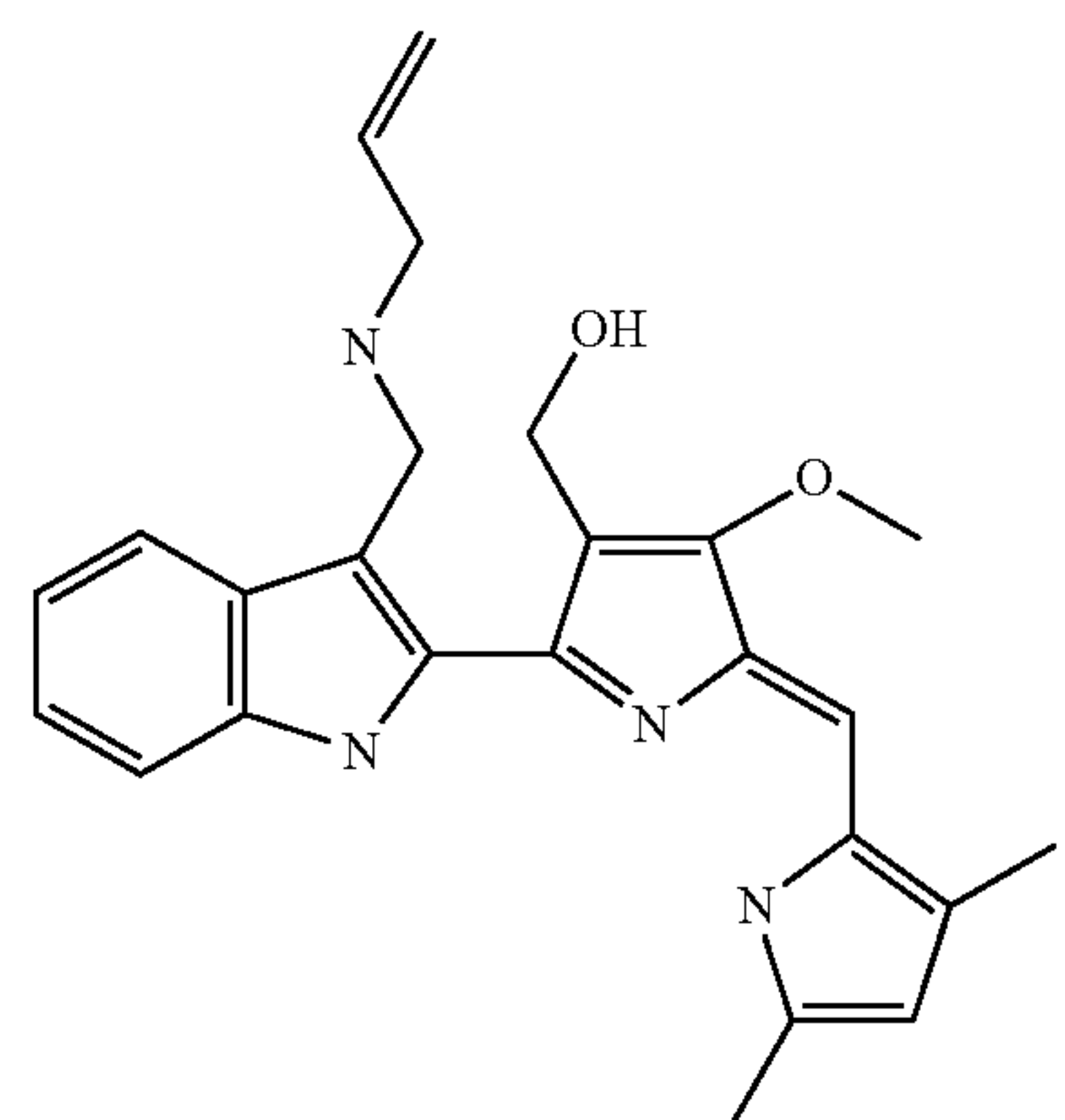
[2-(3-Allylaminomethyl)-1H-indol-2-yl]-5-(3,5-dimethyl-1H-pyrrol-2-ylmethylene)-4-methoxy-5H-pyrrol-3-yl]-methanol
