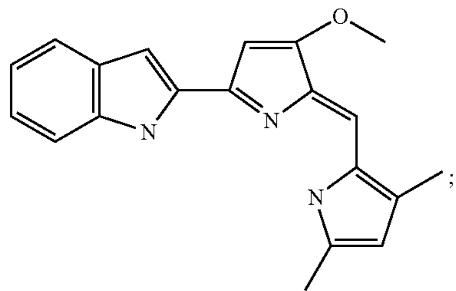
2-[5-(3,5-Dimethyl-1H-pyrrol-2-ylmethylene)-4-methoxy-5H-pyrrol-2-yl]-1H-indole
