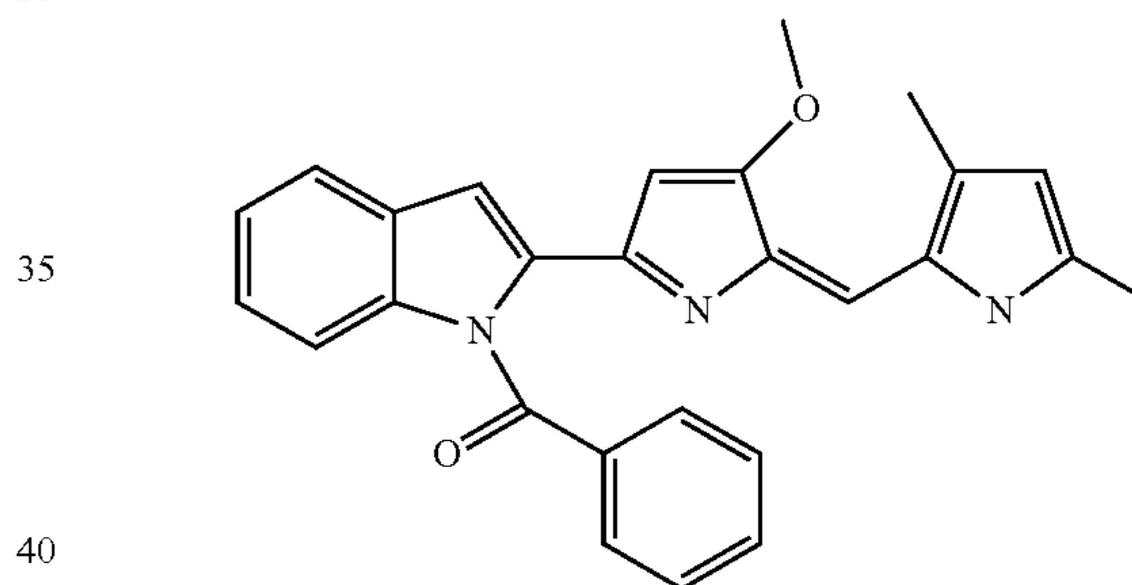
{2-[5-(3,5-Dimethyl-1H-pyrrol-2-ylmethylene)-4-methoxy-5H-pyrrol-2-yl]-indol-1-yl}-phenyl-methanone
