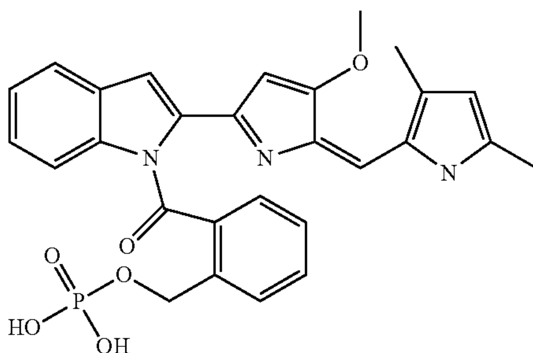
Phosphoric acid mono-(2-(2-[5-(3,5-dimethyl-1H-pyrrol-2-yl)methylene)-4-methoxy-5H-pyrrol-2-yl]-indole-1-carbonyl)-benzyl ester
