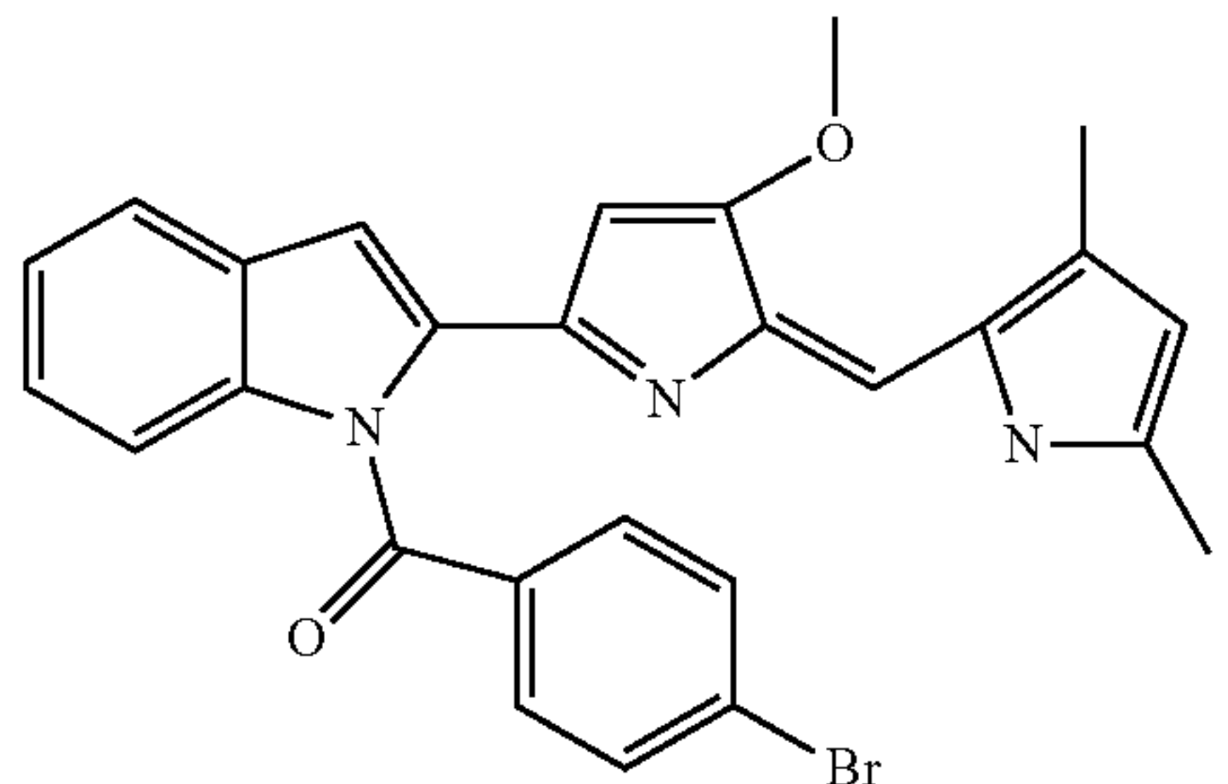
(4-Bromo-phenyl)-{2-[5-(3,5-dimethyl-1H-pyrrol-2-ylmethylene)-4-methoxy-5H-pyrrol-2-yl]-indol-1-yl}-methanone
