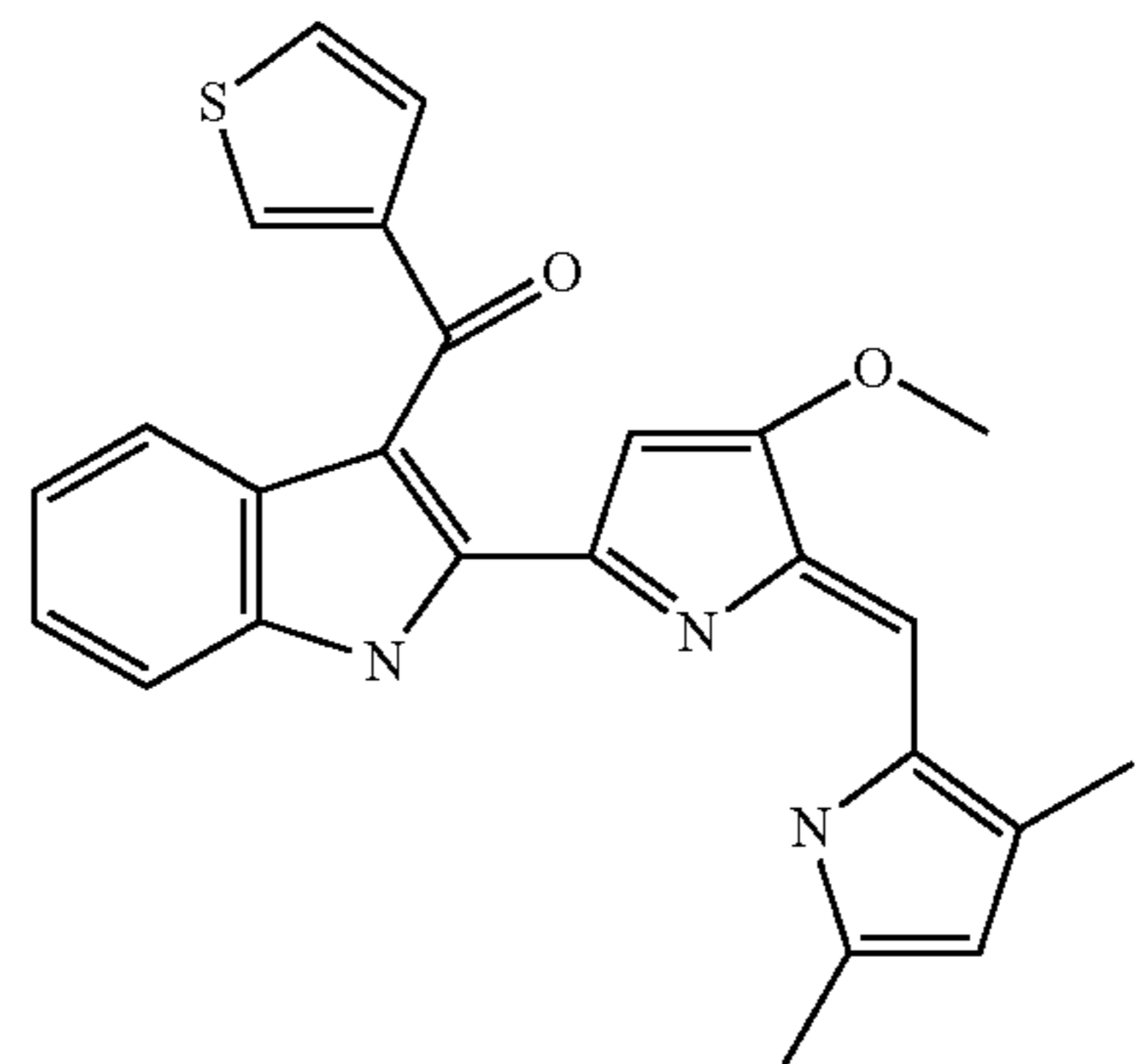
{2-[5-(3,5-Dimethyl-1H-pyrrol-2-ylmethylene)-4-methoxy-5H-pyrrol-2-yl]-1H-indol-3-yl}-thiophen-3-yl-methanone
