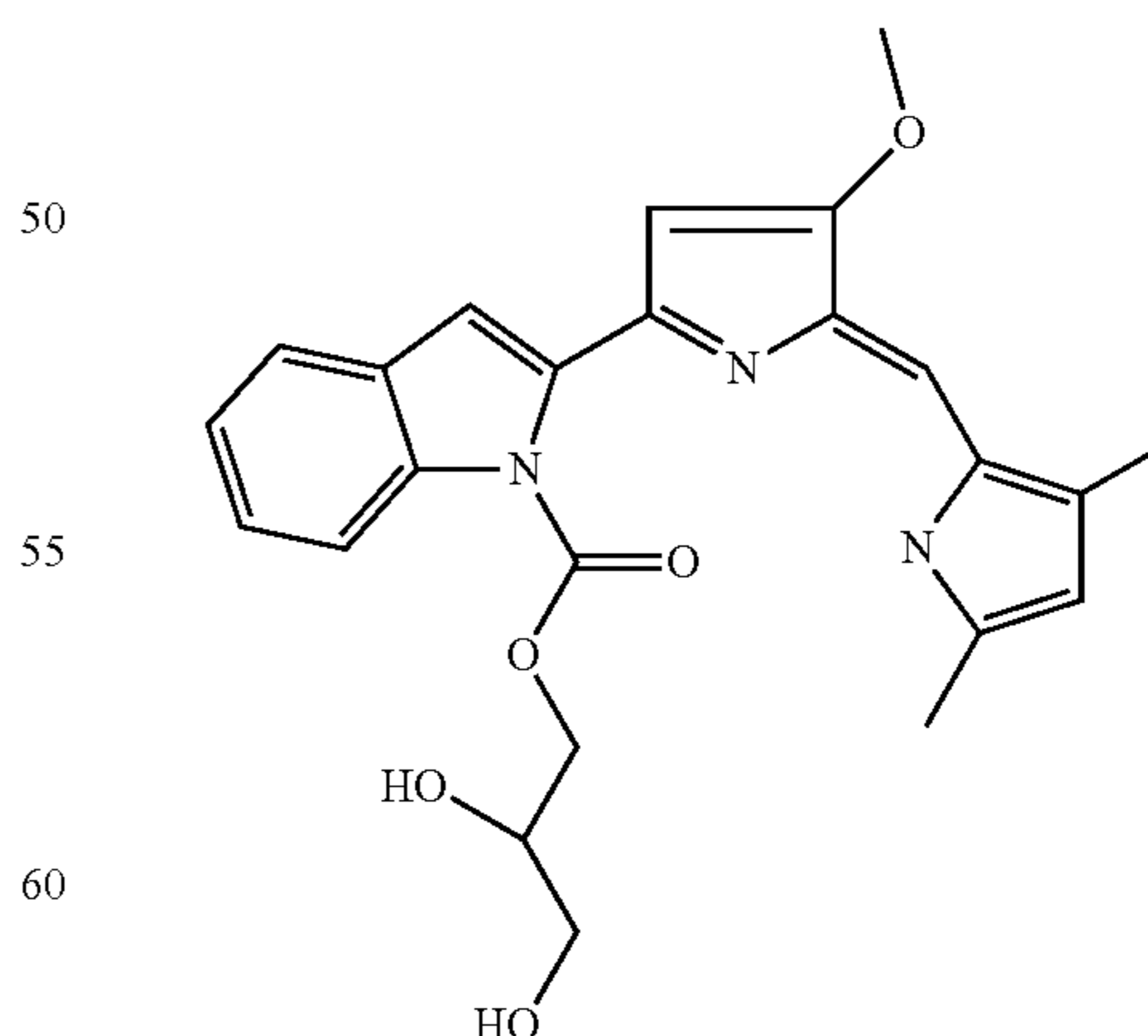
2-[5-(3,5-Dimethyl-1H-pyrrol-2-ylmethylene)-4-methoxy-5H-pyrrol-2-yl]-indole-1-carboxylic acid 2,3-dihydroxypropyl ester
