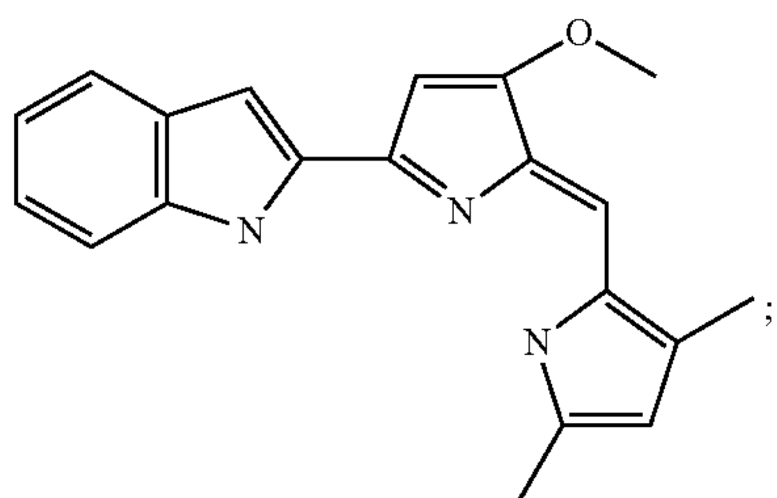
2-[5-(3,5-Dimethyl-1H-pyrrol-2-ylmethylene)-4-methoxy-5H-pyrrol-2-yl]-1H-indole
