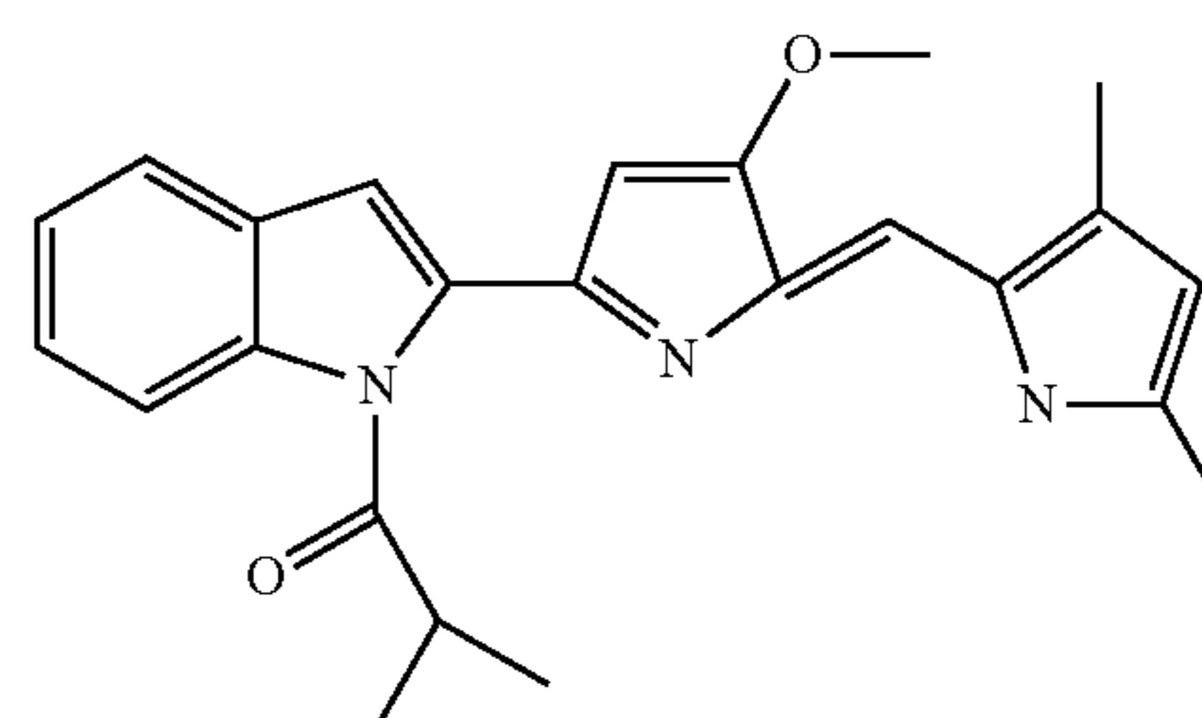
1-(2-[5-(3,5-Dimethyl-1H-pyrrol-2-ylmethylene)-4-methoxy-5H-pyrrol-2-yl]-indol-1-yl)-2-methyl-propan-1-one
