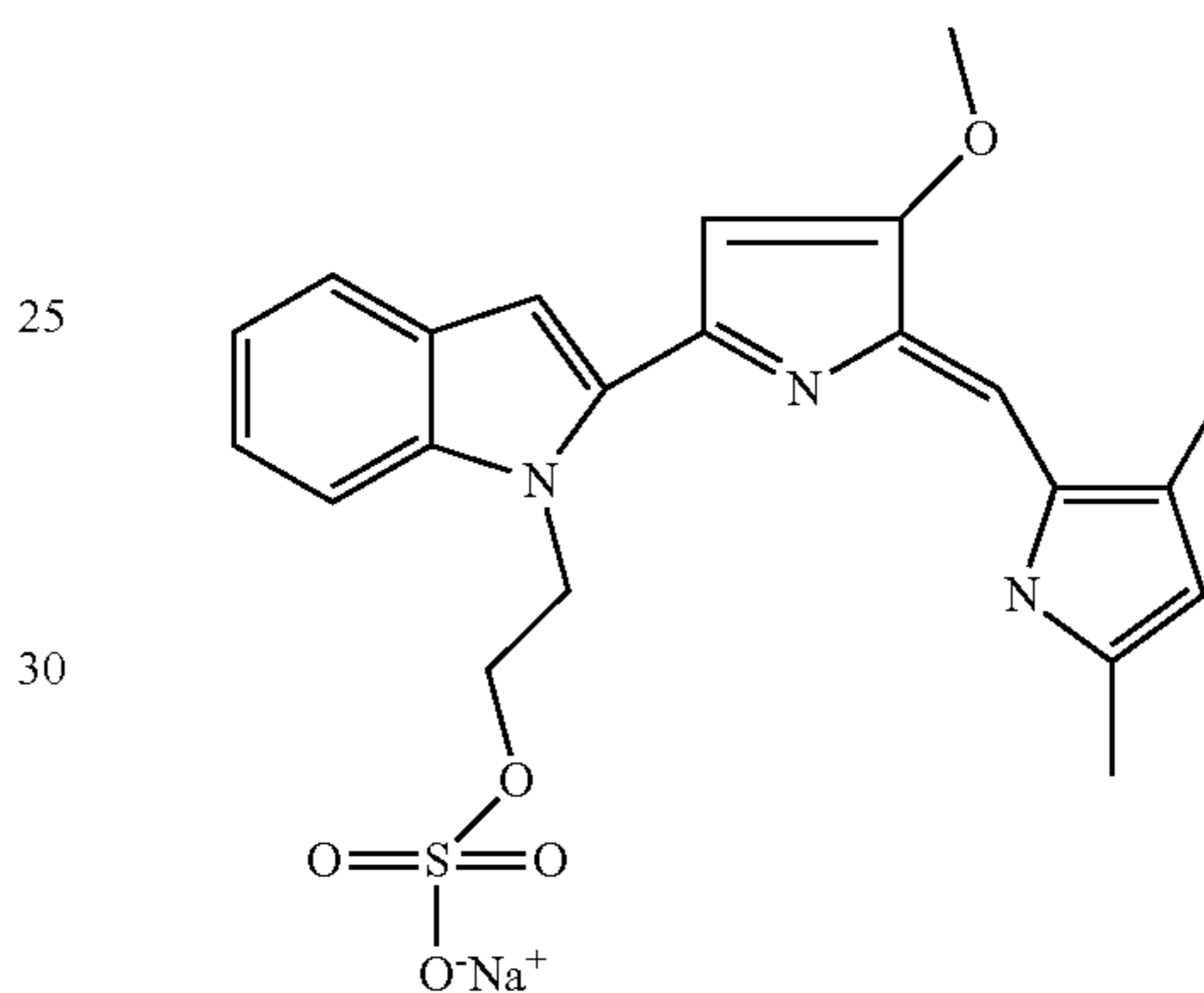
Sodium salt of Sulfuric acid mono-(2-{2-[5-(3,5-dimethyl-1H-pyrrol-2-ylmethylene)-4-methoxy-5H-pyrrol-2-yl]-indol-1-yl}-ethyl) ester
