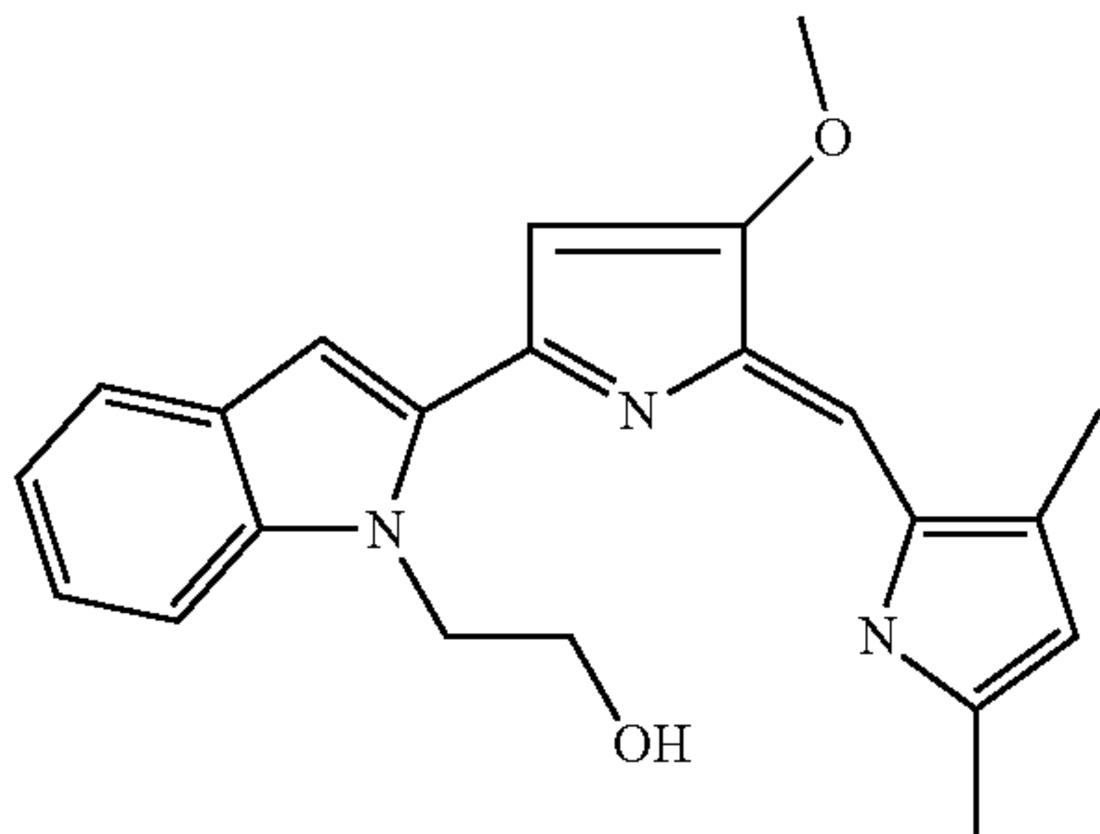
2-{2-[5-(3,5-Dimethyl-1H-pyrrol-2-ylmethylene)-4-methoxy-5H-pyrrol-2-yl]-indol-1-yl}-ethanol
