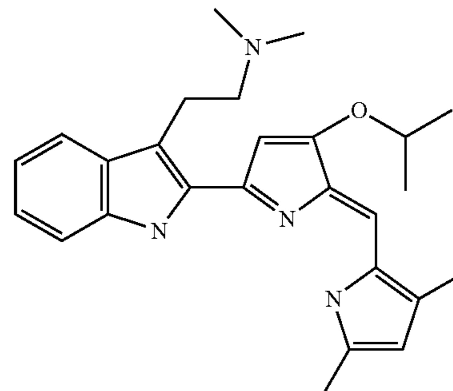
(2-{2-[5-(3,5-Dimethyl-1H-pyrrol-2-ylmethylene)-4-isopropoxy-5H-pyrrol-2-yl]-1H-indol-3-yl}-ethyl)dimethyl-amine
