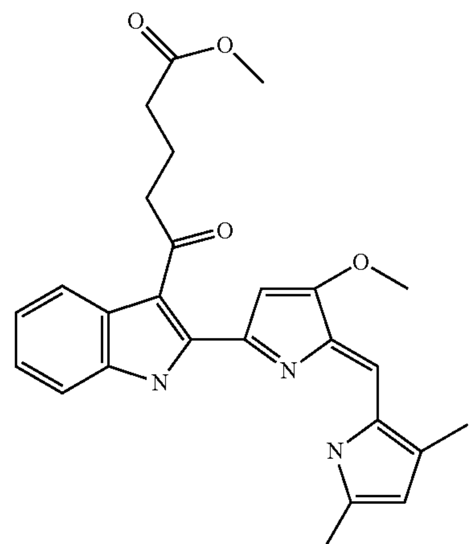
5-(2-[5-(3,5-Dimethyl-1H-pyrrol-2-ylmethylene)-4-methoxy-5H-pyrrol-2-yl]-1H-indol-3-yl)-5-oxo-pentanoic acid methyl ester
