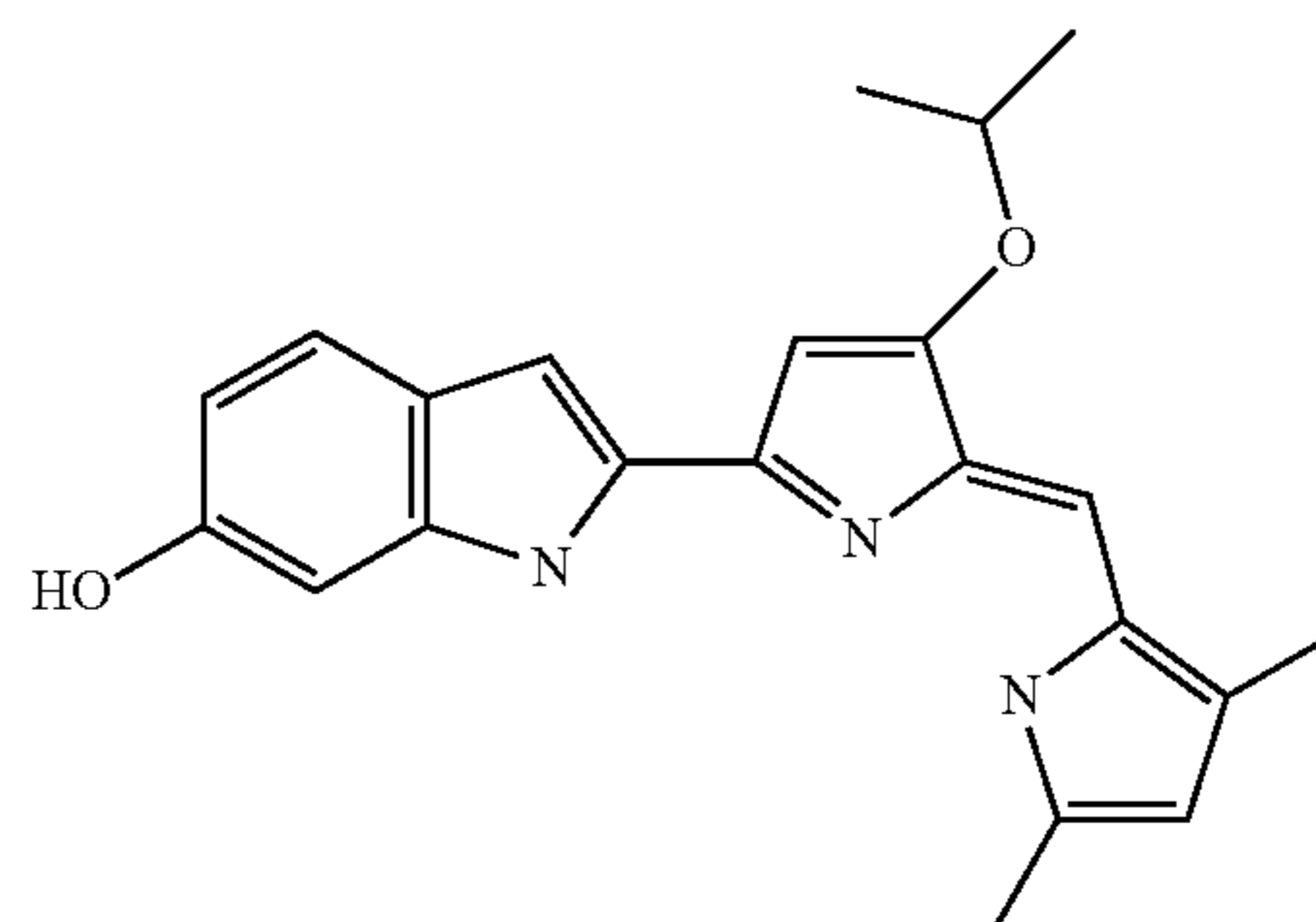
2-[5-(3,5-Dimethyl-1H-pyrrol-2-ylmethylene)-4-isopropoxy-5H-pyrrol-2-yl]-1H-indol-6-ol
