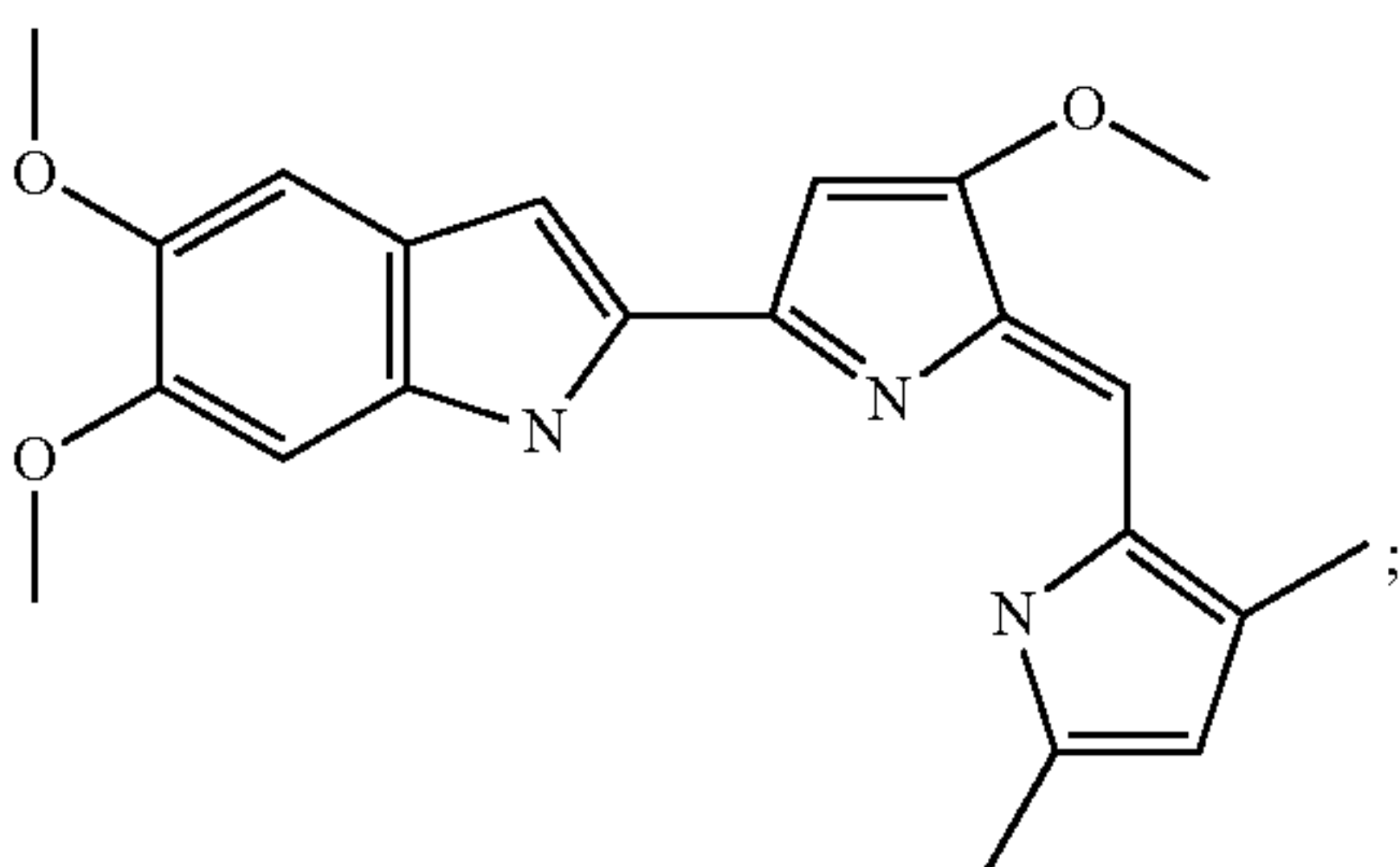
2-[5-(3,5-Dimethyl-1H-pyrrol-2-ylmethylene)-4-methoxy-5H-pyrrol-2-yl]-5,6-dimethoxy-1H-indole
