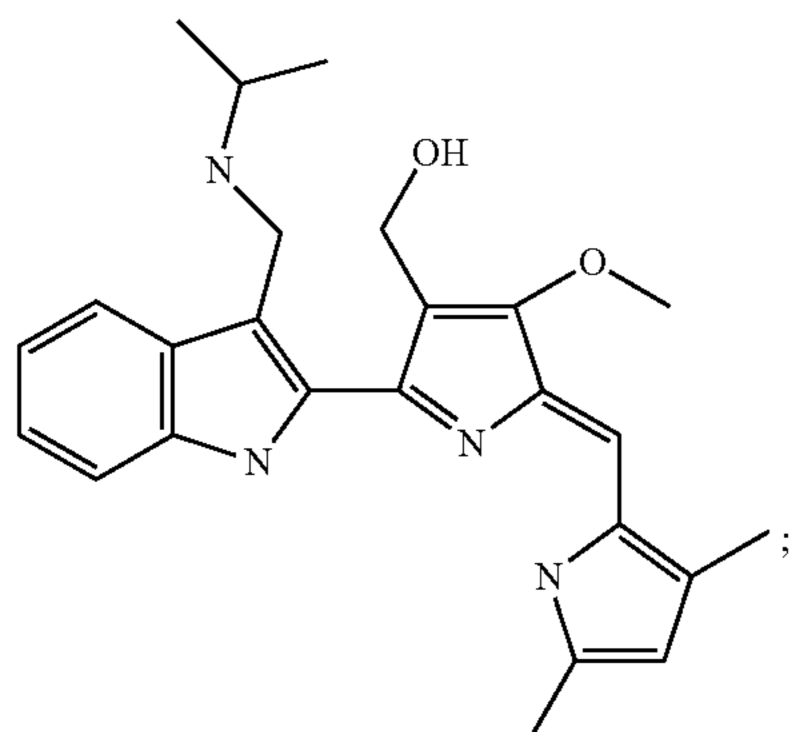
[5-(3,5-Dimethyl-1H-pyrrol-2-ylmethylene)-2-[3-(isopropylamino-methyl)-1H-indol-2-yl]-4-methoxy-5H-pyrrol-3-yl]-methanol
