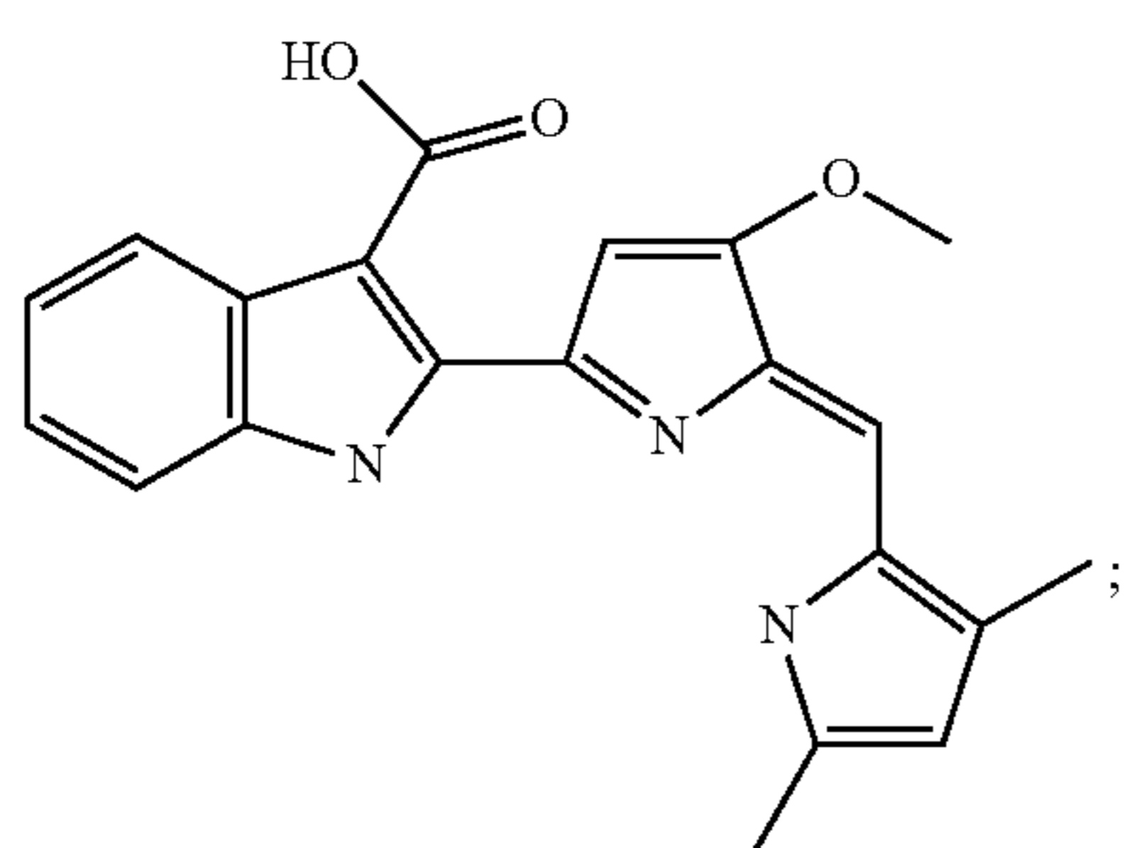
2-[5-(3,5-Dimethyl-1H-pyrrol-2-ylmethylene)-4-methoxy-5H-pyrrol-2-yl]-1H-indole-3-carboxylic acid
