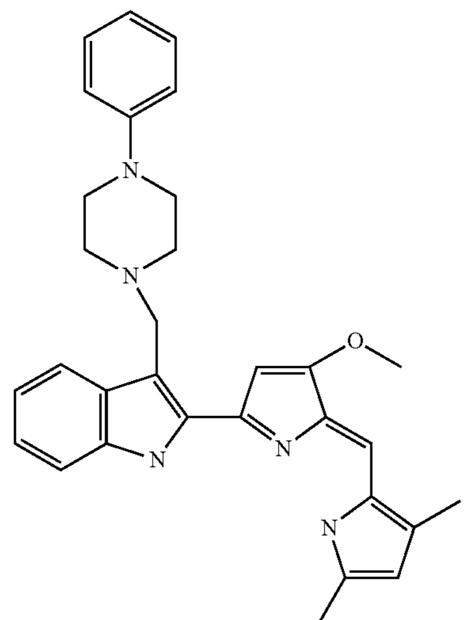
2-[5-(3,5-Dimethyl-1H-pyrrol-2-ylmethylene)-4-methoxy-5H-pyrrol-2-yl]-3-(4-phenylpiperazin-1-ylmethyl)-1H-indole
