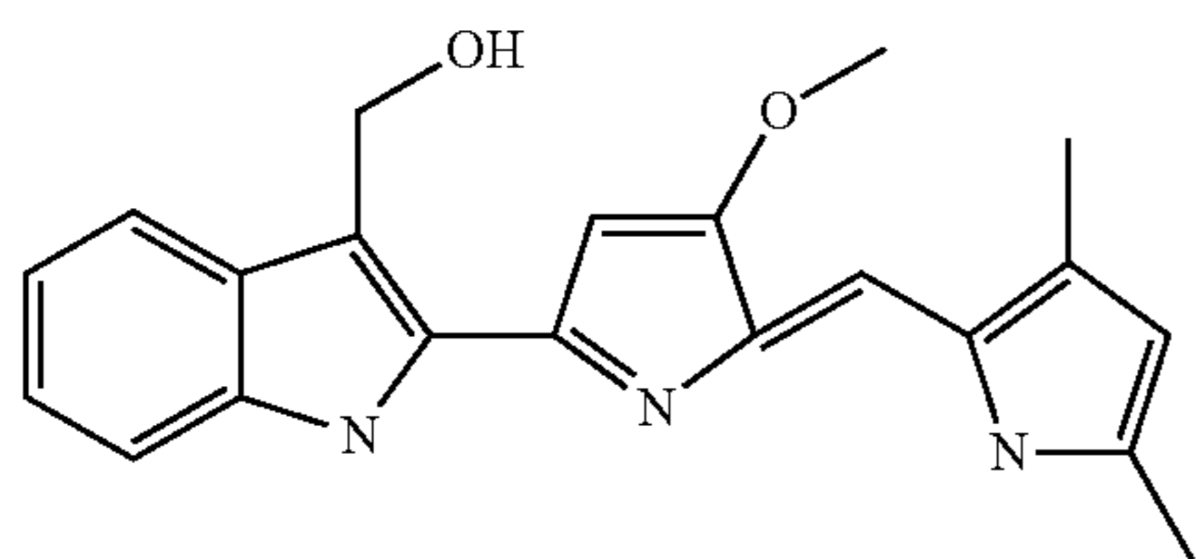
{2-[5-(3,5-Dimethyl-1H-pyrrol-2-ylmethylene)-4-methoxy-5H-pyrrol-2-yl]-1H-indol-3-yl}-methanol
