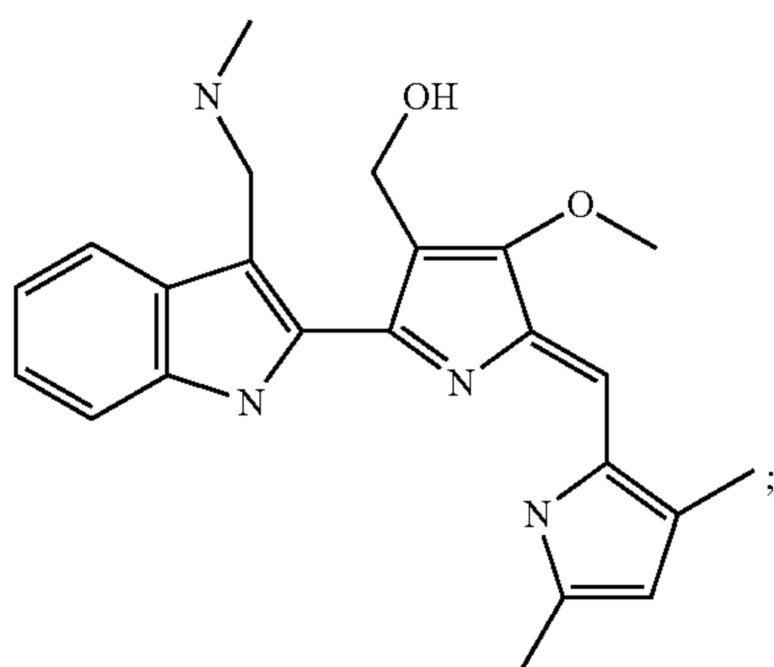
[5-(3,5-Dimethyl-1H-pyrrol-2-ylmethylene)-4-methoxy-2-(3-methylaminomethyl)-1H-indol-2-yl]-5H-pyrrol-3-yl]-methanol
