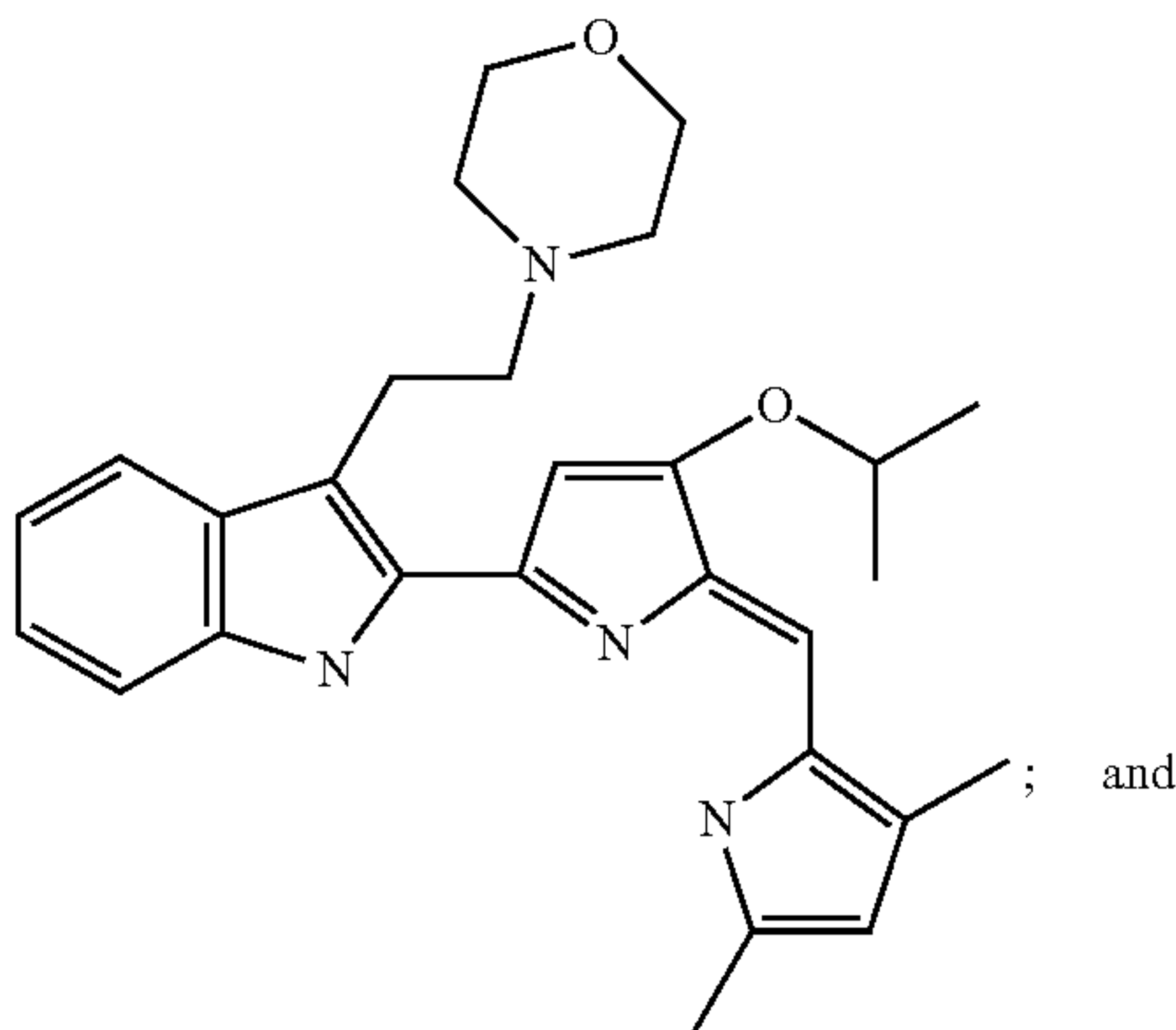
2-[5-(3,5-Dimethyl-1H-pyrrol-2-ylmethylene)-4-isopropoxy-5H-pyrrol-2-yl]-3-(2-morpholin-4-yl-ethyl)-1H-indole
