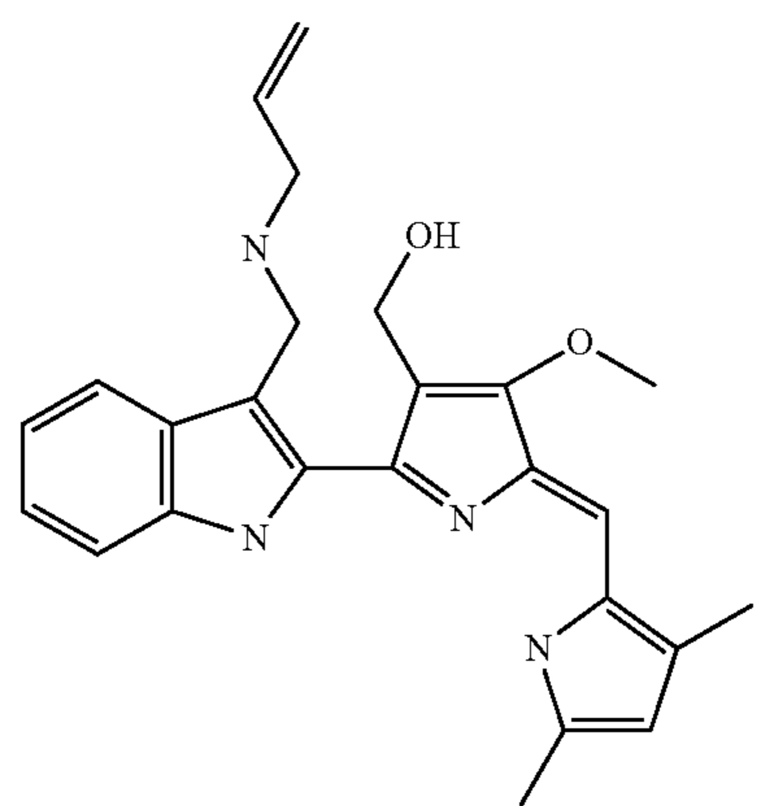
[2-(3-Allylaminomethyl)-1H-indol-2-yl]-5-(3,5-dimethyl-1H-pyrrol-2-ylmethylene)-4-methoxy-5H-pyrrol-3-yl]-methanol
