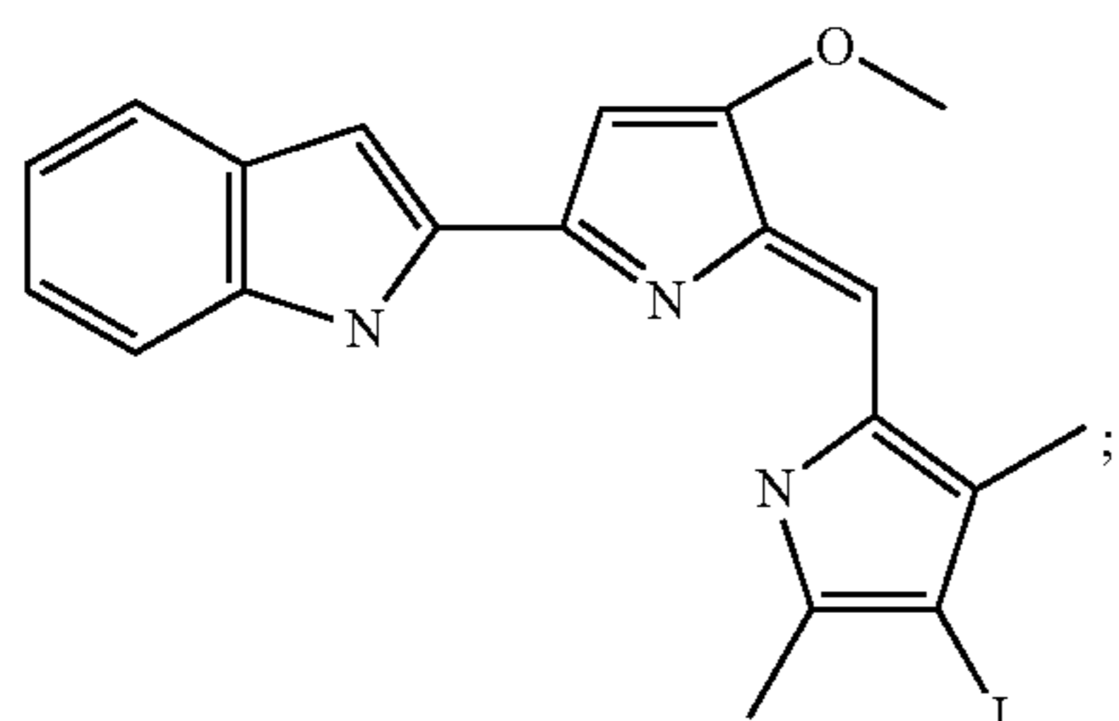
2-[5-(4-Iodo-3,5-dimethyl-1H-pyrrol-2-ylmethylene)-4-methoxy-5H-pyrrol-2-yl]-1H-indole
