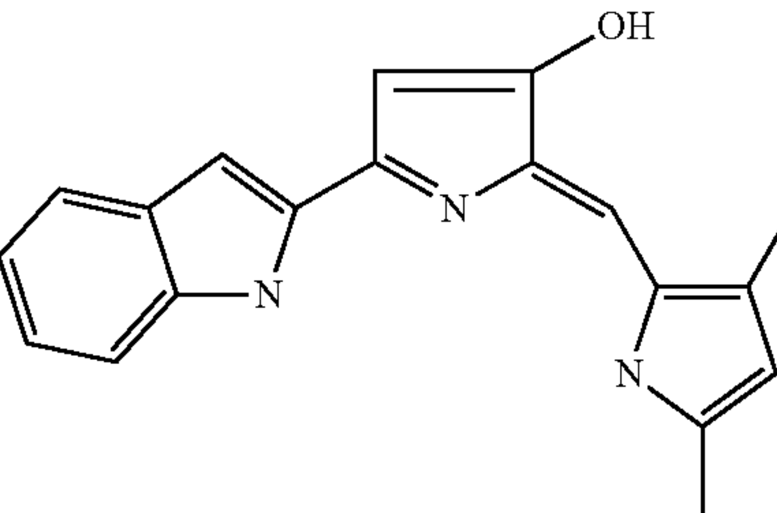
2-(3,5-Dimethyl-1H-pyrrol-2-ylmethylene)-5-(1H-indol-2-yl)-2H-pyrrol-3-ol
