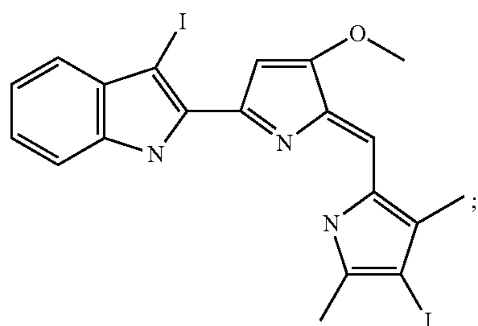
3-Iodo-2-[5-(4-iodo-3,5-dimethyl-1H-pyrrol-2-ylmethylene)-4-methoxy-5H-pyrrol-2-yl]-1H-indole
