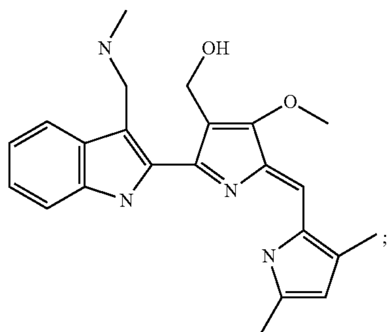
[5-(3,5-Dimethyl-1H-pyrrol-2-ylmethylene)-4-methoxy-2-(3-methylaminomethyl)-1H-indol-2-yl]-5H-pyrrol-3-yl]-methanol
