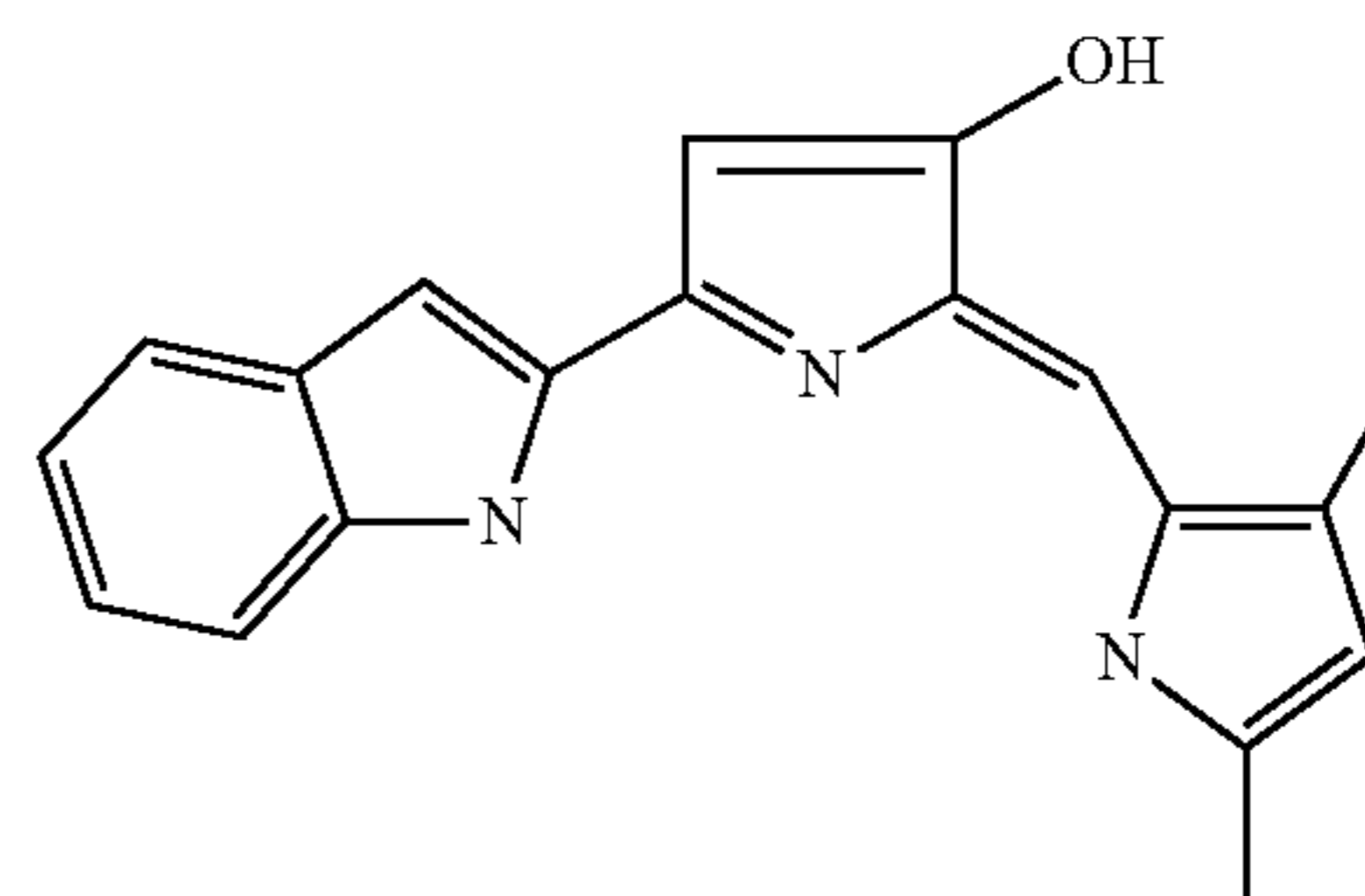
2-(3,5-Dimethyl-1H-pyrrol-2-ylmethylene)-5-(1H-indol-2-yl)-2H-pyrrol-3-ol
