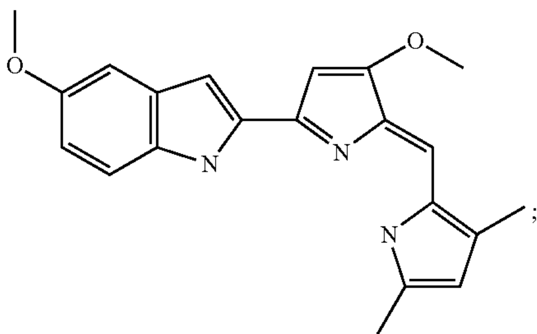
2-[5-(3,5-Dimethyl-1H-pyrrol-2-ylmethylene)-4-methoxy-5H-pyrrol-2-yl]-5-methoxy-1H-indole
