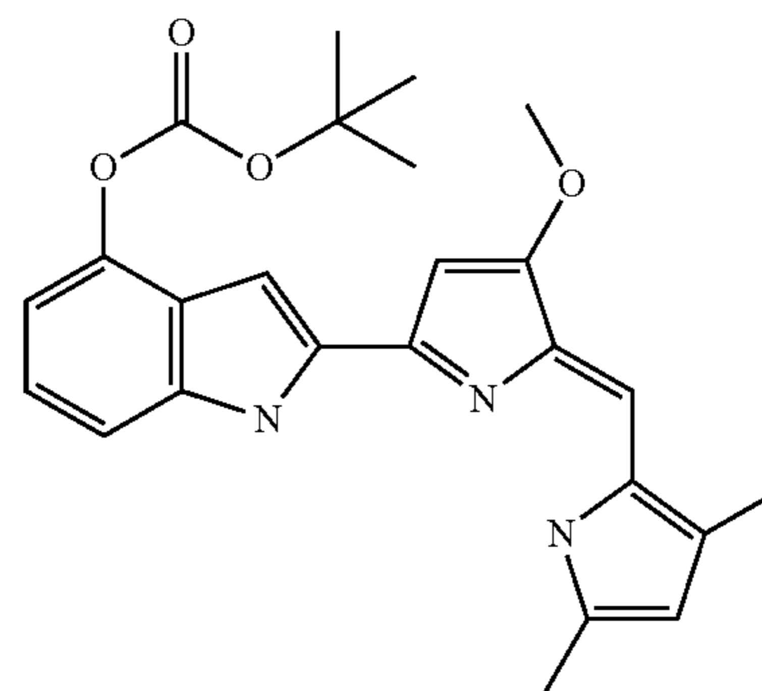
Carbonic acid tert-butyl ester 2-[5-(3,5-dimethyl-1H-pyrrol-2-ylmethylene)-4-methoxy-5H-pyrrol-2-yl]-1H-indol-4-yl ester
