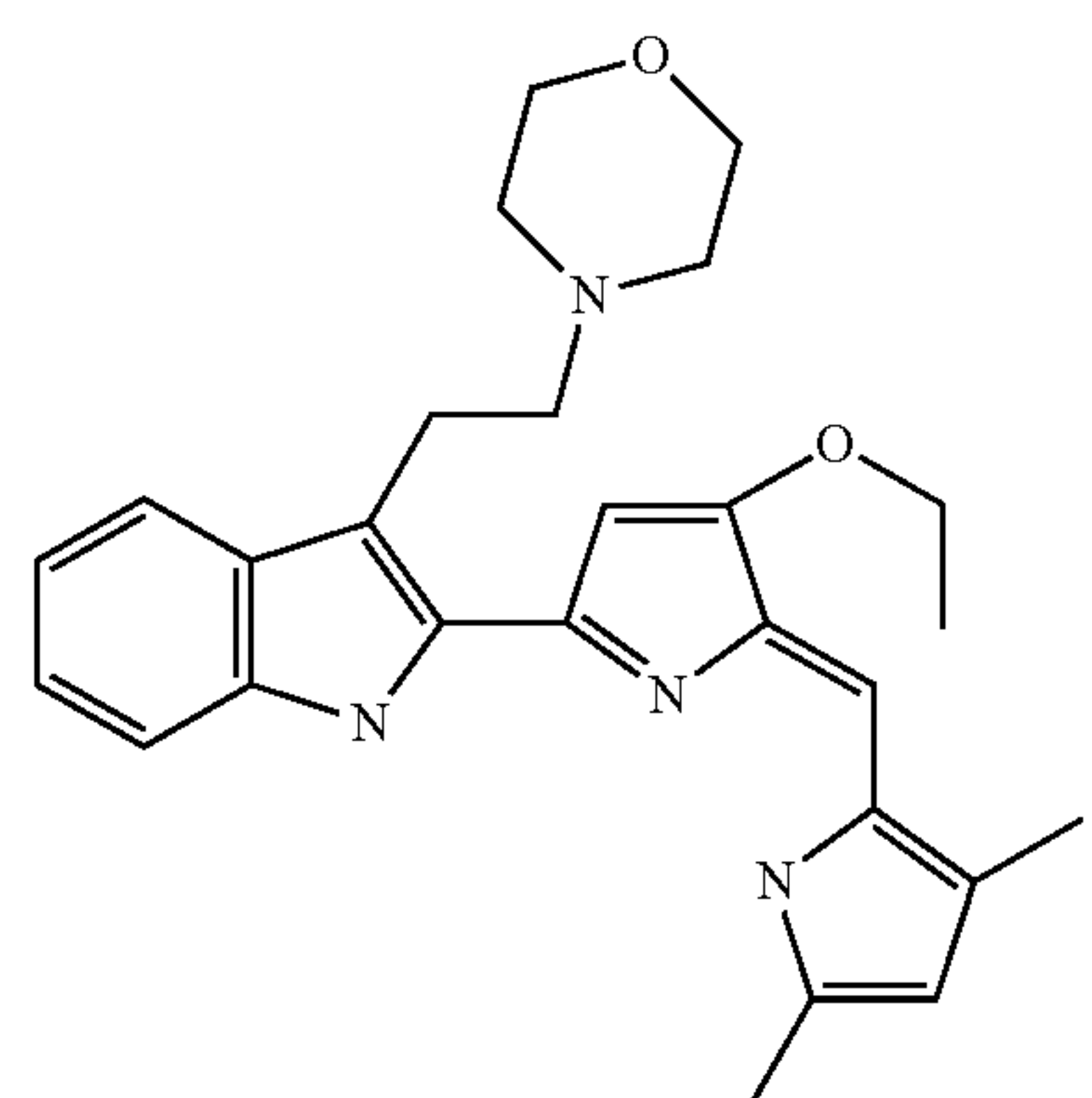
2-[5-(3,5-Dimethyl-1H-pyrrol-2-ylmethylene)-4-ethoxy-5H-pyrrol-2-yl]-3-(2-morpholin-4-ylethyl)-1H-indole
