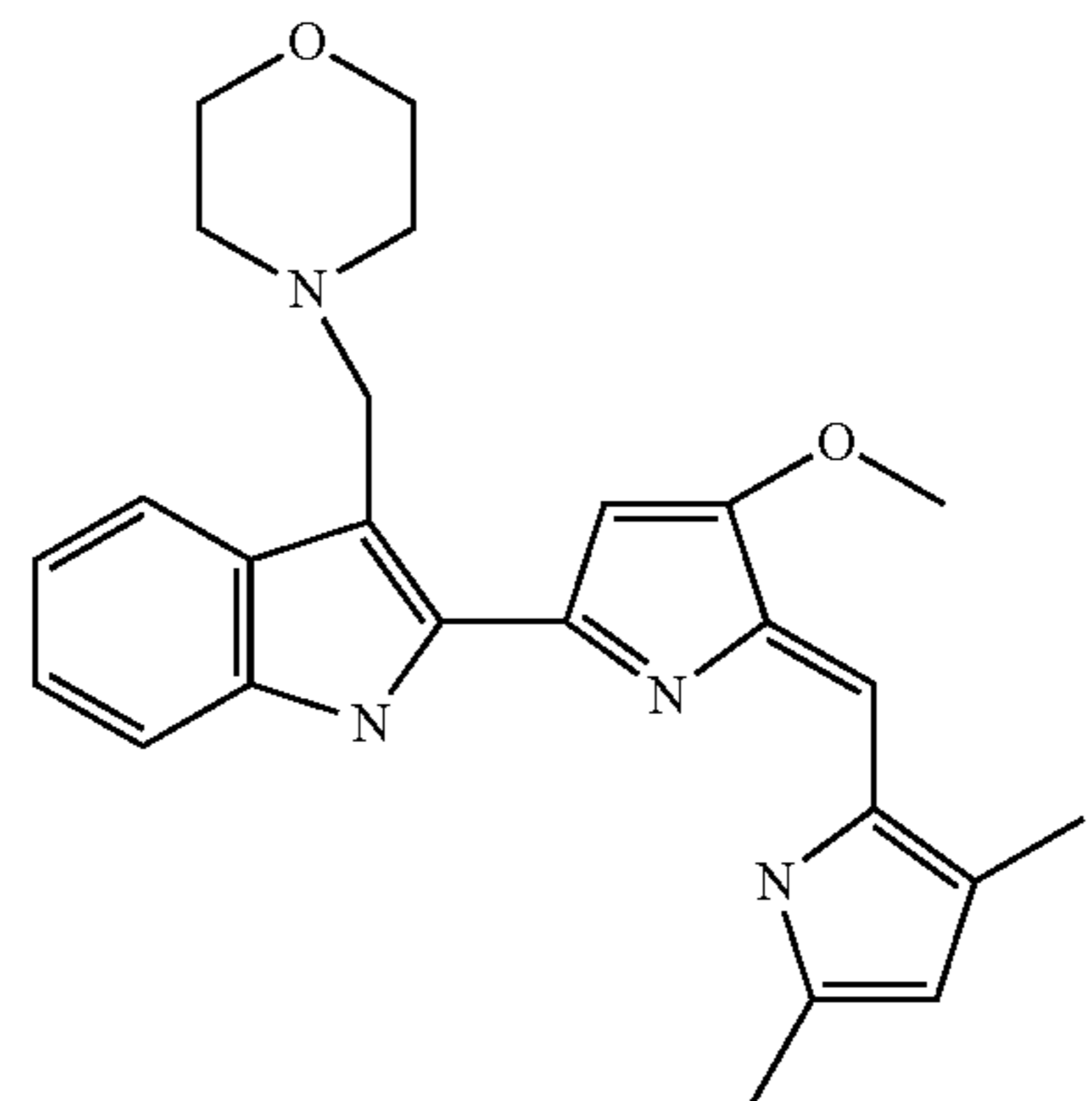
2-[5-(3,5-Dimethyl-1H-pyrrol-2-ylmethylene)-4-methoxy-5H-pyrrol-2-yl]-3-morpholin-4-ylmethyl-1H-indole
