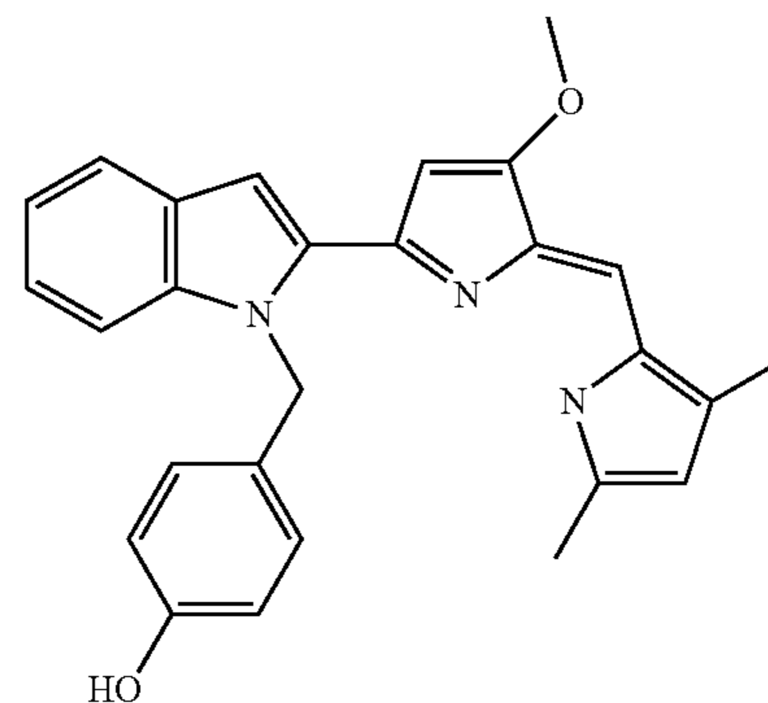
4-{2-[5-(3,5-Dimethyl-1H-pyrrol-2-ylmethylene)-4-methoxy-5H-pyrrol-2-yl]-indol-1-ylmethyl}-phenol
