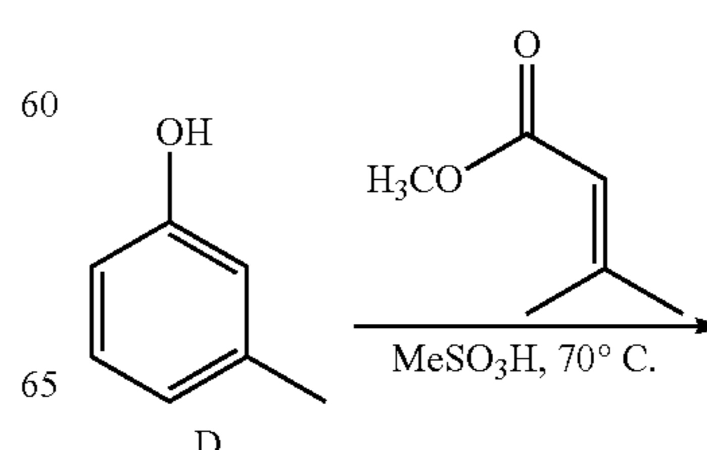
Scheme 3
