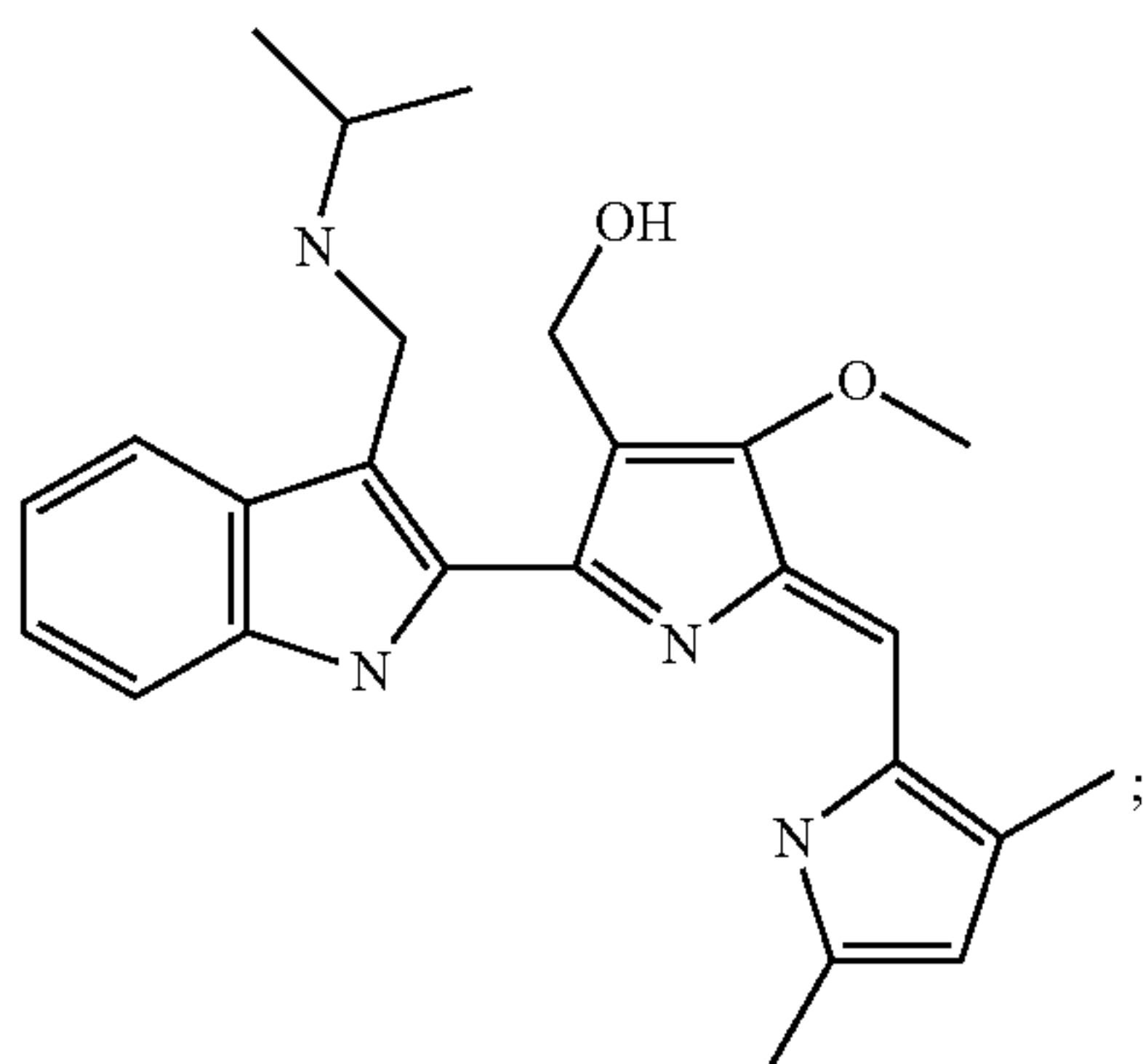
{5-(3,5-Dimethyl-1H-pyrrol-2-ylmethylene)-2-[3-(isopropylamino-methyl)-1H-indol-2-yl]-4-methoxy-5H-pyrrol-3-yl}-methanol
