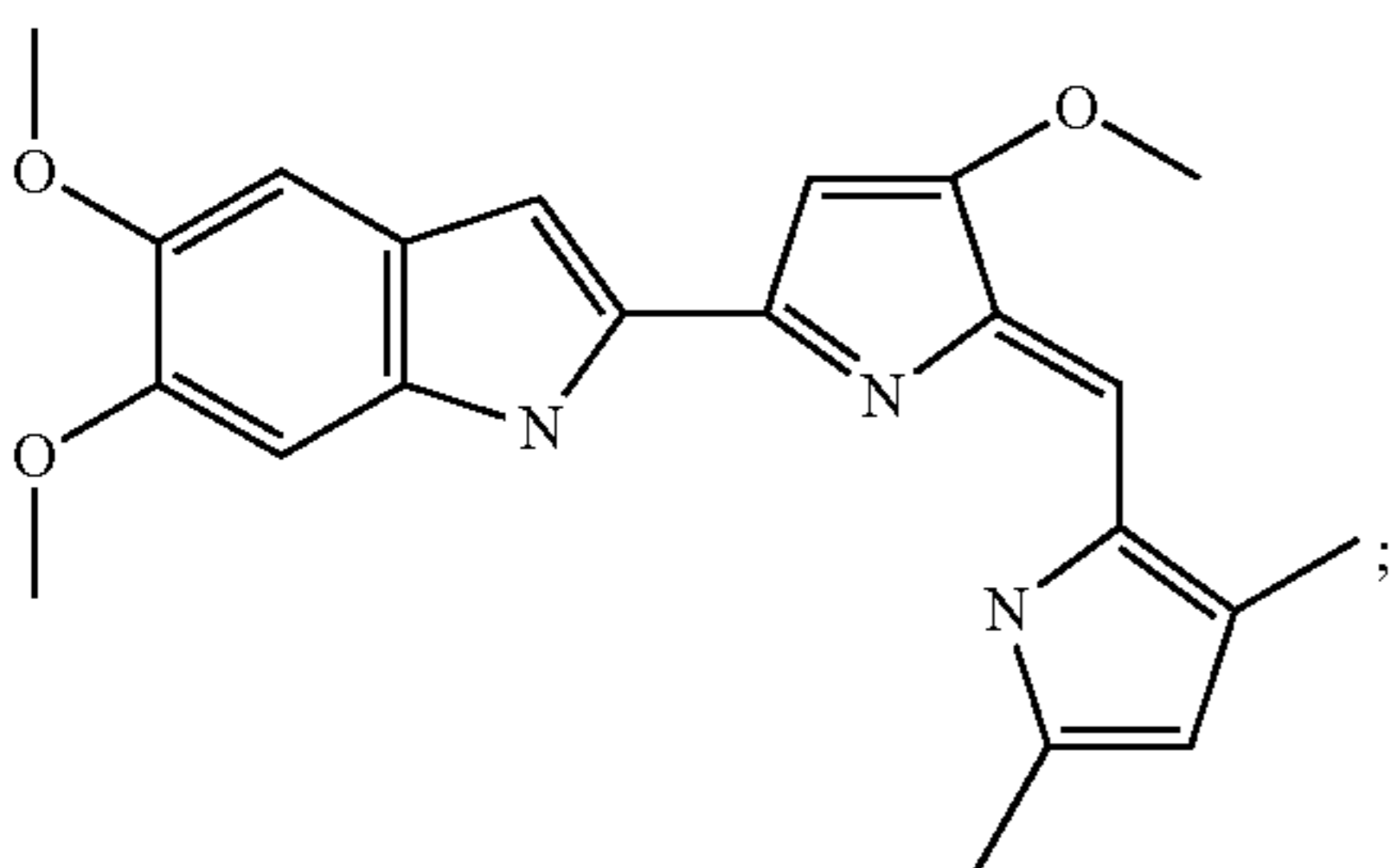
2-[5-(3,5-Dimethyl-1H-pyrrol-2-ylmethylene)-4-methoxy-5H-pyrrol-2-yl]-5,6-dimethoxy-1H-indole
