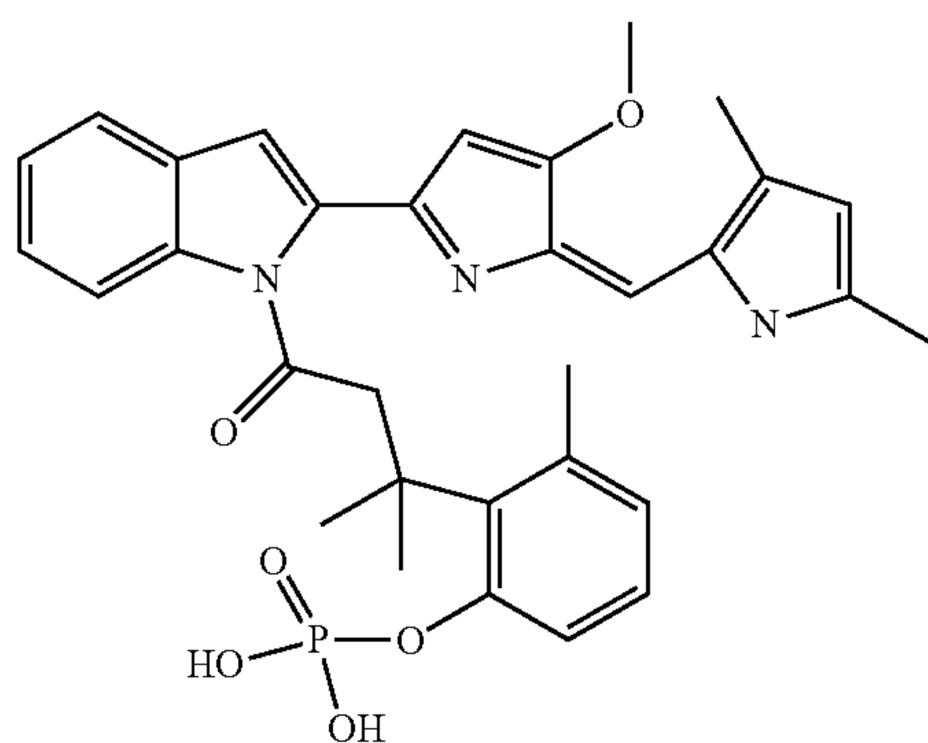
Phosphoric acid mono-[2-(3-(2-[5-(3,5-dimethyl-1H-pyrrol-2-yl)methylene)-4-methoxy-5H-pyrrol-2-yl]-indol-1-yl)-1, 1-dimethyl-3-oxo-propyl]-3-methyl-phenyl ester
