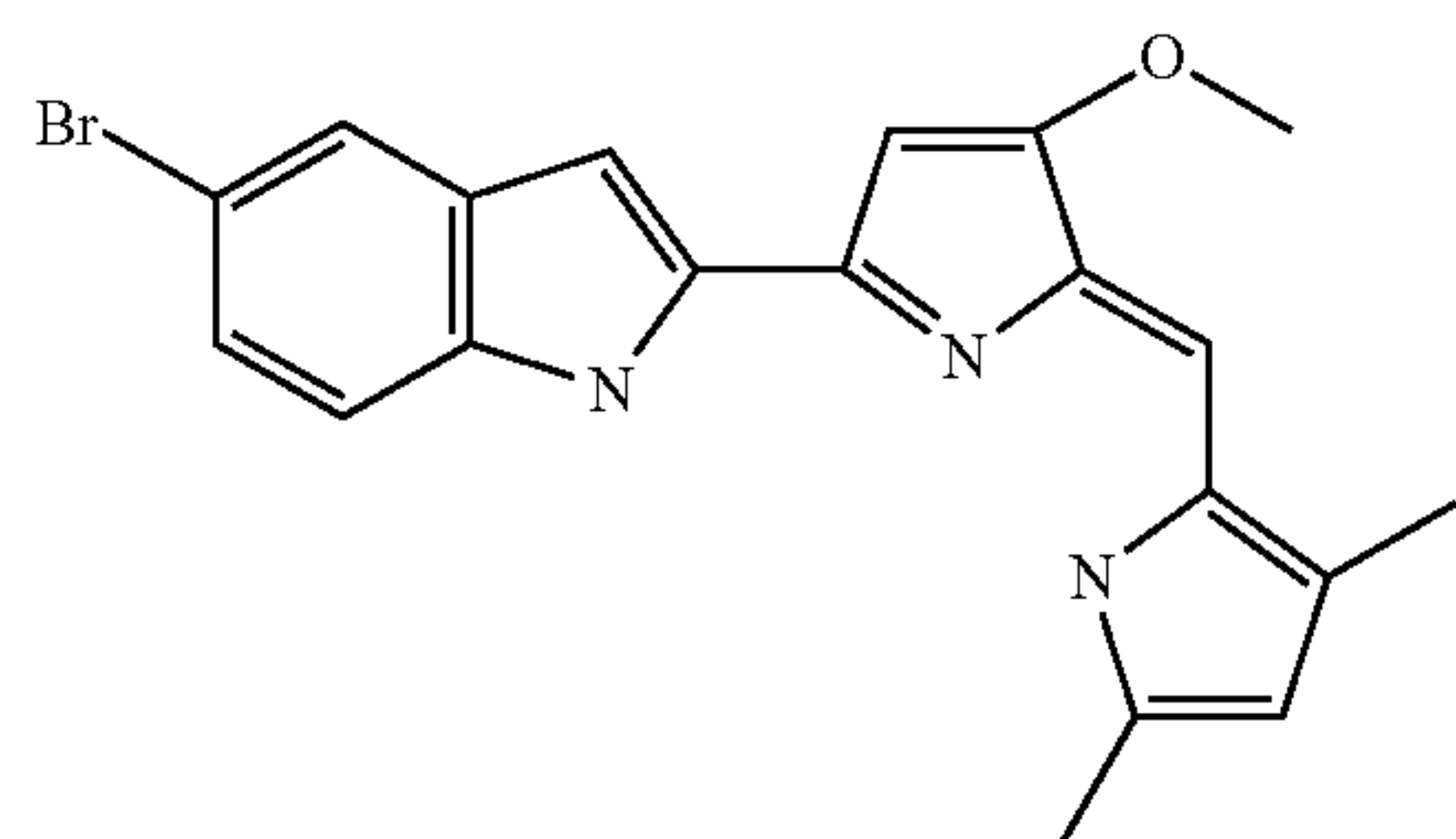
5-Bromo-2-[5-(3,5-dimethyl-1H-pyrrol-2-ylmethylene)-4-methoxy-5H-pyrrol-2-yl]-1H-indole
