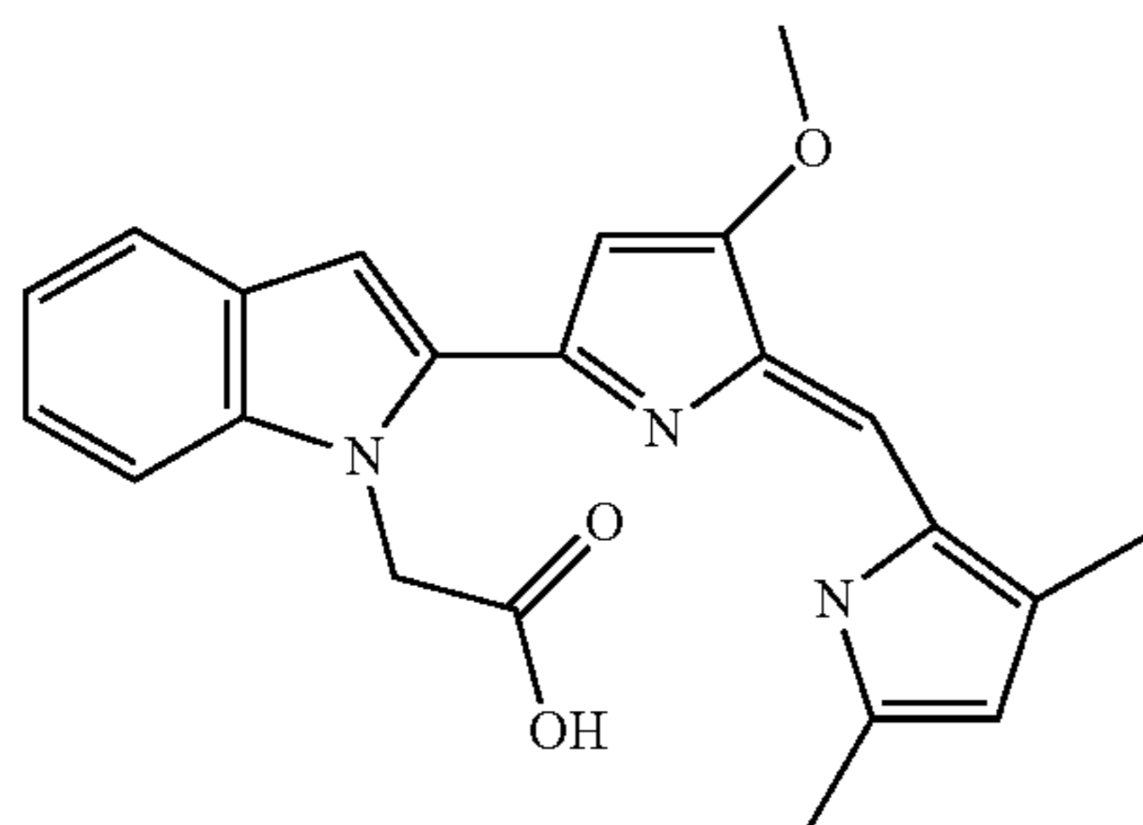
{2-[5-(3,5-Dimethyl-1H-pyrrol-2-ylmethylene)-4-methoxy-5H-pyrrol-2-yl]-indol-1-yl}-acetic acid
