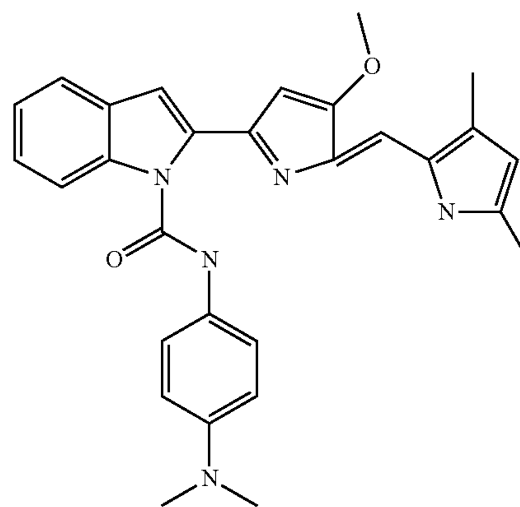
2-[5-(3,5-Dimethyl-1H-pyrrol-2-ylmethylene)-4-methoxy-5H-pyrrol-2-yl]-indole-1-carboxylic acid (4-dimethylamino-phenyl)-amide
