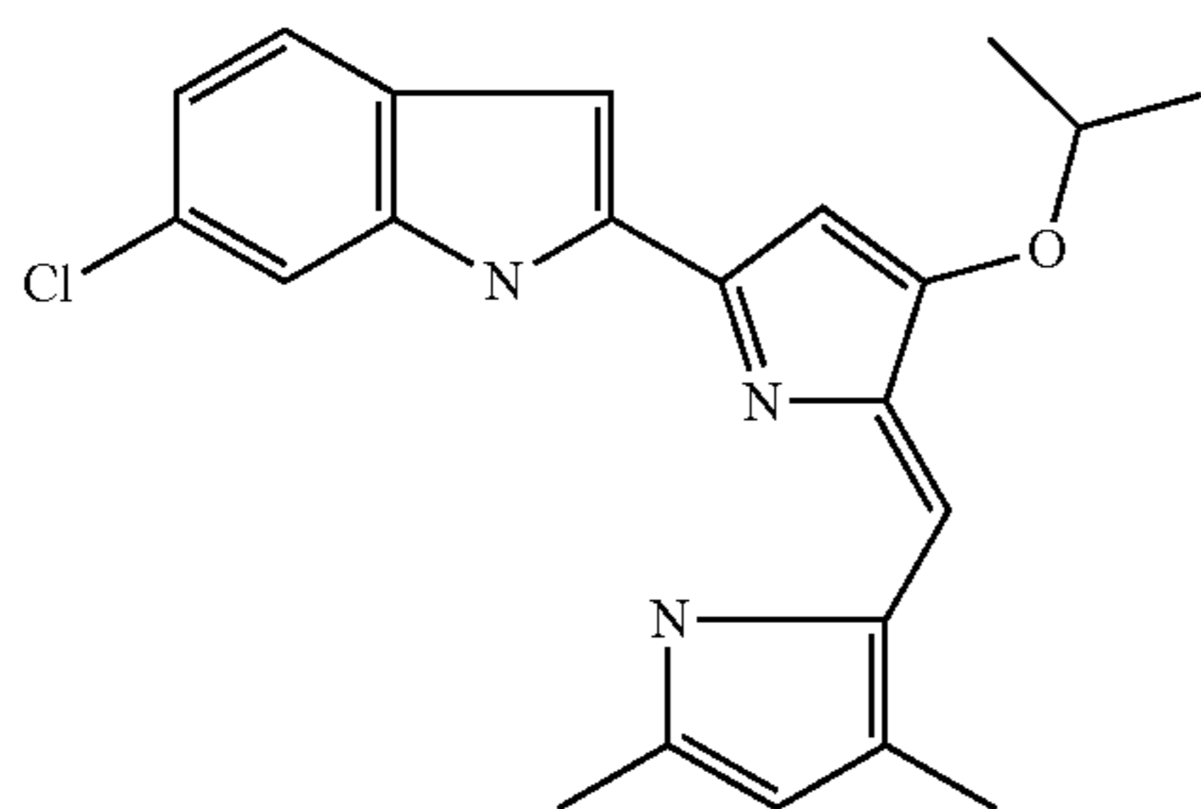
6-Chloro-2-[5-(3,5-dimethyl-1H-pyrrol-2-ylmethylene)-4-isopropoxy-5H-pyrrol-2-yl]-1H-indole
