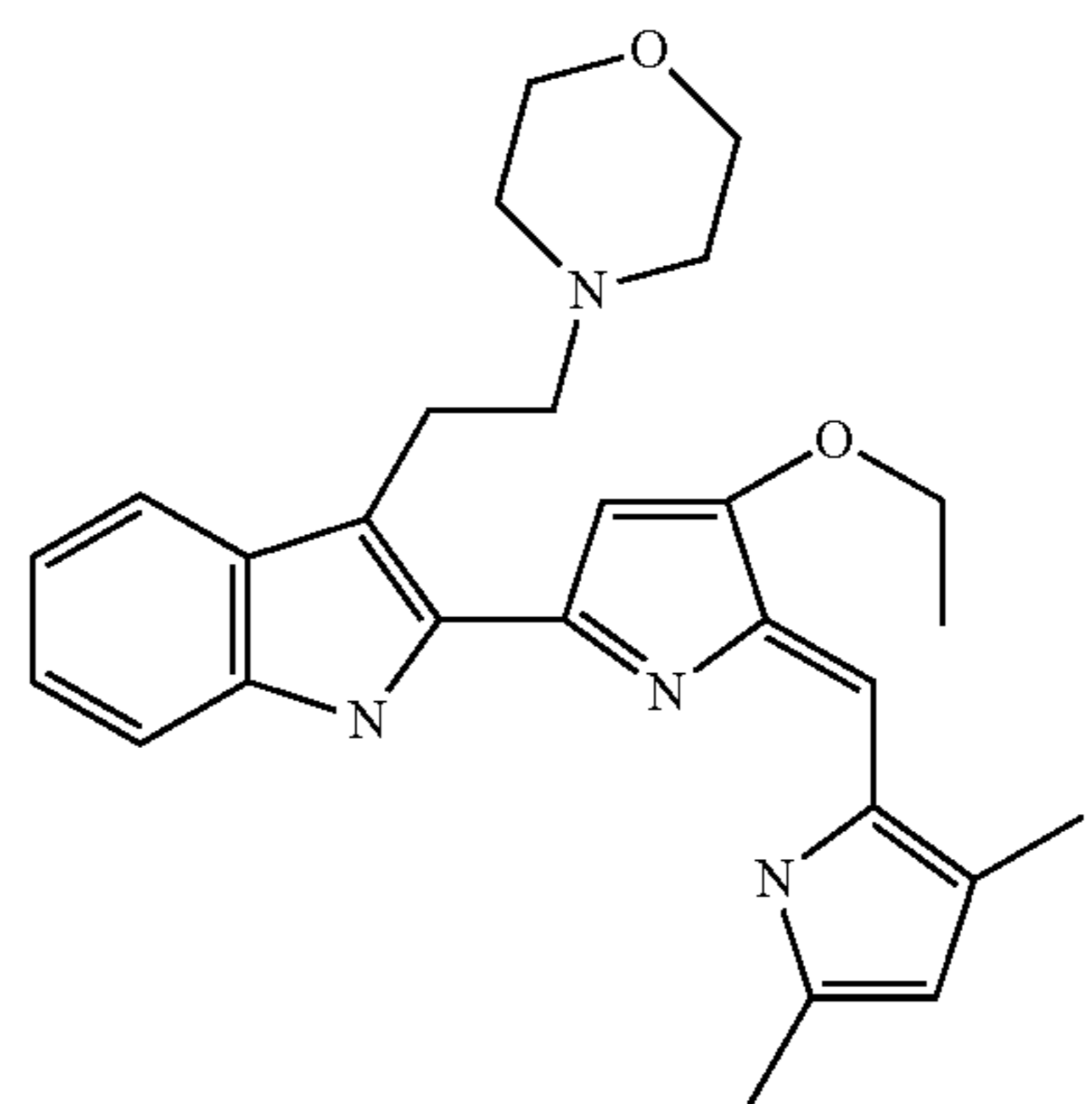
2-[5-(3,5-Dimethyl-1H-pyrrol-2-ylmethylene)-4-ethoxy-5H-pyrrol-2-yl]-3-(2-morpholin-4-ylethyl)-1H-indole
