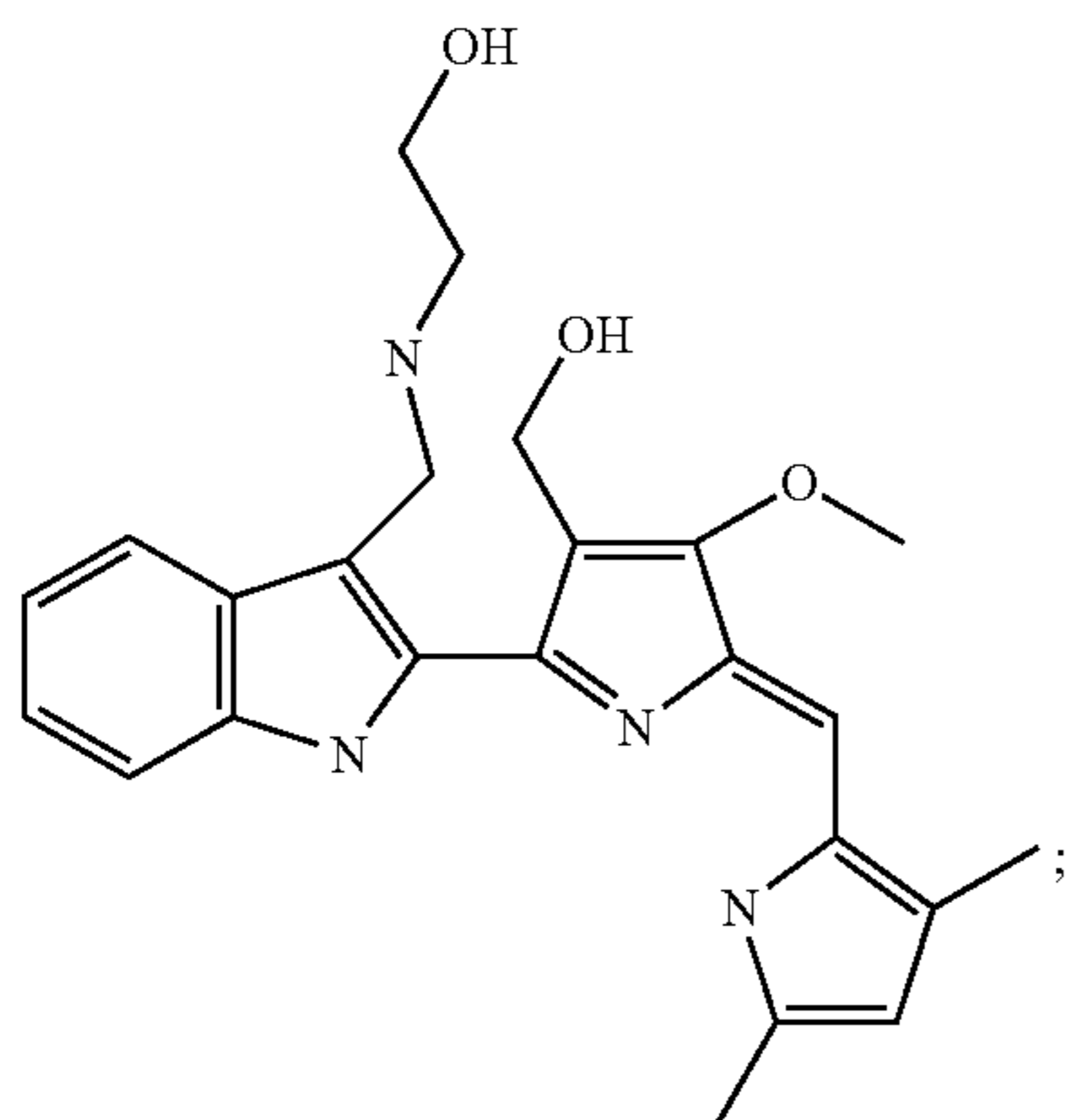
2-((2-[5-(3,5-Dimethyl-1H-pyrrol-2-ylmethylene)-3-hydroxymethyl-4-methoxy-5H-pyrrol-2-yl]-1H-indol-3-ylmethyl)-amino)ethanol
