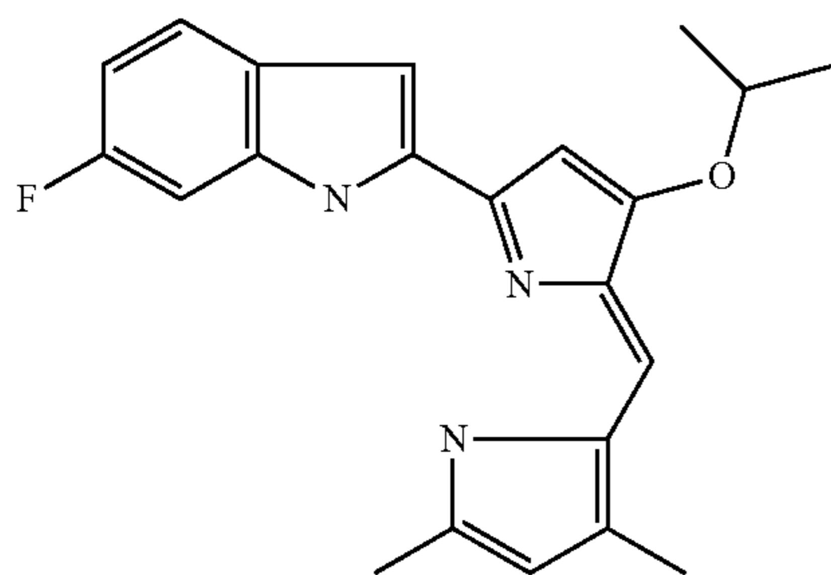
2-[5-(3,5-Dimethyl-1H-pyrrol-2-ylmethylene)-4-isopropoxy-5H-pyrrol-2-yl]-6-fluoro-1H-indole
