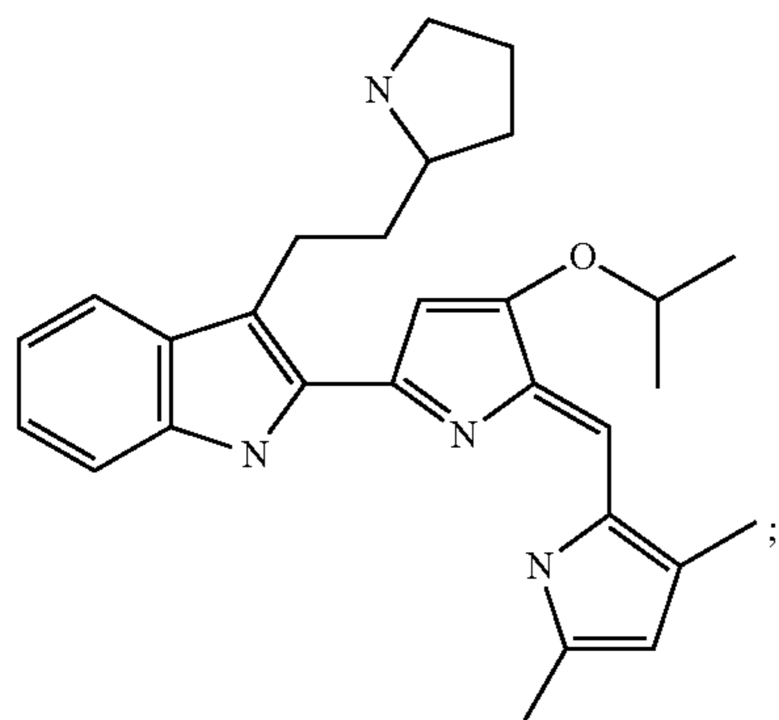
2-[5-(3,5-Dimethyl-1H-pyrrol-2-ylmethylene)-4-isopropoxy-5H-pyrrol-2-yl]-3-(2-pyrrolidin-2-yl-ethyl)-1H-indole
