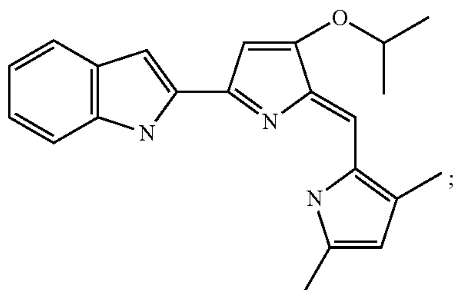
2-[5-(3,5-Dimethyl-1H-pyrrol-2-ylmethylene)-4-isopropoxy-5H-pyrrol-2-yl]-1H-indole
