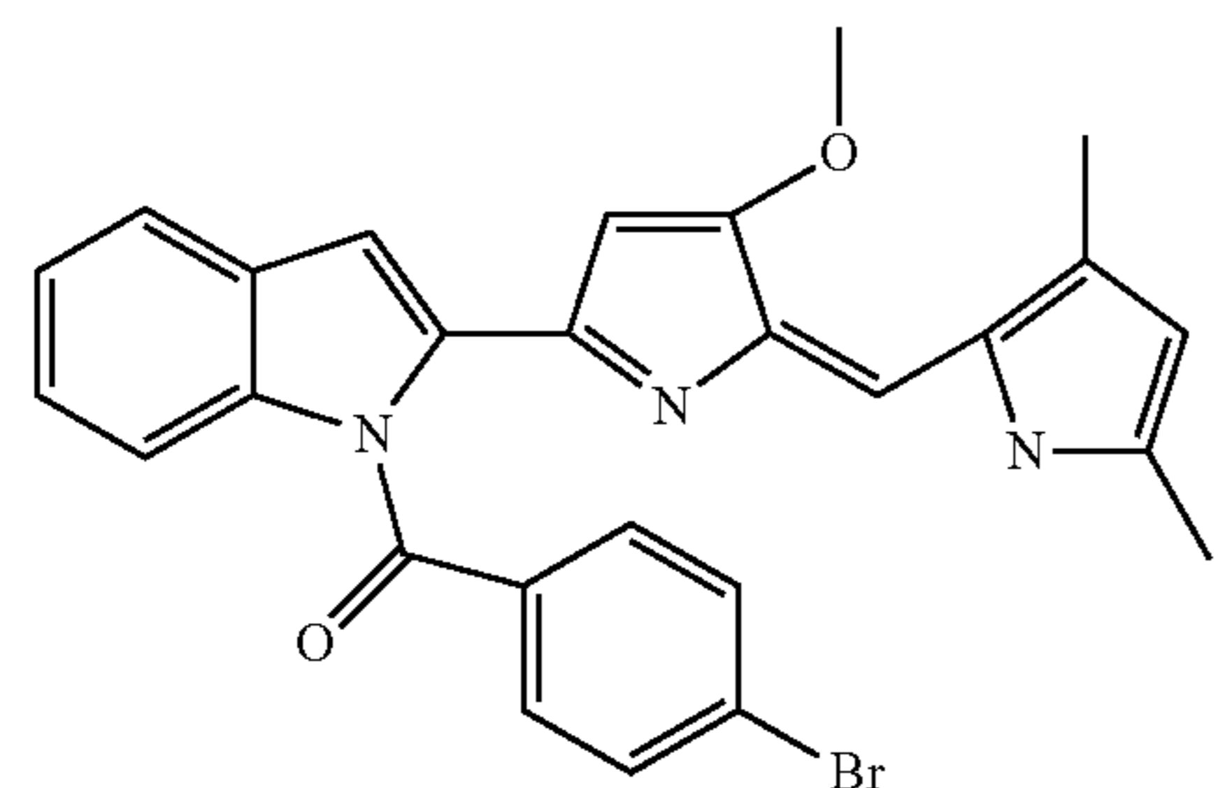
(4-Bromo-phenyl)-{2-[5-(3,5-dimethyl-1H-pyrrol-2-ylmethylene)-4-methoxy-5H-pyrrol-2-yl]-indol-1-yl}-methanone
