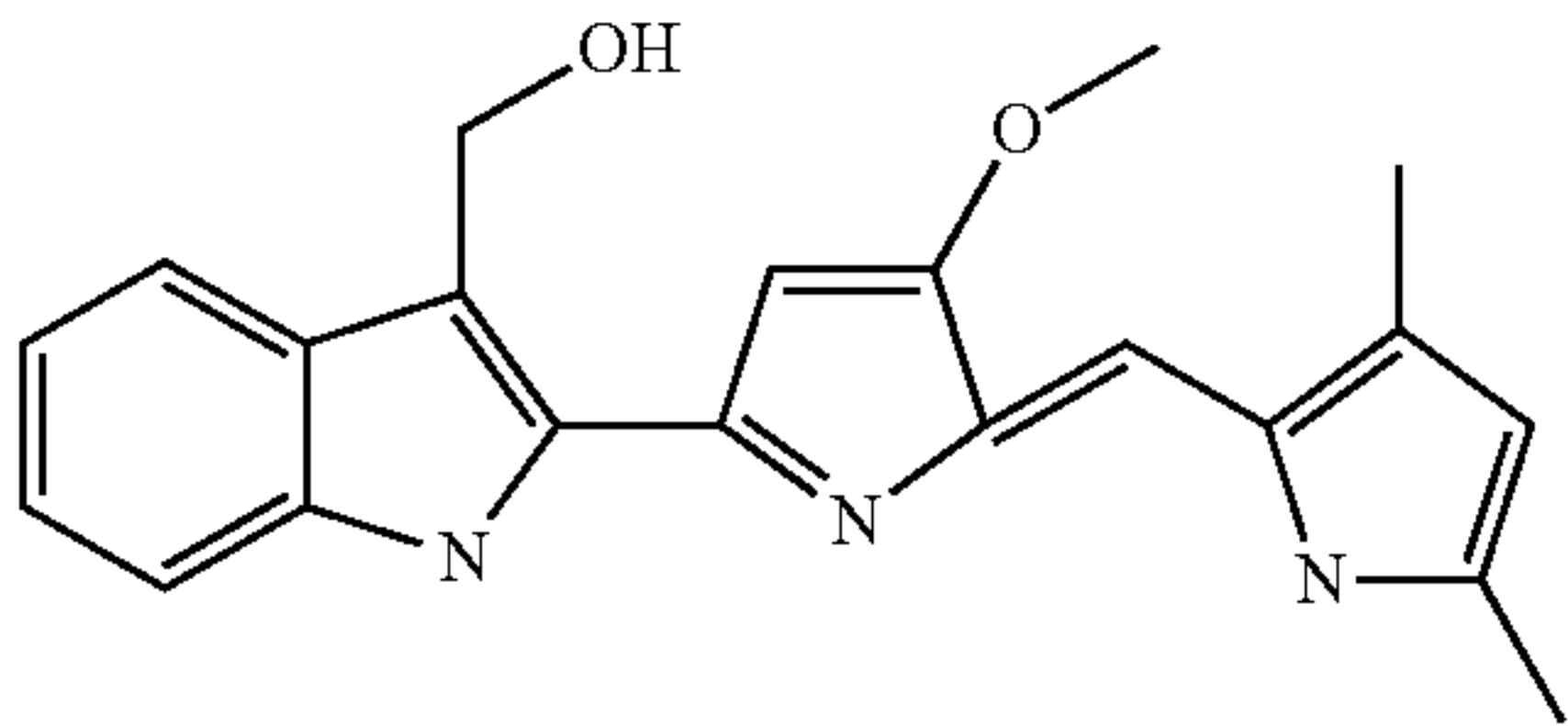
{2-[5-(3,5-Dimethyl-1H-pyrrol-2-ylmethylene)-4-methoxy-5H-pyrrol-2-yl]-1H-indol-3-yl}-methanol
