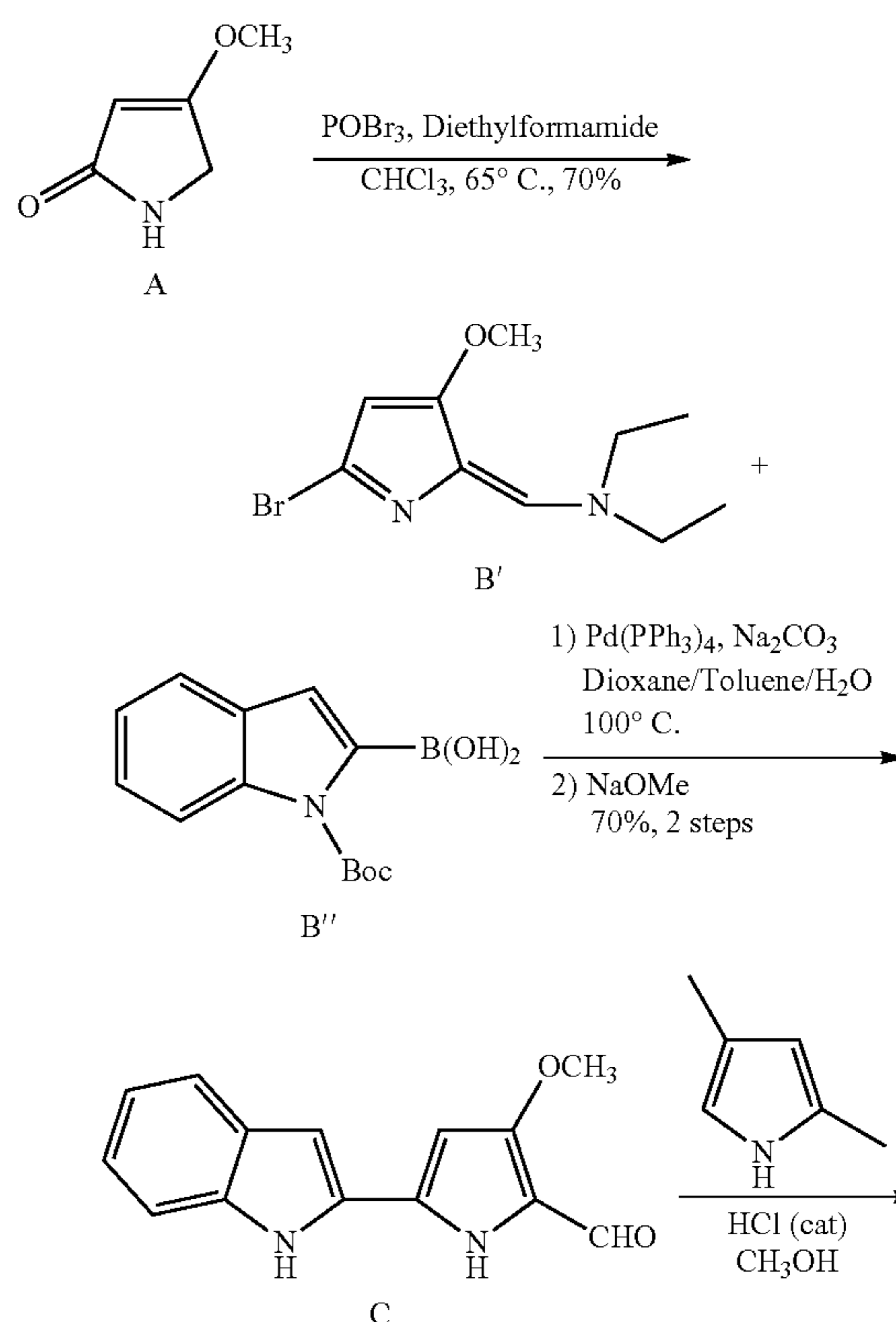
Scheme 2b
