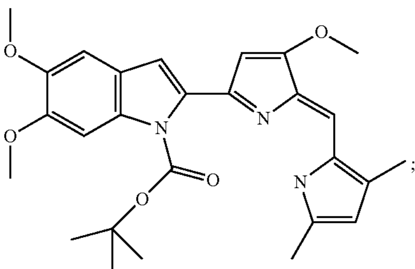
2-[5-(3,5-Dimethyl-1H-pyrrol-2-ylmethylene)-4-methoxy-5H-pyrrol-2-yl]-5,6-dimethoxy-indole-1-carboxylic acid tert-butyl ester
