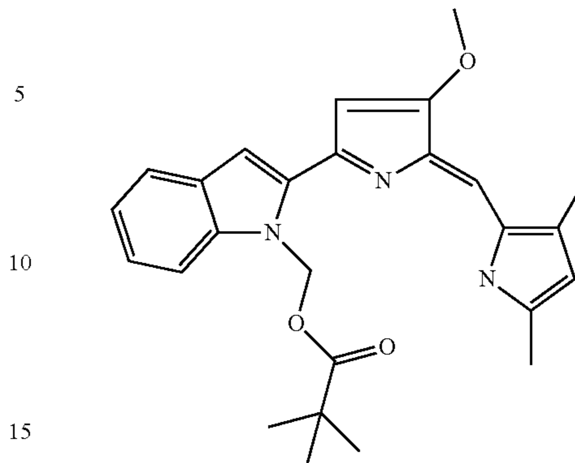
2,2-Dimethyl-propionic acid 2-[5-(3,5-dimethyl-1H-pyrrol-2-ylmethylene)-4-methoxy-5H-pyrrol-2-yl]-indol-1-ylmethyl ester
