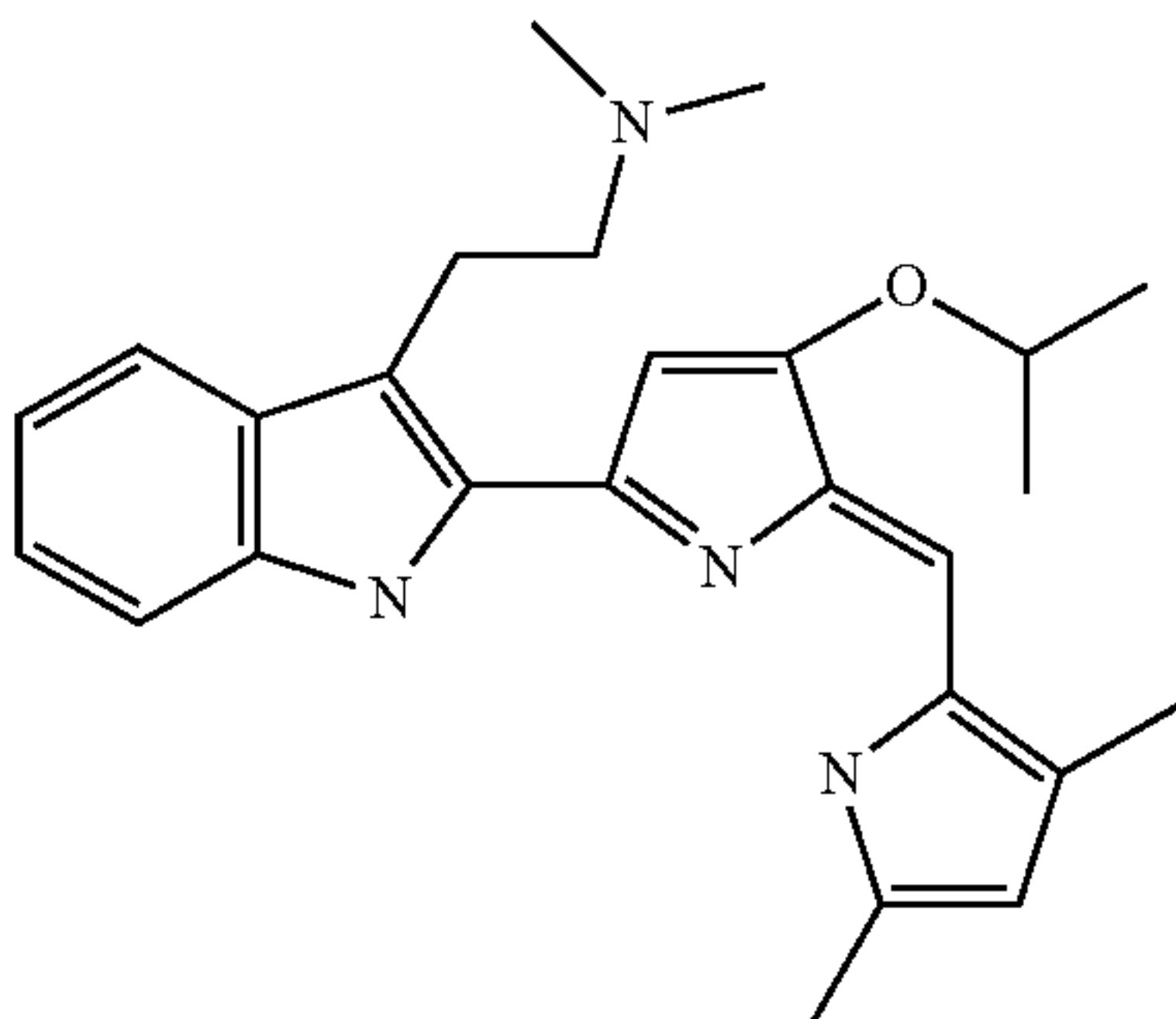
(2-{2-[5-(3,5-Dimethyl-1H-pyrrol-2-ylmethylene)-4-isopropoxy-5H-pyrrol-2-yl]-1H-indol-3-yl}-ethyl)dimethyl-amine
