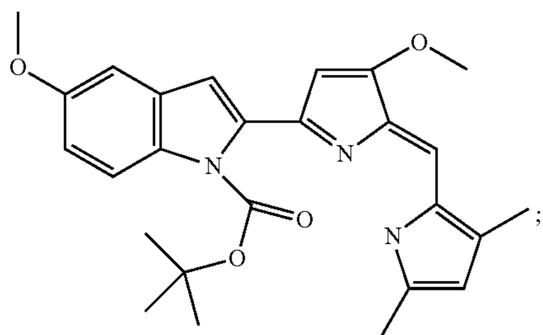
2-[5-(3,5-Dimethyl-1H-pyrrol-2-ylmethylene)-4-methoxy-5H-pyrrol-2-yl]-5-methoxy-indole-1-carboxylic acid tert-butyl ester
