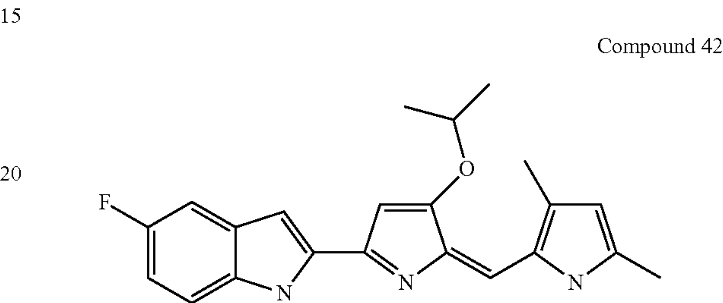
2-[5-(3,5-Dimethyl-1H-pyrrol-2-ylmethylene)-4-isopropoxy-5H-pyrrol-2-yl]-5-fluoro-1H-indole
