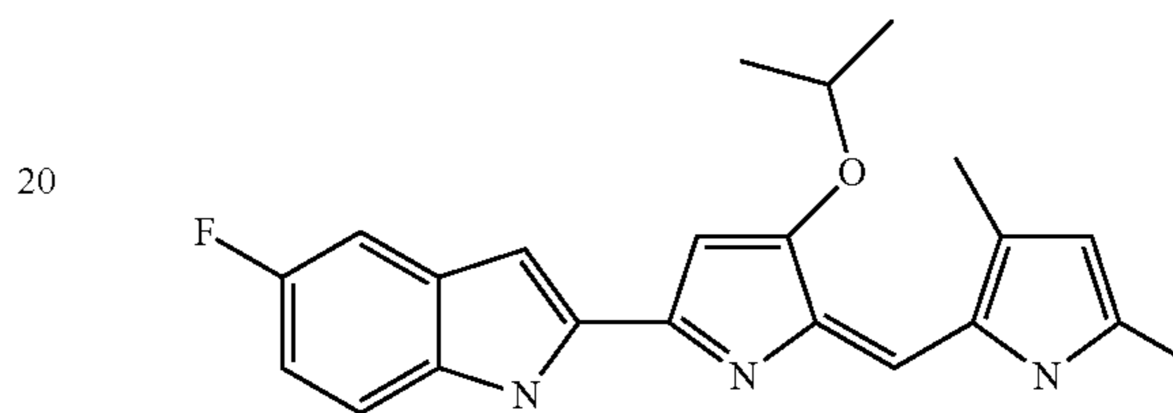
2-[5-(3,5-Dimethyl-1H-pyrrol-2-ylmethylene)-4-isopropoxy-5H-pyrrol-2-yl]-5-fluoro-1H-indole
