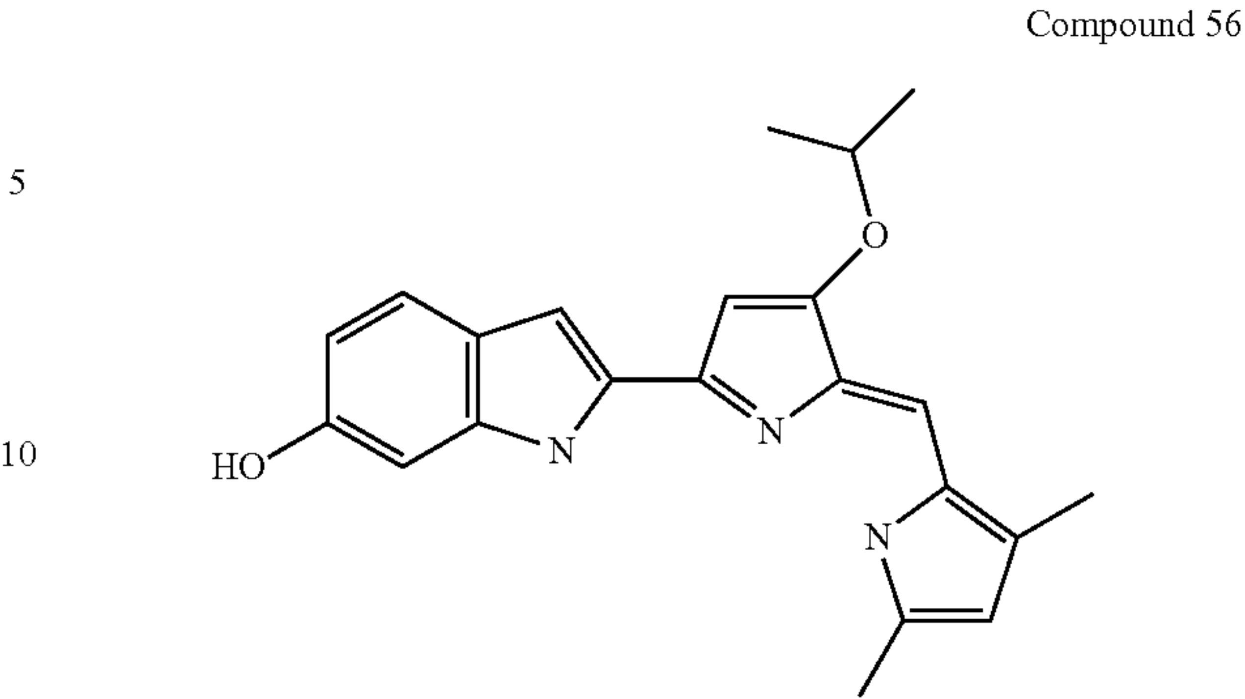
2-[5-(3,5-Dimethyl-1H-pyrrol-2-ylmethylene)-4-isopropoxy-5H-pyrrol-2-yl]-1H-indol-6-ol
