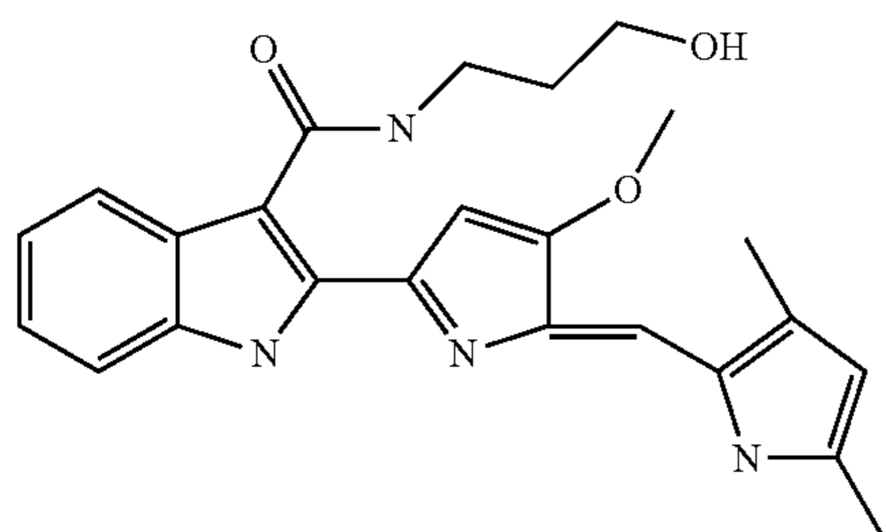
2-[5-(3,5-Dimethyl-1H-pyrrol-2-ylmethylene)-4-methoxy-5H-pyrrol-2-yl]-1H-indole-3-carboxylic acid (3-hydroxypropyl)-amide
