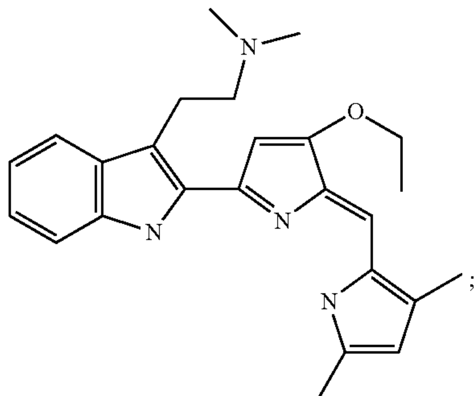
(2-{2-[5-(3,5-Dimethyl-1H-pyrrol-2-ylmethylene)-4-ethoxy-5H-pyrrol-2-yl]-1H-indol-3-yl}-ethyl)dimethyl-amine
