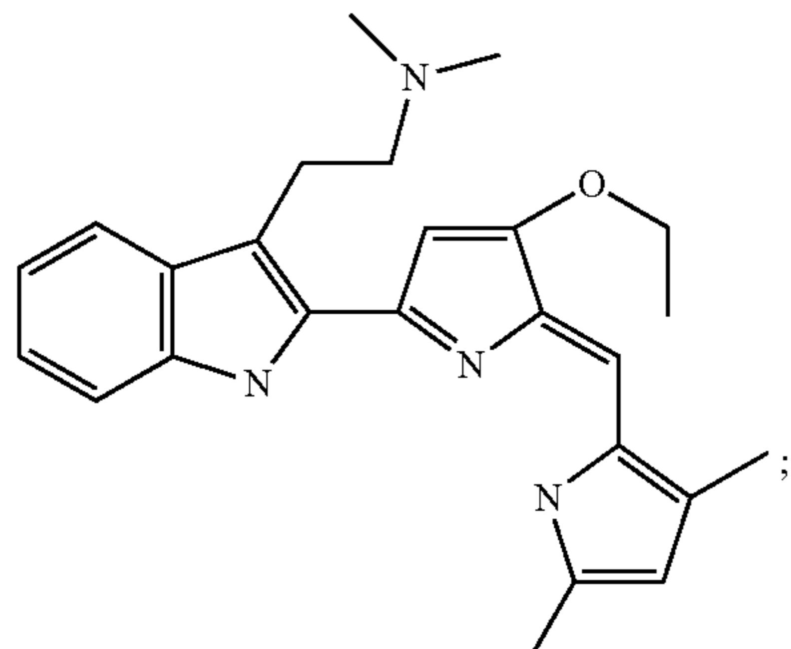
(2-{2-[5-(3,5-Dimethyl-1H-pyrrol-2-ylmethylene)-4-ethoxy-5H-pyrrol-2-yl]-1H-indol-3-yl}-ethyl)dimethyl-amine
