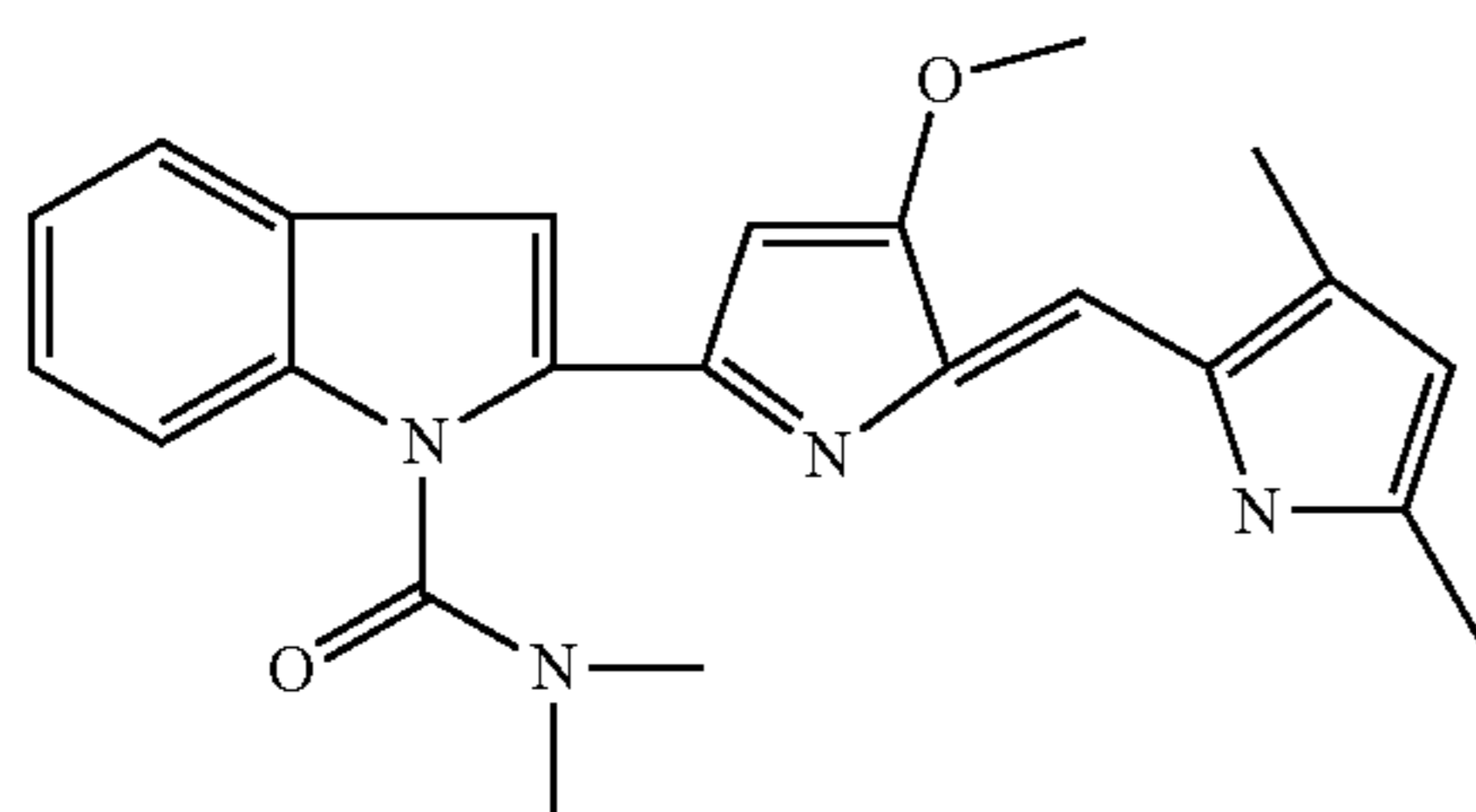
2-[5-(3,5-Dimethyl-1H-pyrrol-2-ylmethylene)-4-methoxy-5H-pyrrol-2-yl]-indole-1-carboxylic acid dimethylamide
