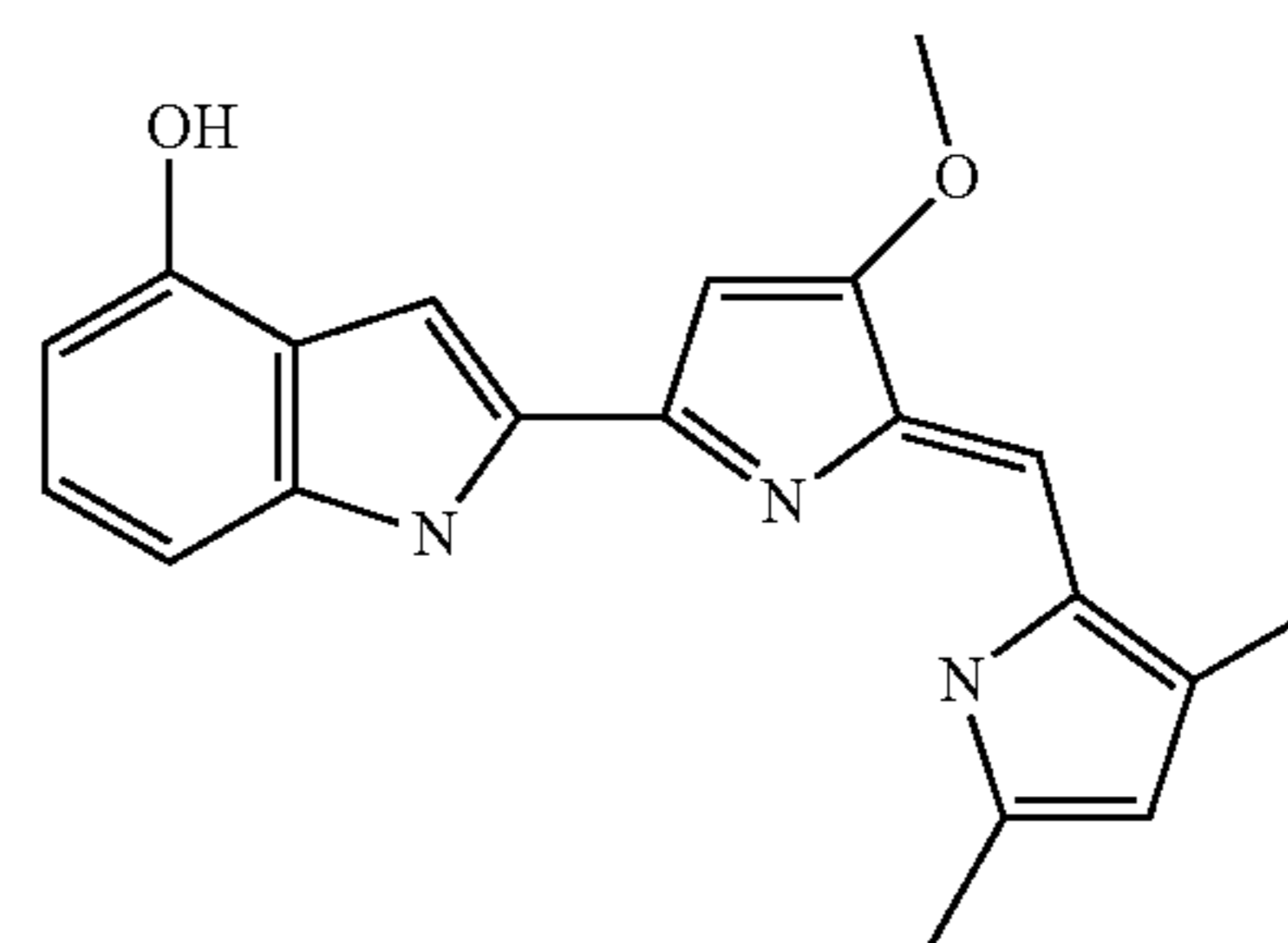
2-[5-(3,5-Dimethyl-1H-pyrrol-2-ylmethylene)-4-methoxy-5H-pyrrol-2-yl]-1H-indol-4-ol
