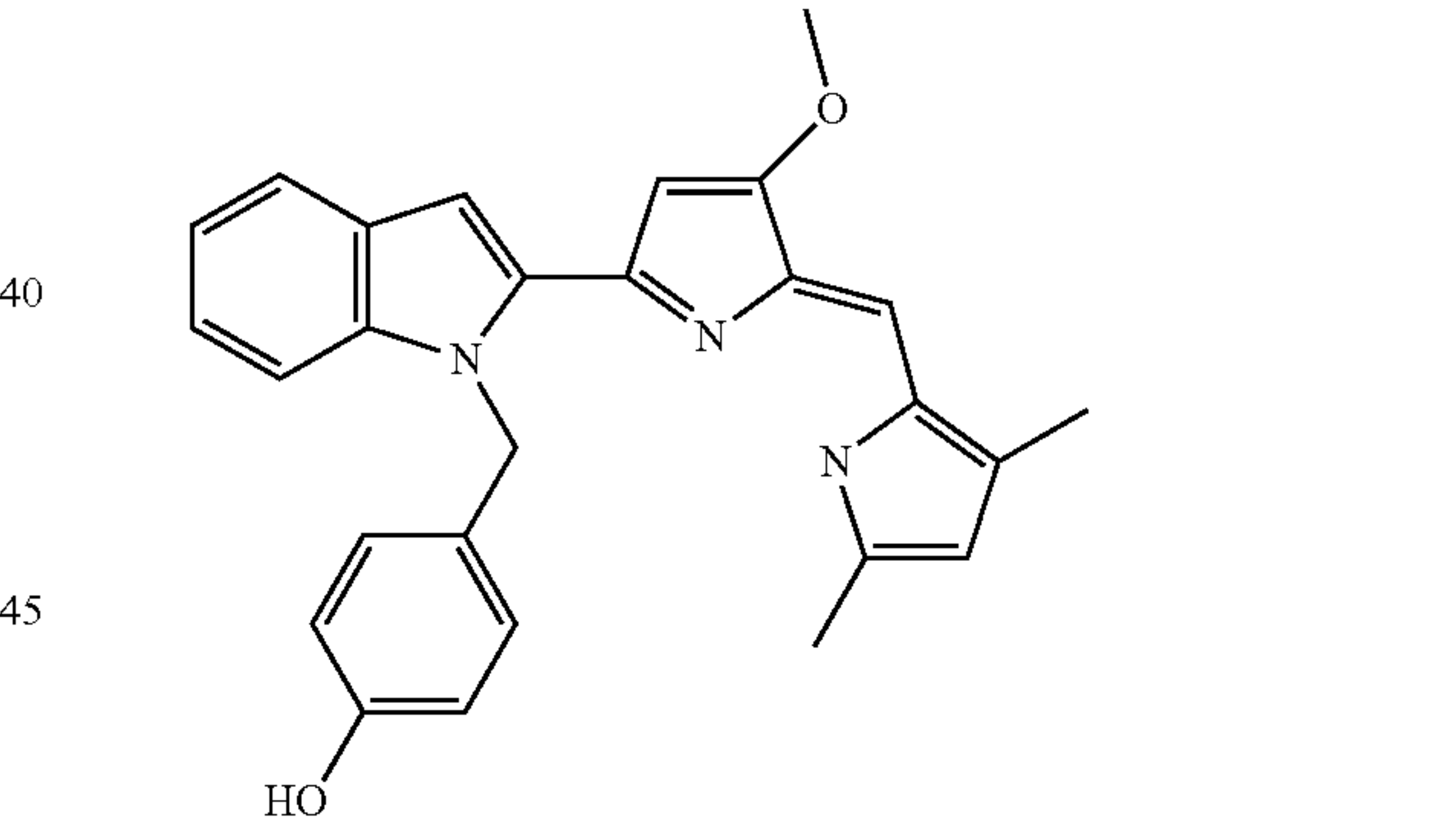
4-{2-[5-(3,5-Dimethyl-1H-pyrrol-2-ylmethylene)-4-methoxy-5H-pyrrol-2-yl]-indol-1-ylmethyl}-phenol
