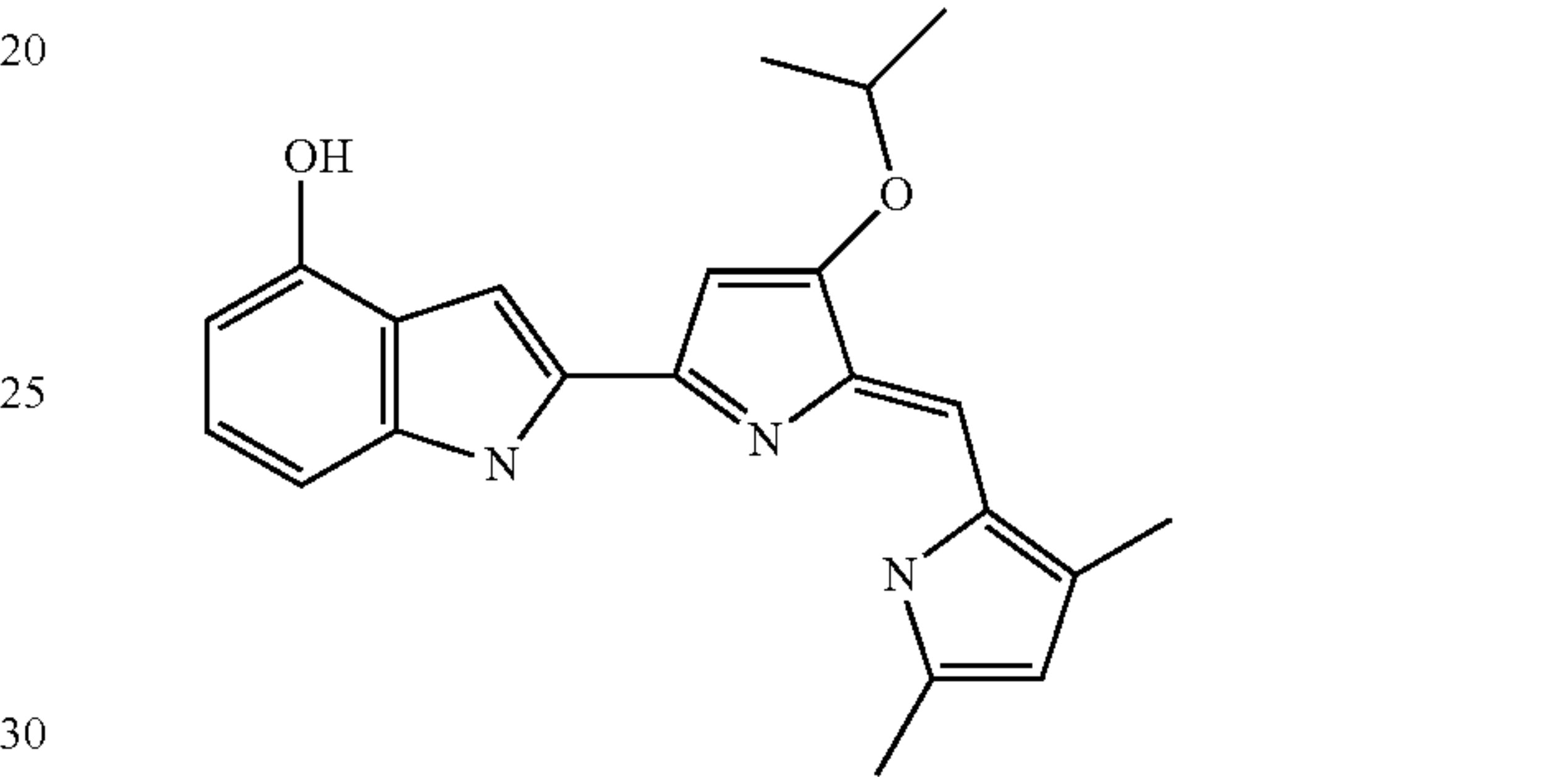
2-[5-(3,5-Dimethyl-1H-pyrrol-2-ylmethylene)-4-isopropoxy-5H-pyrrol-2-yl]-1H-indol-4-ol
