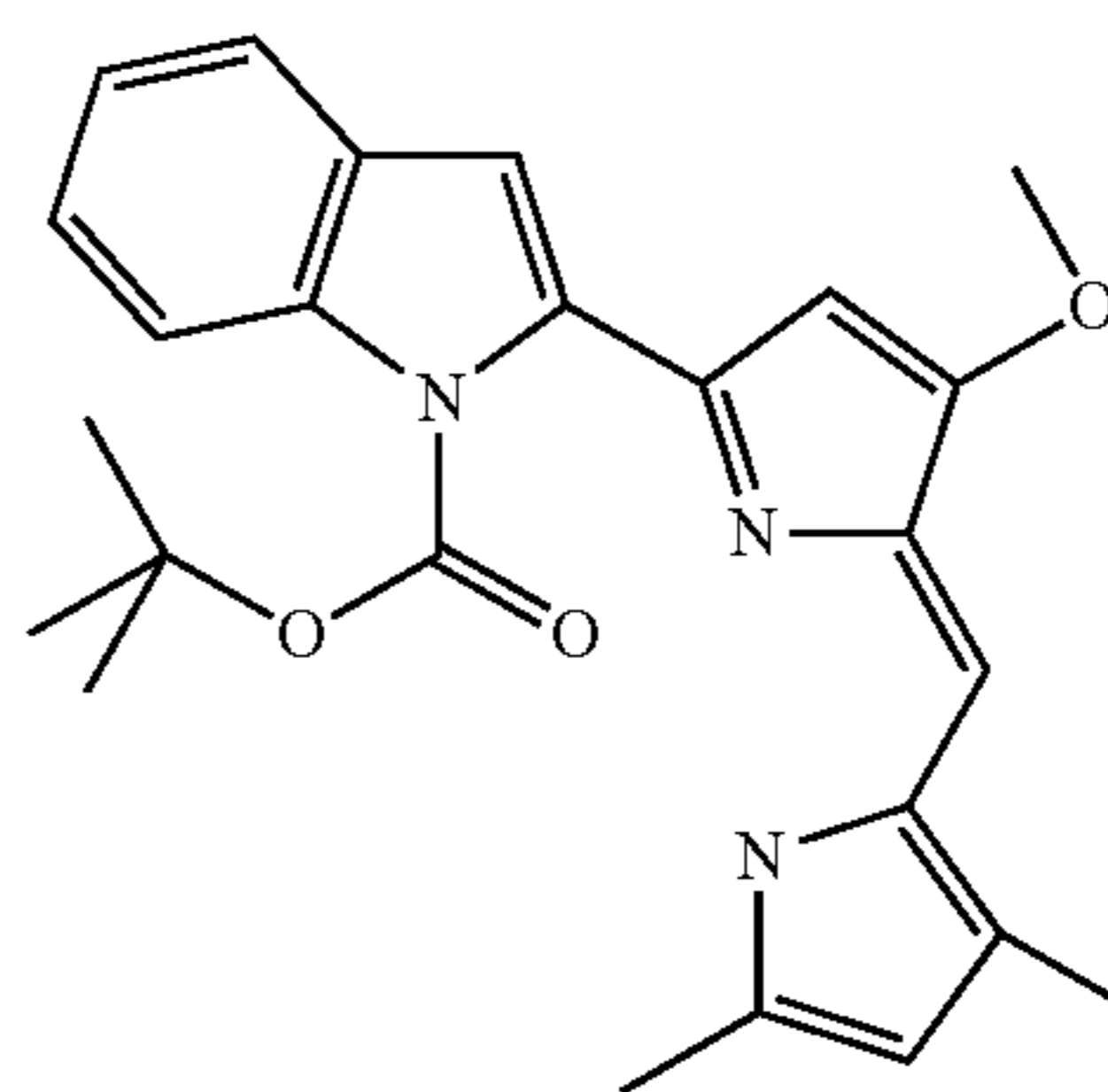
2-[5-(3,5-Dimethyl-1H-pyrrol-2-ylmethylene)-4-methoxy-5H-pyrrol-2-yl]-indole-1-carboxylic acid tert-butyl ester
