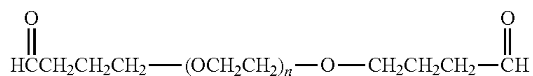
Homobifunctional PEG Butyraldehyde Derivative
