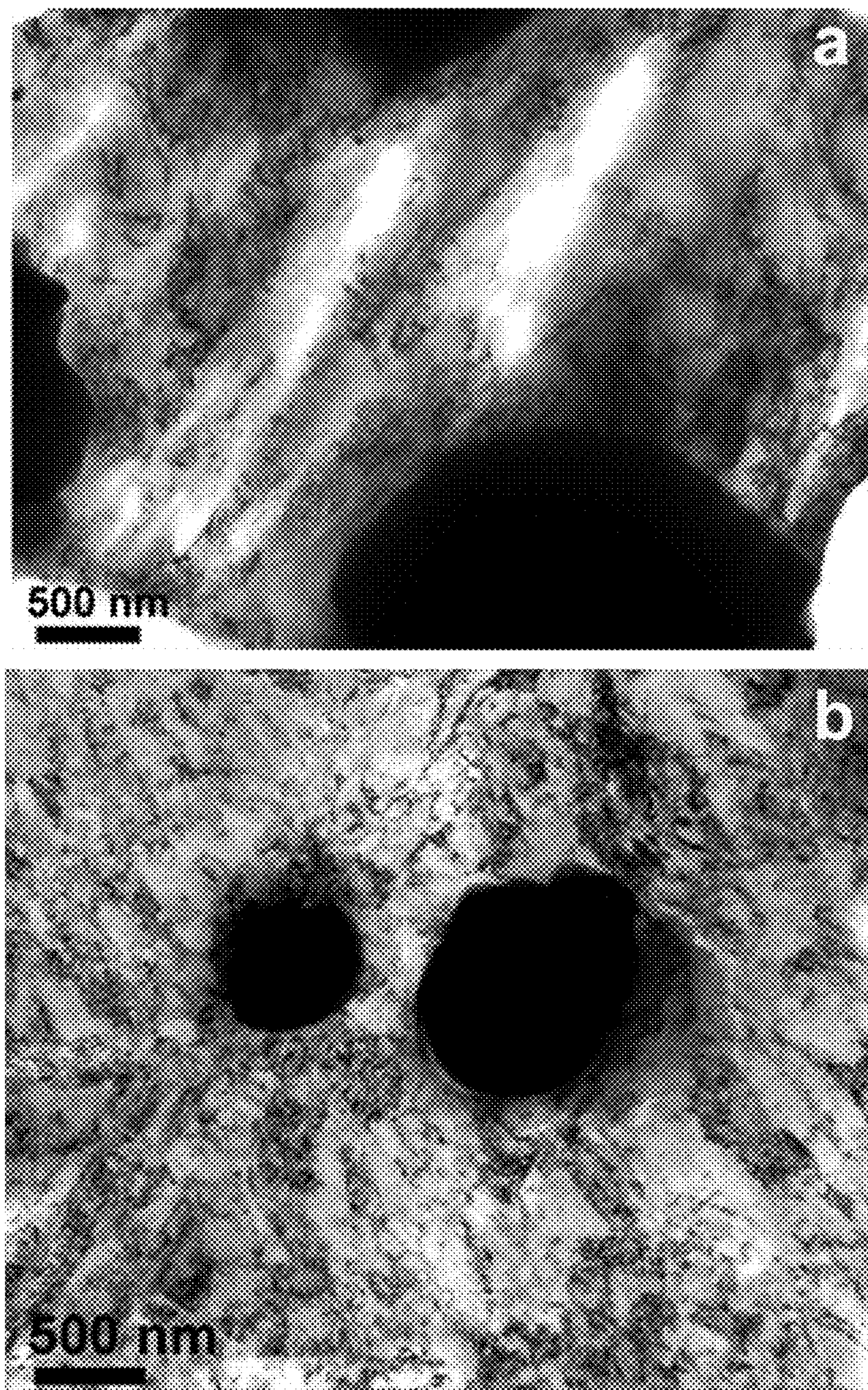
FIG. 60 TEM images of the microstructure in the tensile specimen from the Alloy 51 after cycling deformation to 10% and annealing at 1100°C for 1 hour (3 times), then tested to failure a) in the grip section and b) in the gage.
