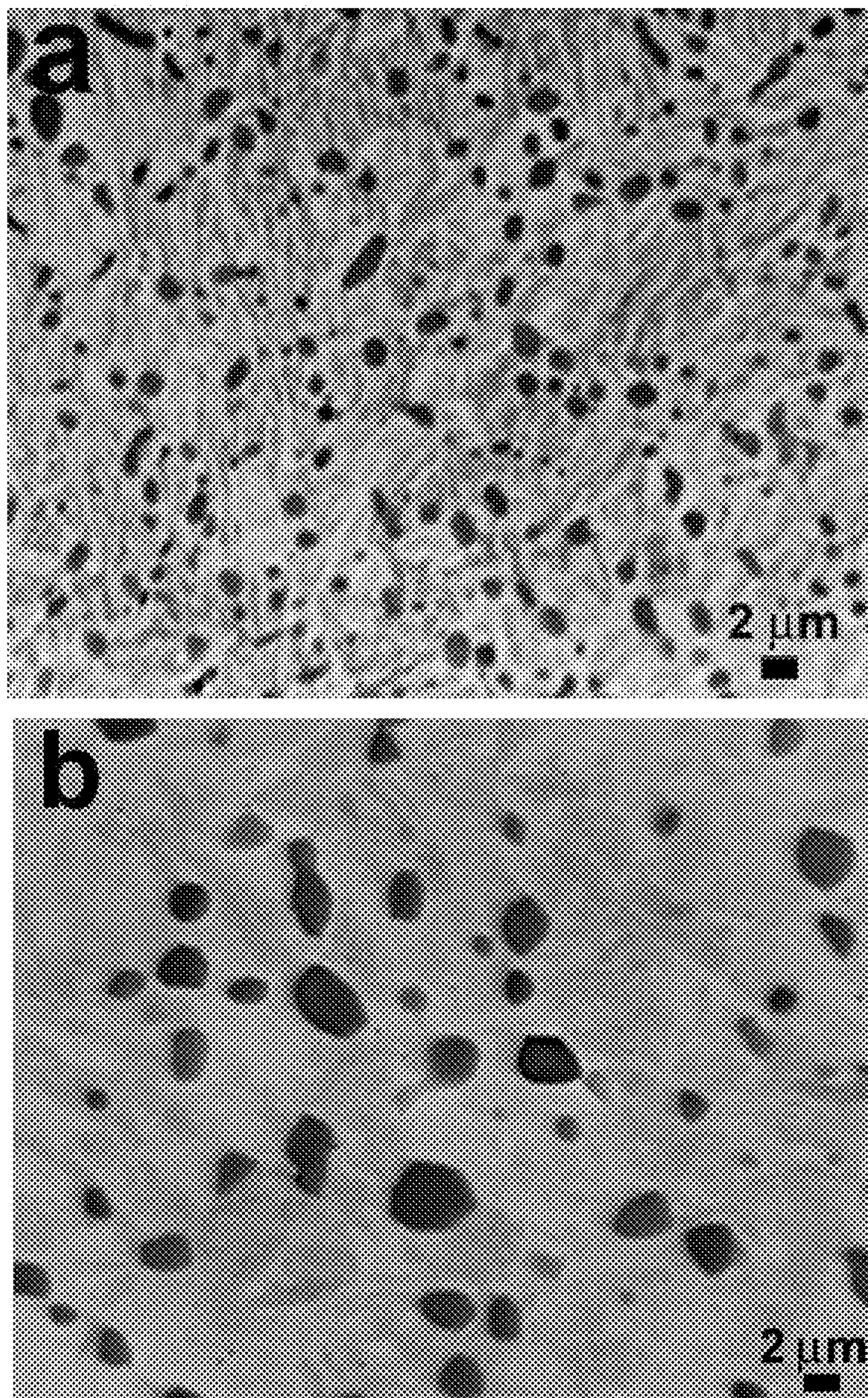
FIG. 56 SEM images of microstructure of the gage section of the tensile specimens from the Alloy 6 after pre-straining to 3% and annealing at 1100°C for 1 hour at different magnification.
