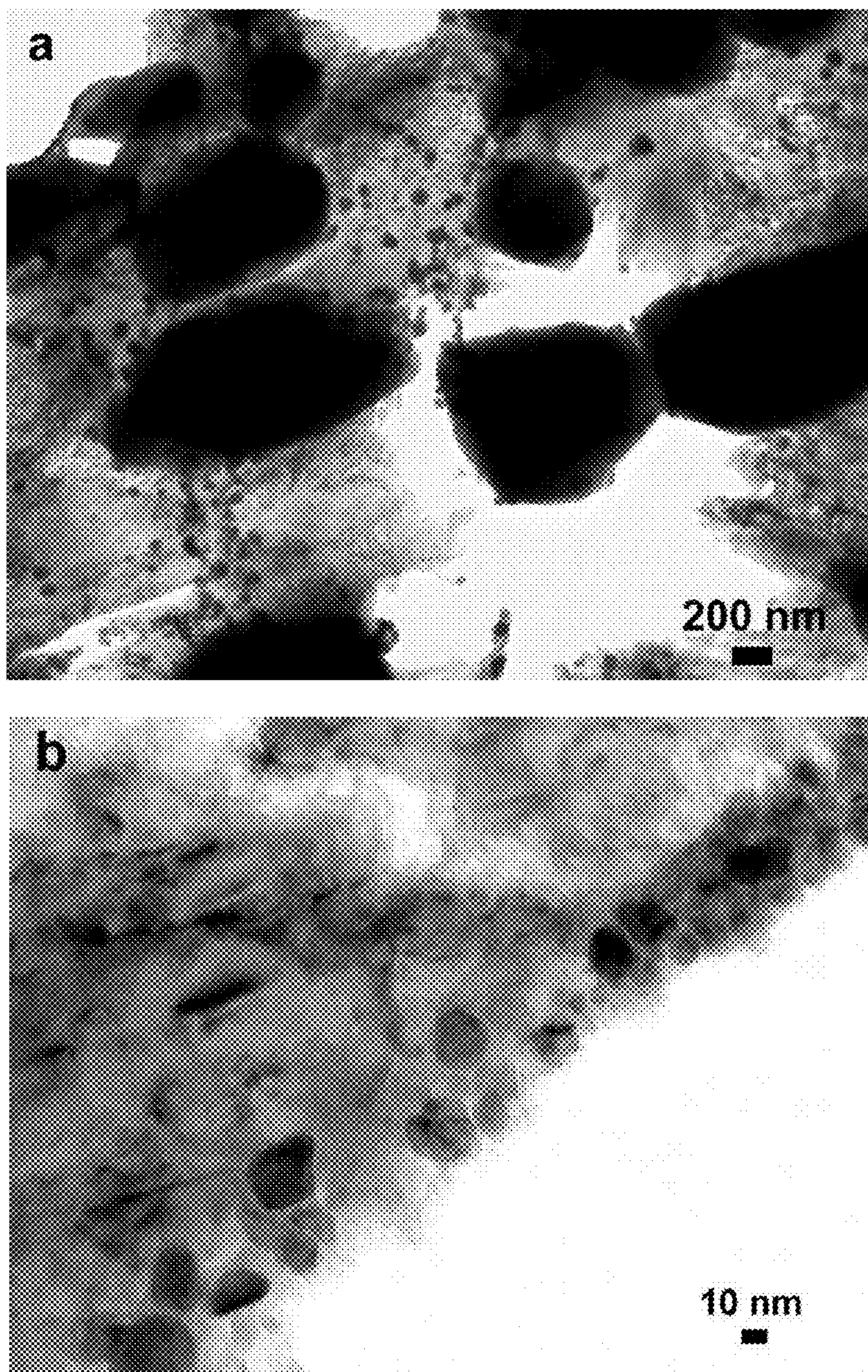
FIG. 68 The bright-field TEM micrographs of the microstructure in the Alloy 20 specimen gage after tension at 850°C with tensile elongation of 23%.
