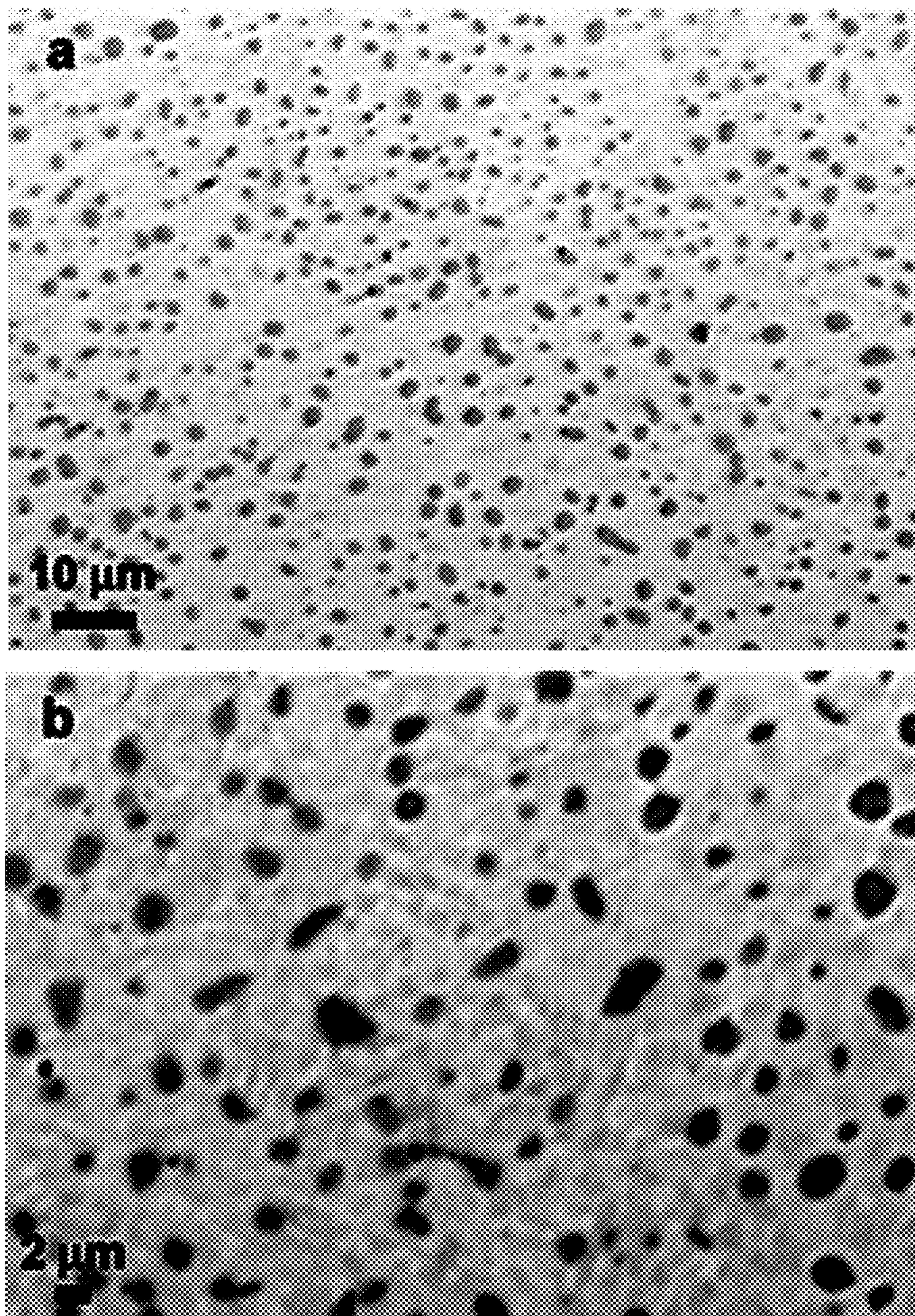
FIG. 42 The backscattered SEM images of the microstructure in the Alloy 27 specimen after HIP cycle at 1100°C for 1 hr and heat treatment at 700°C for 1 hr (prior deformation).
