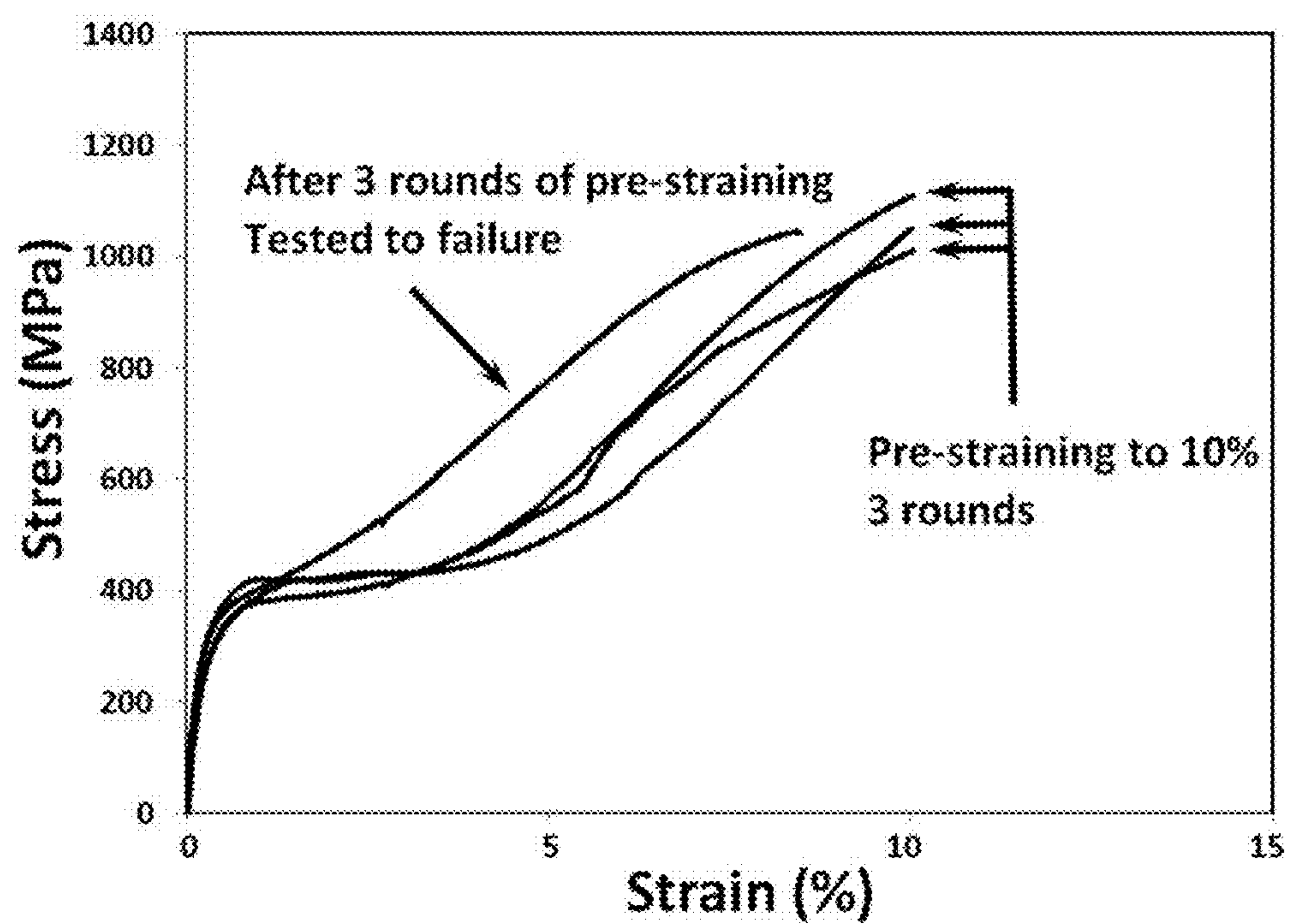
FIG. 57 Stress strain curves for the Alloy 51 specimen that has been subjected to 3 rounds of tensile testing to a 10% deformation followed by annealing between rounds and tested to failure.
