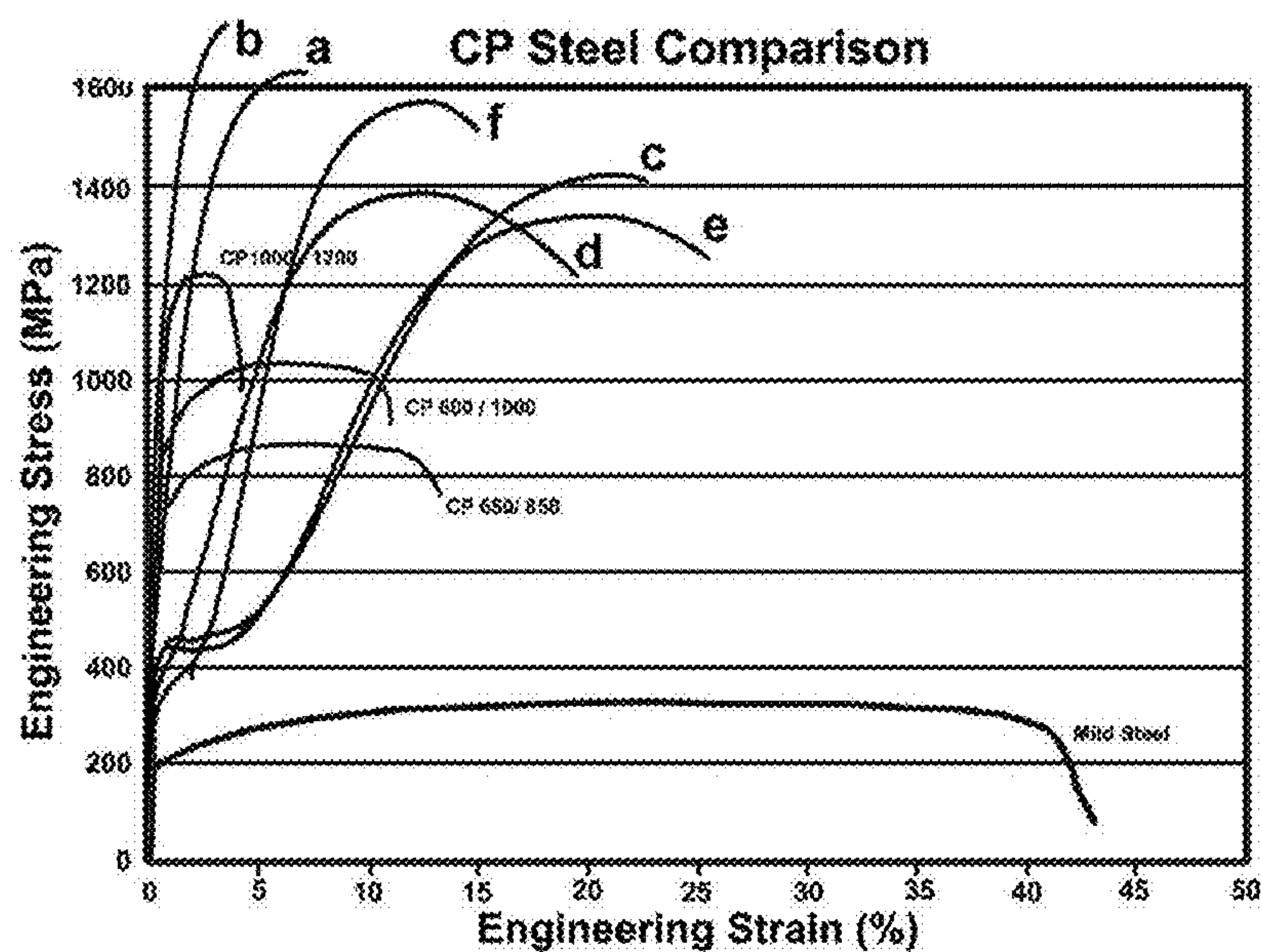
FIG. 10 Comparison of stress-strain curves of new non-stainless steel sheet types with existing Complex Phase (CP) steels.
