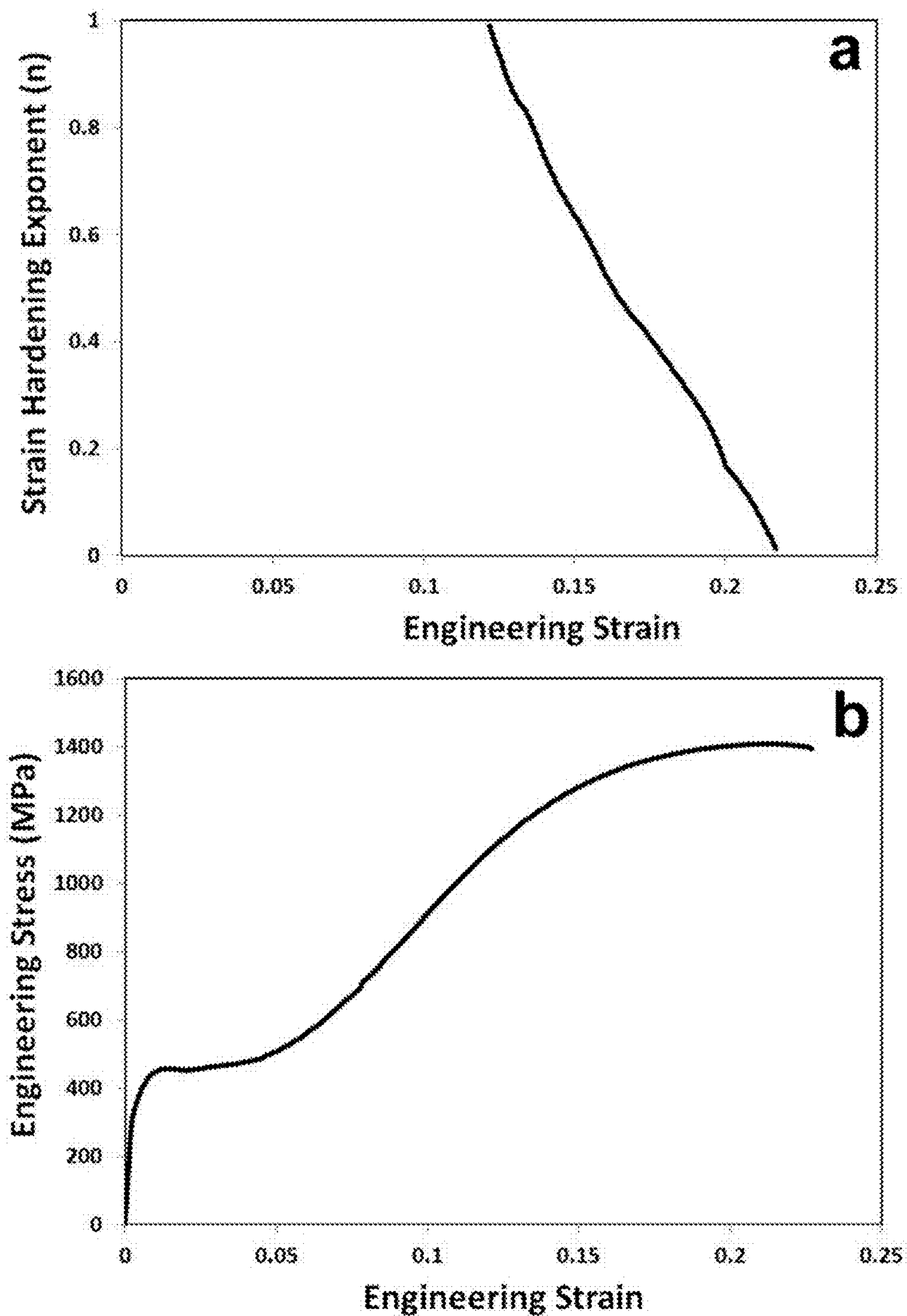
FIG. 46 (a) Strain hardening coefficient in the Alloy 51 as a function of strain; (b) Corresponding stress-strain curve.
