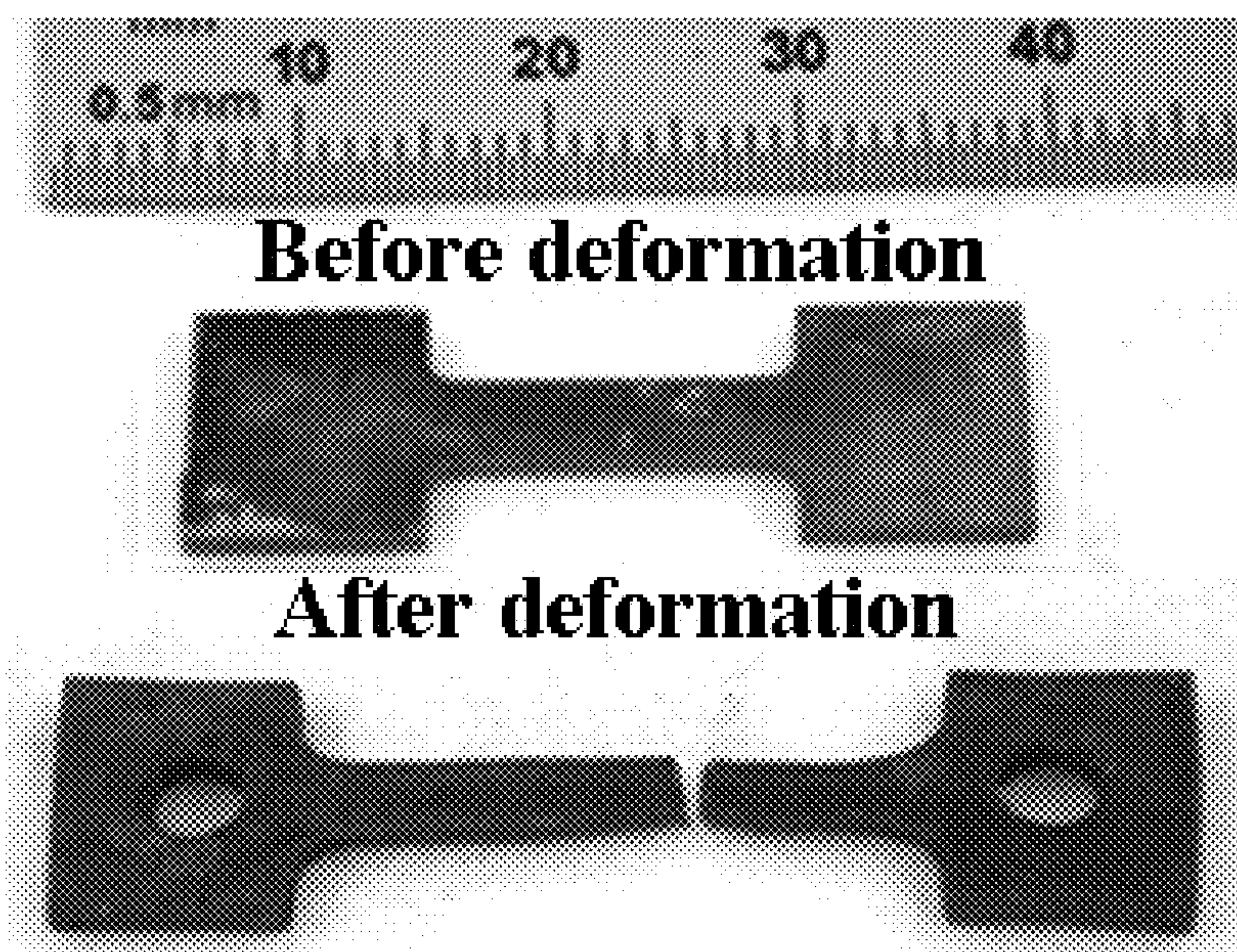
FIG.62 View of the Class 3 alloy specimen after HIP cycle and heat treatment before and after deformation to 57.5%.
