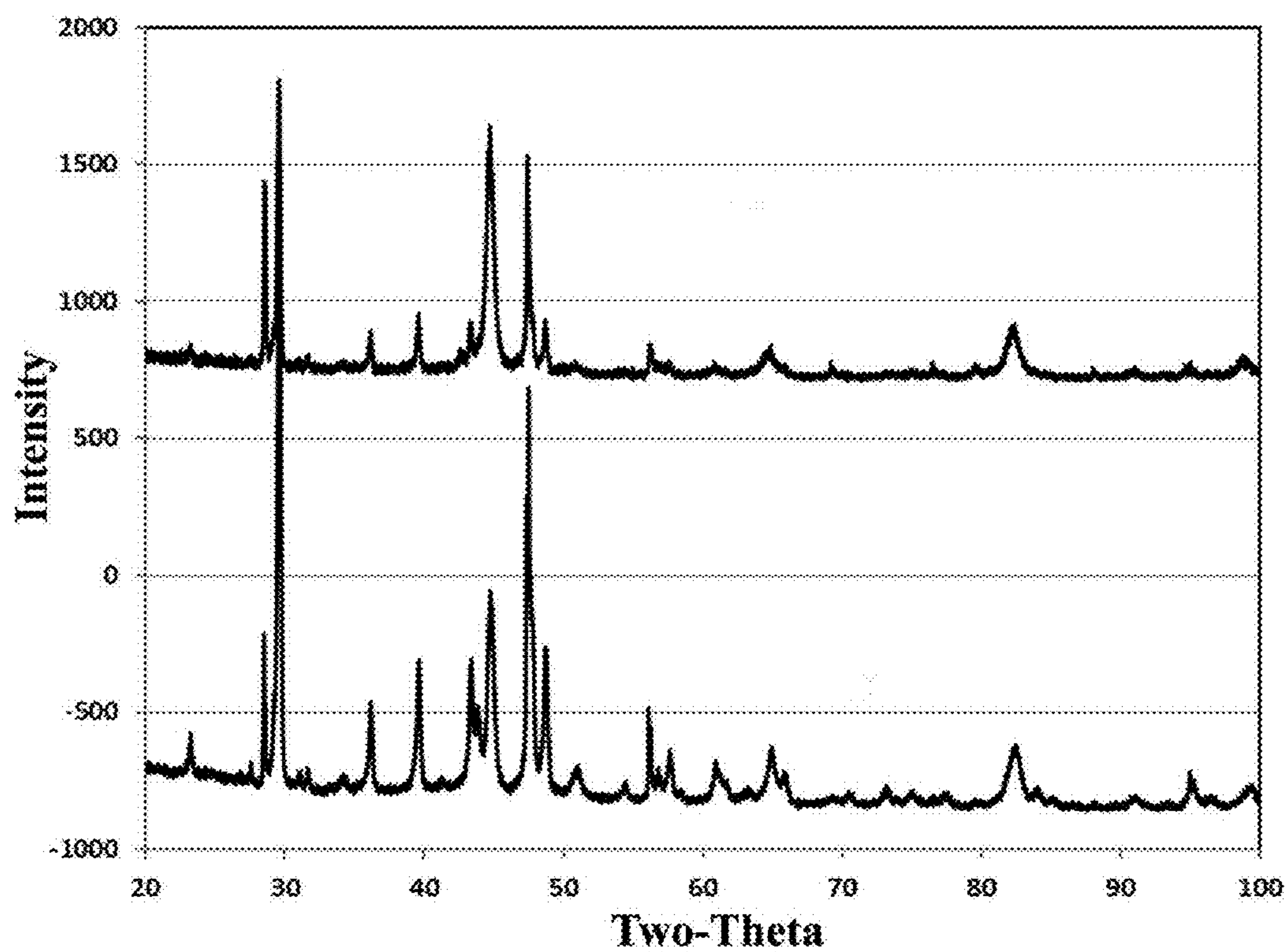
FIG. 30 Comparison between X-ray data for the specimen from the Alloy 51 plate after the HIP cycle at 1100°C for 1 hour and heat treatment at 700°C for 1 hour after tensile testing: 1) in a grip section (top curve) and 2) in a gage section (bottom curve).
