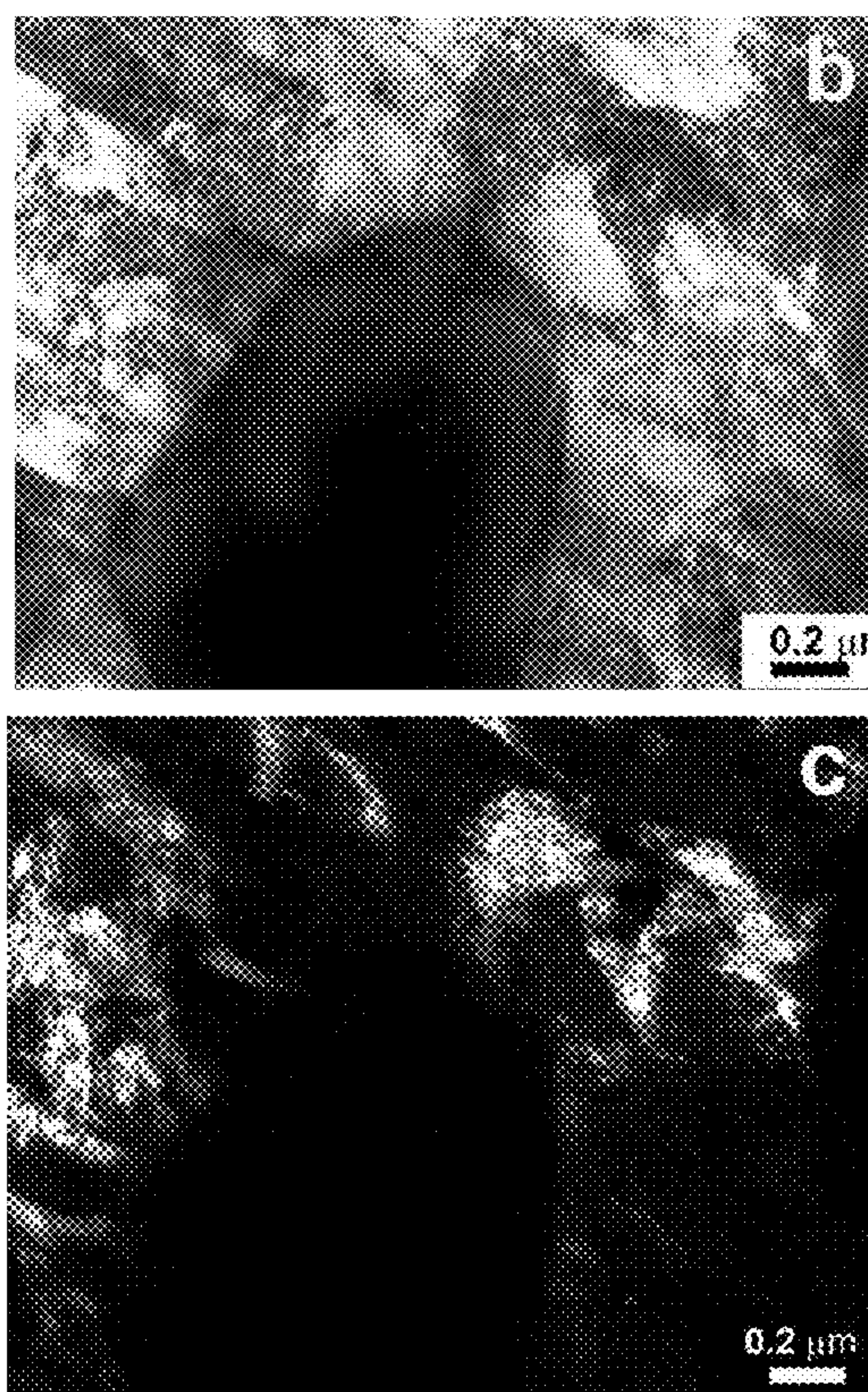
FIG. 26 The TEM micrographs of the microstructure in the Alloy 6 plate sample at 1100°C for 1 hour. (a) A number of precipitates formed and distributed homogeneously in the matrix with lath structure; (b) The detailed microstructure of the lath microstructure near precipitates. (c) Dark-field TEM image showing grains within lath structure.
