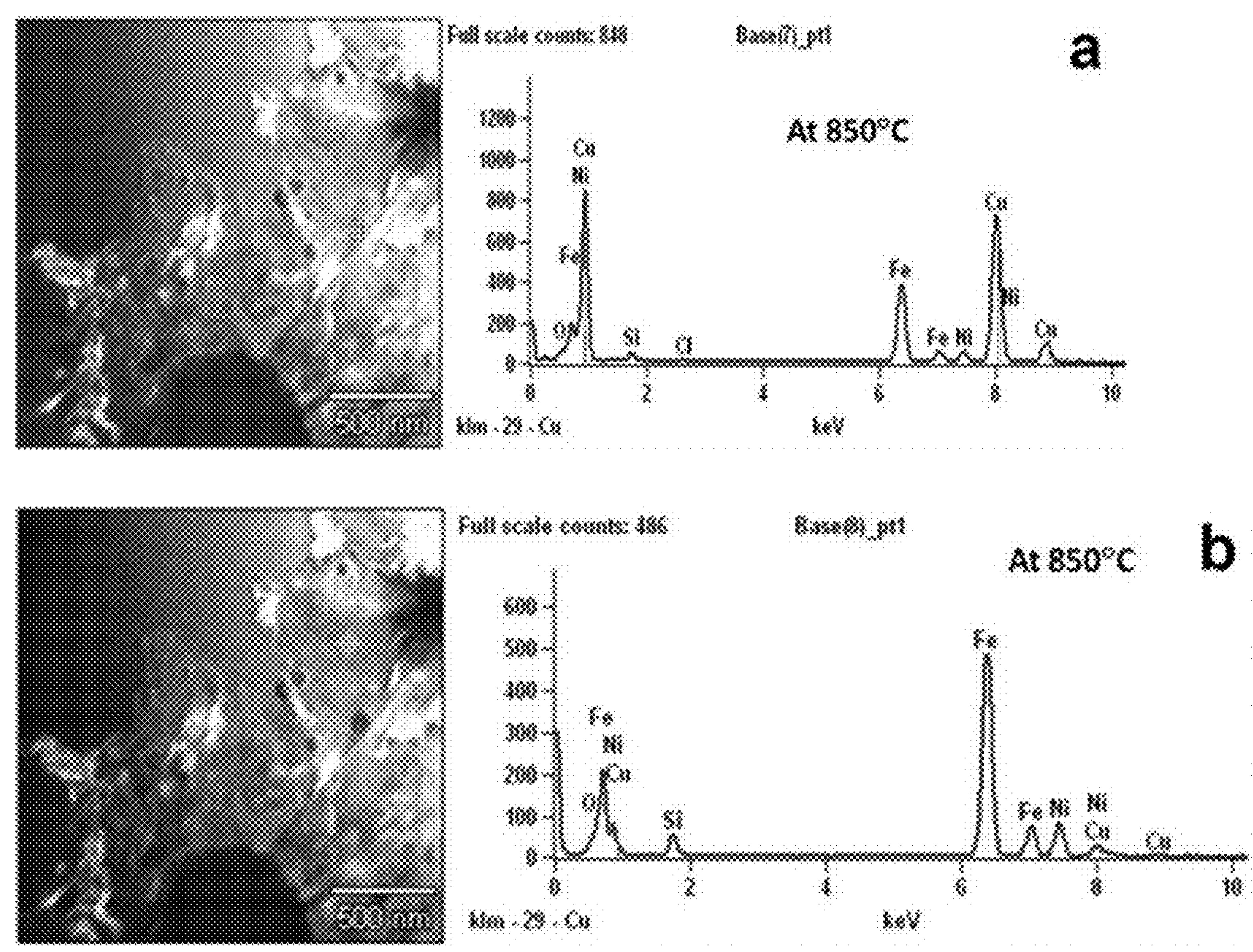
FIG. 69 TEM EDS analysis on the nano-precipitates formed in the Alloy 20 specimens.
