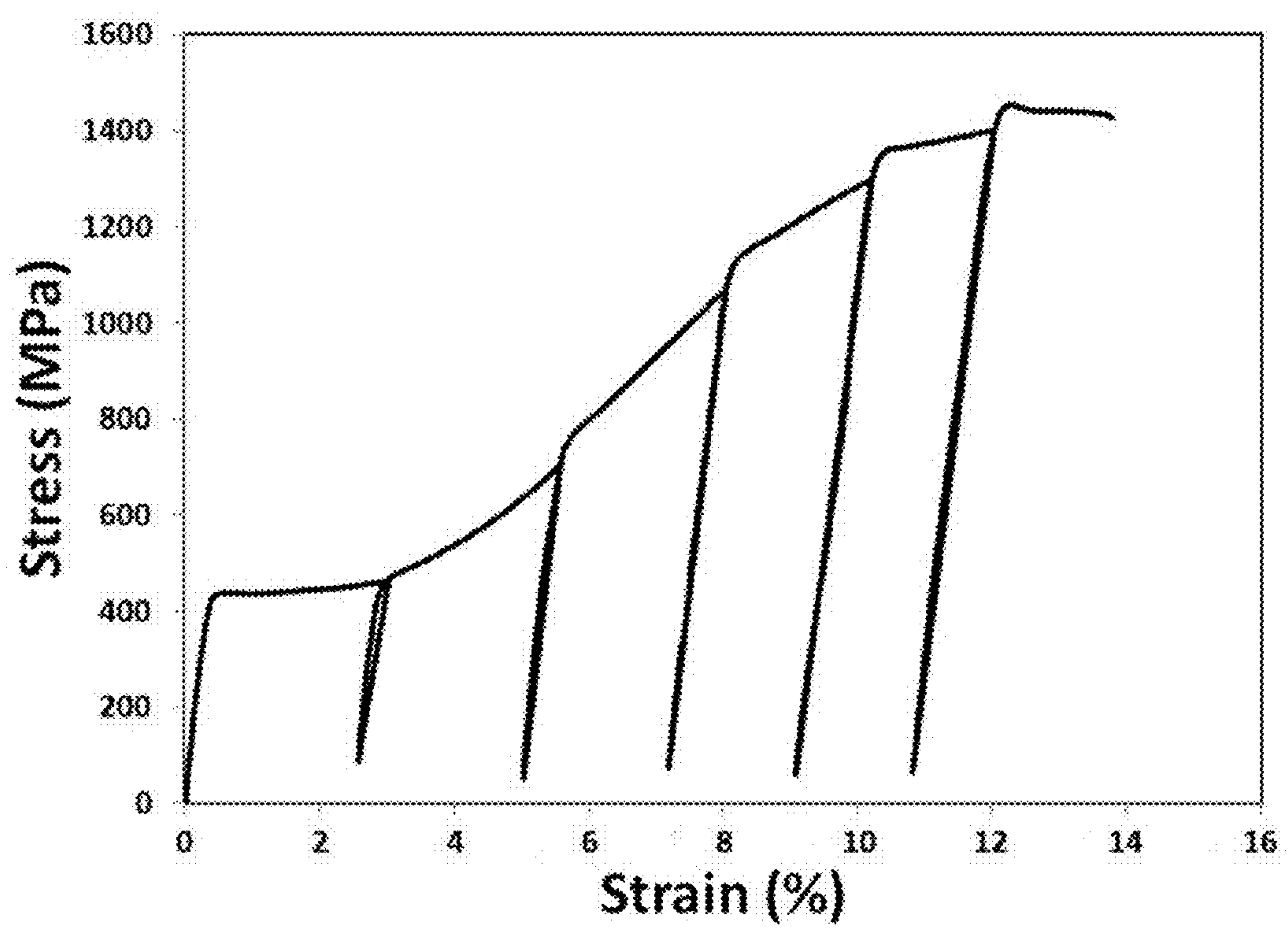
FIG. 48 Stress-strain curves for the Alloy 51 specimen tested in tension with incremental straining.
