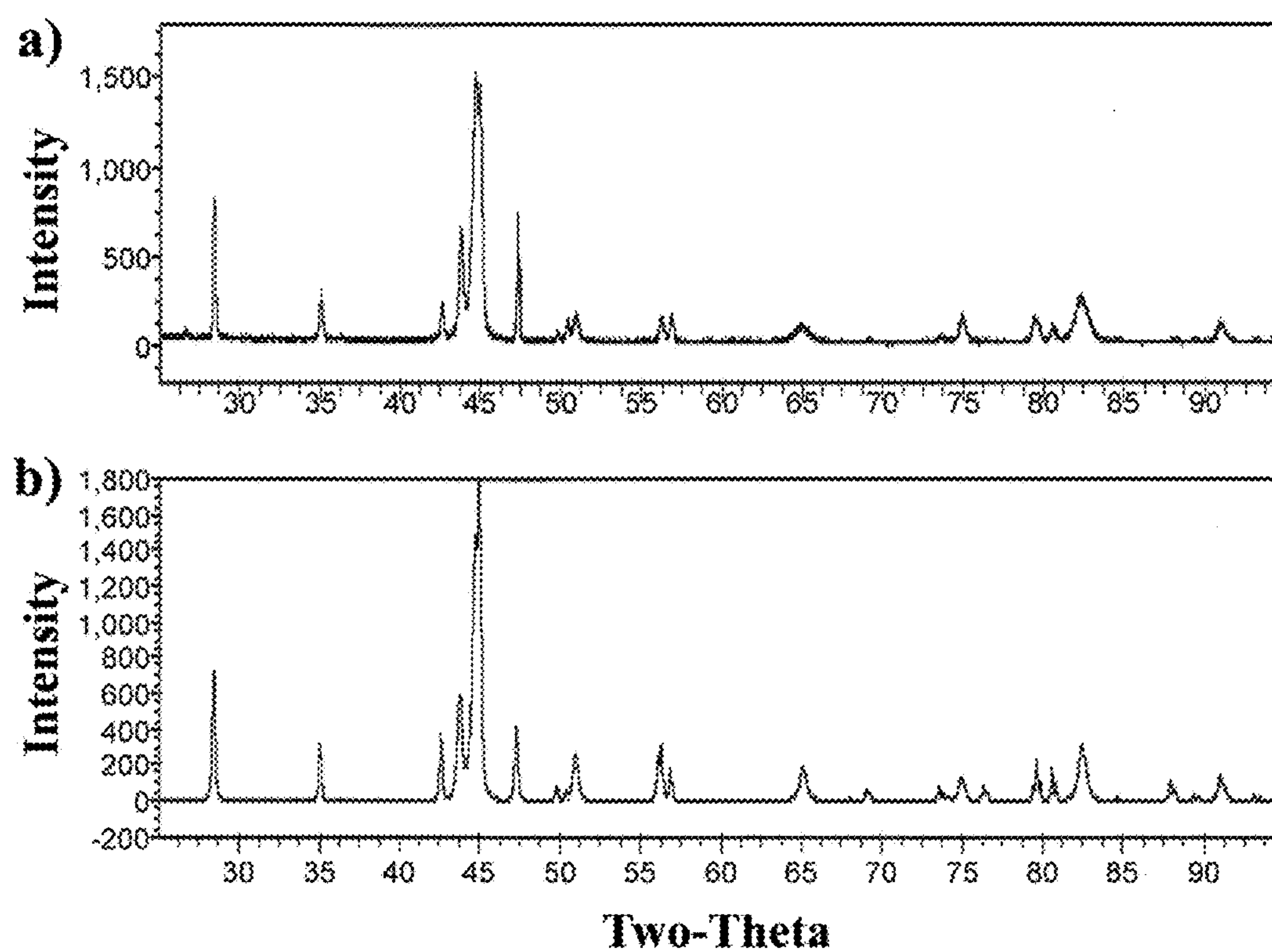
FIG. 15 X-ray diffraction data (intensity vs two-theta) for Alloy 51 plate in the HIPed condition (1100°C for 1 hour); a) Measured pattern, b) Rietveld calculated pattern with peaks identified.
