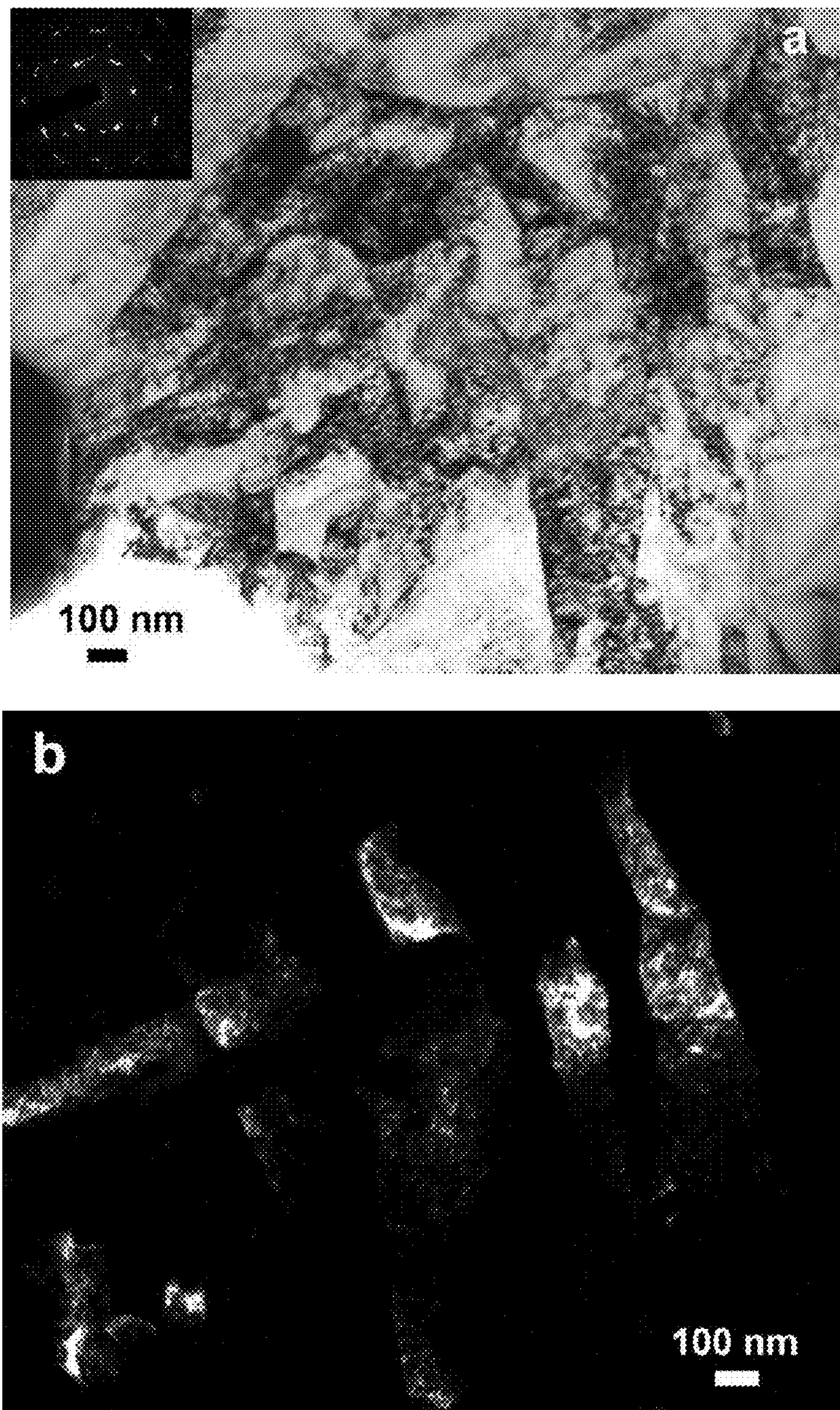
FIG. 70 The (a) bright-field and (b) dark field TEM micrographs of the microstructure in the Alloy 22 specimen gage after tension at 700°C with tensile elongation of 34.5%.
