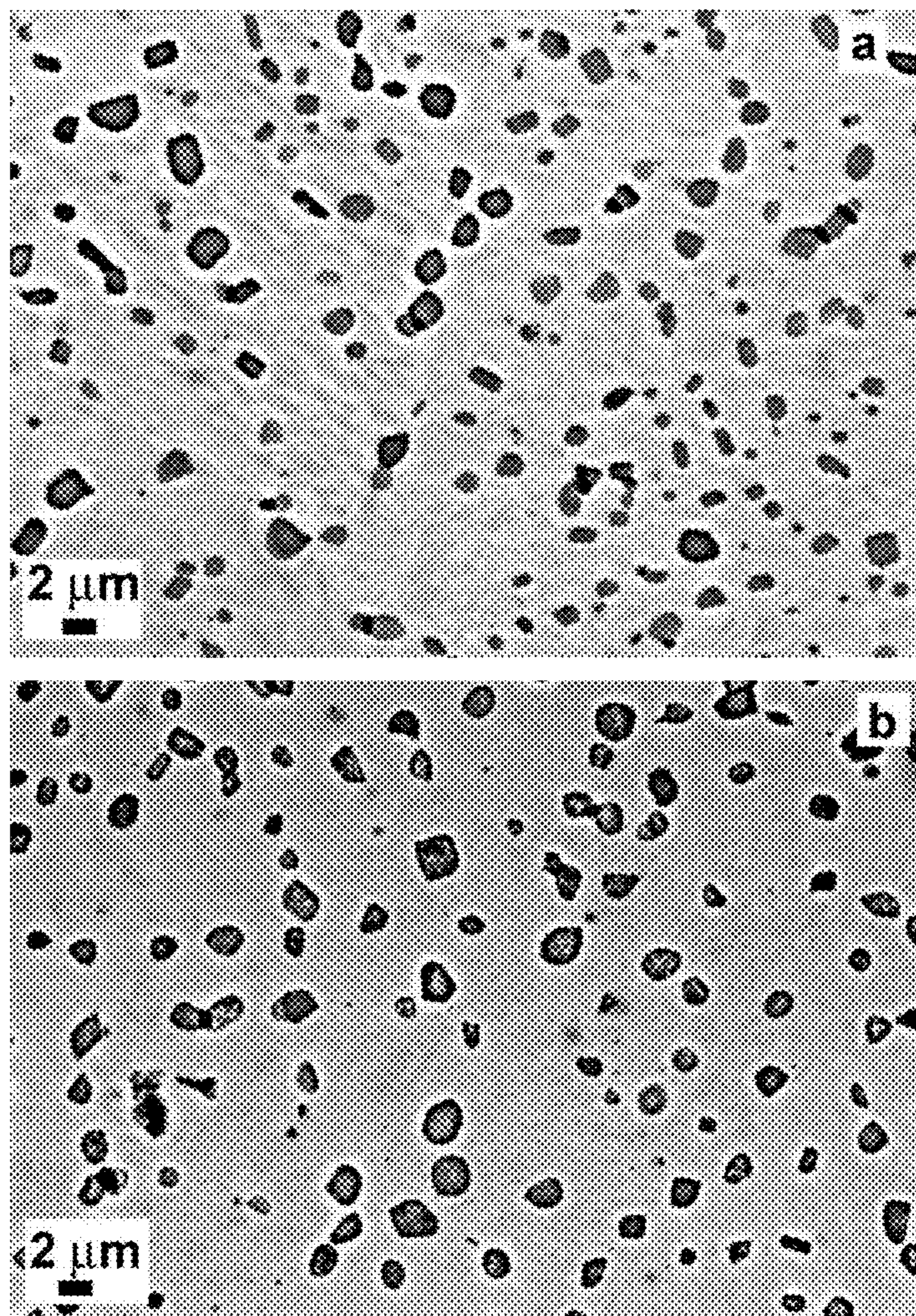
FIG. 29 SEM images of the microstructure in the specimen from the Alloy 51 after the HIP cycle at 1100°C for 1 hour, heat treatment at 700°C for 1 hour and deformation at room temperature (a) in a grip section and (b) in a gage section.
