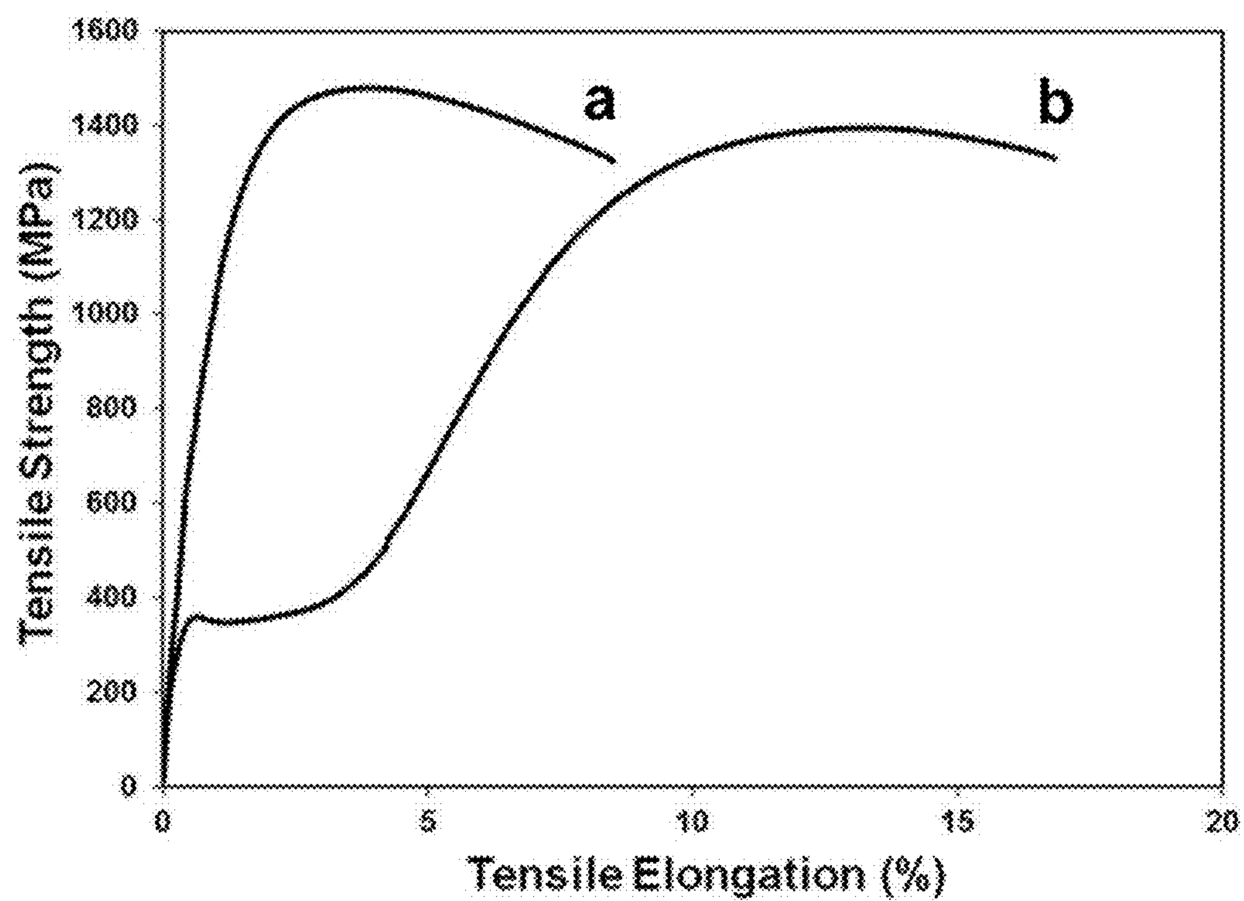
FIG. 40 Representative stress-strain curves for (a) Alloy 17 and (b) Alloy 27 specimens after same thermal mechanical treatment tested at room temperature.
