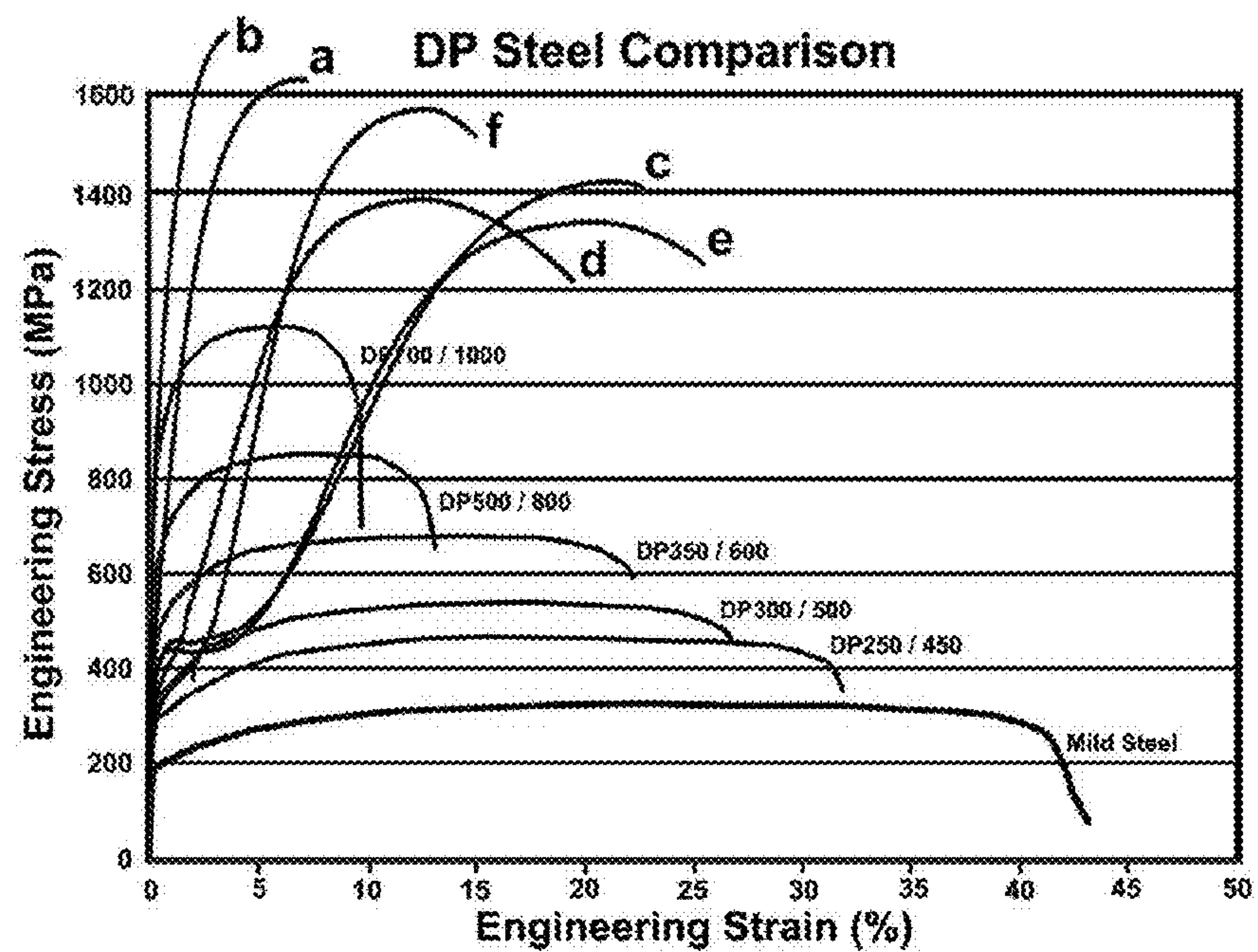
FIG. 9 Comparison of stress-strain curves of new non-stainless steel sheet types with existing Dual Phase (DP) steels.
