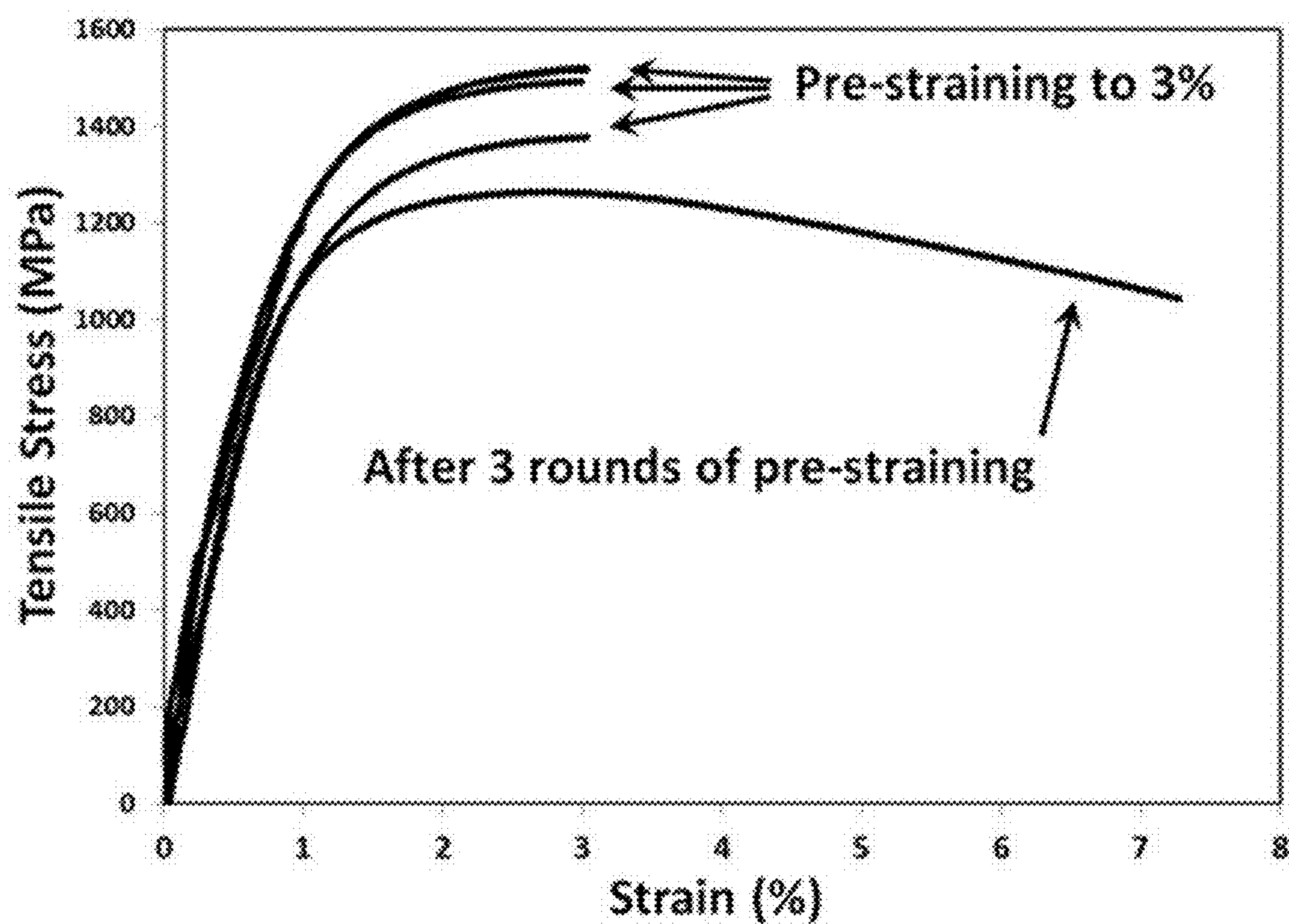
FIG. 61 Stress - strain curves for the Alloy 6 specimen that has been subjected to 3 rounds of tensile testing to a 3% deformation followed by annealing between steps and tested to failure.
