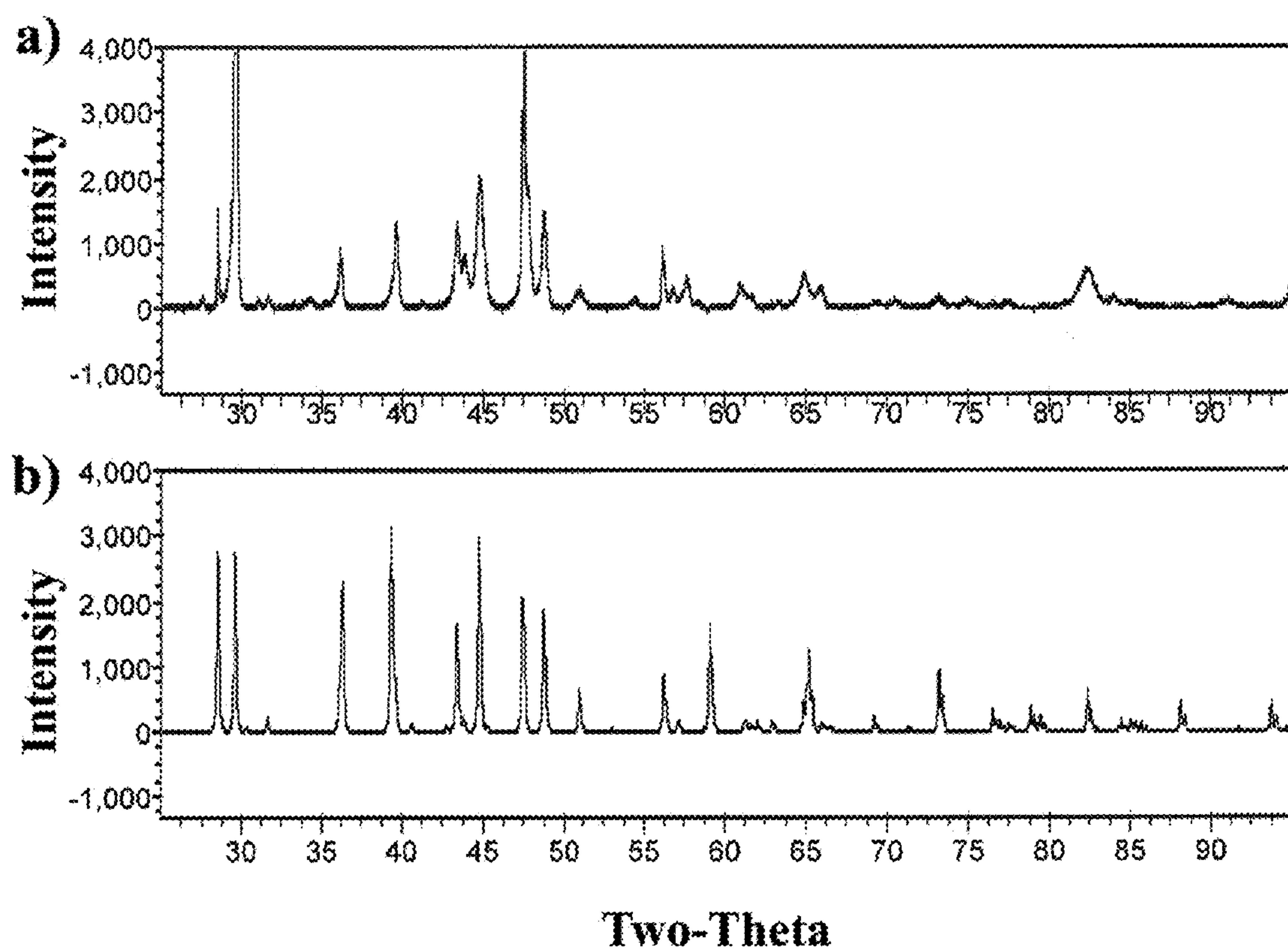
FIG. 31 X-ray diffraction data (intensity vs two-theta) for the gage section of tensile tested specimen from the Alloy 51 plate in the HIPed condition (1100°C for 1 hour) and heat treated at 700°C for 1 hour; a) Measured pattern, b) Rietveld calculated pattern with peaks identified.
