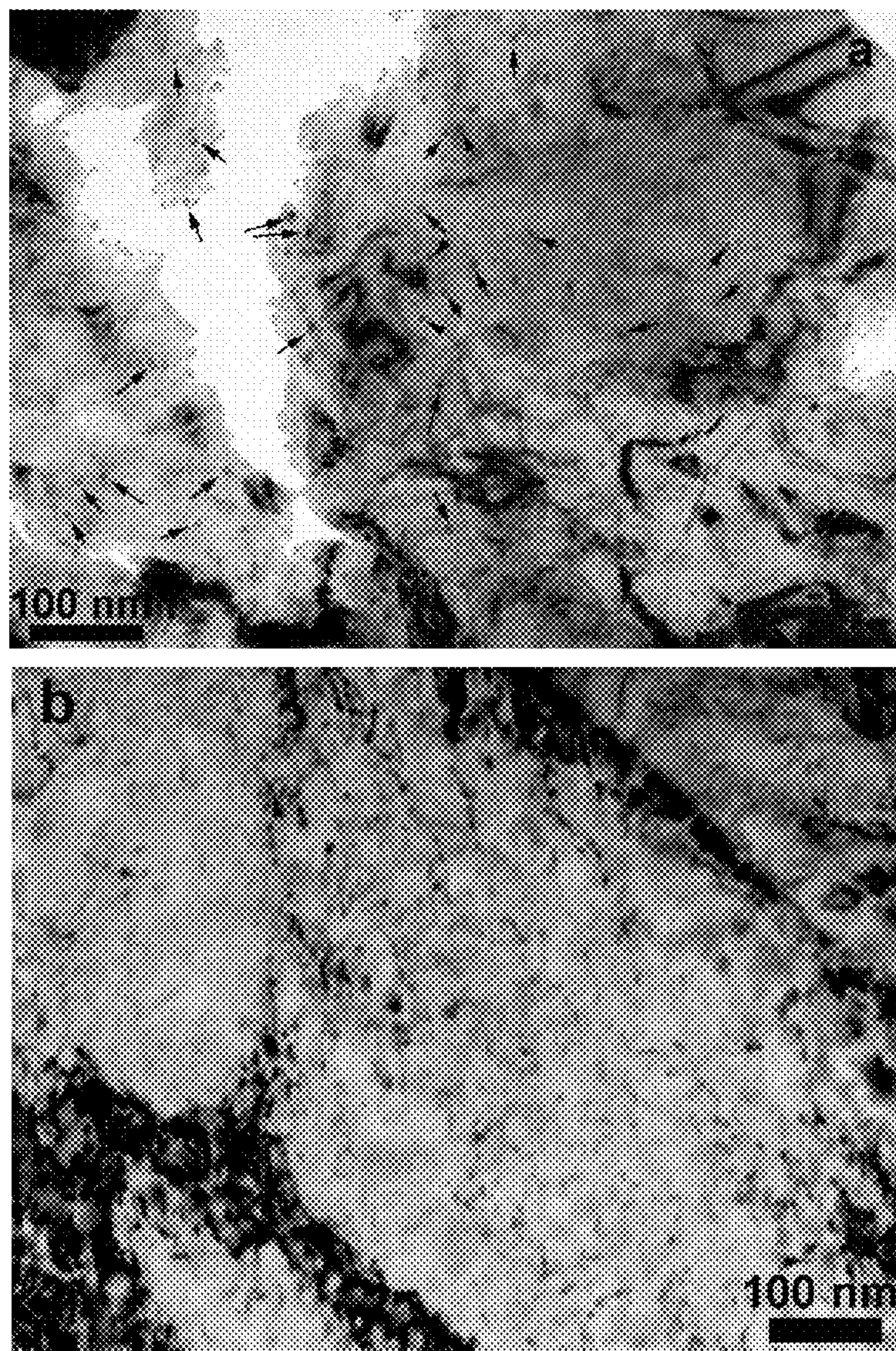
FIG. 33 TEM micrographs of microstructure in the specimen from the Alloy 51 plate HIPed at 1100°C for 1 hour and heat treated at 700°C for 1 hour; a) Before tensile testing, nano-precipitates are observed after heat treatment.; b) After tensile testing, dislocation pinning by the nano-precipitates is observed.
