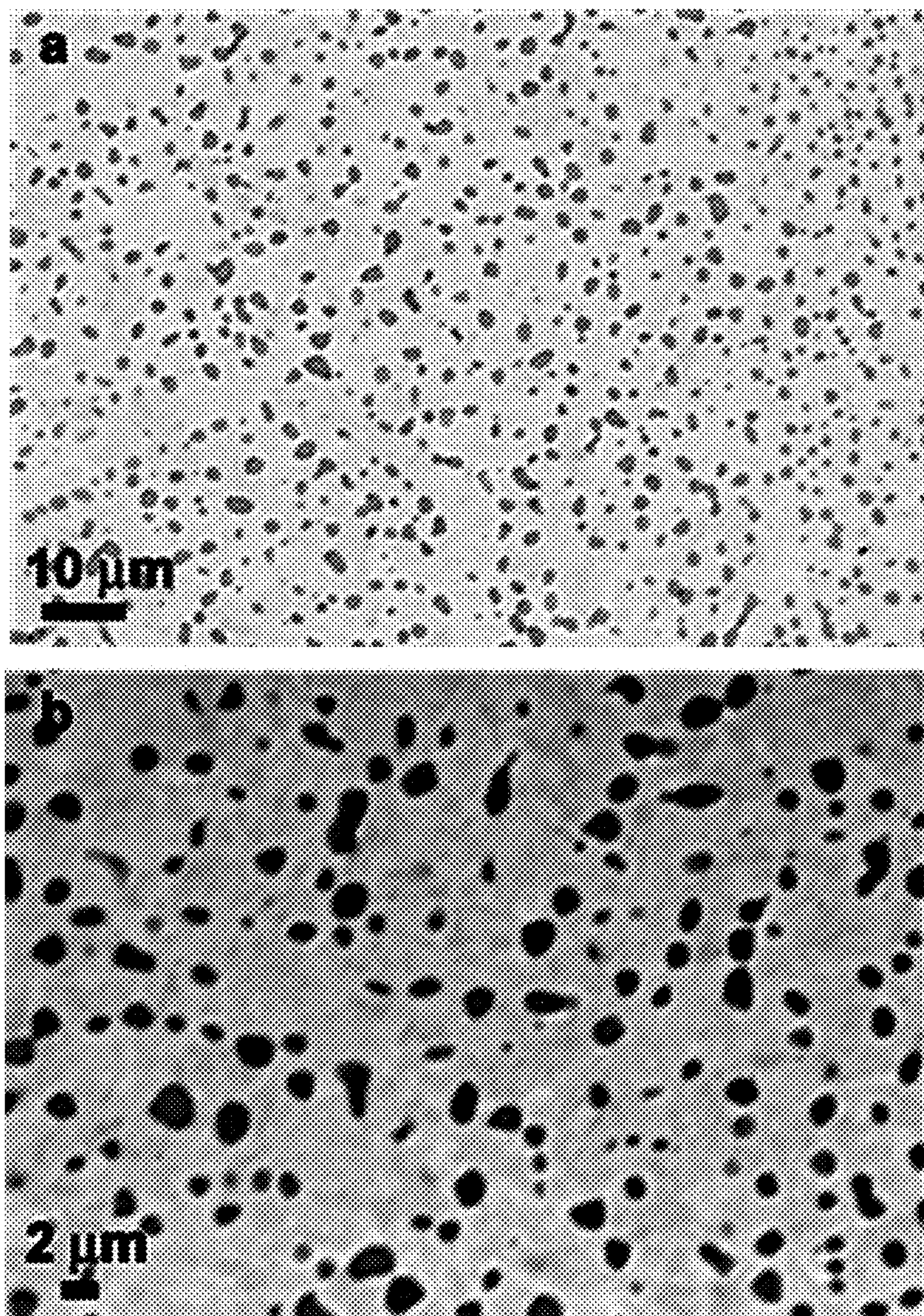
FIG. 41 The backscattered SEM images of the microstructure in the Alloy 17 specimen after HIP cycle at 1100°C for 1 hr and heat treatment at 700°C for 1 hr (prior deformation).
