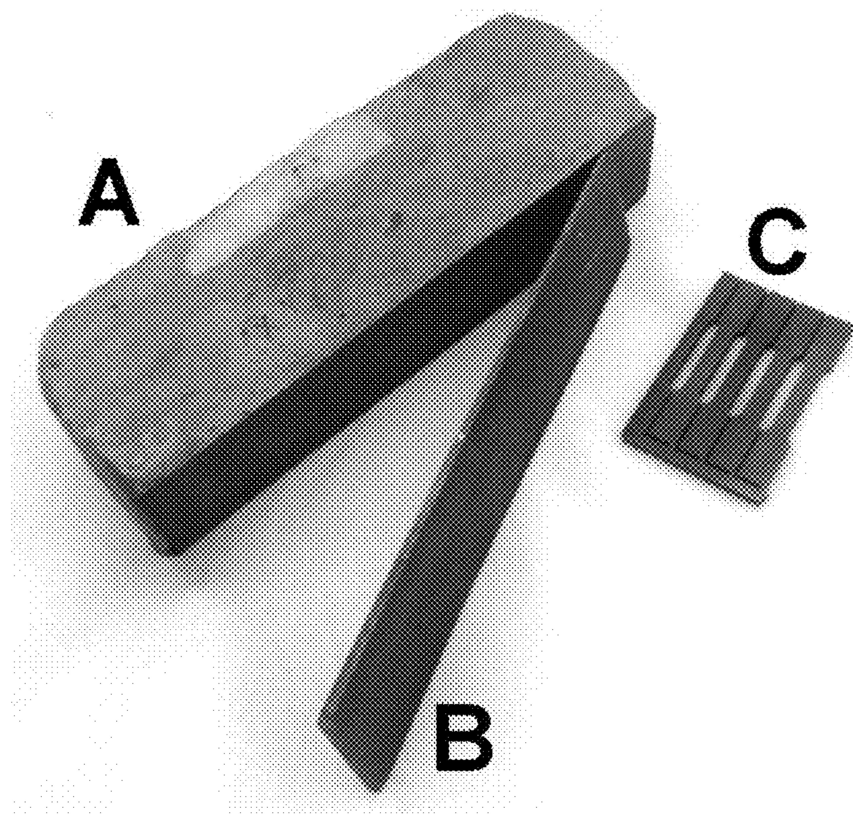
FIG. 72 As-cast plate with thickness of 1 inch (A), a thin sheet cut from the plate (B) and tensile specimens (C) from Alloy 6.
