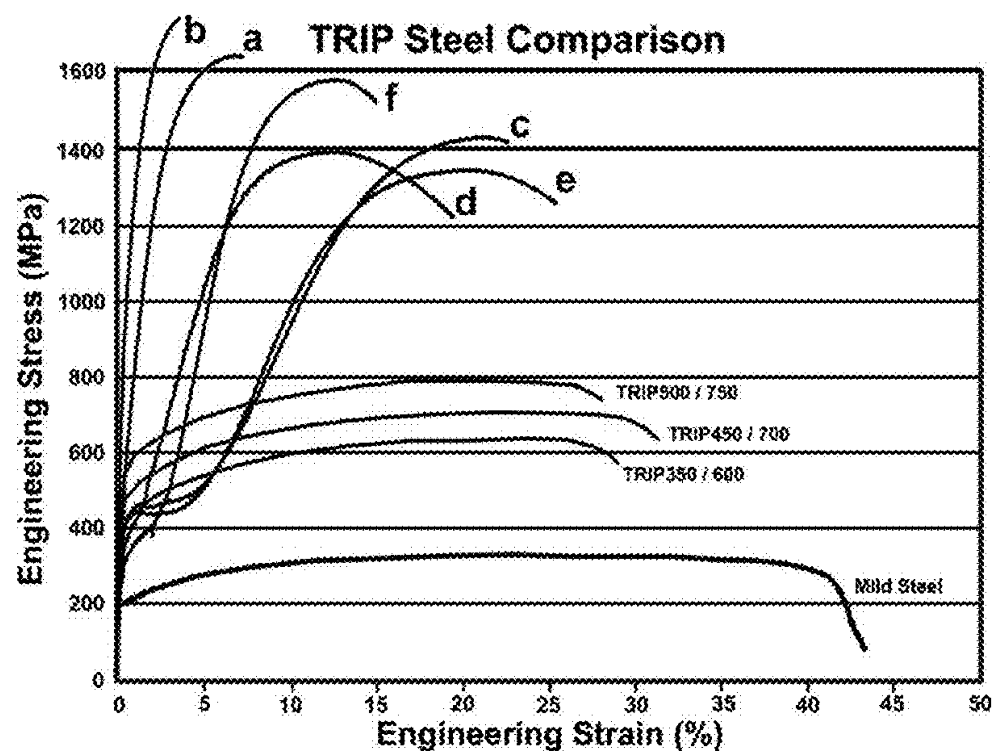
FIG. 11 Comparison of stress-strain curves of new non-stainless steel sheet types with existing Transformation Induced Plasticity (TRIP) steels.
