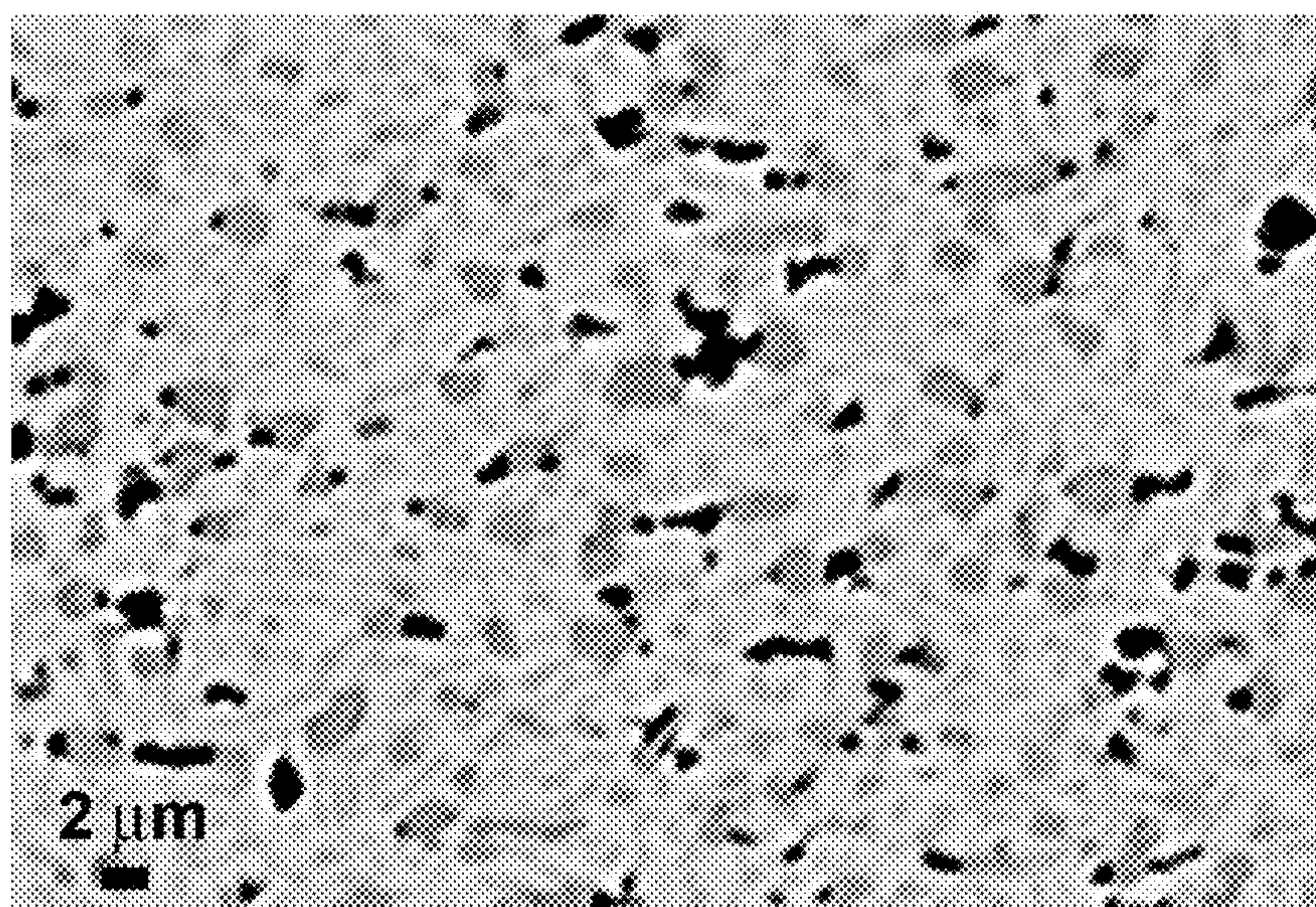
FIG. 63 The backscattered SEM micrograph of the gage microstructure of Alloy 20 specimen after tension at 700°C with tensile elongation of 88.5%.
