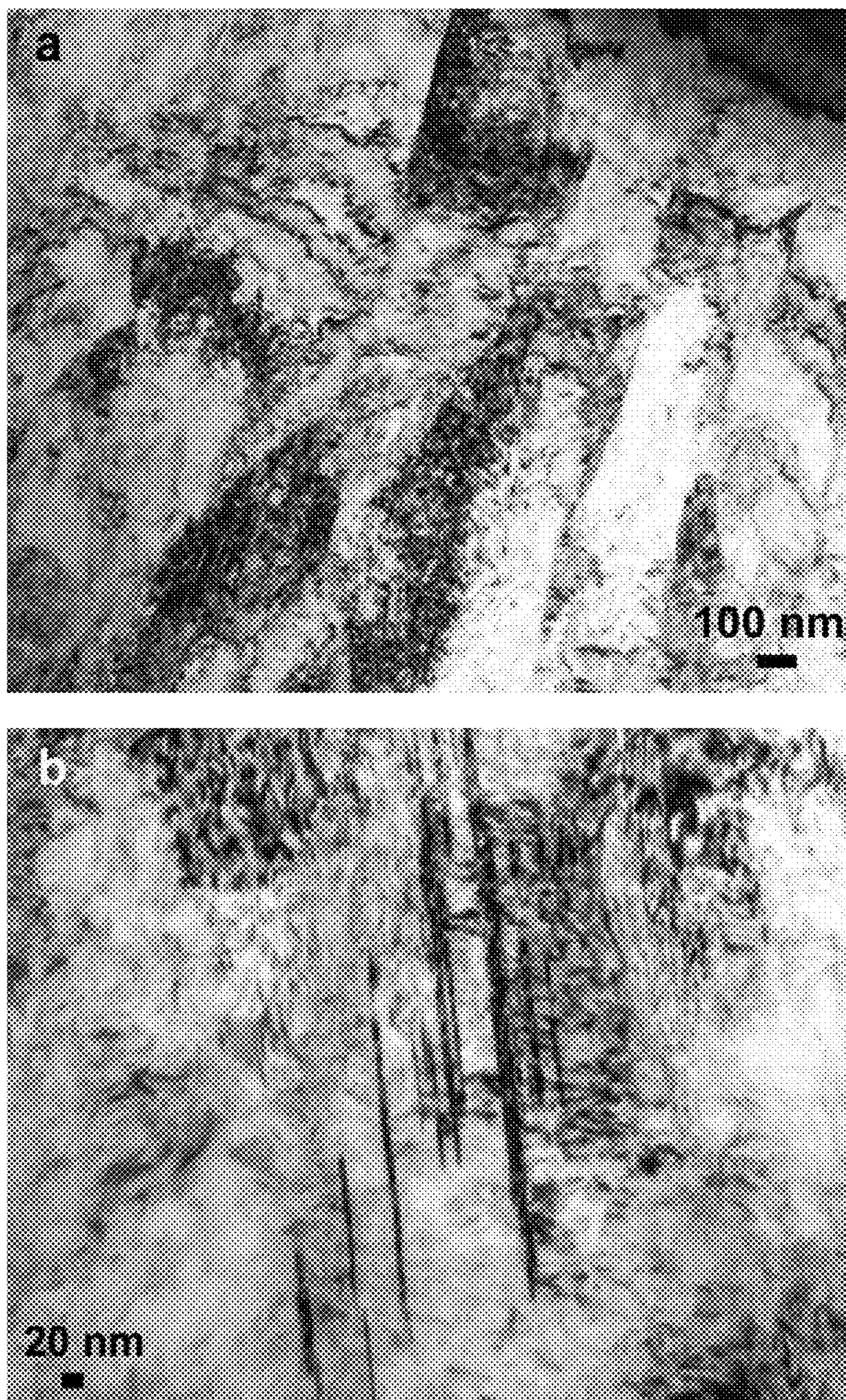
FIG. 71 The bright-field TEM micrographs of the microstructure in the Alloy 22 specimen gage after tension at 850°C with tensile elongation of 13.5%.
