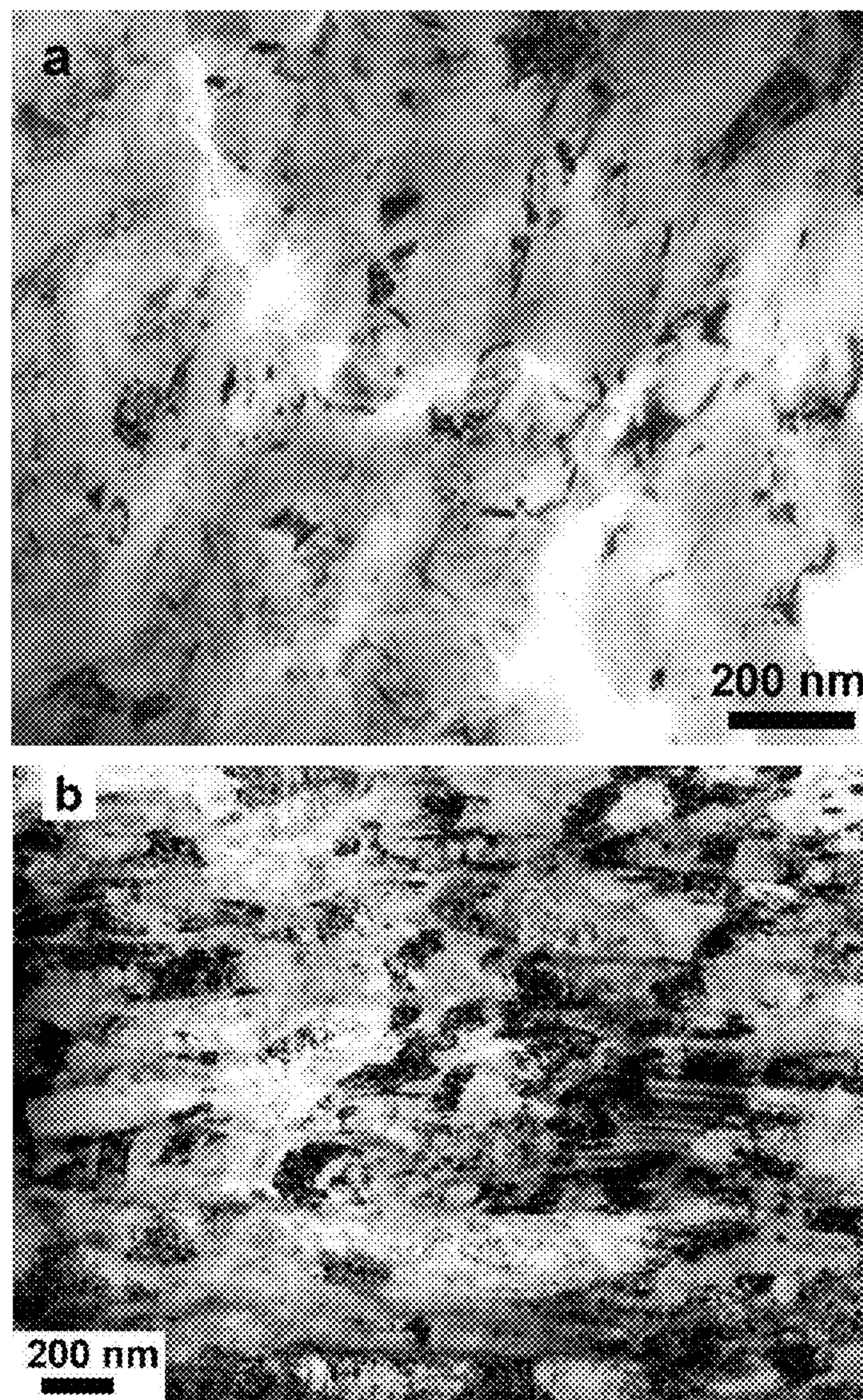
FIG. 32 TEM micrographs of microstructure in the specimen from the Alloy 51 plate HIPed at 1100°C for 1 hour and heat treated at 700°C for 1 hour; a) Before tensile testing; b) After tensile testing.
