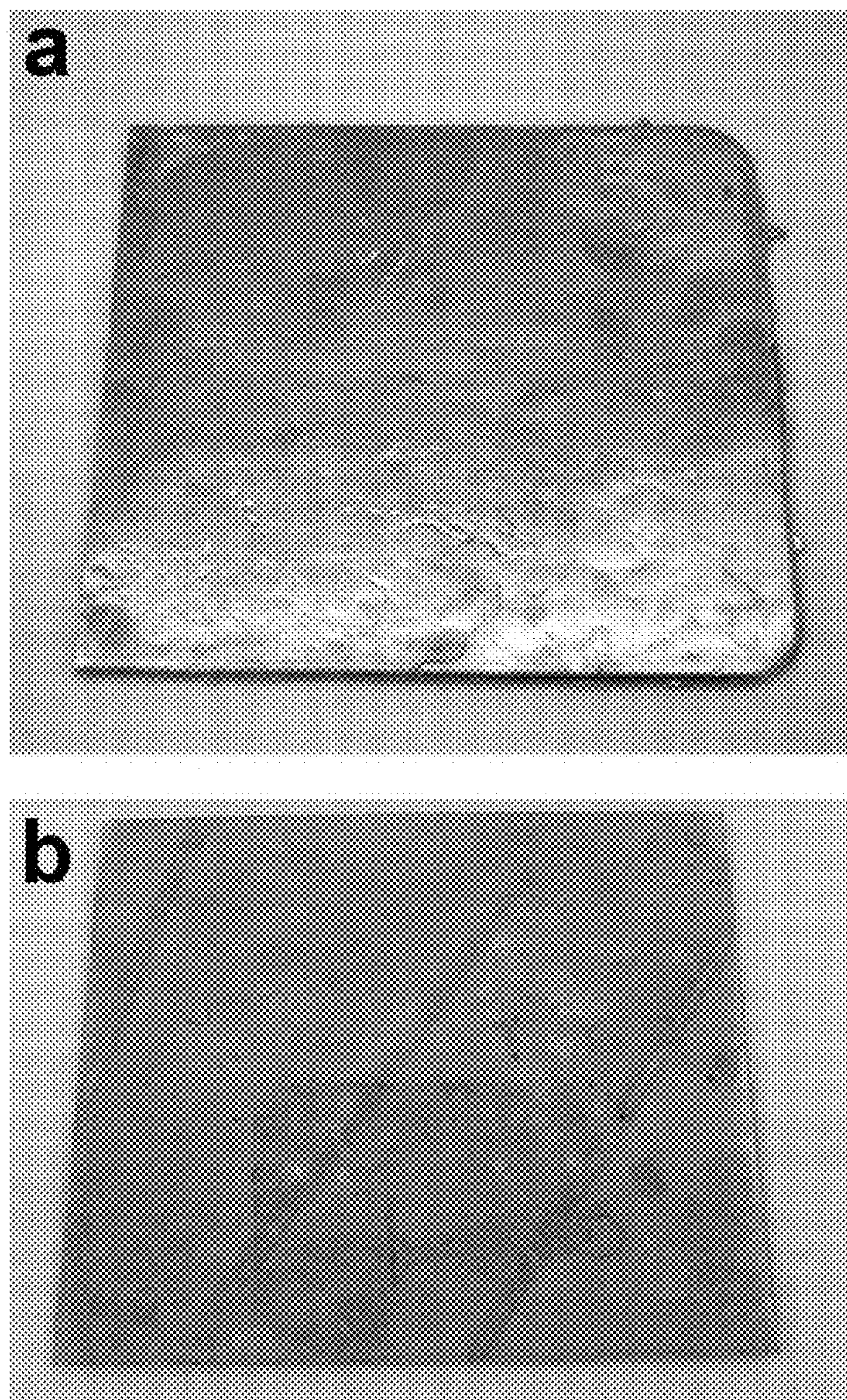
FIG. 8 Pictures of the Alloy 6 plate; a) As-cast, b) After HIP cycle C at 1100°C for 1 hour.
