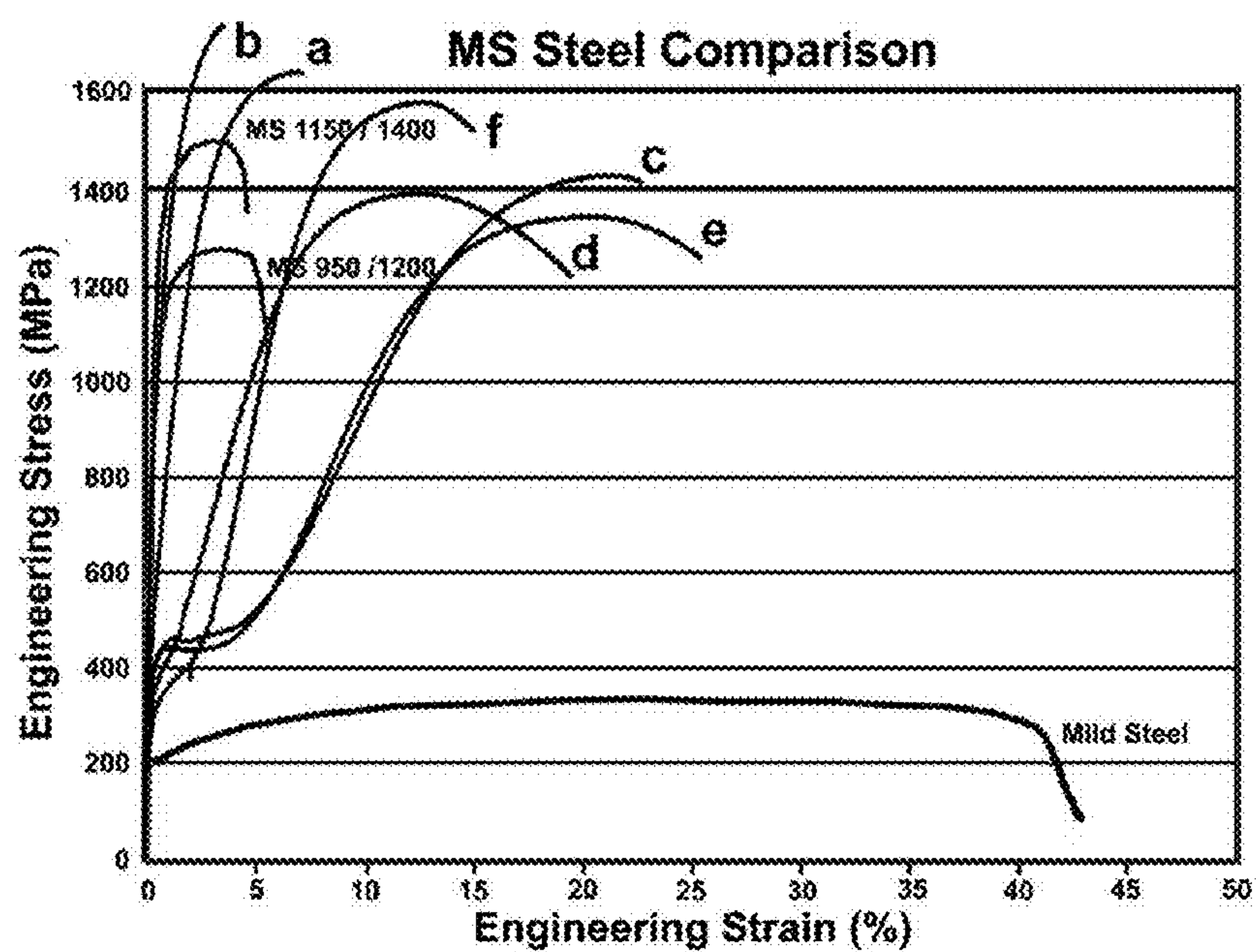
FIG. 12 Comparison of stress-strain curves of new non-stainless steel sheet types with existing Martensitic (MS) steels.
