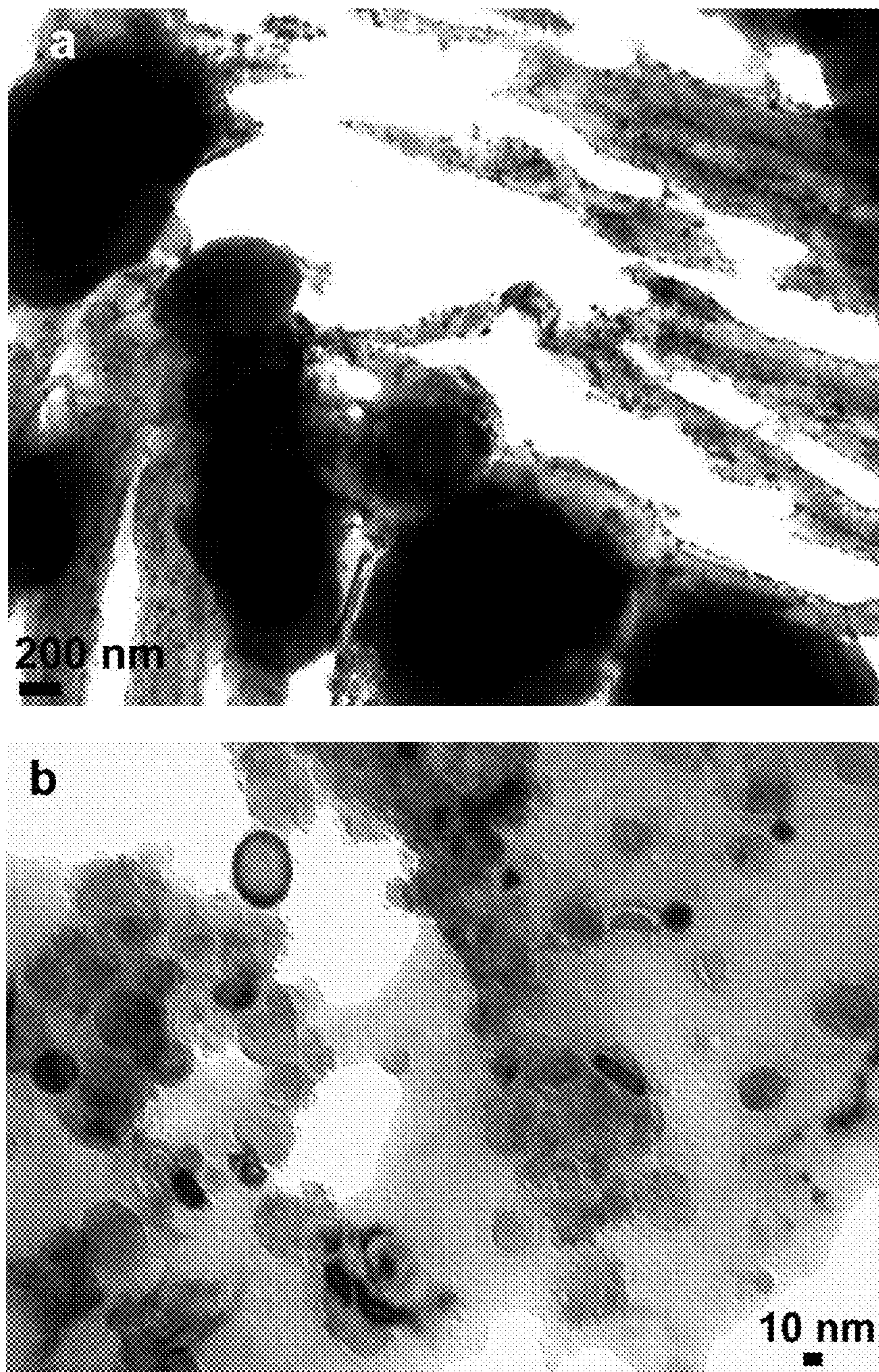
FIG. 67 The bright-field TEM micrographs of the microstructure in the Alloy 20 specimen gage after tension at 700°C with tensile elongation of 88.5%.
