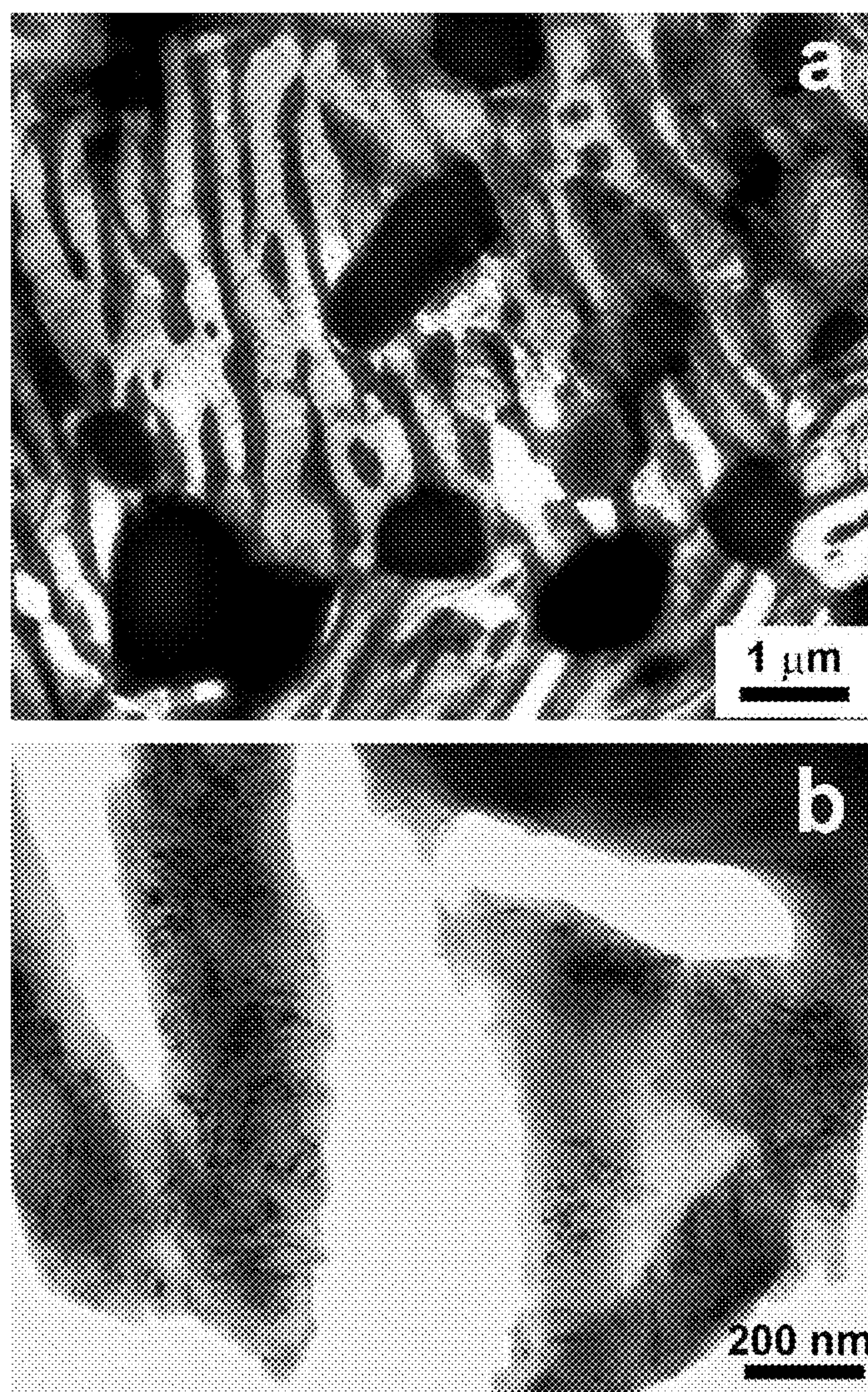
FIG. 27 The TEM micrographs of the microstructure in the Alloy 6 plate sample after HIP cycle at 1100°C for 1 hour and heat treatment at 700°C for 60 minutes with slow furnace cooling. (a) The precipitates grew slightly, but the lath structure in the matrix developed into lamellae structure. (b) A structure of the matrix at higher magnification.
