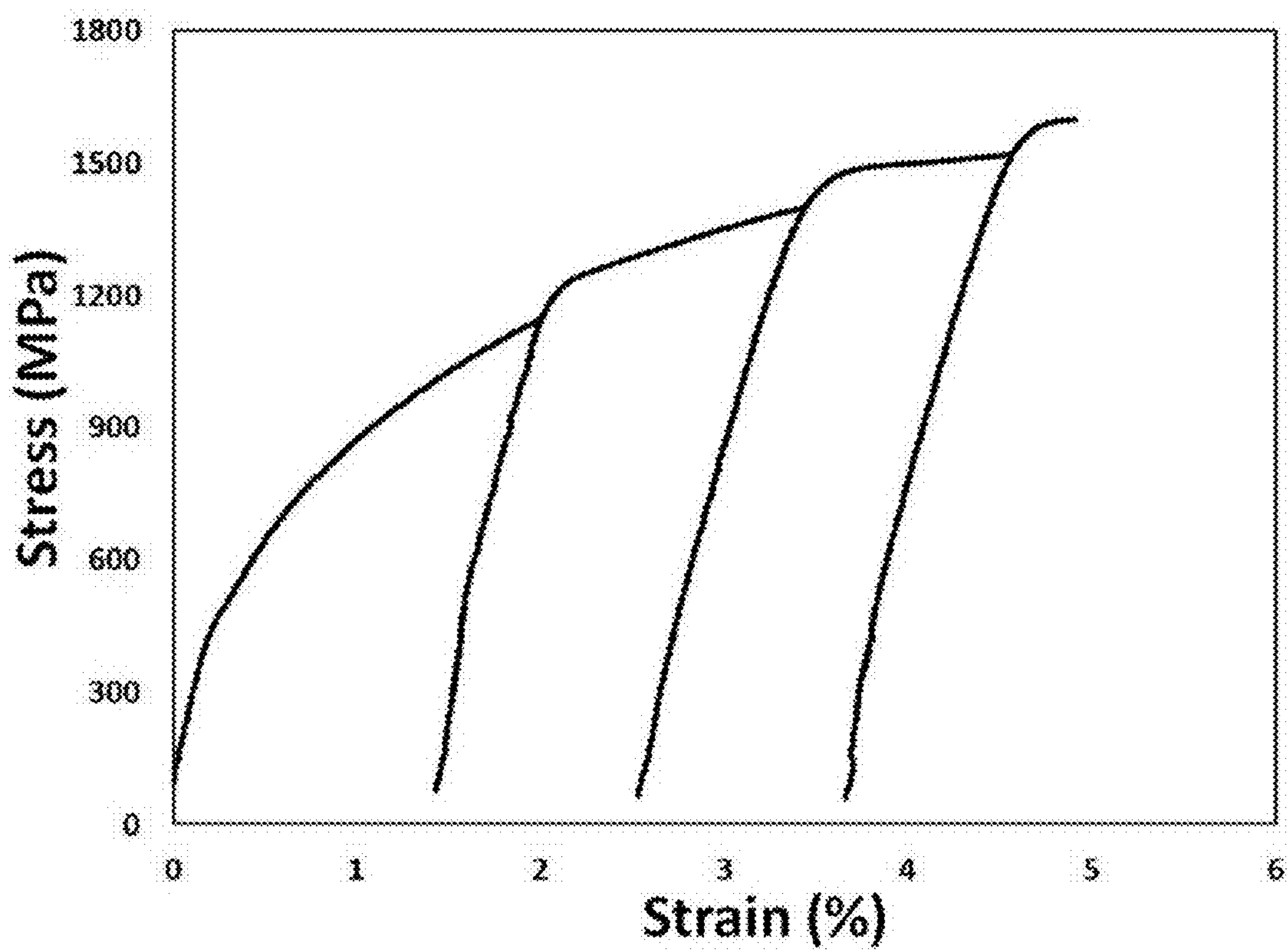
FIG. 49 Stress-strain curves for the Alloy 6 specimen tested in tension with incremental straining.
