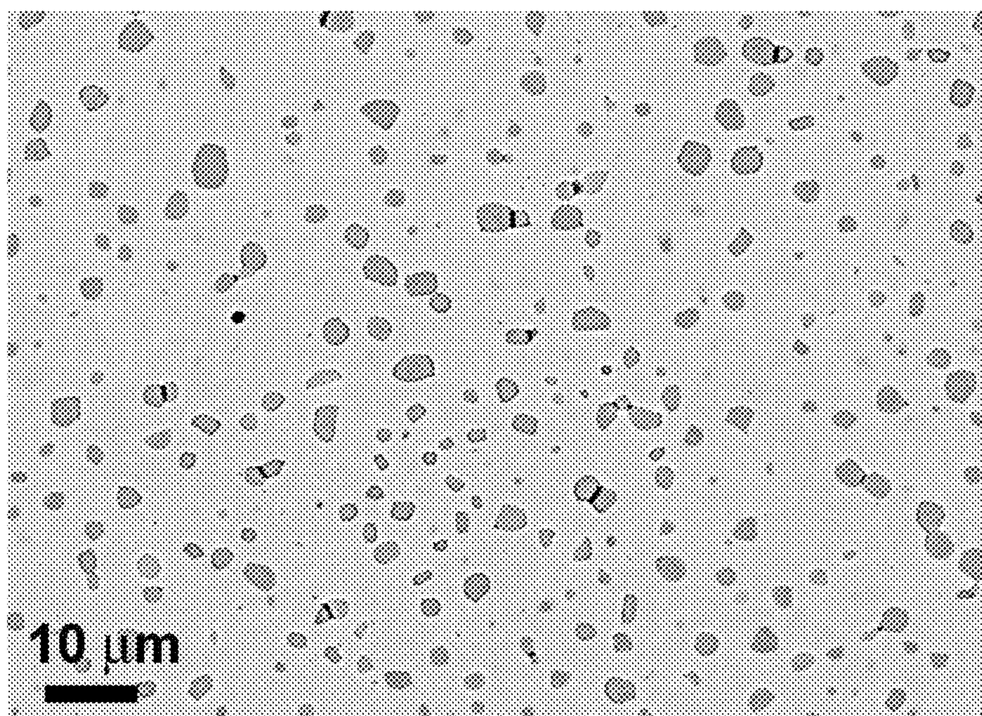
FIG. 59 A SEM image of the microstructure in the gage of the tensile specimen from the Alloy 51 after cycling deformation to 10% and annealing at 1100°C for 1 hour (3 times), then tested to failure.
