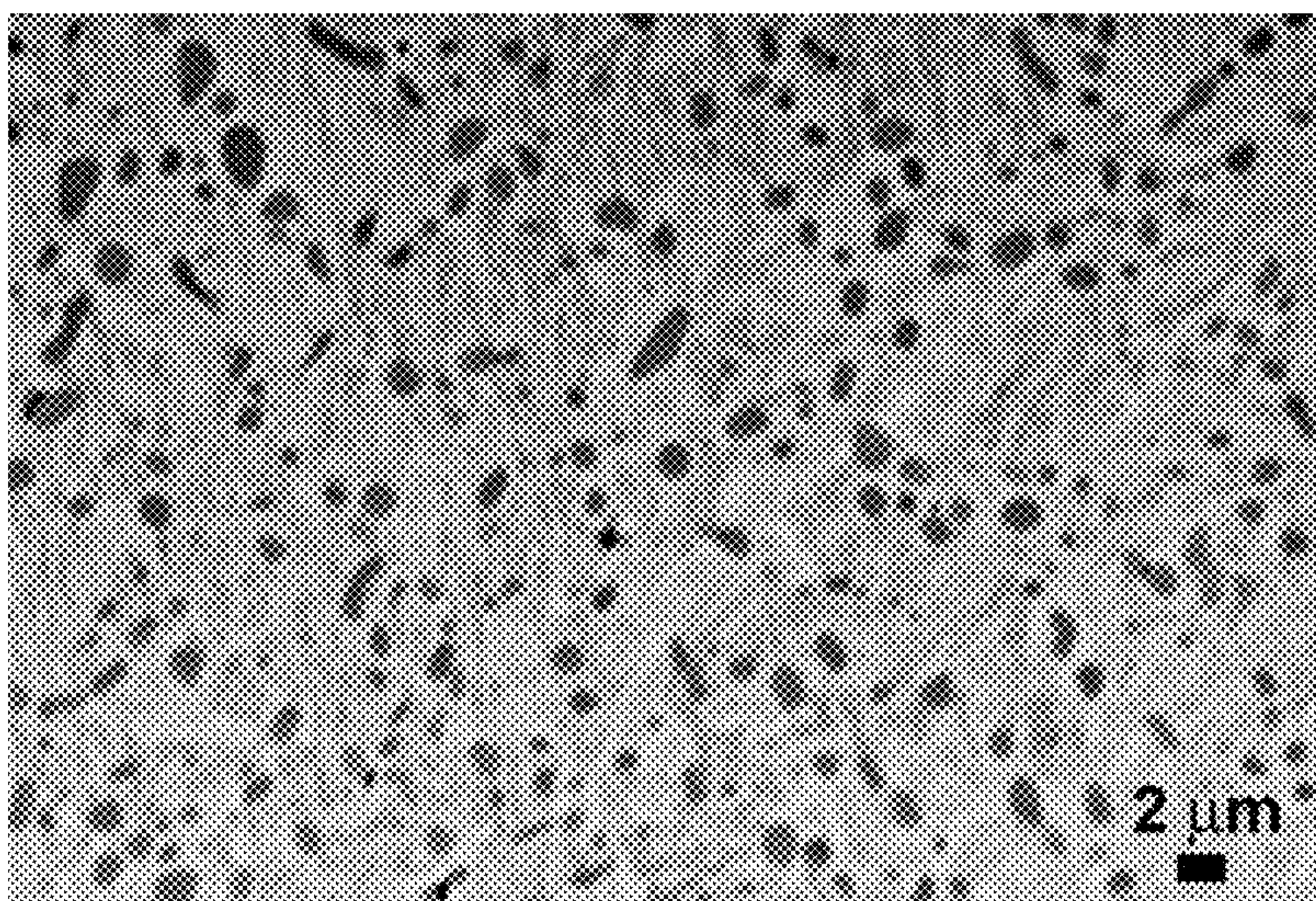
FIG. 20 The backscattered SEM micrograph of the microstructure in the Alloy 6 plate sample after HIP cycle at 1100°C for 1 hour and heat treated at 700°C for 60 minutes with slow furnace cooling.
