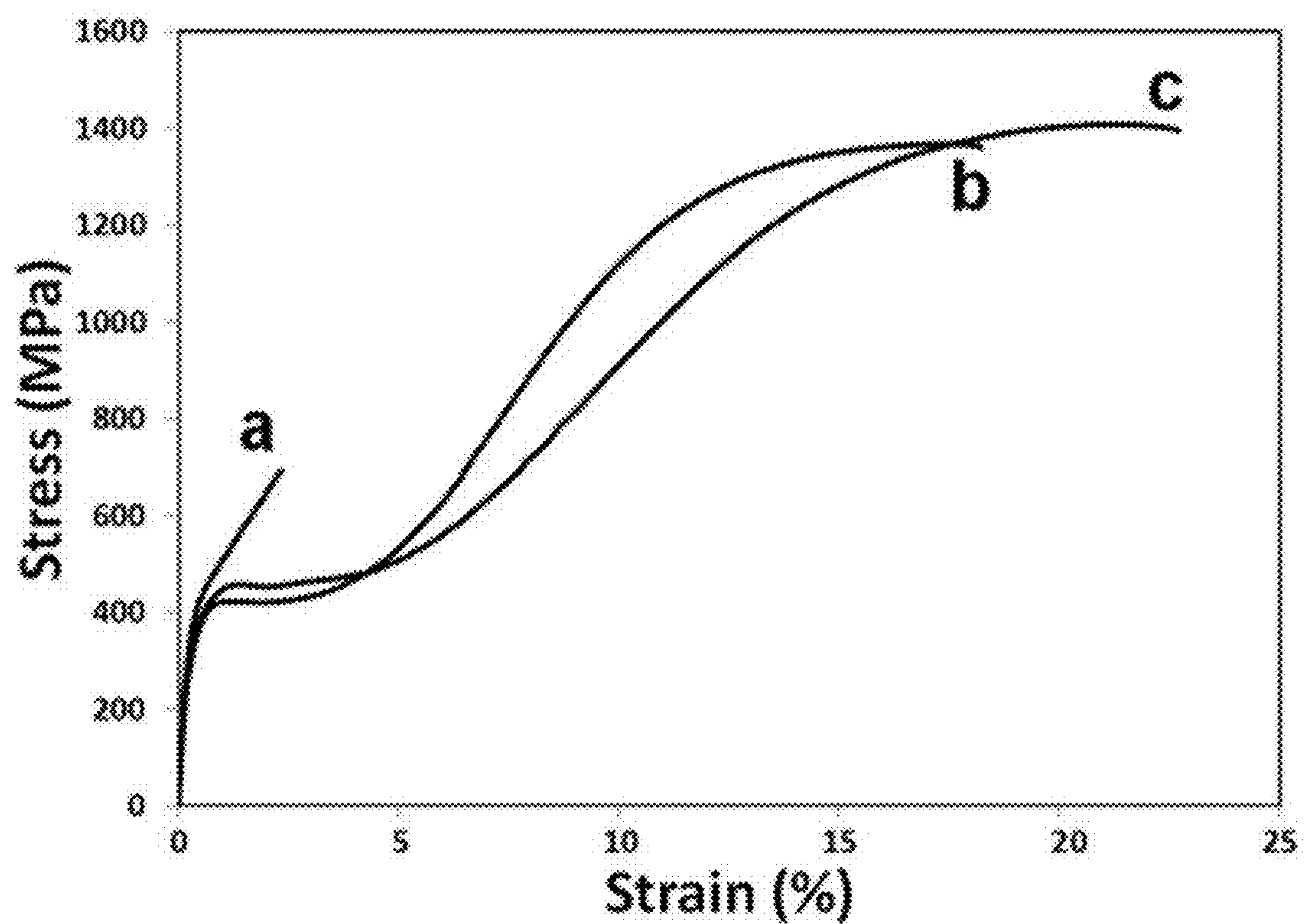
FIG. 28 Tensile properties of Alloy 51 plate in various conditions; a) As-cast, b) After HIP cycle at 1100°C for 1 hour and c) After HIP cycle at 1100°C for 1 hour and heat treating at 700°C for 1 hour.
