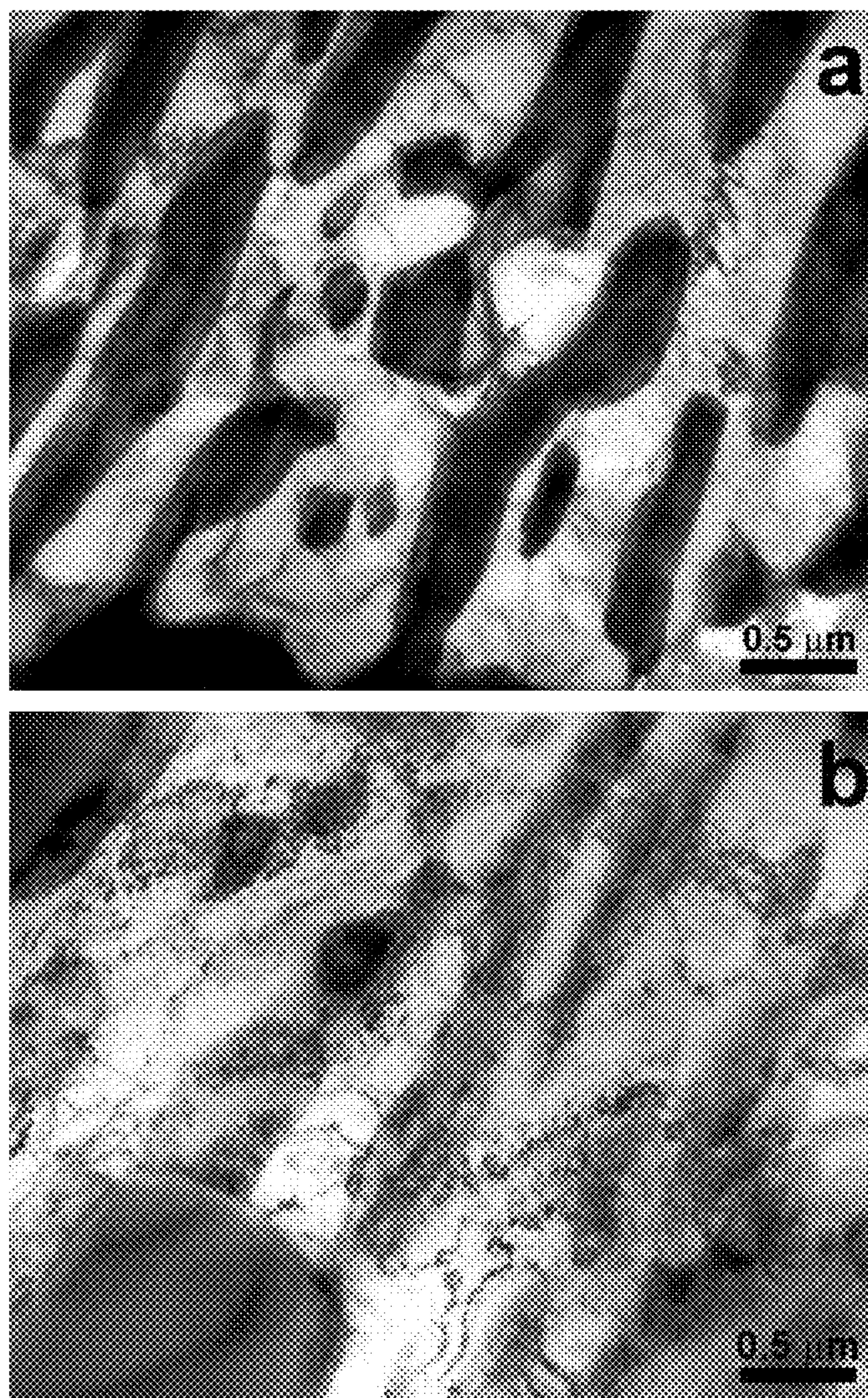
FIG. 39 TEM micrographs of the microstructure in the specimen from the Alloy 6 plate after HIP cycle at 1100°C for 1 hour and heat treatment at 700°C for 60 minutes with slow furnace cooling; a) Before tensile testing; b) After tensile testing.
