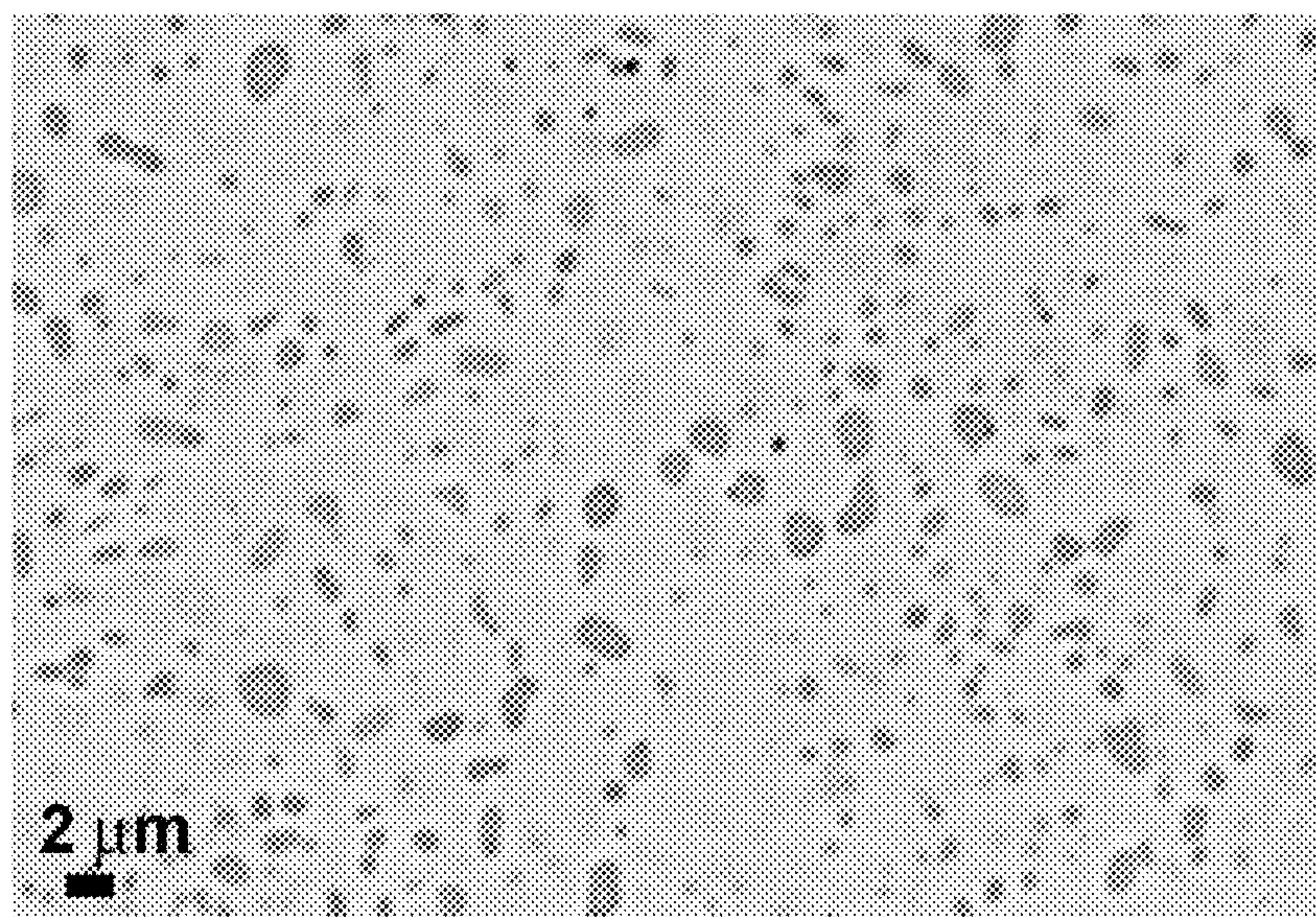
FIG. 66 The backscattered SEM micrograph of the gage microstructure of Alloy 22 specimen after tension at 850°C with tensile elongation of 13.5%.
