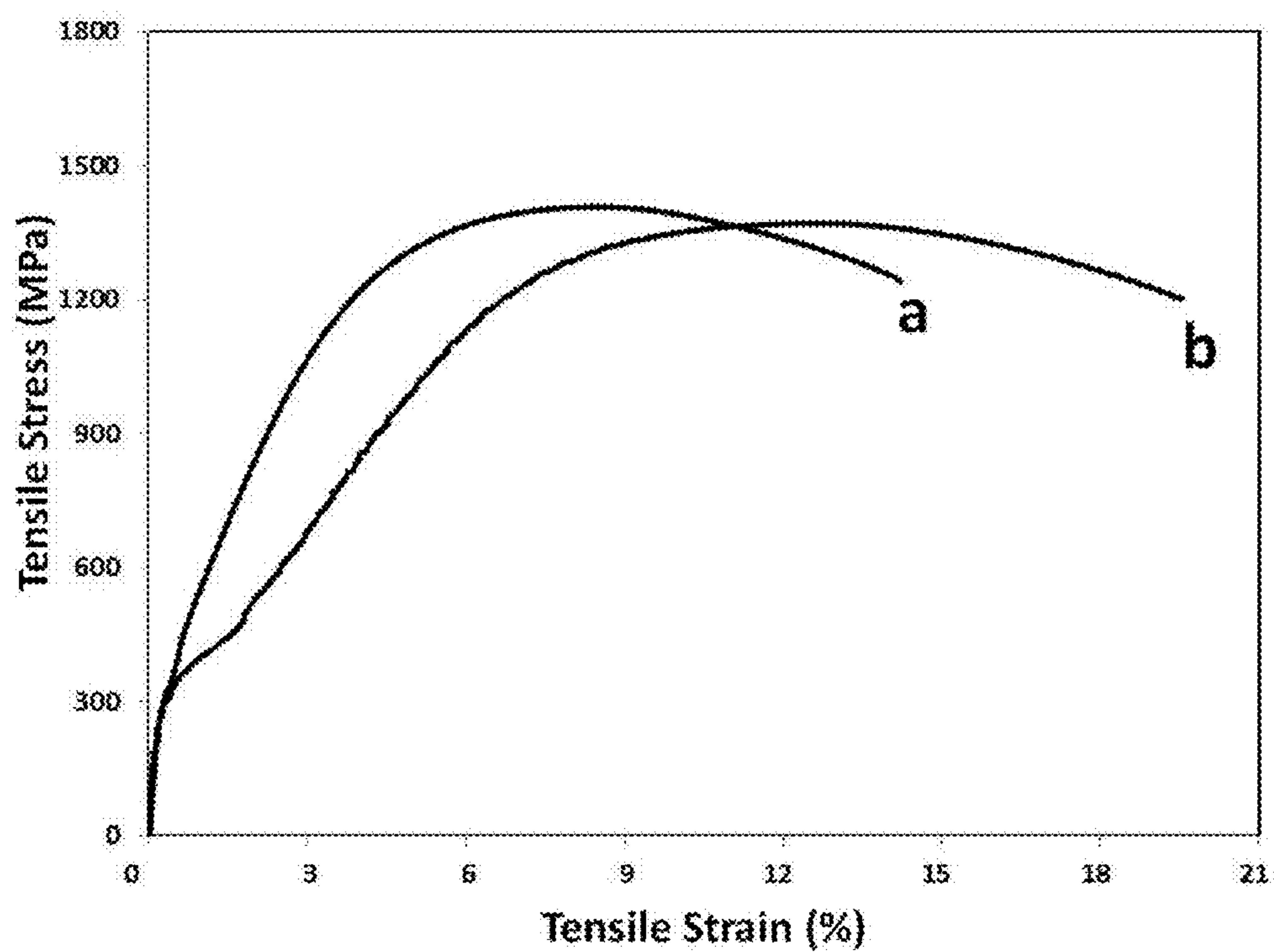
FIG. 45 Stress-strain curves recorded at tensile testing of specimens from the Alloy 52 plate after HIP cycle and heat treatment at (a) 850 °C for 1 with cooling in air and (b) 700 °C for 1 with slow cooling with furnace.
