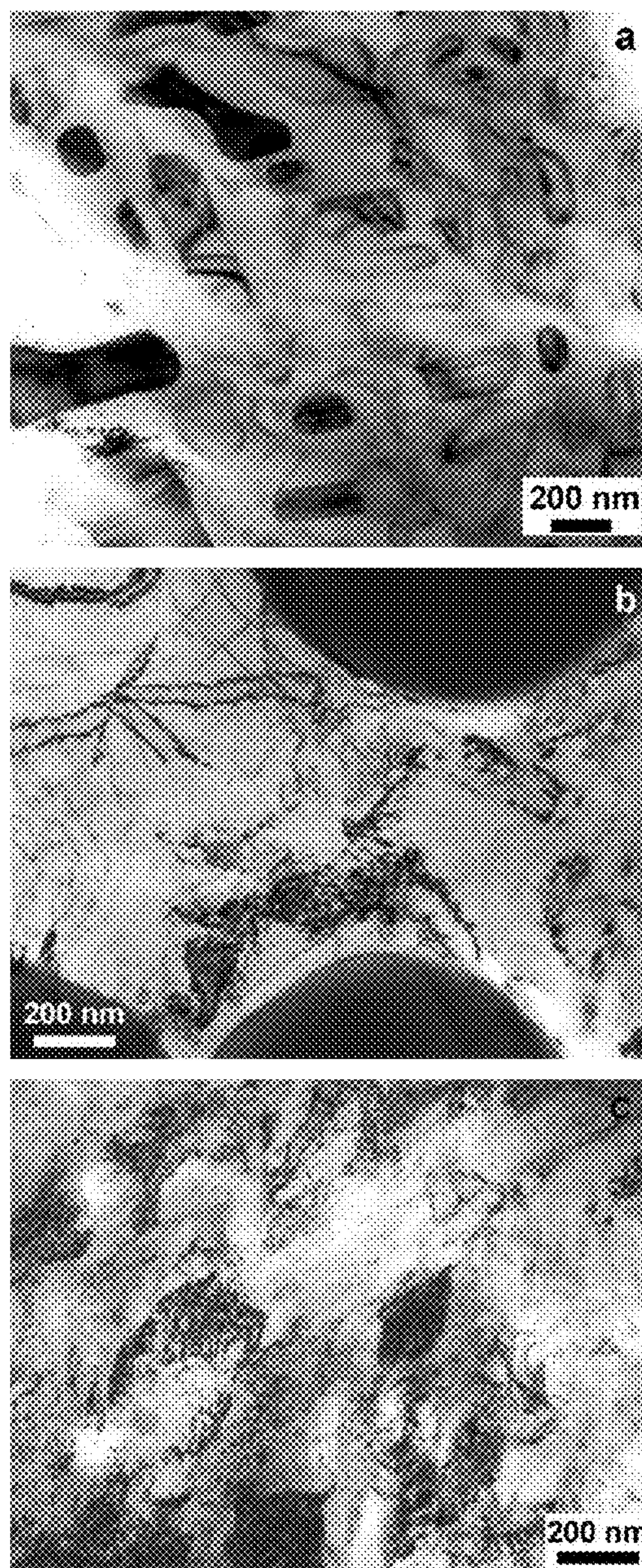
FIG. 17 TEM micrographs of the Alloy 51 plate sample; a) As-Cast, b) HIPed at 1100°C for 1 hour, and c) HIPed at 1100°C for 1 hour and heat treated at 700°C for 1 hour. Observations are consistent with SEM and X-ray diffraction analysis results.
