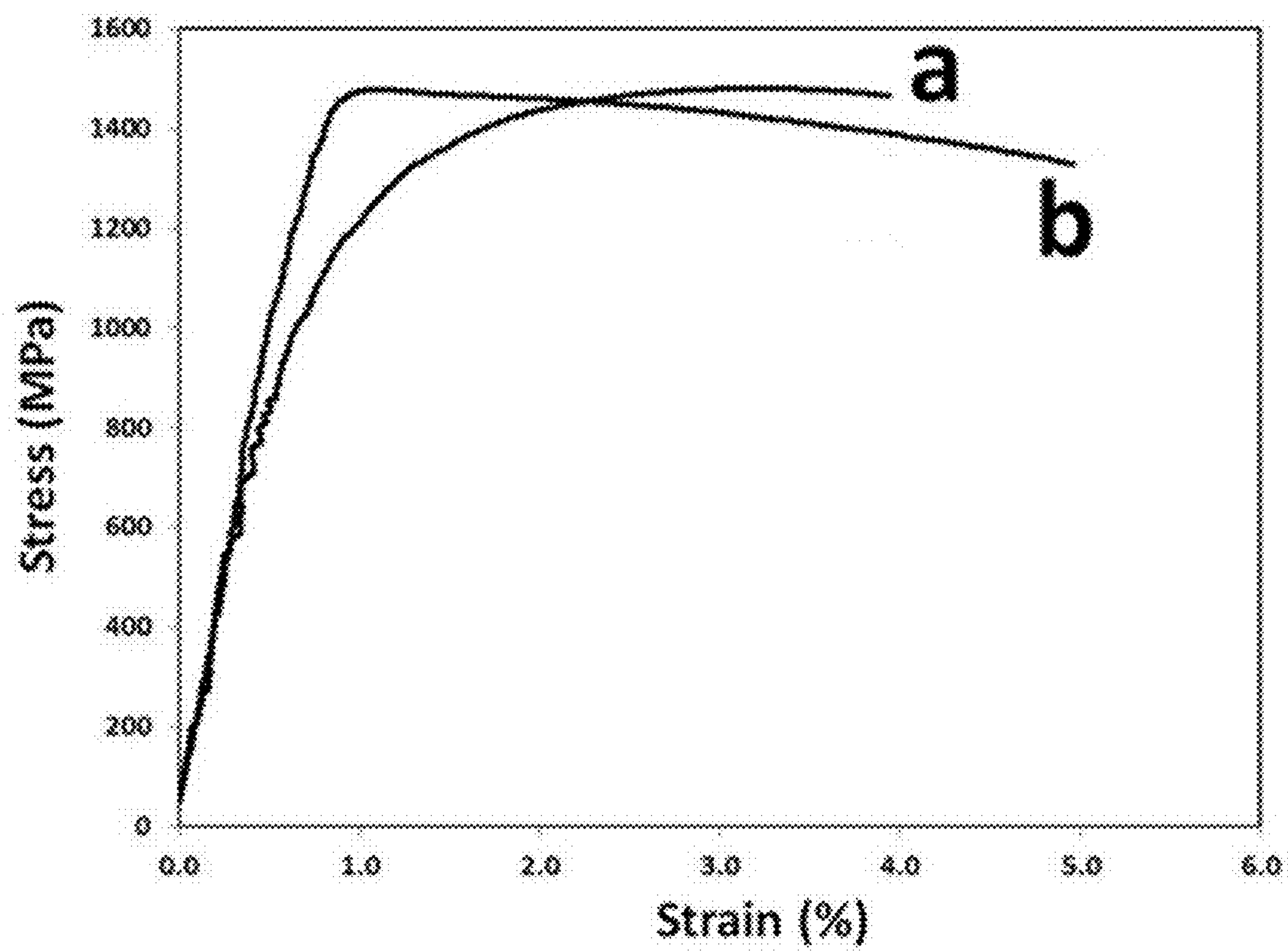
FIG. 52 Stress – strain curves for the Alloy 6 specimens tested (a) in initial state and (b) after pre-straining to 3% and tested to failure.
