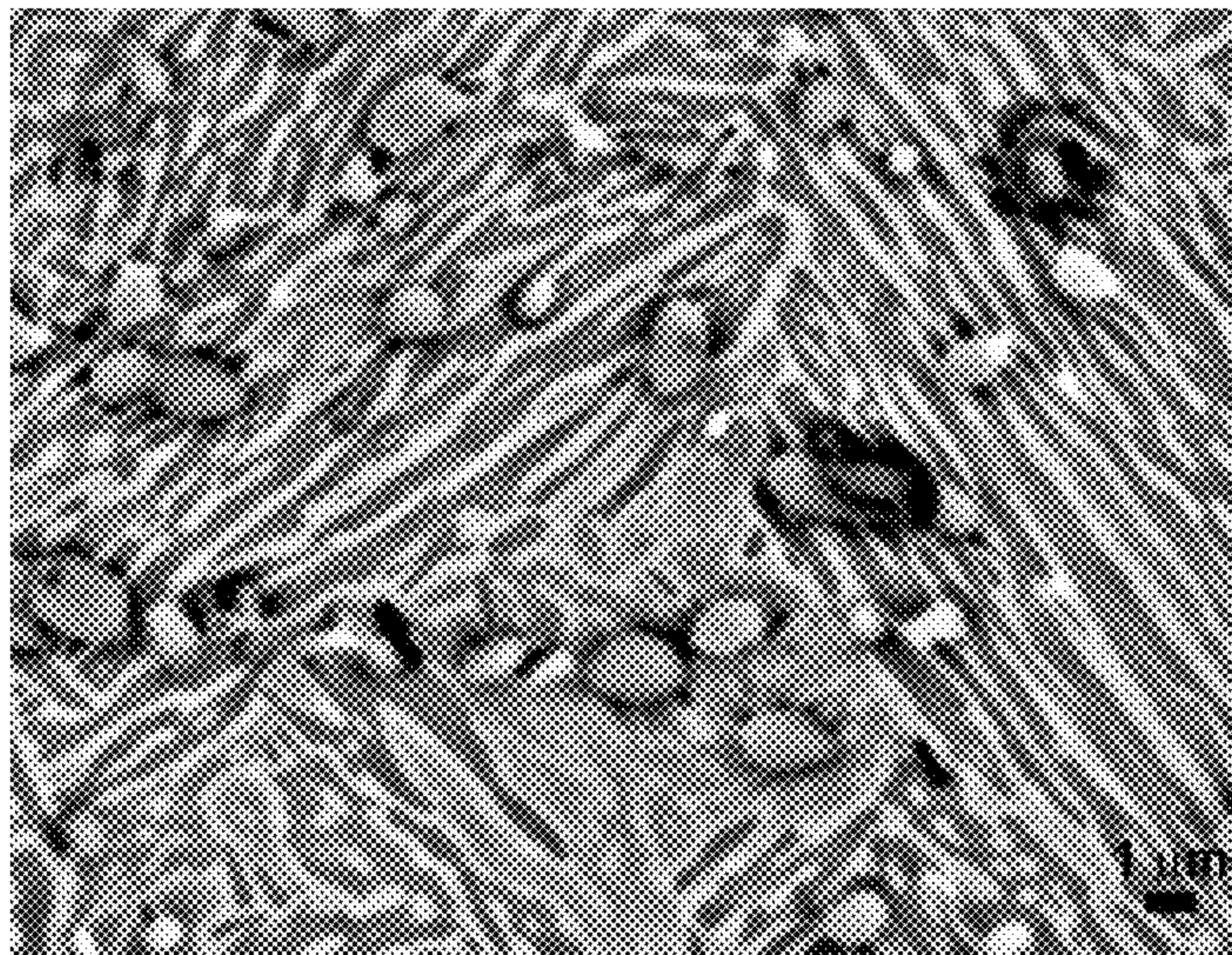
FIG. 21 The backscattered SEM micrograph of the microstructure in the etched Alloy 6 sample after at 1100°C for 1 hour and heat treated at 700°C for 60 minutes with slow furnace cooling at higher magnification.
