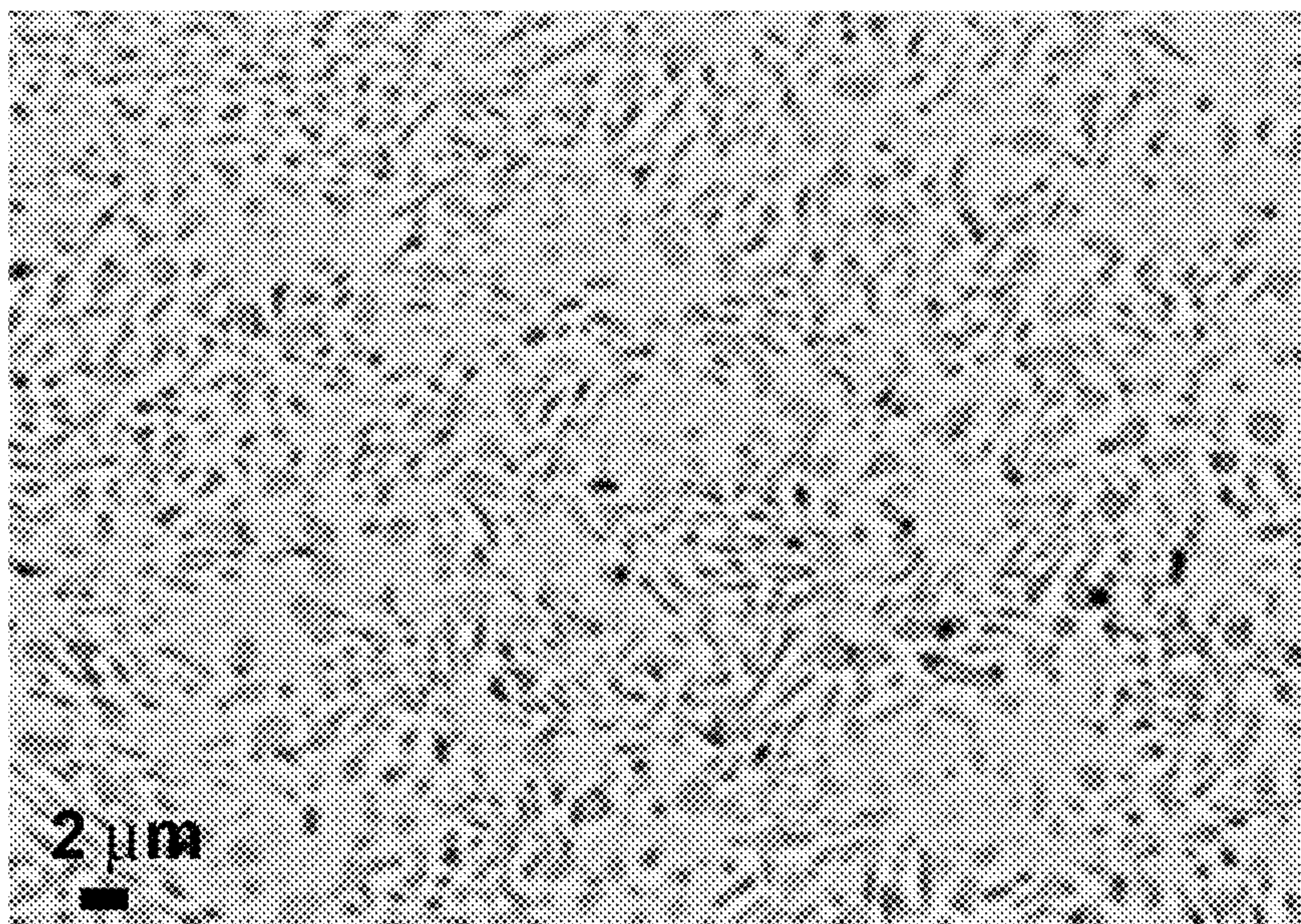
FIG. 65 The backscattered SEM micrograph of the gage microstructure of Alloy 22 specimen after tension at 700°C with tensile elongation of 34.5%.
