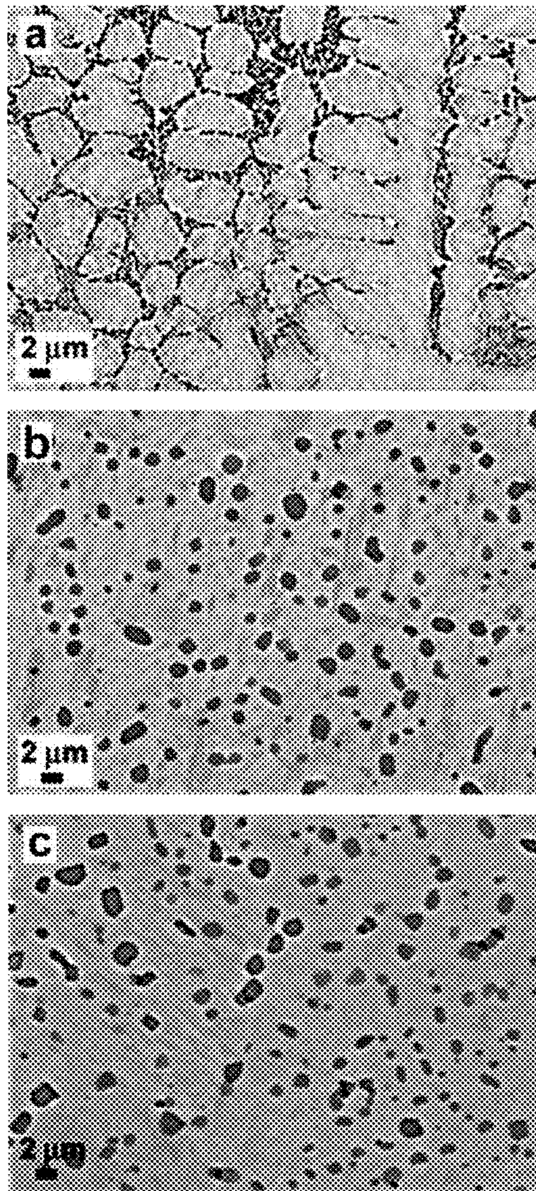
FIG. 13 SEM backscattered electron micrographs of the Alloy 51 plate sample; a) As-Cast, b) HIPed at 1100°C for 1 hour, and c) HIPed at 1100°C for 1 hour and heat treated at 700°C for 1 hour with air cooling.
