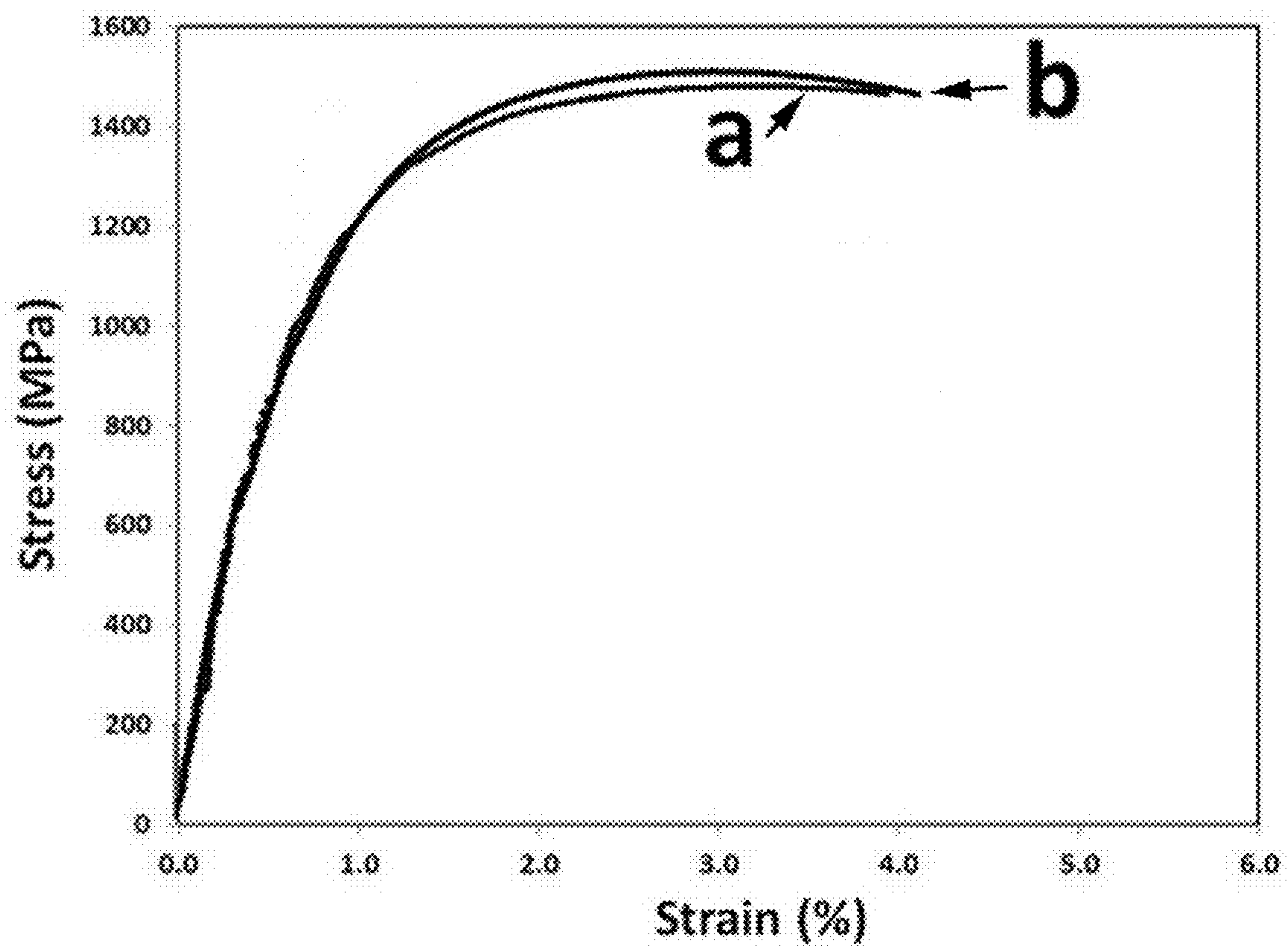
FIG. 55 Stress – strain curves for the Alloy 6 specimens tested (a) in initial state and (b) after pre-straining to 3% and subsequent annealing at 1100 °C for 1 hour.
