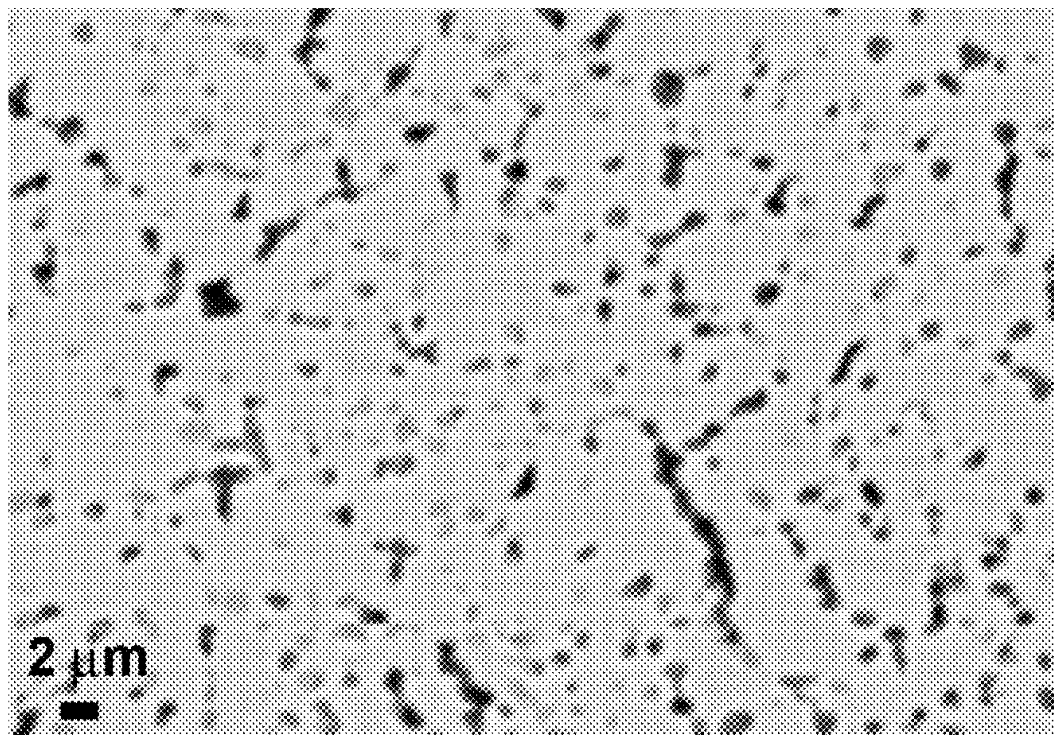
FIG. 64 The backscattered SEM micrograph of the gage microstructure of Alloy 20 specimen after tension at 850°C with tensile elongation of 23%.
