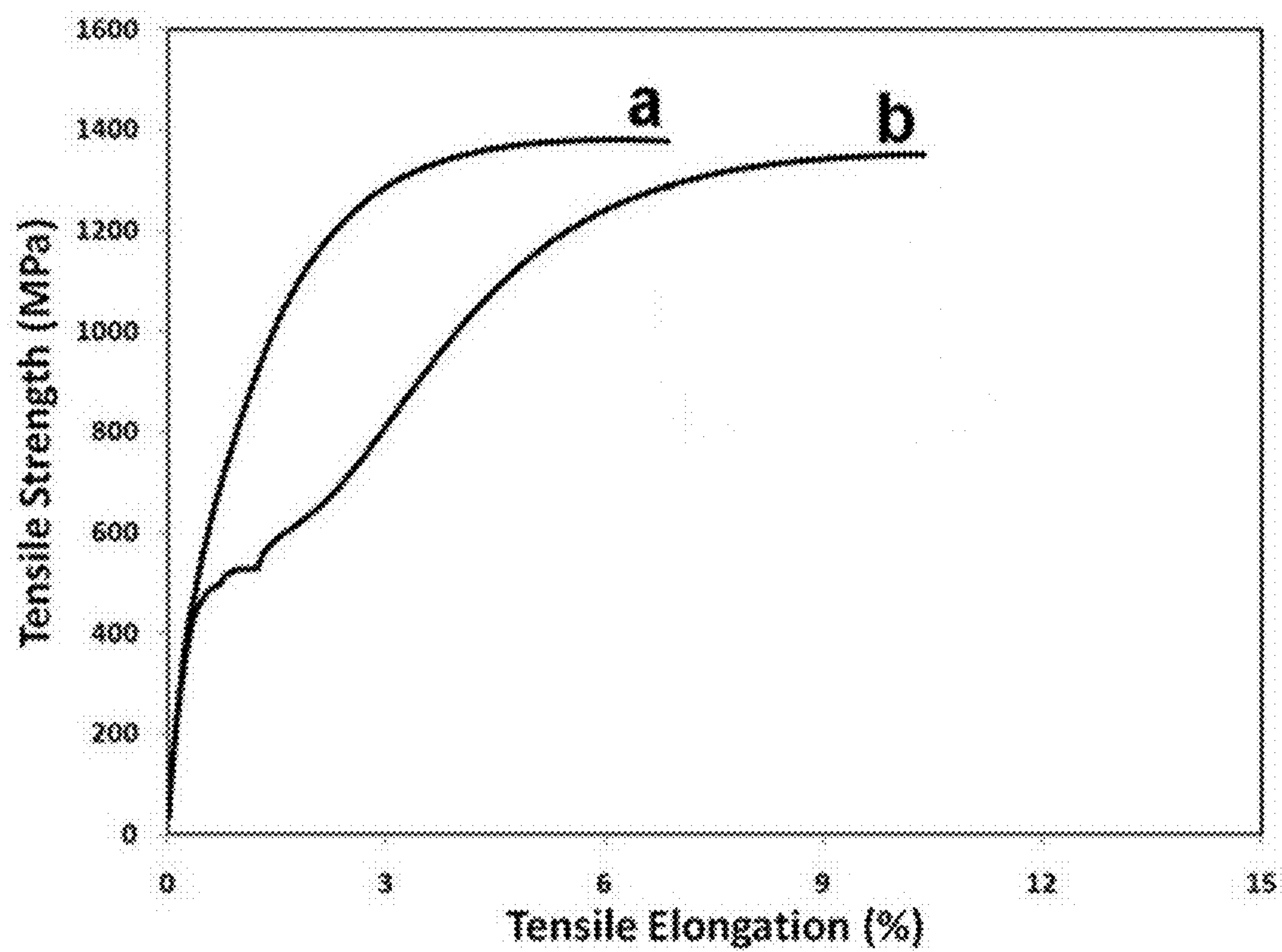
FIG. 43 Stress-strain curves recorded at tensile testing of specimens from the Alloy 2 plate after HIP cycle and heat treatment at 700°C for 1 with cooling (a) in air and (b) with furnace.
