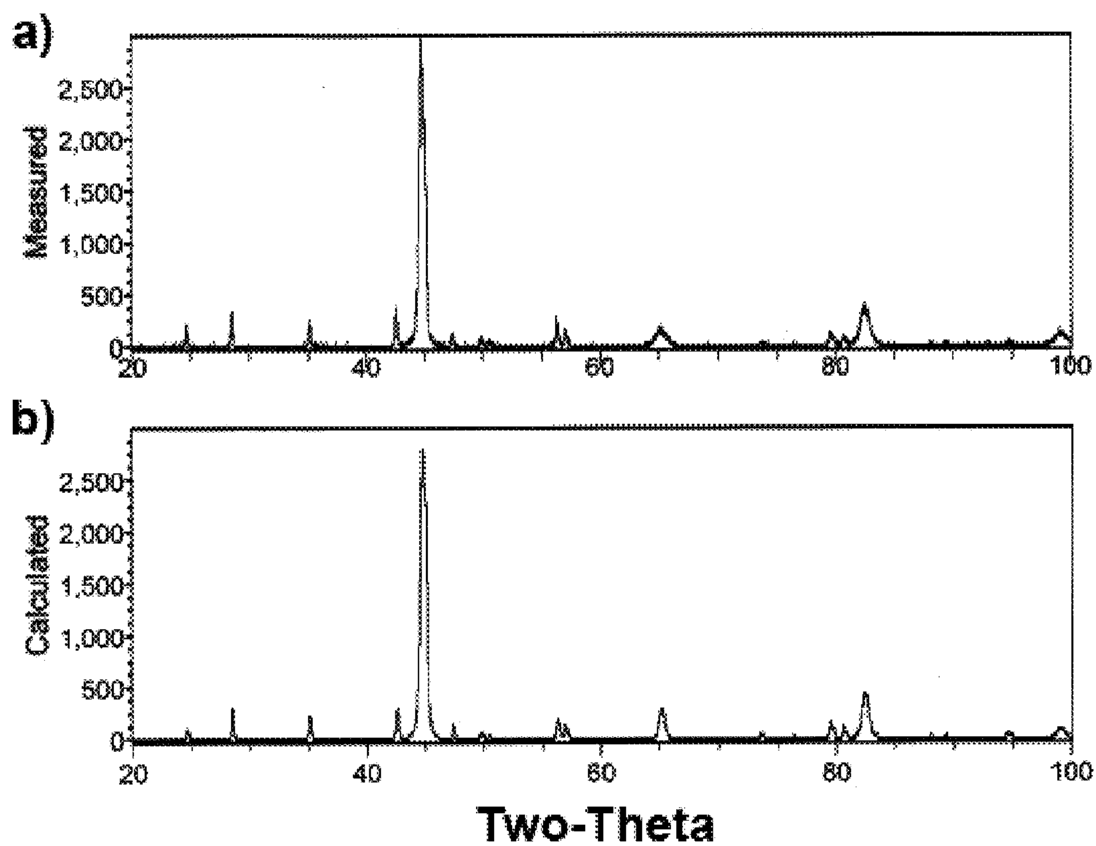
FIG. 23 X-ray diffraction data (intensity vs two-theta) for plate sample from the Alloy 6 in the HIPed condition (1100°C for 1 hour); a) Measured pattern, b) Rietveld calculated pattern with peaks identified.
