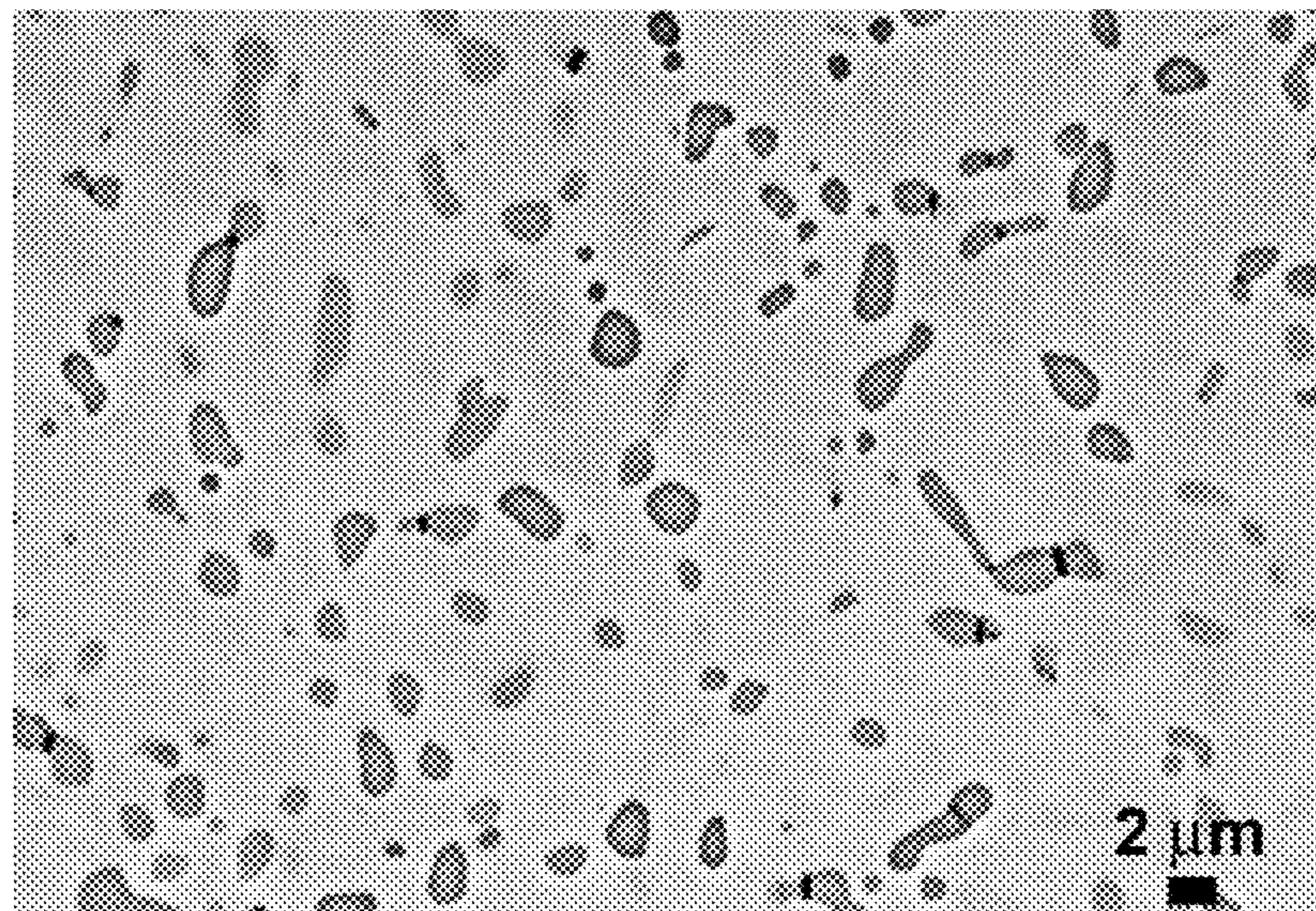
FIG. 19 The backscattered SEM micrograph of the microstructure in the Alloy 6 plate sample after HIP cycle at 1100°C for 1 hour.
