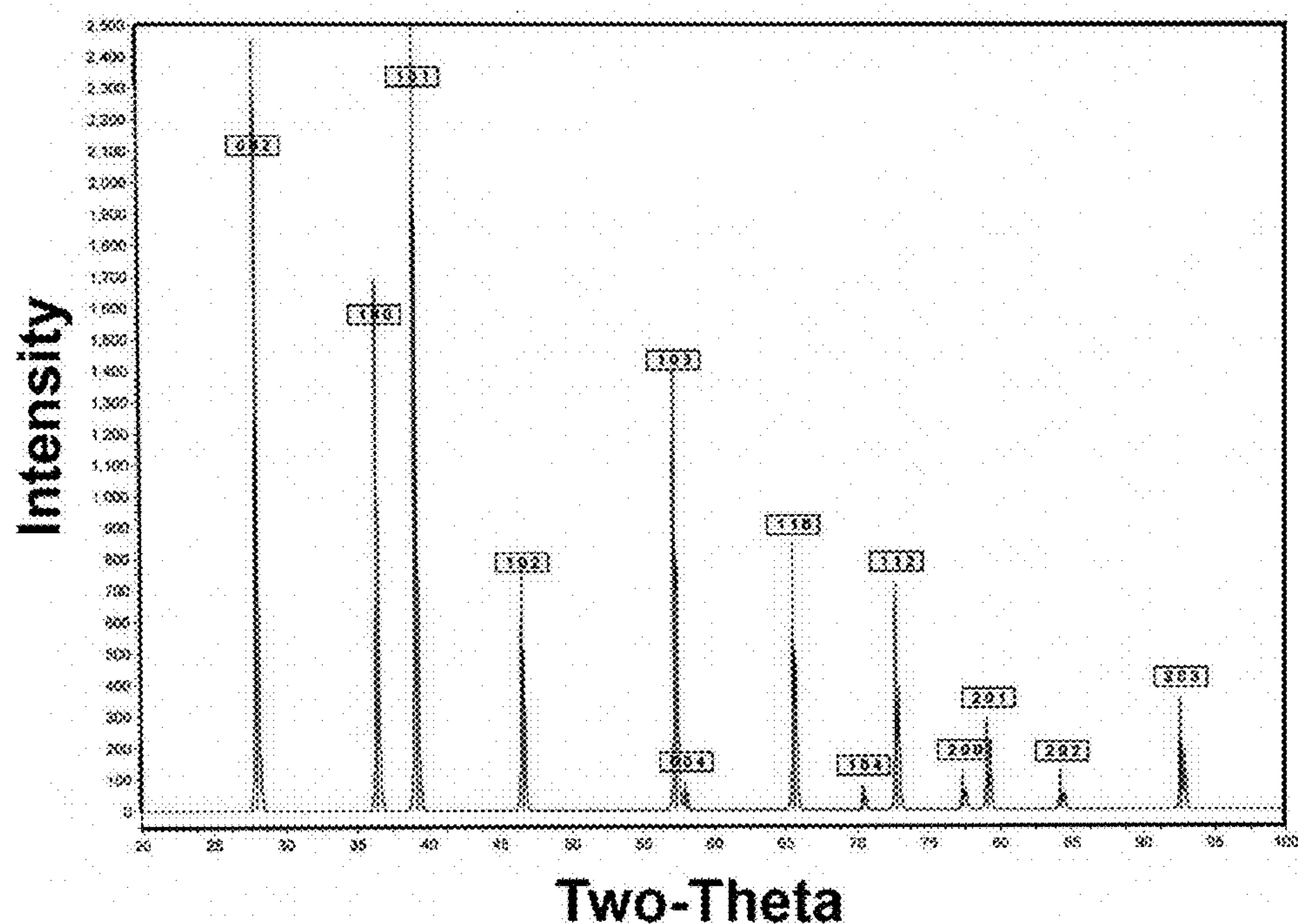
FIG. 38 Calculated X-ray diffraction pattern (intensity vs two-theta) for the newly identified hexagonal phase (space group #186) found in the gage section of tensile tested specimen from Alloy 6 plate in the HIPed condition (1100°C for 1 hour) and heat treated at 700°C slow cool to room temperature (670 minute total time) condition. Note that the diffraction planes are listed in parenthesis.
