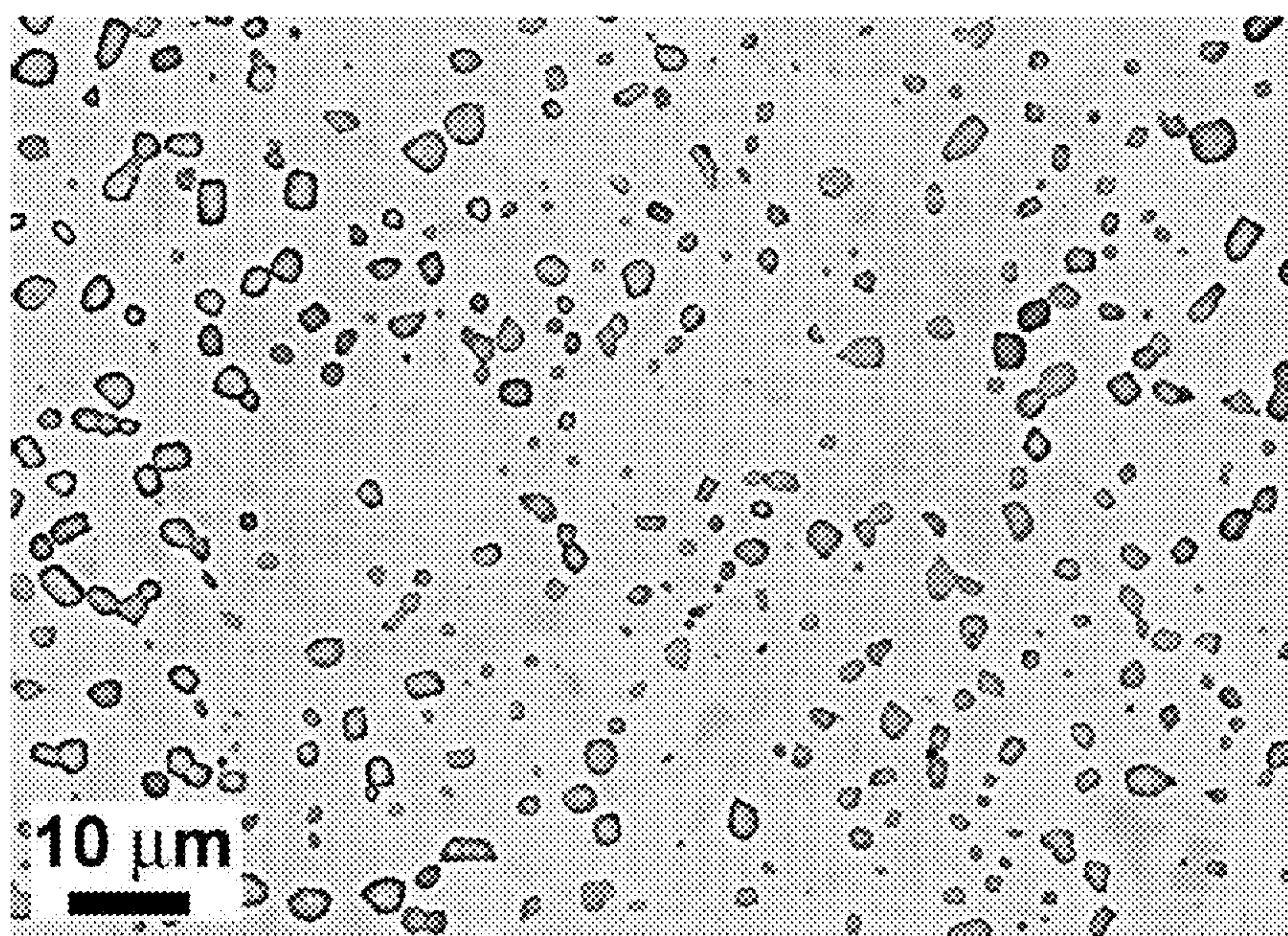
FIG. 54 A SEM image of microstructure of the gage section of the tensile specimens from the Alloy 51 after pre-straining to 10% and annealing at 1100°C for 1 hour.
