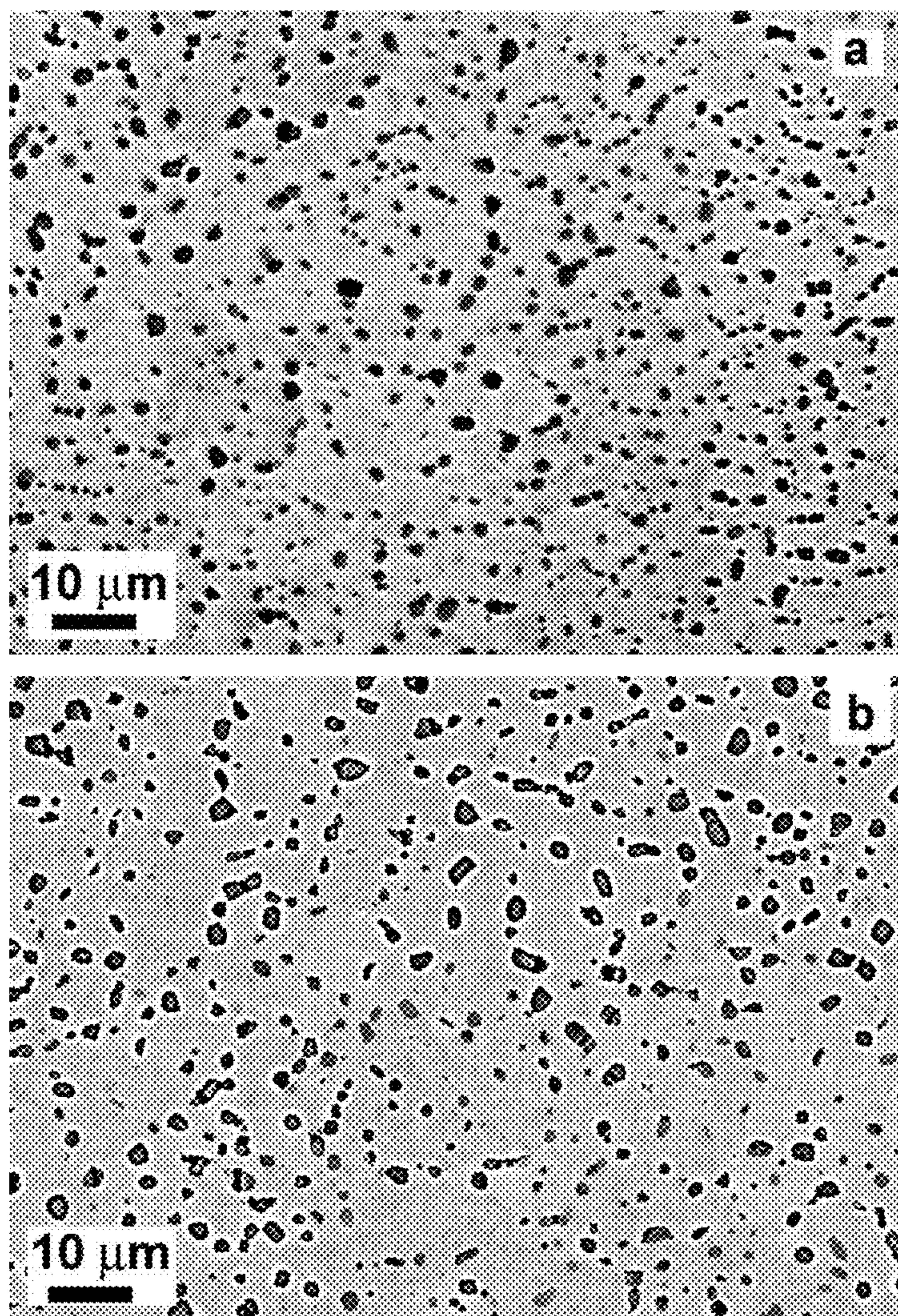
FIG. 51 SEM images of microstructure of the gage section of the tensile specimens from the Alloy 51 before and after pre-straining to 10%.
