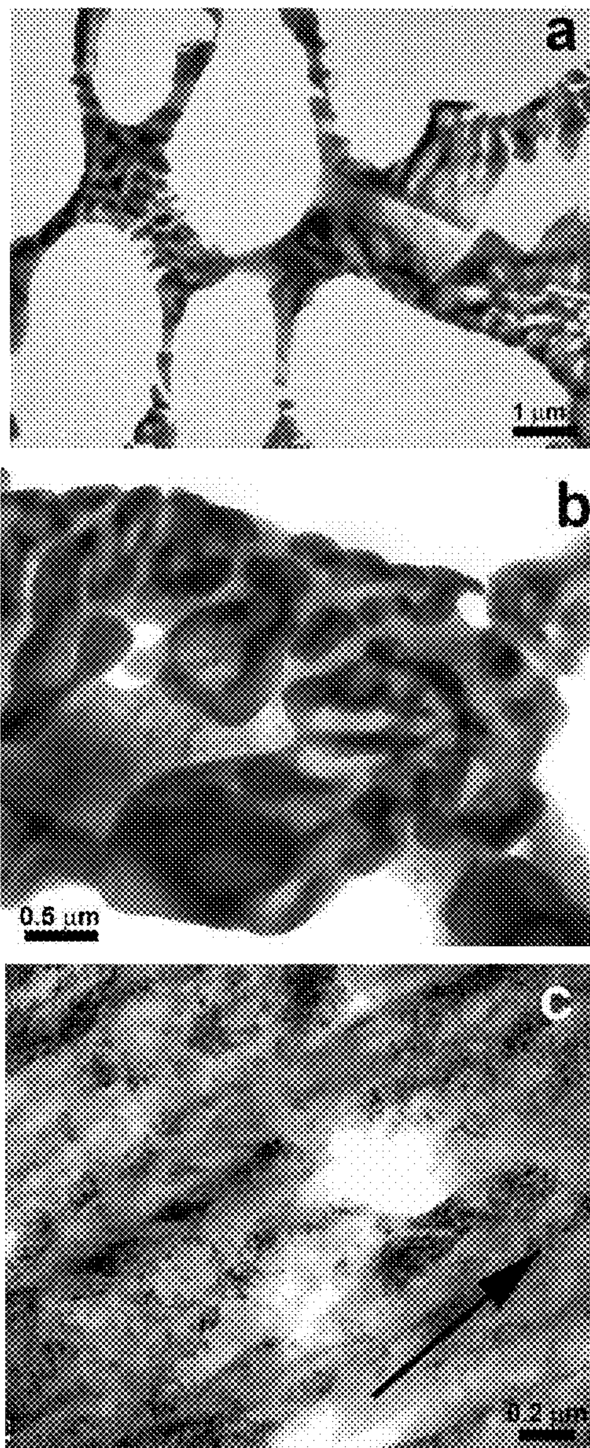
FIG. 25 TEM micrographs of microstructure in the plate sample from the as-cast Alloy 6. (a) The microstructure at the intergranular region in the as-cast sample (corresponding to the region B in FIG. 18); (b) Magnified image at the intergranular region showing the detailed structure of precipitates; (c) The microstructure of matrix grains, which are aligned in one direction indicated by the arrow.
