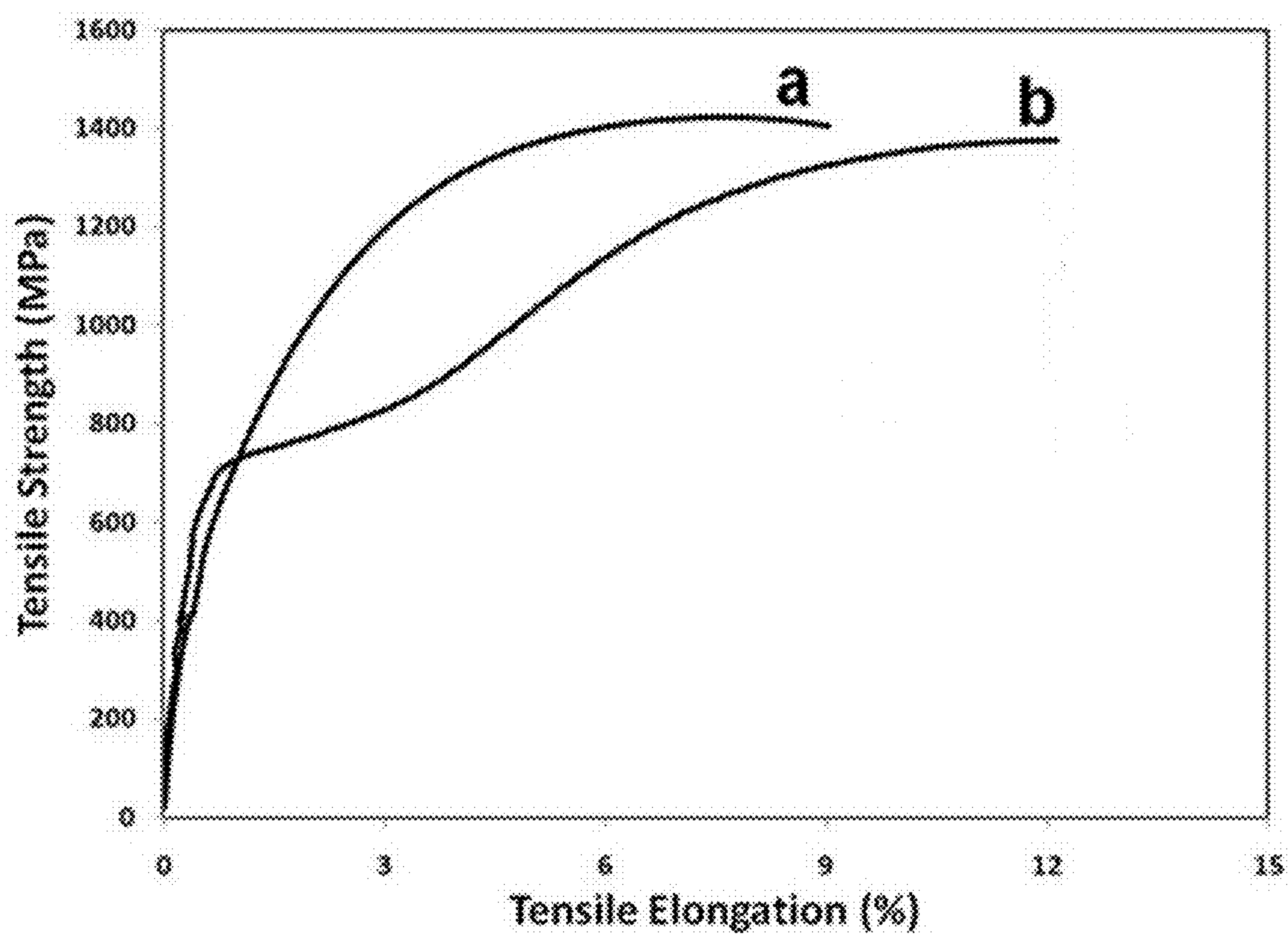
FIG. 44 Stress-strain curves recorded at tensile testing of specimens from the Alloy 5 plate after HIP cycle and heat treatment at 700 °C for 1 with cooling (a) in air and (b) with furnace.
