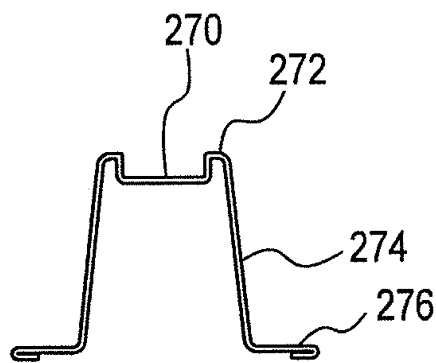
SECTION B-B
