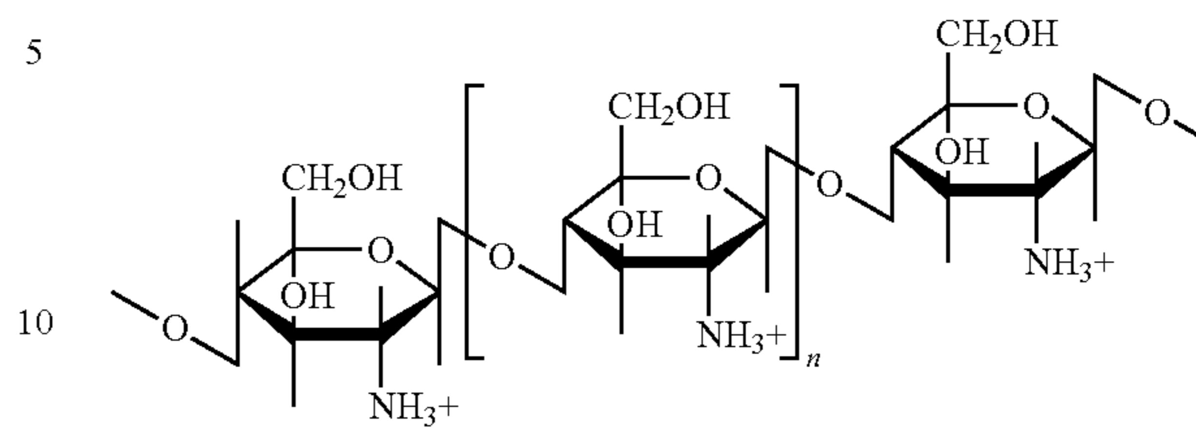
Scheme 2. Structure of fully deacetylated chitosan (poly D-glucosamine, protonated form at low pH).
