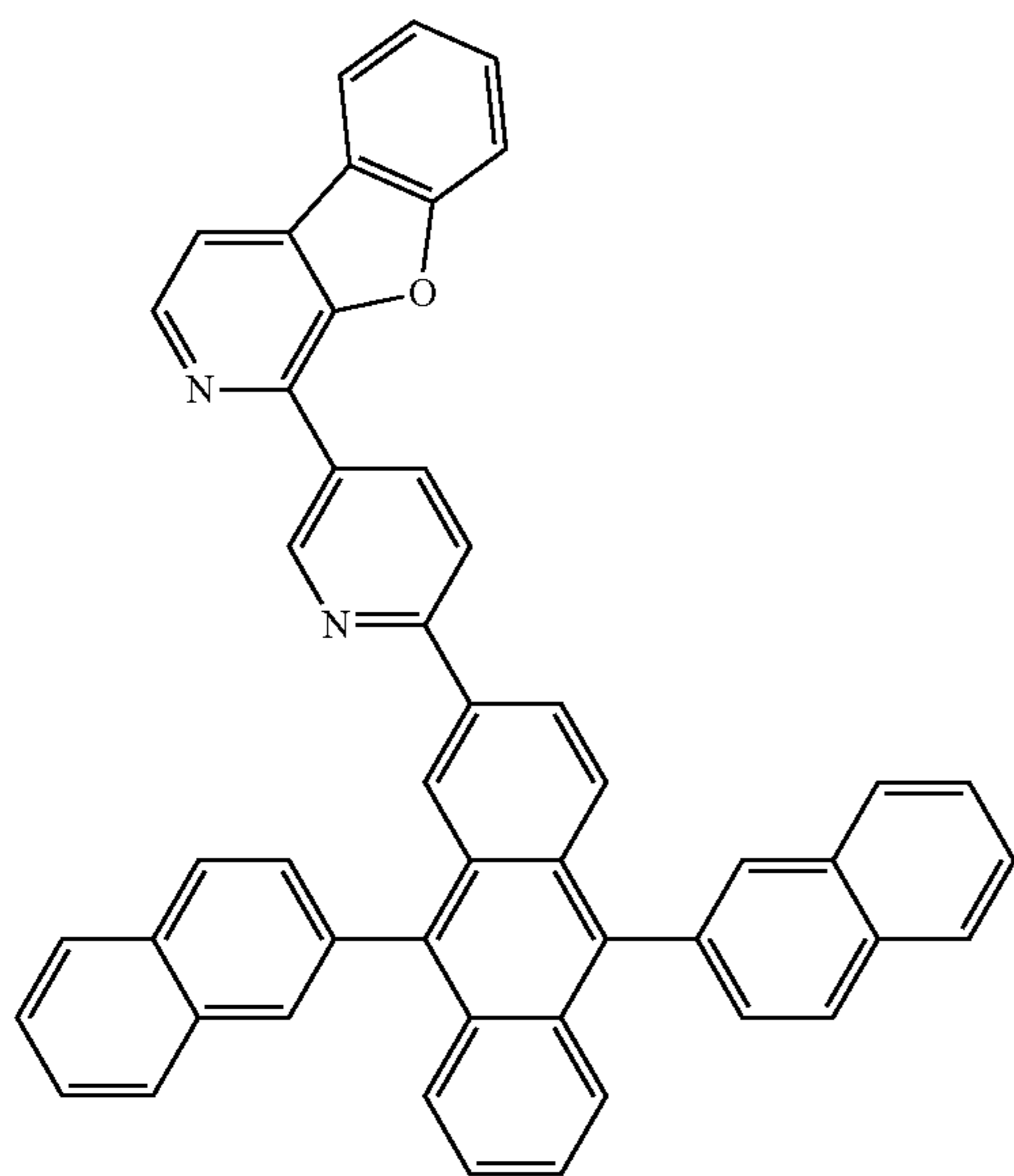
Compound 21
