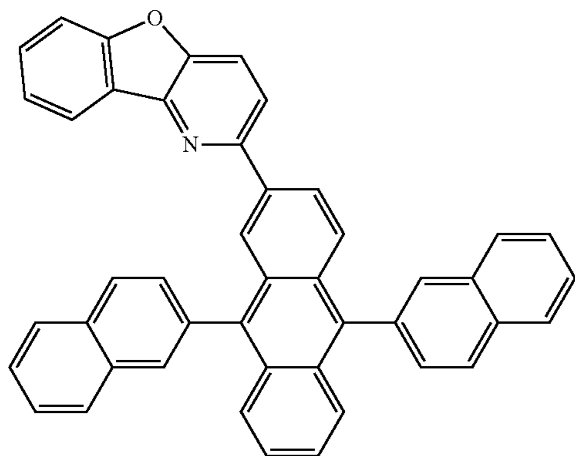
Compound 34
