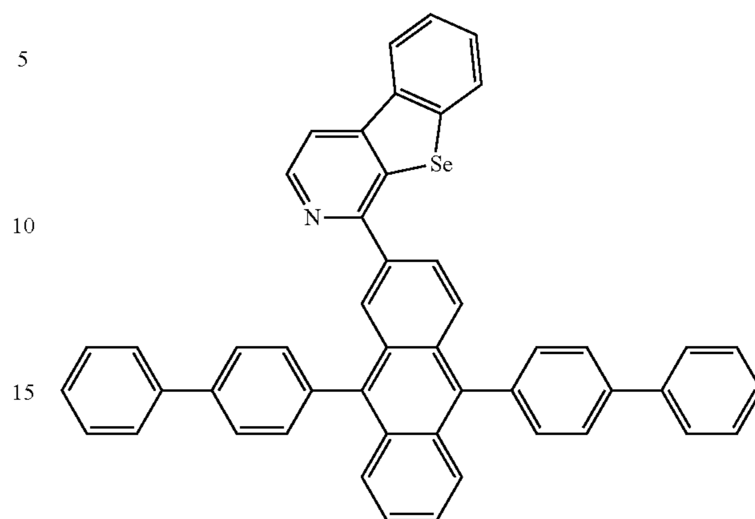
Compound 43
