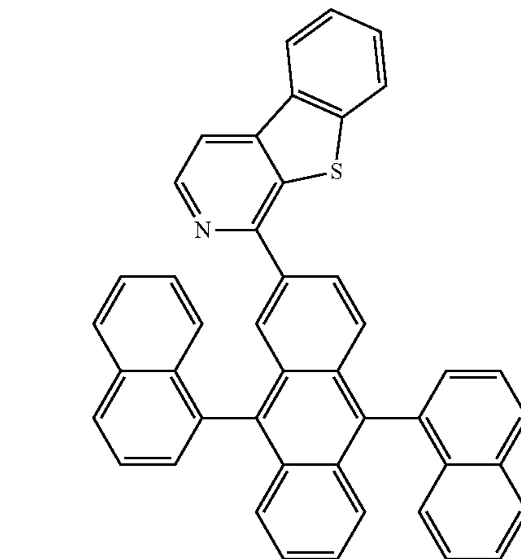
Compound 5
