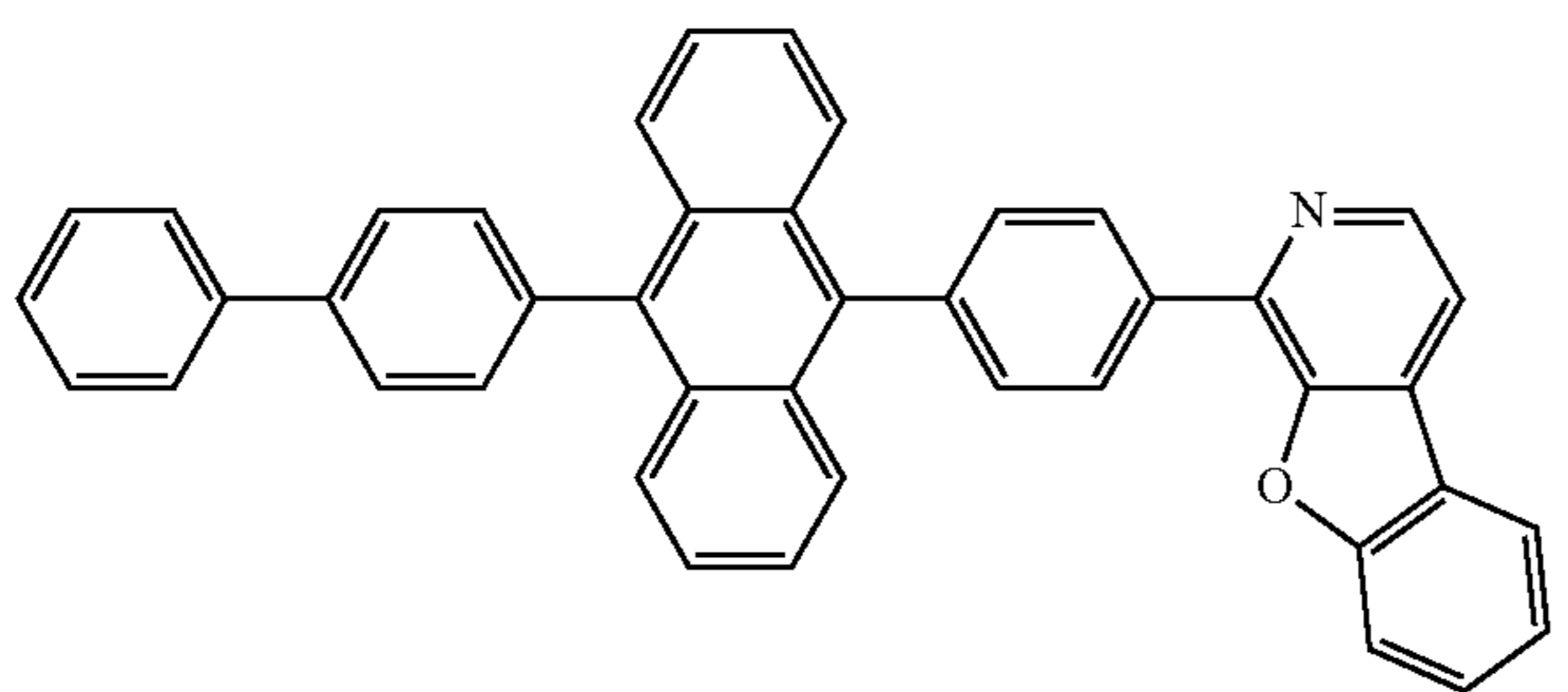
Compound 30
