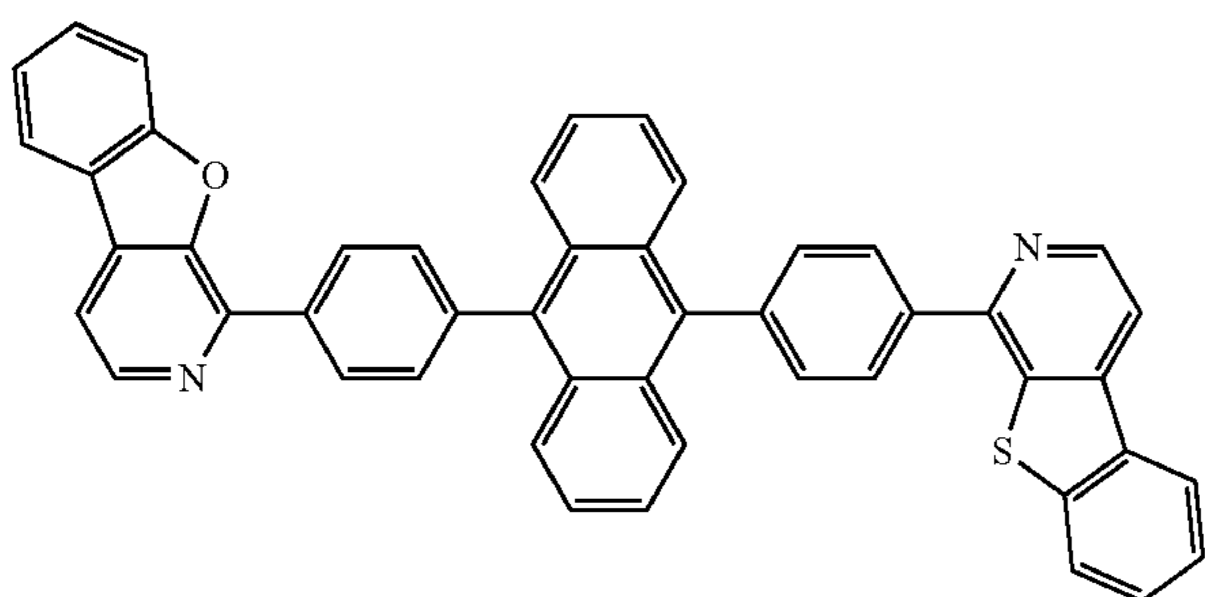
Compound 57
