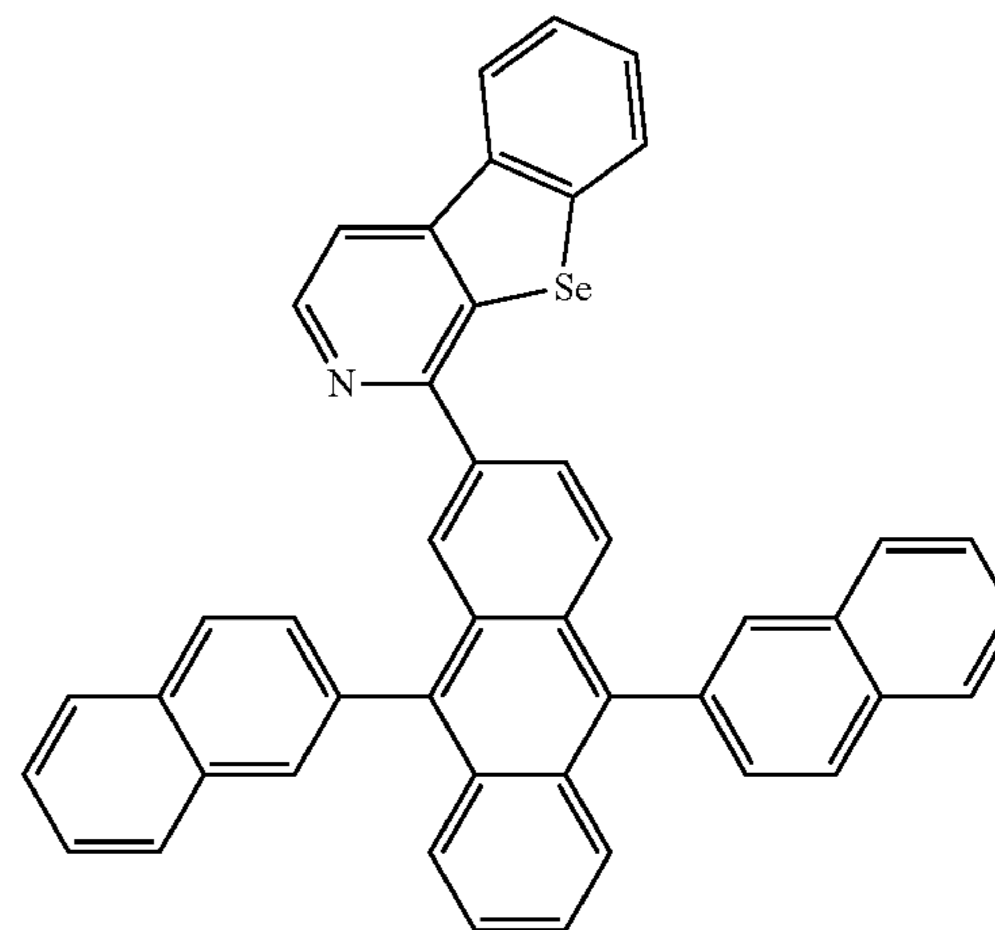
Compound 38
