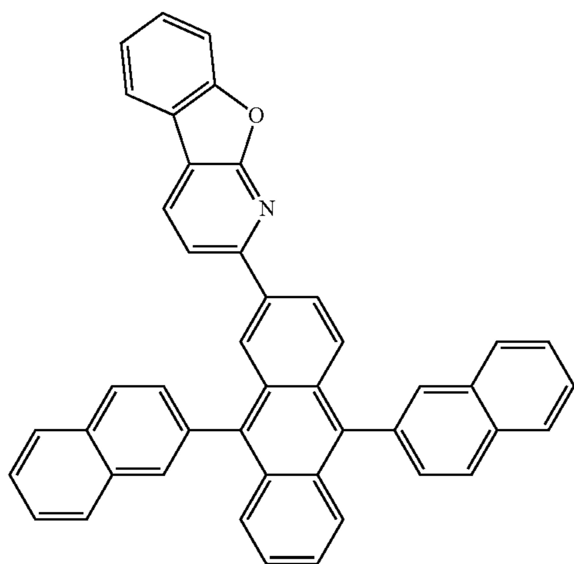
Compound 35
