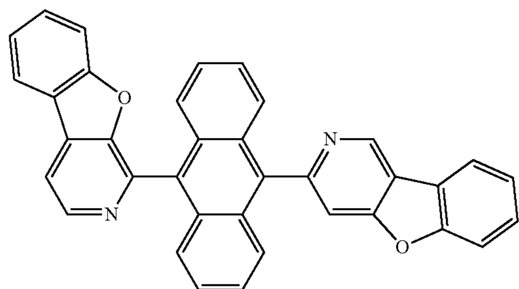
Compound 58
