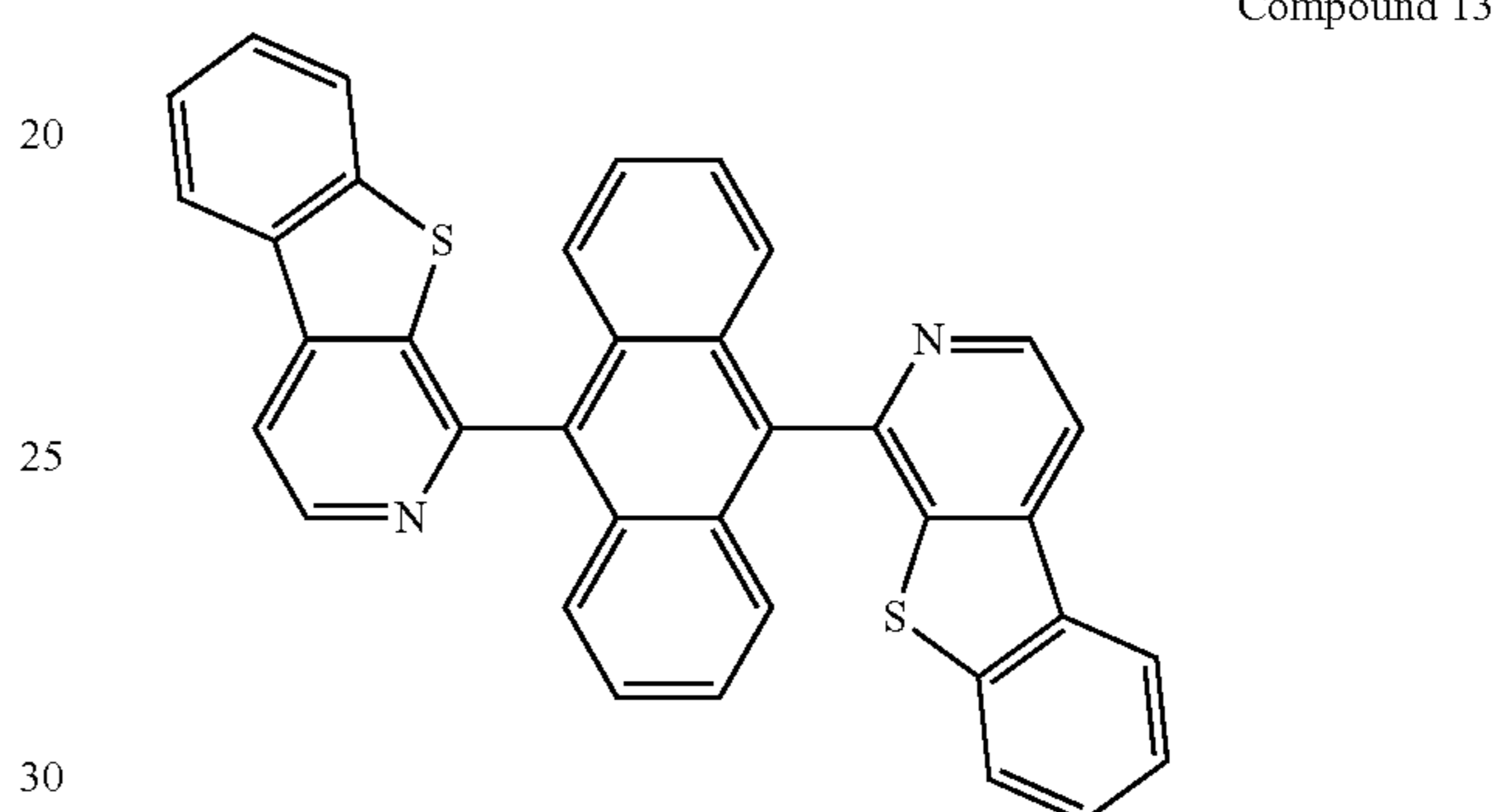
Compound 9
