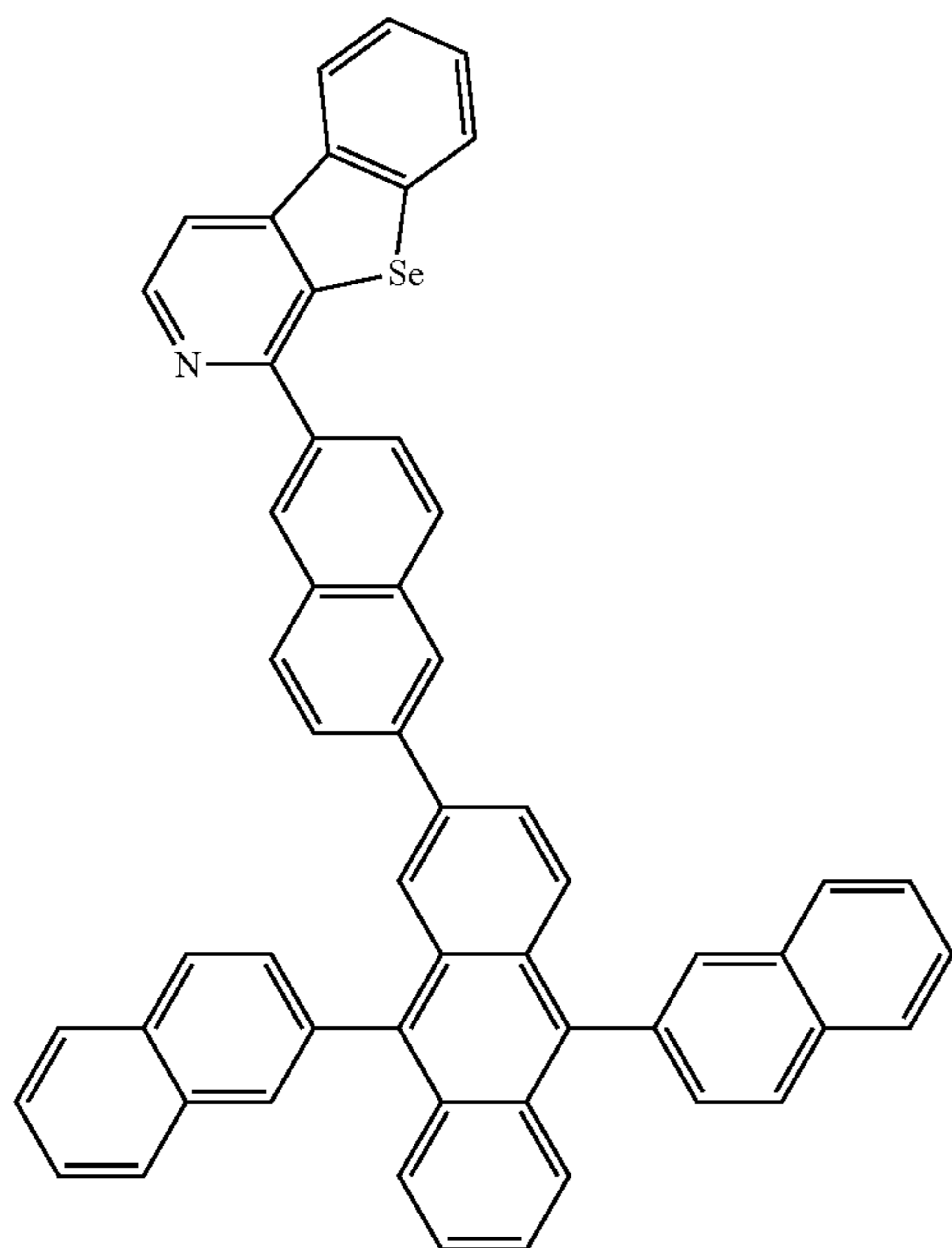
Compound 42
