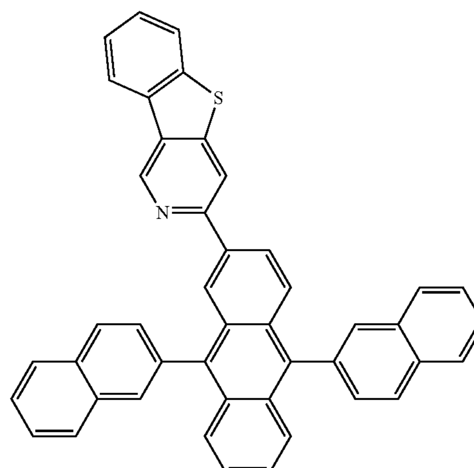
Compound 18
