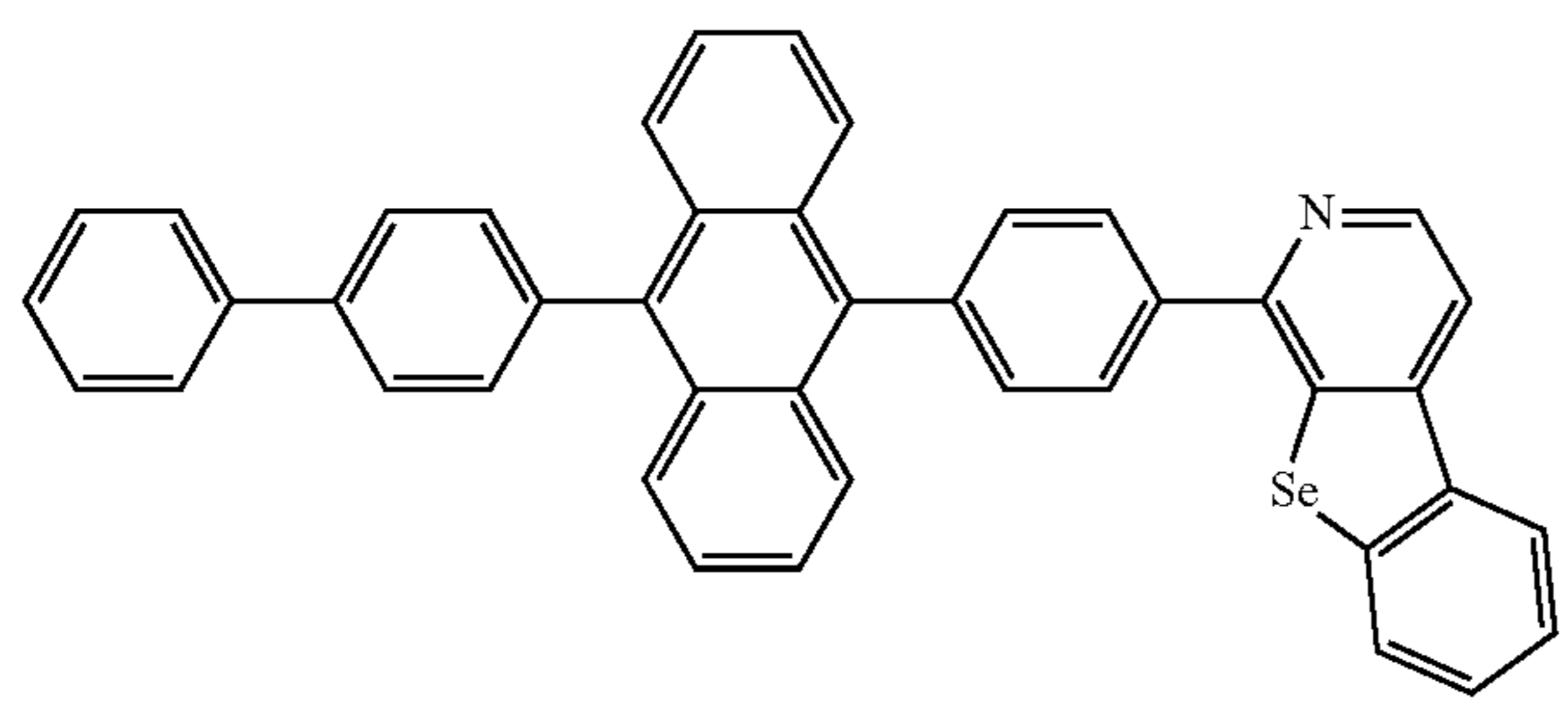
Compound 49
