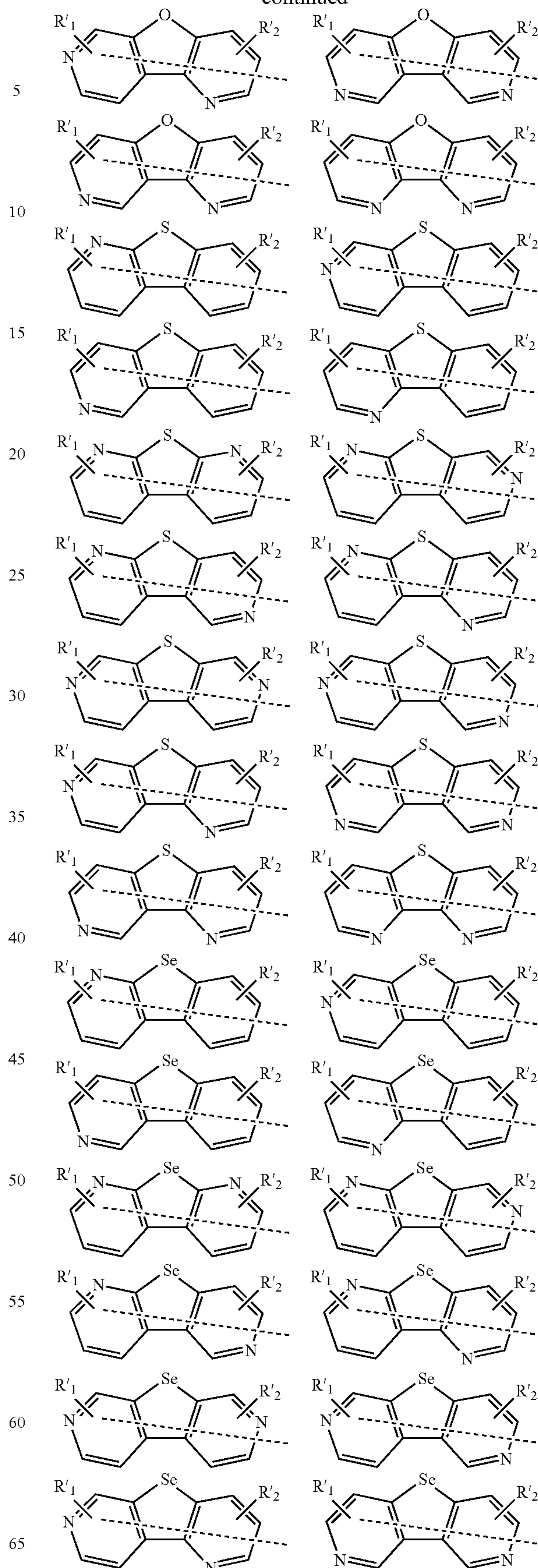
Formula II
