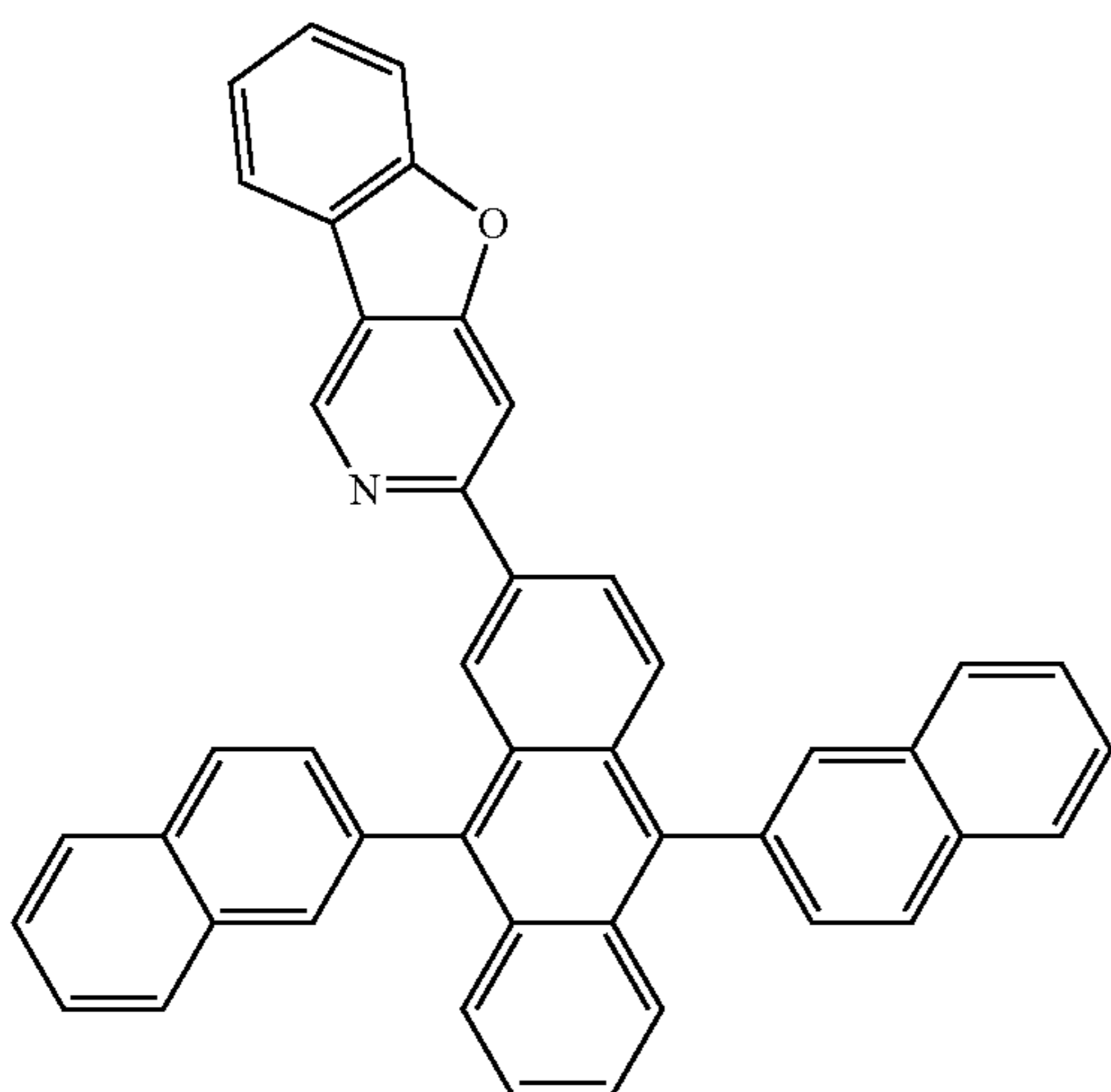
Compound 36
