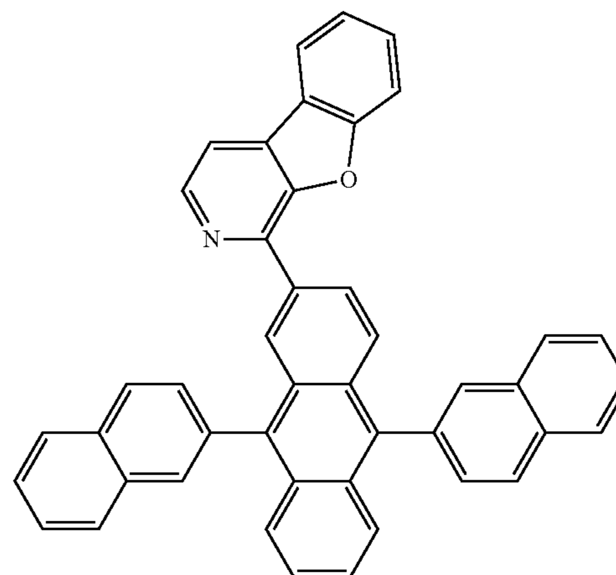
Compound 20
