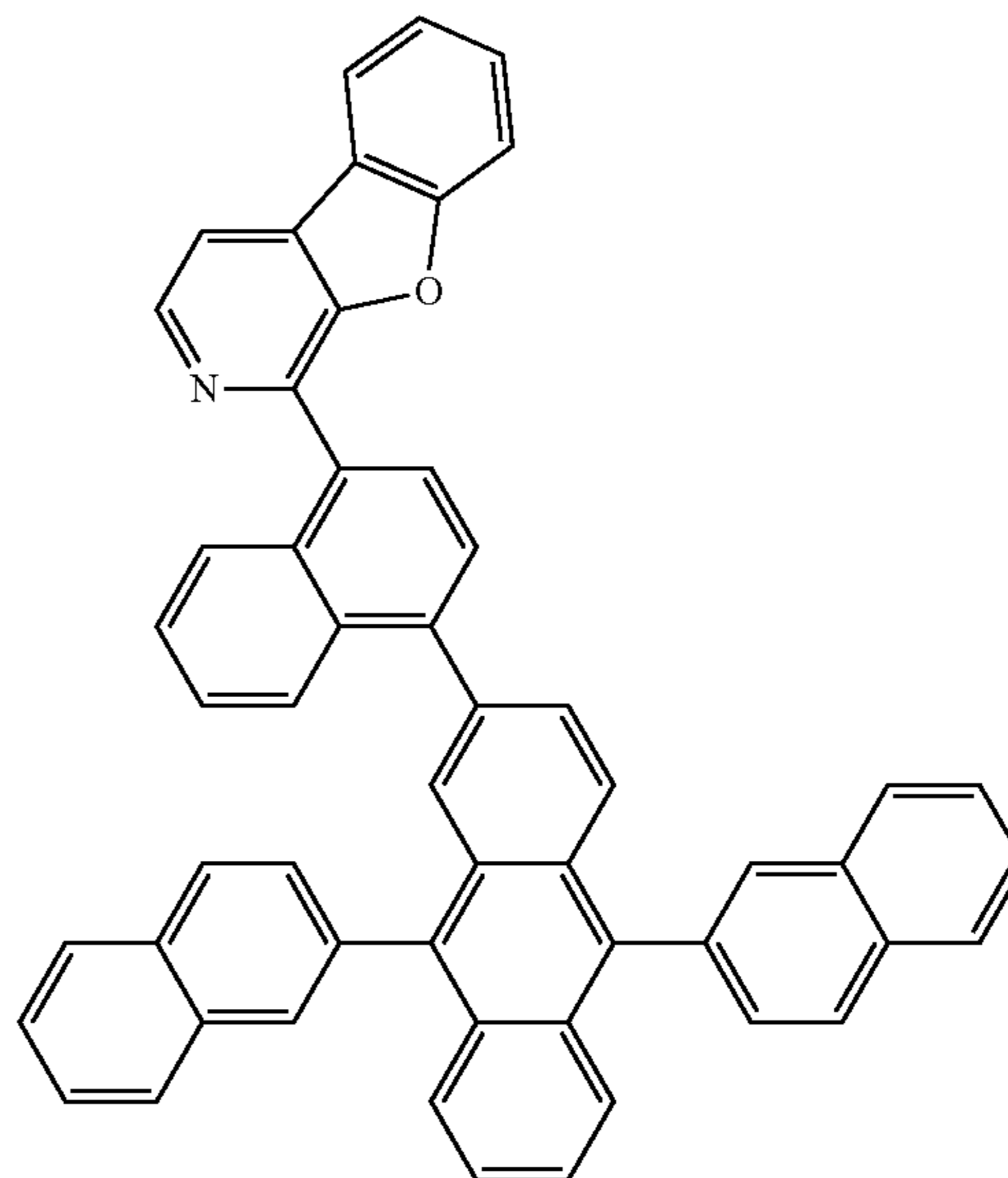
Compound 23
