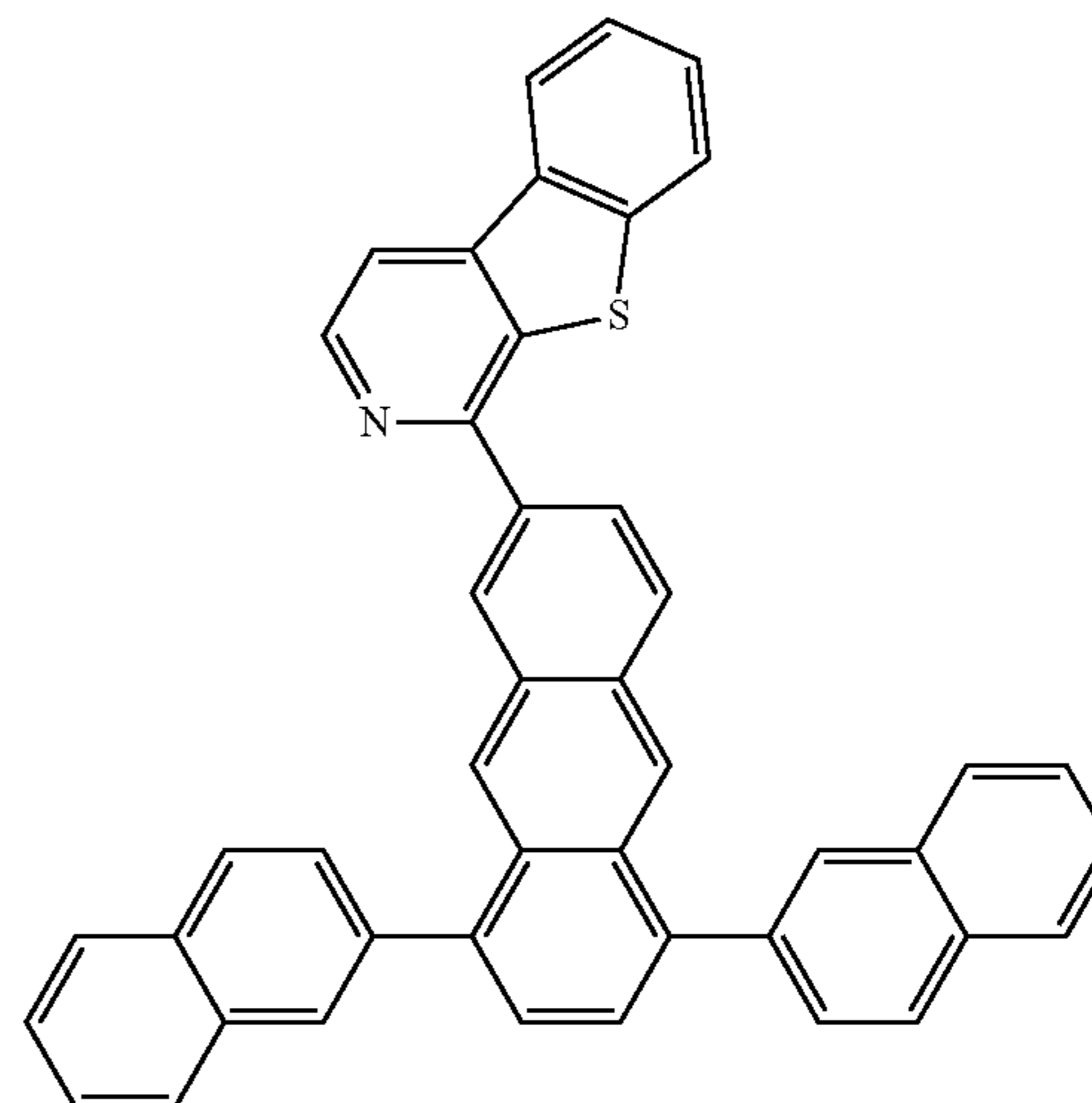
Compound 1
