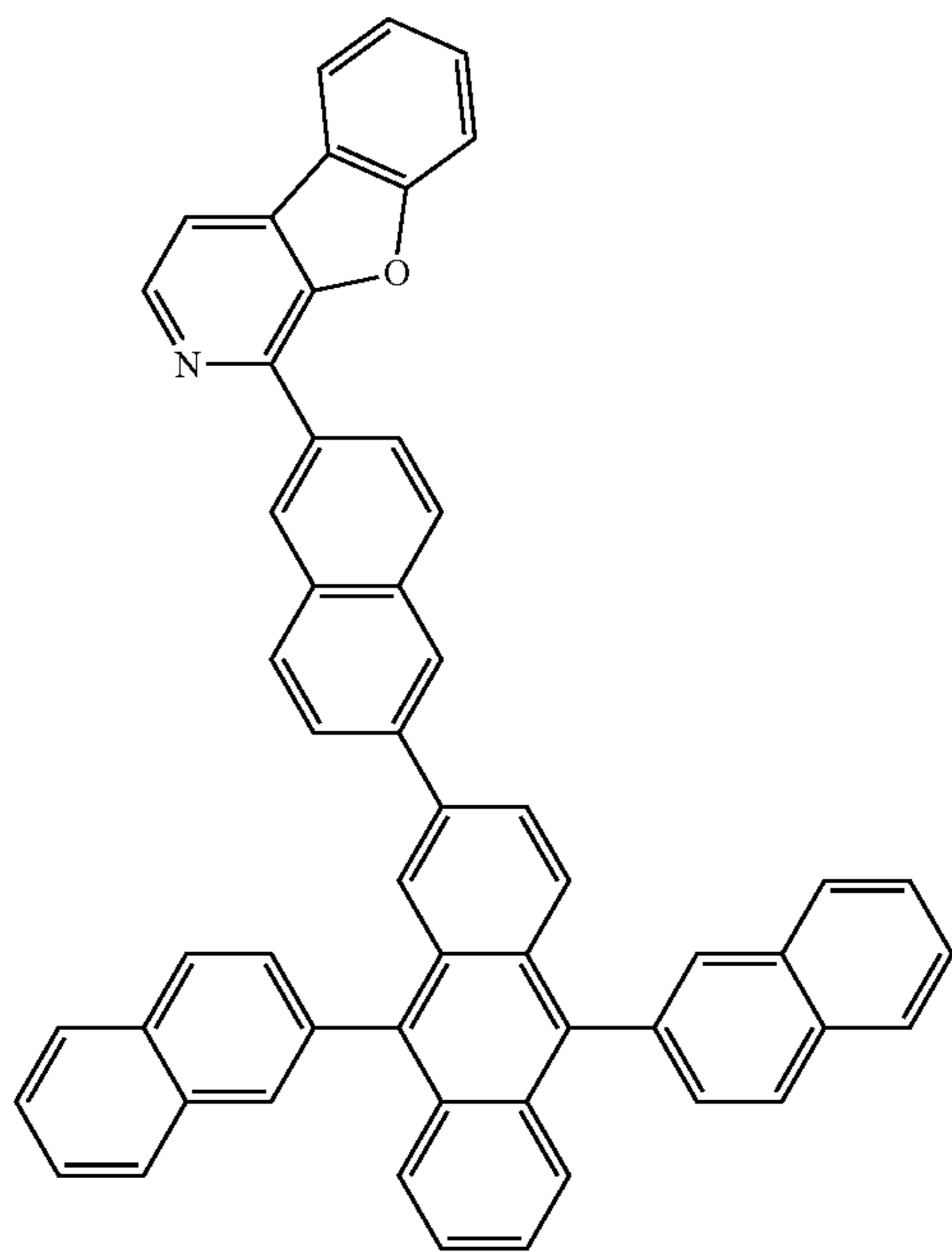
Compound 24
