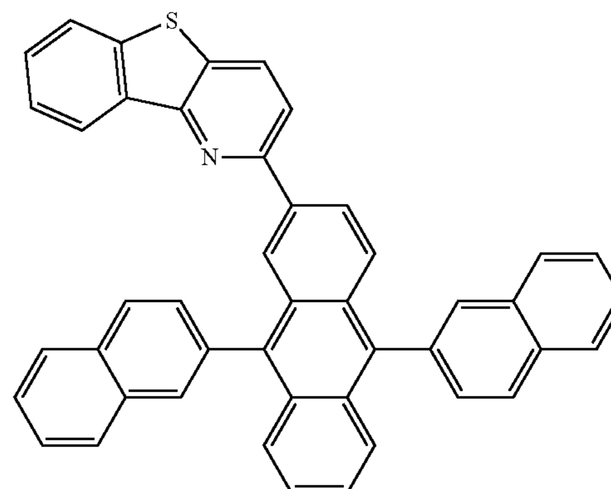
Compound 16
