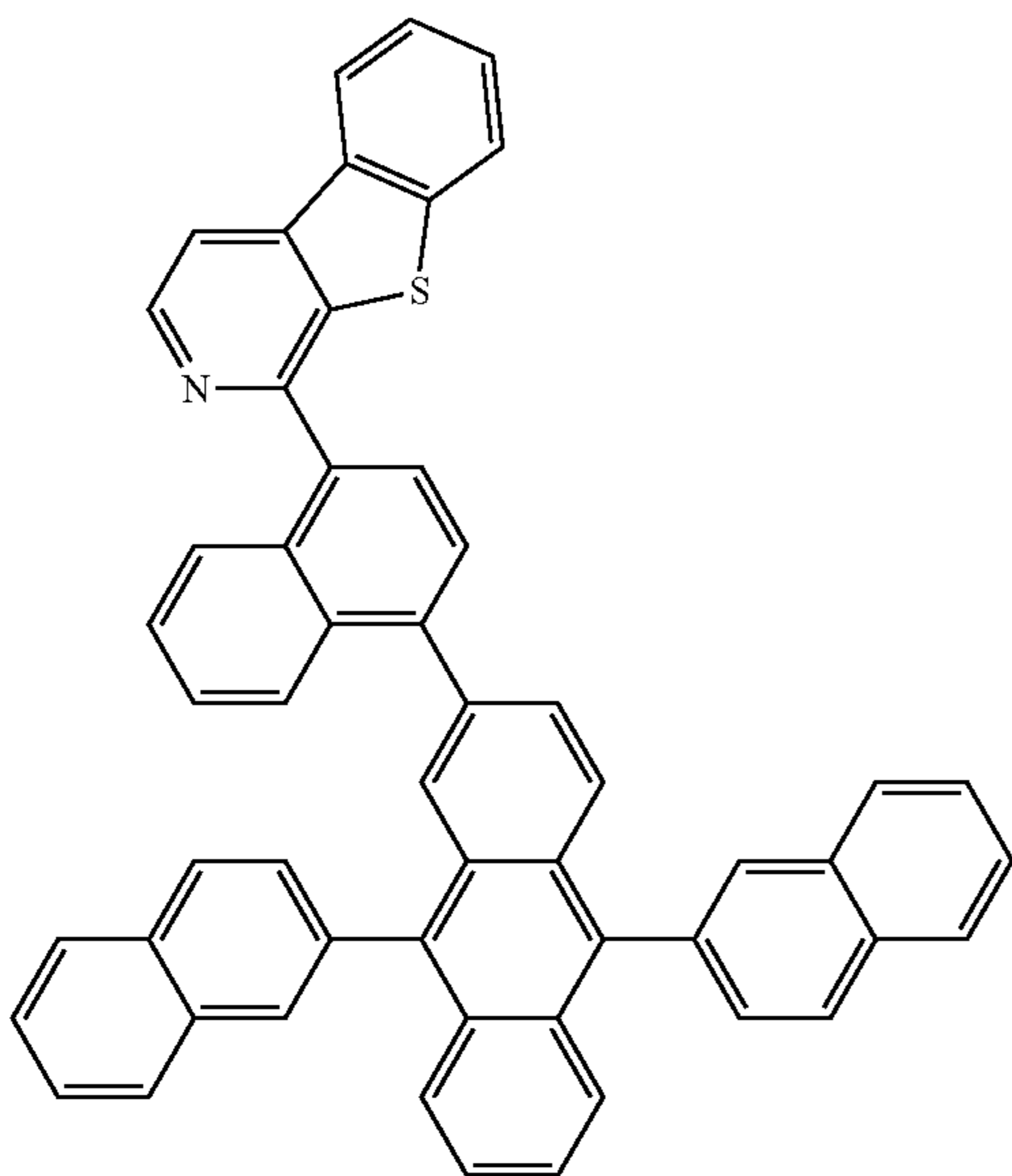
Compound 5
