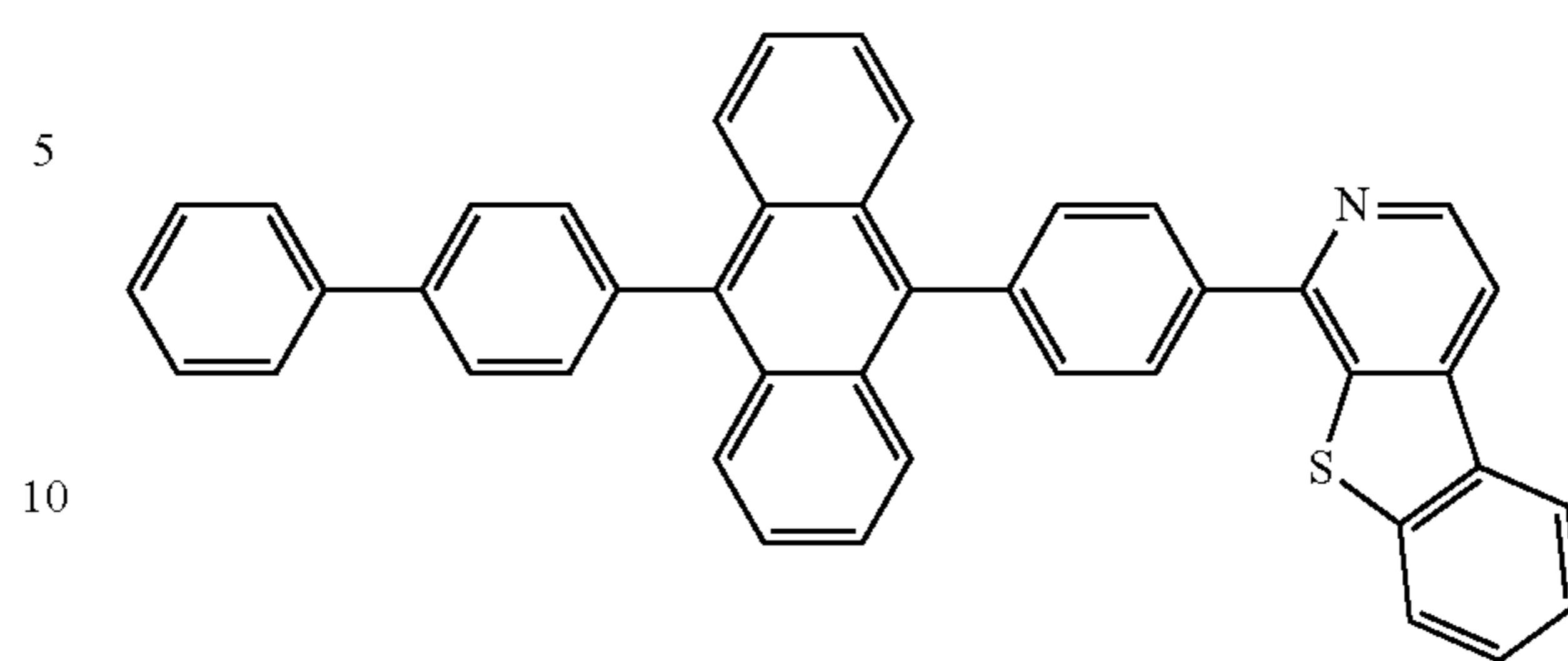
Compound 12
