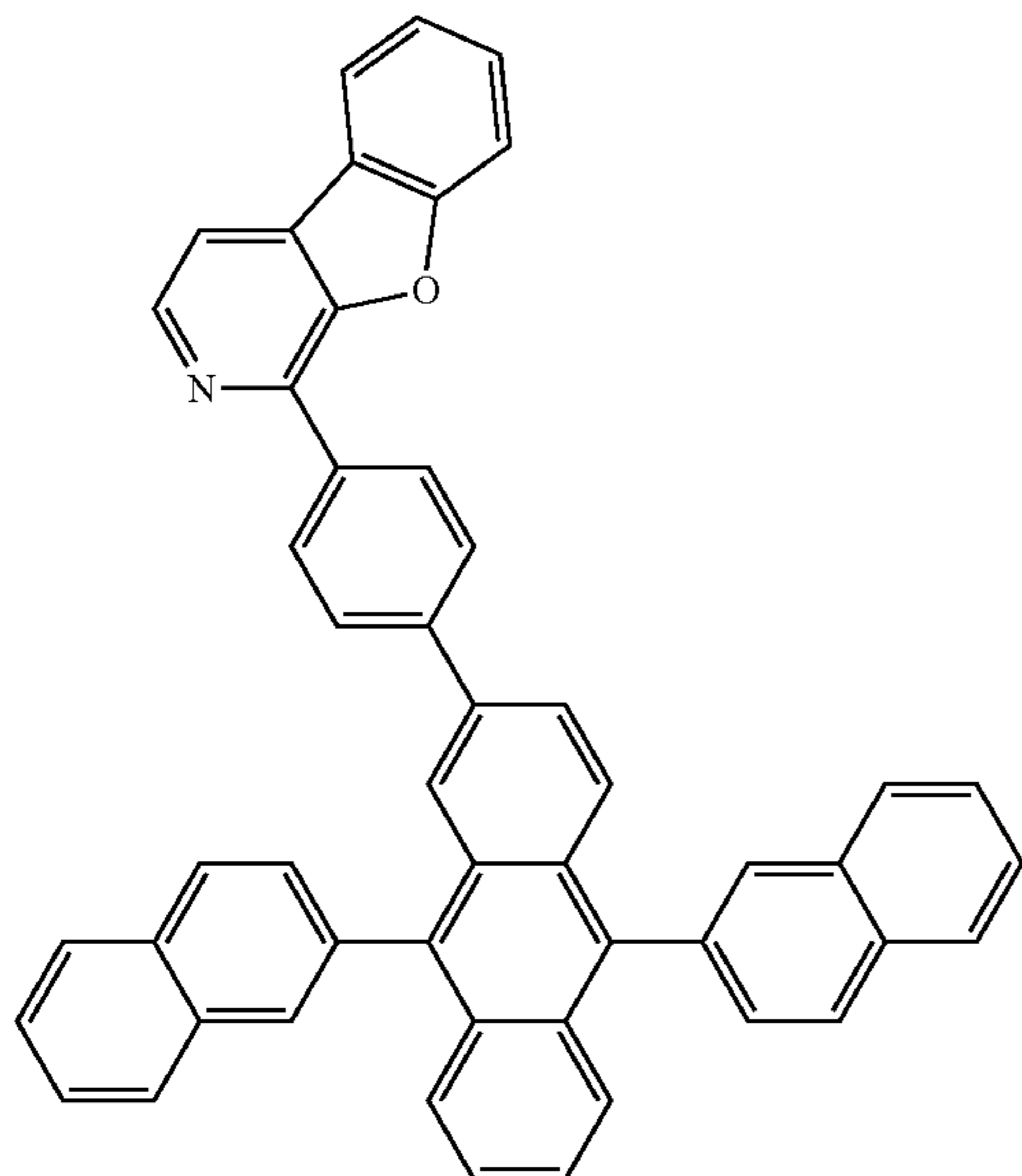
Compound 21
