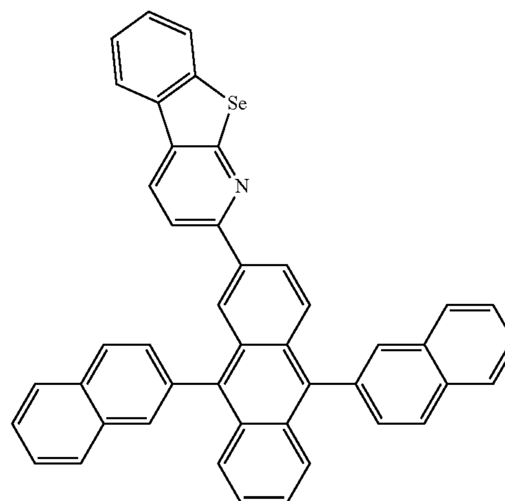
Compound 53
