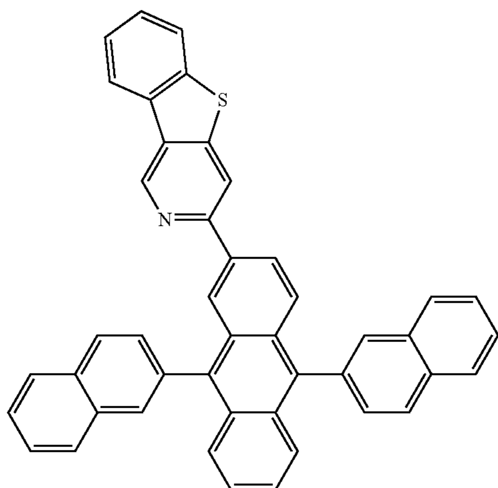
Compound 18
