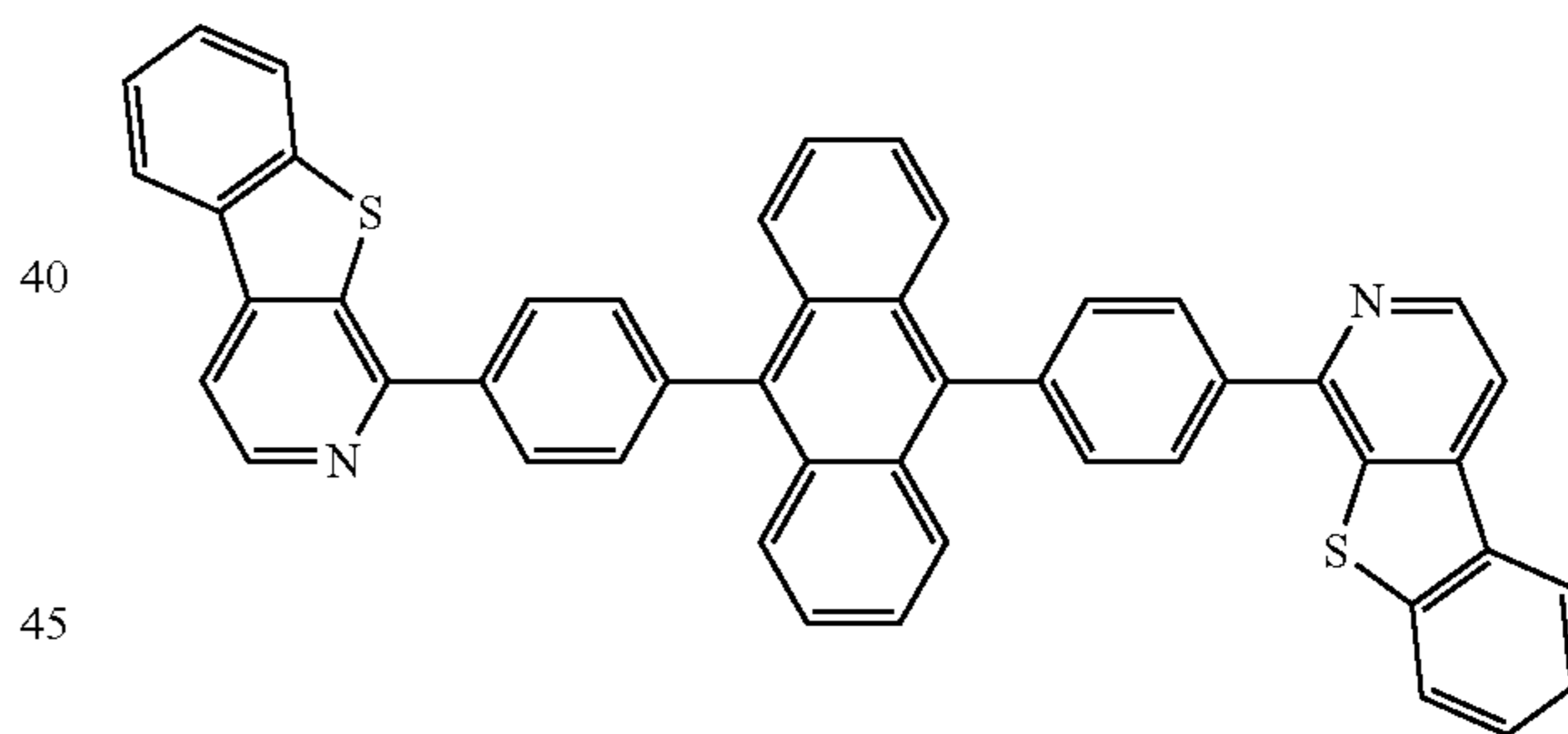
Compound 14
