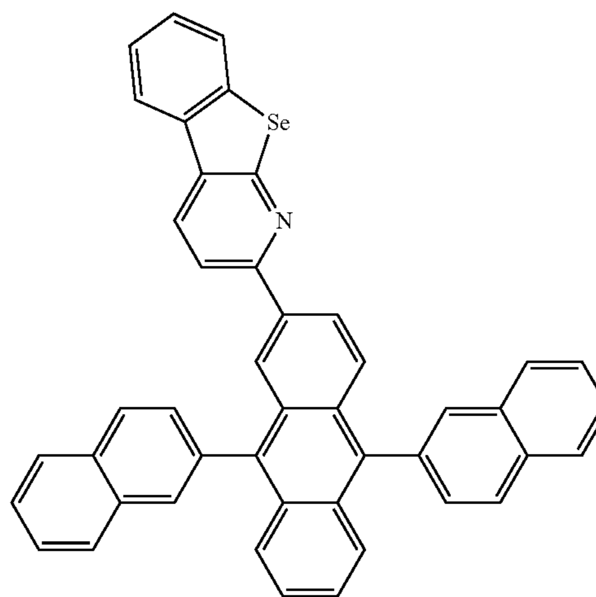
Compound 53
