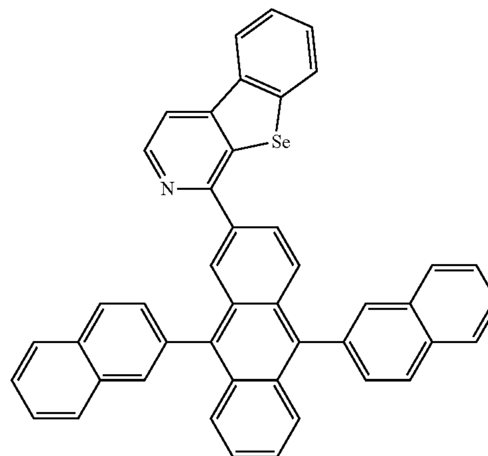
Compound 37
