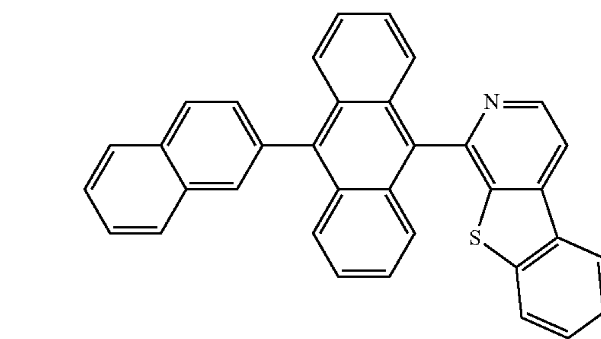
Compound 10
