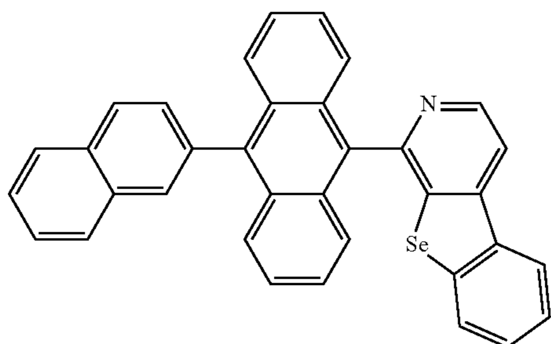
Compound 46
