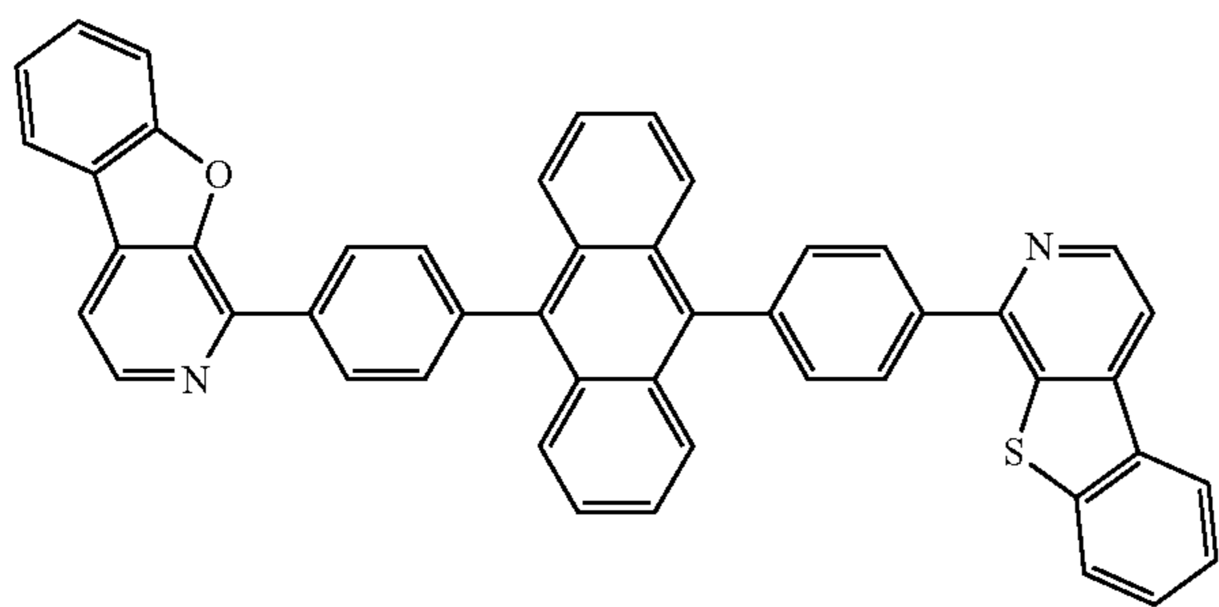
Compound 56
