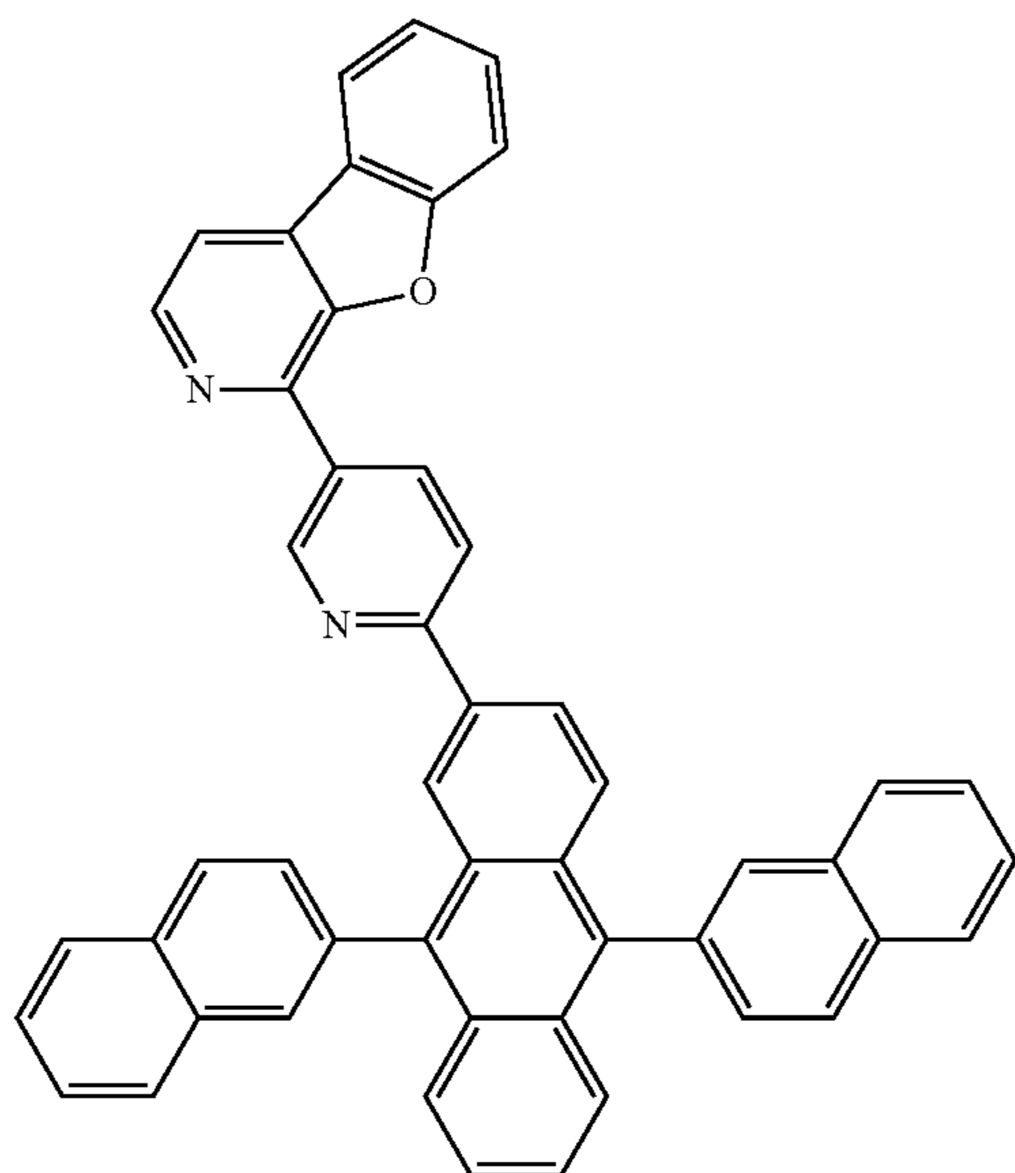
Compound 21
