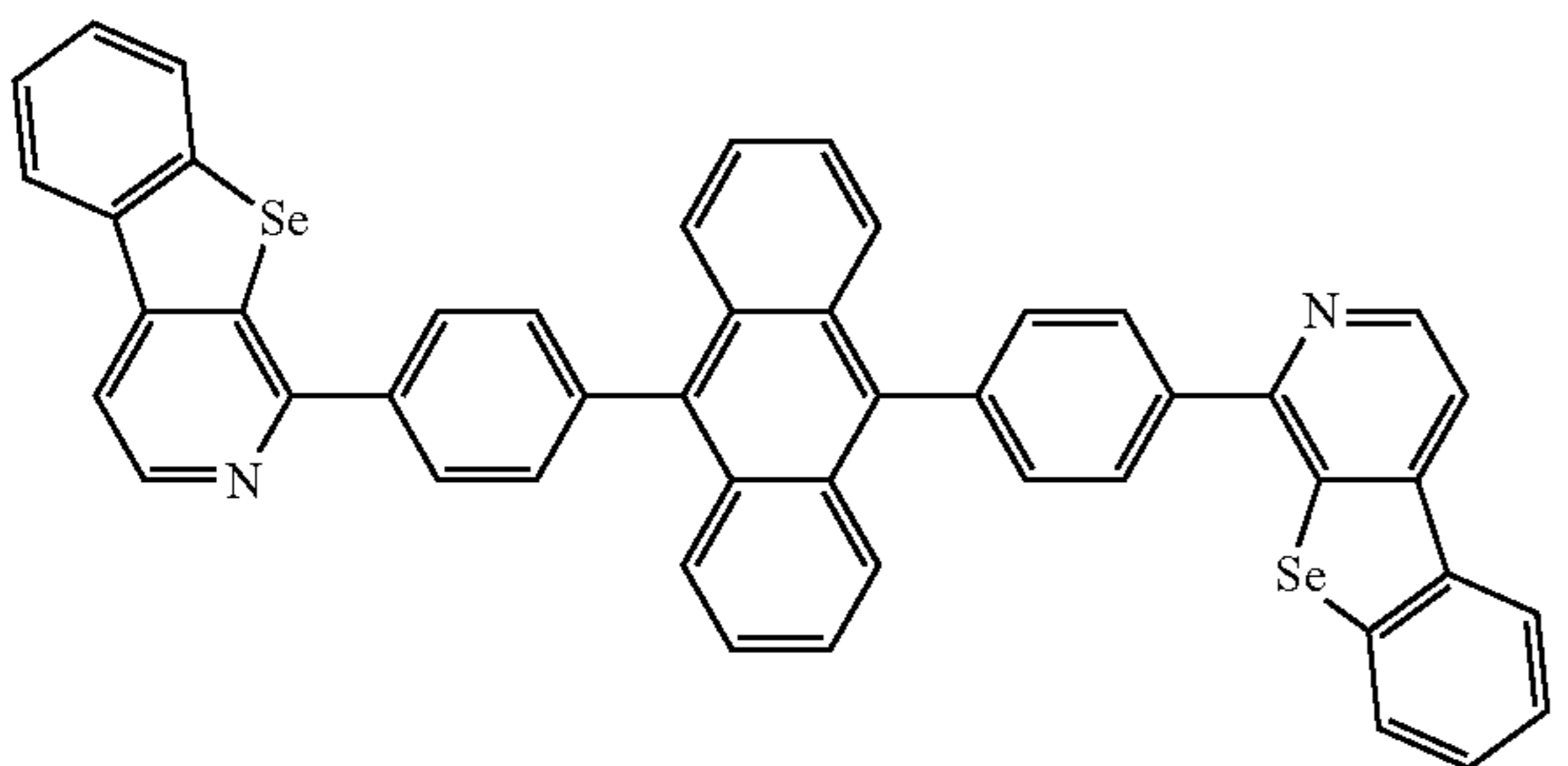
Compound 51
