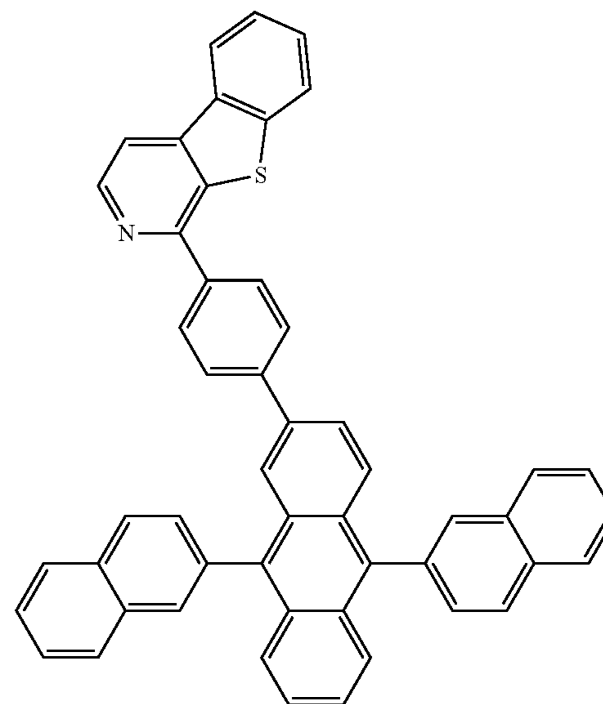
Compound 2
