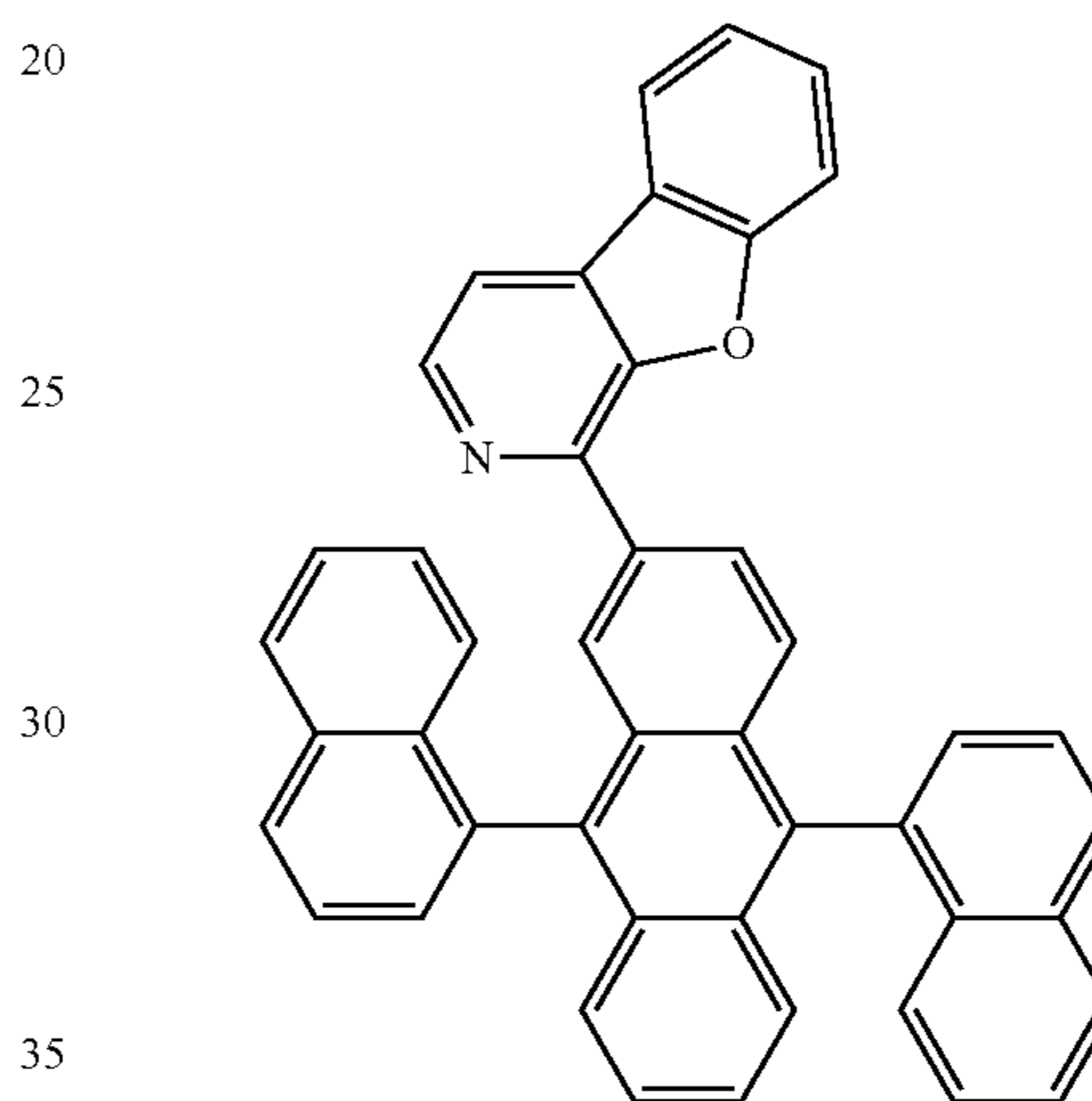
Compound 23
