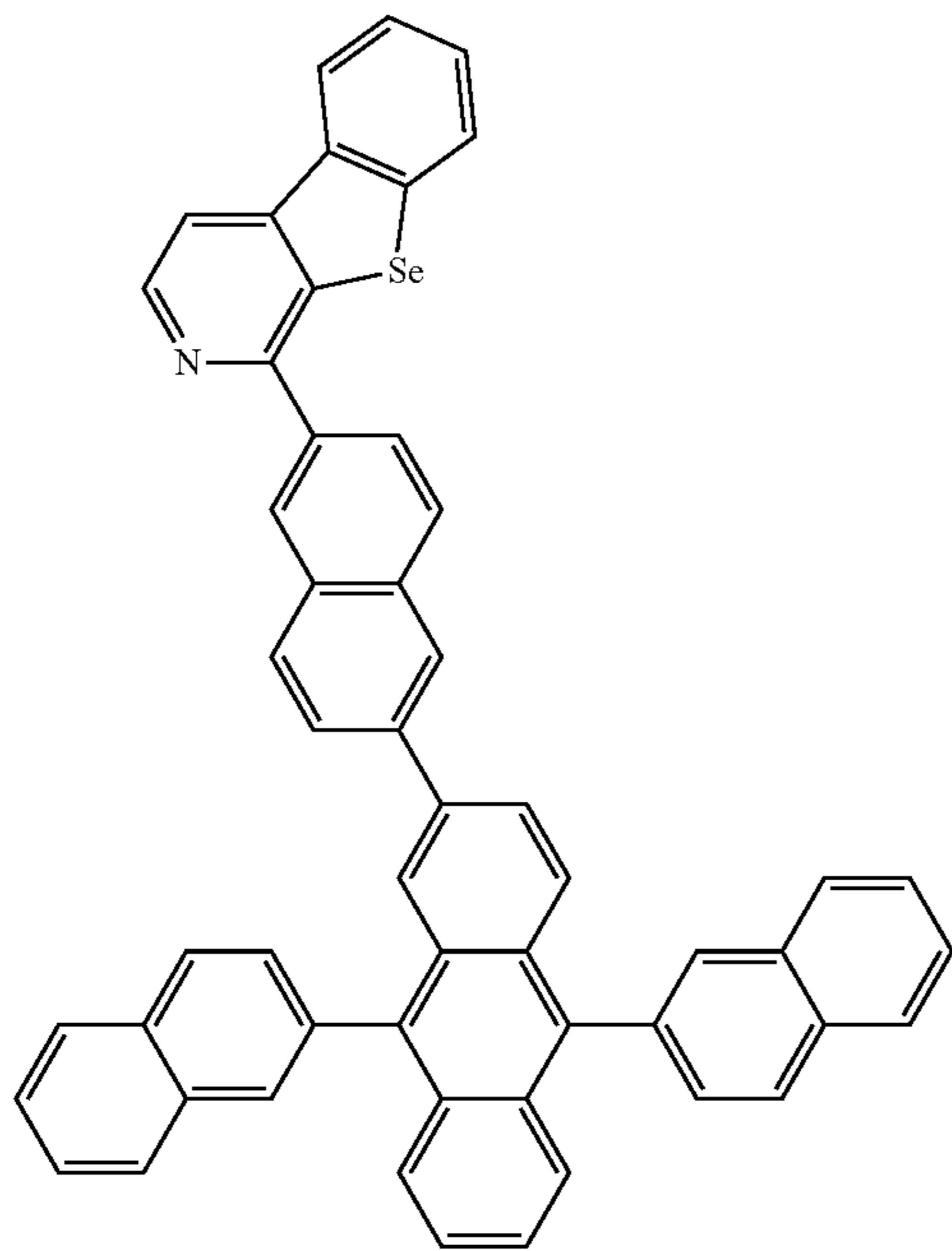
Compound 41
