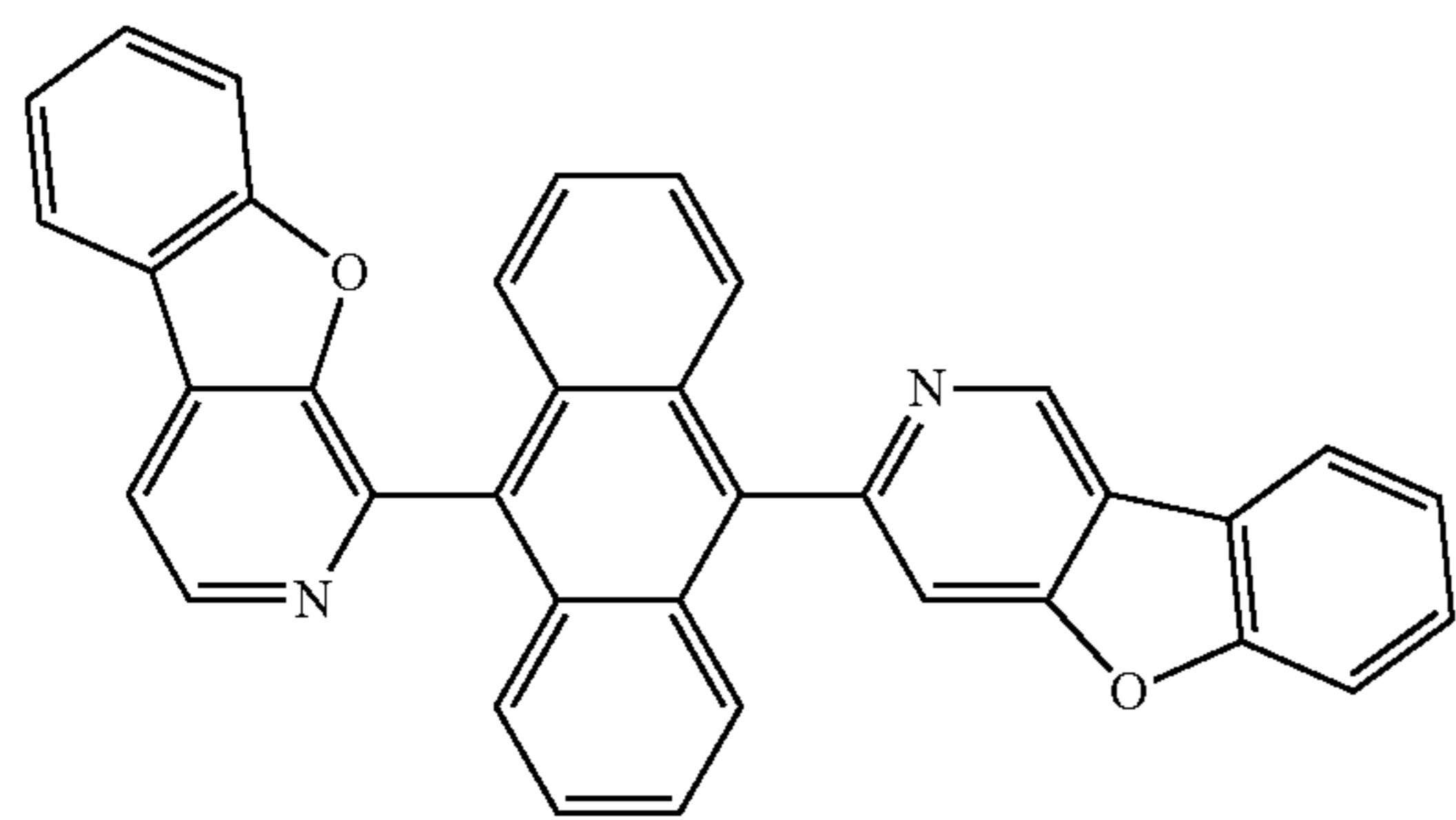
Compound 58
