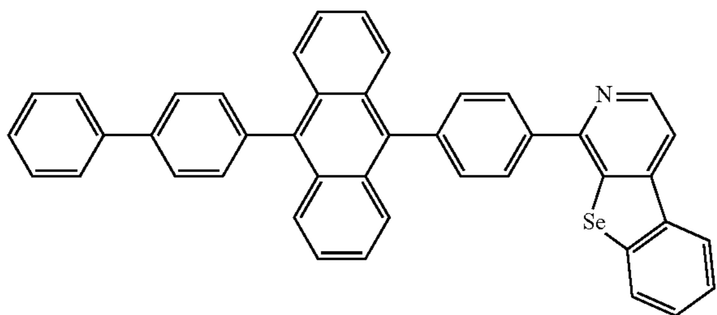
Compound 48
