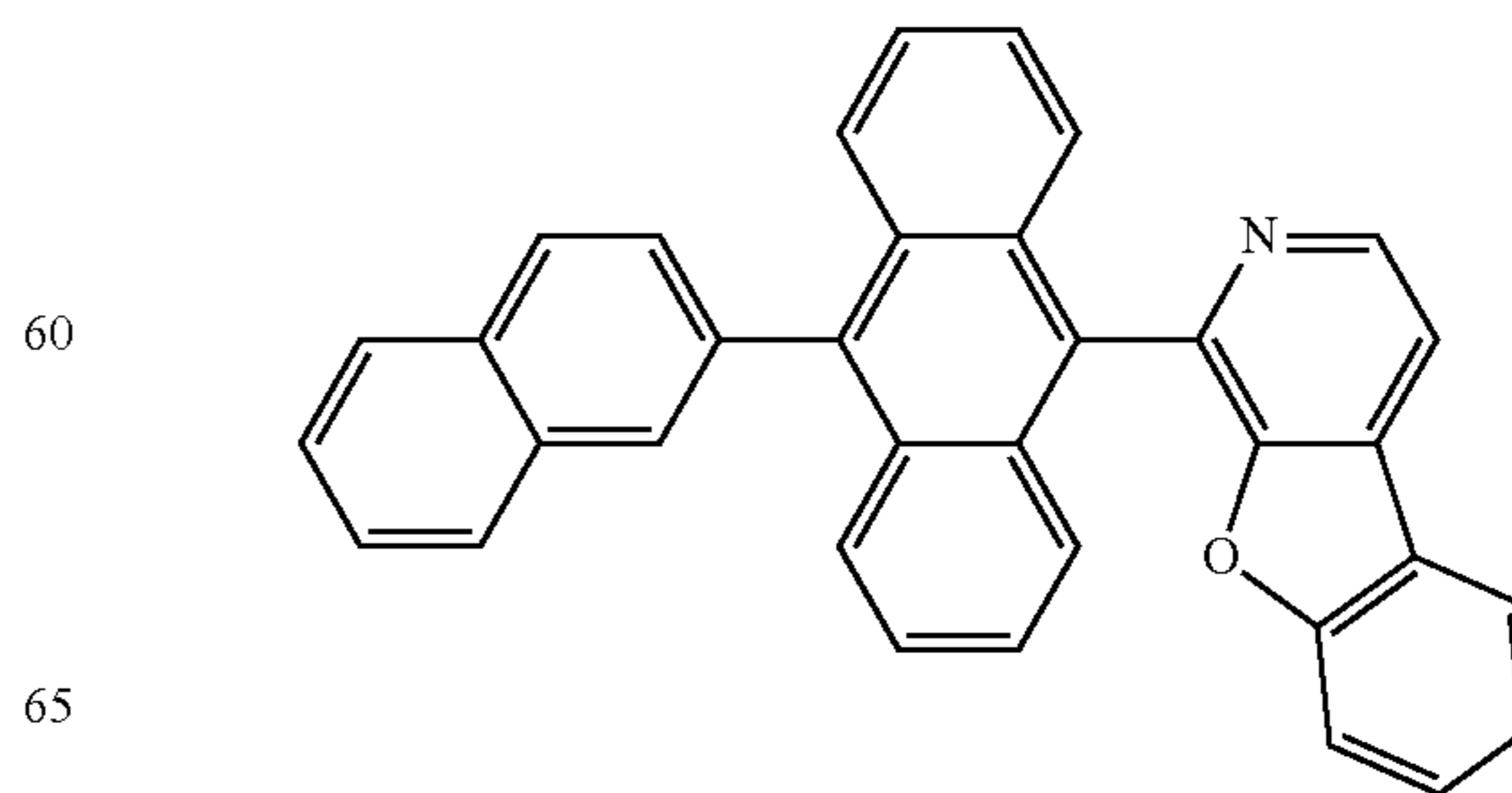
Compound 28
