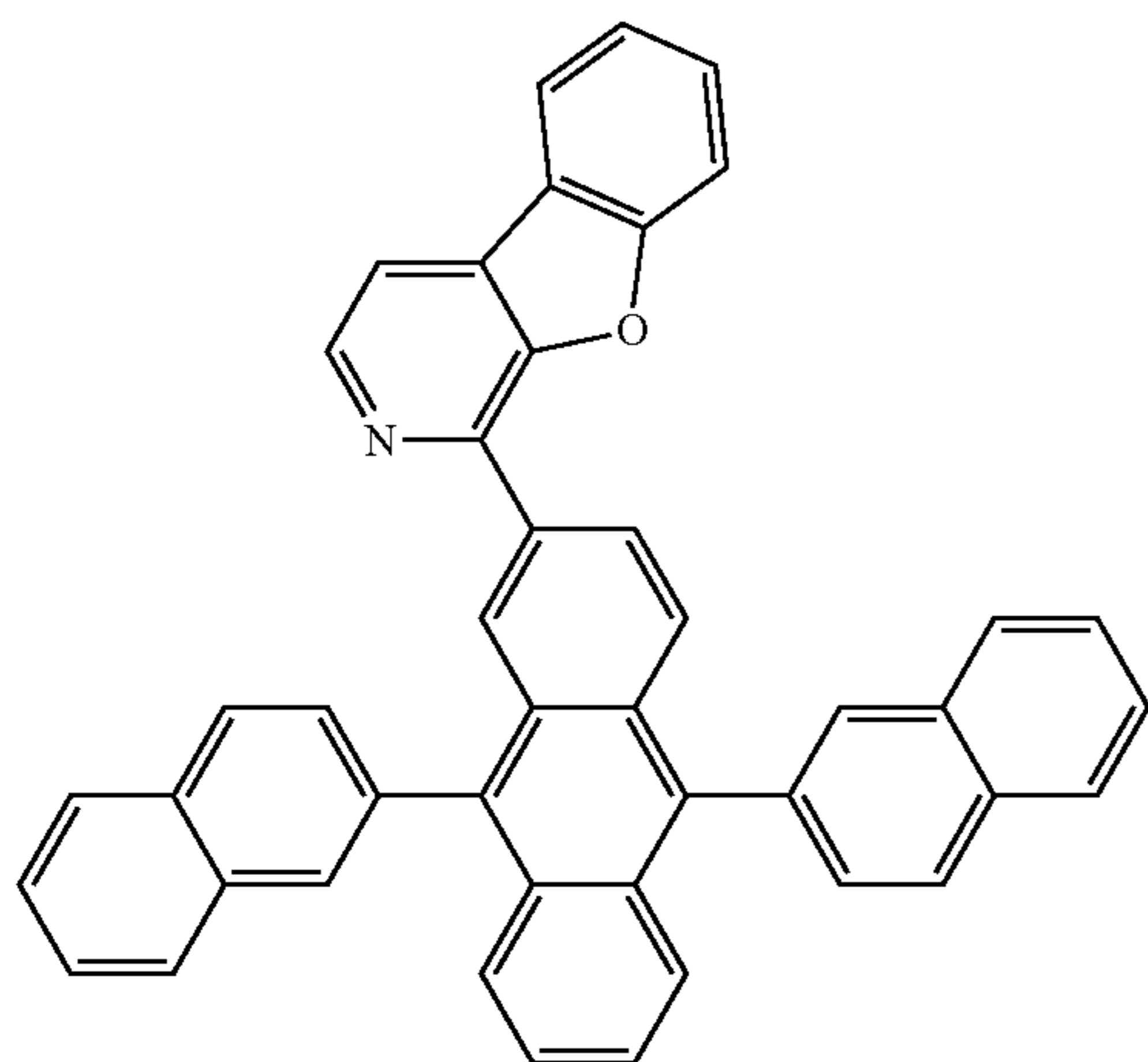
Compound 20
