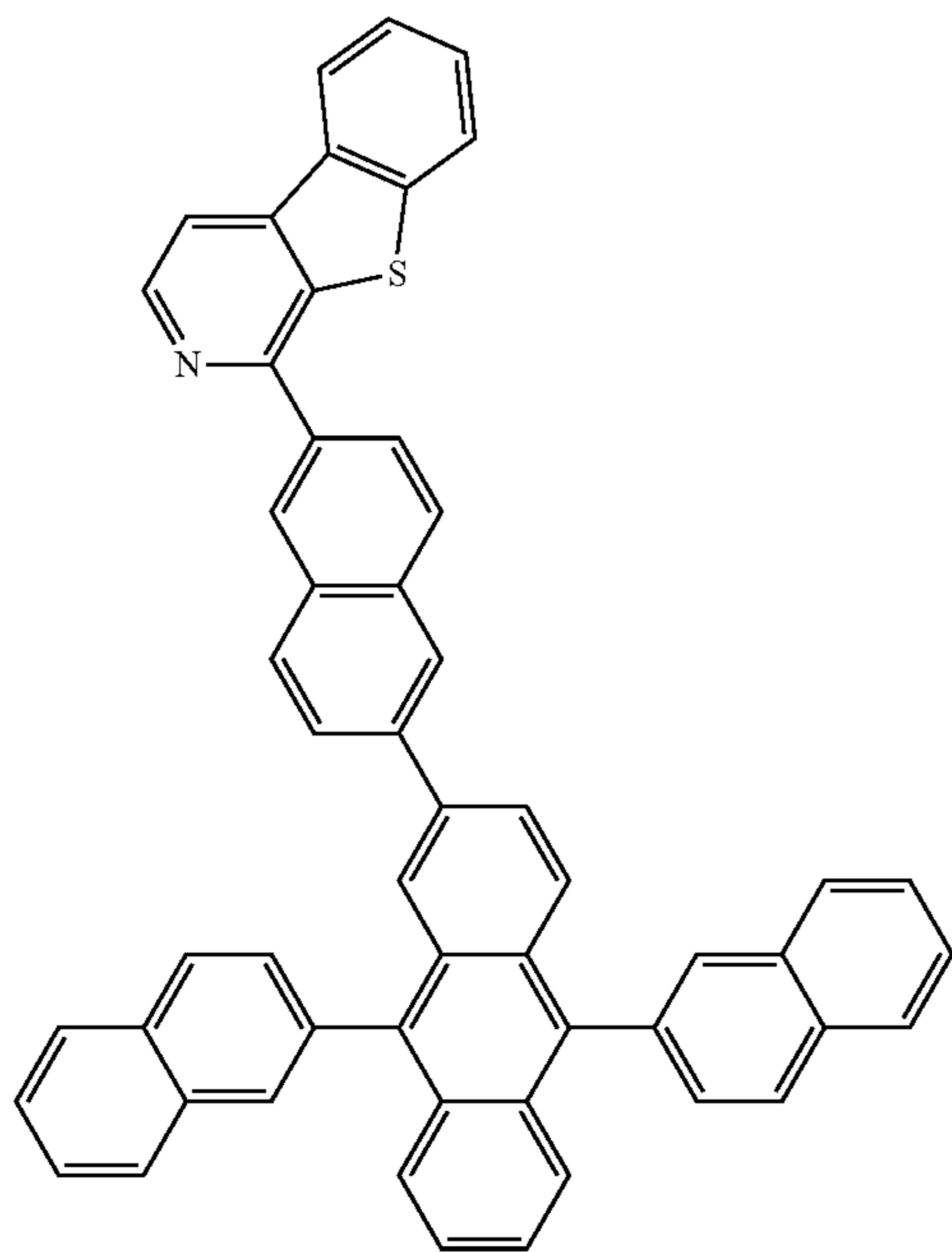
Compound 5
