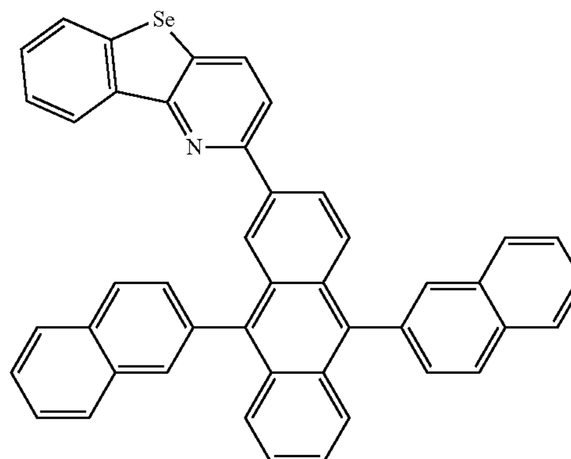
Compound 52
