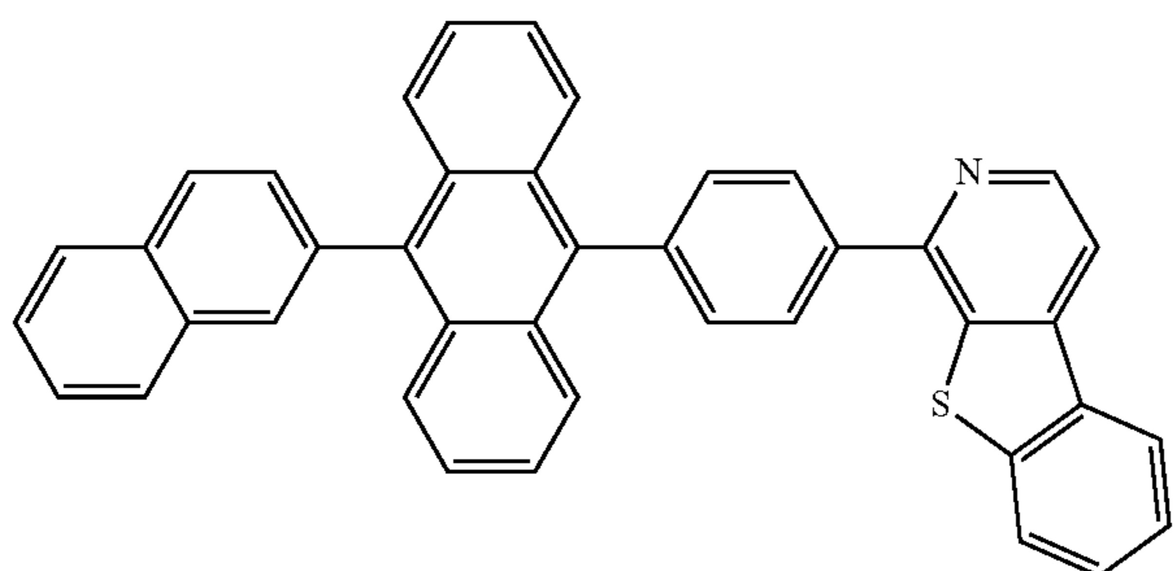
Compound 11
