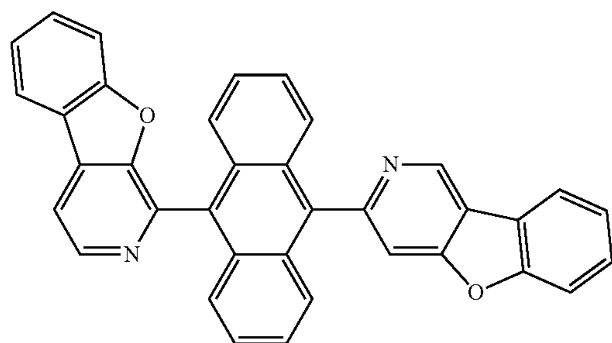
Compound 58
