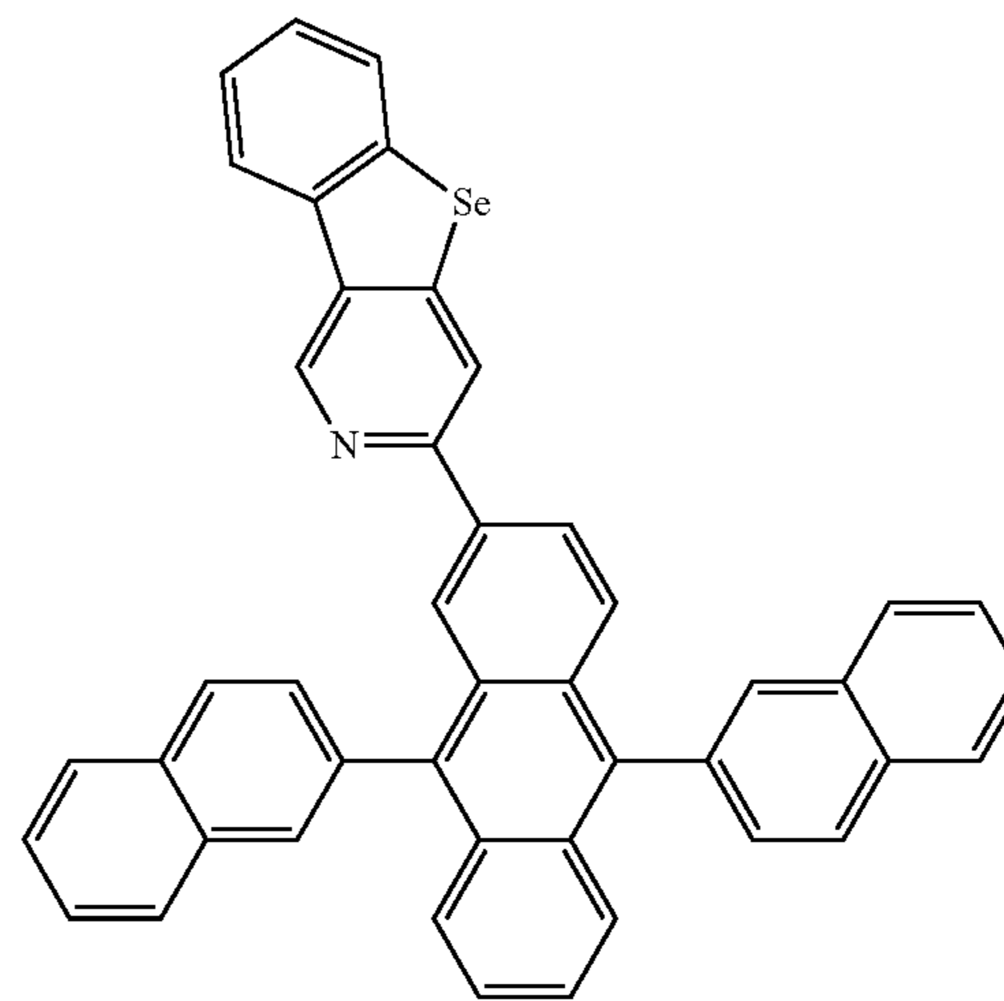
Compound 54
