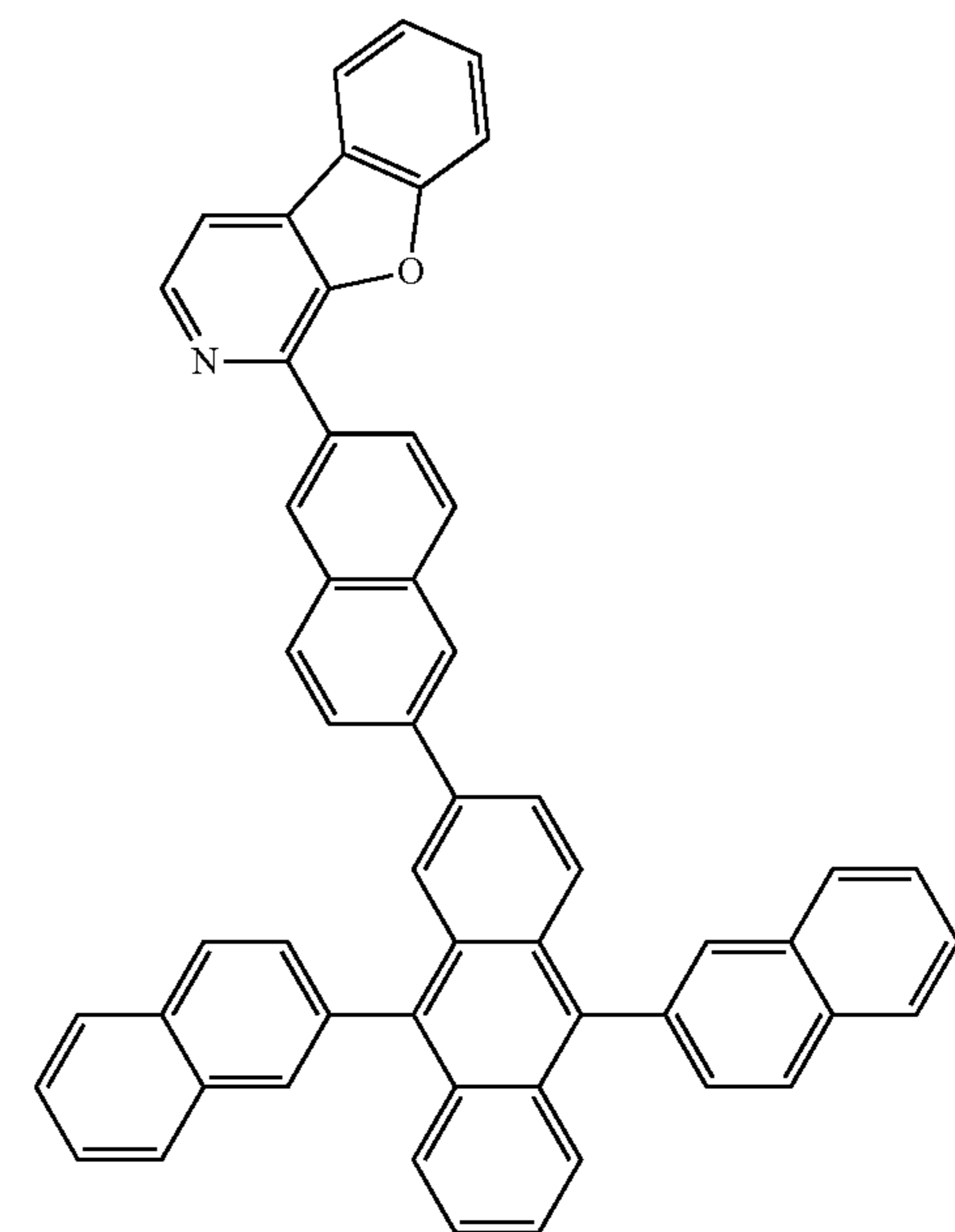
Compound 24
