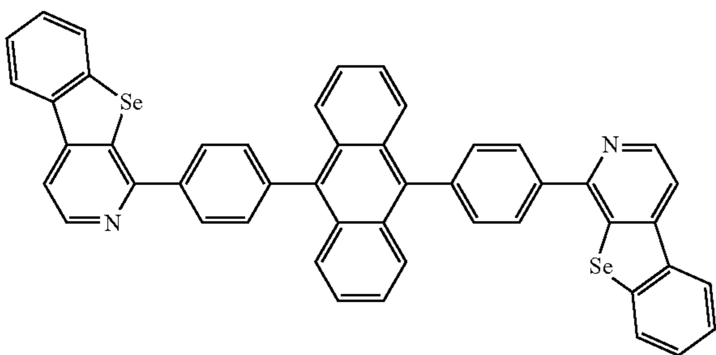
Compound 50
