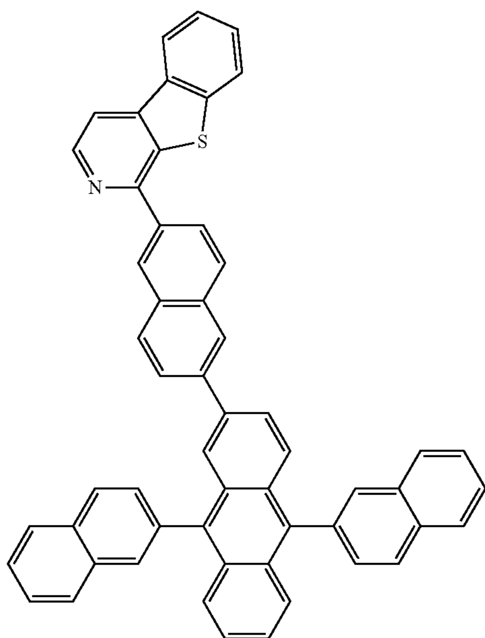
Compound 5
