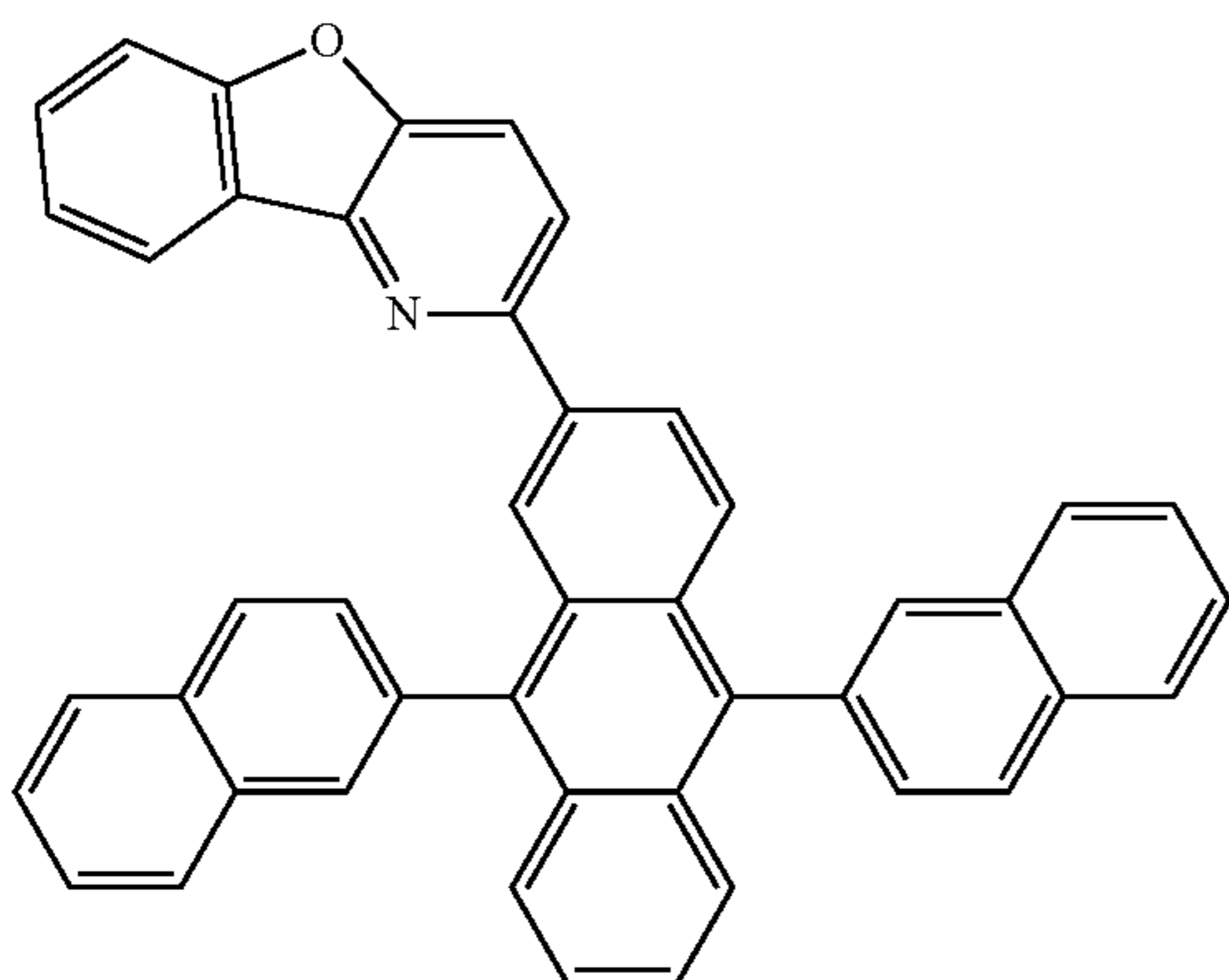
Compound 34
