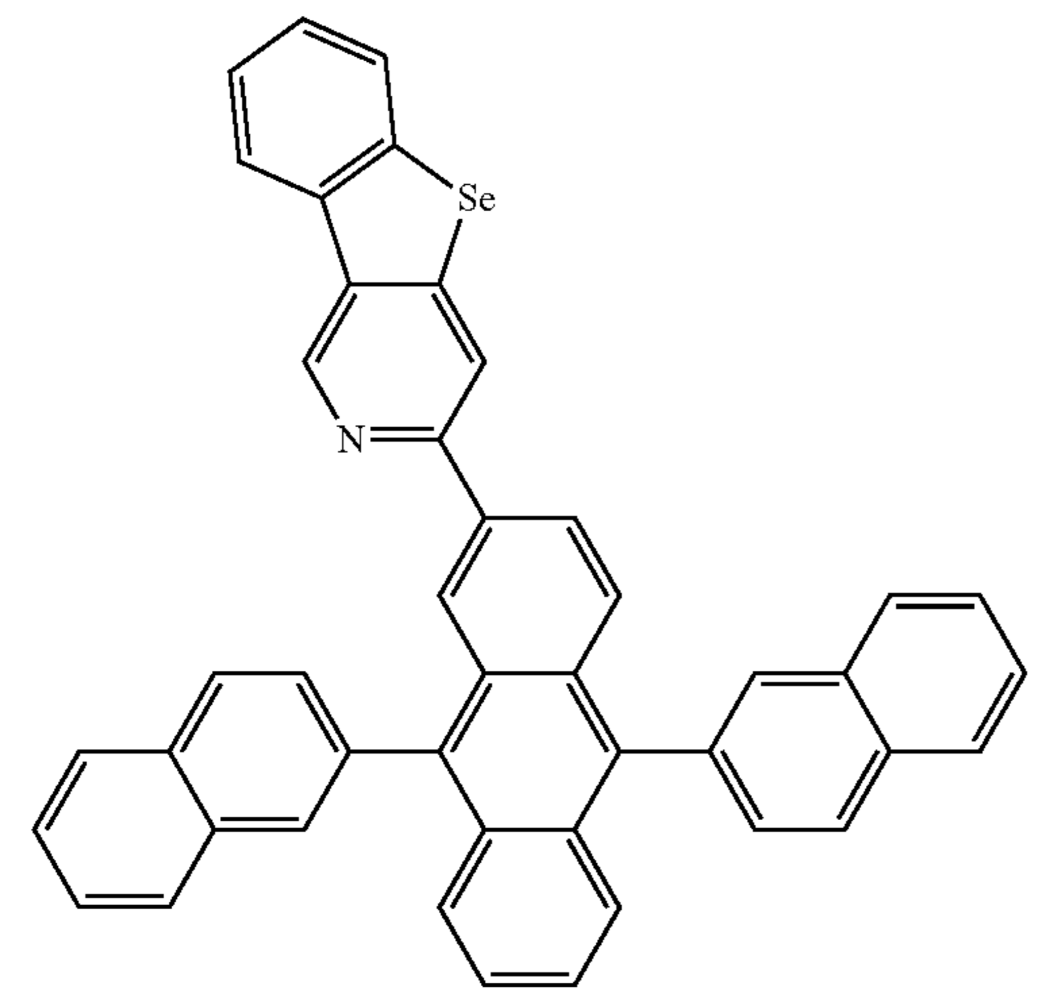
Compound 54
