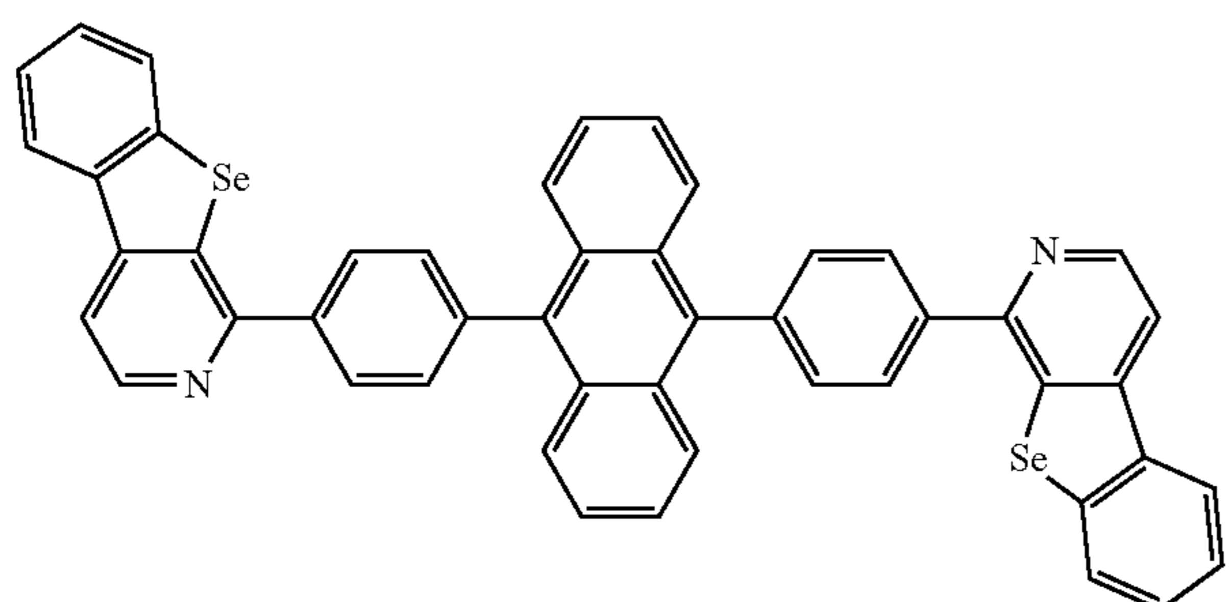
Compound 50
