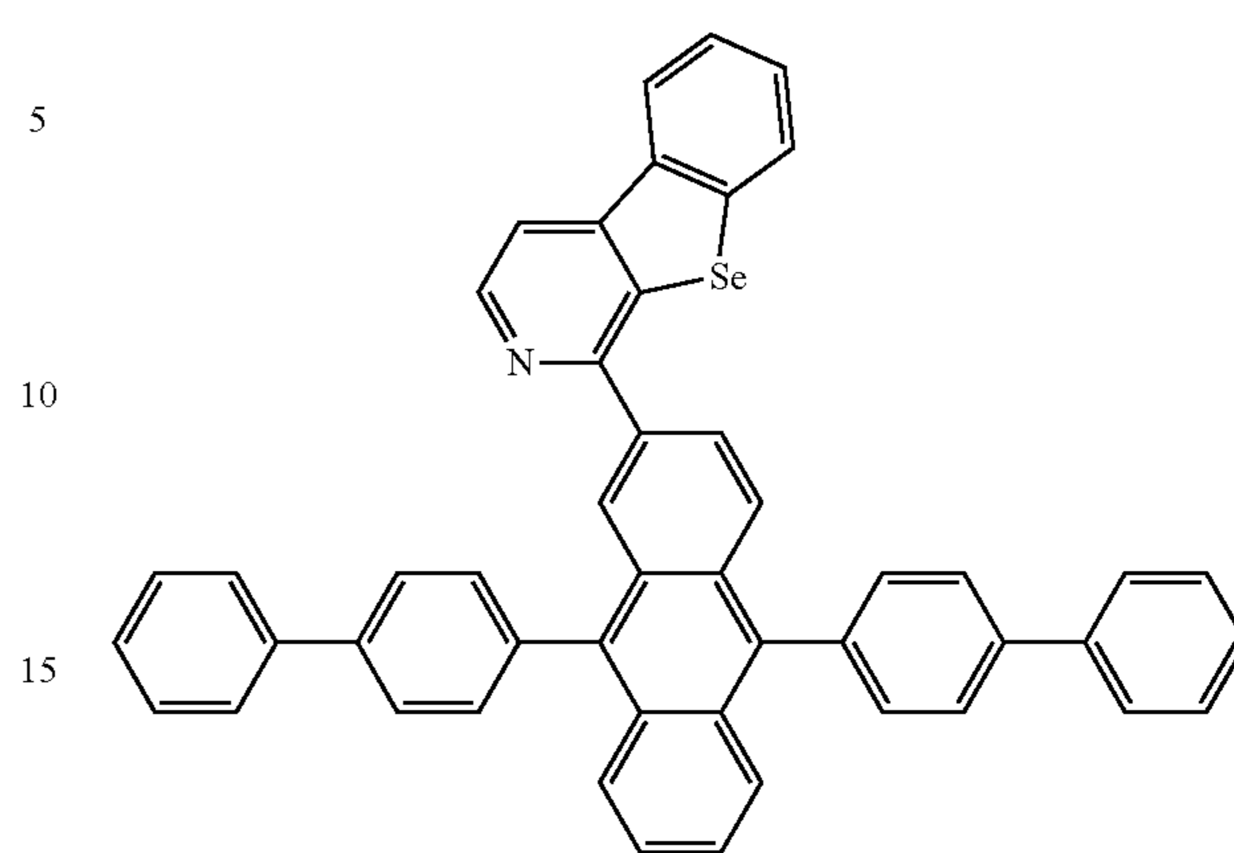
Compound 44
