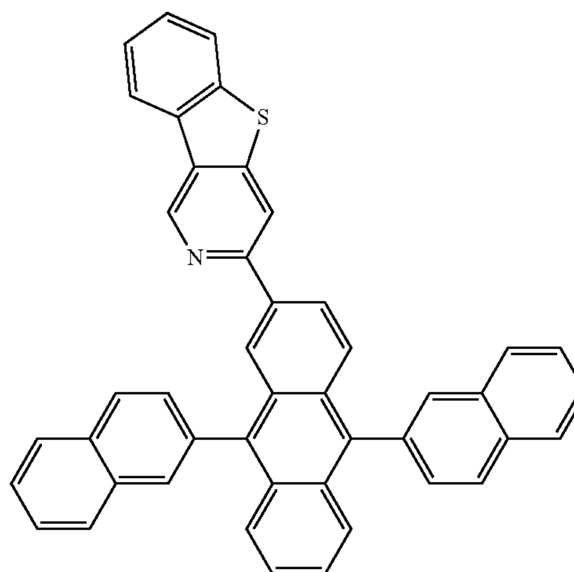
Compound 18
