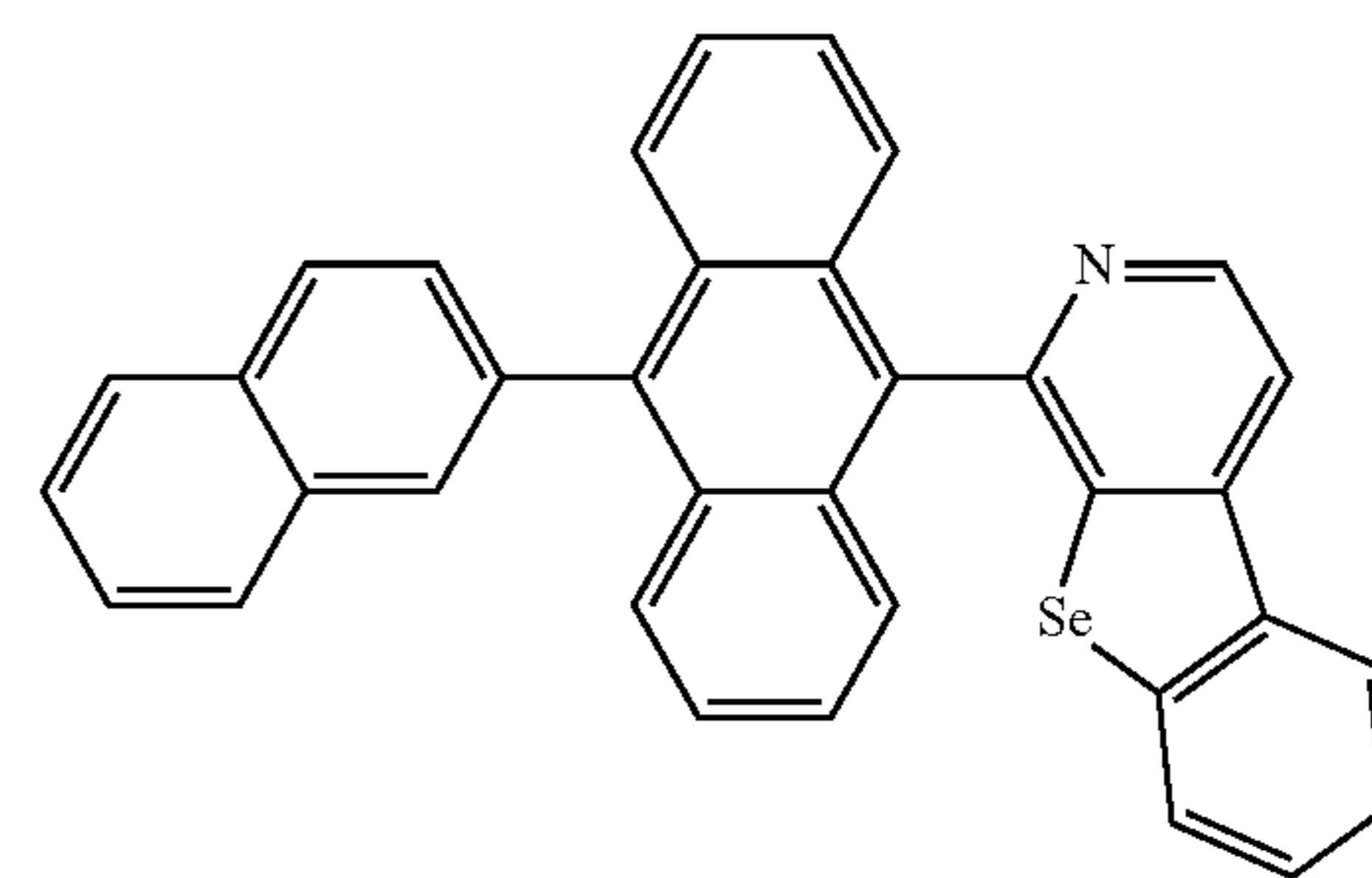
Compound 46
