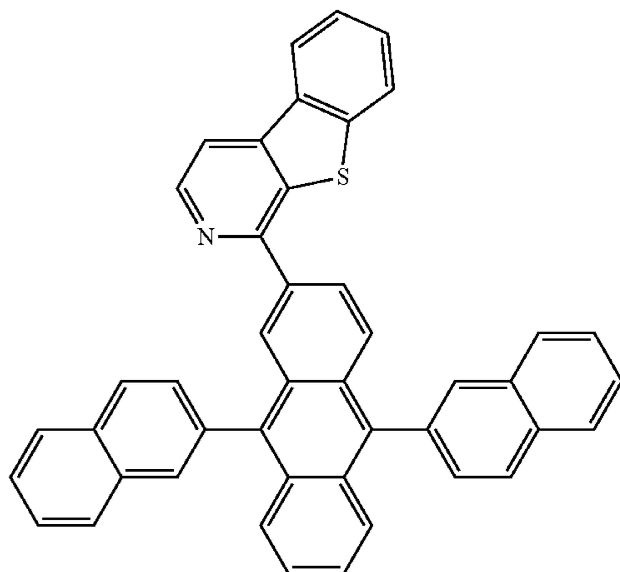
Compound 1
