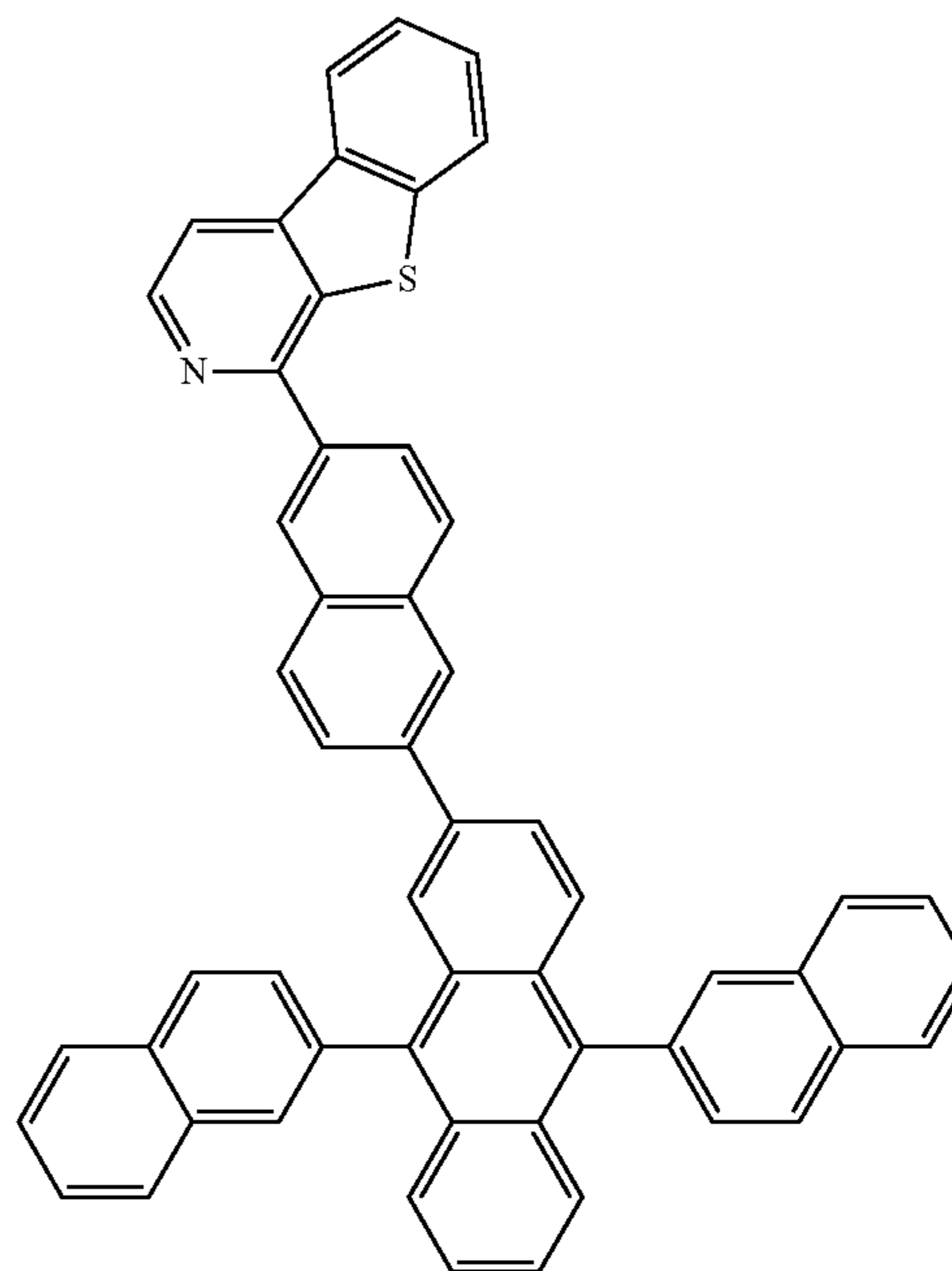
Compound 5
