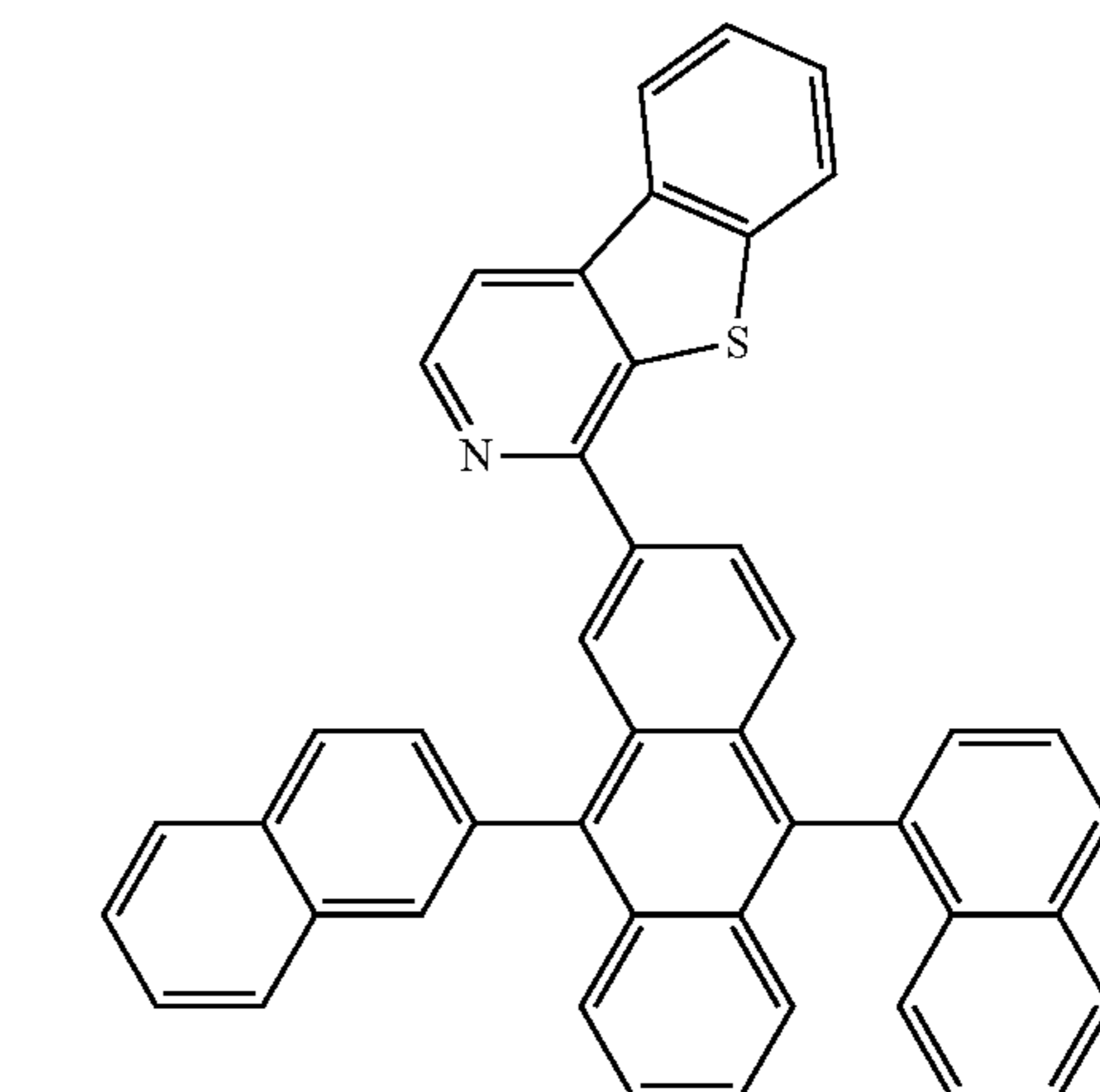
Compound 6
