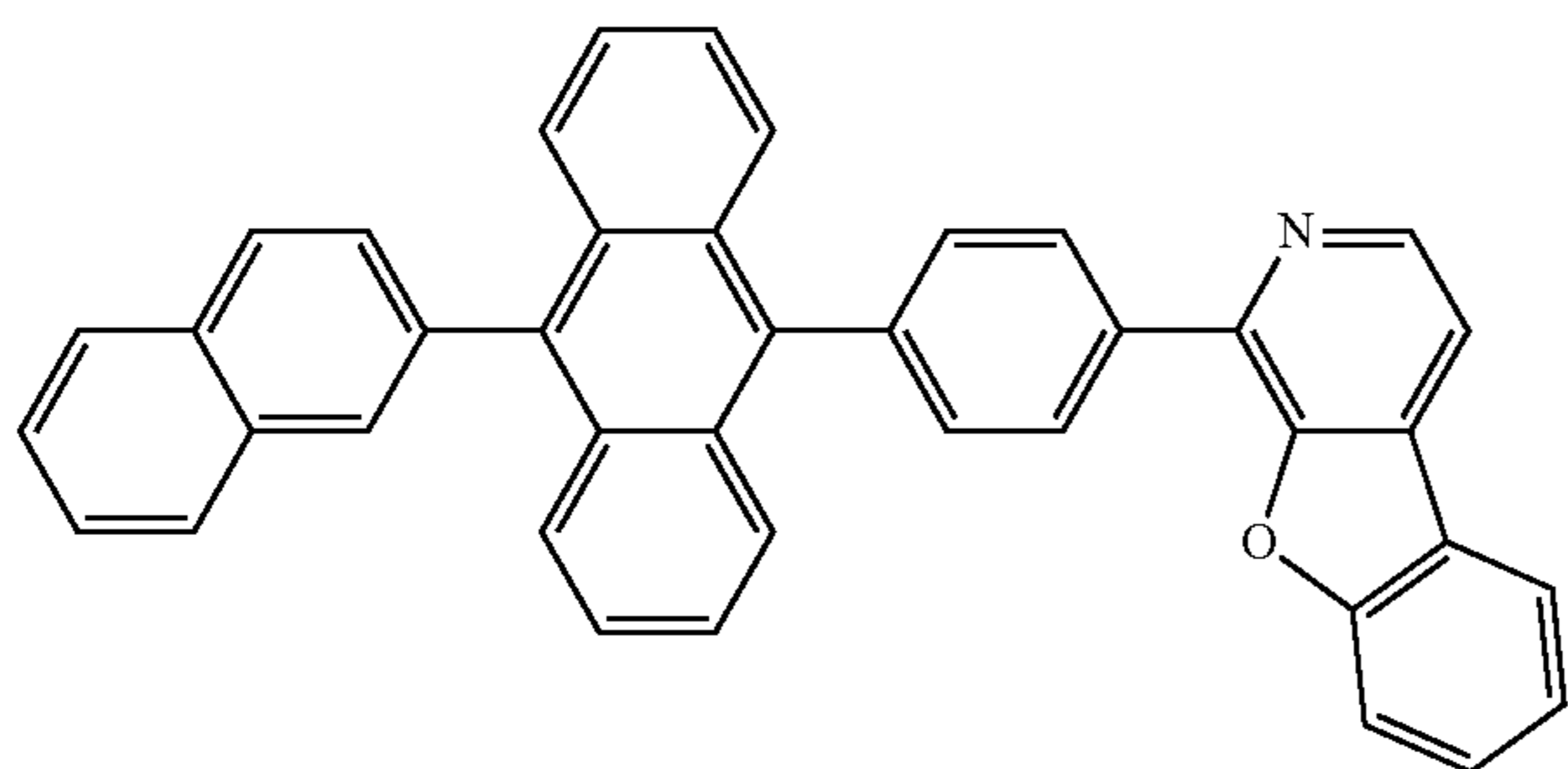
Compound 29
