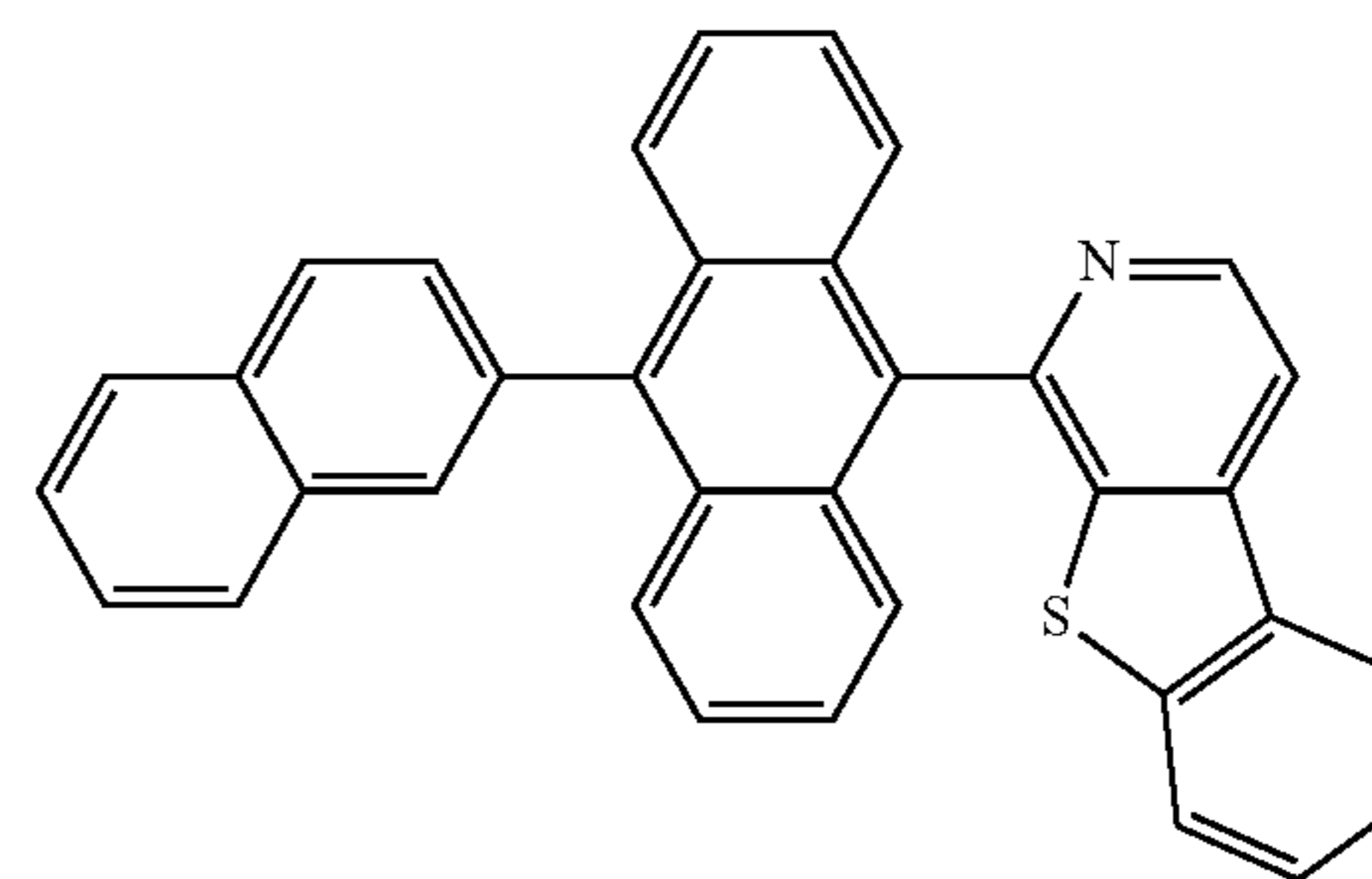
Compound 10
