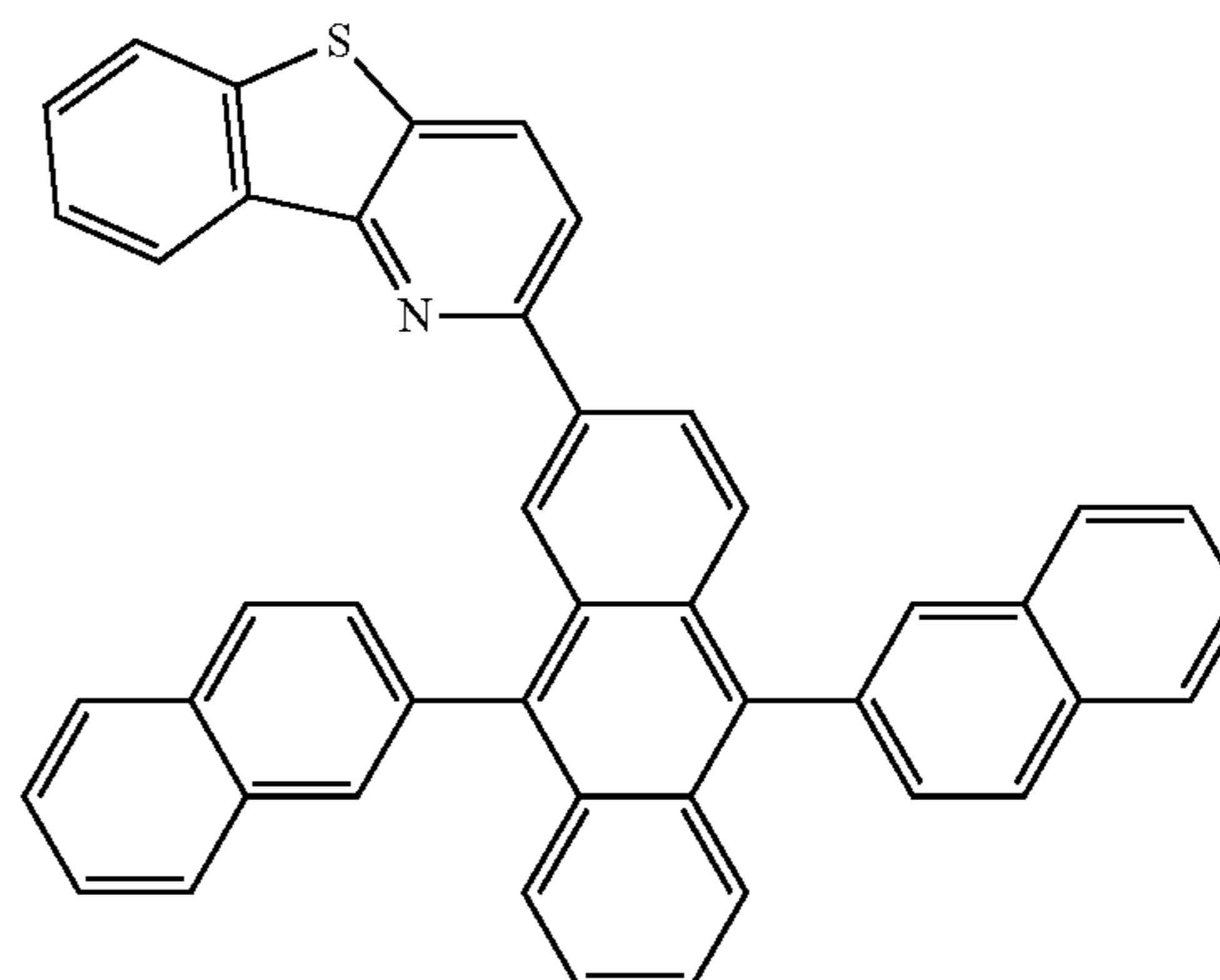
Compound 16
