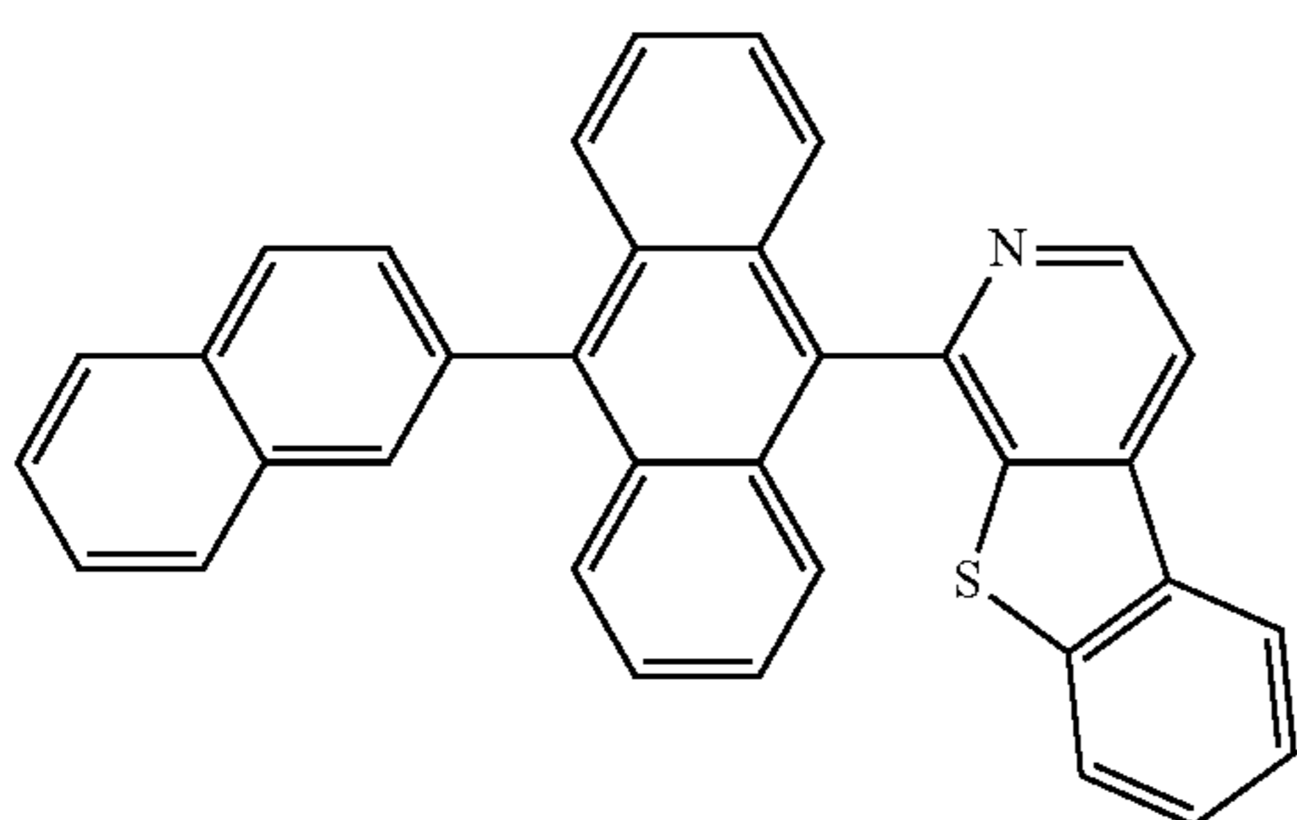
Compound 10
