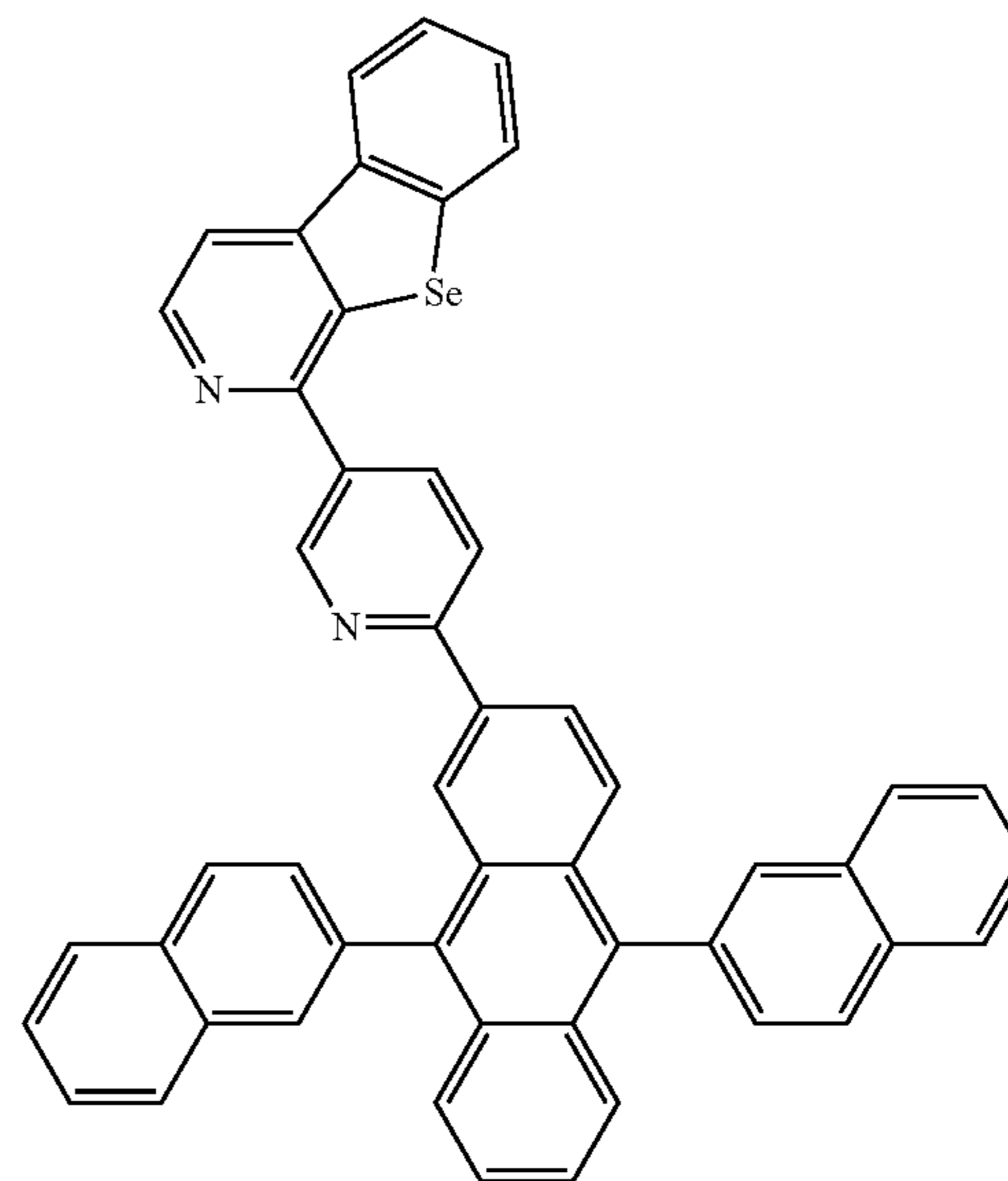
Compound 39
