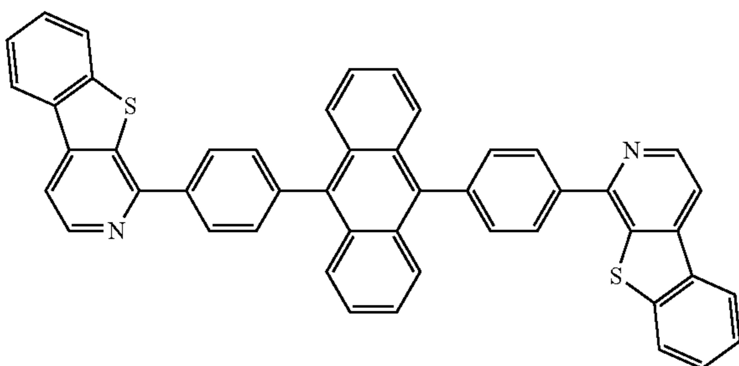
Compound 14
