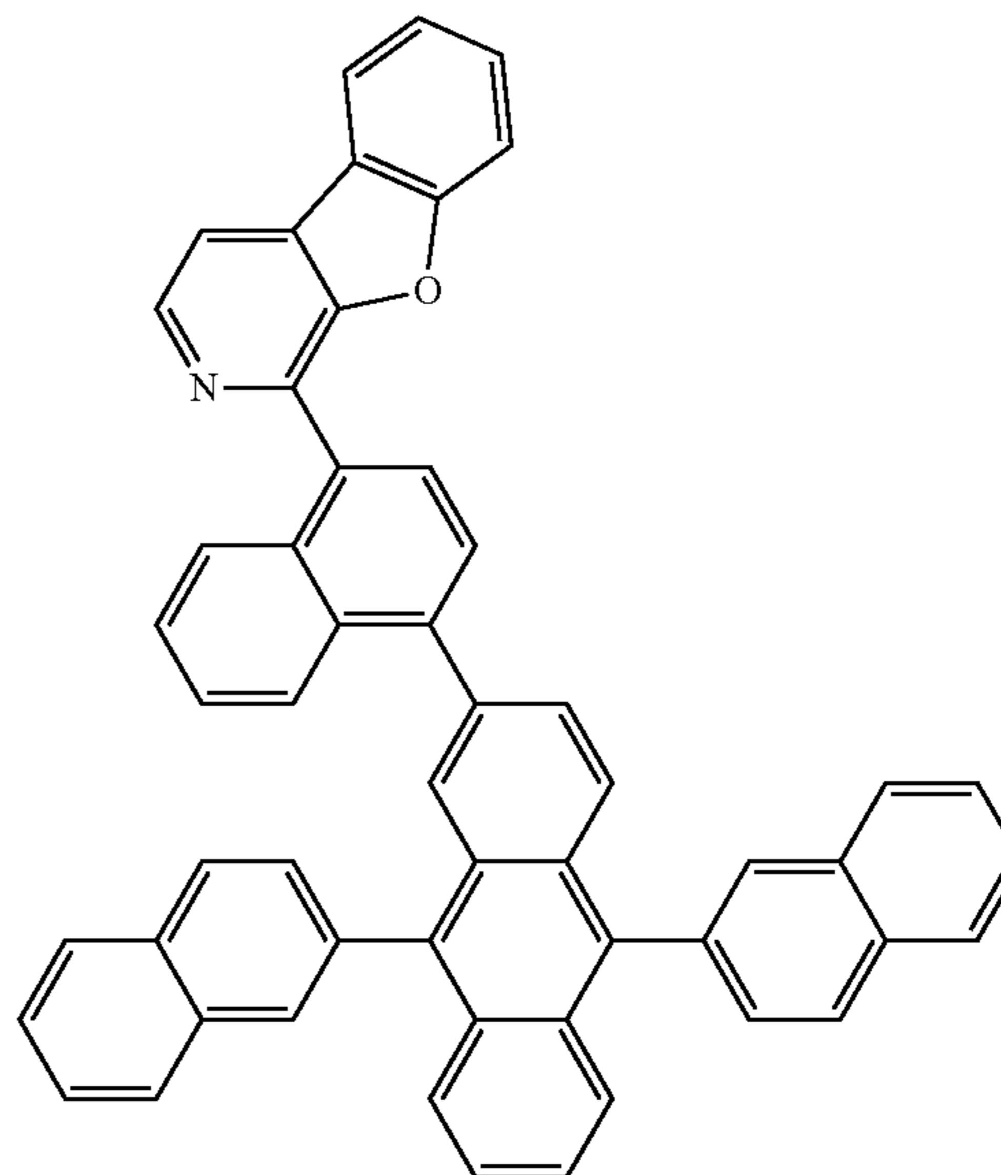
Compound 23
