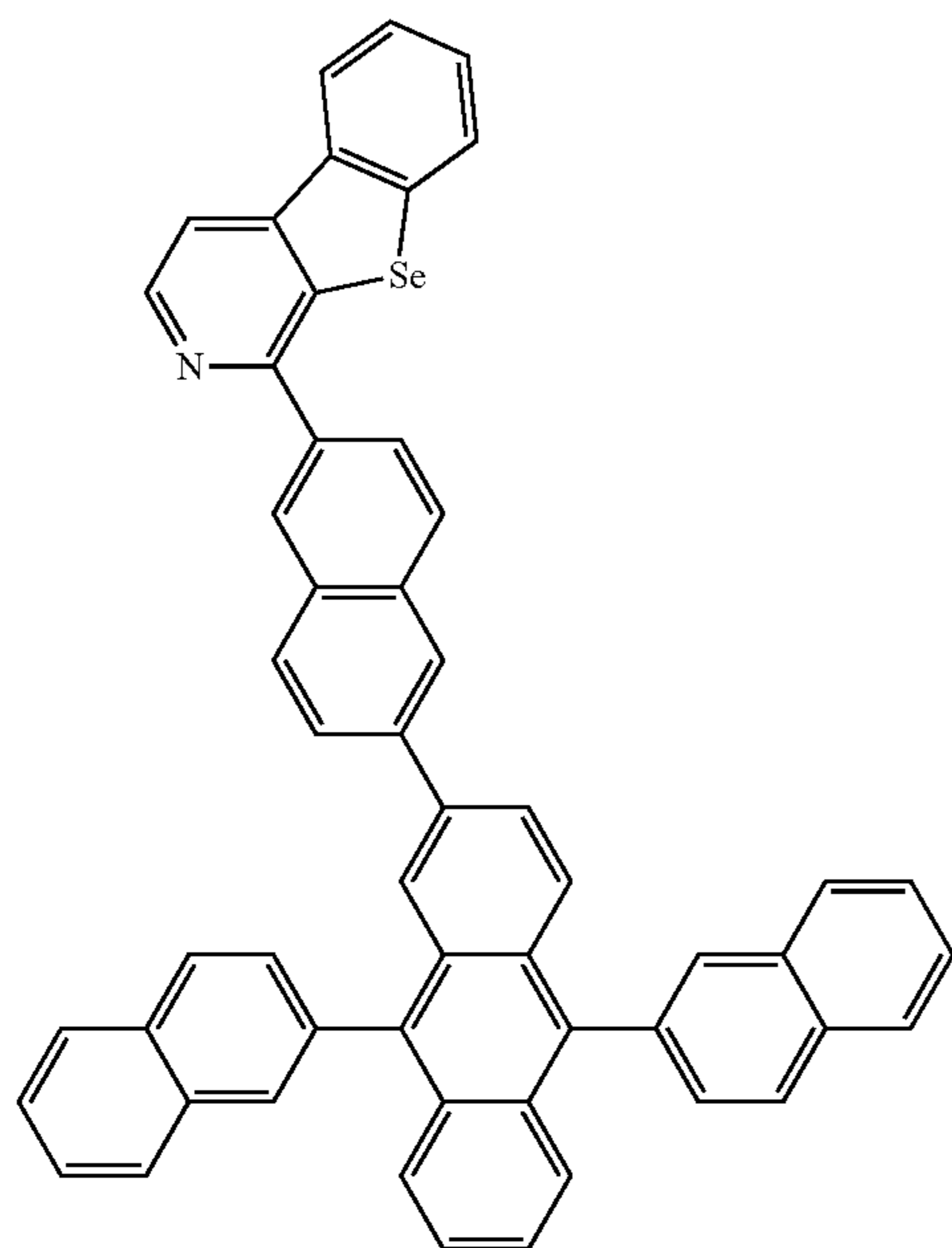
Compound 42
