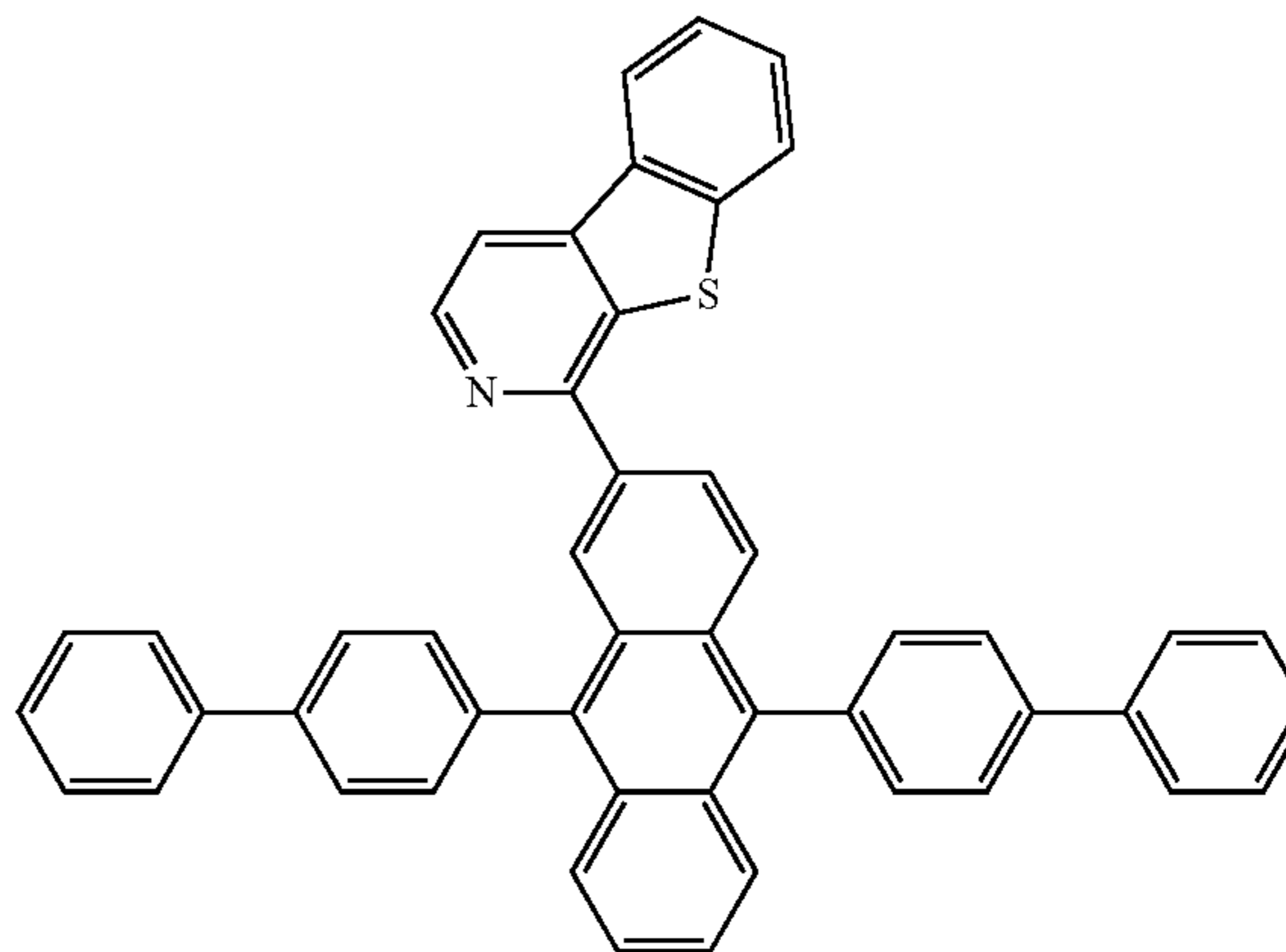
Compound 7
