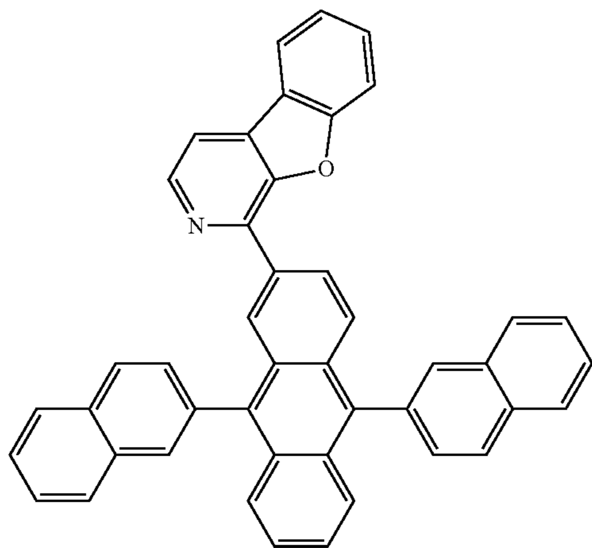
Compound 19
