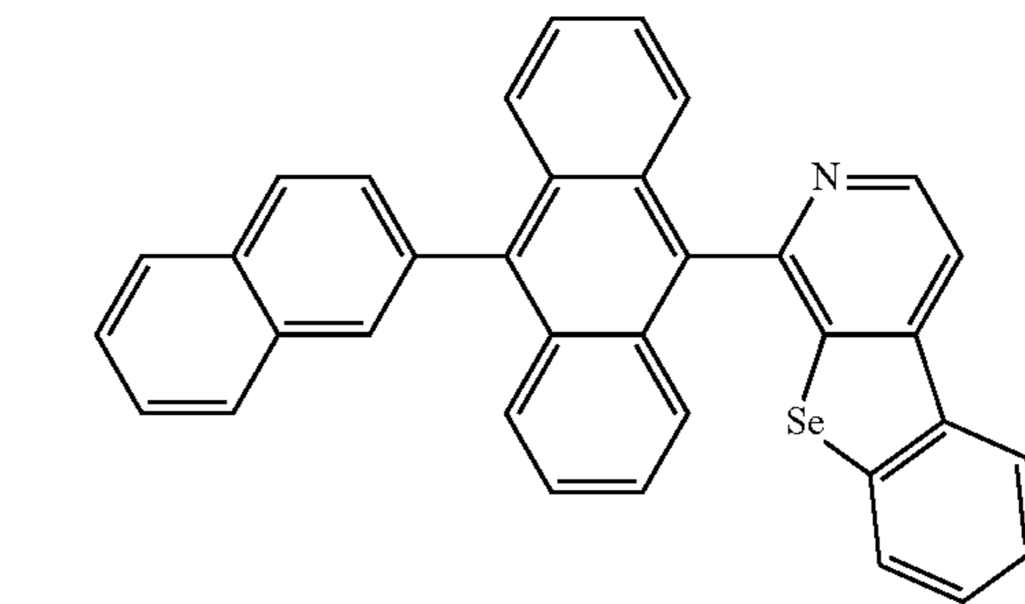
Compound 46
