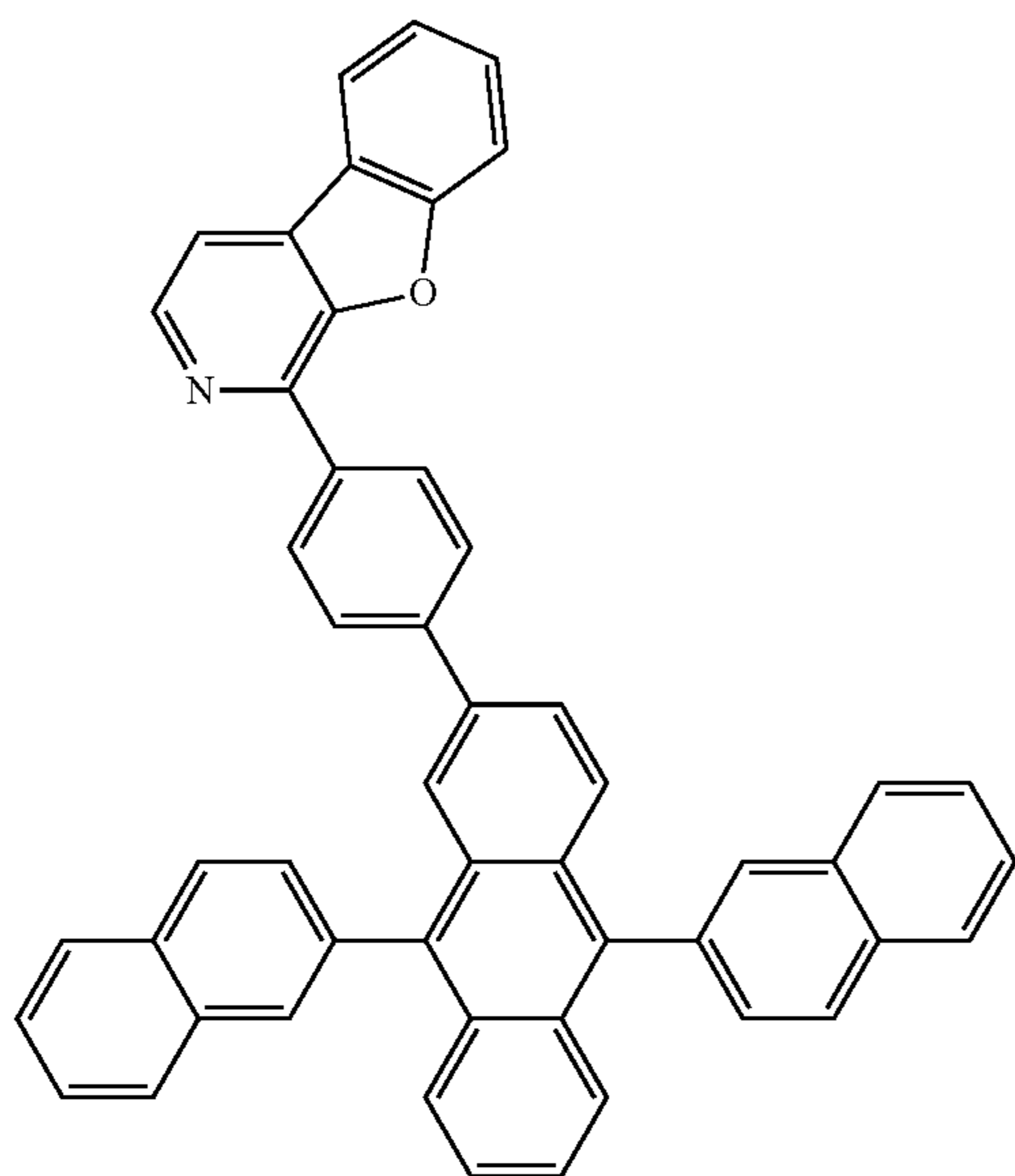
Compound 21
