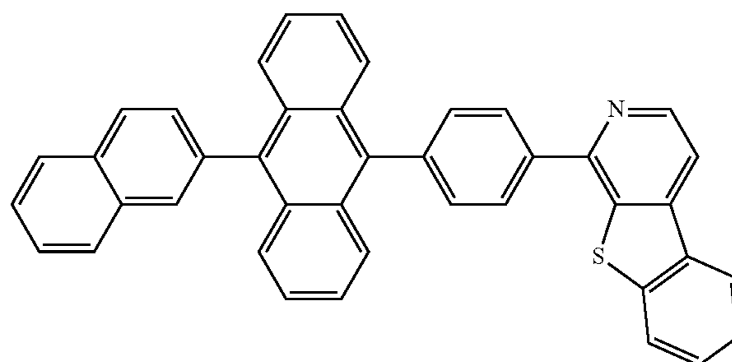
Compound 11
