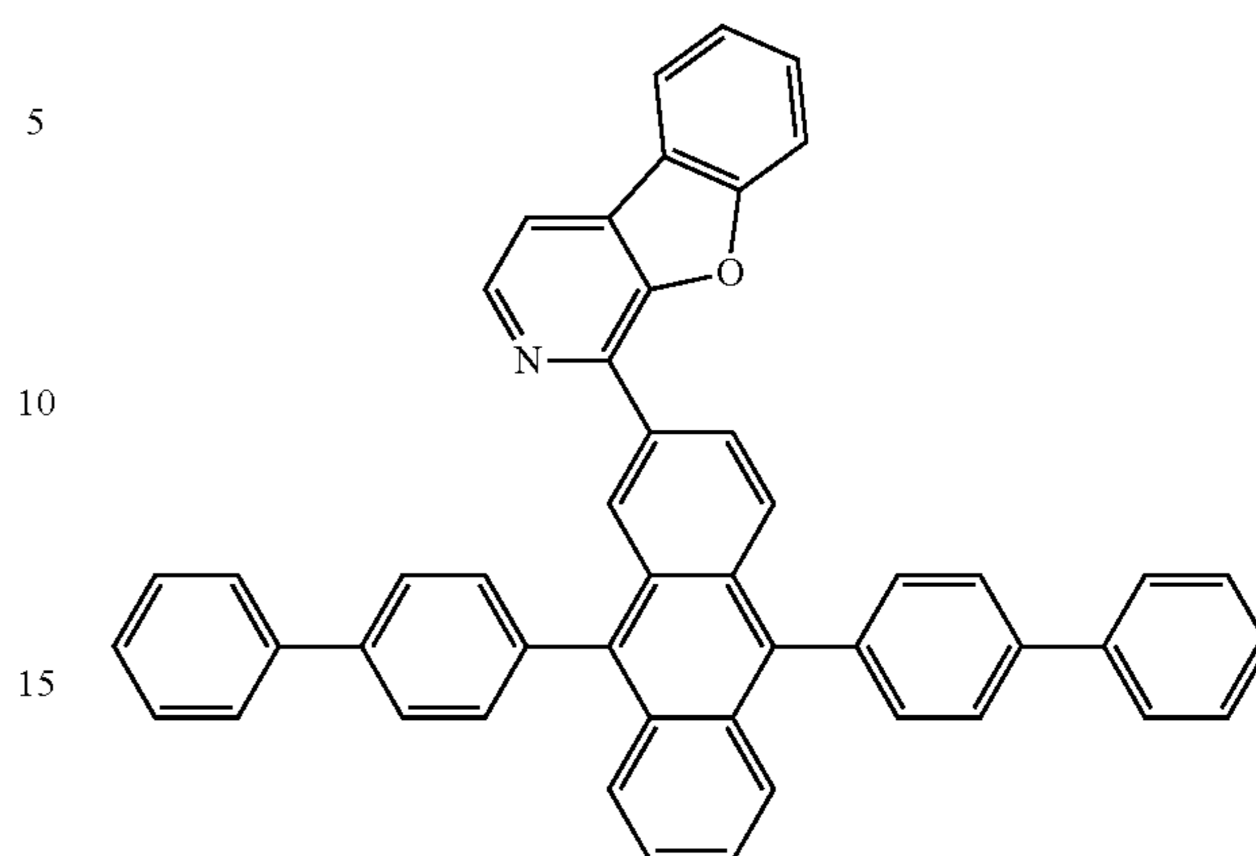
Compound 26
