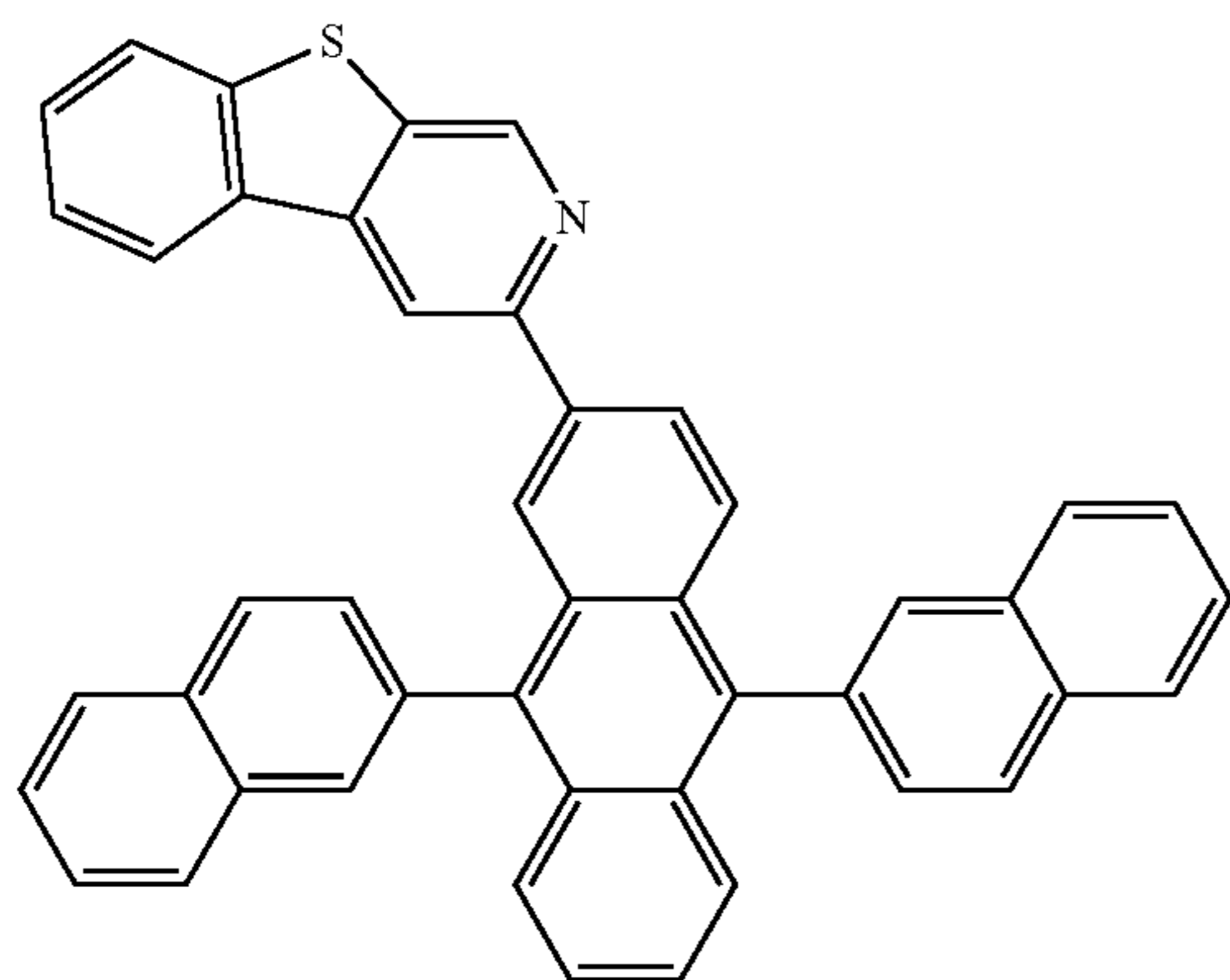
Compound 15
