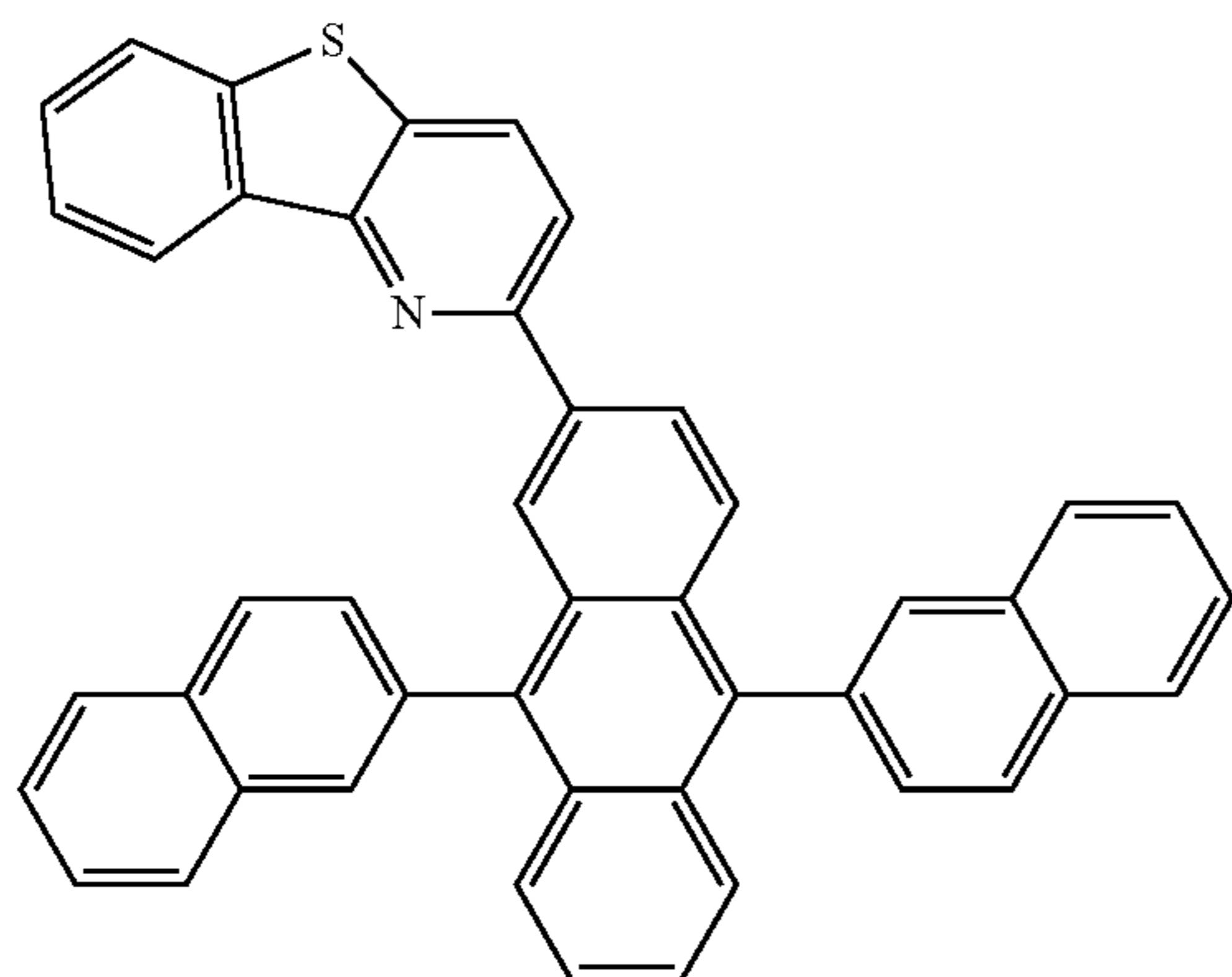
Compound 16
