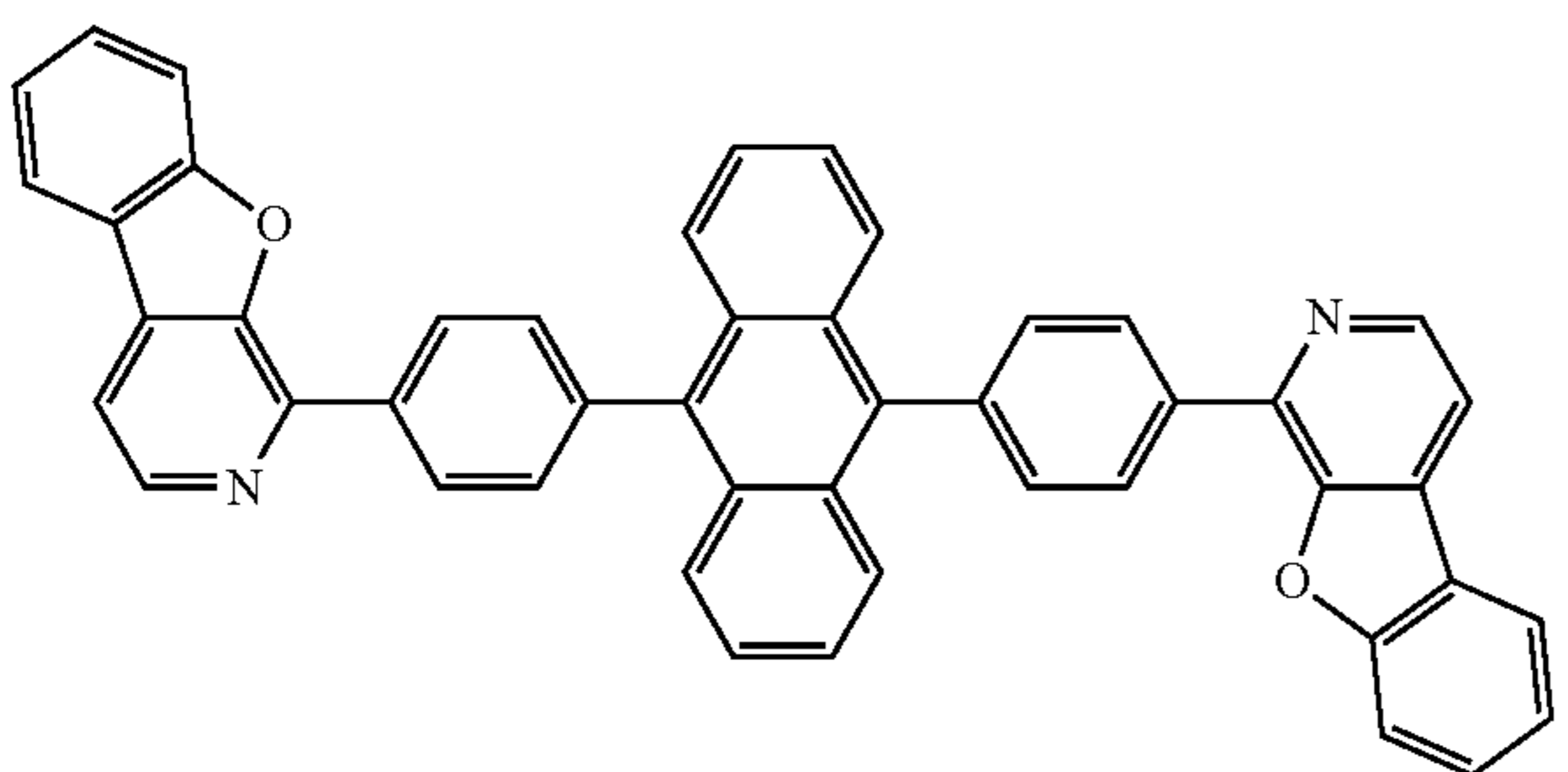
Compound 32
