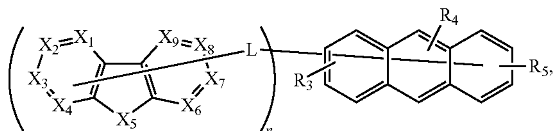
Formula VI
