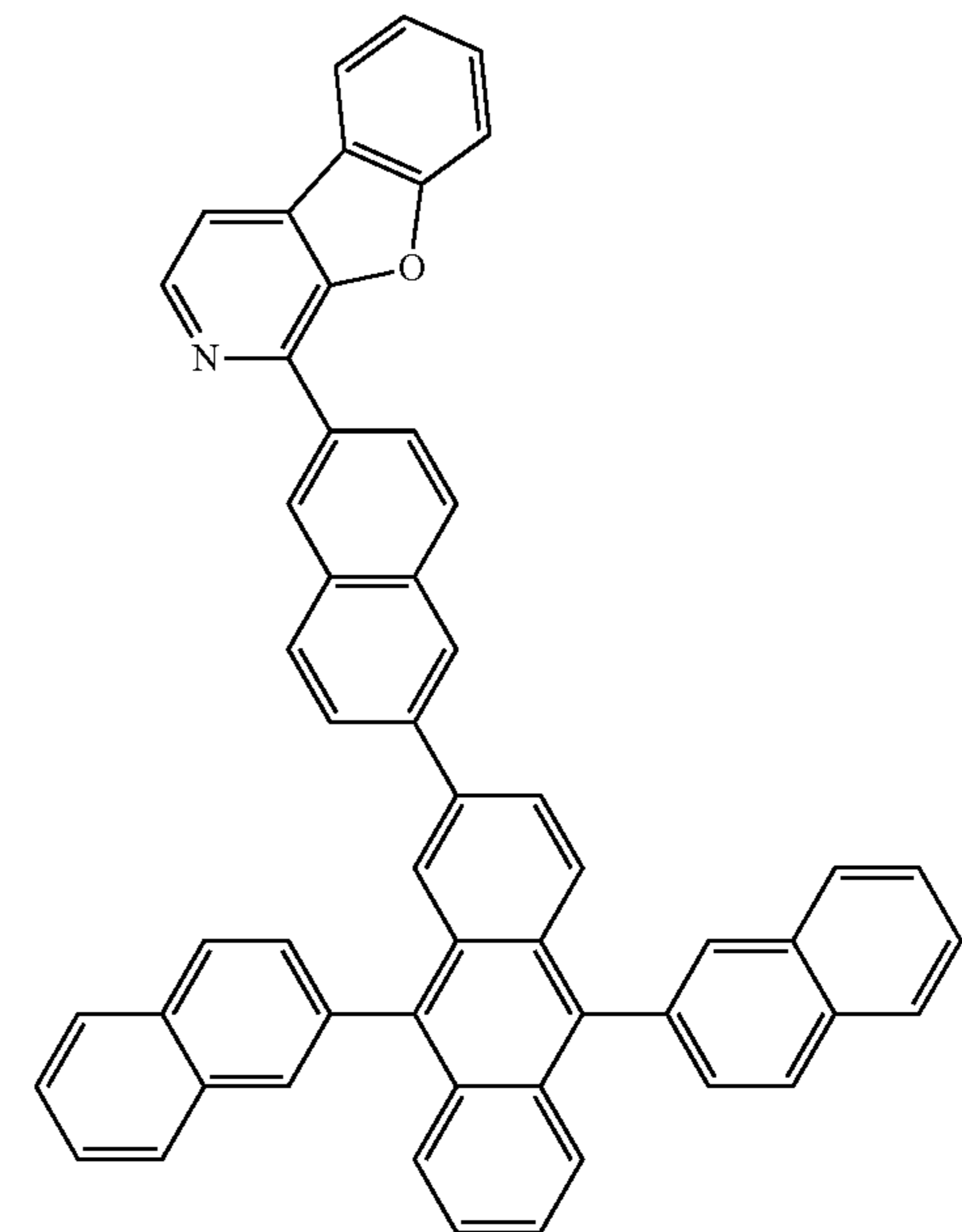
Compound 24
