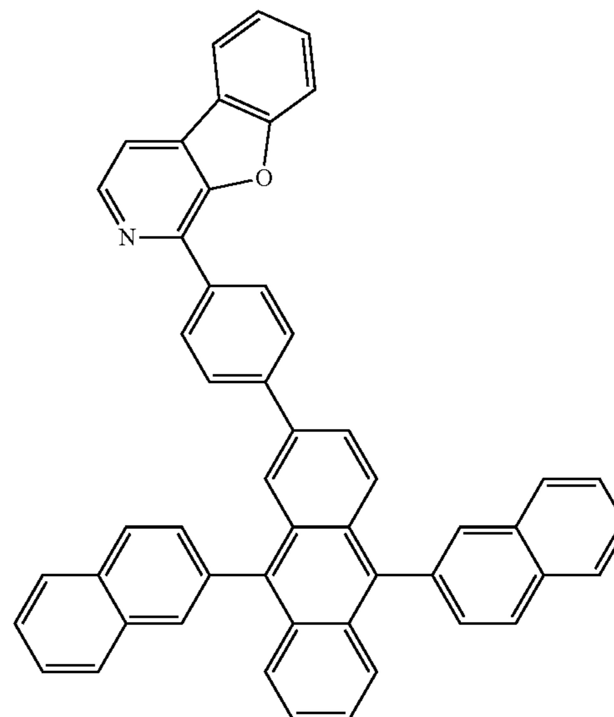
Compound 20
