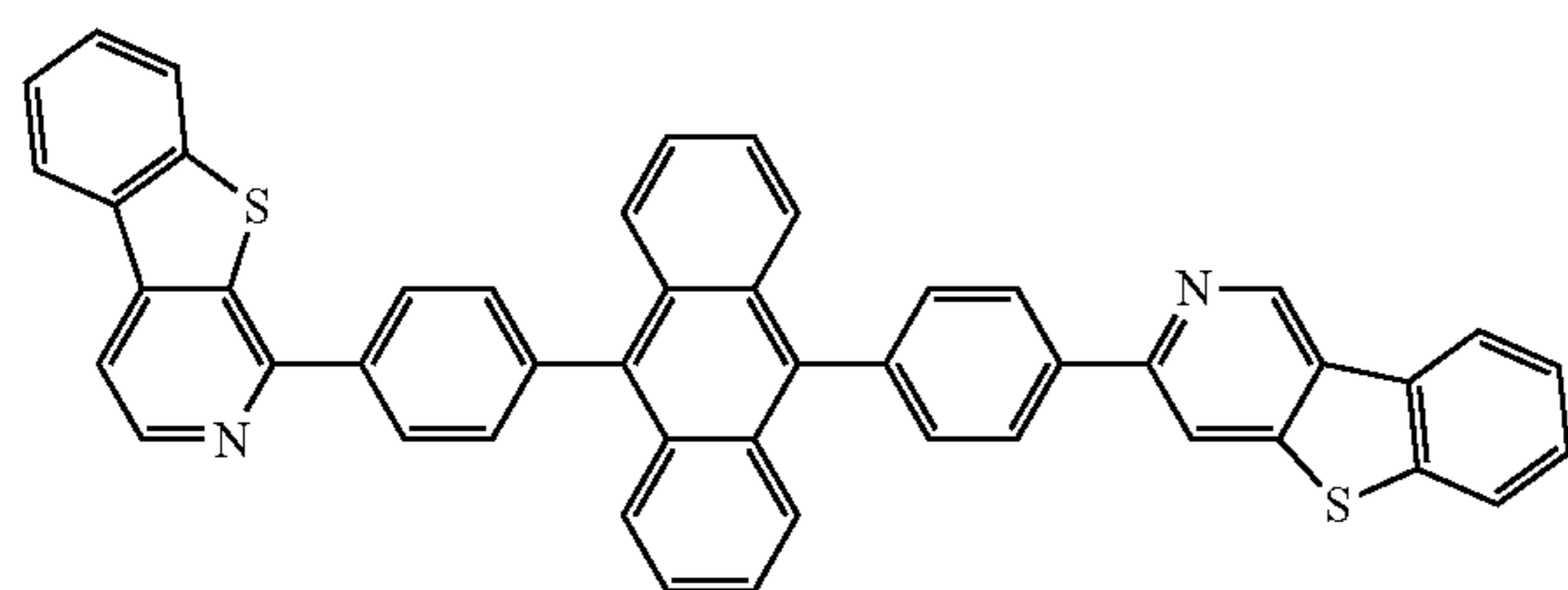
Compound 59
