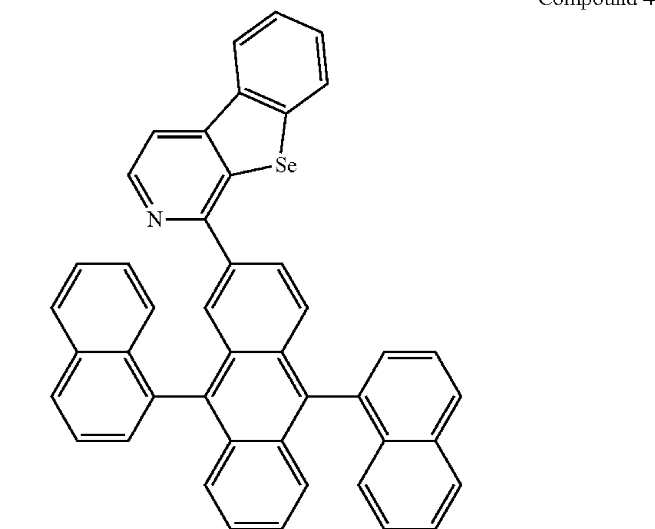
Compound 45
