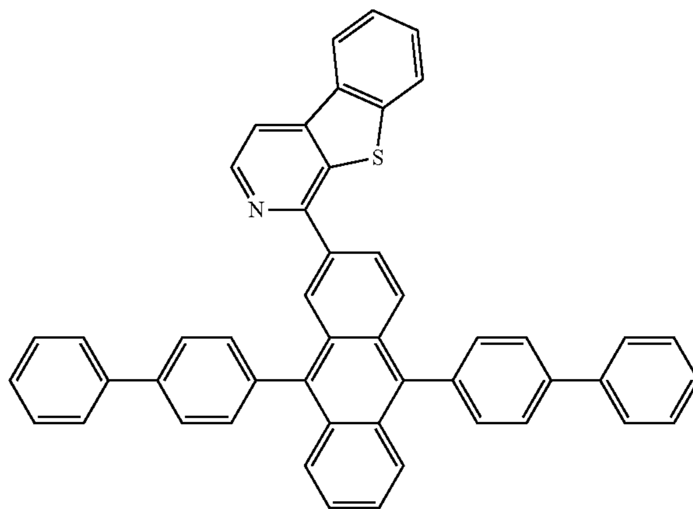
Compound 8
