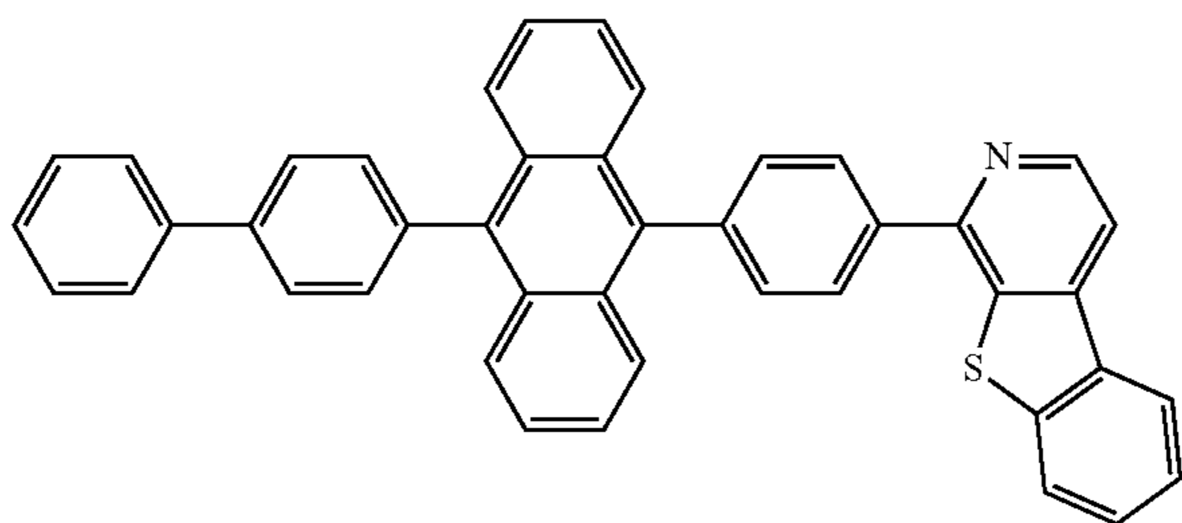
Compound 12
