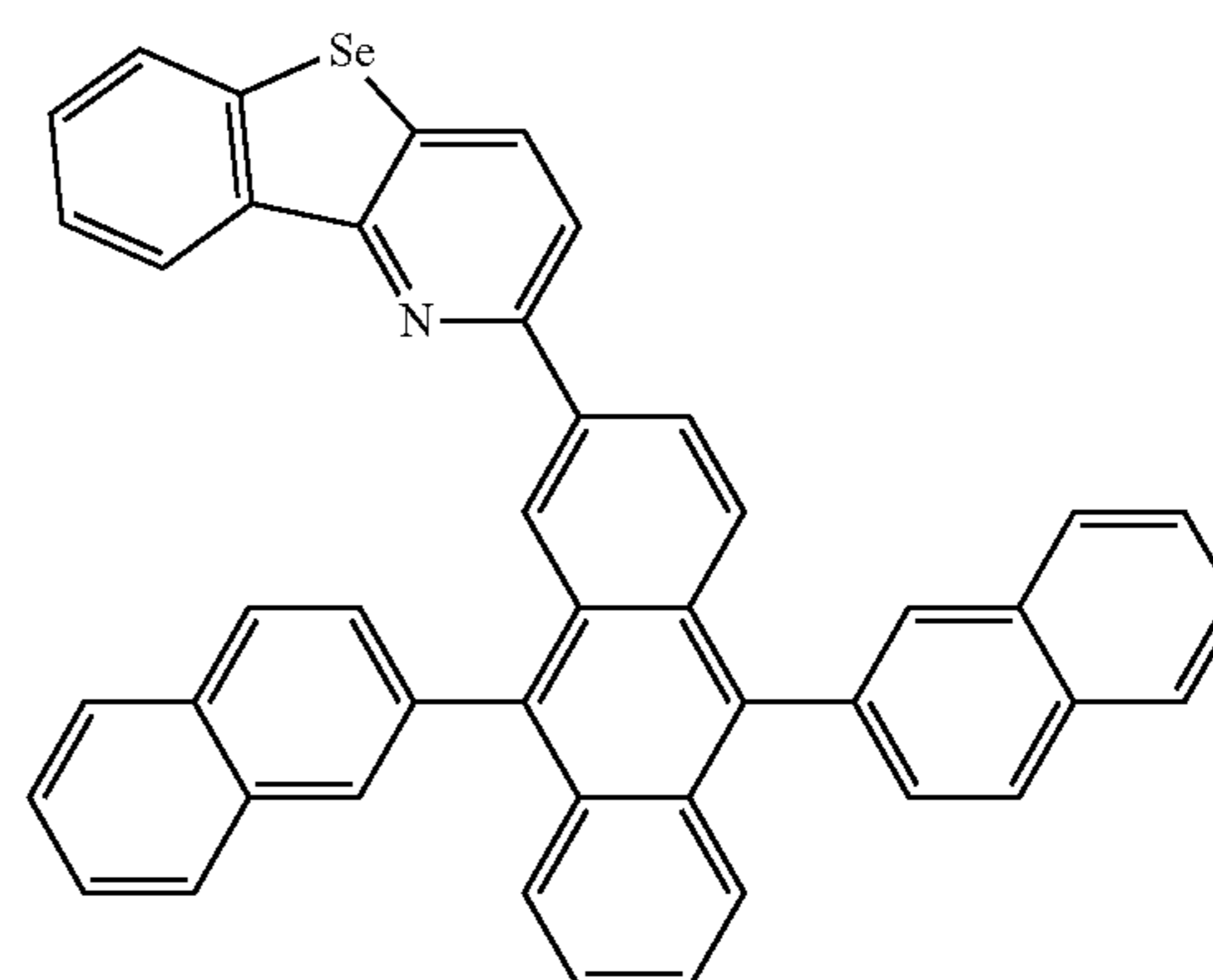
Compound 52
