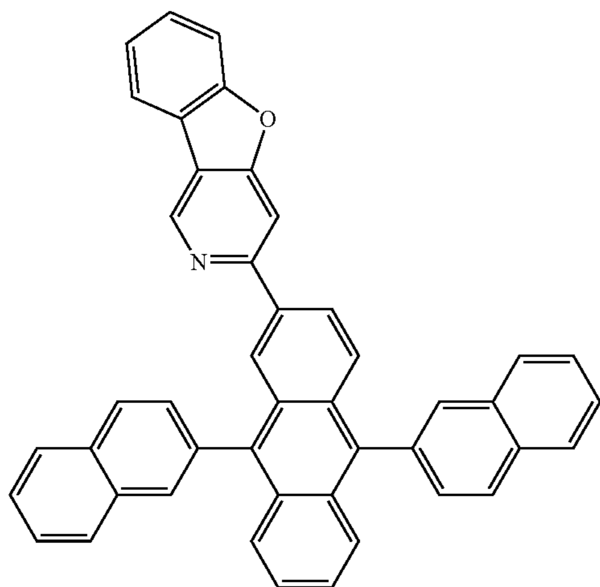
Compound 36
