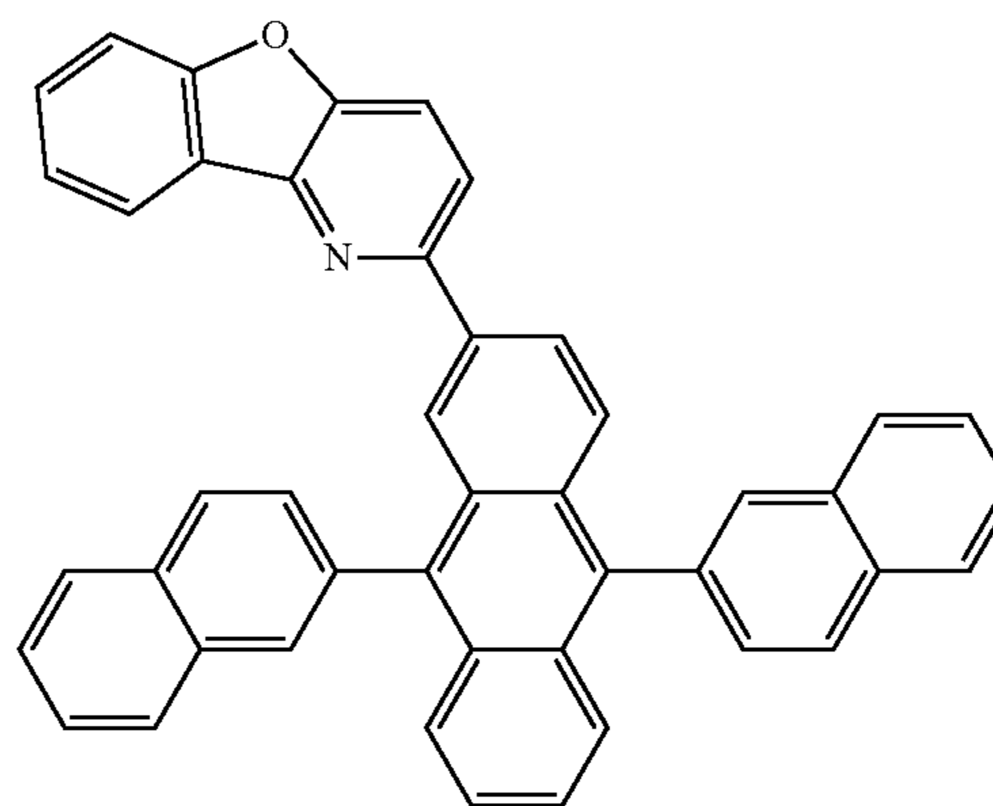
Compound 34
