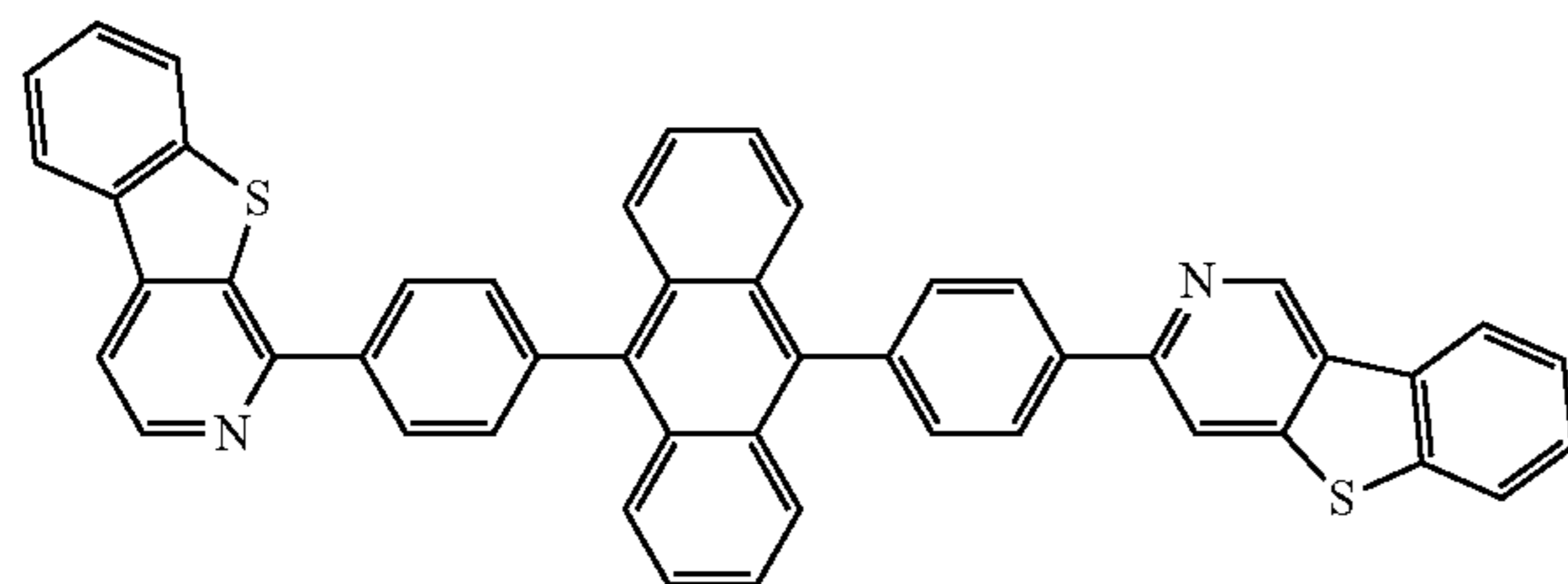
Compound 58
