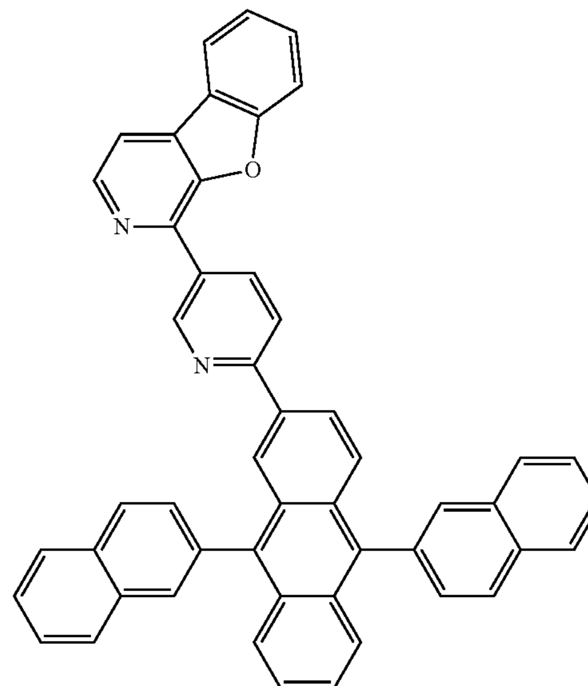
Compound 21
