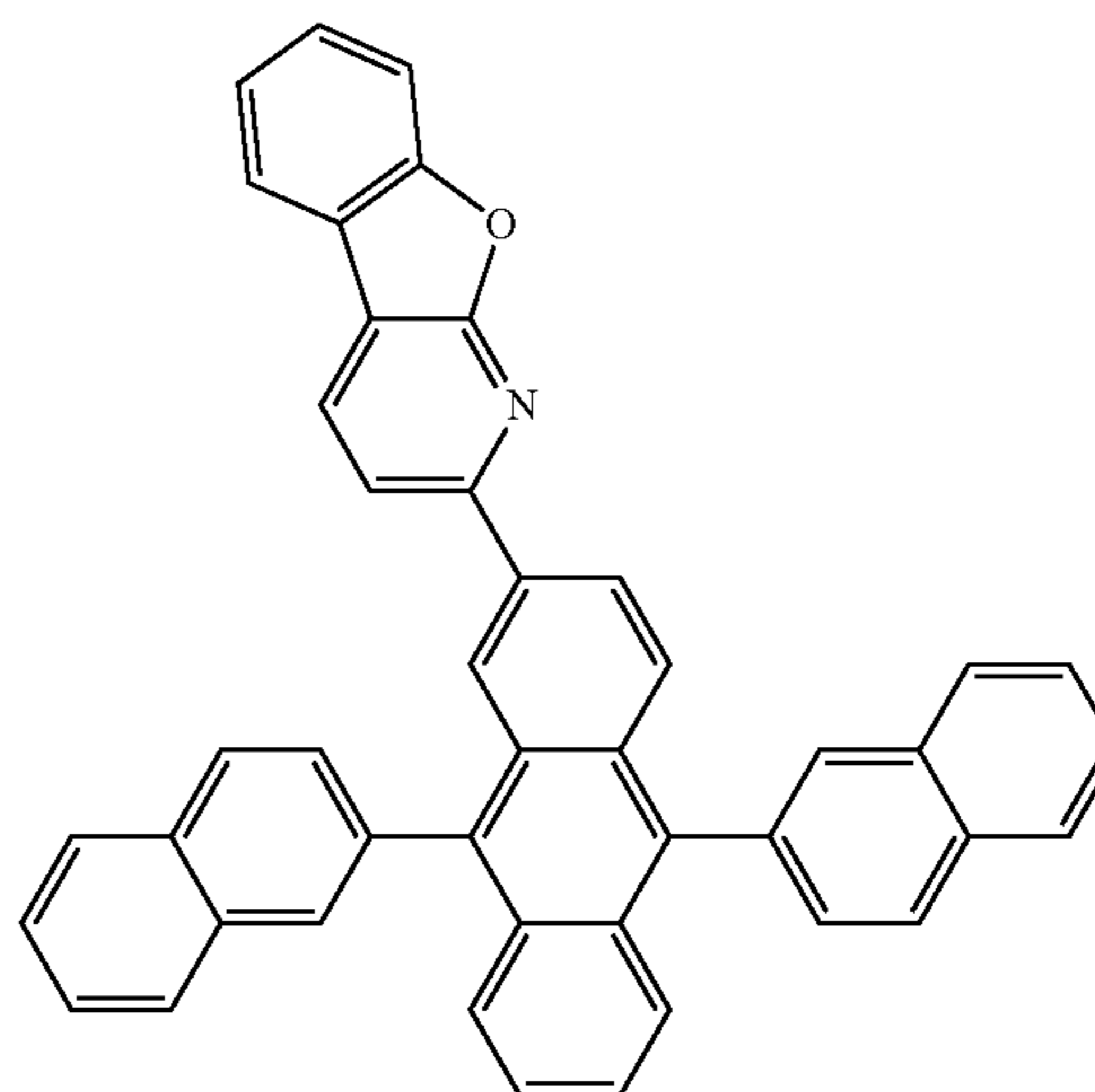
Compound 35
