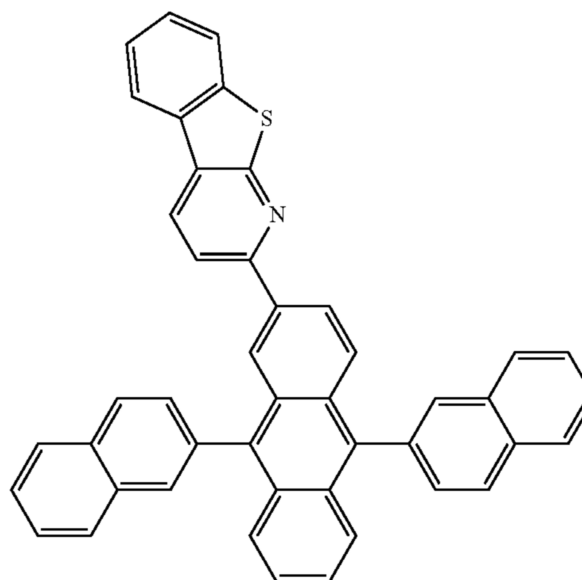
Compound 17
