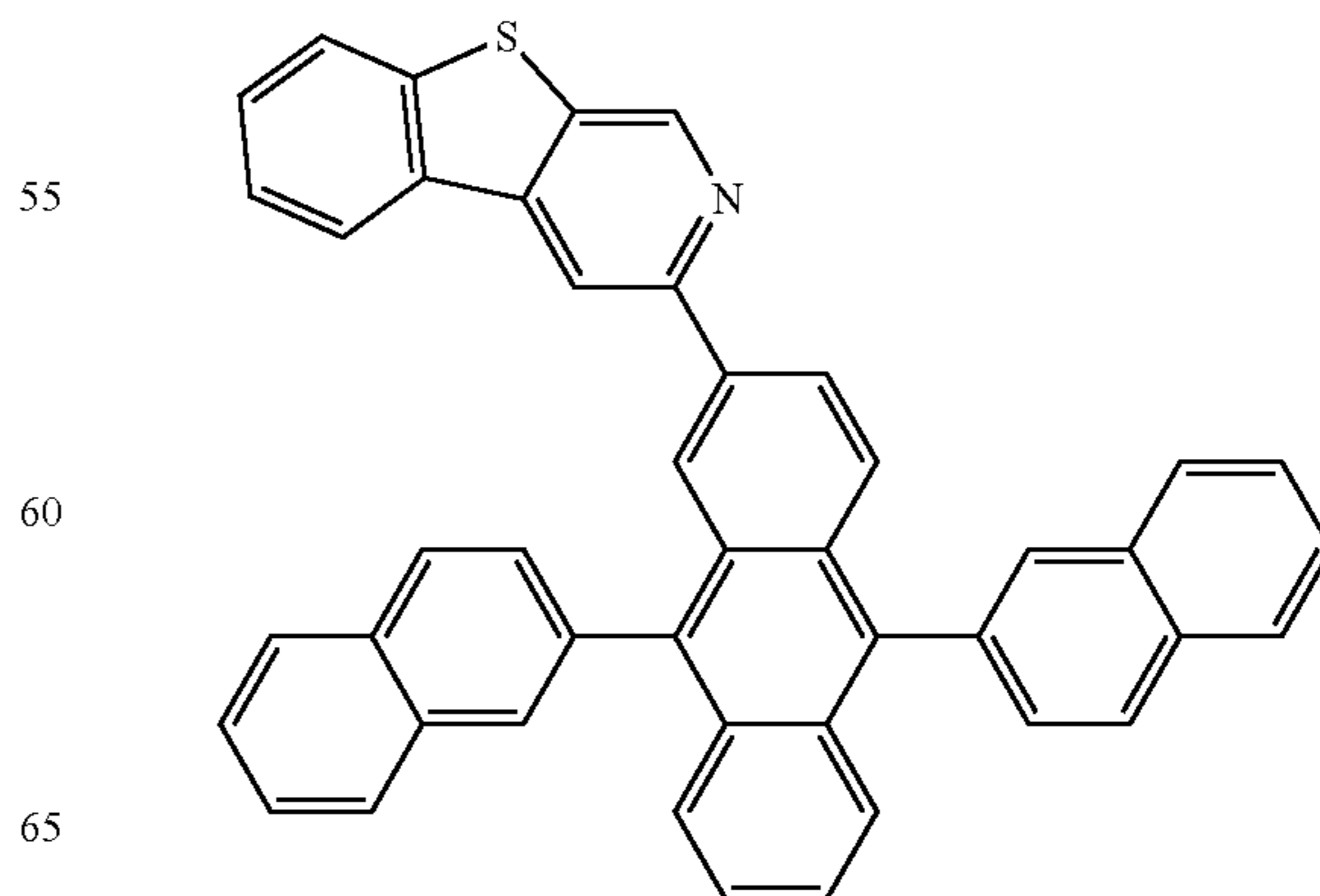
Compound 15
