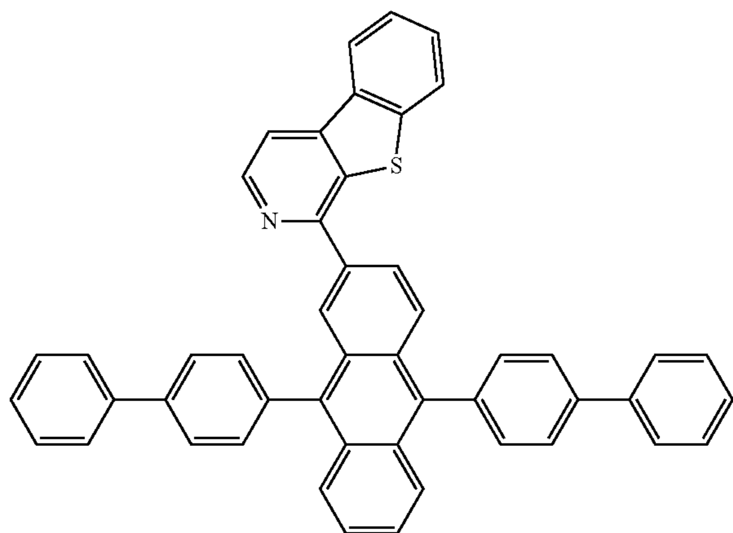
Compound 7
