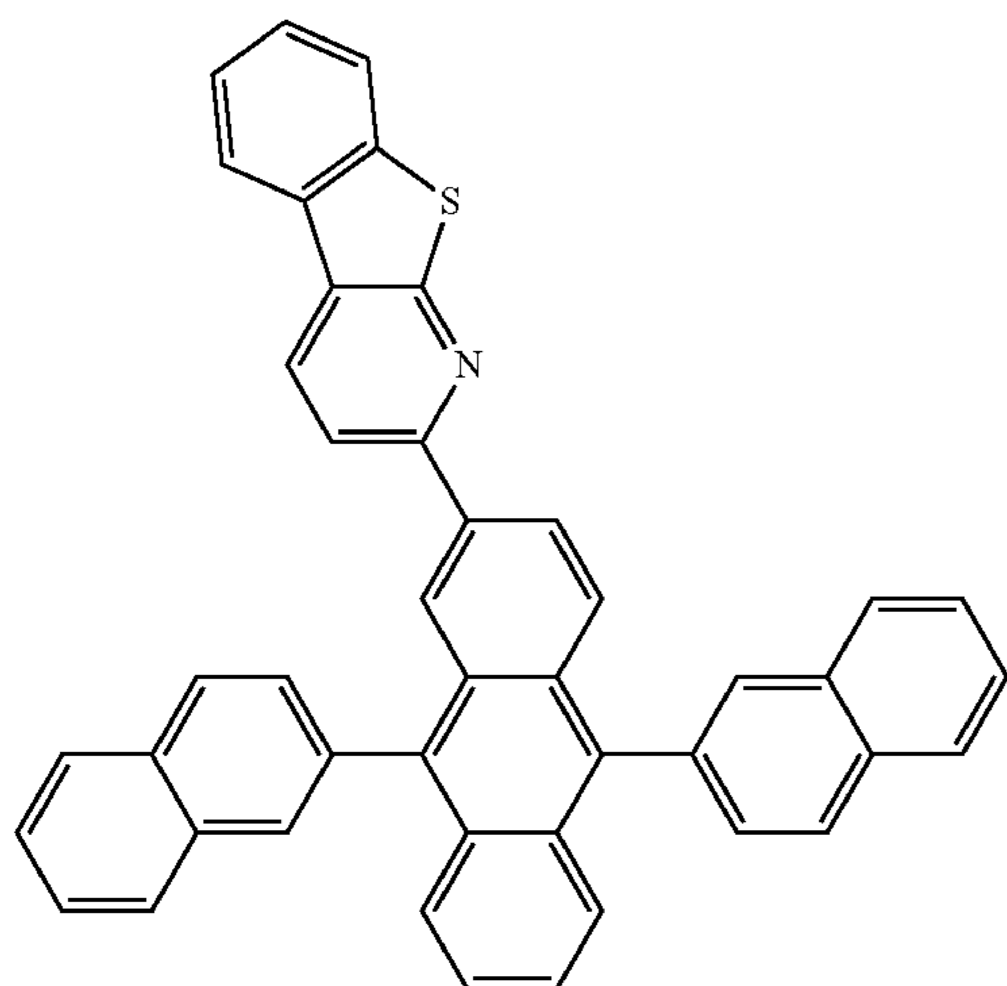
Compound 17
