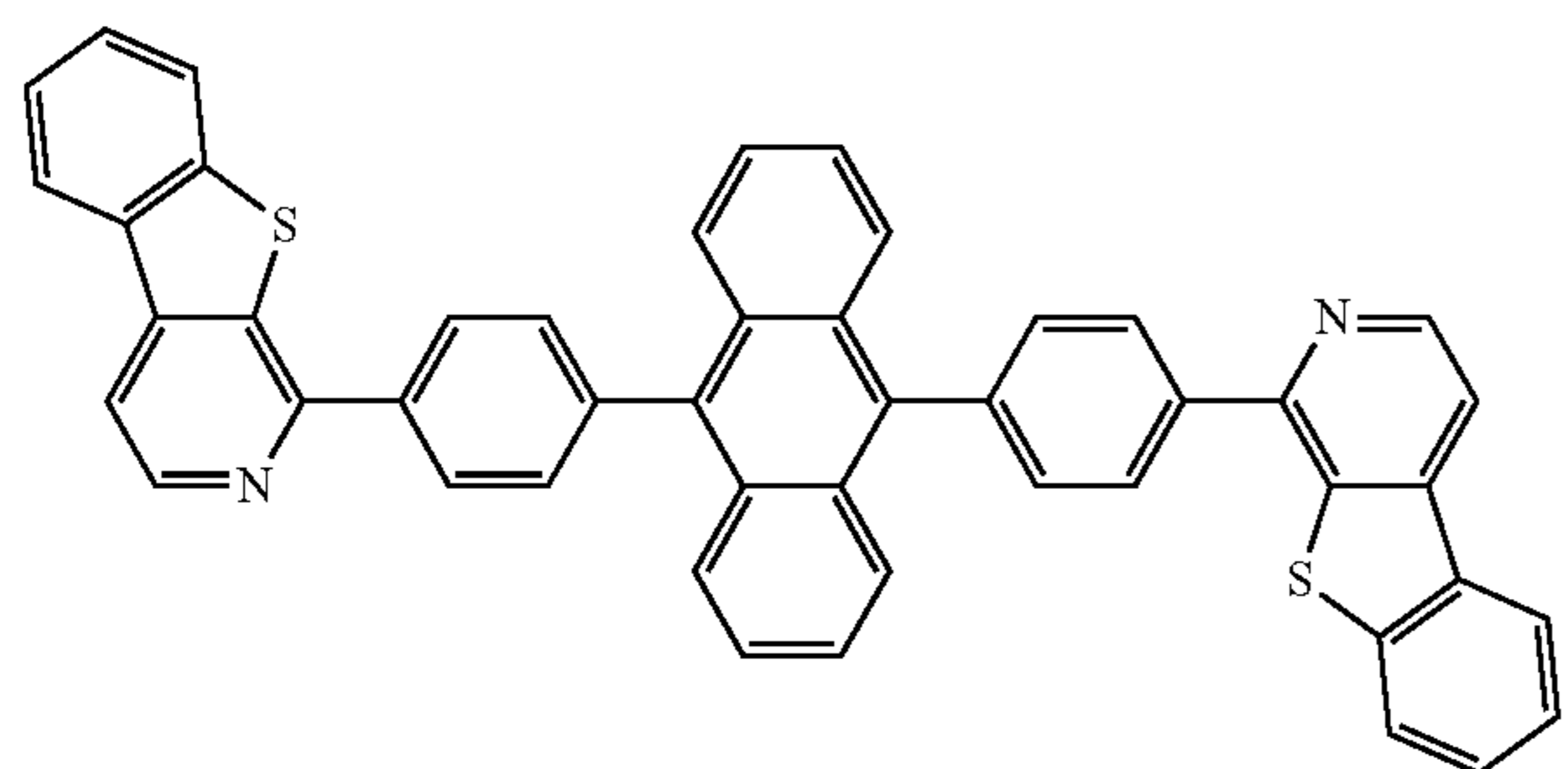
Compound 14
