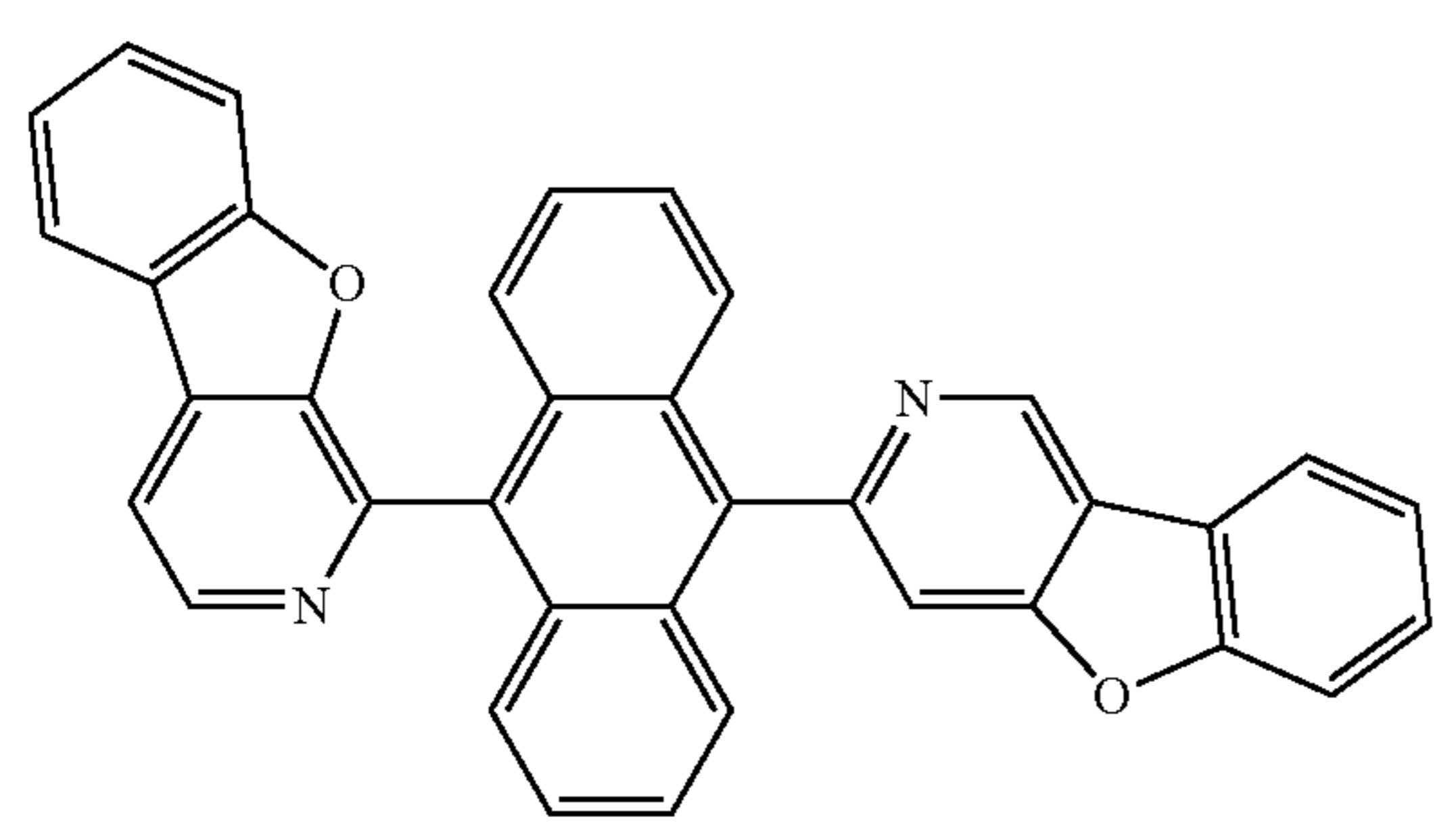
Compound 57
