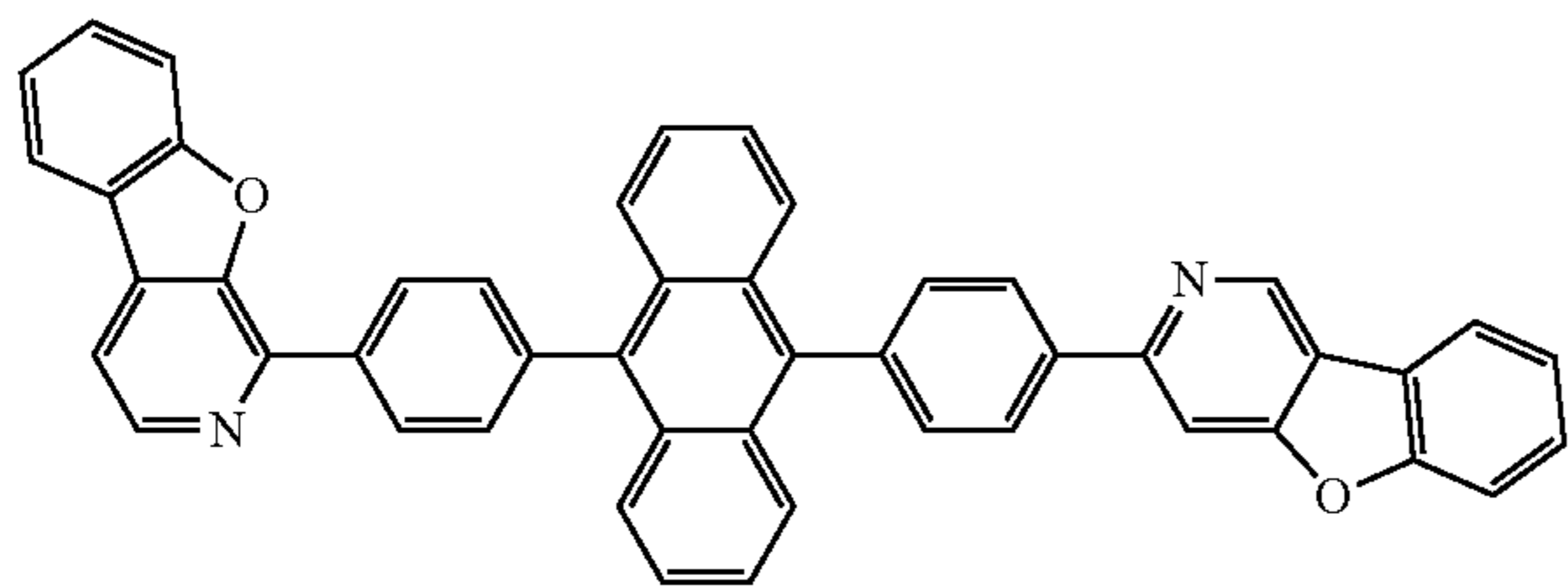
Compound 59
