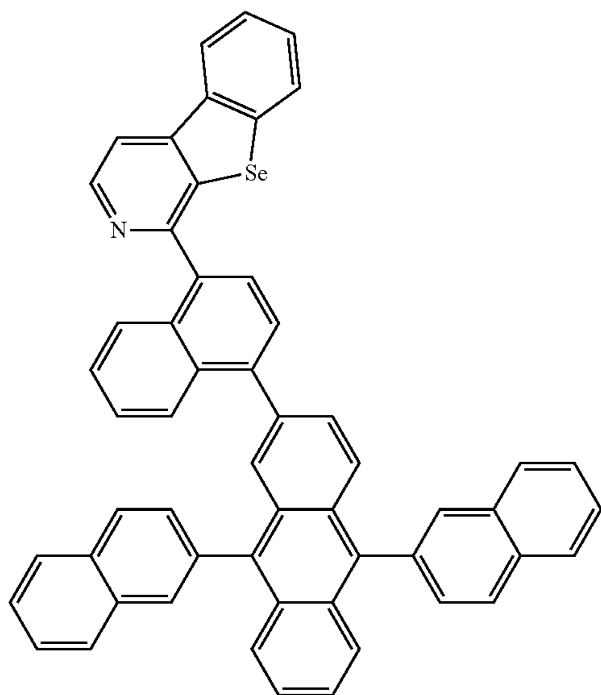
Compound 41
