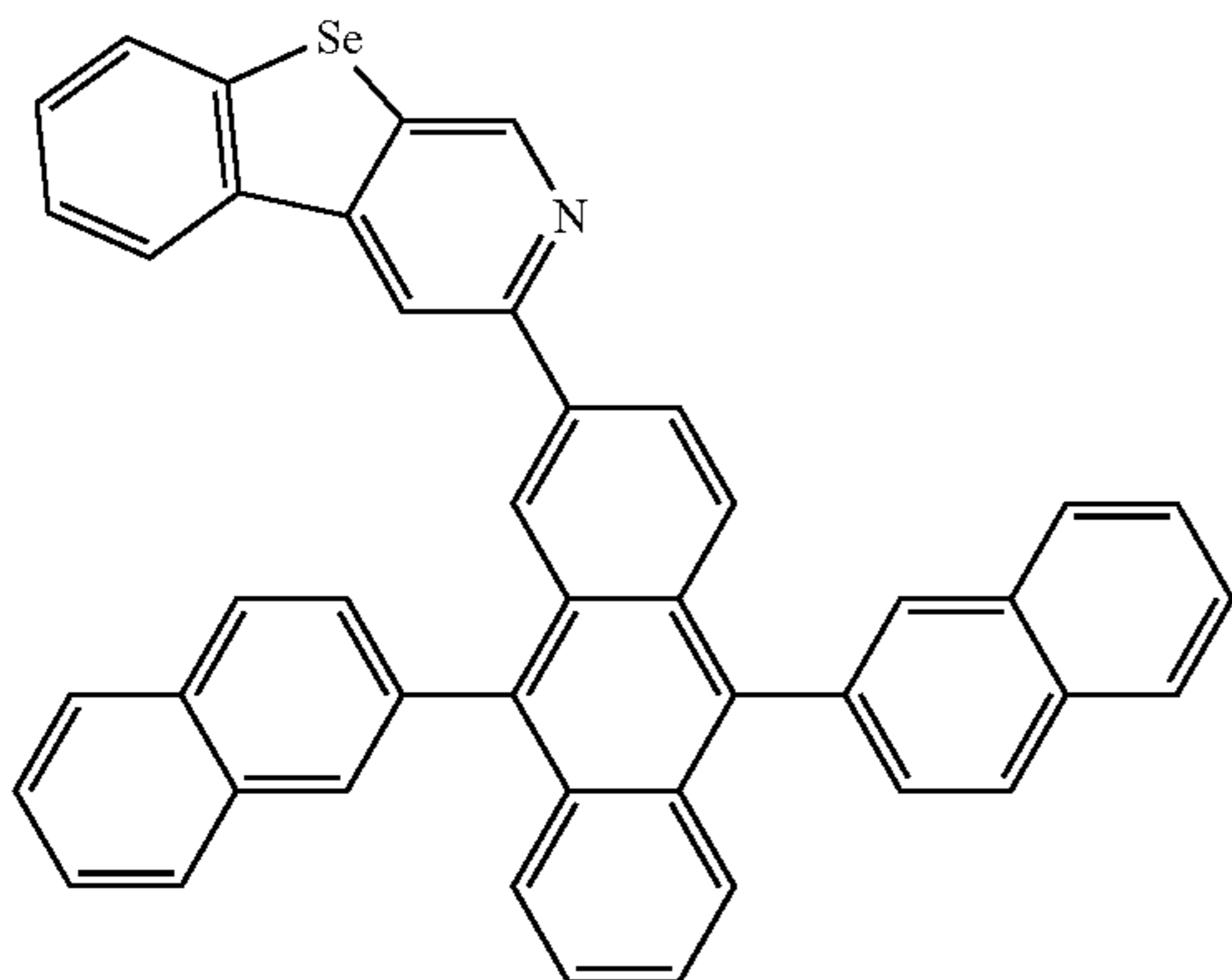
Compound 51
