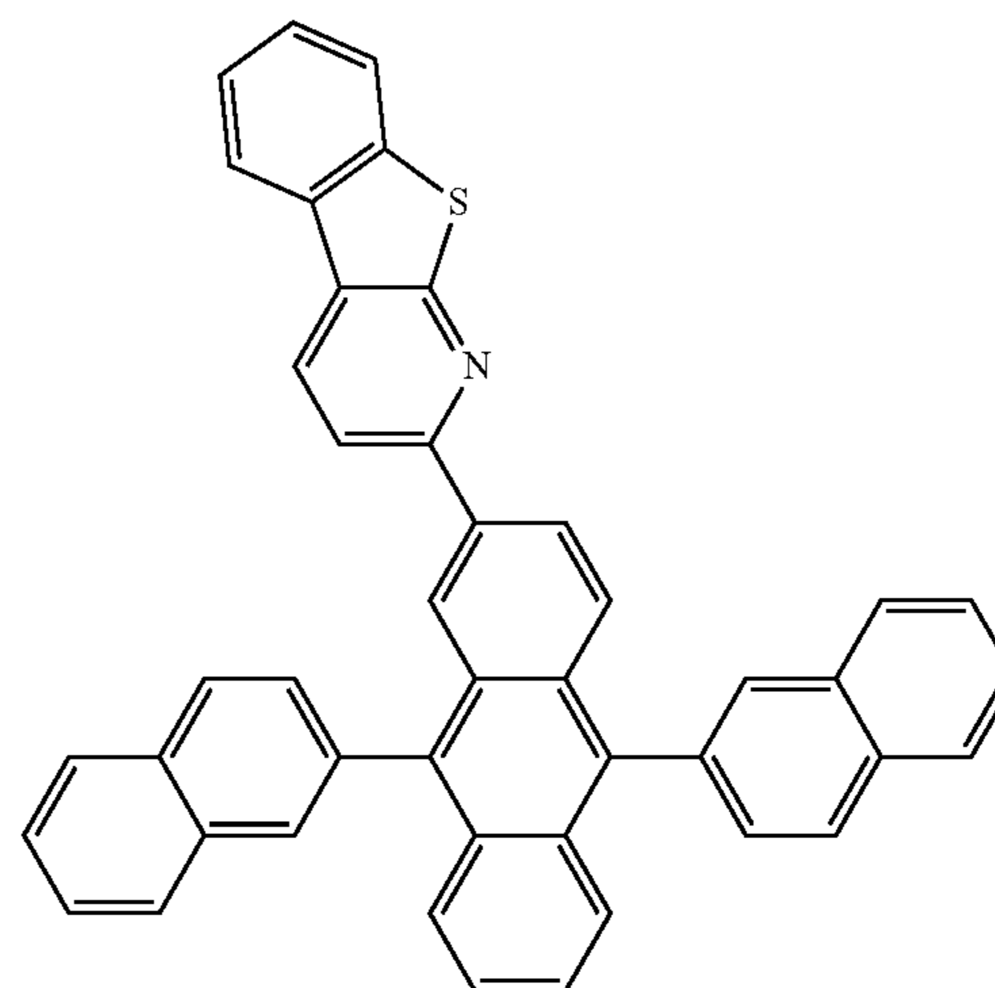
Compound 17
