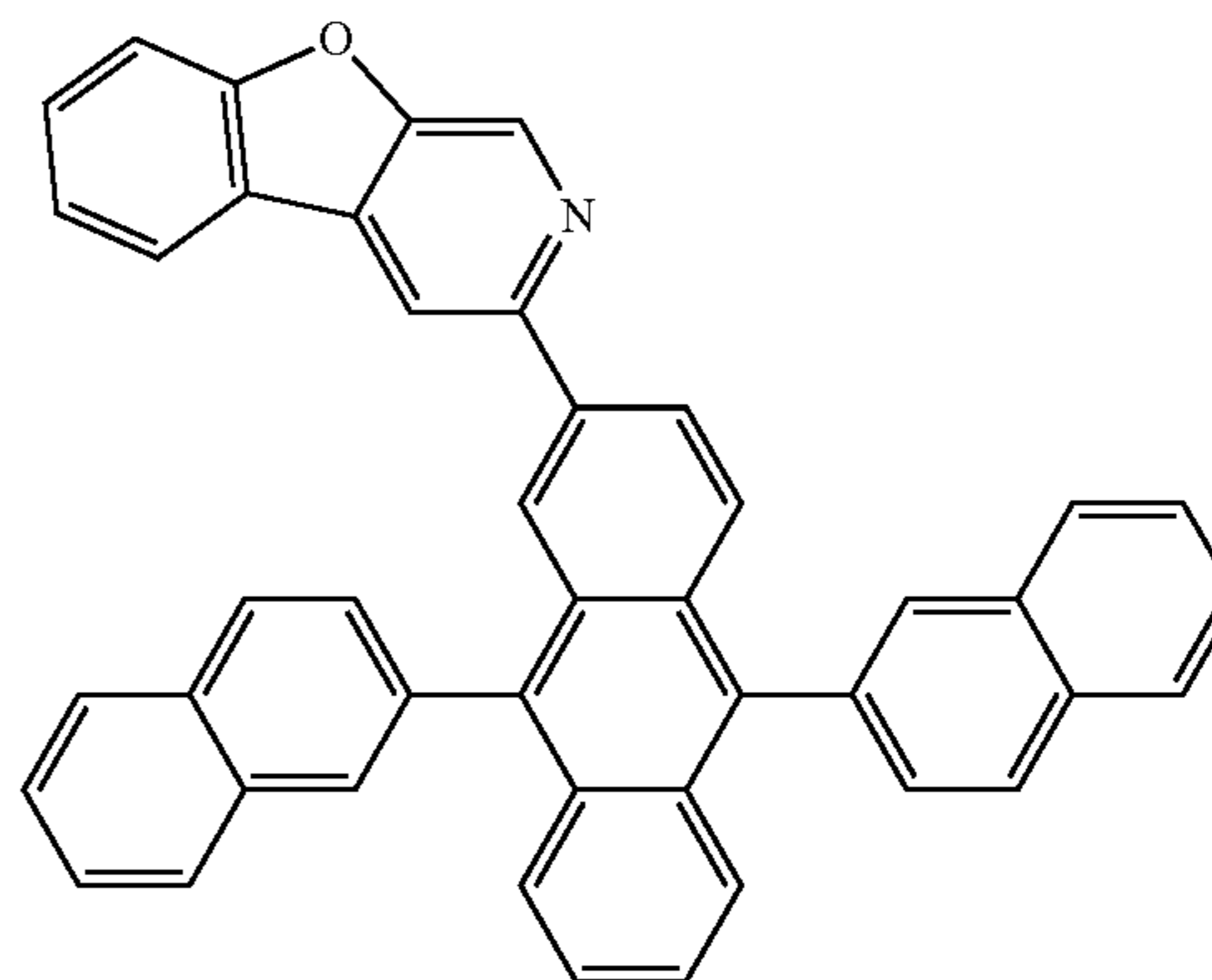
Compound 33
