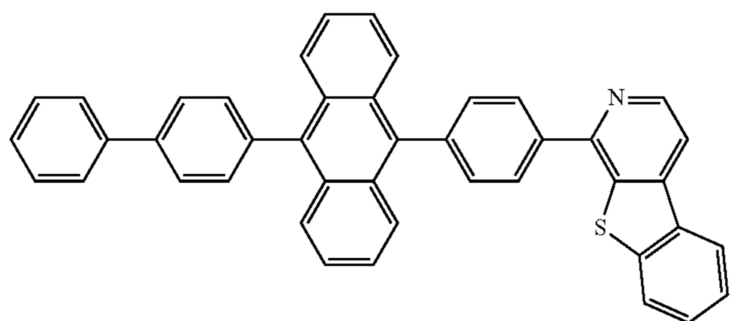
Compound 12
