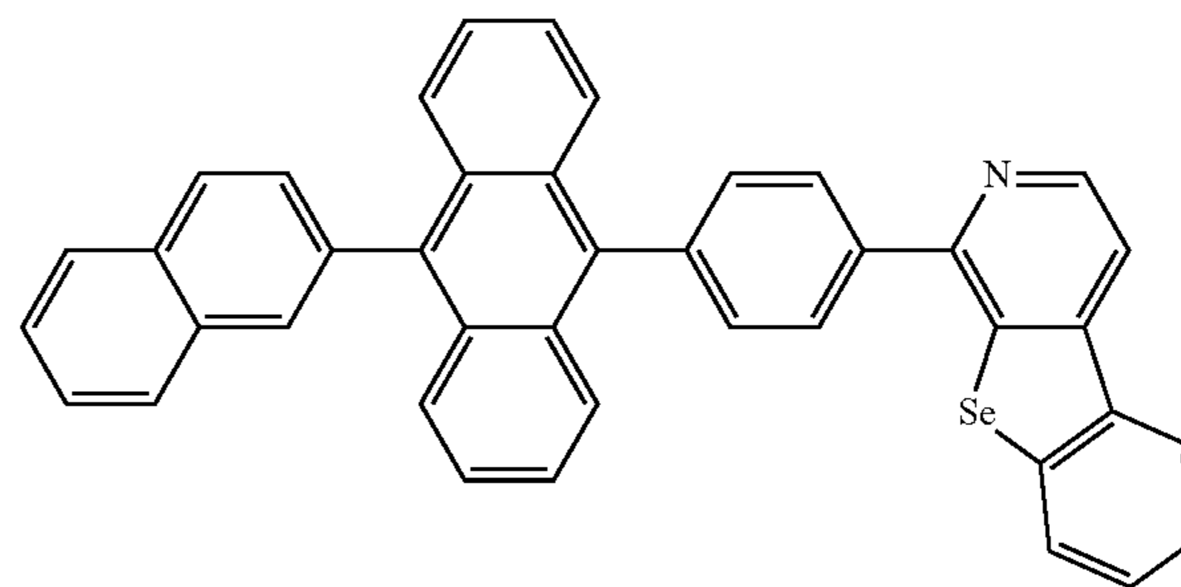
Compound 47
