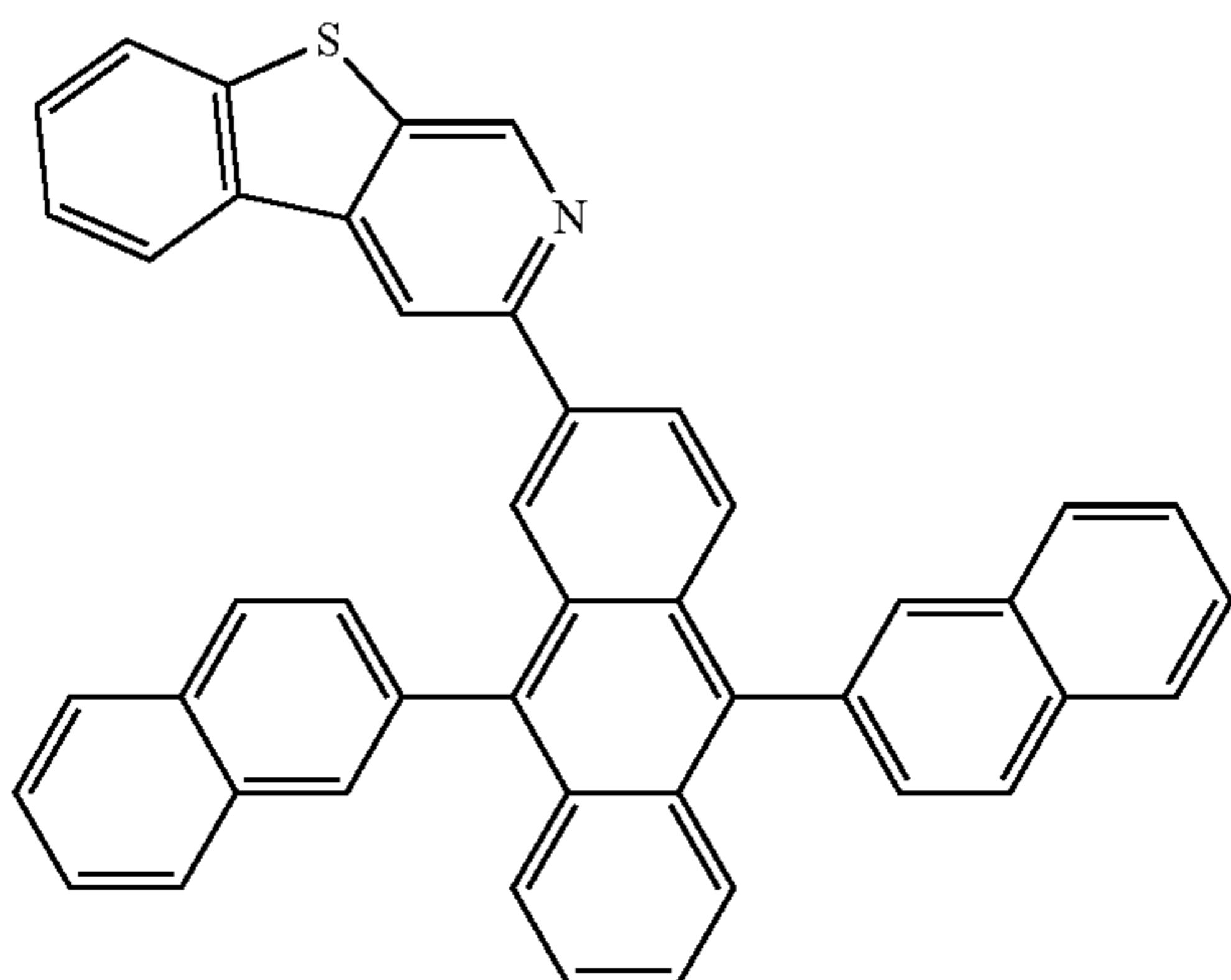
Compound 15
