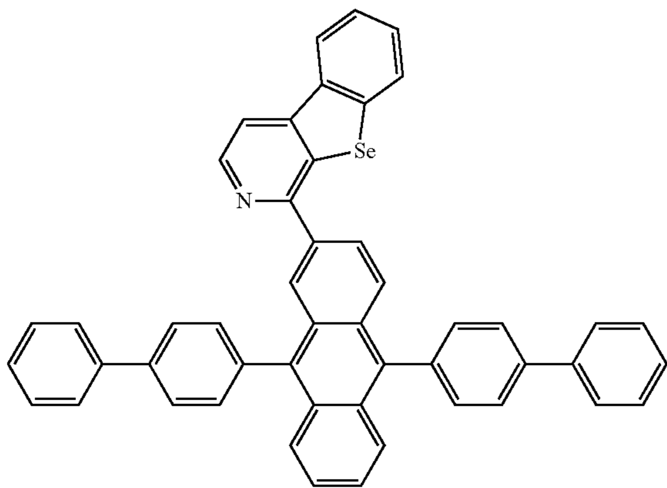
Compound 43
