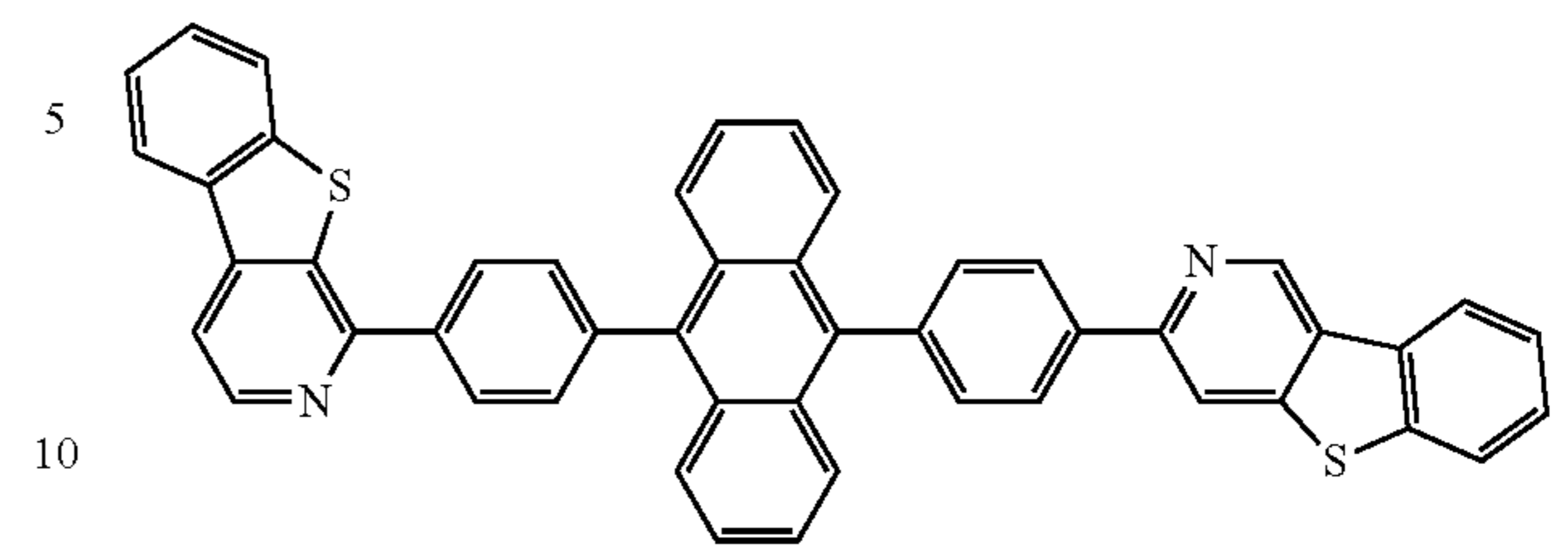
Compound 58
