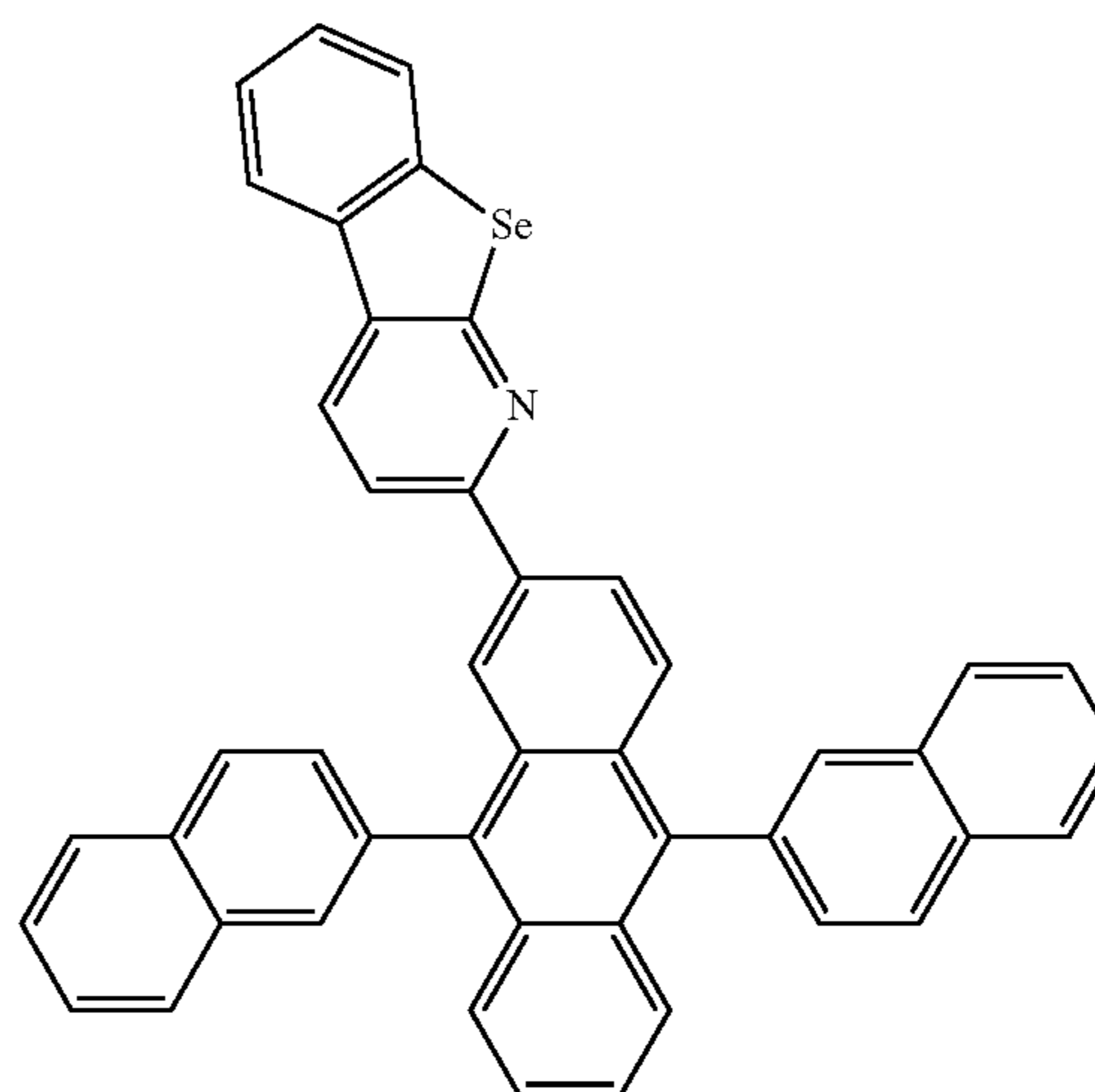
Compound 53
