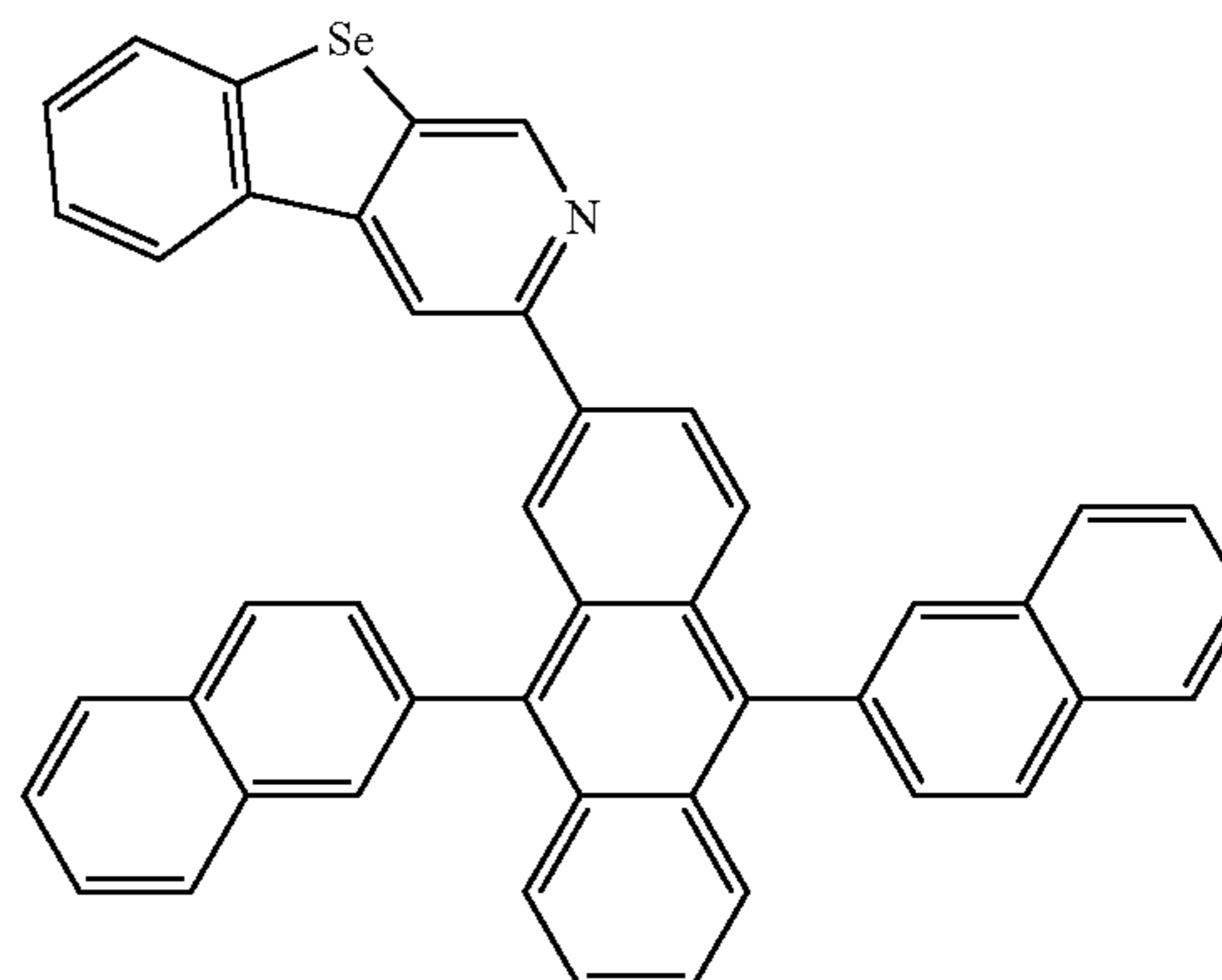
Compound 51
