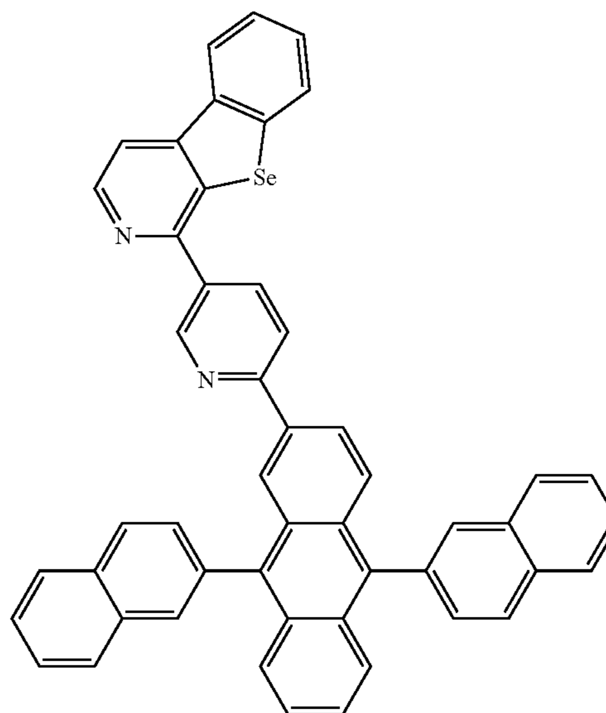
Compound 39
