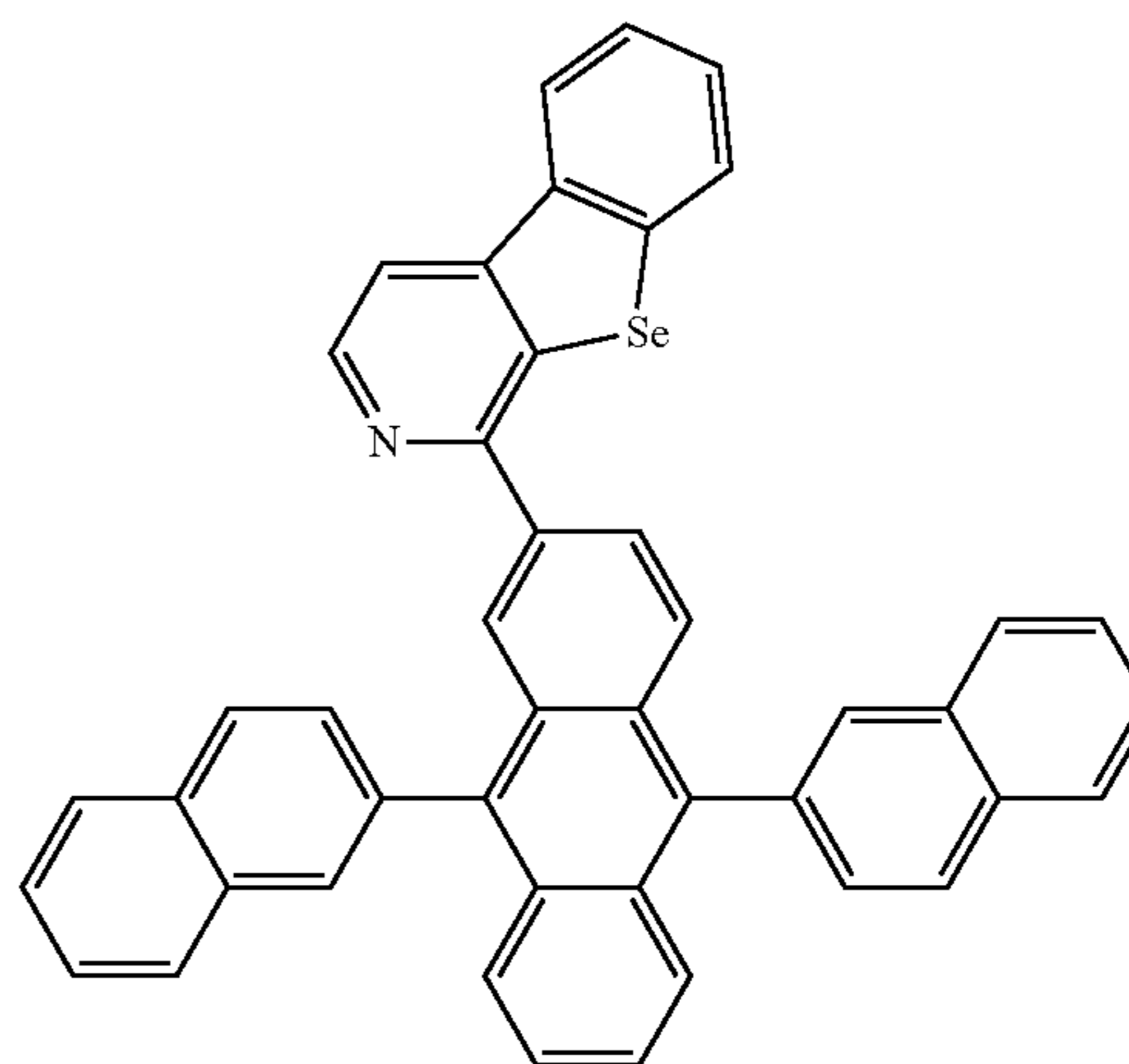
Compound 38
