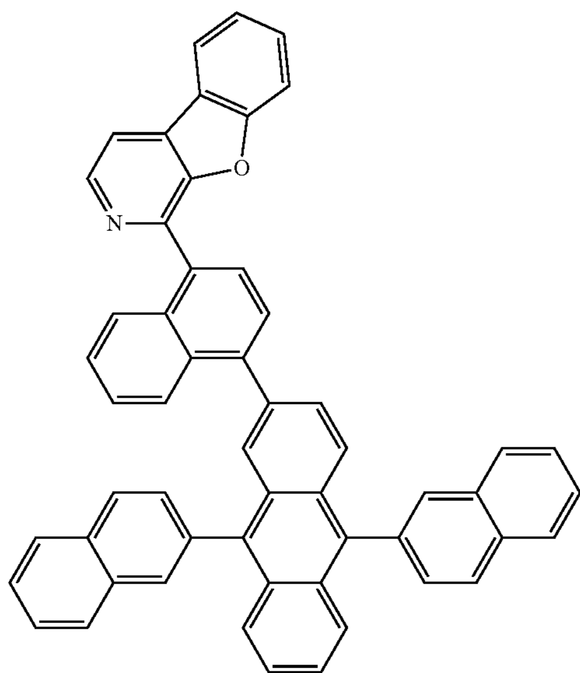
Compound 23
