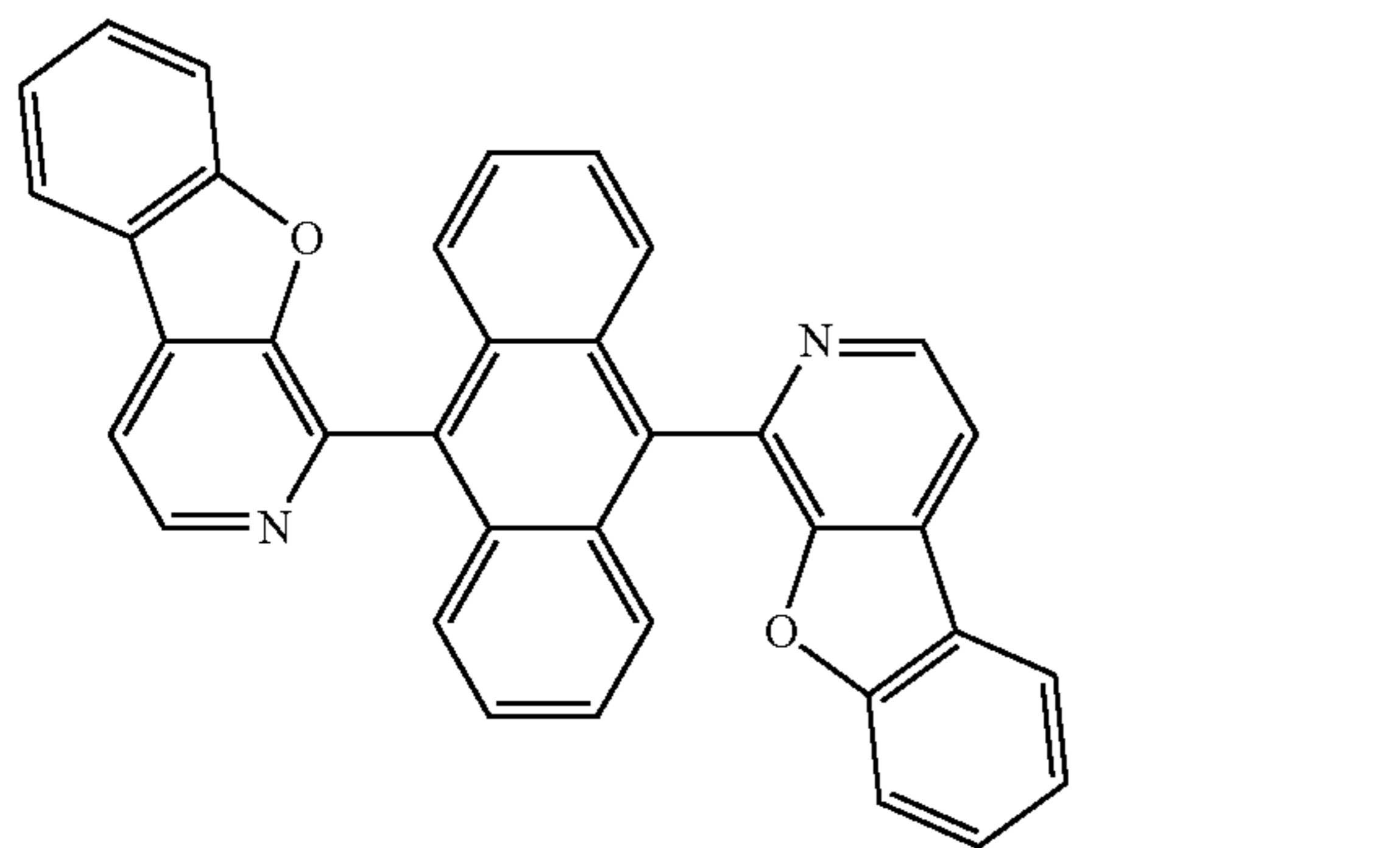
Compound 31
