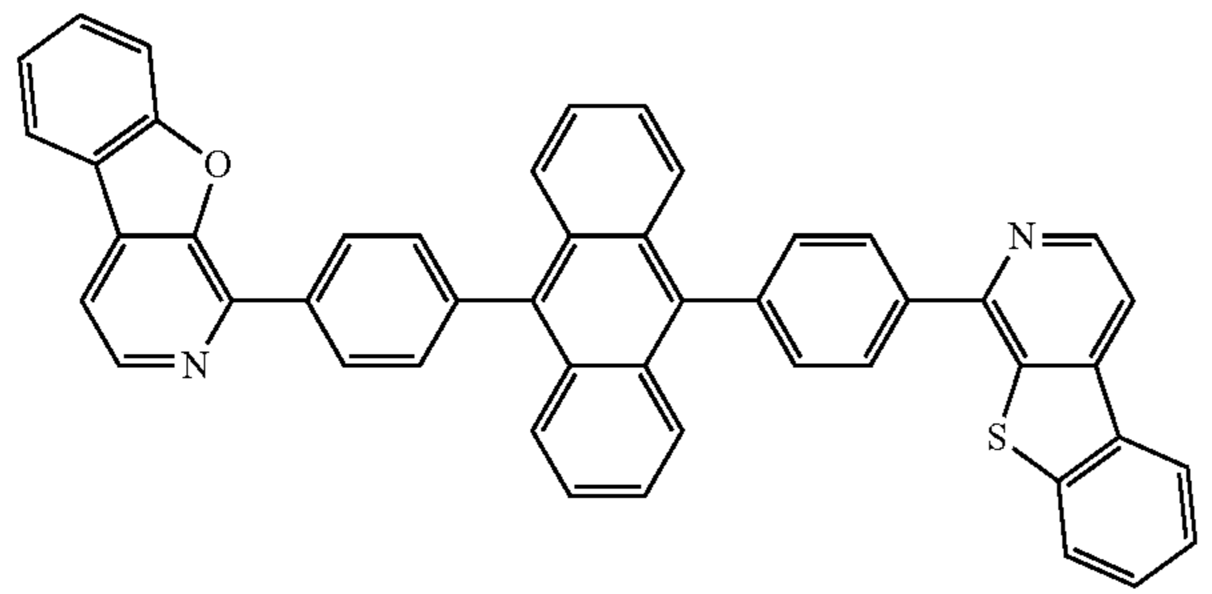
Compound 56
