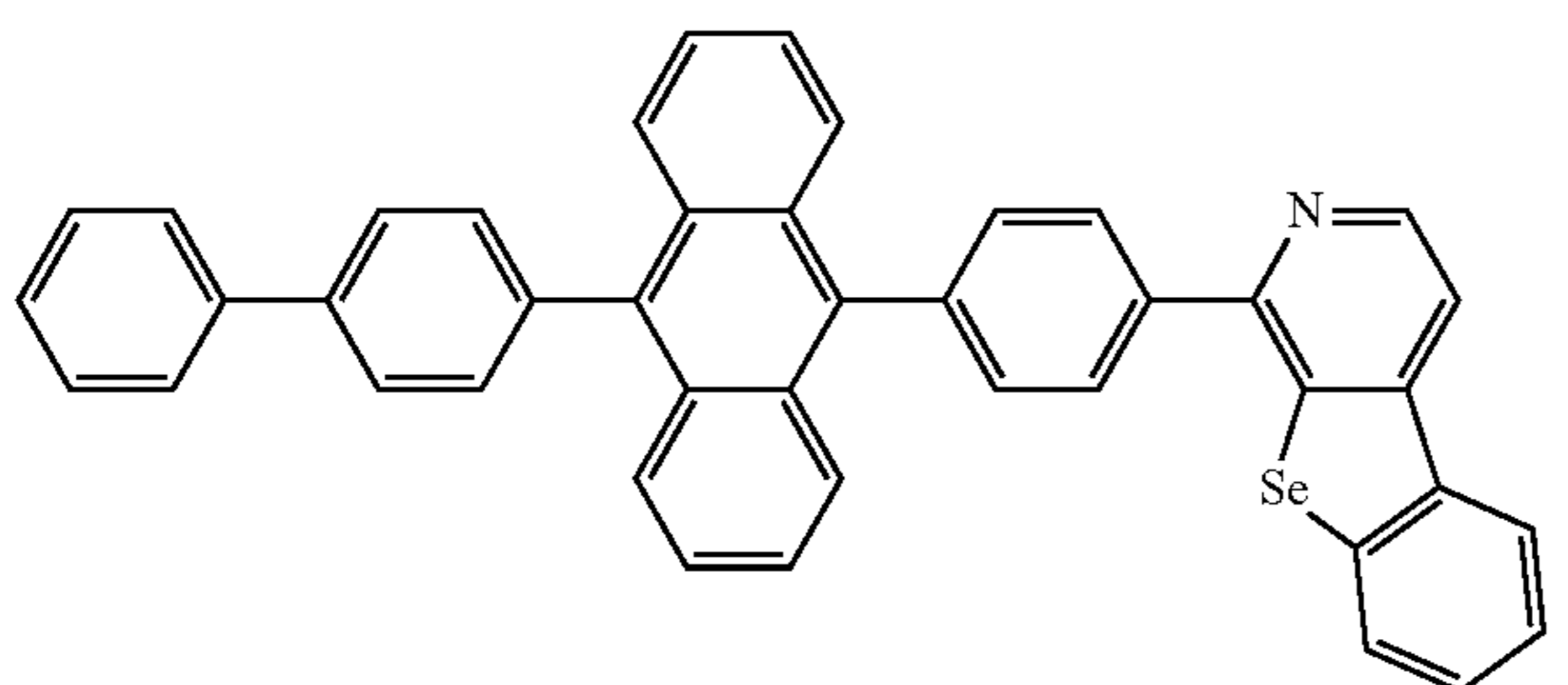
Compound 49
