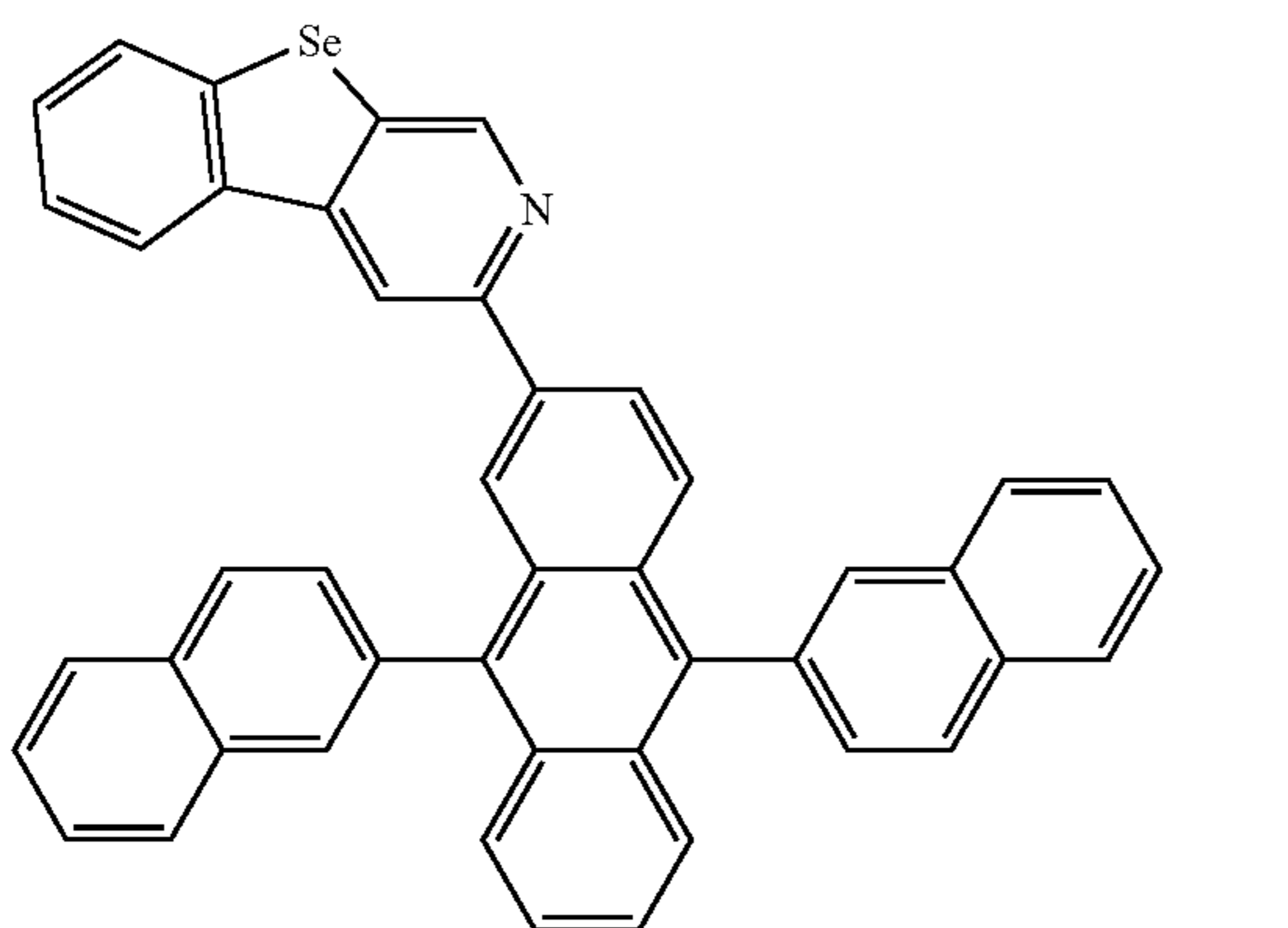
Compound 51
