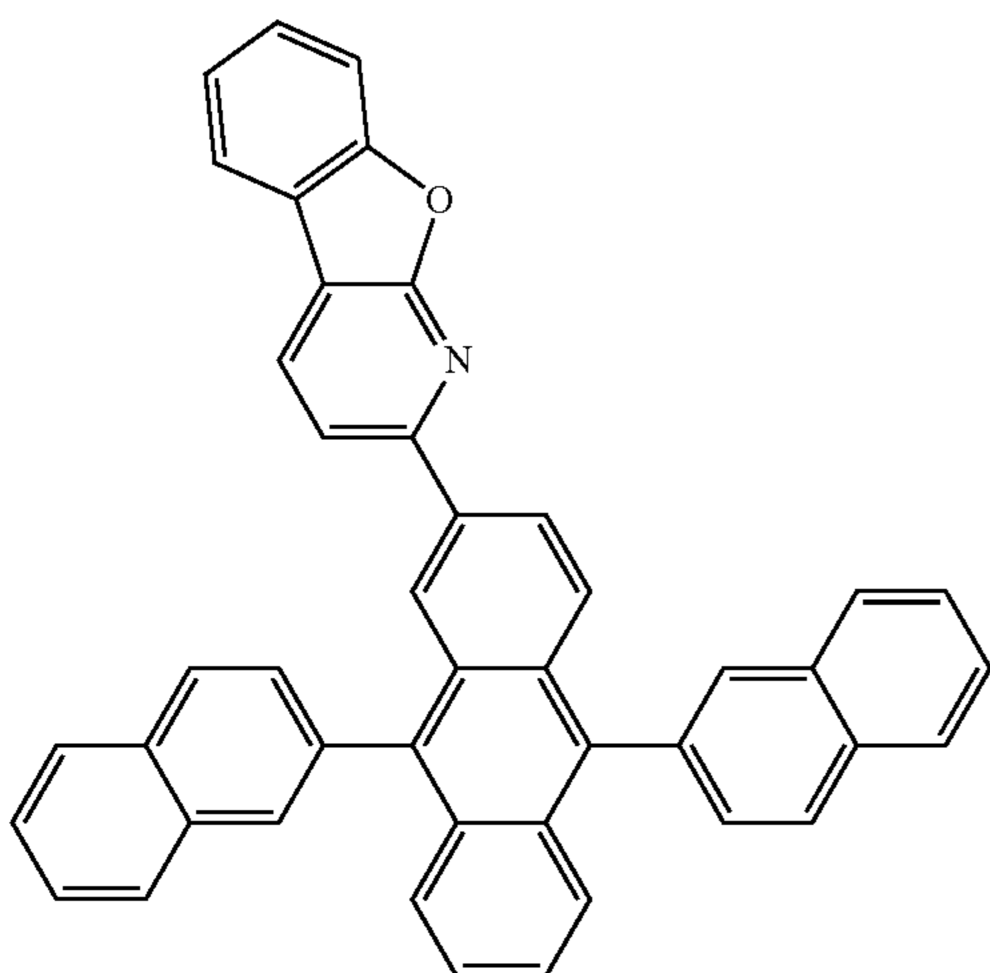
Compound 35
