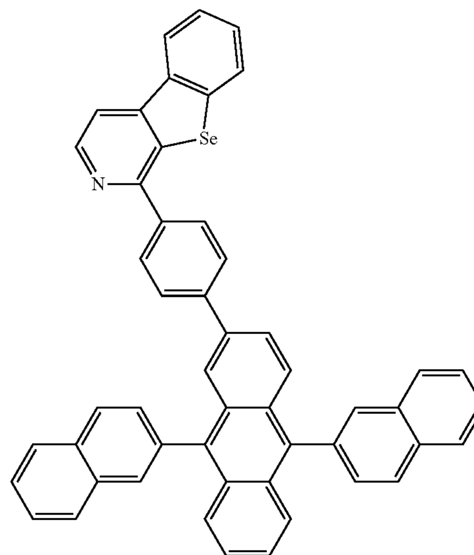
Compound 39
