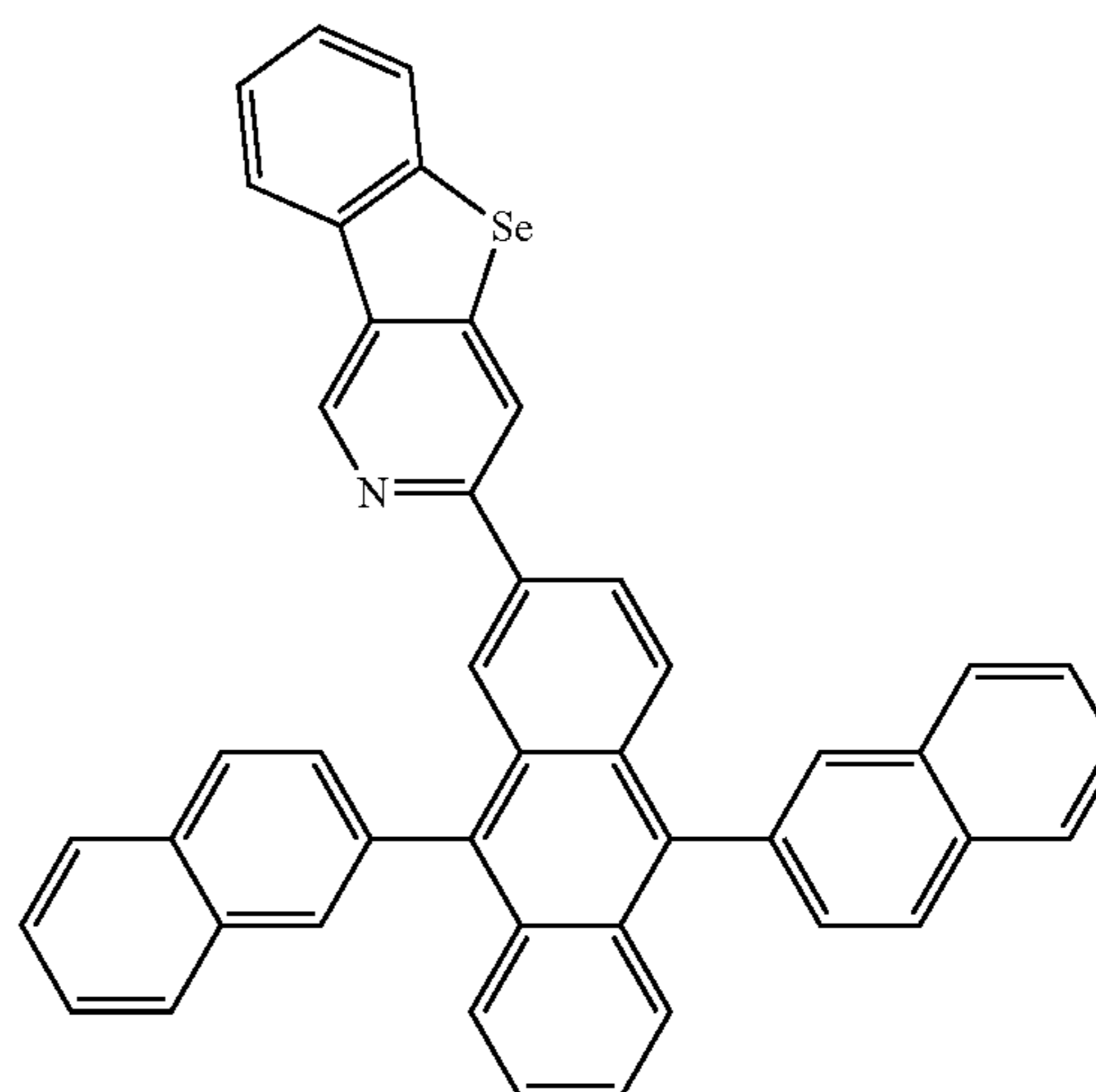
Compound 54
