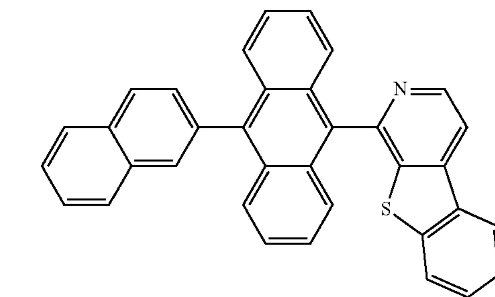
Compound 11
