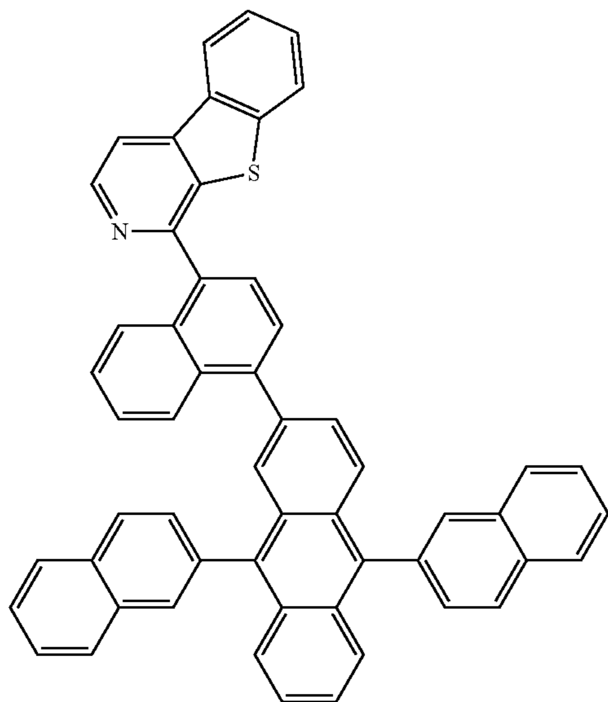
Compound 4
