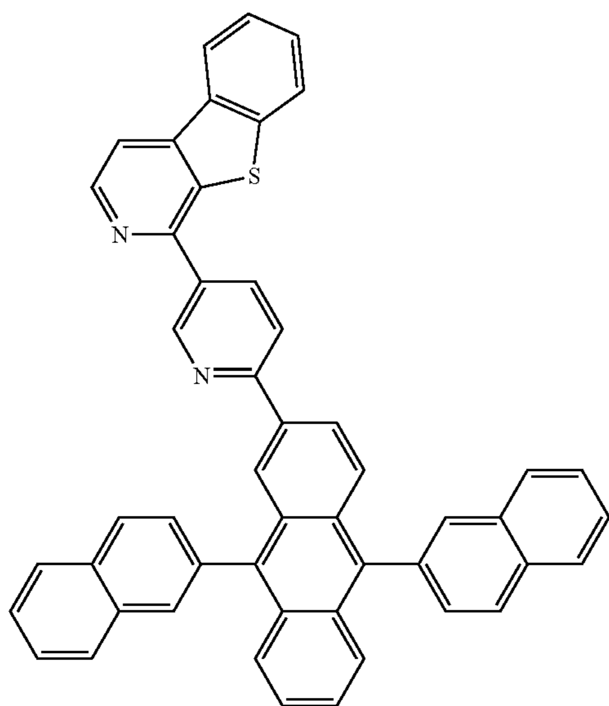
Compound 3 5
