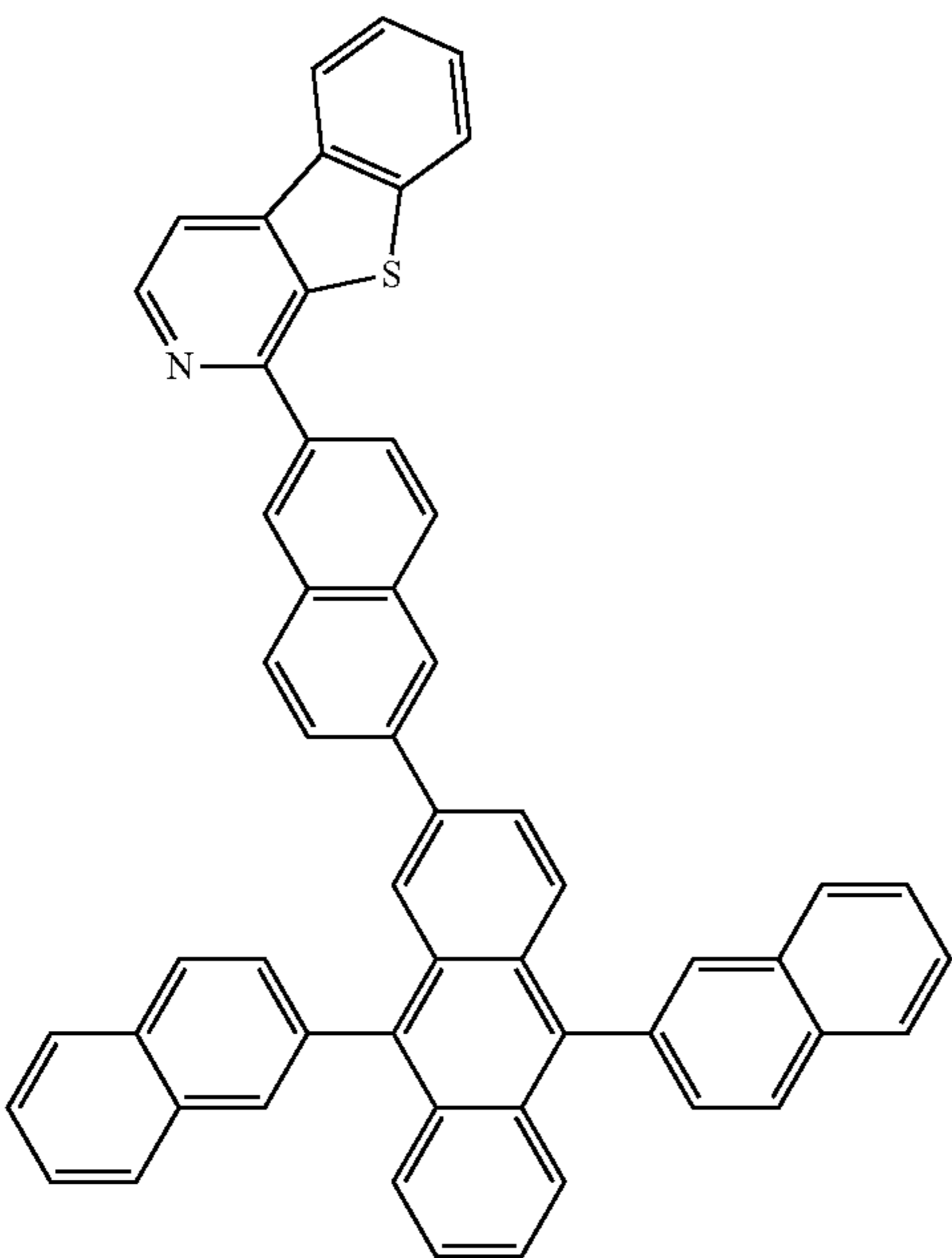
Compound 6
