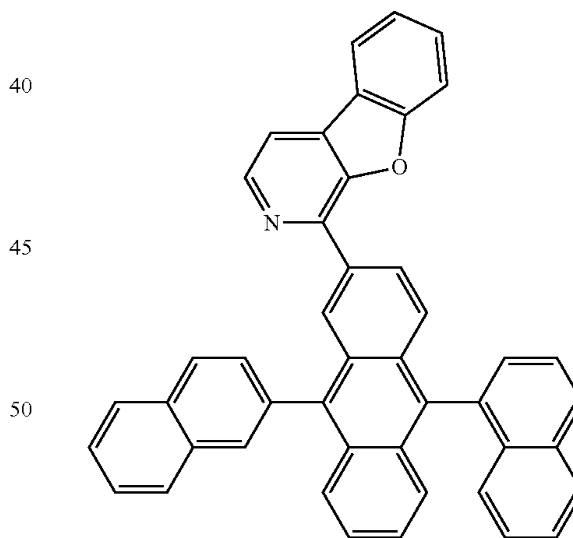
Compound 24
