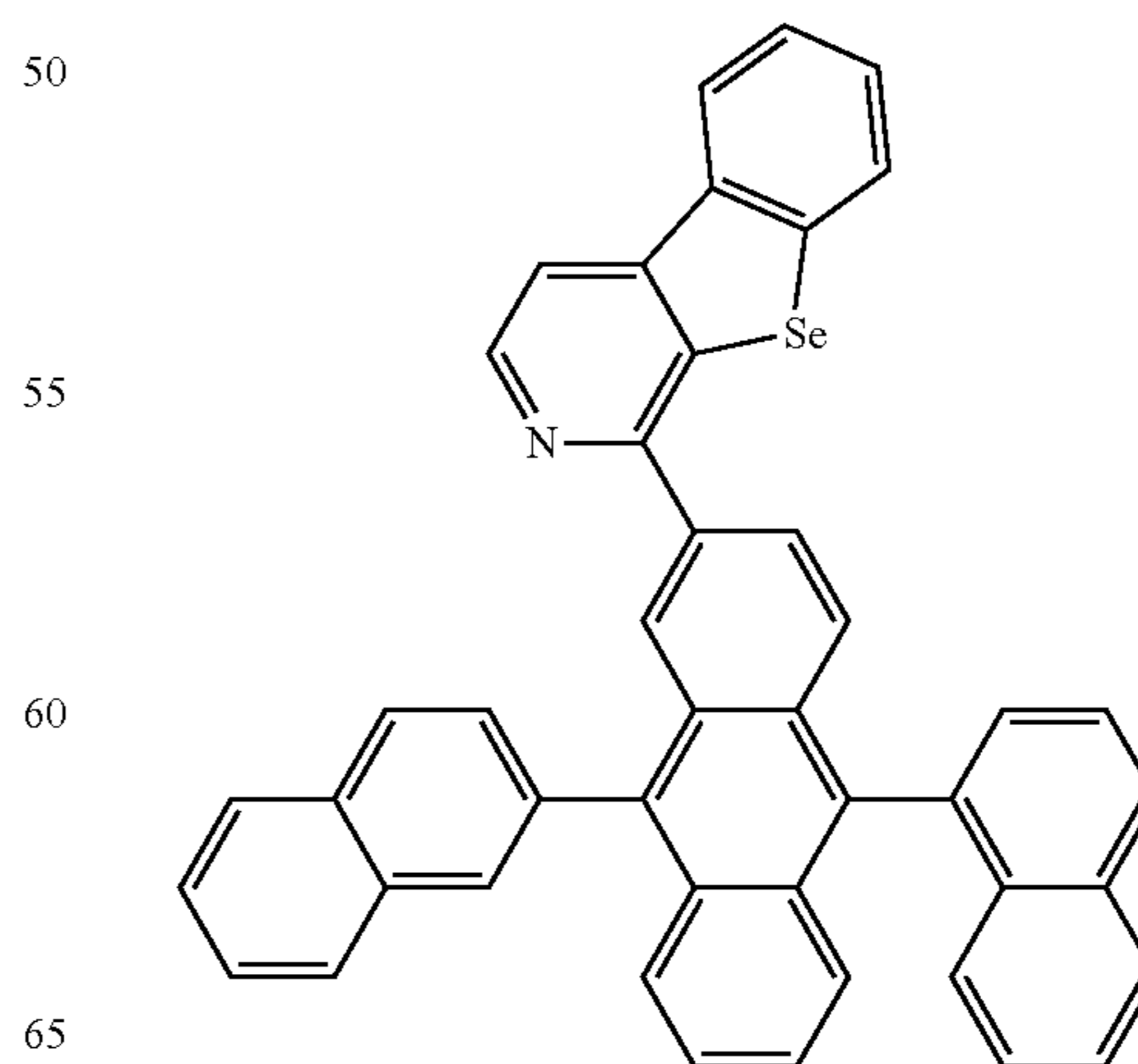
Compound 42
