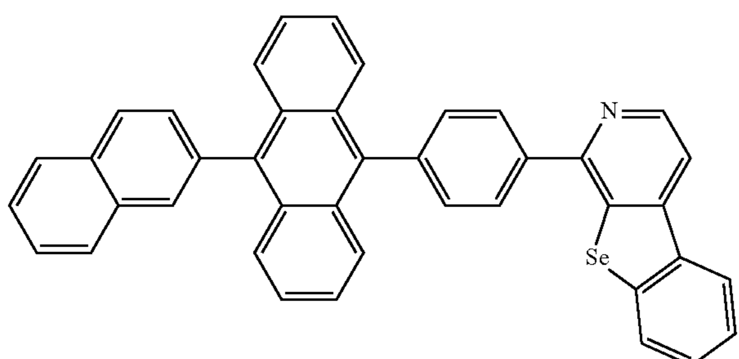
Compound 48
