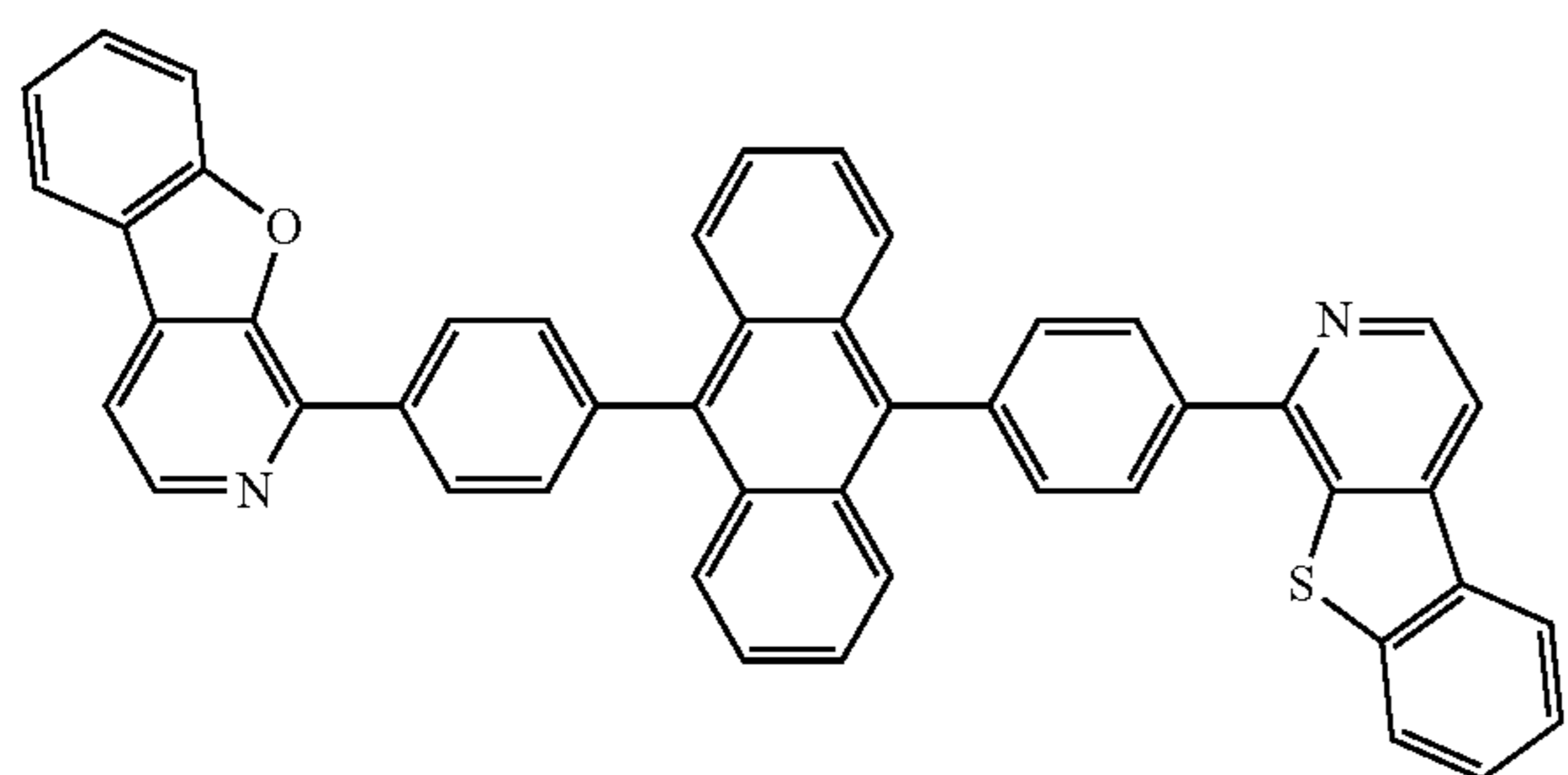
Compound 56
