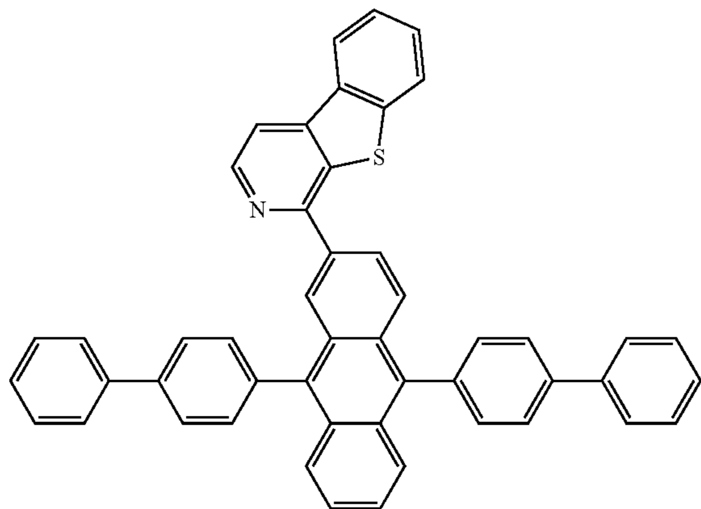
Compound 7
