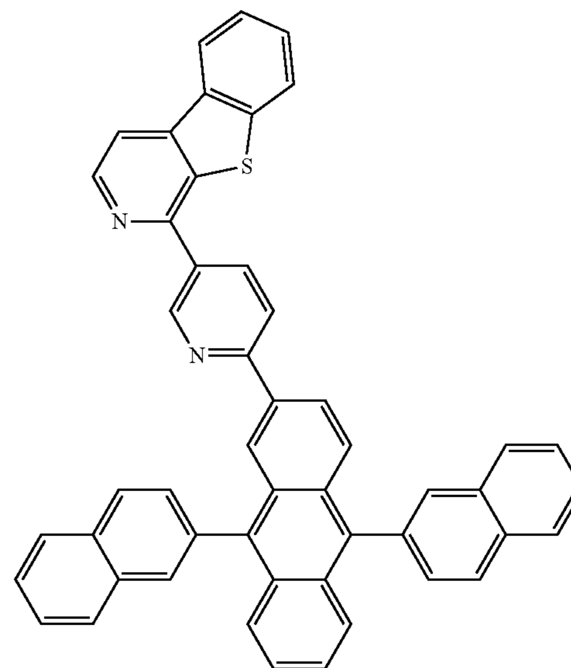
Compound 3
