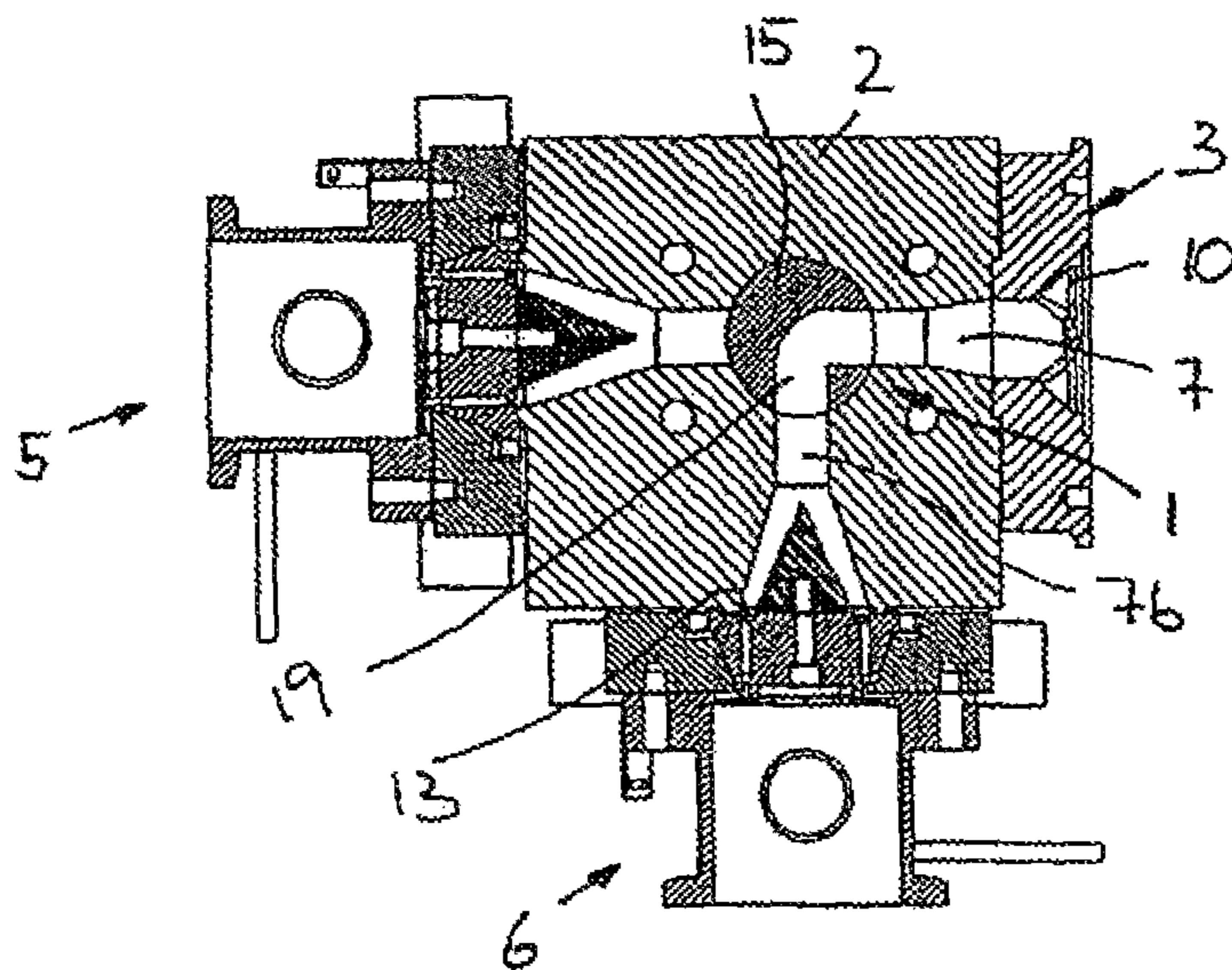
SECTIONAL REPRESENTATION C-C Fig. 17
