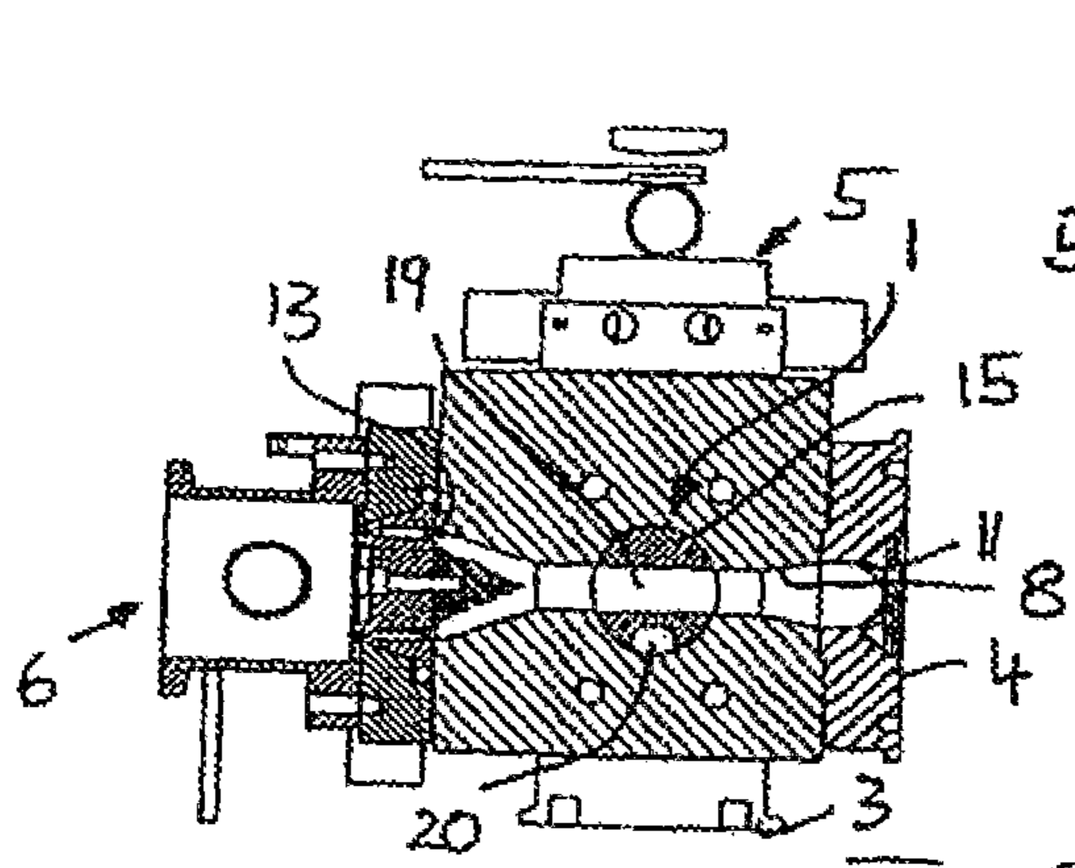
SECTIONAL REPRESENTATION B-B
