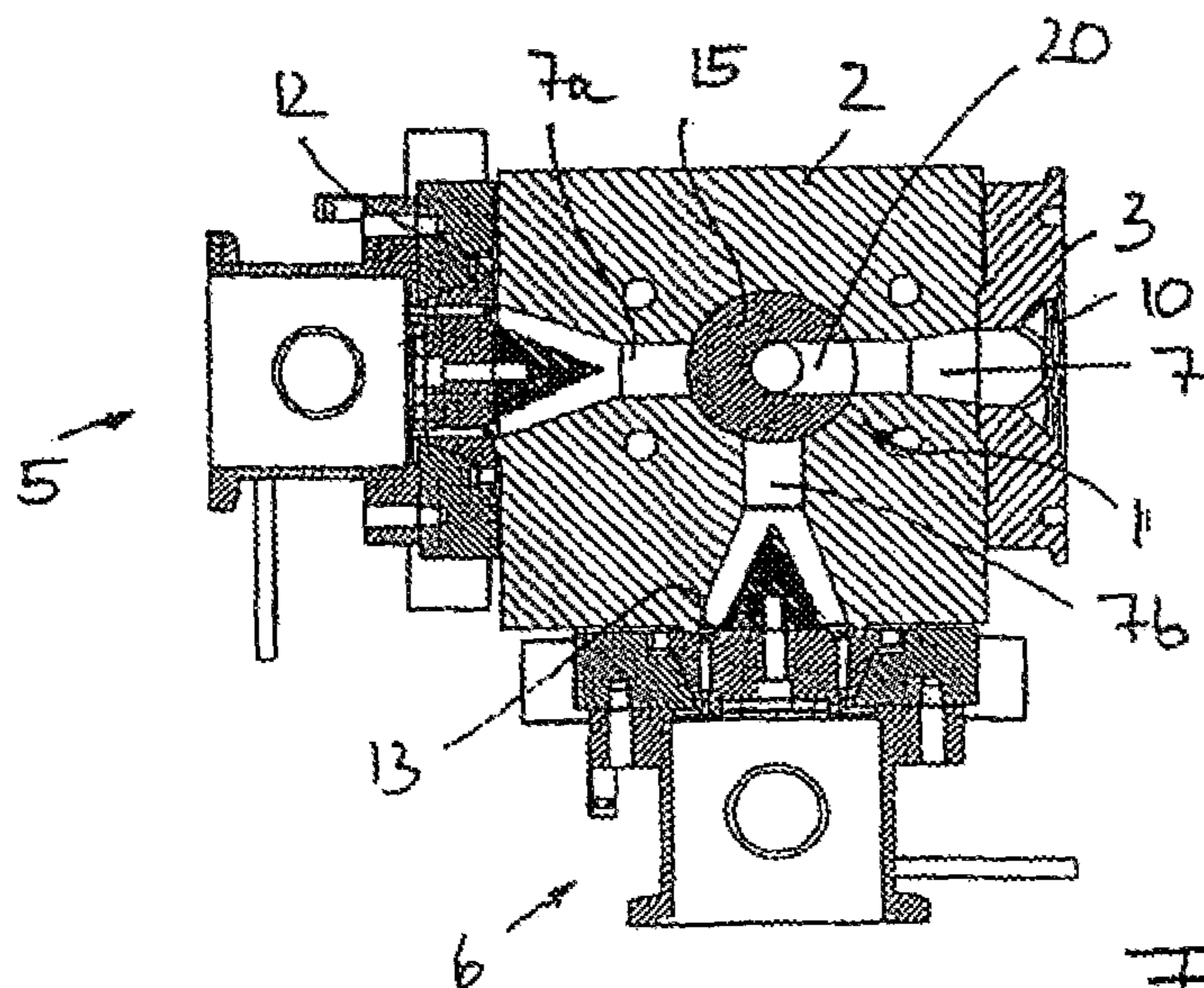
SECTIONAL REPRESENTATION A-A
