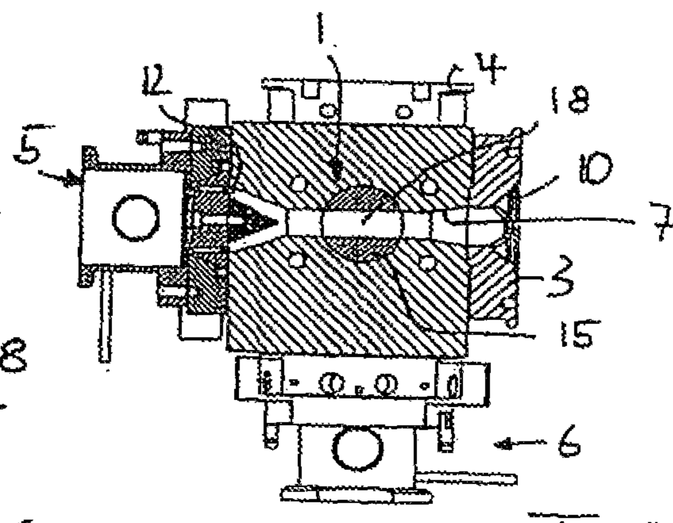
SECTIONAL REPRESENTATION A-A
