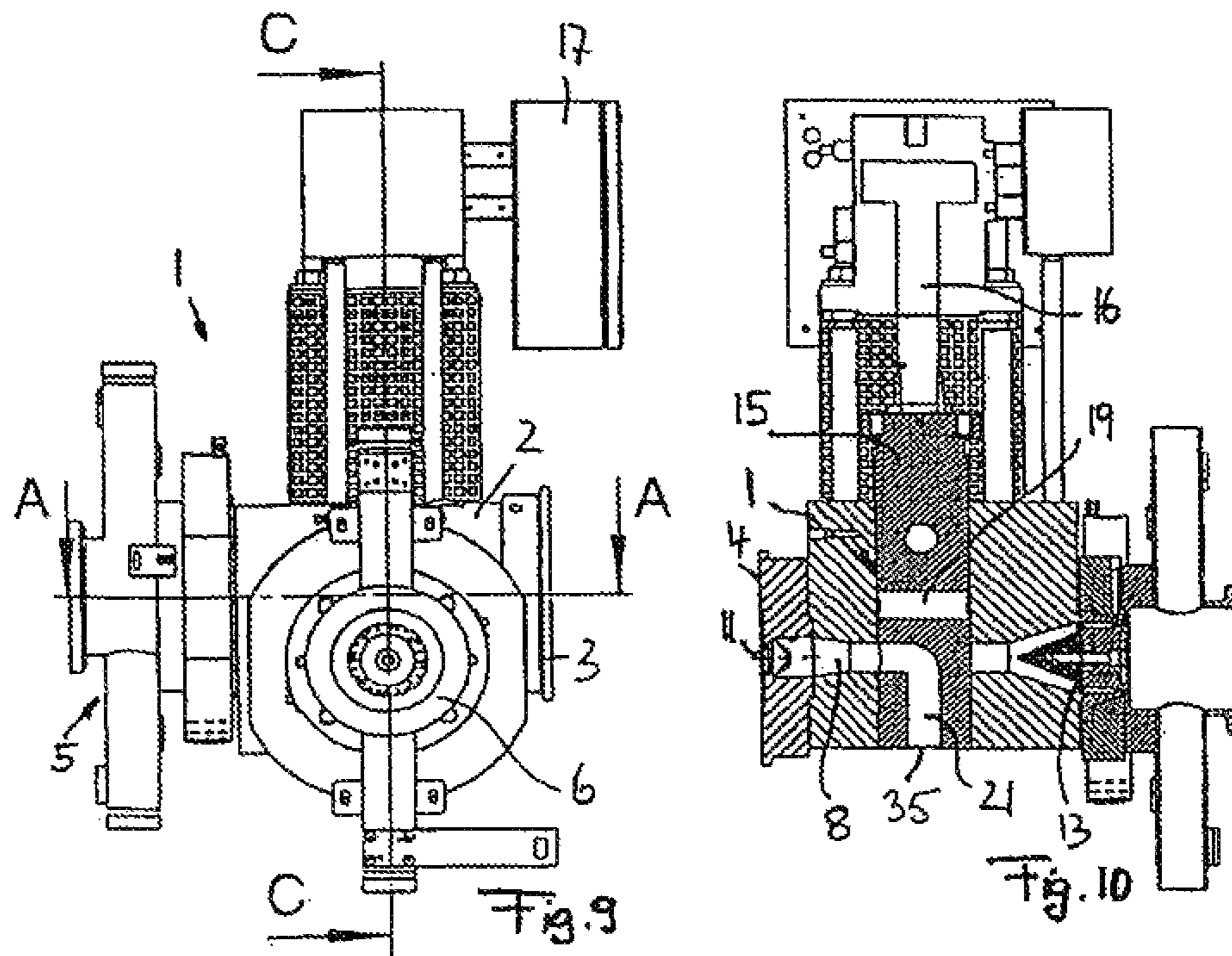
SECTIONAL REPRESENTATION C-C
