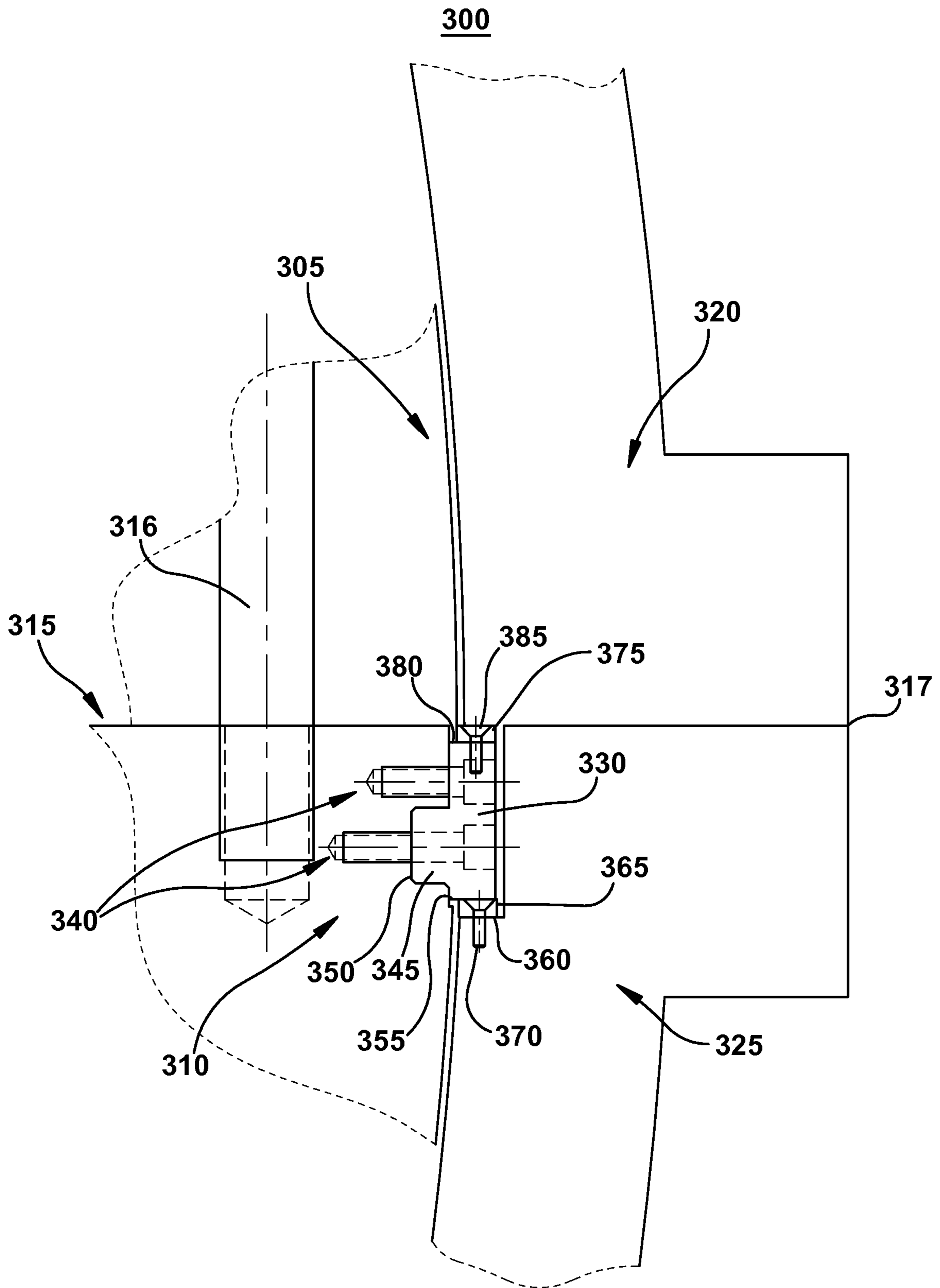
FIG. 3 (Prior Art)
