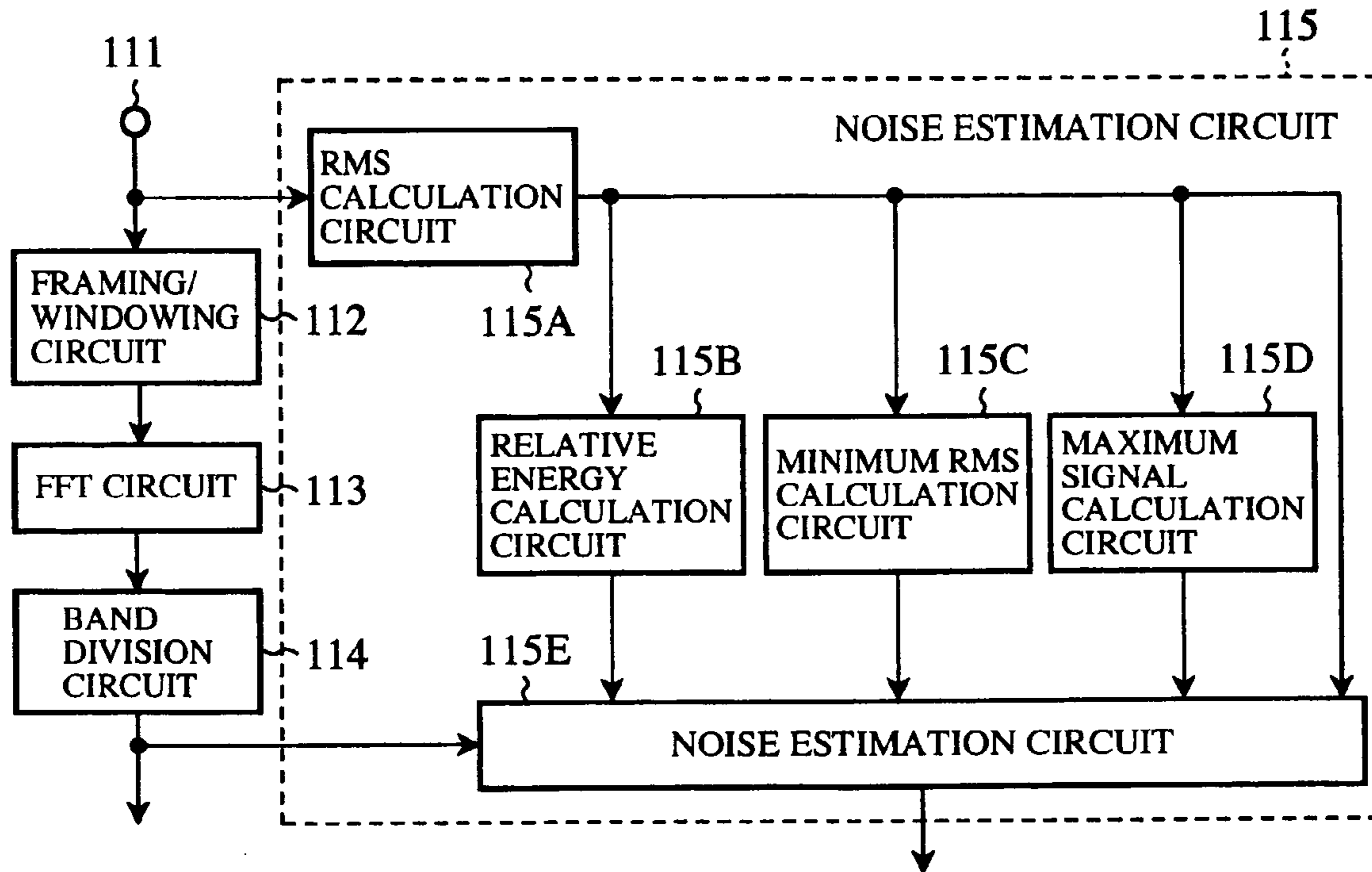
FIG.2 BACKGROUND ART
