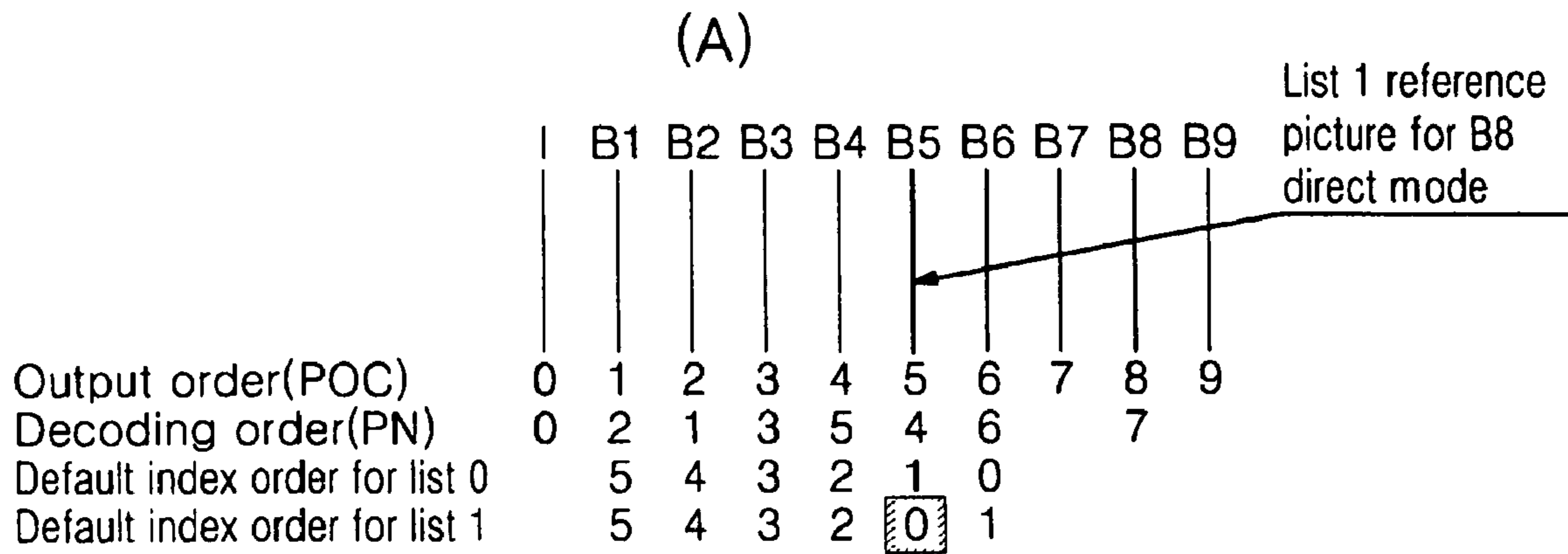
FIG. 2 (Related Art)
