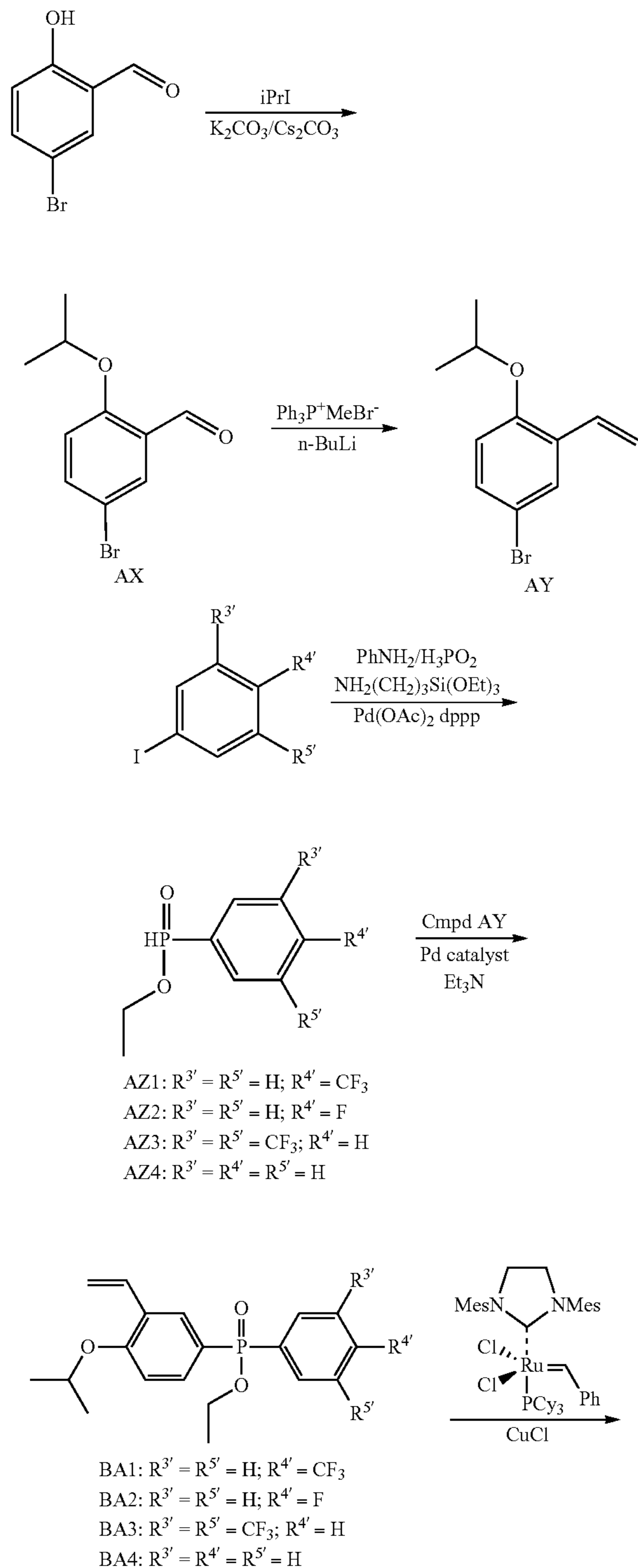
Scheme 2
