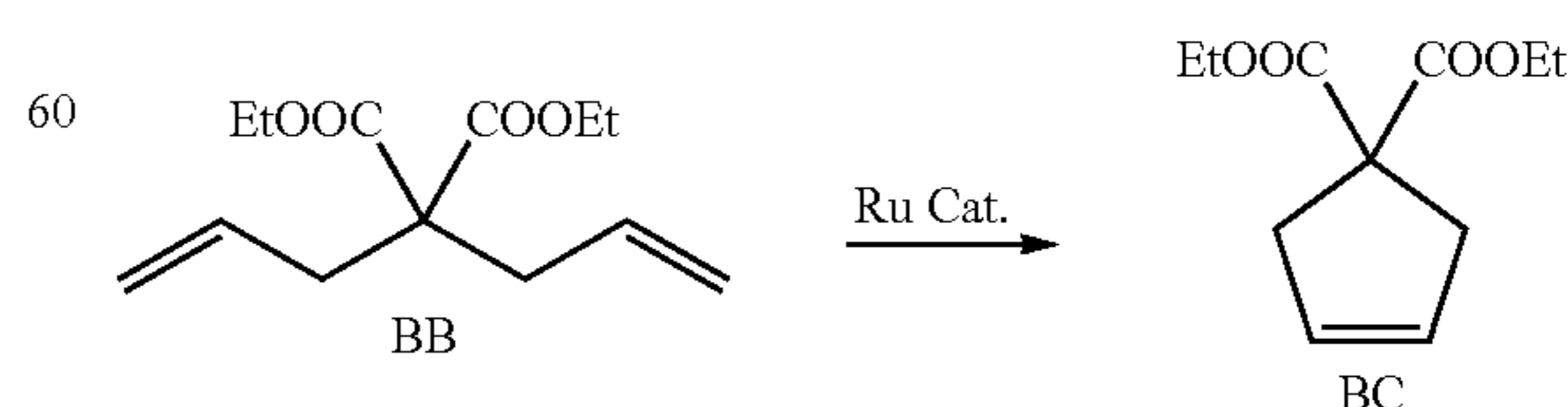
Scheme 7
