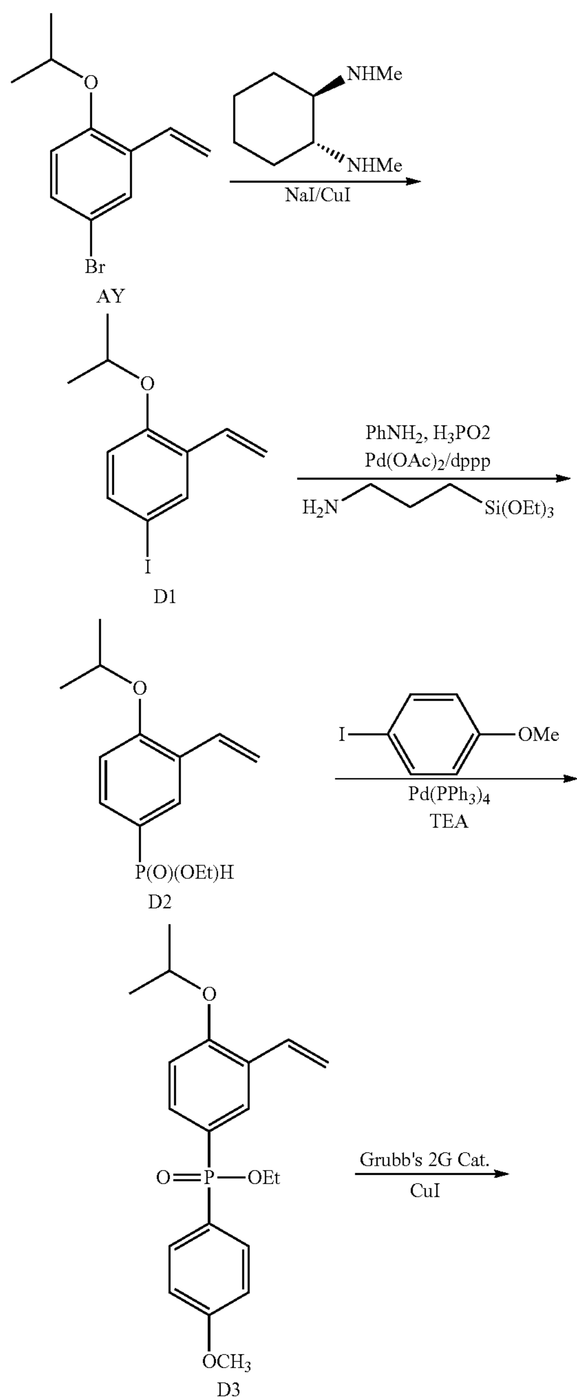
Scheme 4
