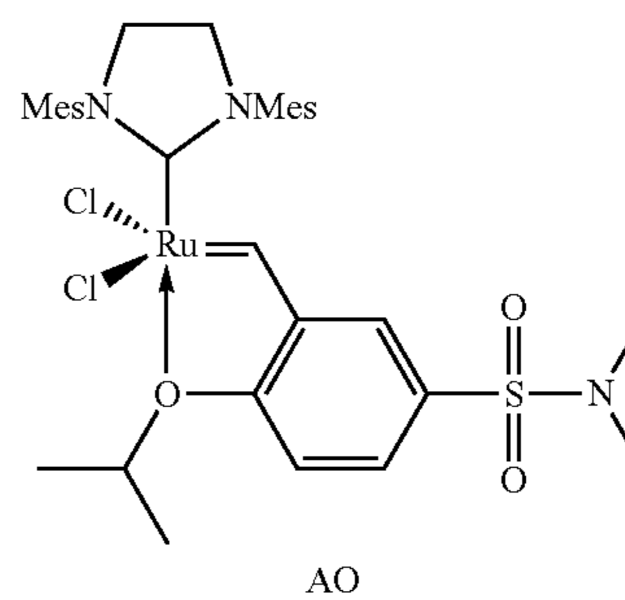
Scheme 9
