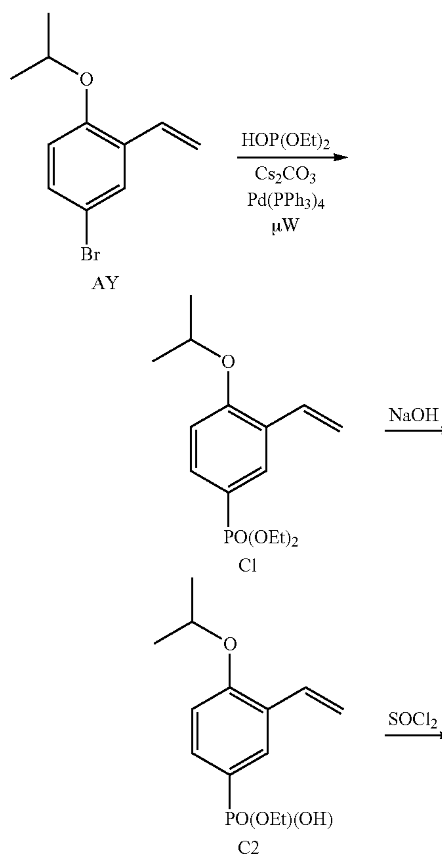
Scheme 3
