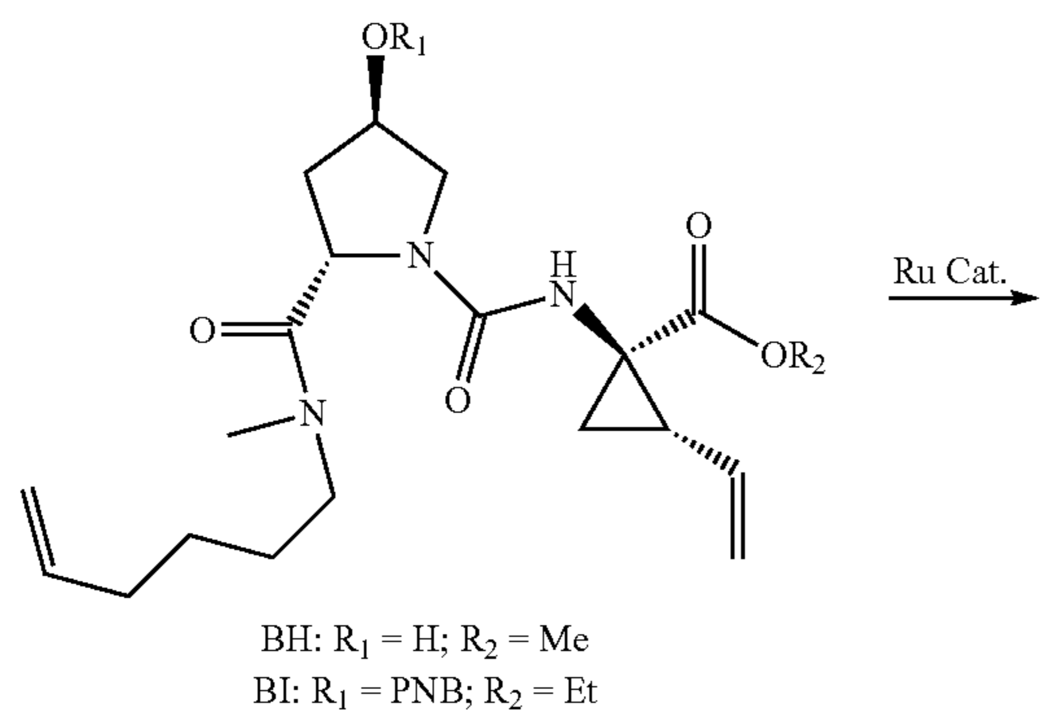
Scheme 8
