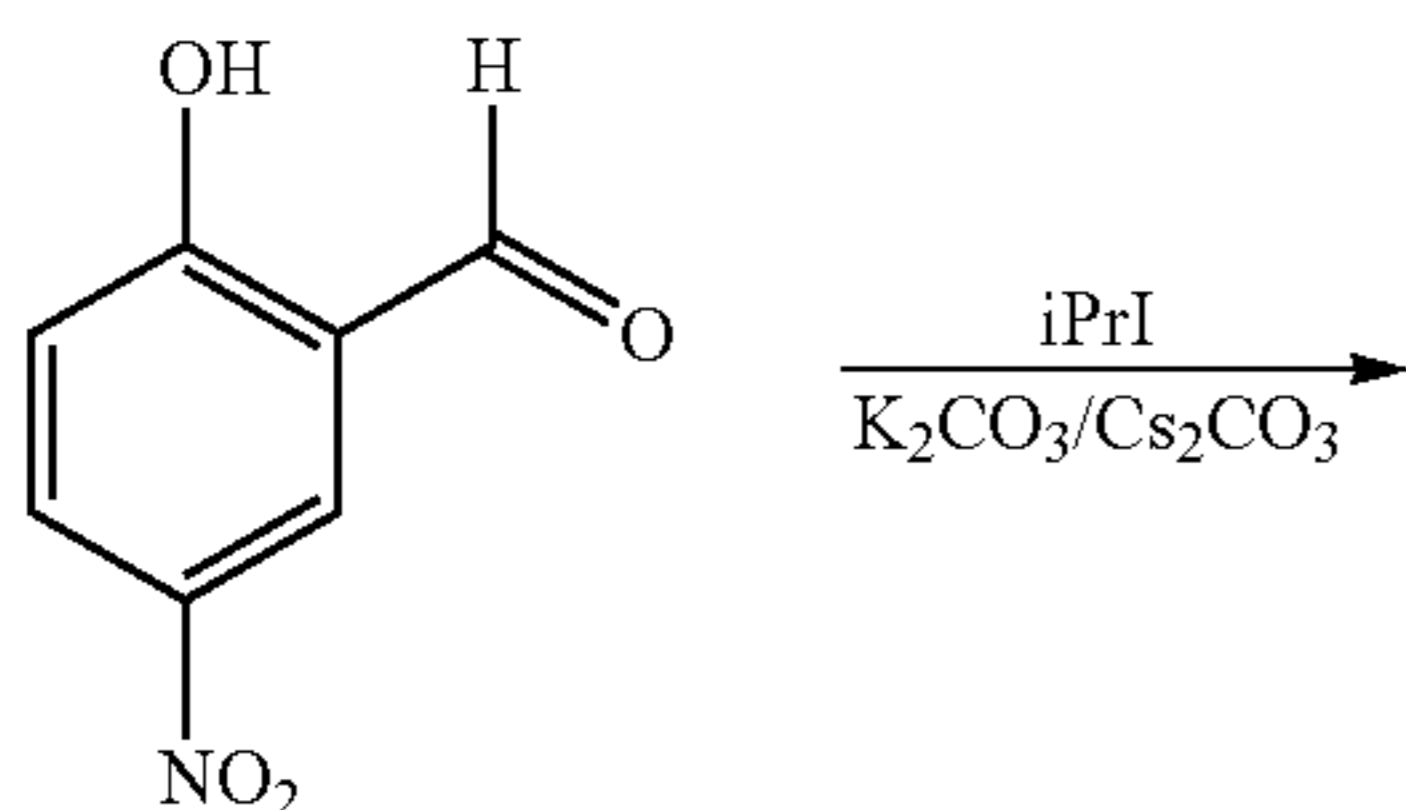
Scheme 5
