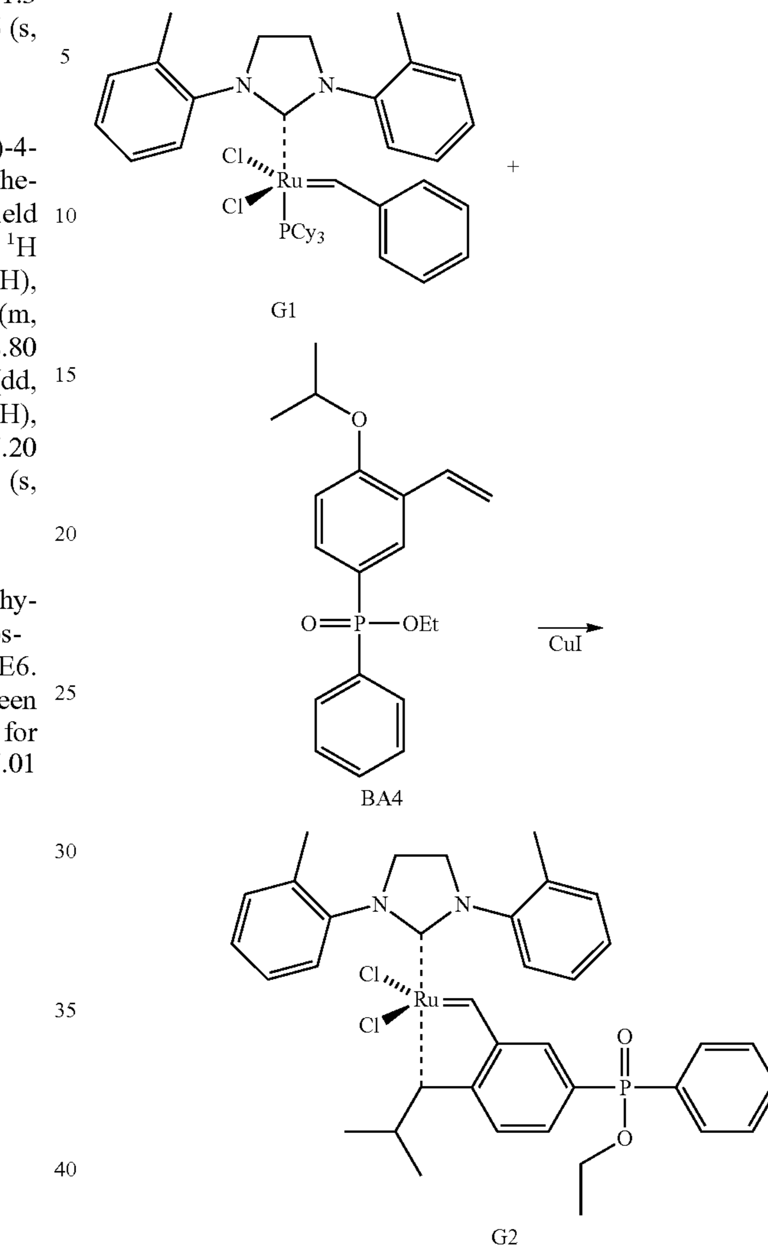
Scheme 6
