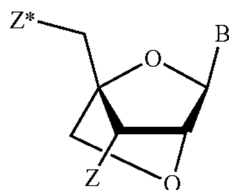
Beta-D-oxy-LNA
