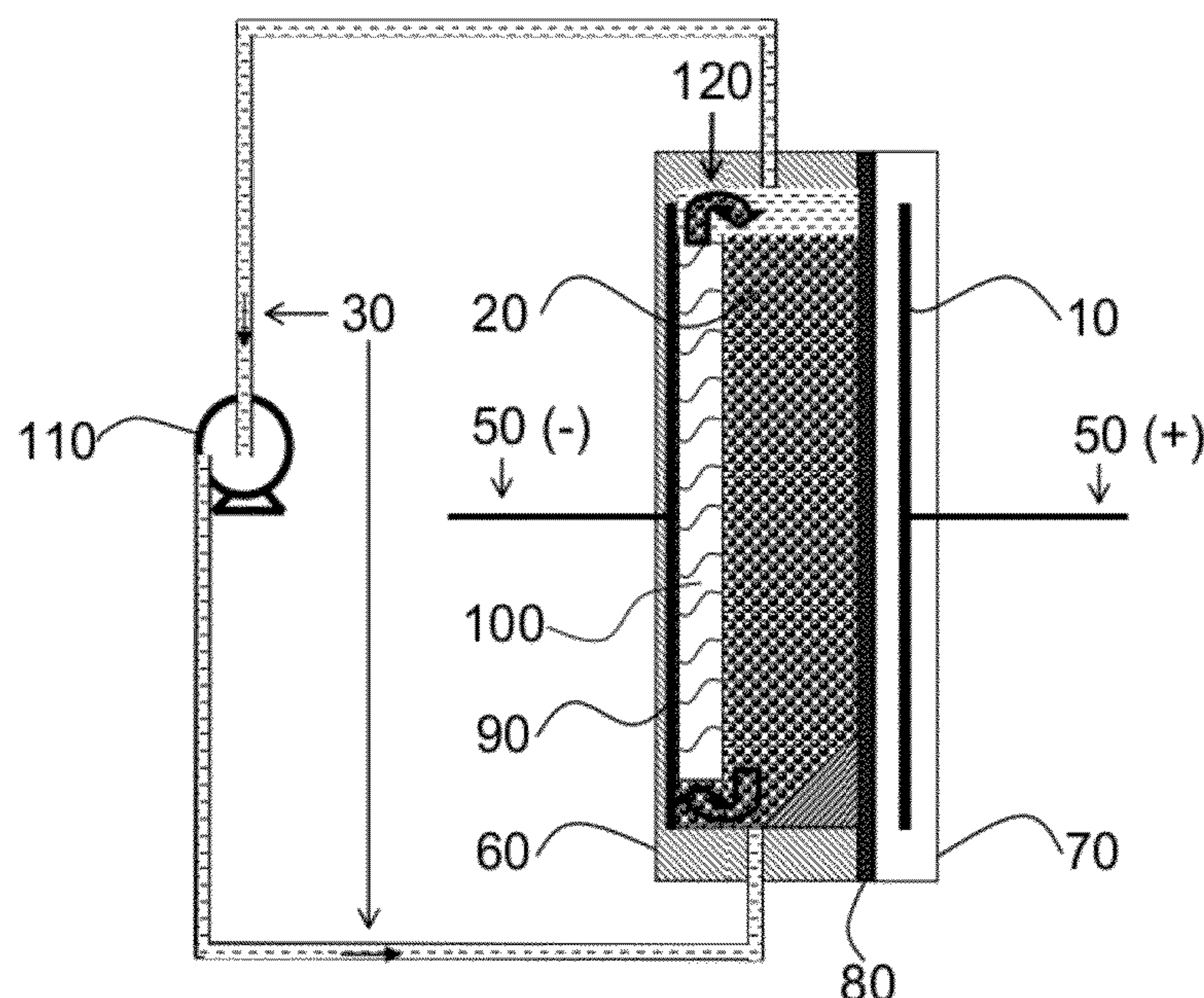
Side View
