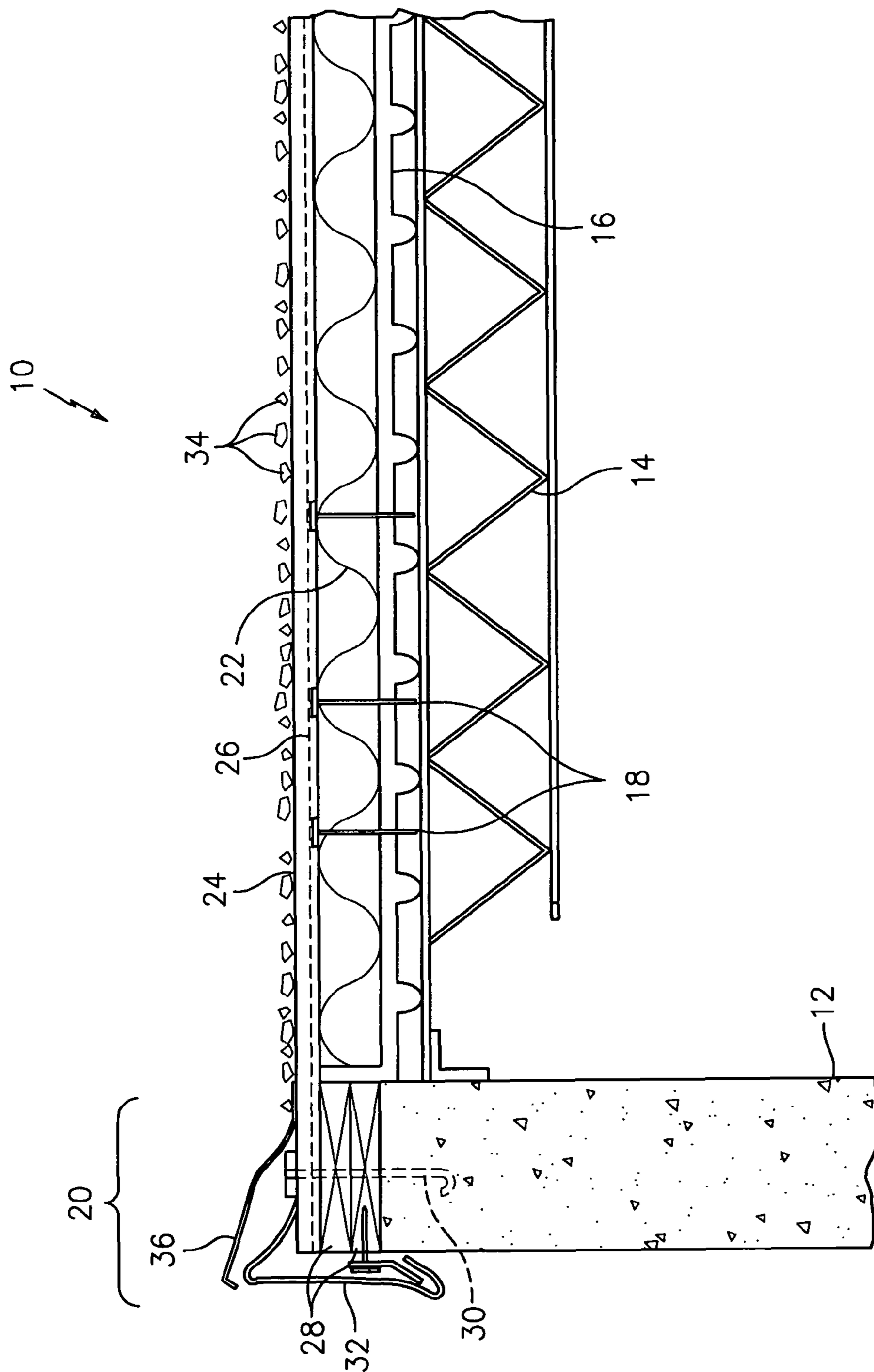
FIG. 1 (PRIOR ART)
