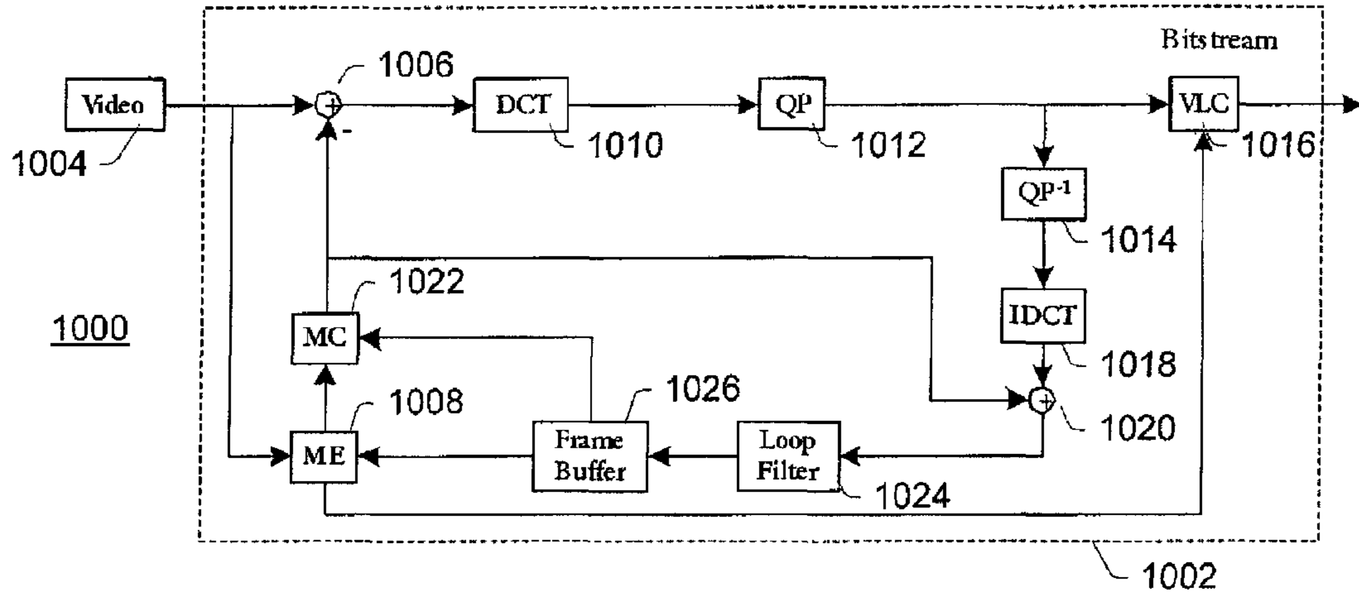
Fig. 10 (Prior Art)
