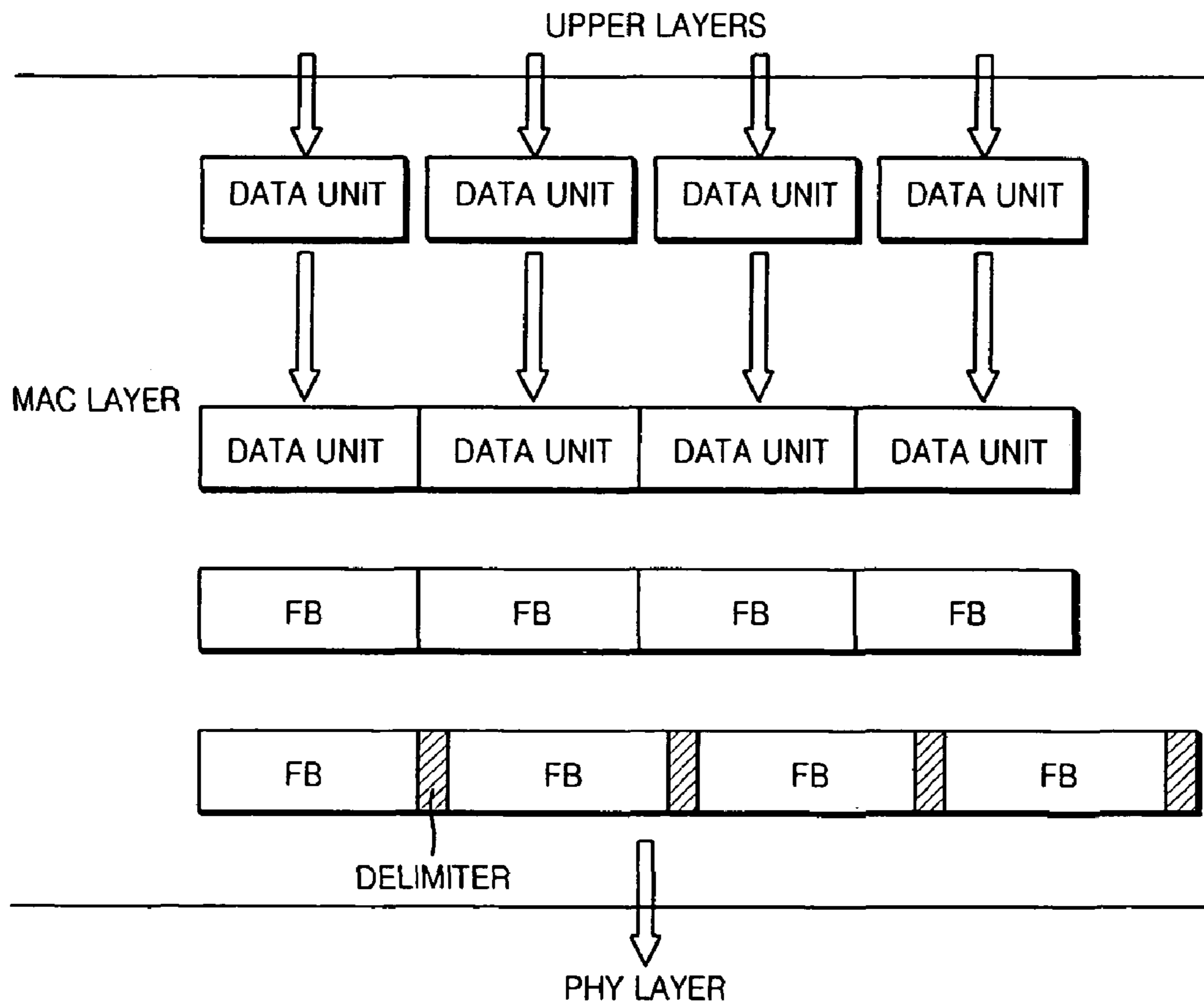
FIG. 2 (PRIOR ART)
