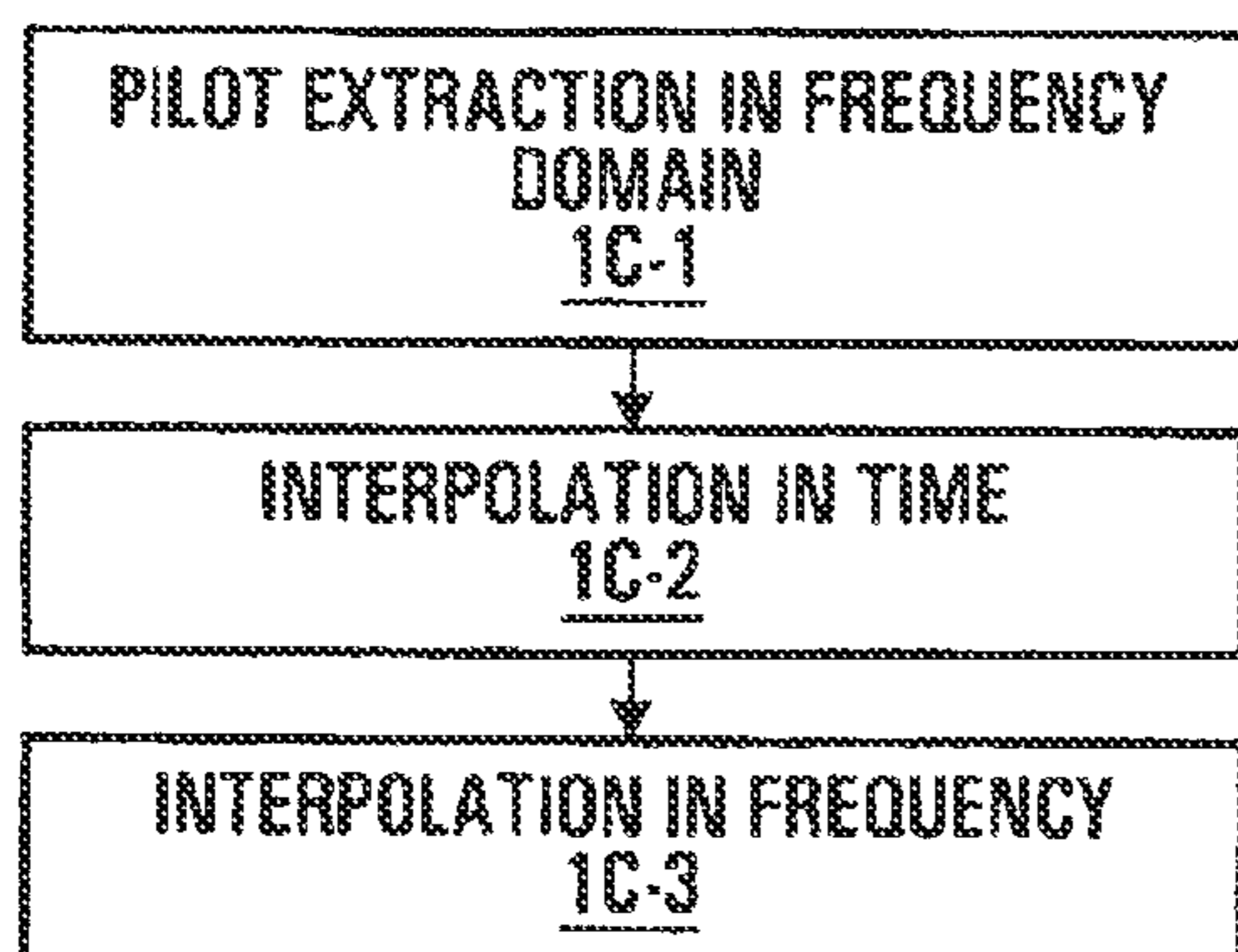
FIG. 1C (PRIOR ART)
