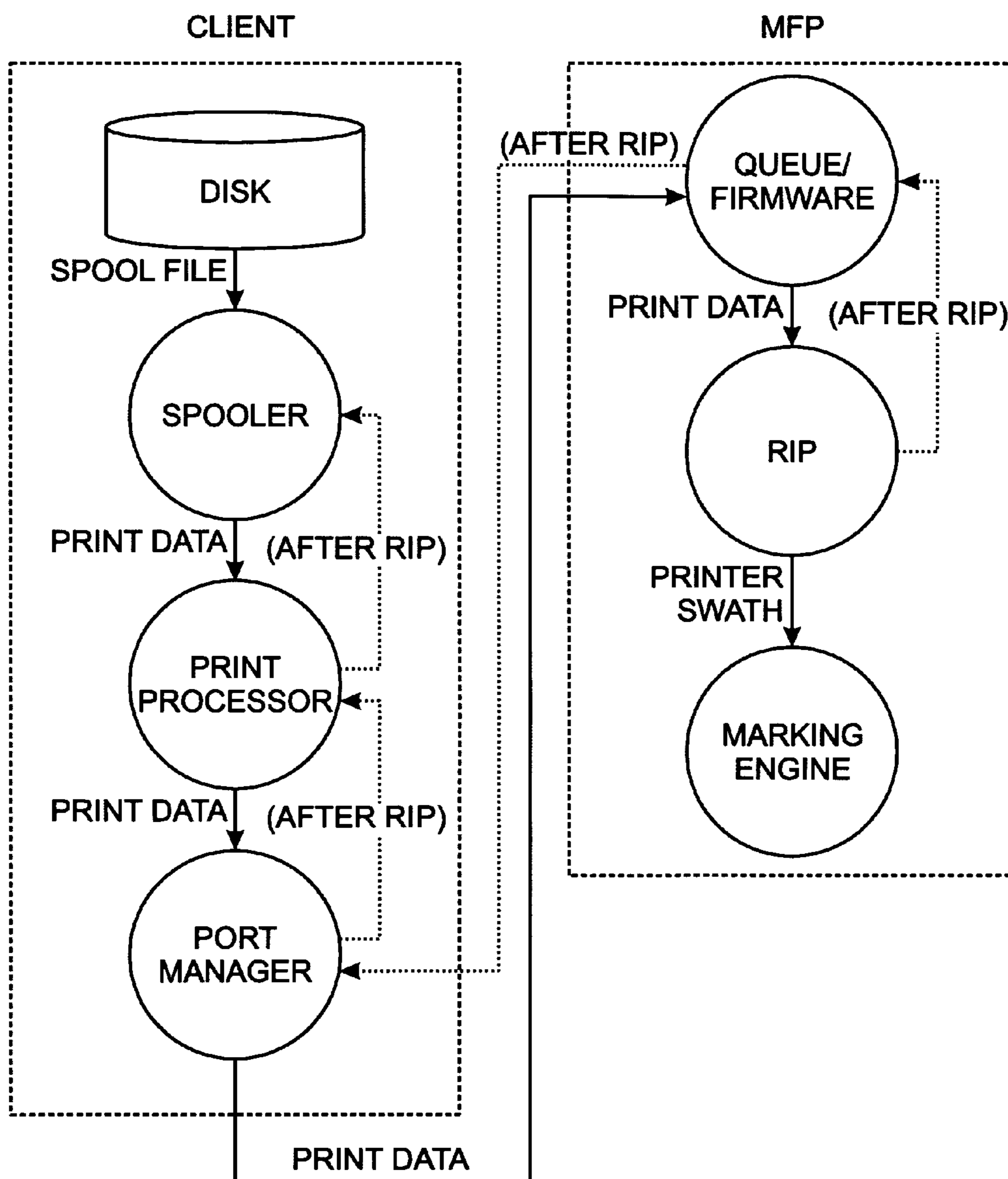
Fig. 1 (PRIOR ART)
