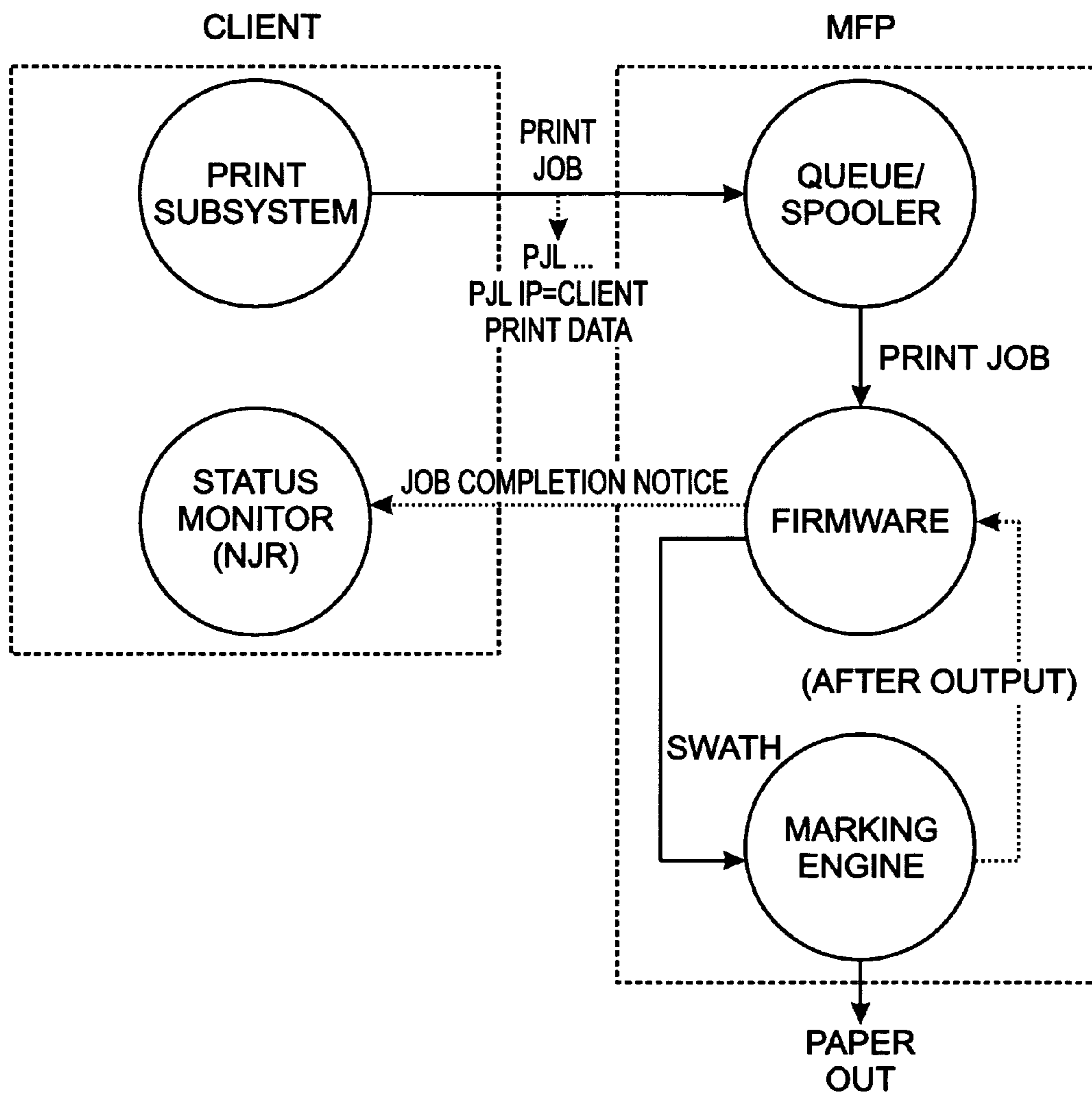
Fig. 2 (PRIOR ART)
