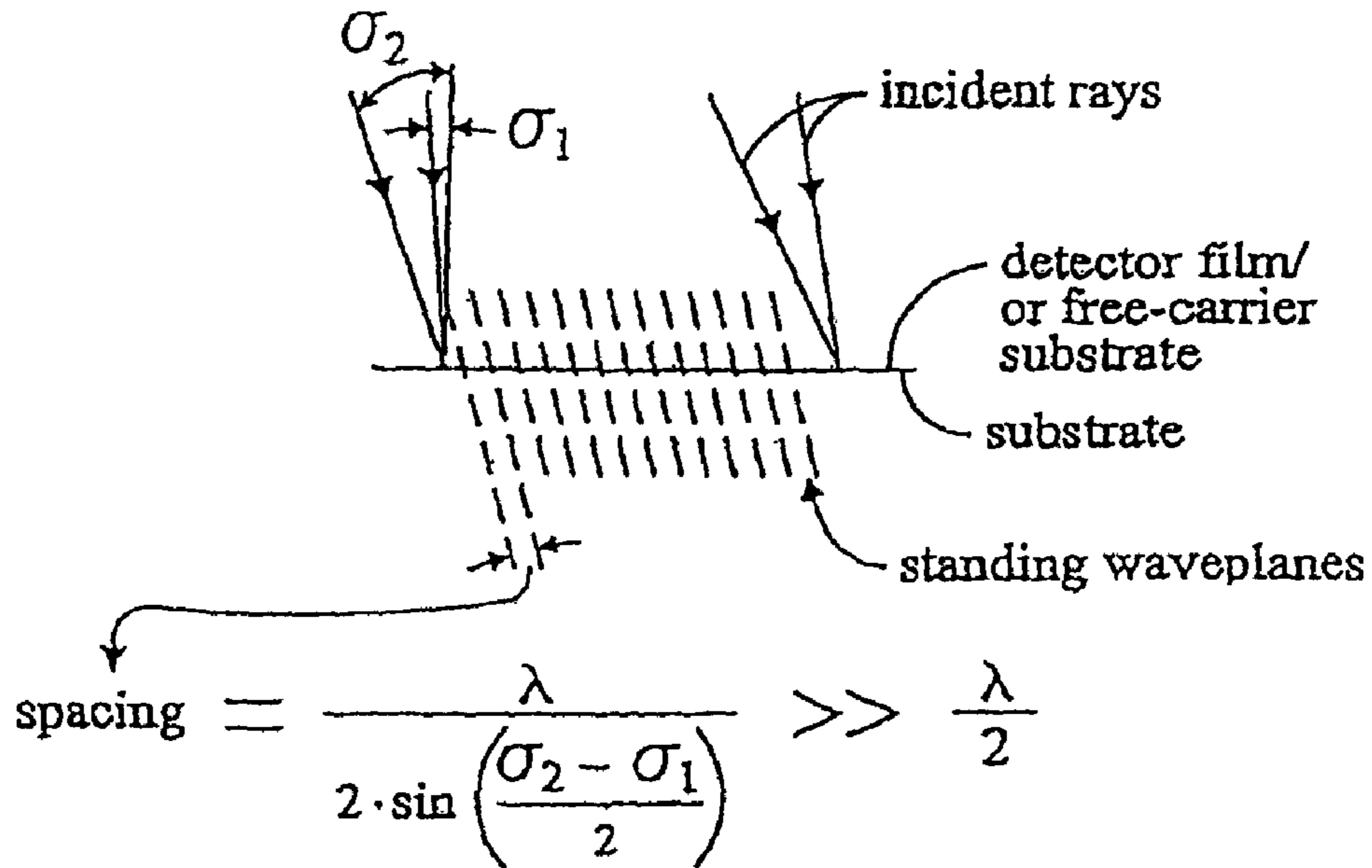
Conventional Method (single sided Hologram/Interferogram)
