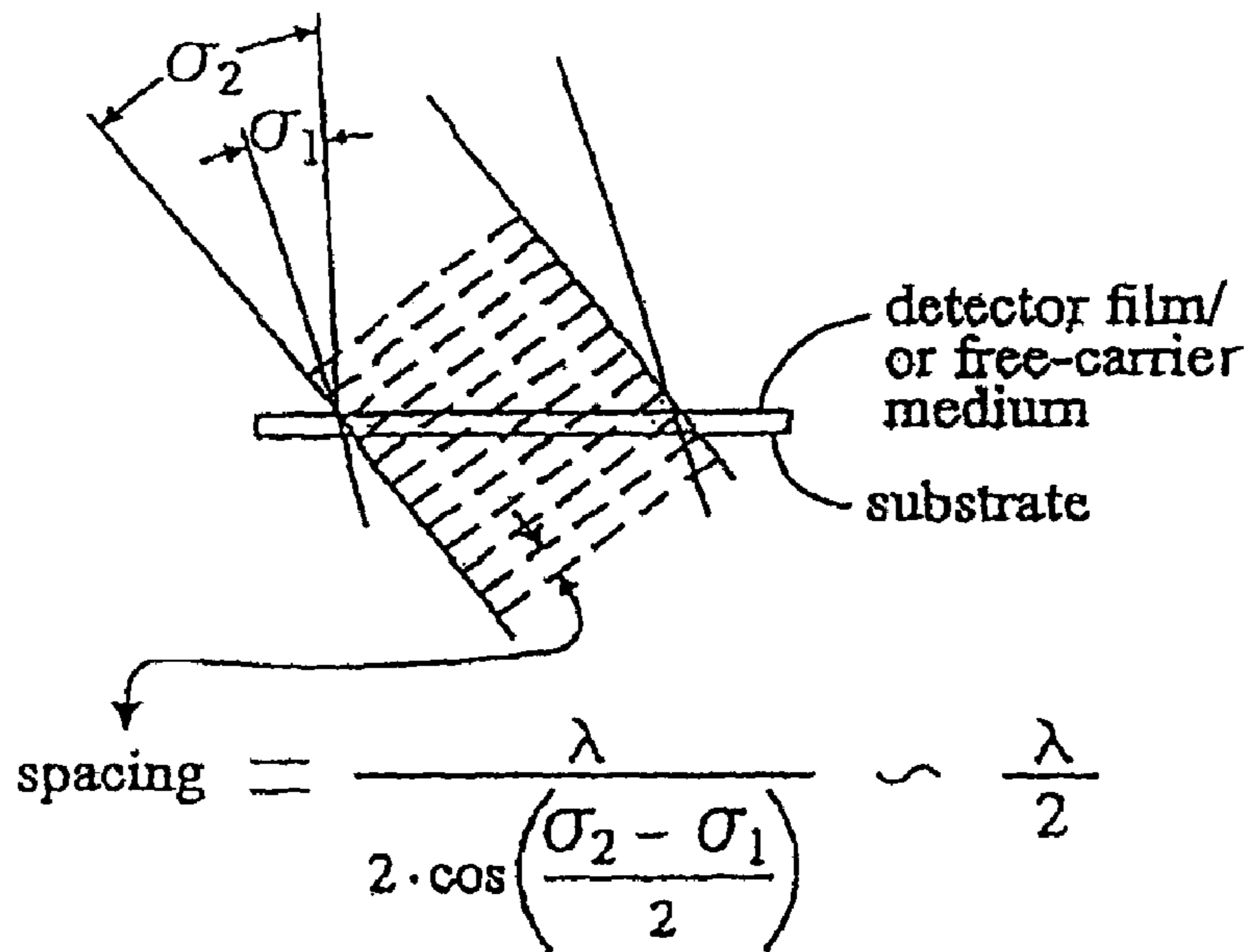
Double Sided Method (Holography/Interferogram)
