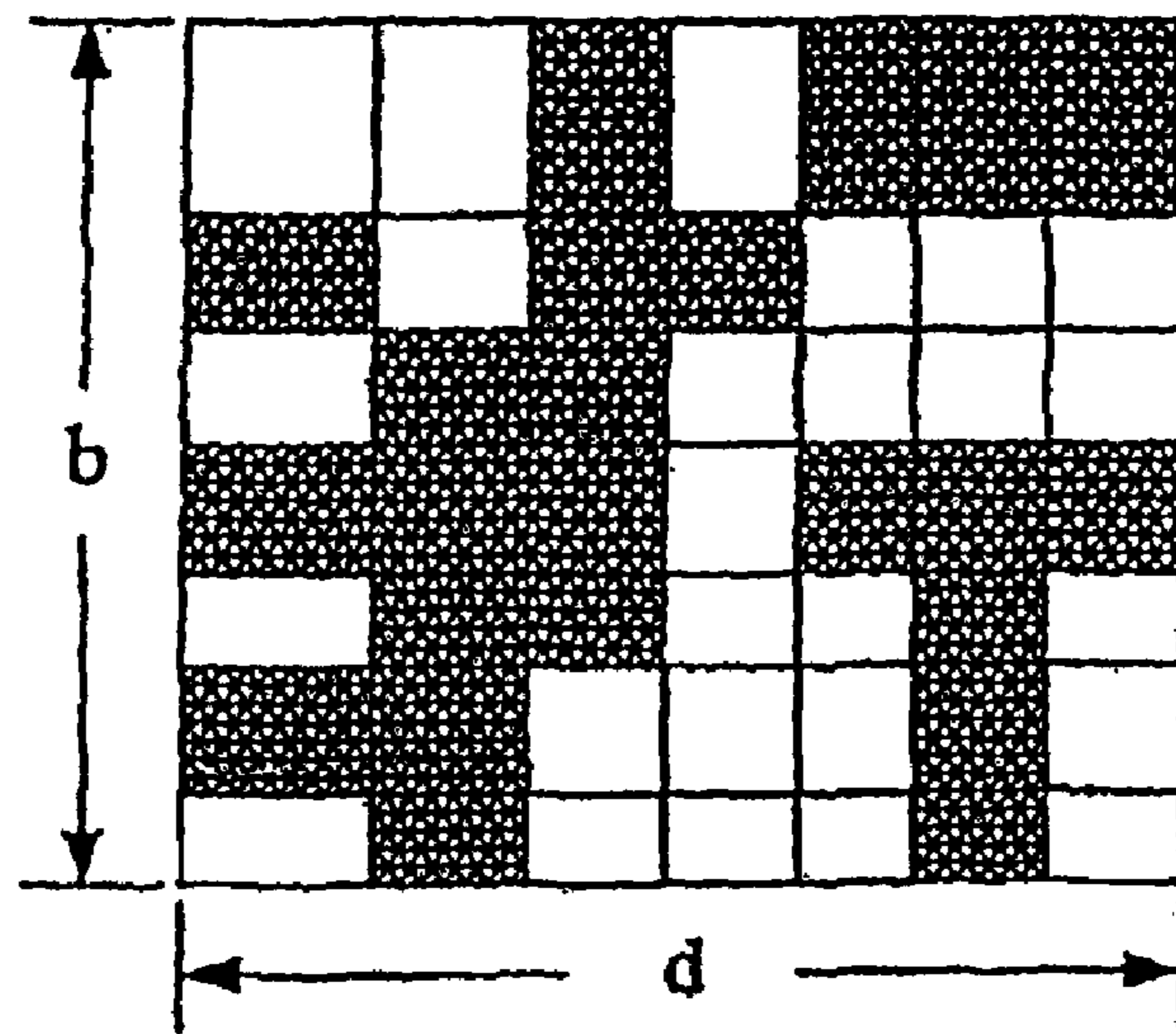
Illustration showing arrangement of generalized Gury detour-phase IR Hologram
