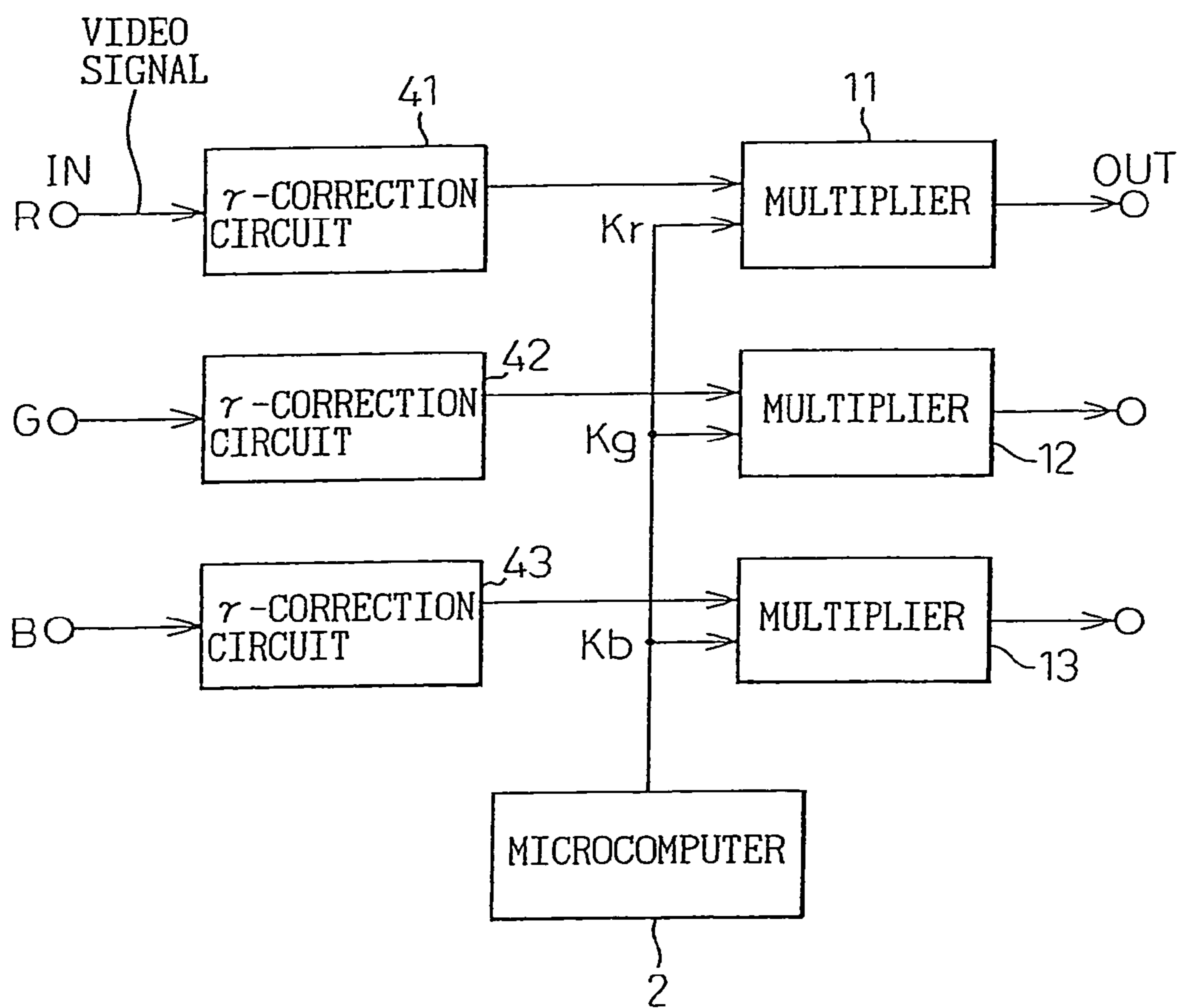
Fig. 4 (PRIOR ART)
