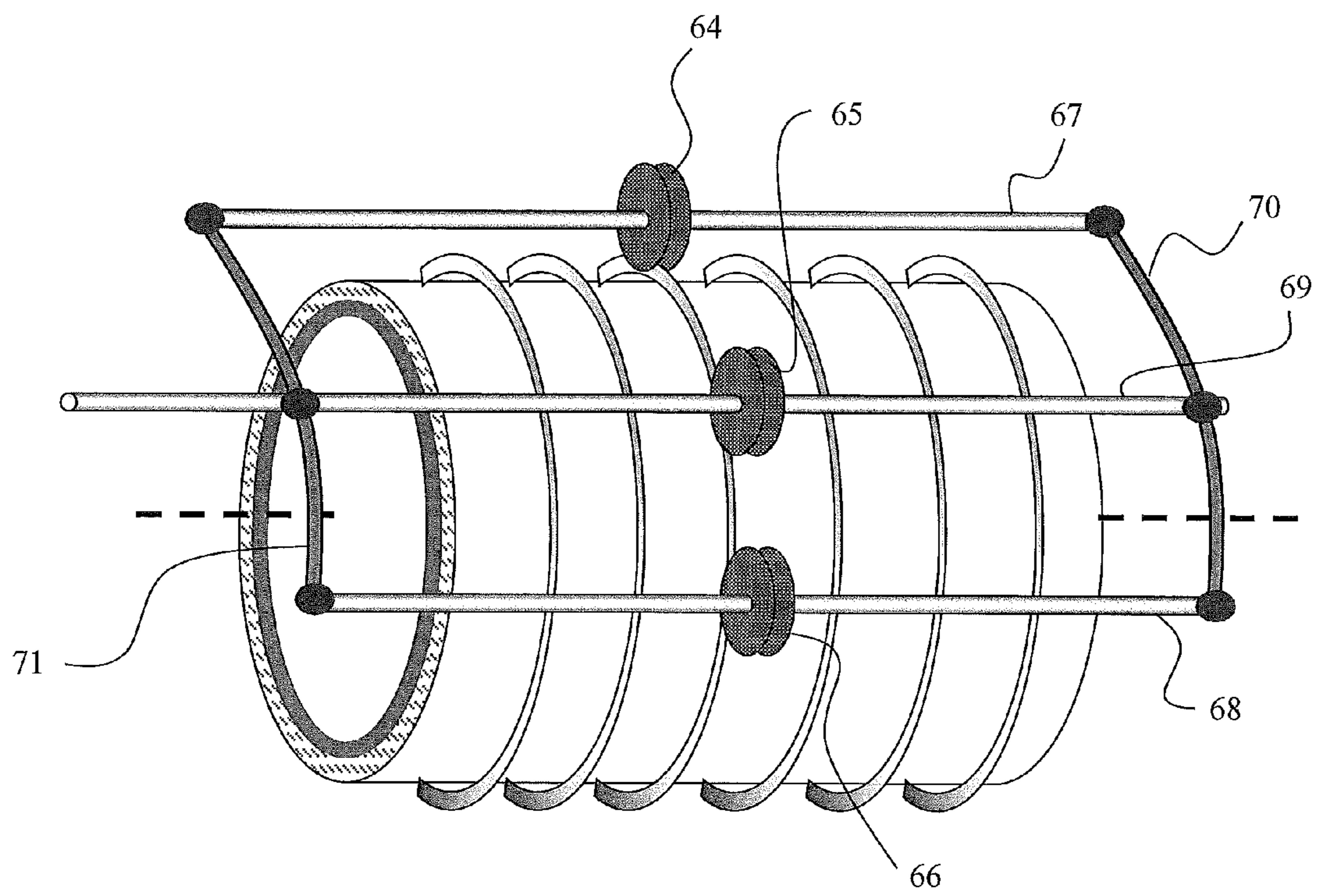
FIGURE 19: Linear, high power, phase shifter.
