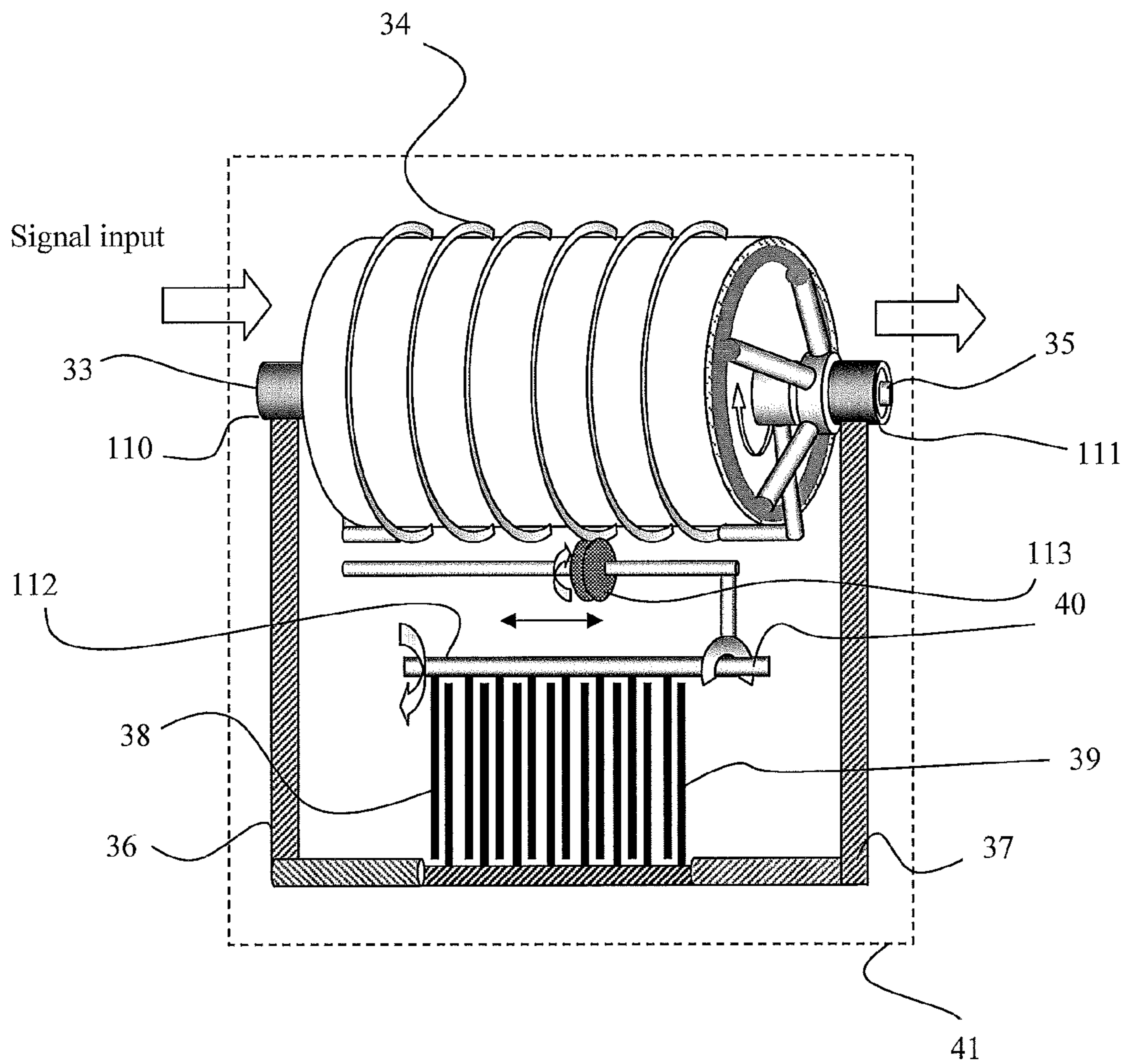
FIGURE 11: Low frequency impedance tuner
