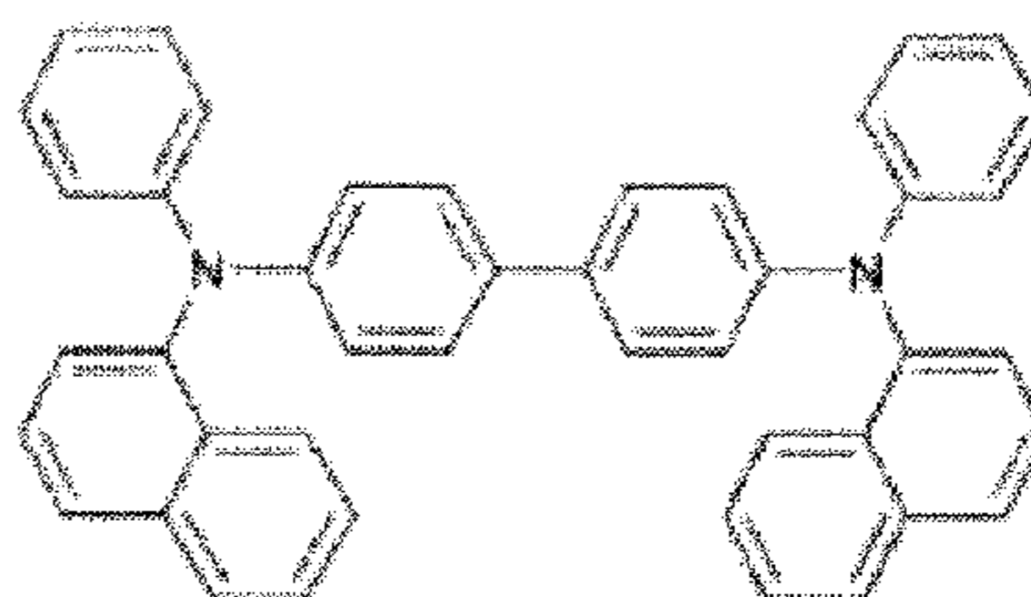
4-4'-bis[N-(1-naphthyl)-N-phenyl-amino]biphenyl (NPD)
