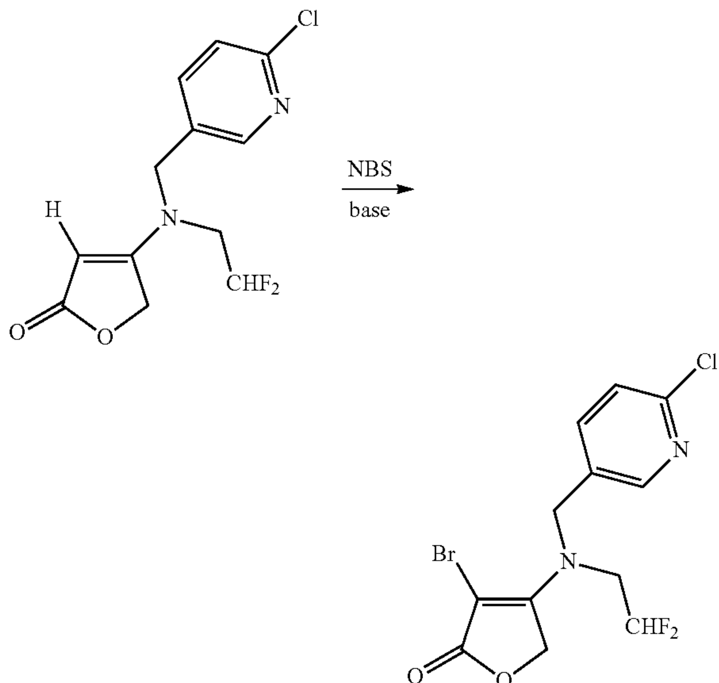
Scheme IX:
