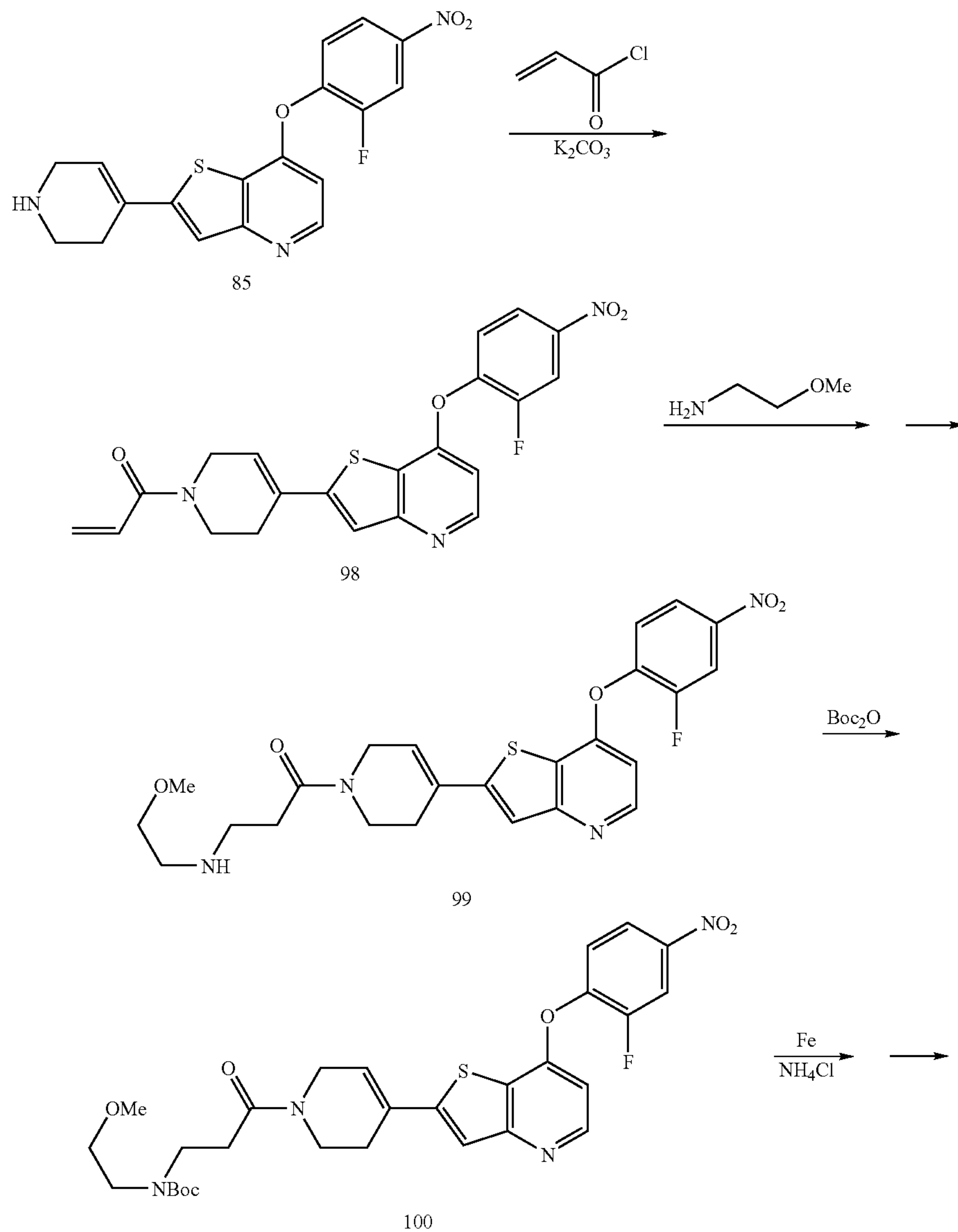
Scheme 4
