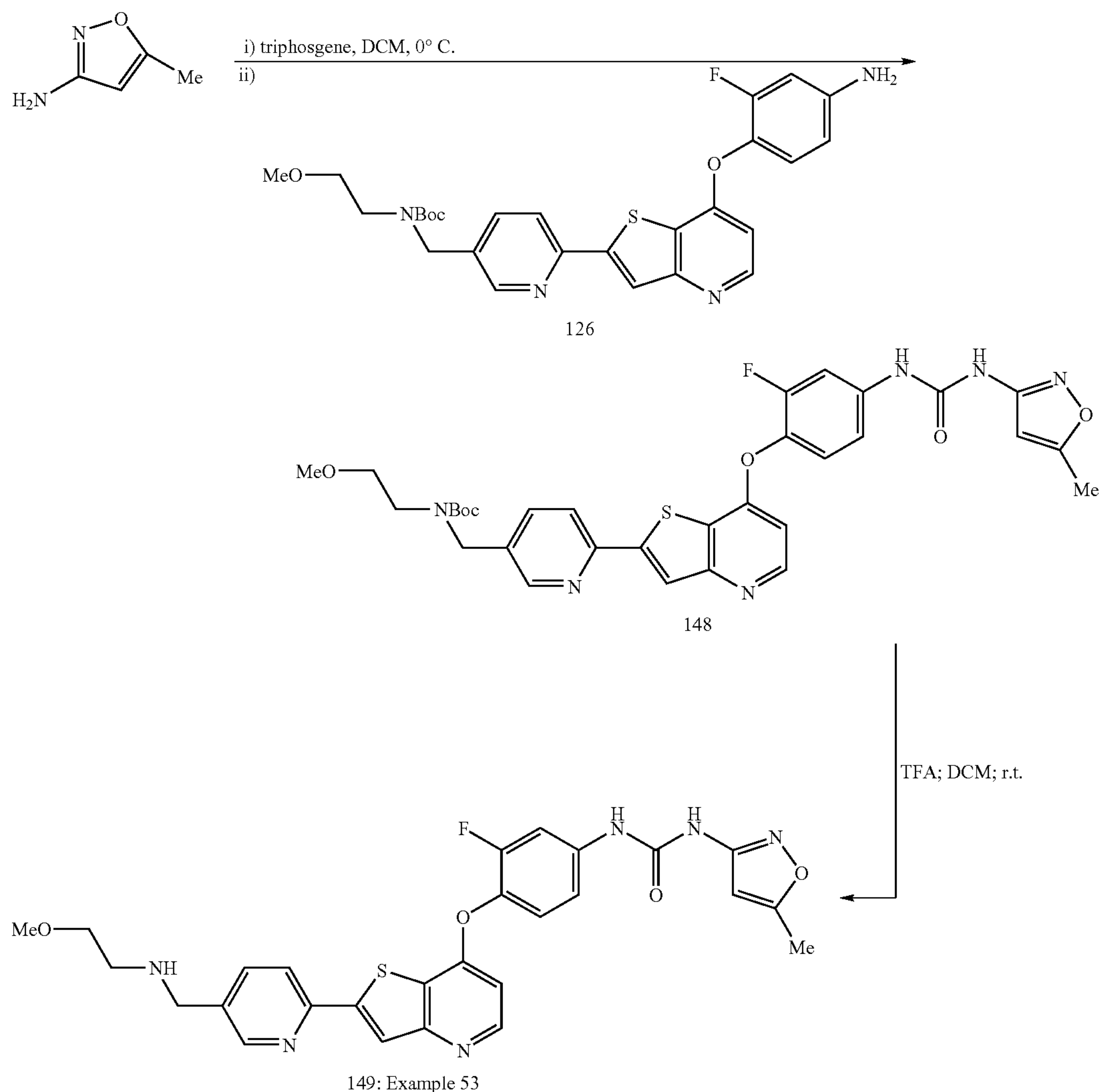
Scheme 11
