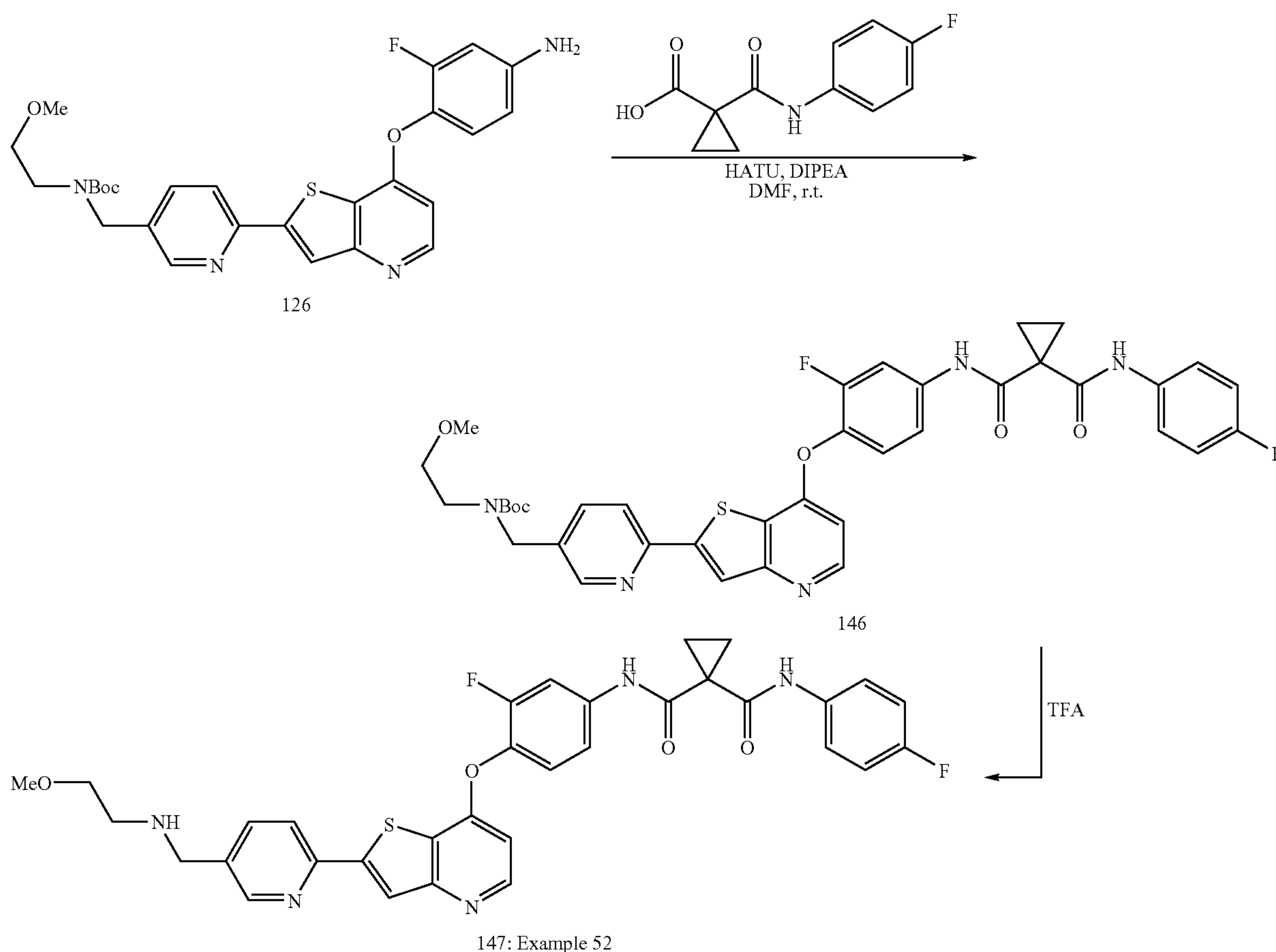
Scheme 10
