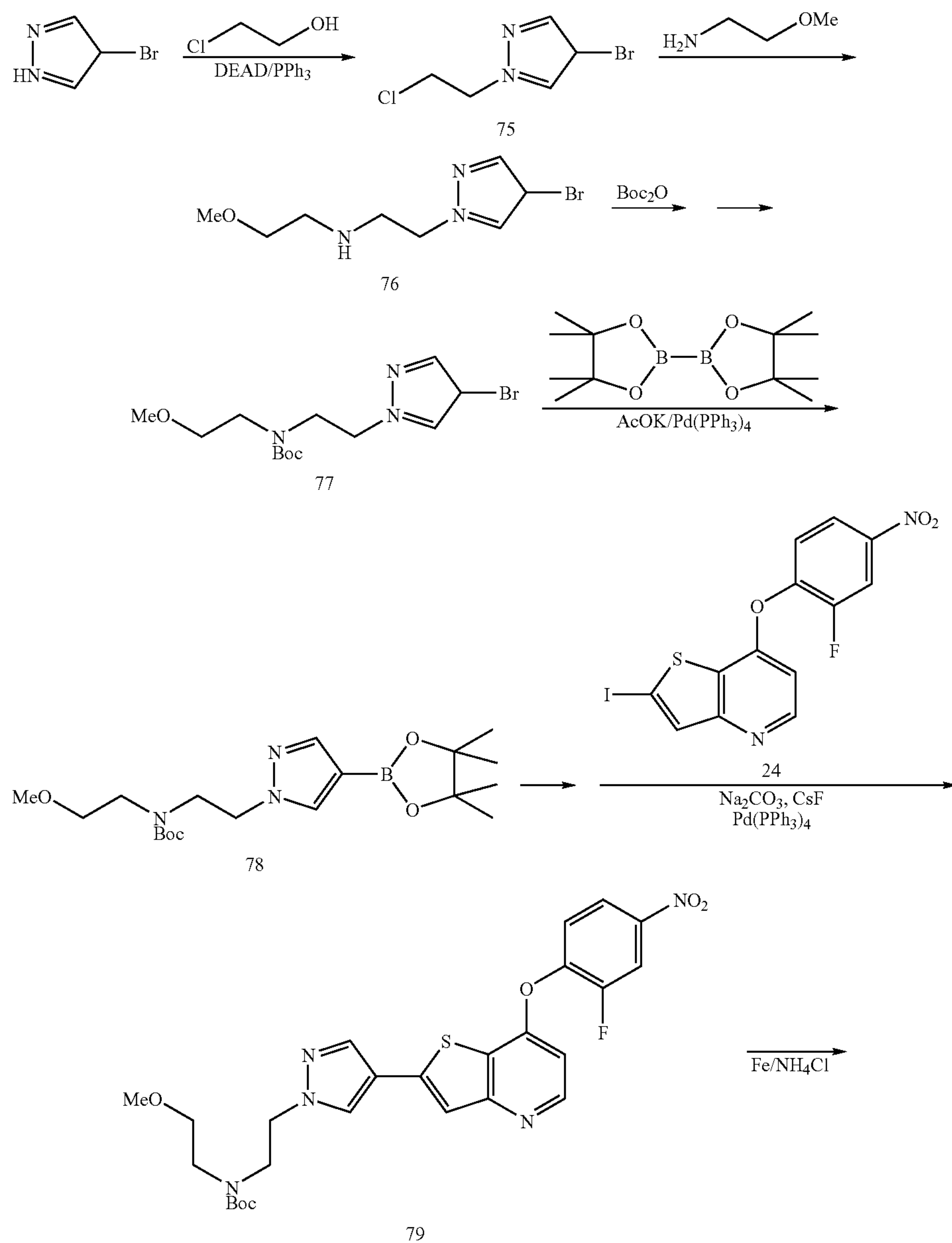
Scheme 3
