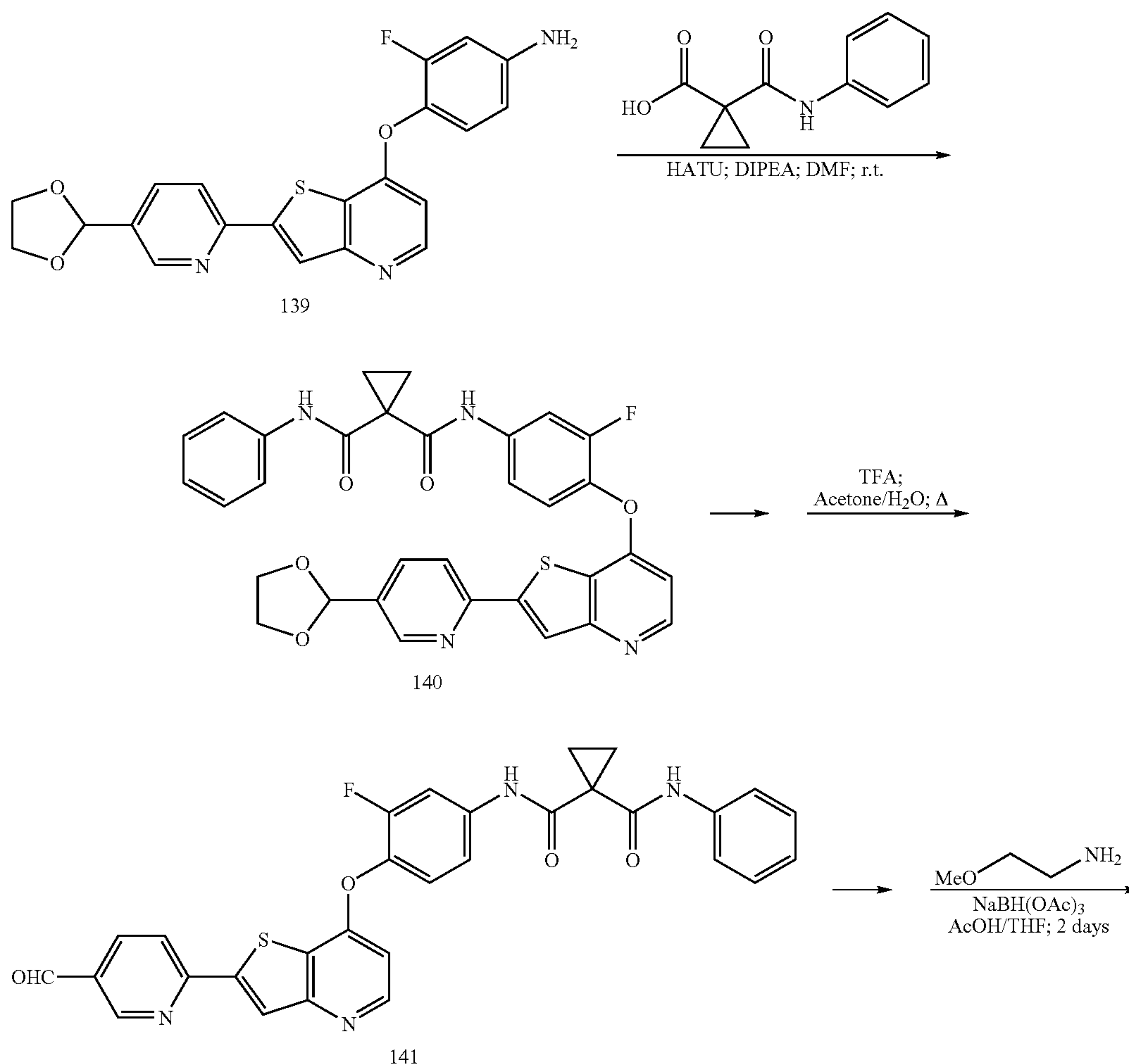
Scheme 8
