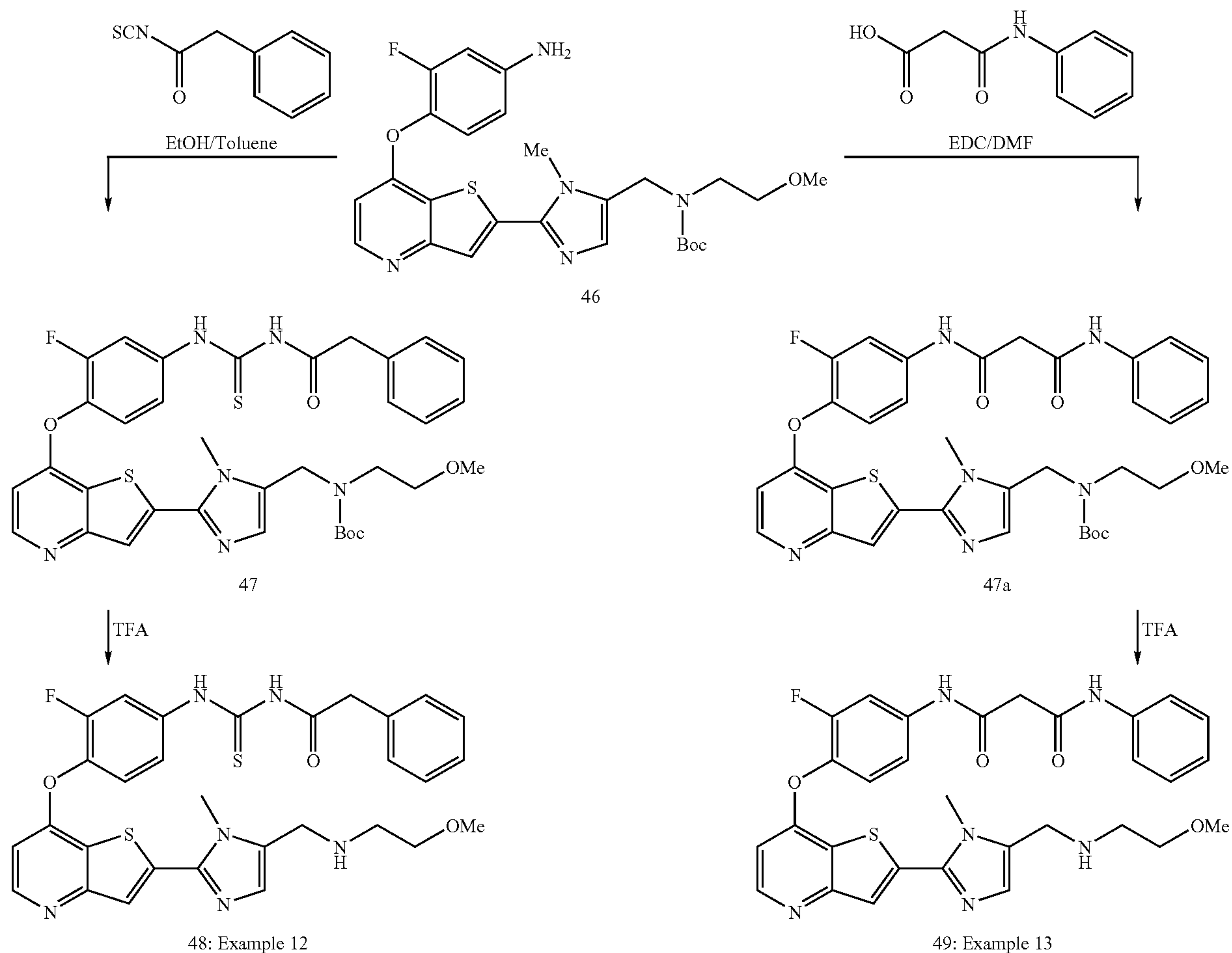
Scheme 2
