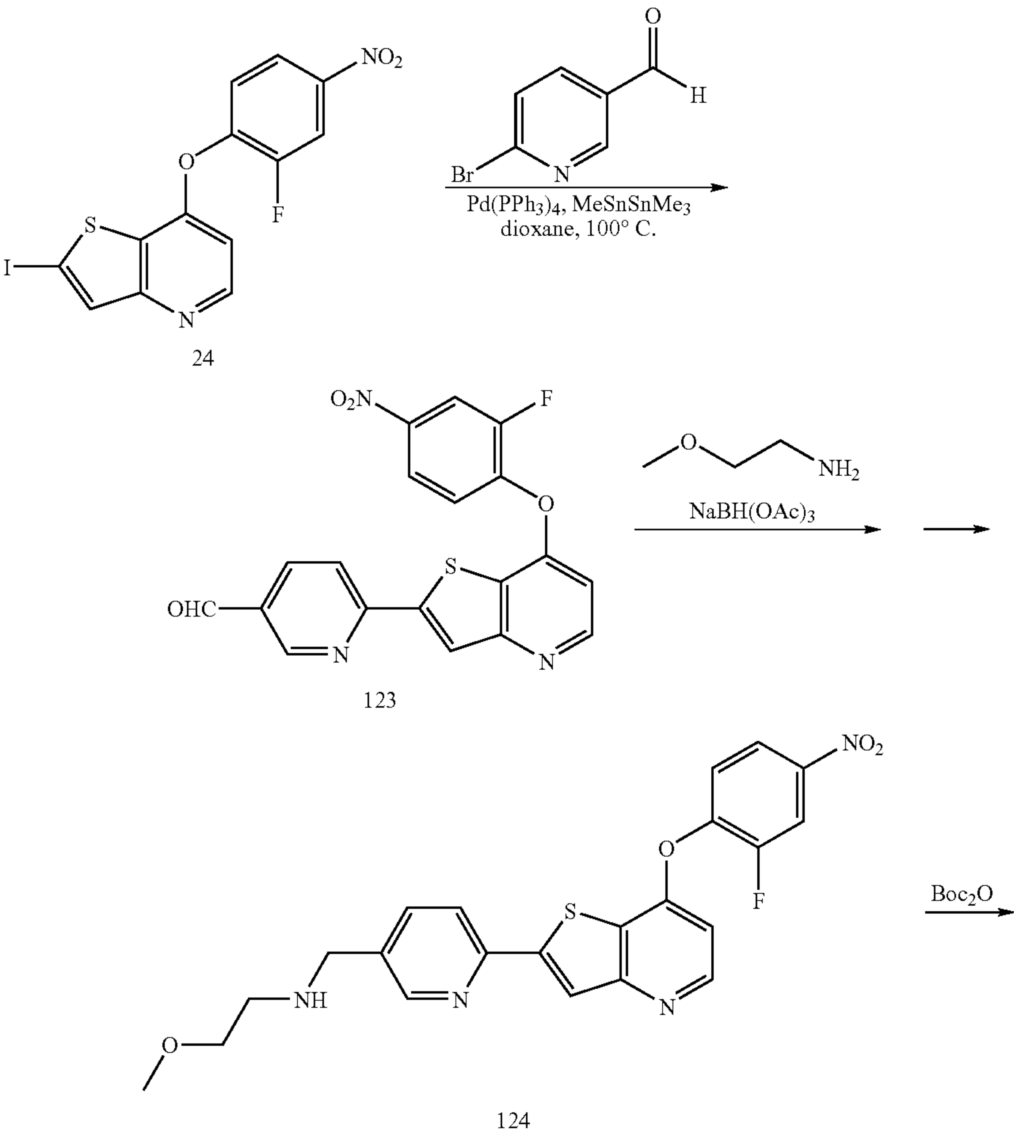
Scheme 6
