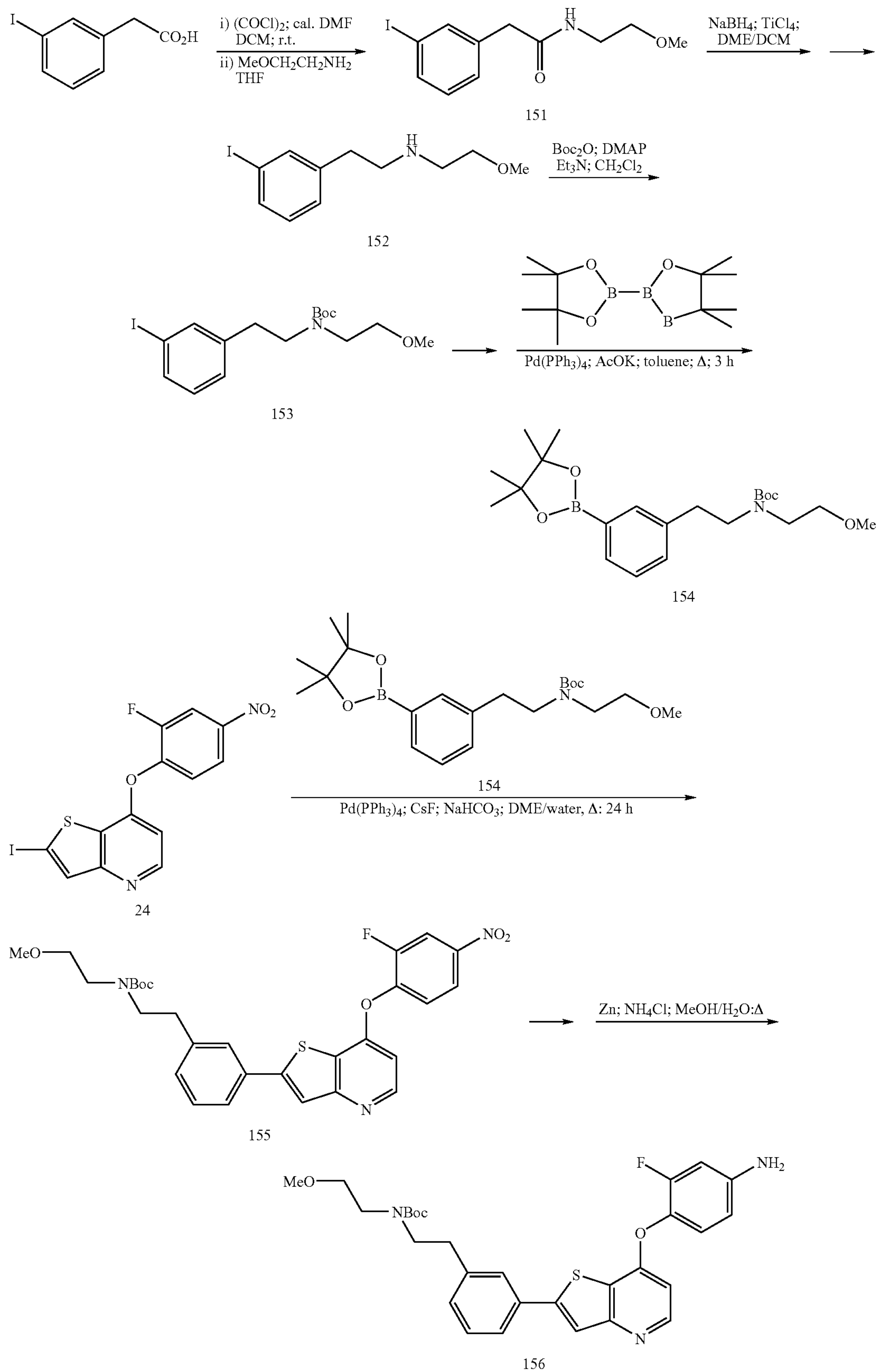
Scheme 12
