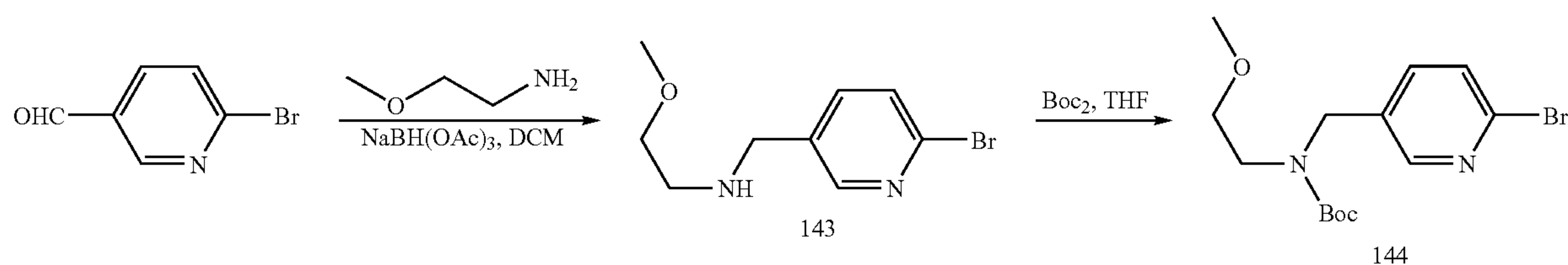
Scheme 9
