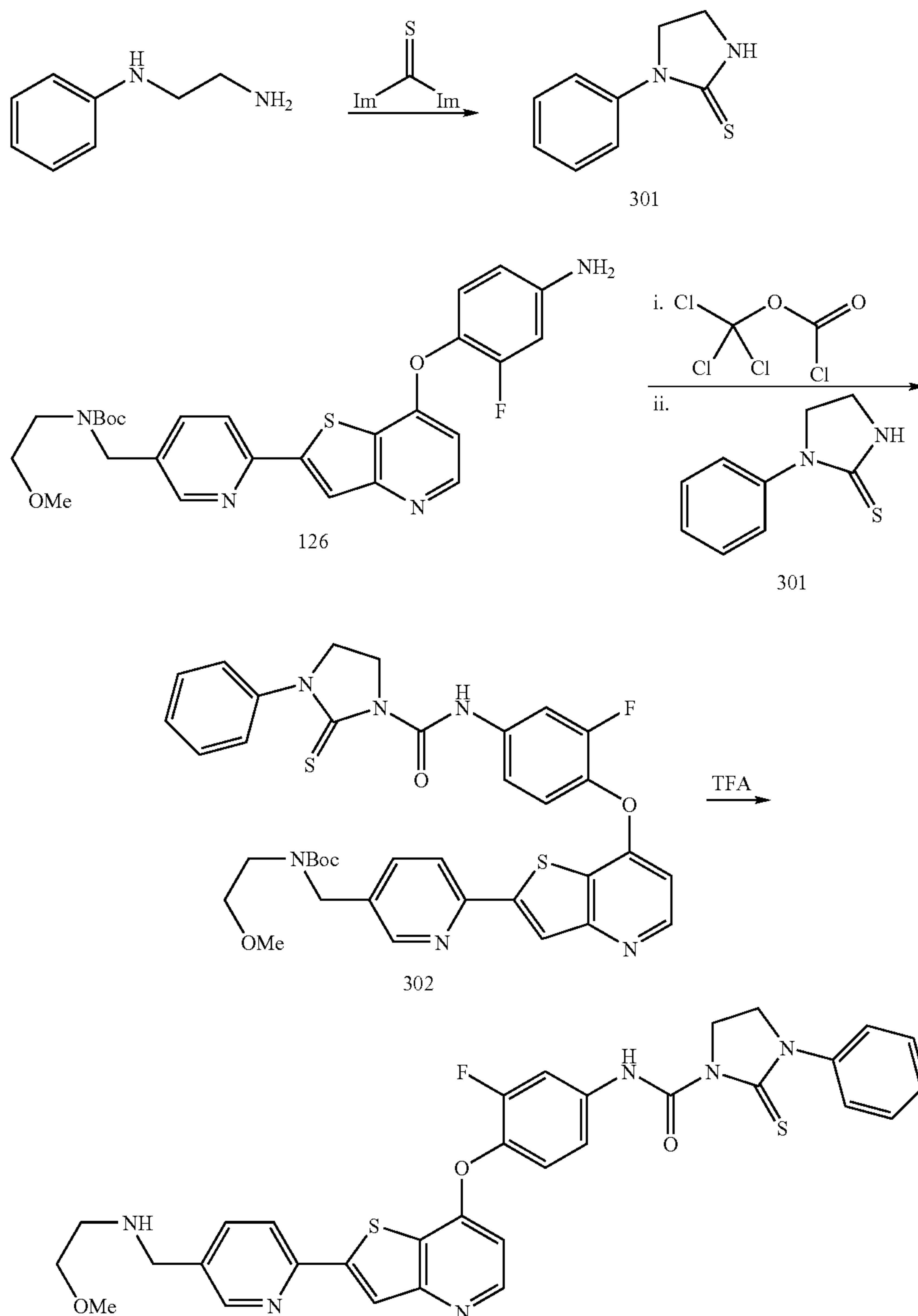
Scheme 16
