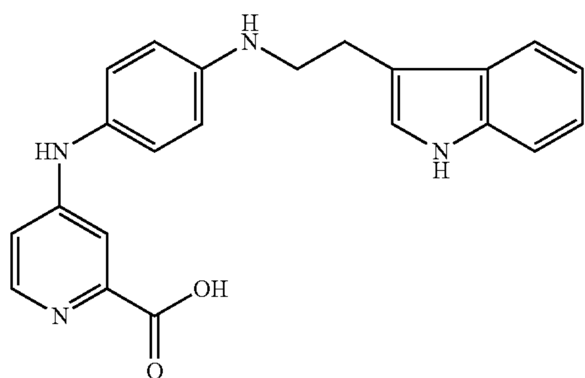
Co. No. 58; mp. 190° C. Ex. [B2]
