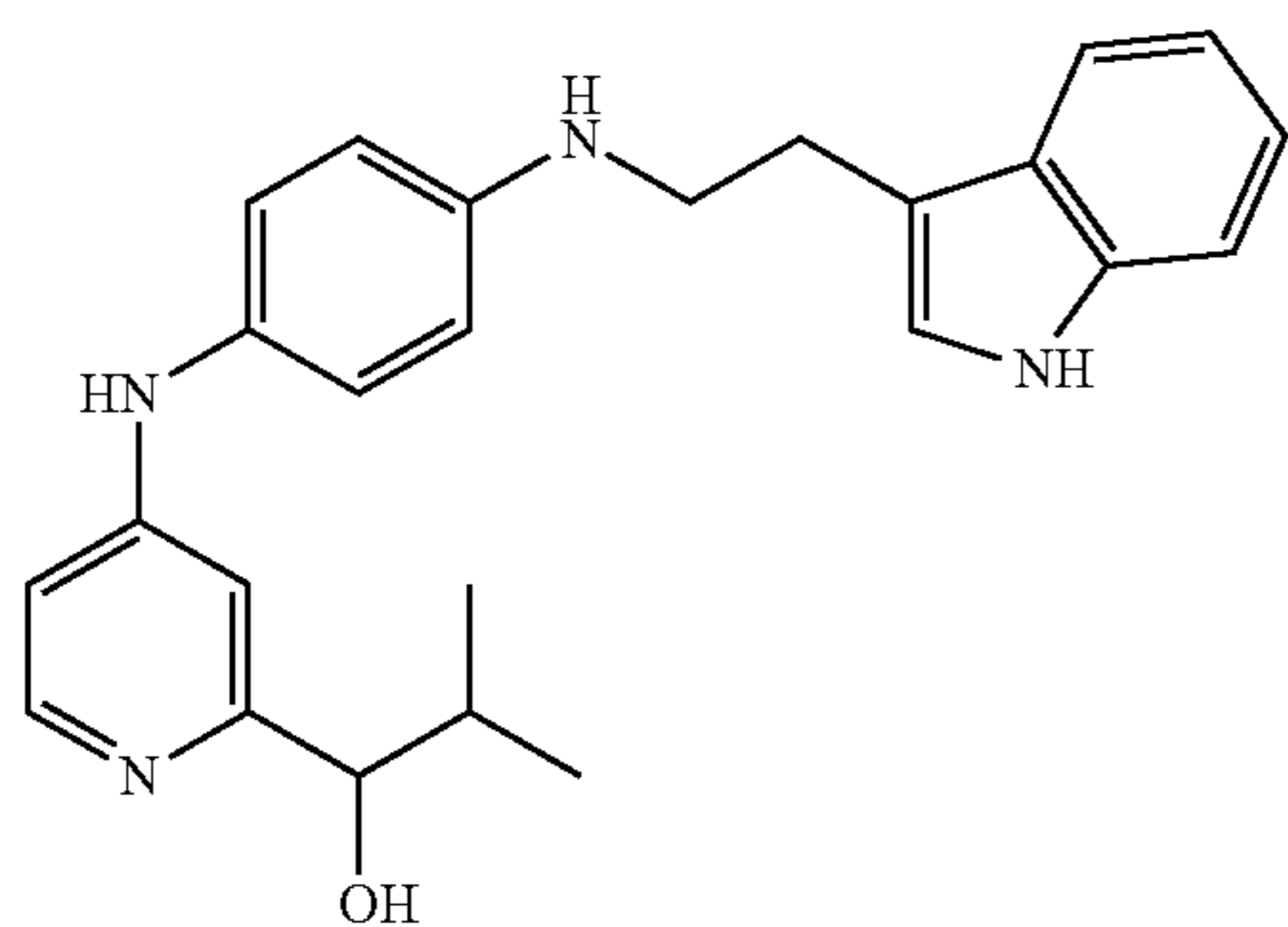
Co. No. 137; ms. 401 Ex. [B12]; from int. 53
