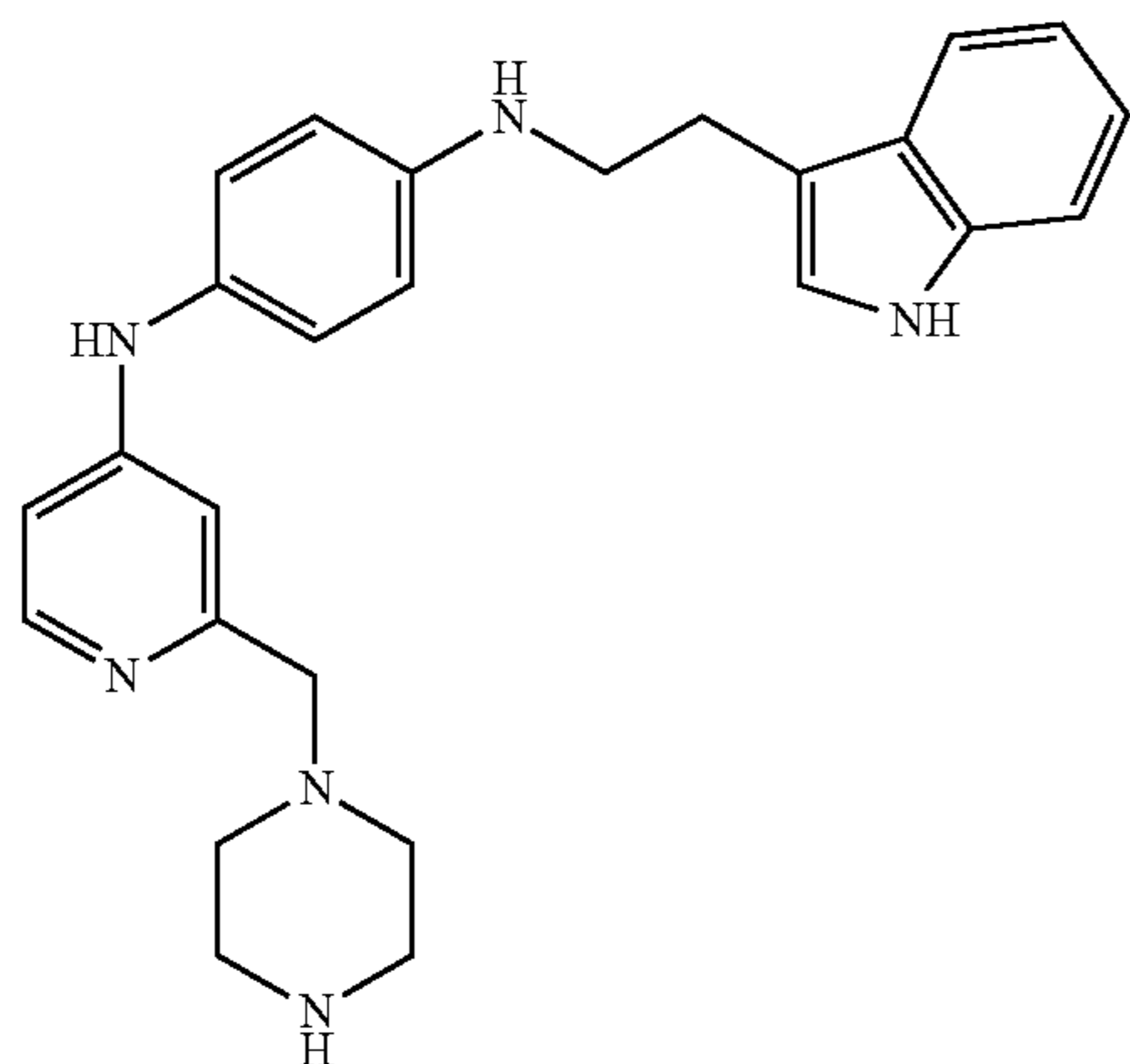
Co. No. 91; ms. 427 Ex. [B17]
