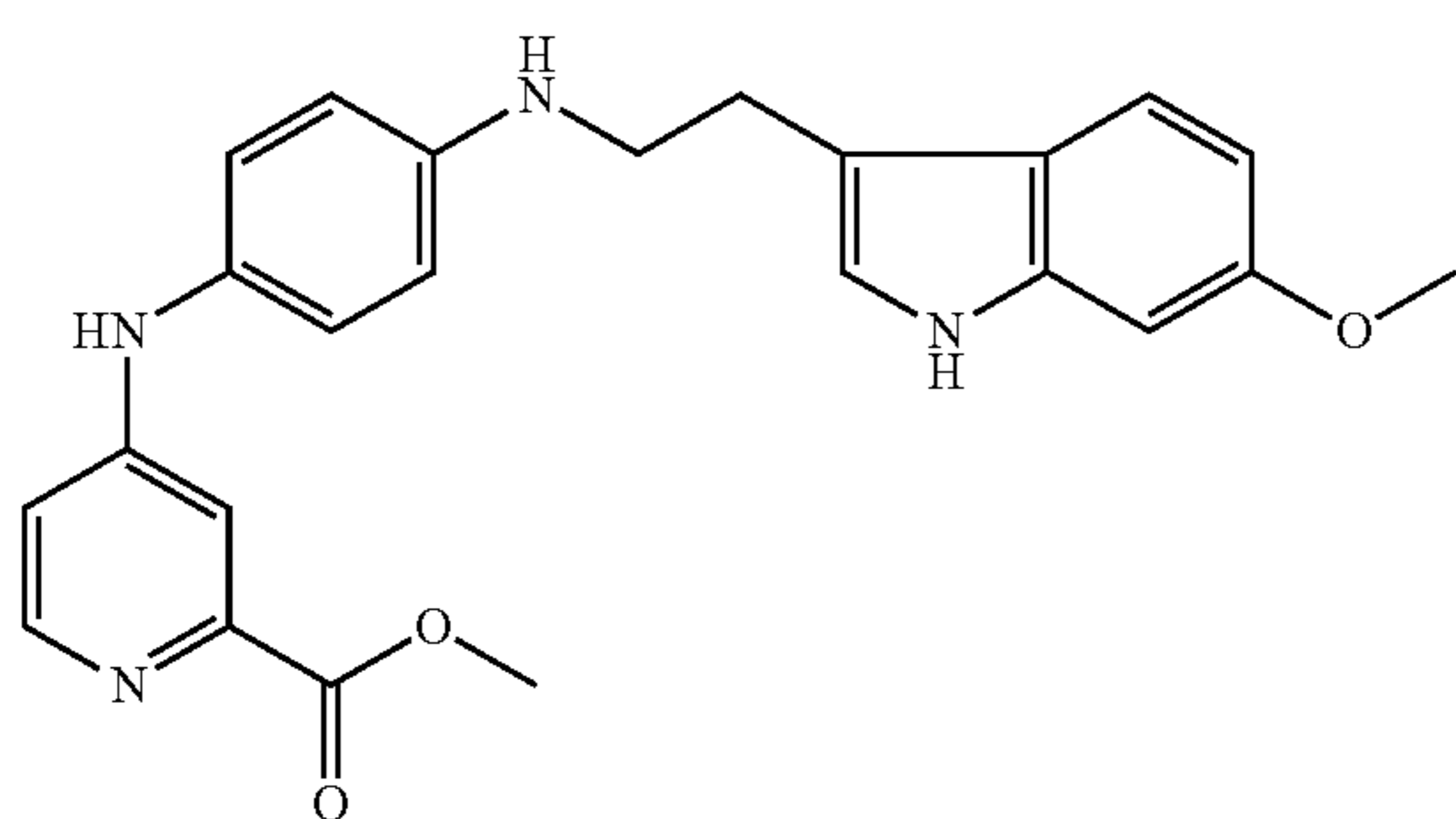
Co. No. 178; ms. 416 Ex. [B2]
