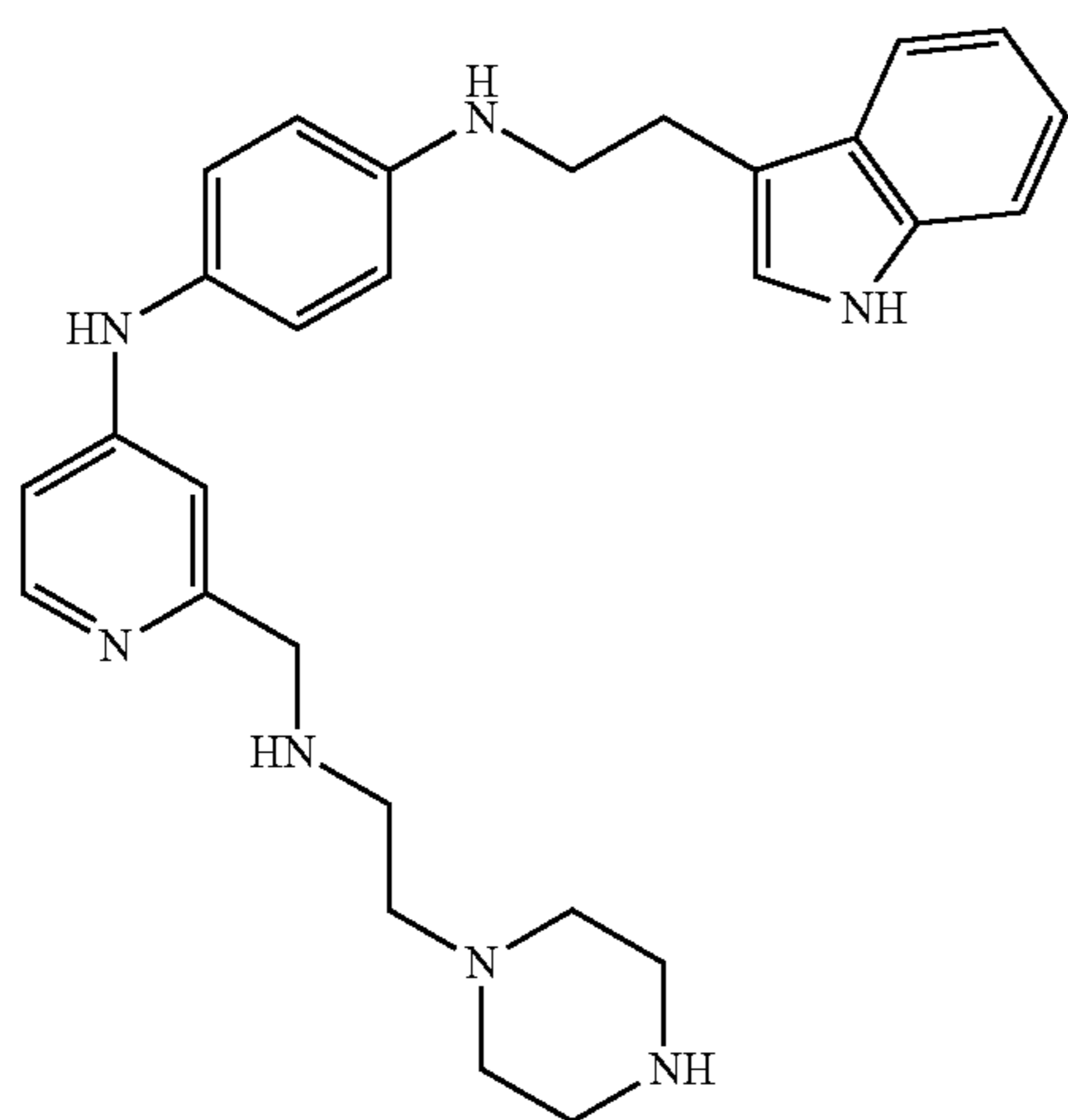
Co. No. 95; ms. 470 Ex. [B21]
