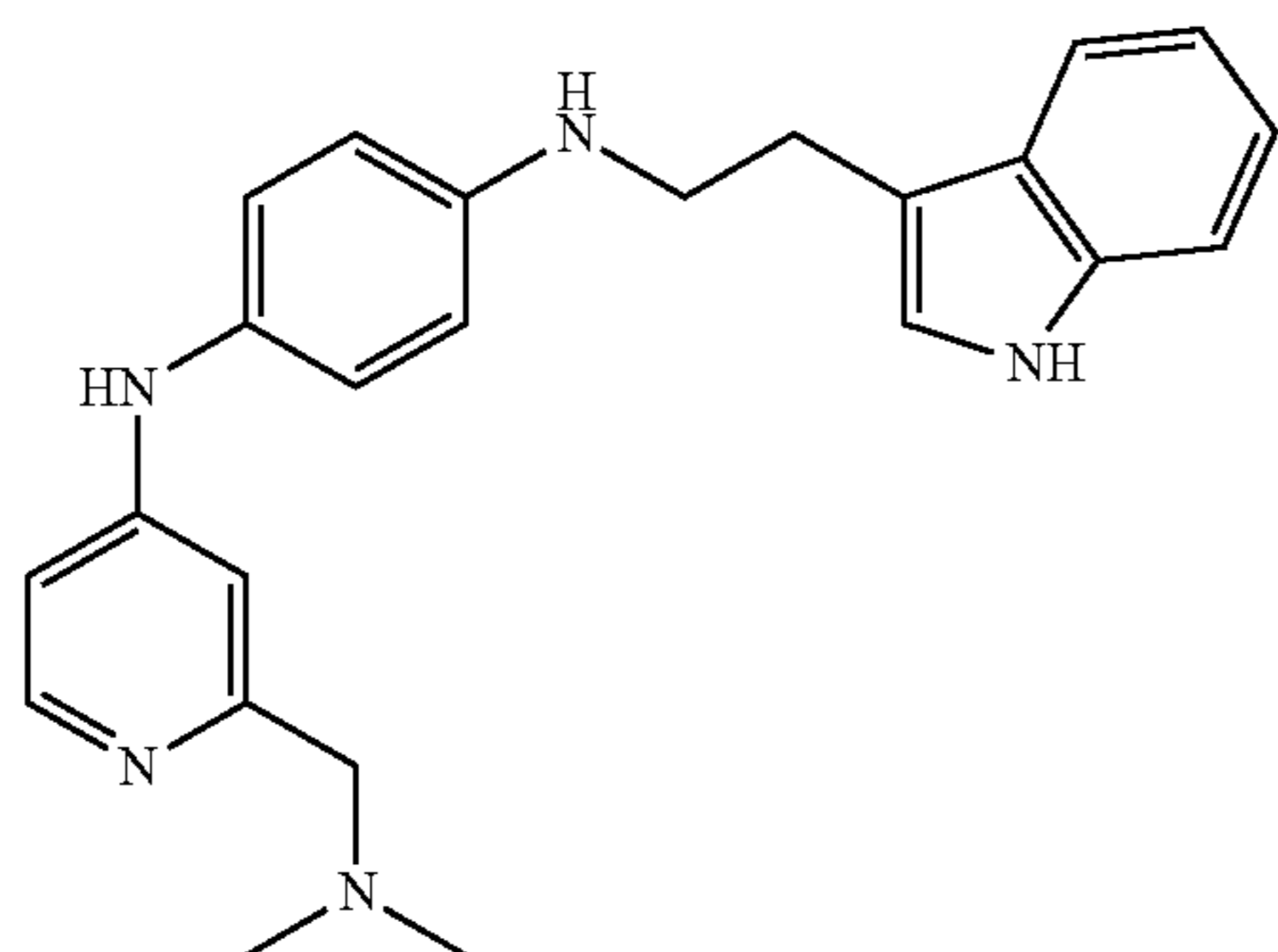
Co. No. 158; ms. 386 Ex. [B12]
