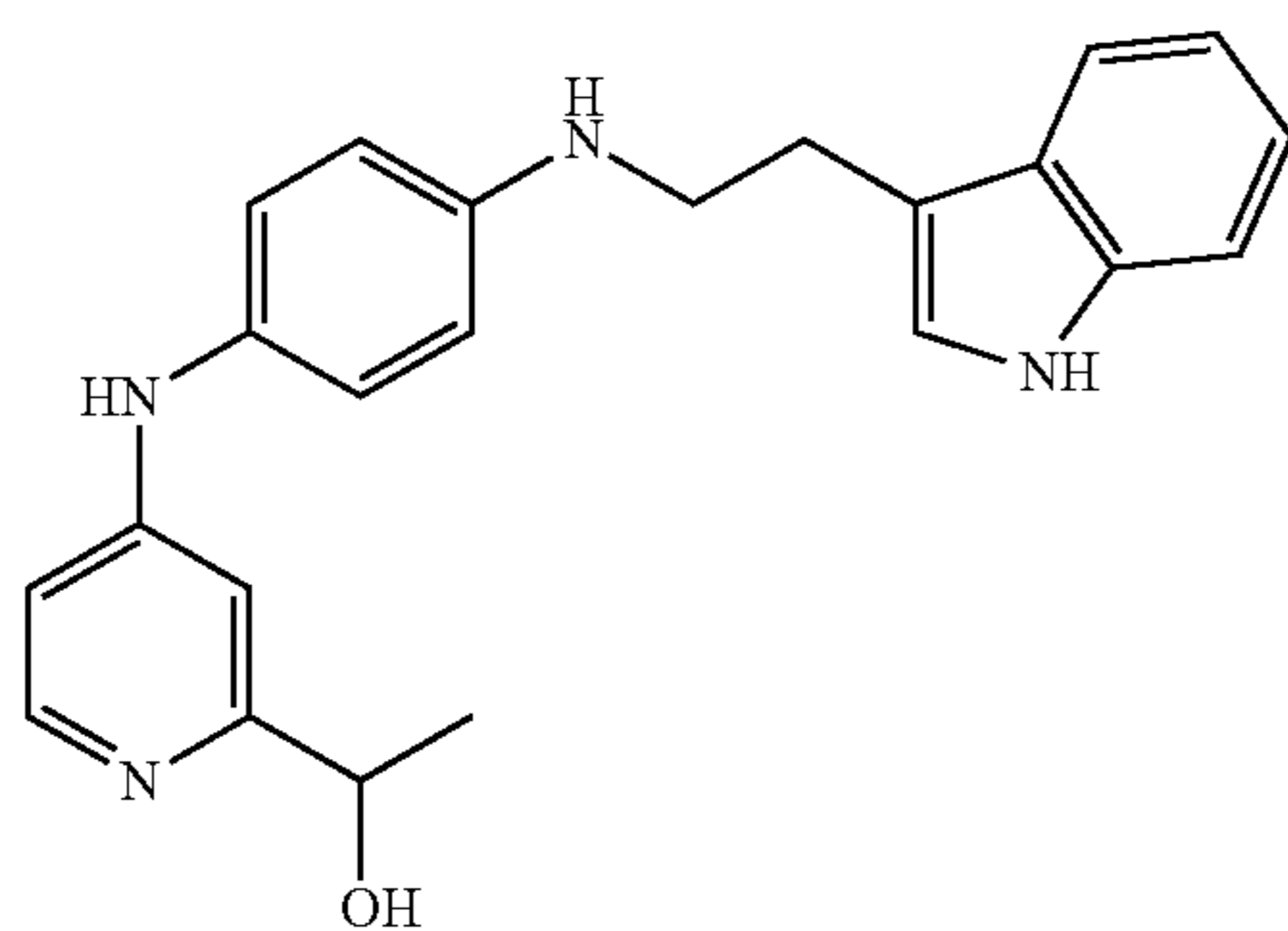
Co. No. 104; ms. 373 Ex. [B30]
