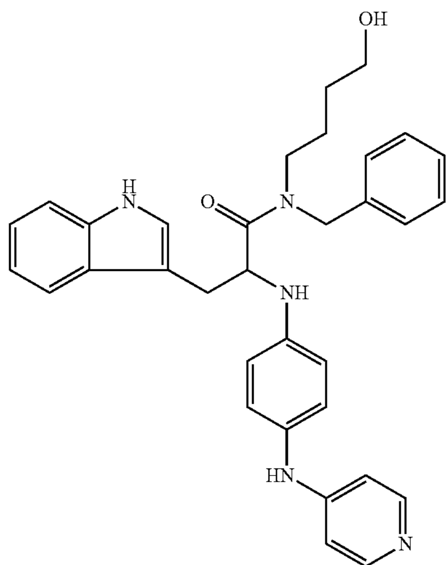
Co. No. 207; ms. 533 Ex. [B45]
