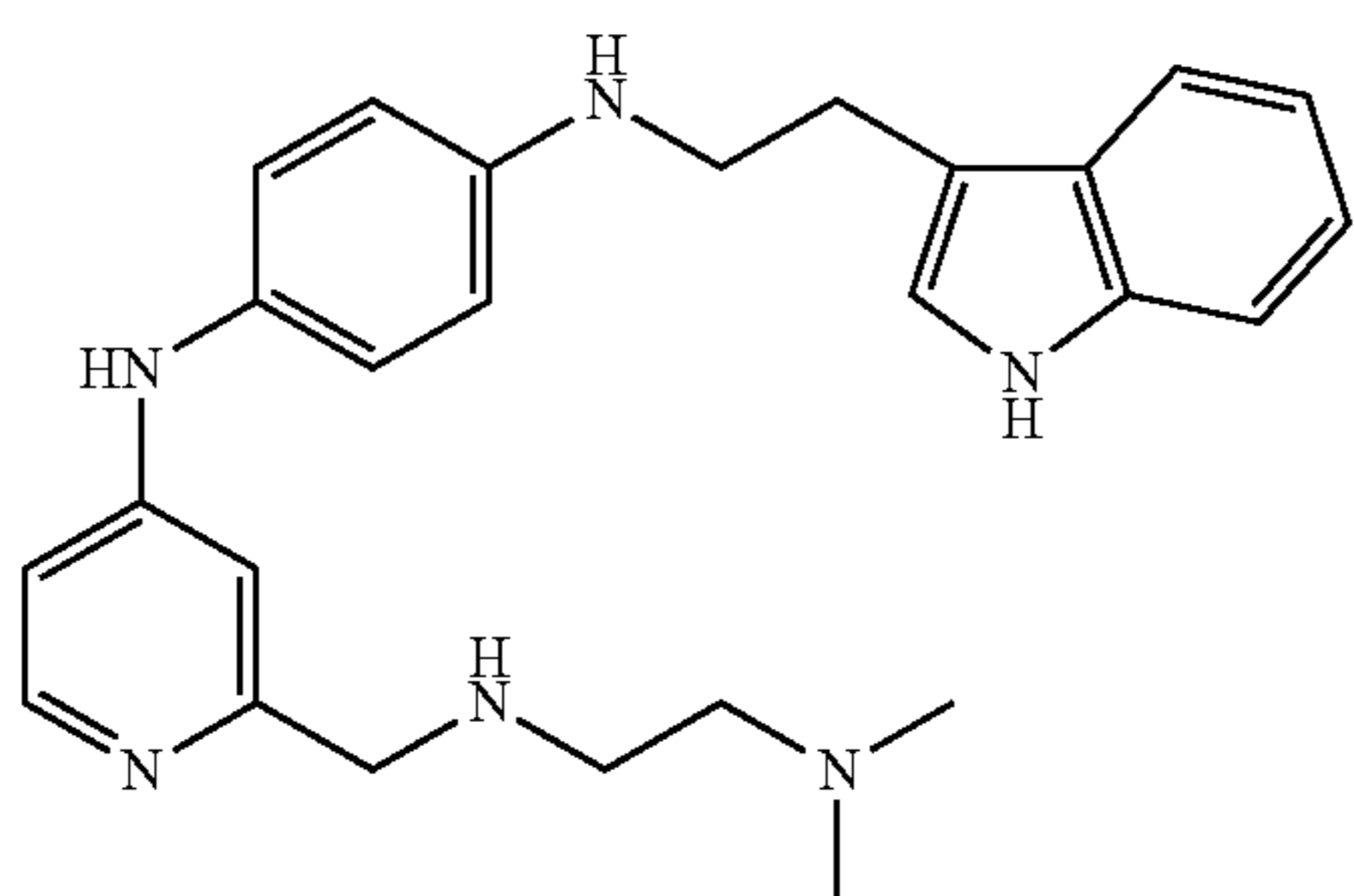
Co. No. 59; mp. 70° C. Ex. [B2]
