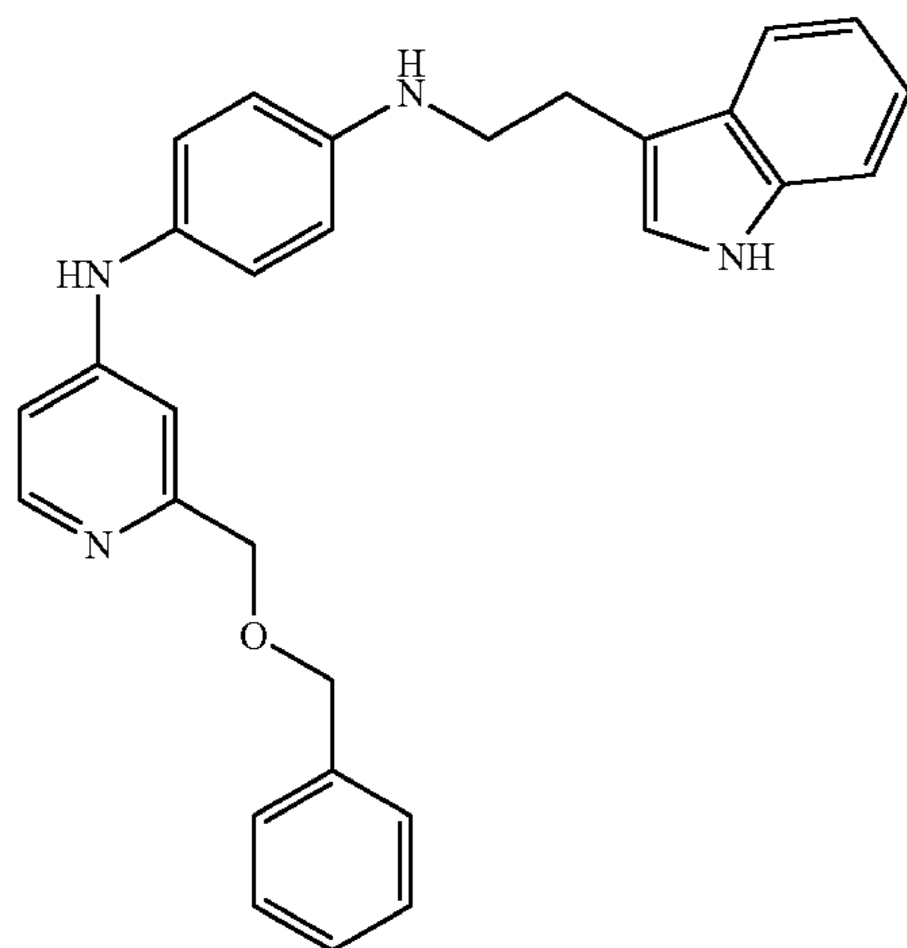
Co. No. 167; ms. 449 Ex. [B12]
