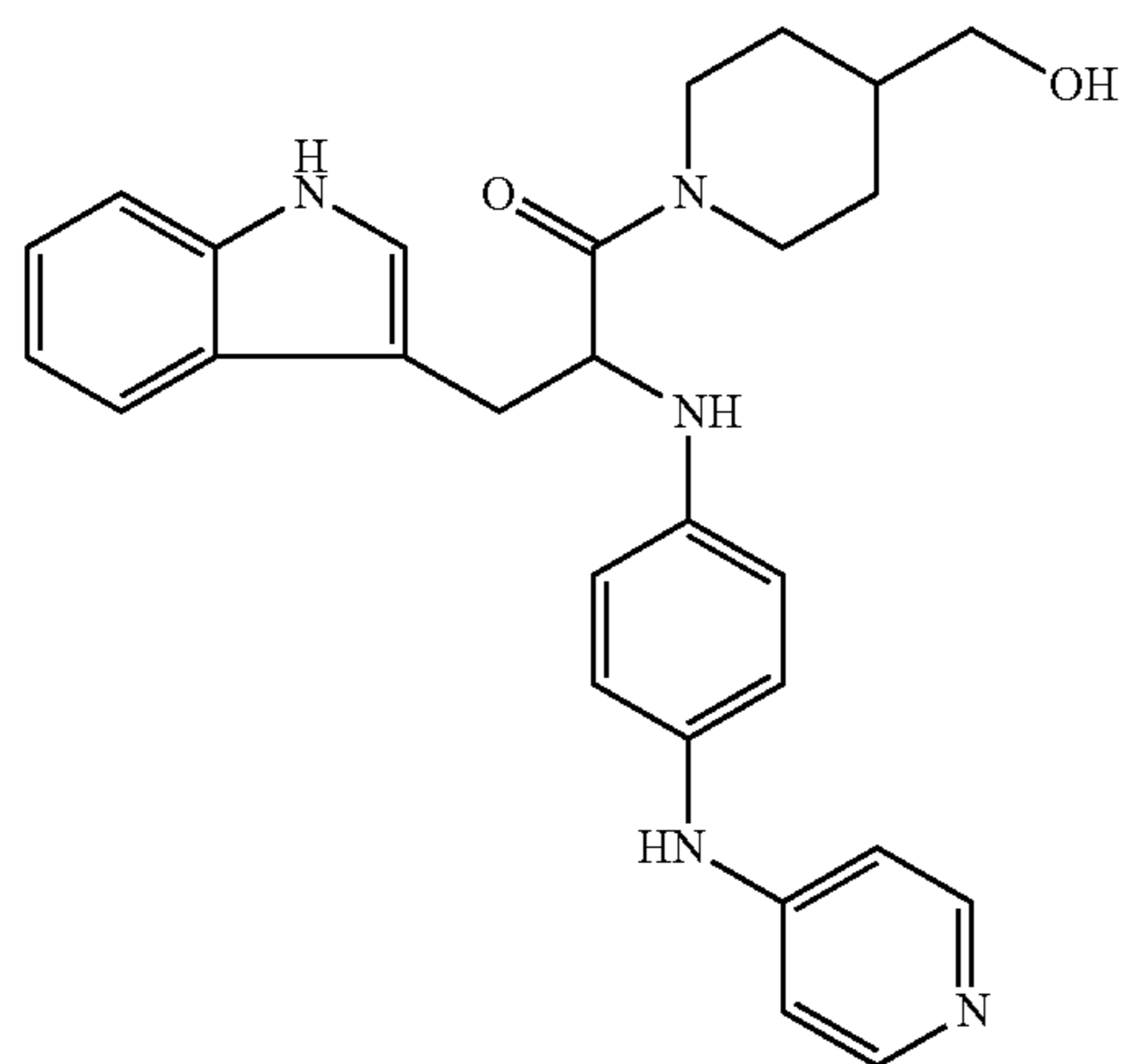
Co. No. 224; ms. 469 Ex. [B45]
