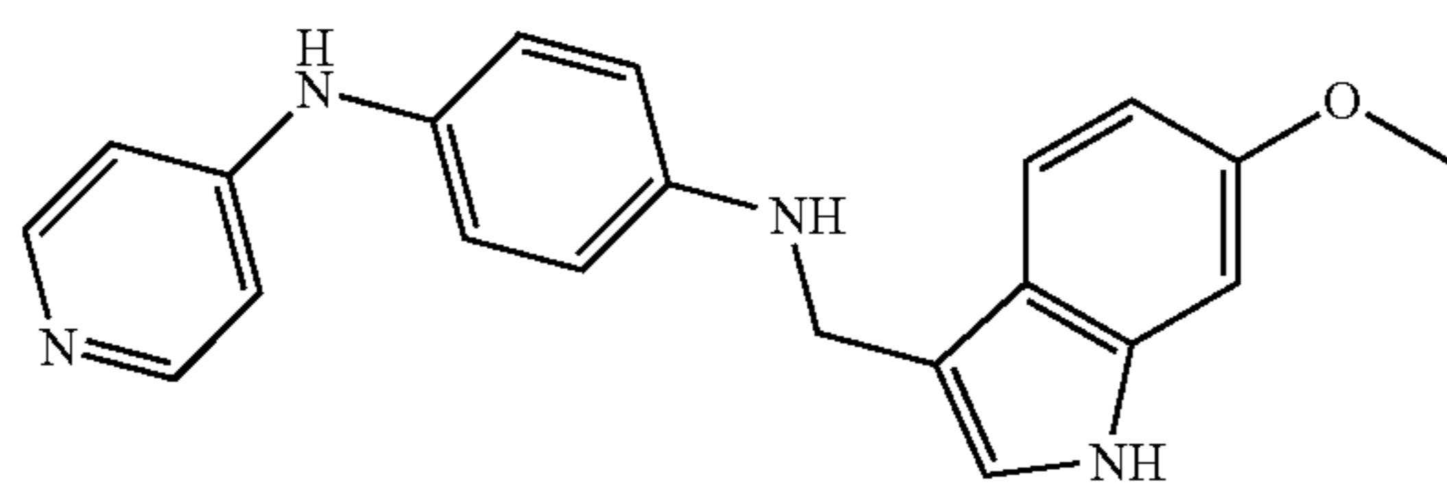
Co. No. 7; mp. 145° C. Ex. [B7]
