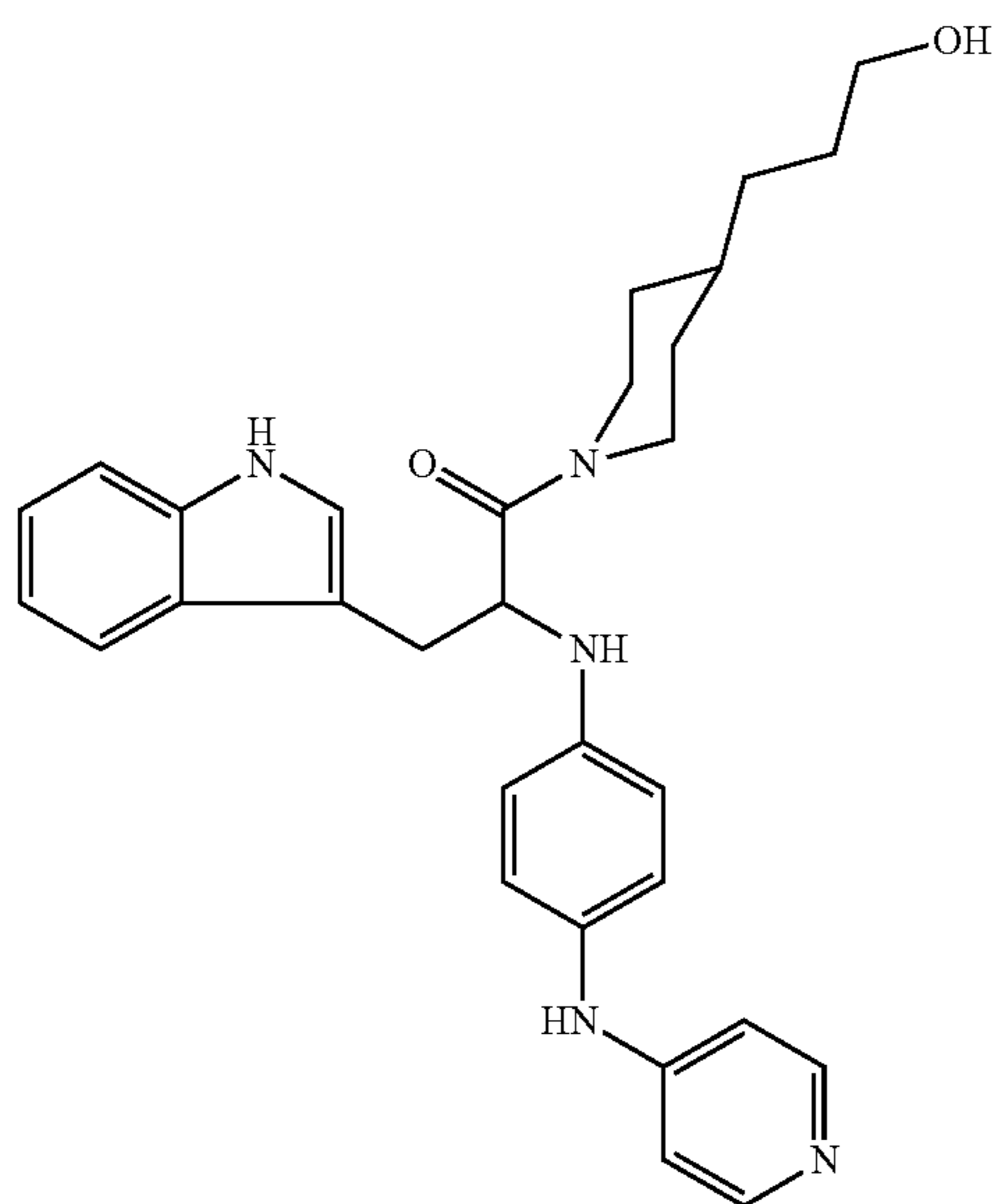
Co. No. 217; ms. 497 Ex. [B45]
