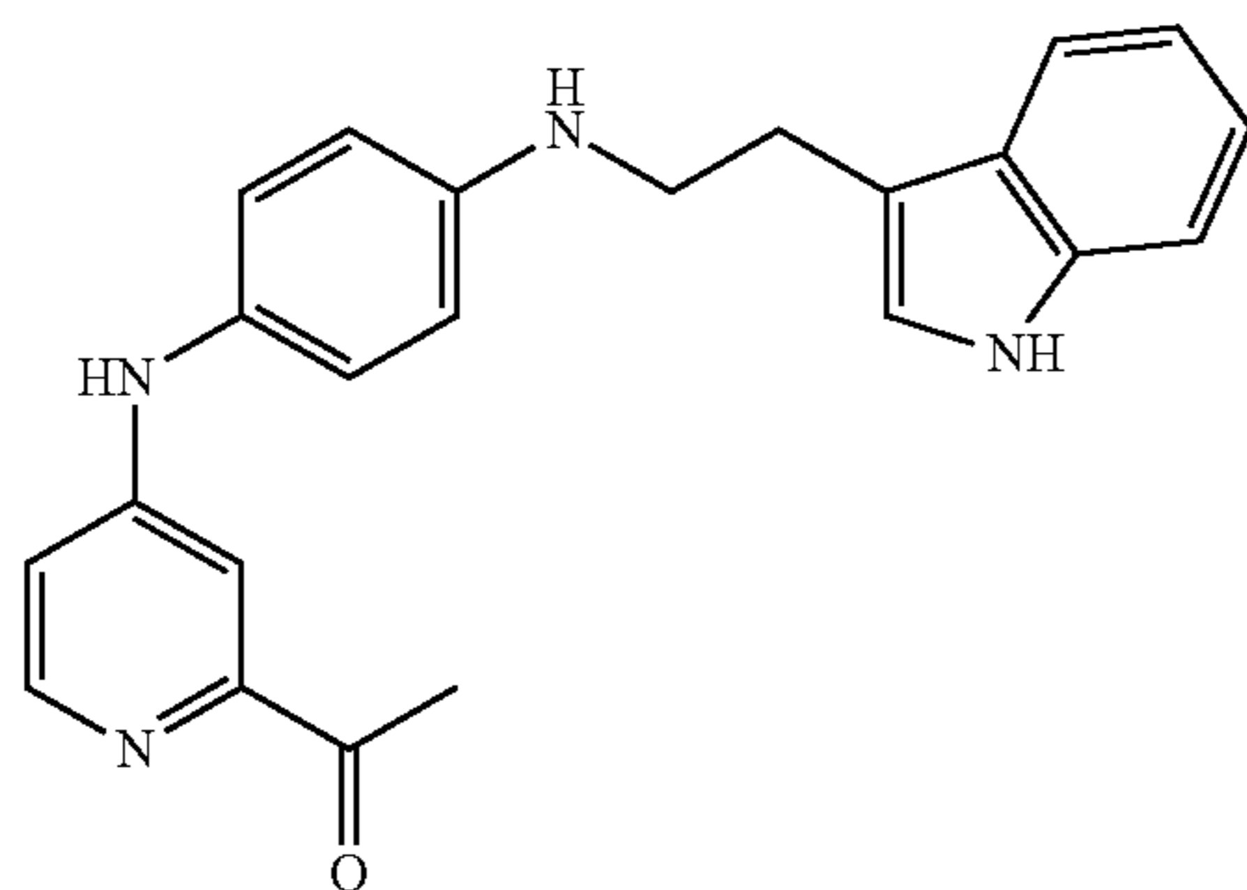
Co. No. 105; ms. 371 Ex. [B31]
