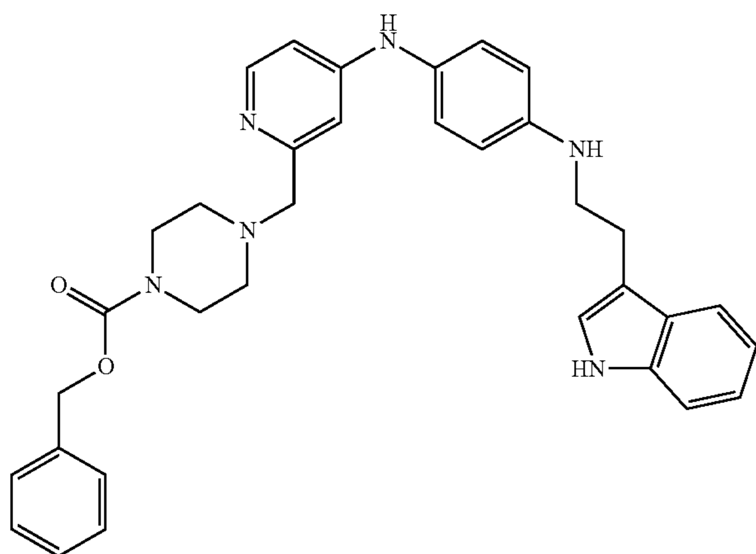
Co. No. 90; ms. 561 Ex. [B16]
