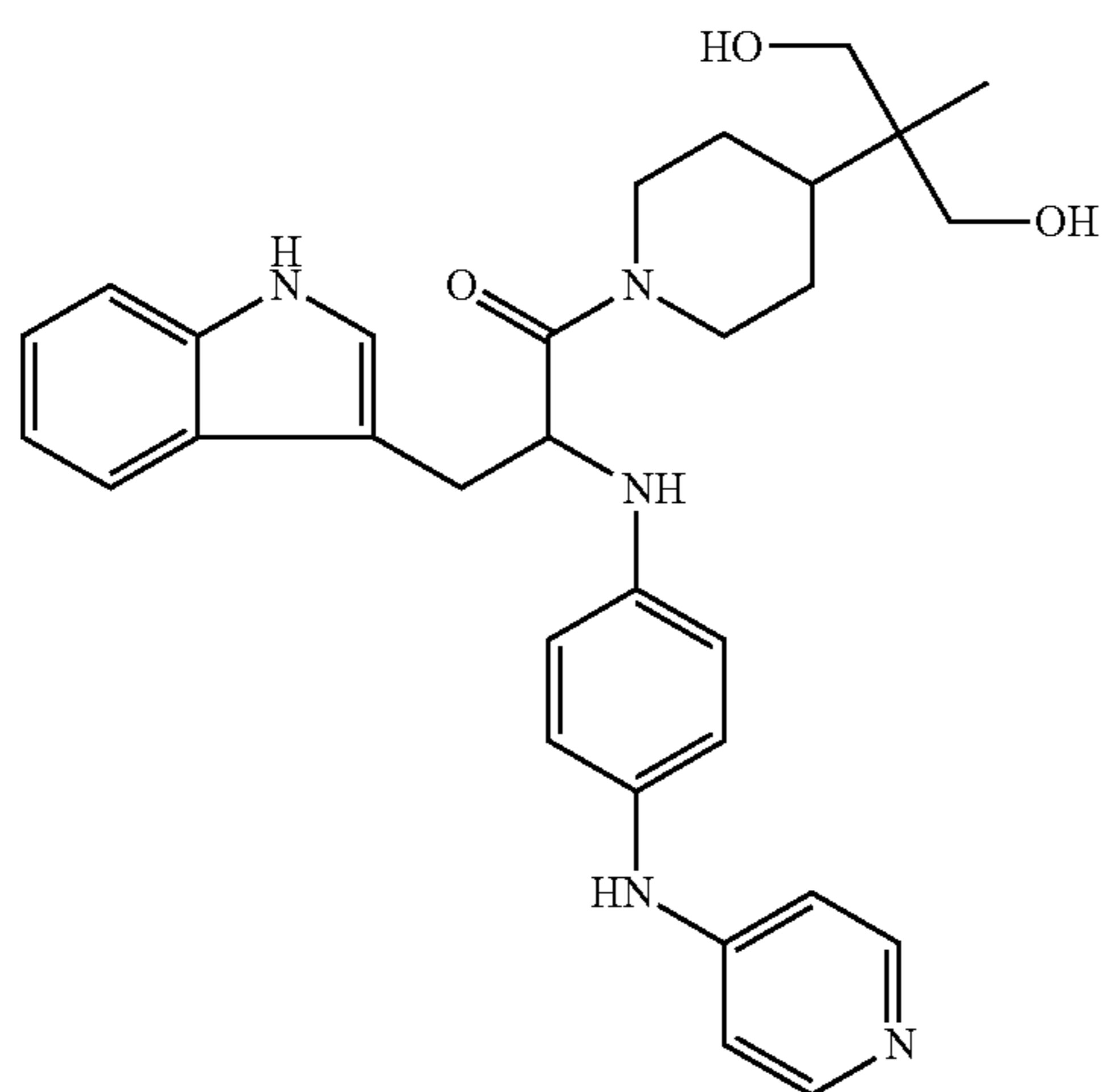
Co. No. 221; ms. 527 Ex. [B45]
