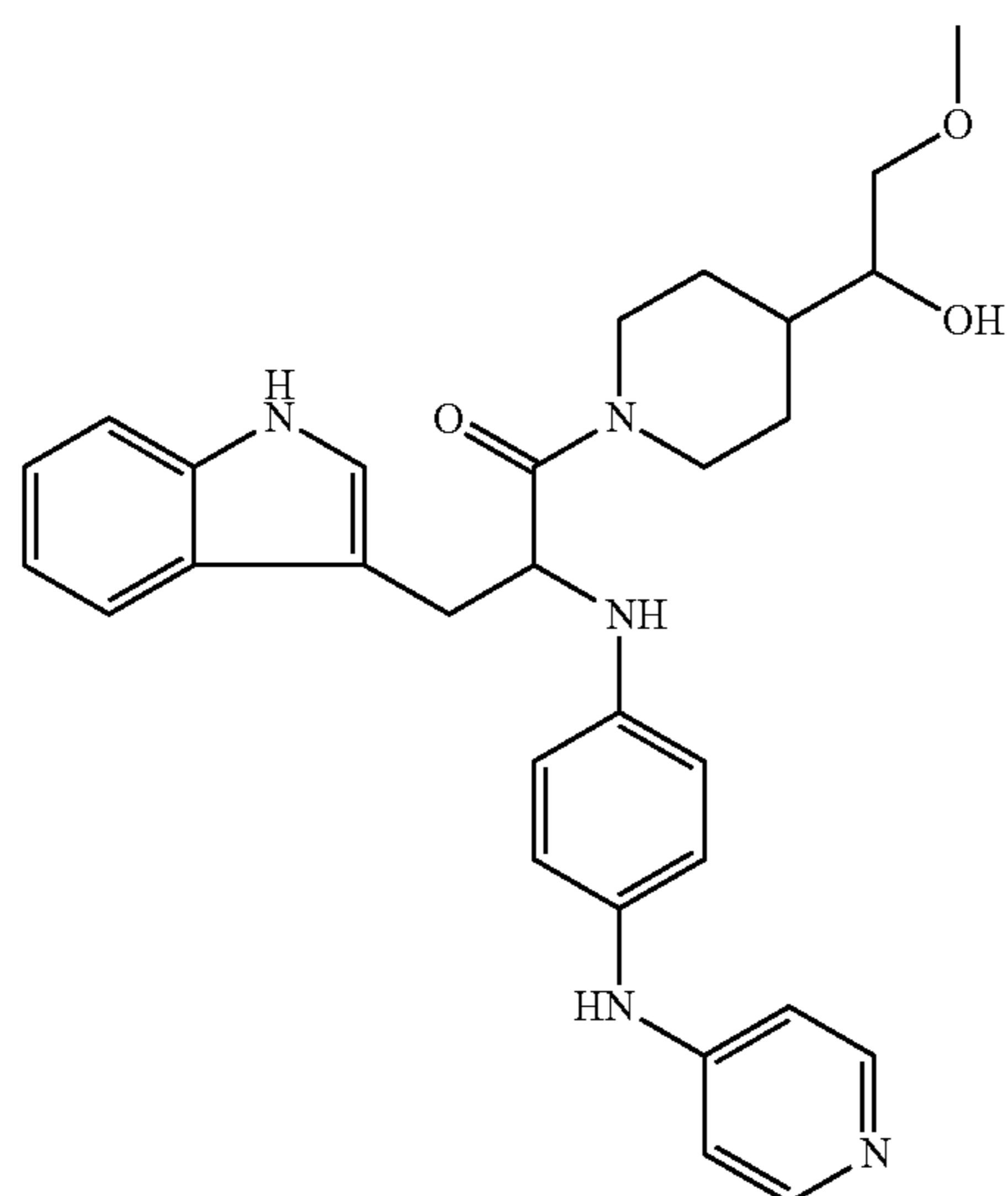
Co. No. 223; ms. 513 Ex. [B45]
