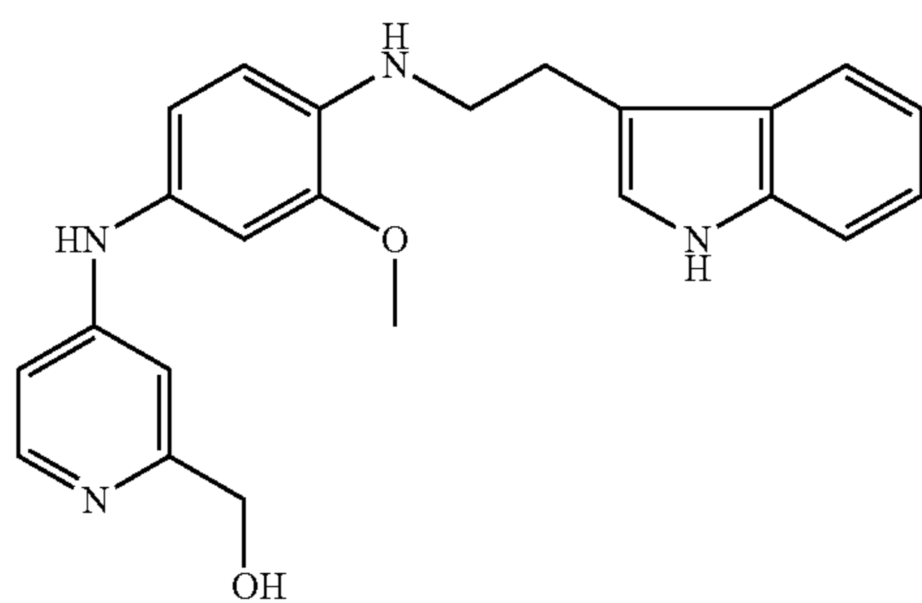
Co. No. 179; ms. 388 Ex. [B2]
