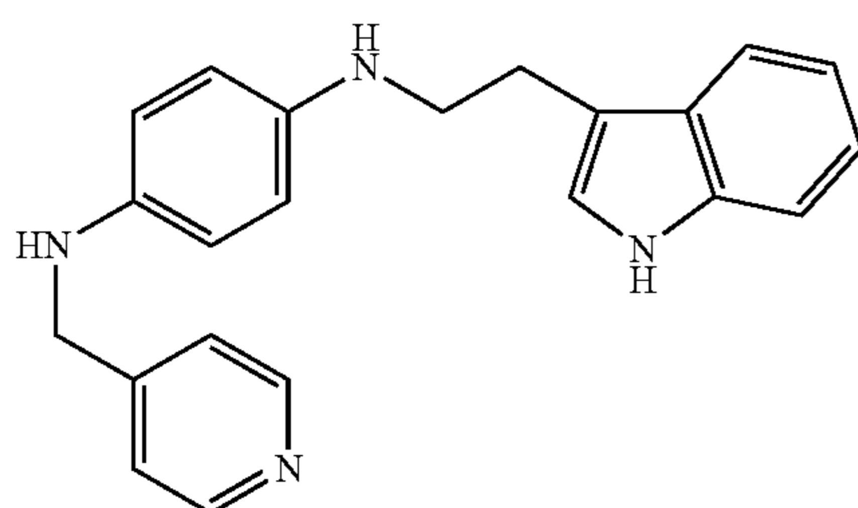
Co. No. 9; mp. 132° C. Ex. [B9]
