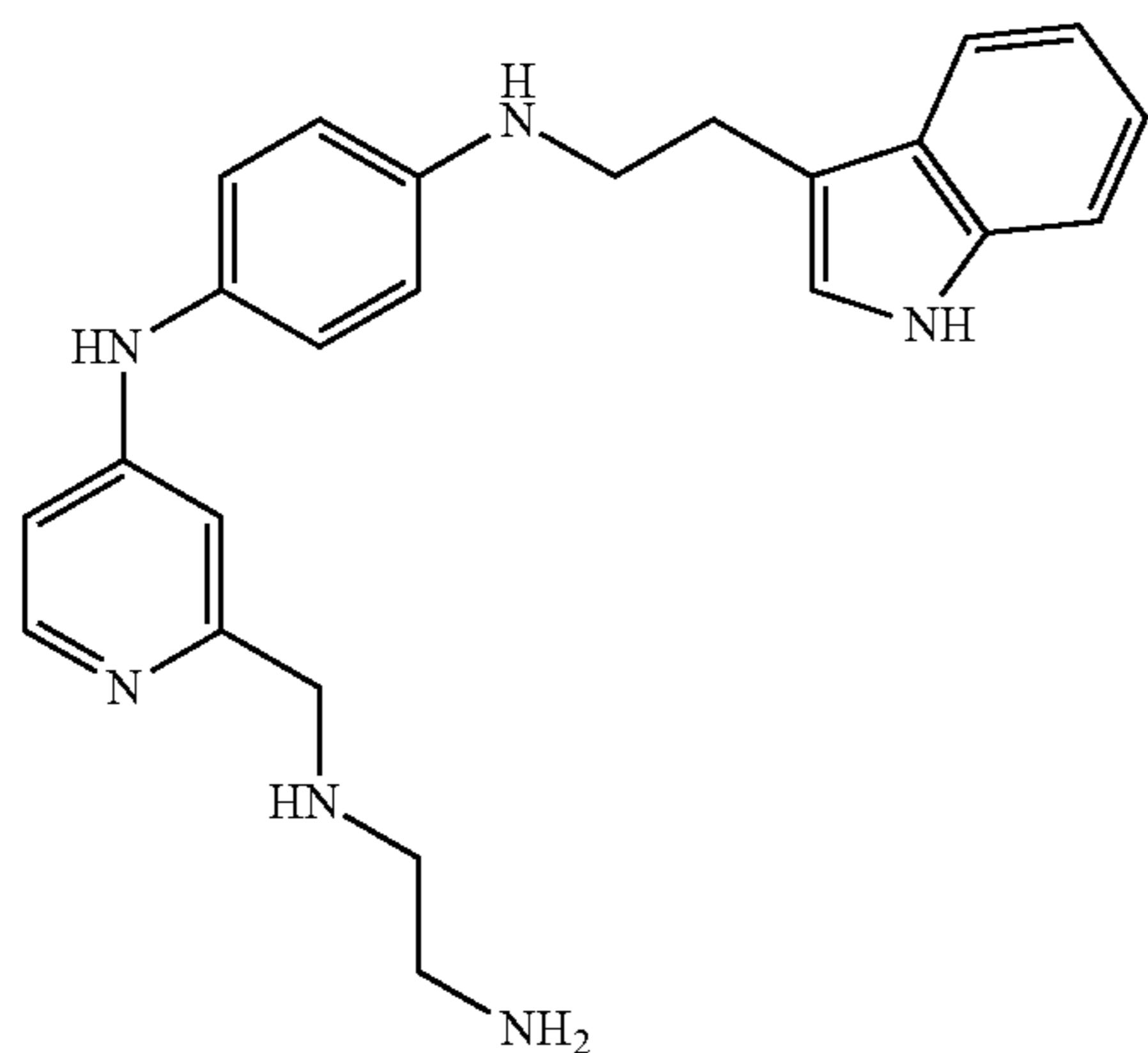
Co. No. 93; ms. 401 Ex. [B19]
