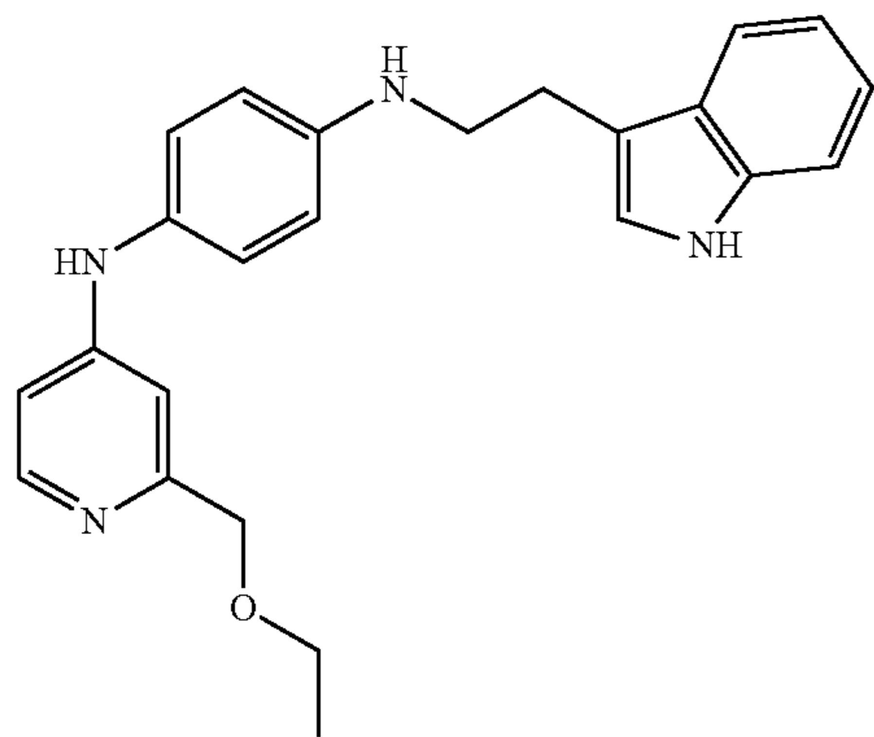
Co. No. 134; ms. 387 Ex. [B12]
