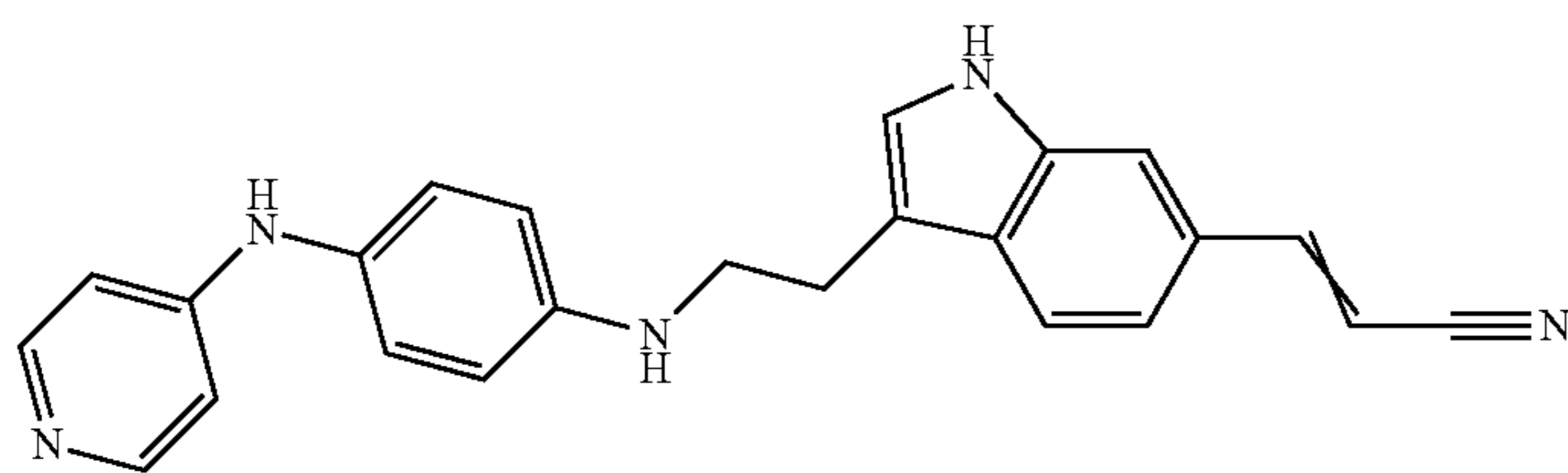
Co. No. 194; E/Z mixture (80/20) Ex. [B2]
