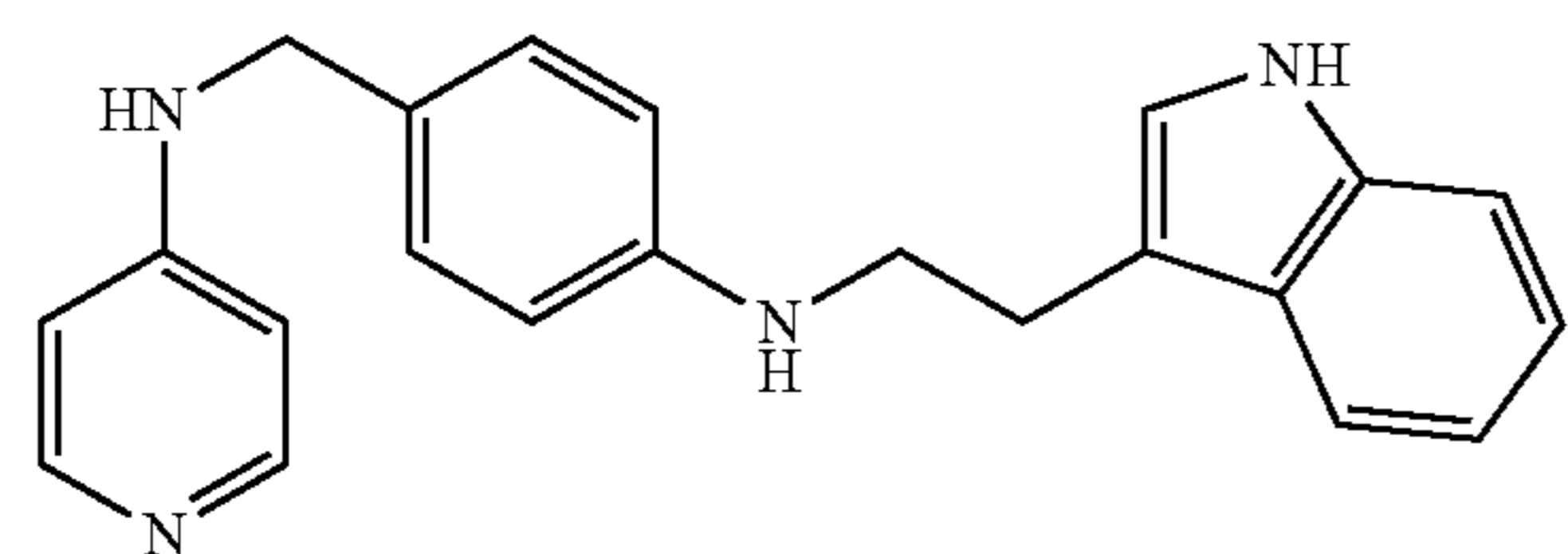
Co. No. 11; mp. 122° C. Ex. [B11]
