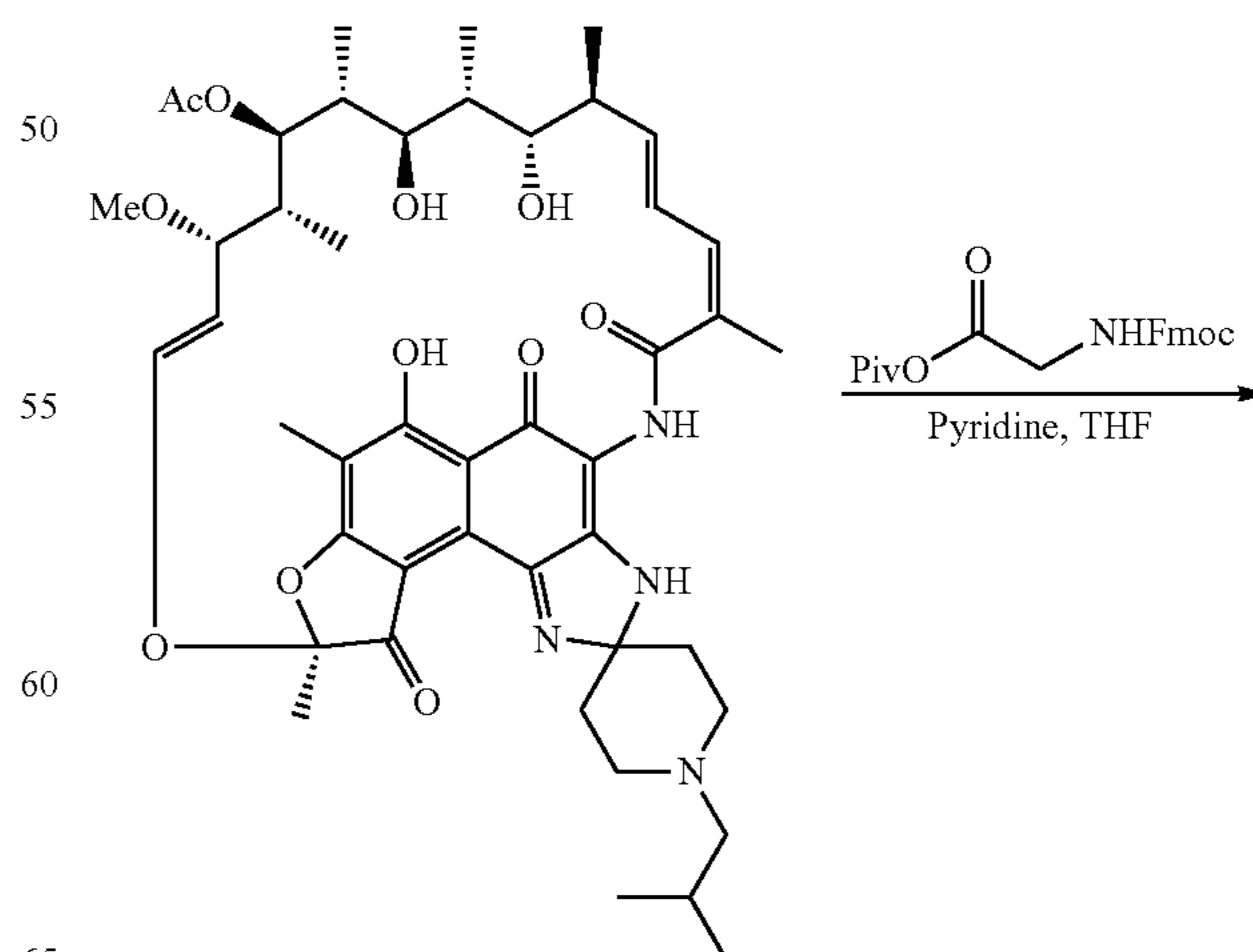
Scheme 5. Synthesis of rifabutin-bisphosphonate conjugate 21
