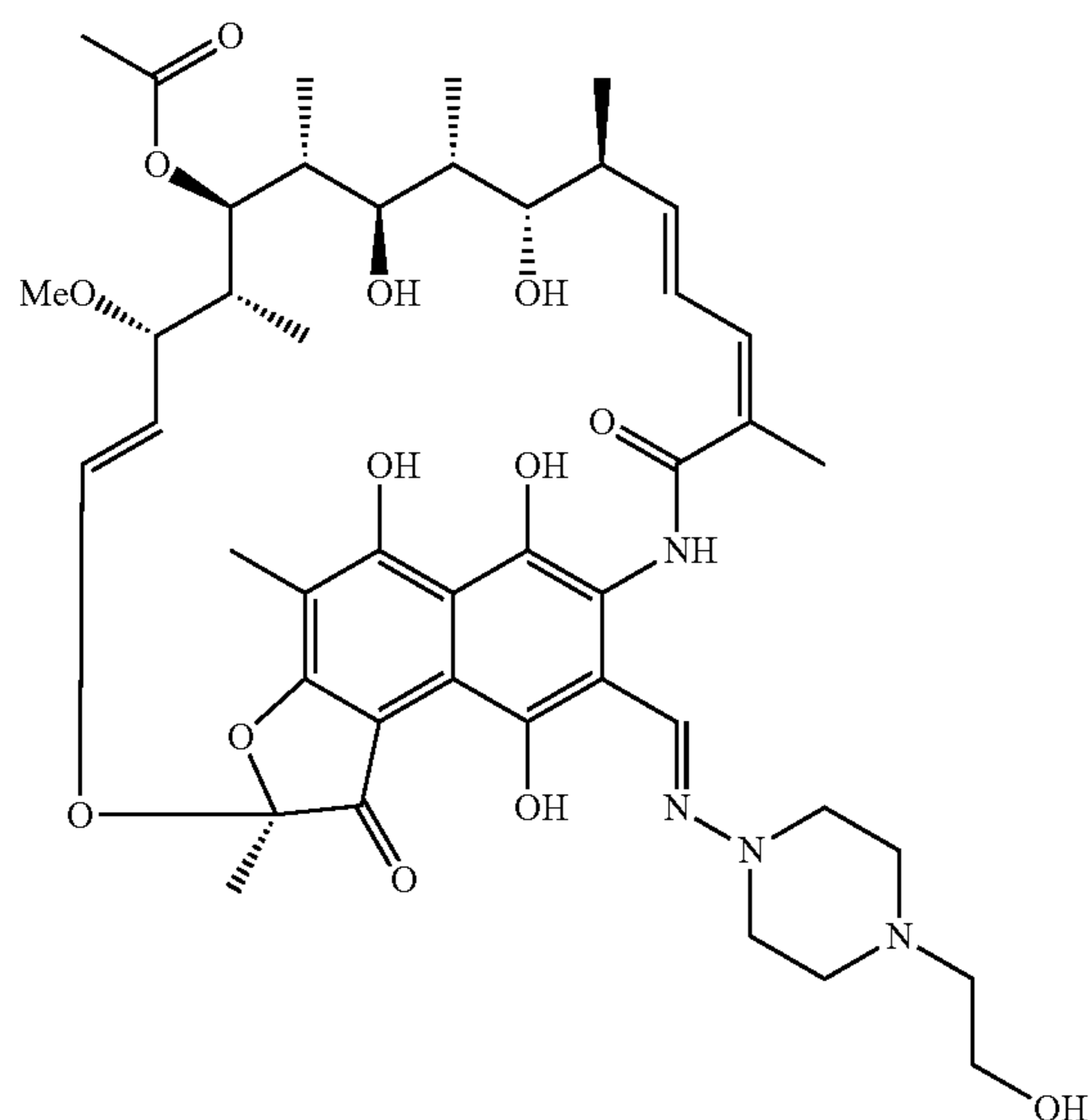
Rifamycin derivative
