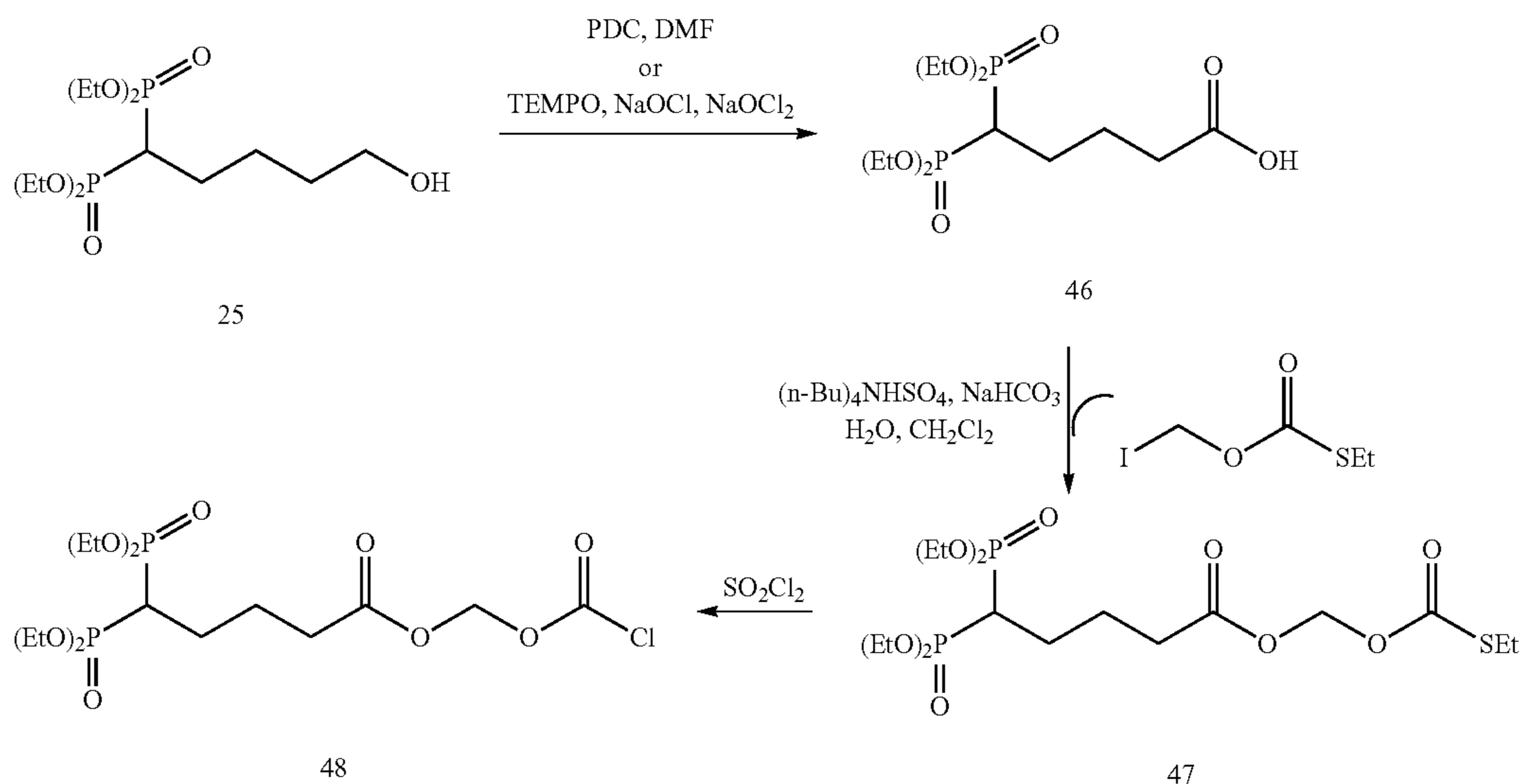
Scheme 13. Preparation of (carbonochloridoxy)methyl 5,5-bis(diethylphosphono)pentanoate
