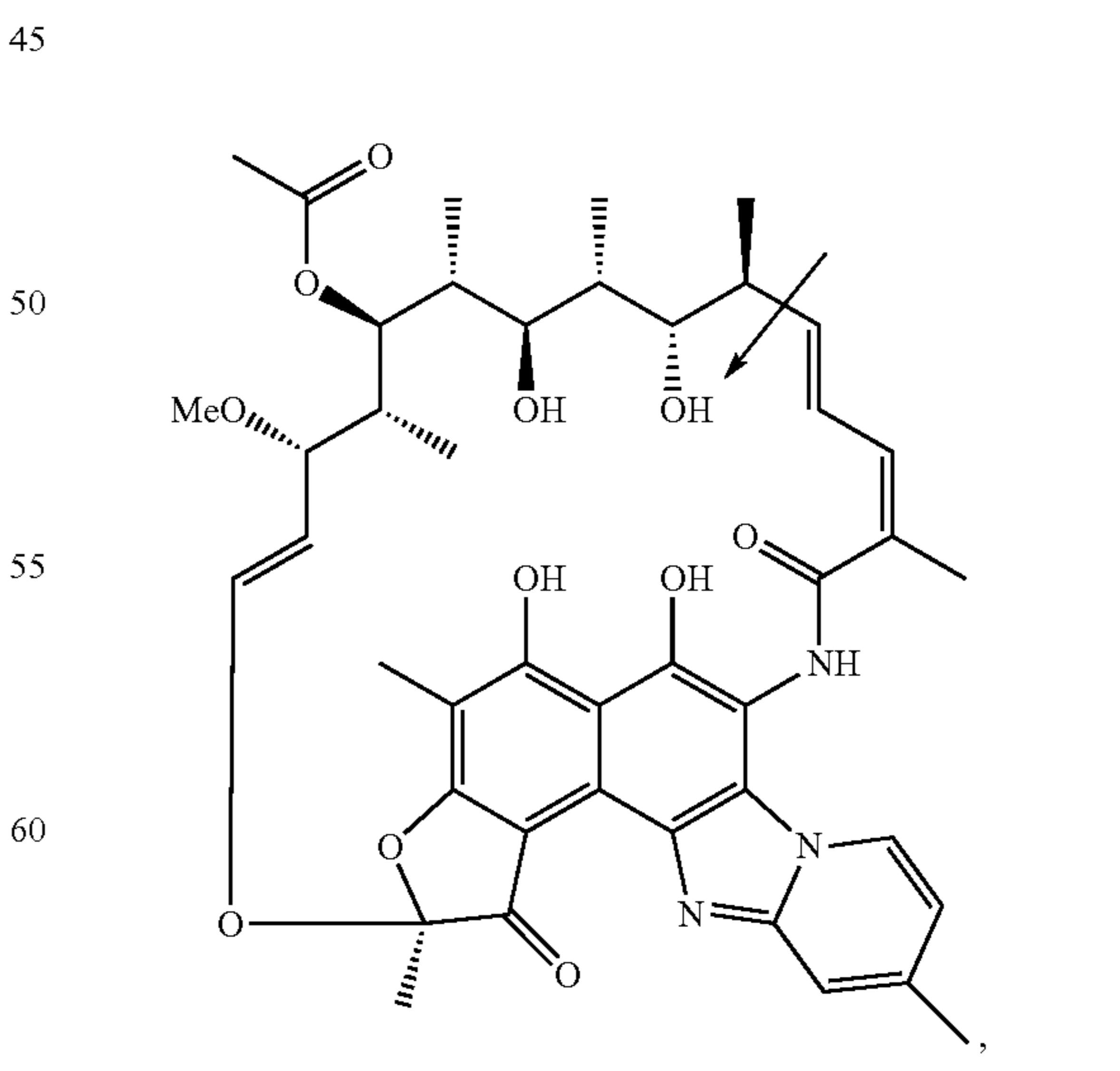
Rifamixin
