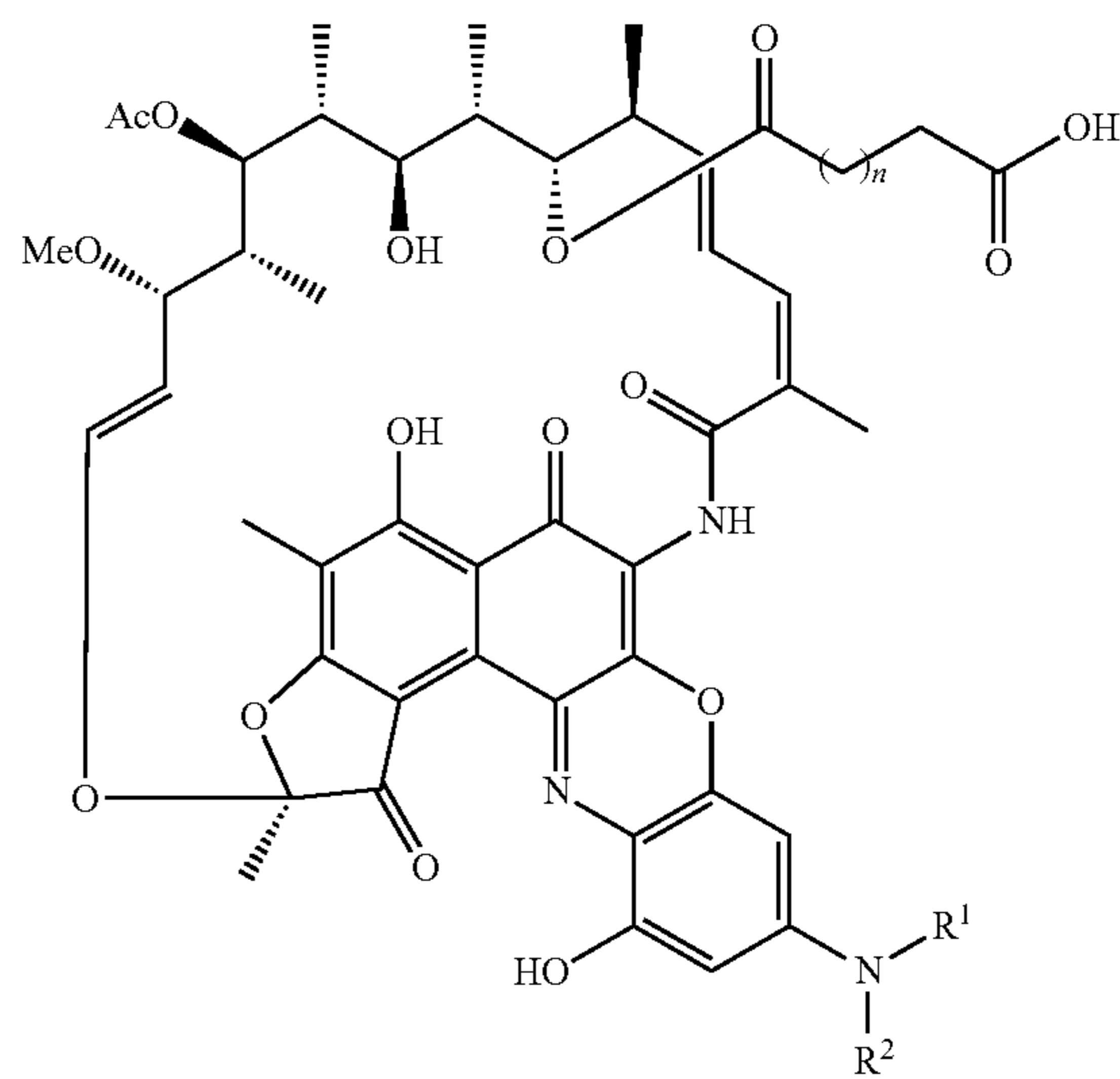
LVIIa n = 1 LVIIb n = 2
