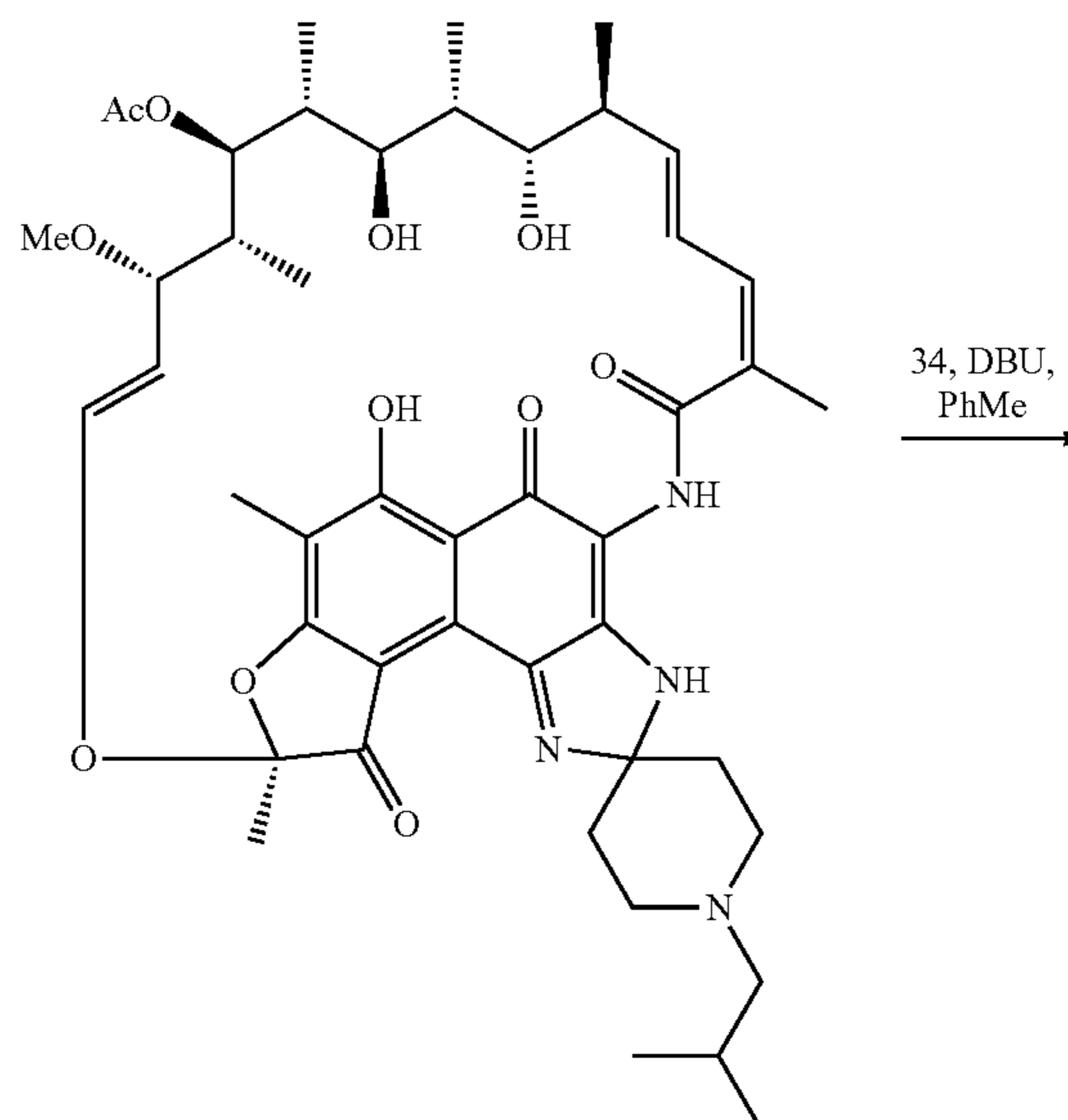
Scheme 9. Preparation of Rifabutin bisphosphonate conjugate 36.
