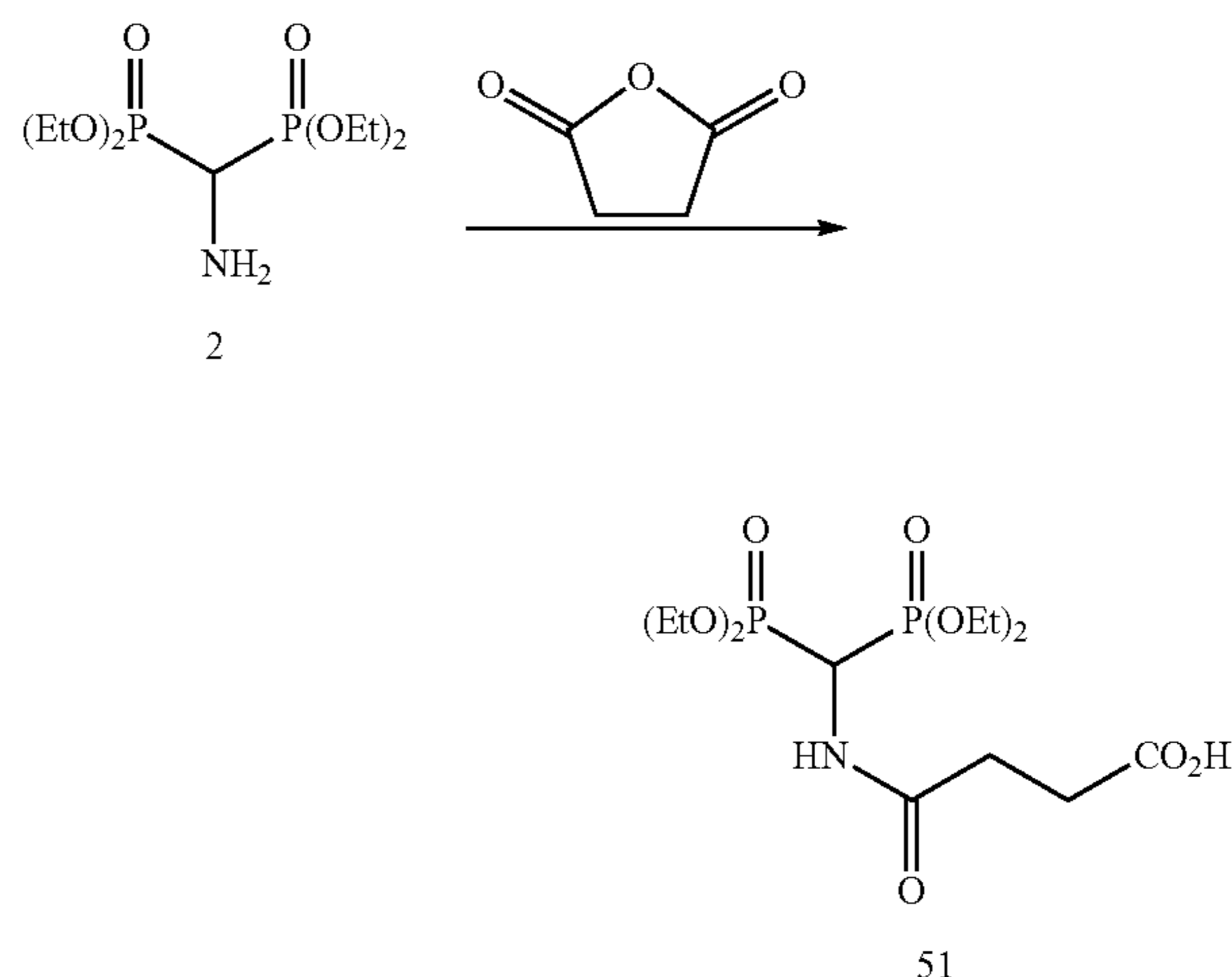
Scheme 15. Preparation of 3-[(tetraethylbisphosphonomethyl)carbamoyl]propanoic acid
