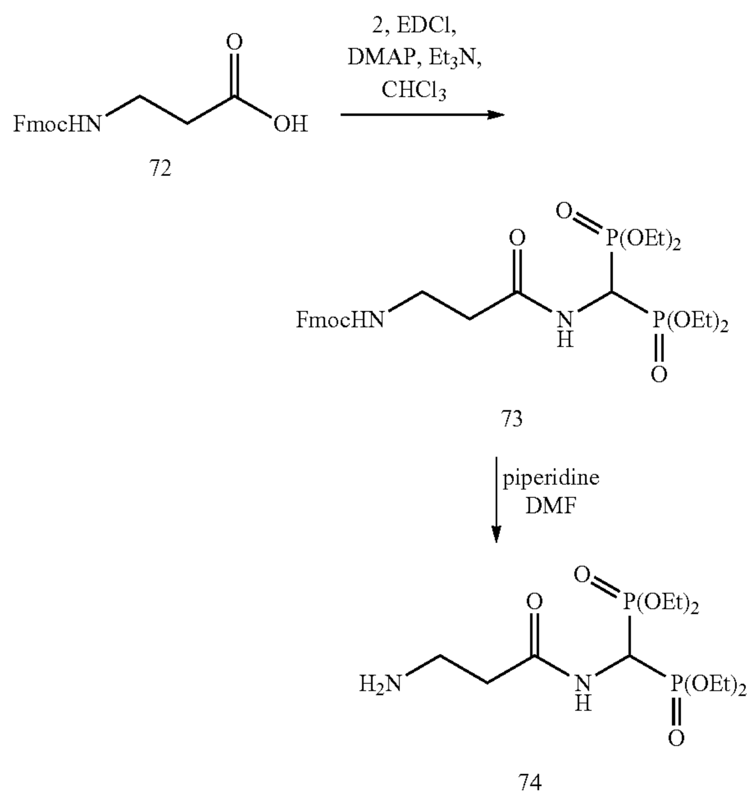
Scheme 25. Preparation of tetraethyl (3-aminopropanoylamino)methylene-1,1-bisphosphonate
