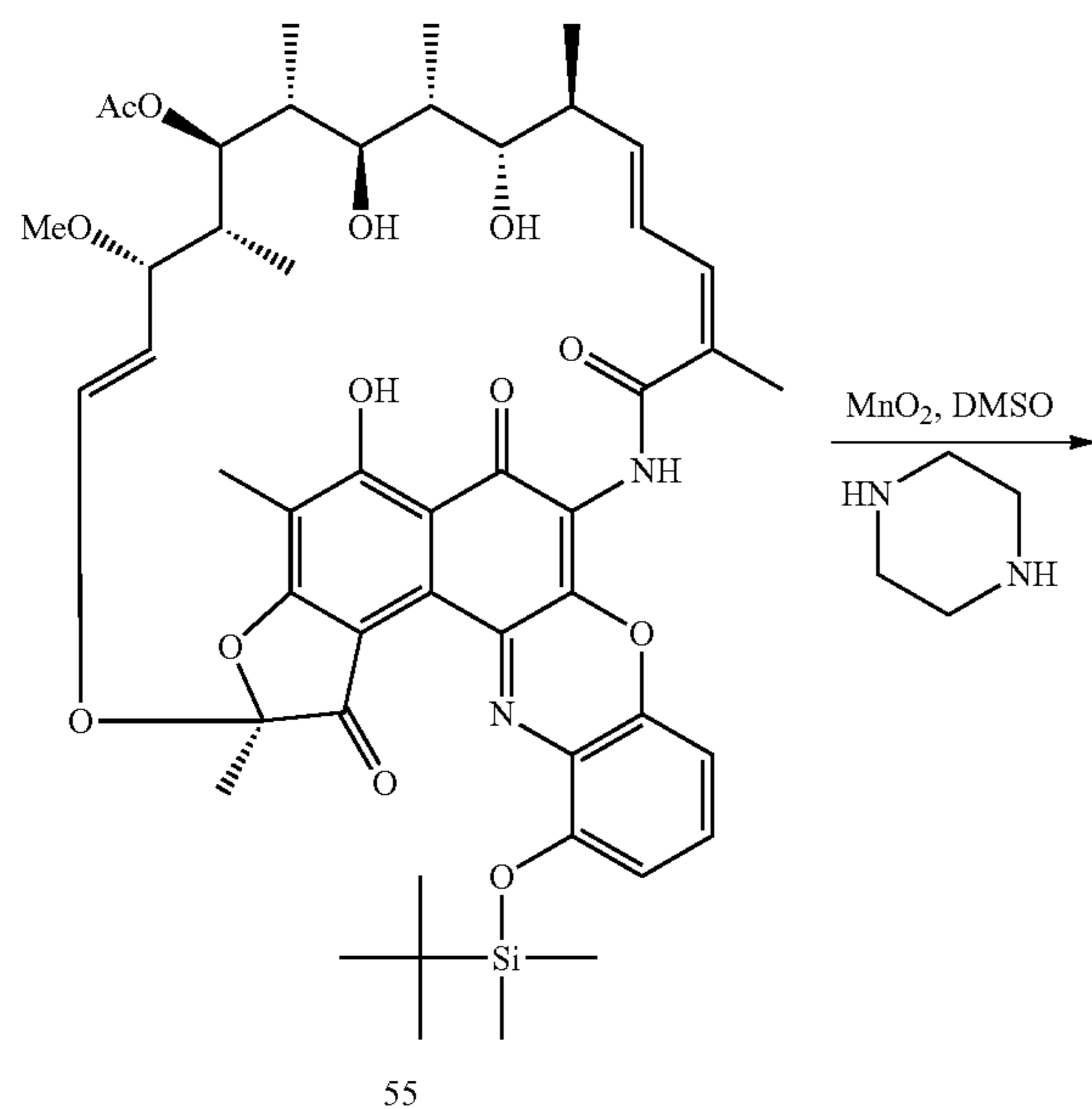
Scheme 23. Preparation of 3'-hydroxybenzoxazinorifamycin derivative 69.
