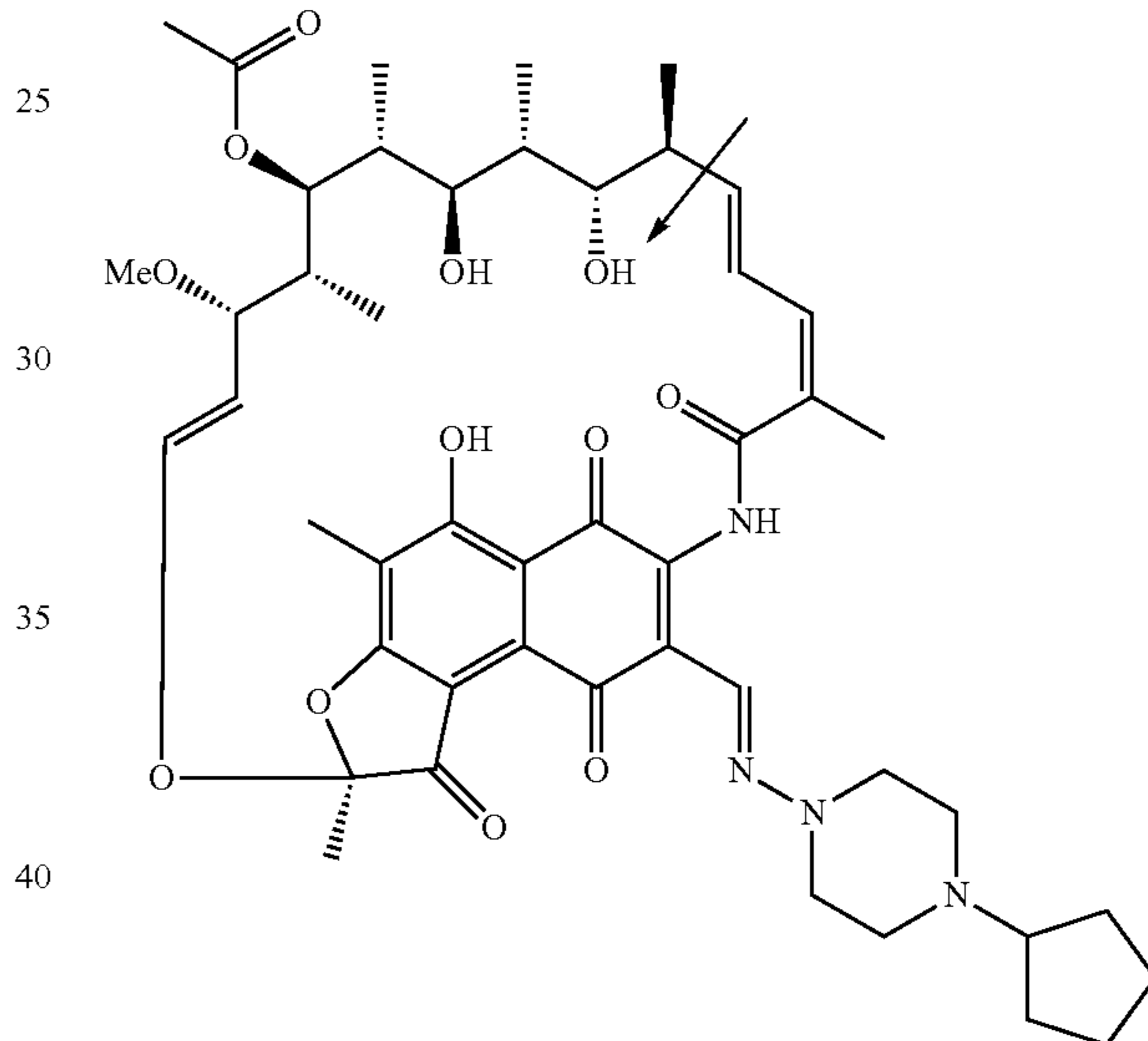
Rifapentin quinone form
