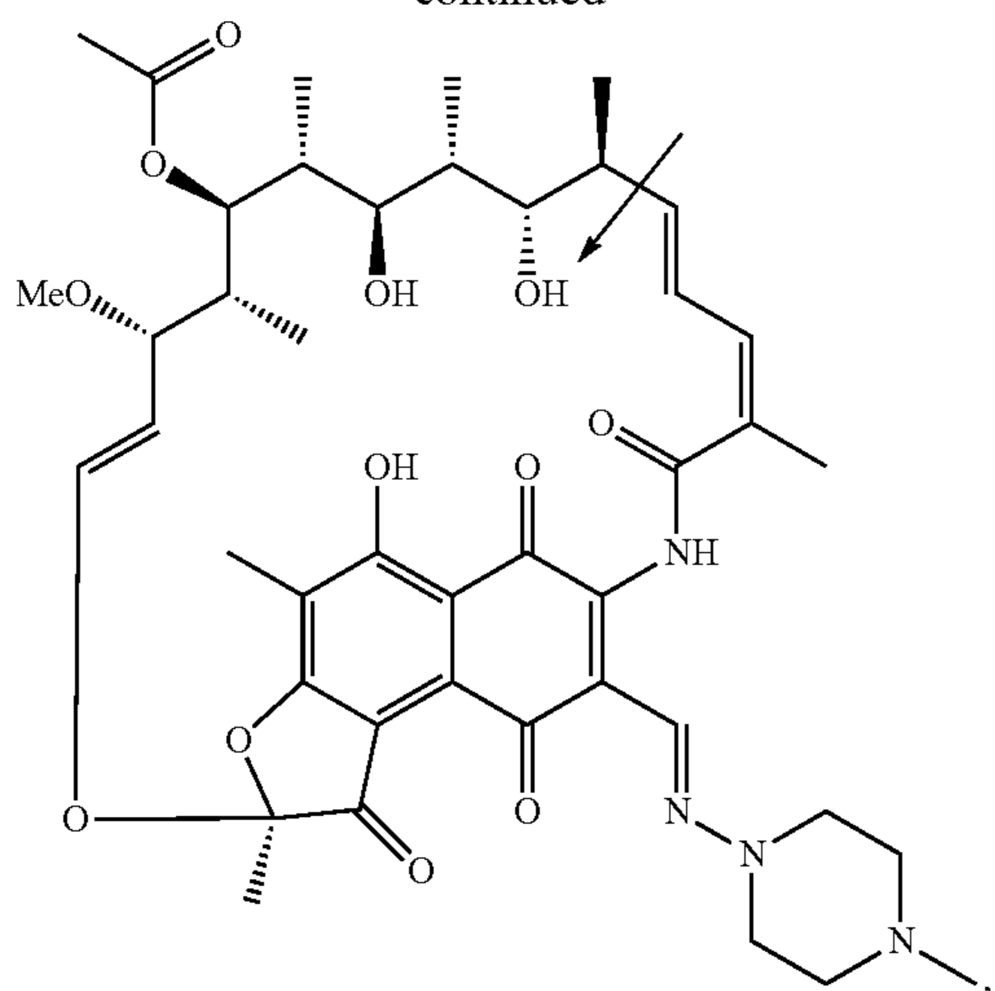
Rifampicin quinone form
