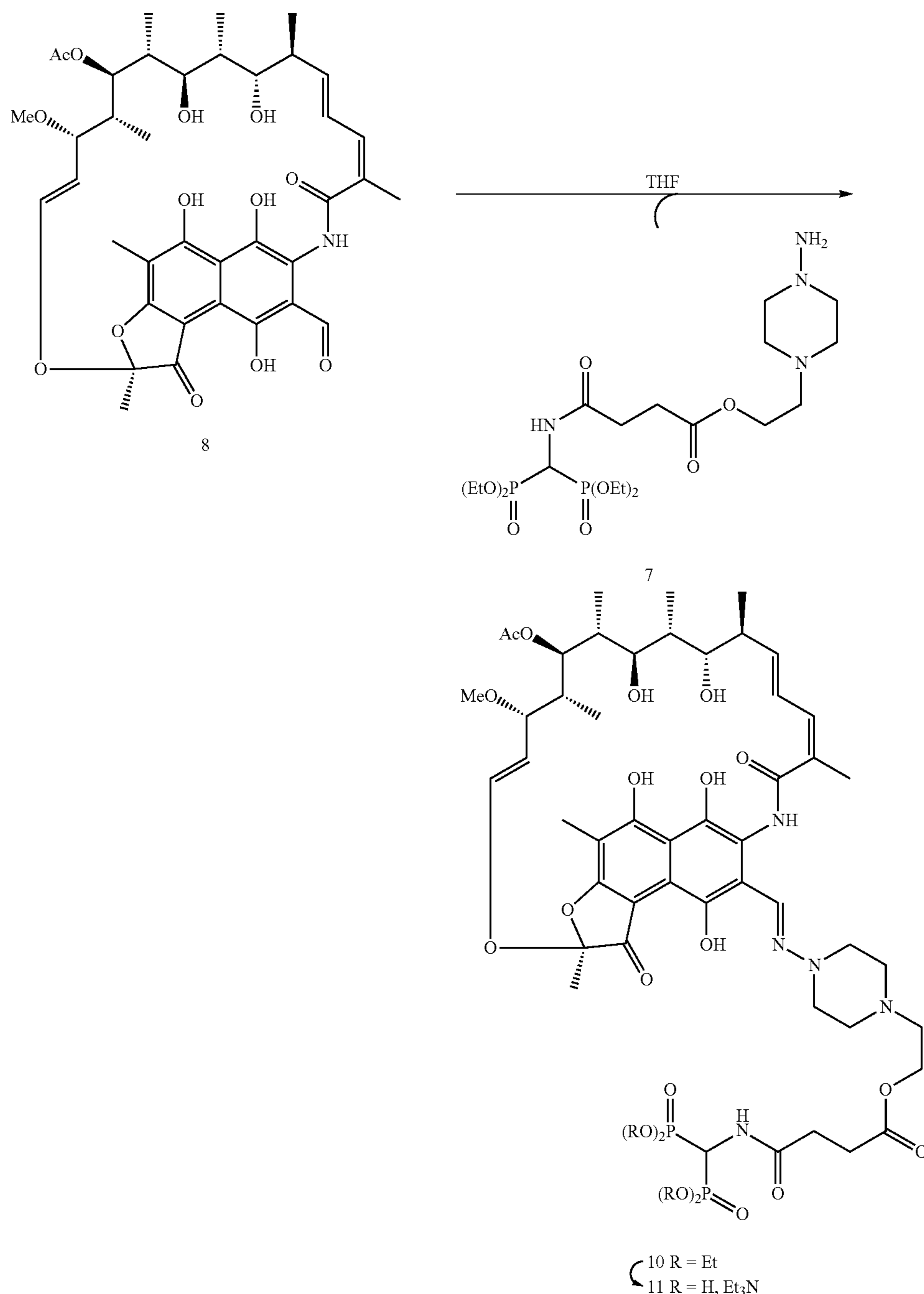
Scheme 3.
