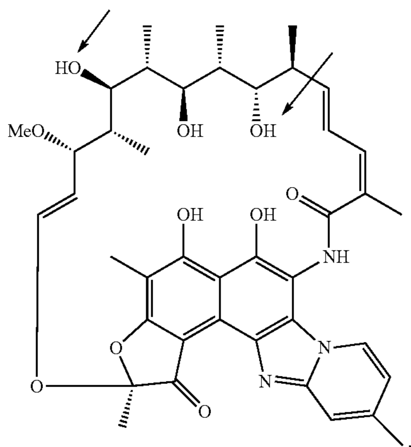
Deacetylated rifamixin
