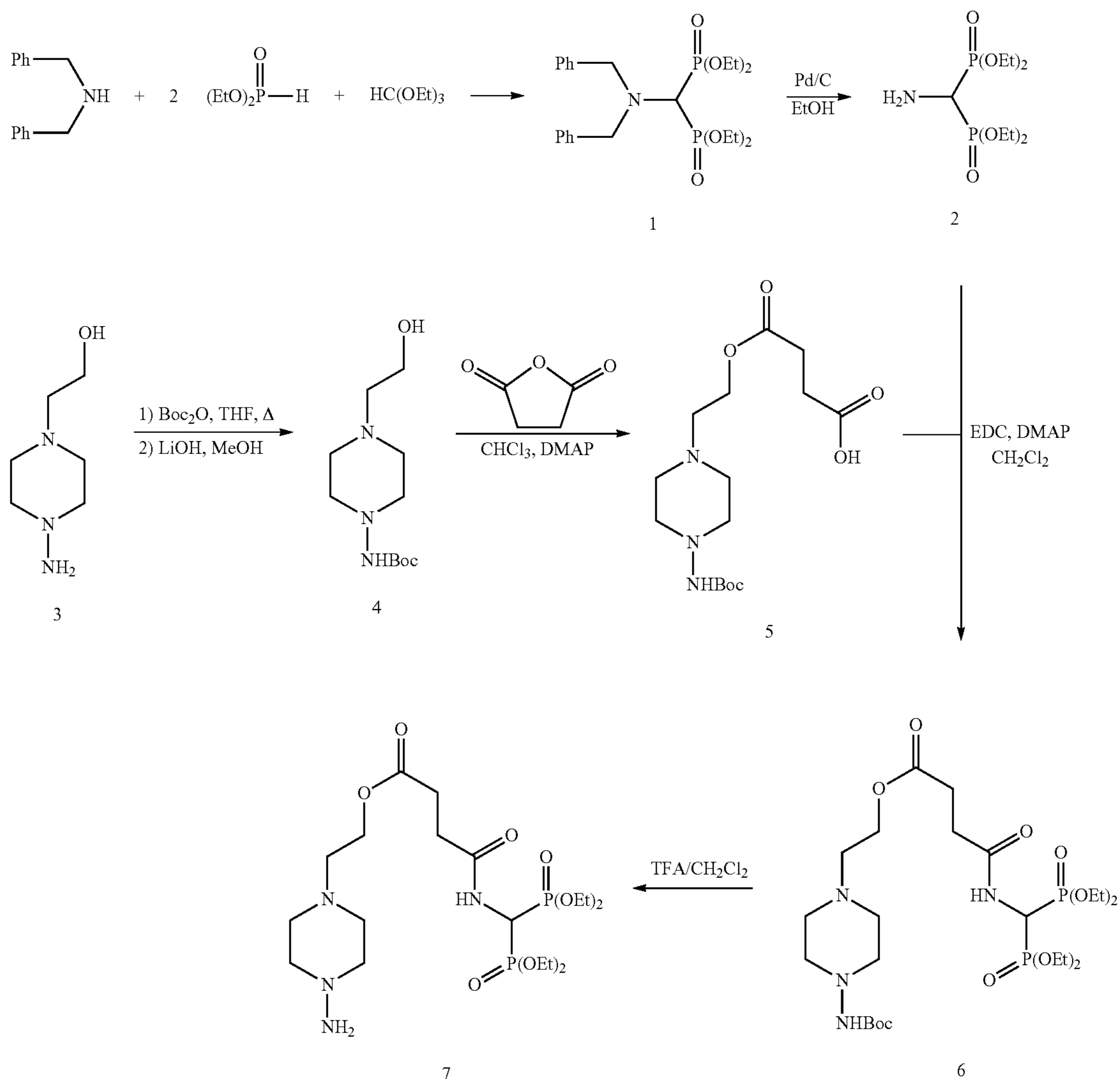
Scheme 1. Synthesis of Tetraethyl (4-(2-(1-amino-piperazin-4-yl)ethoxy)-4-oxo-butanoylamino)methylene-1,1-bisphosphonate (7)
