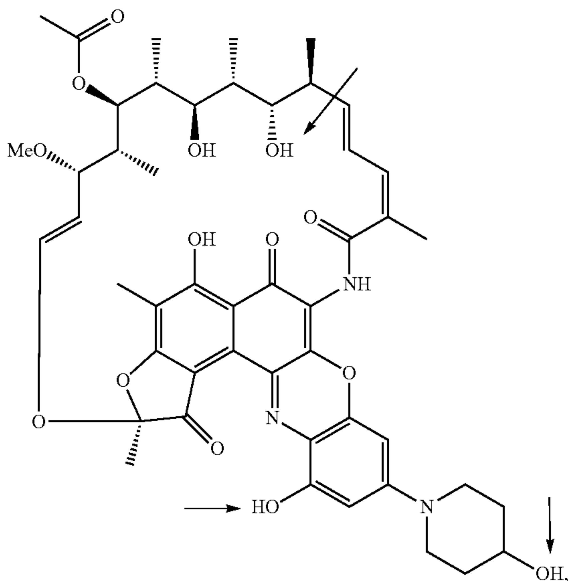
Compound 63
