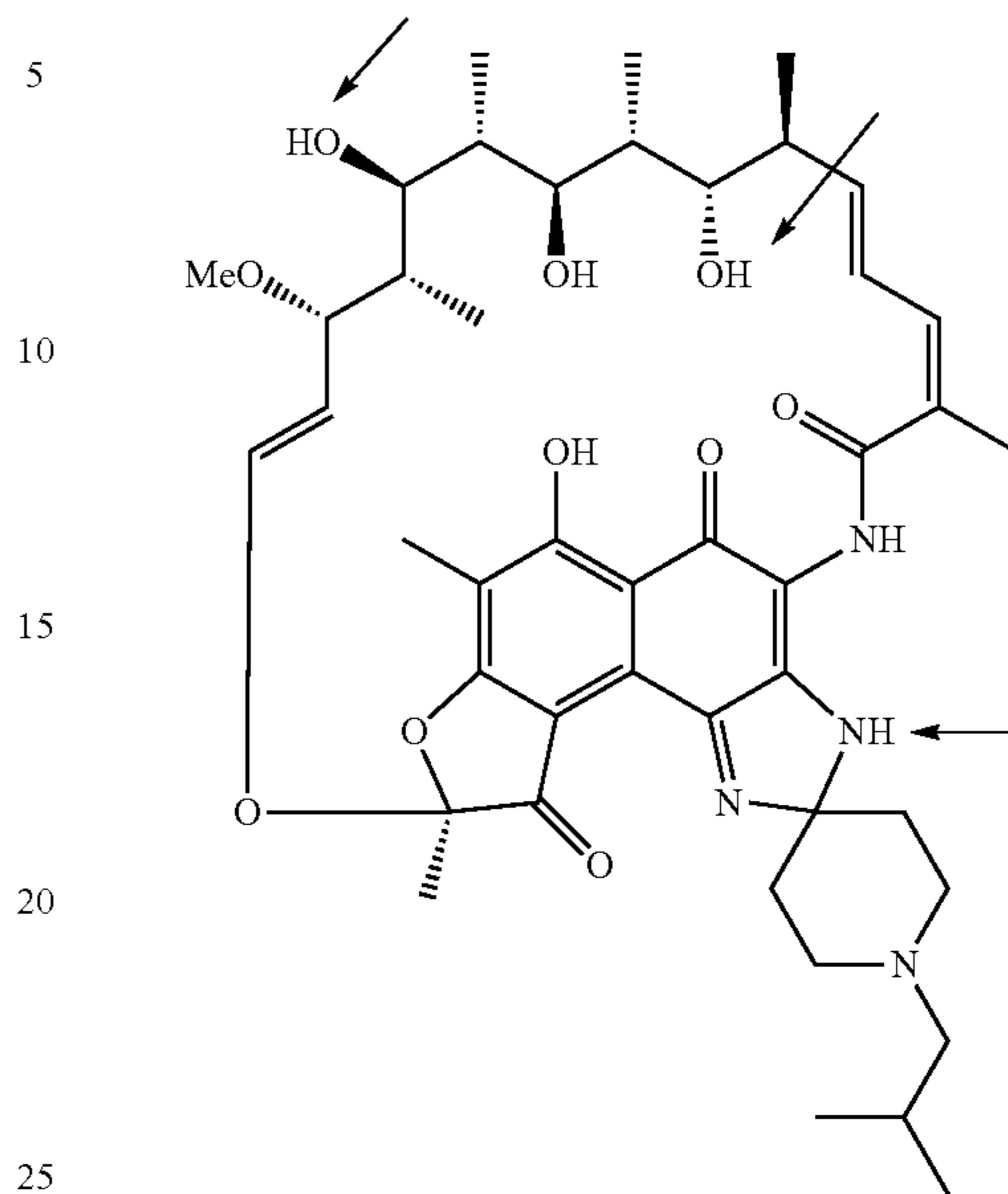
Deacetylated rifabutin
