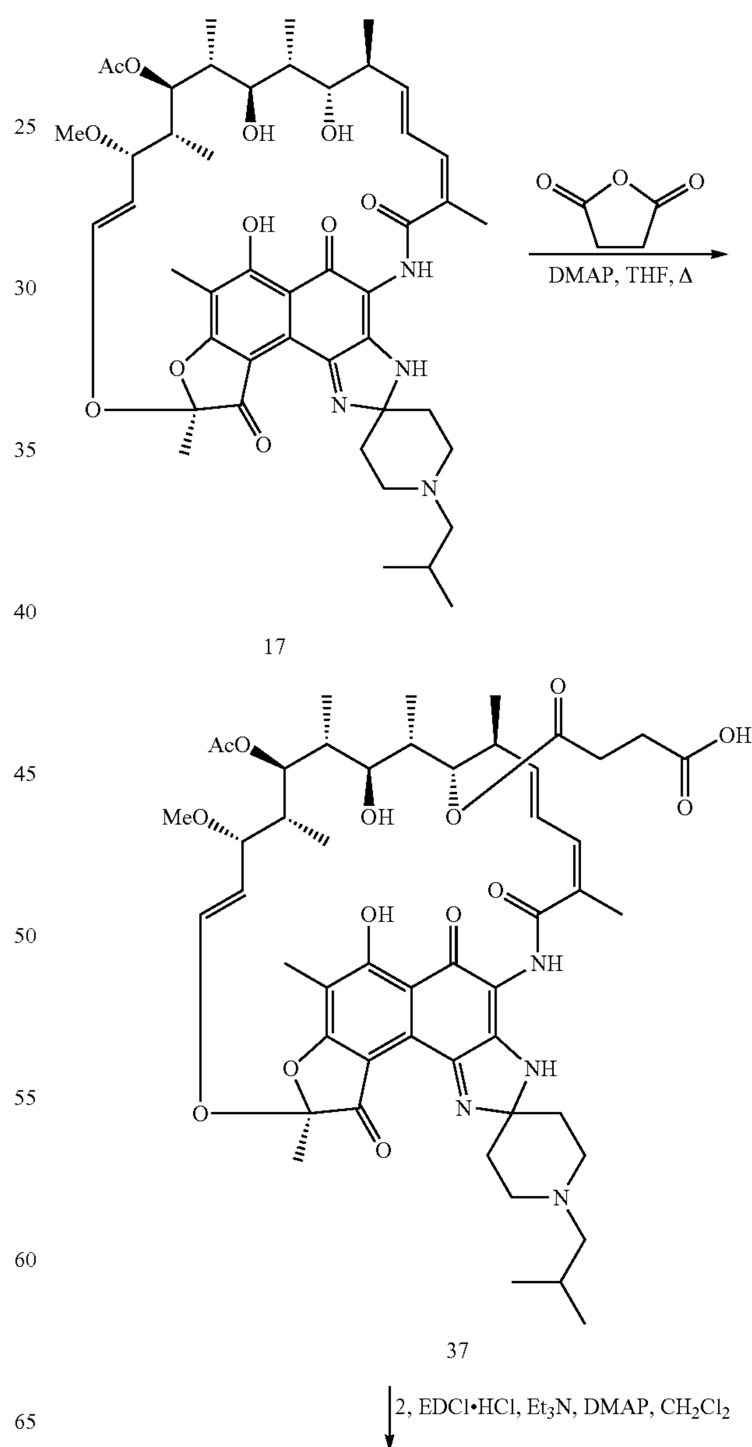
Scheme 10. Preparation of Rifabutin-bisphosphonate conjugate 39
