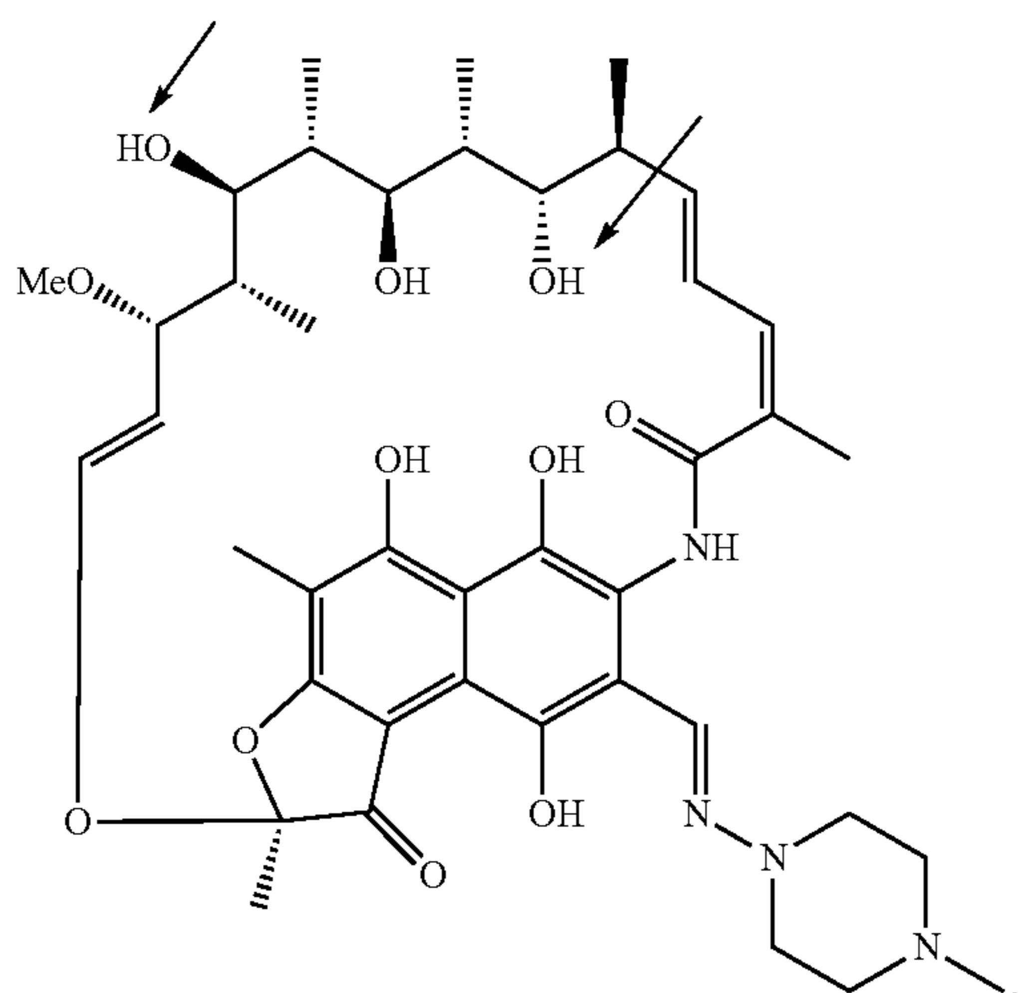
Decacetylated rifampicin
