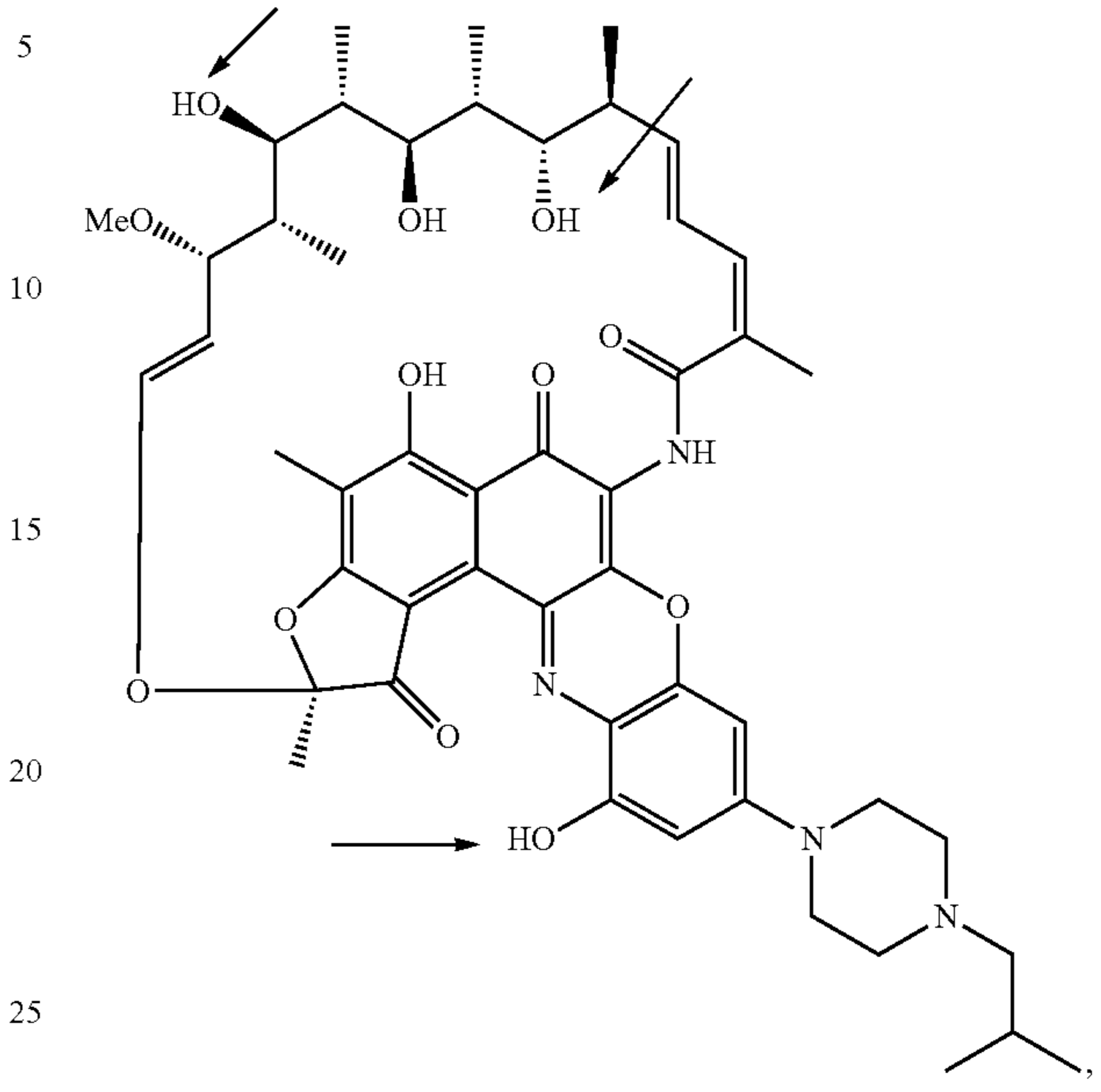
Deacetylated rifalazil
