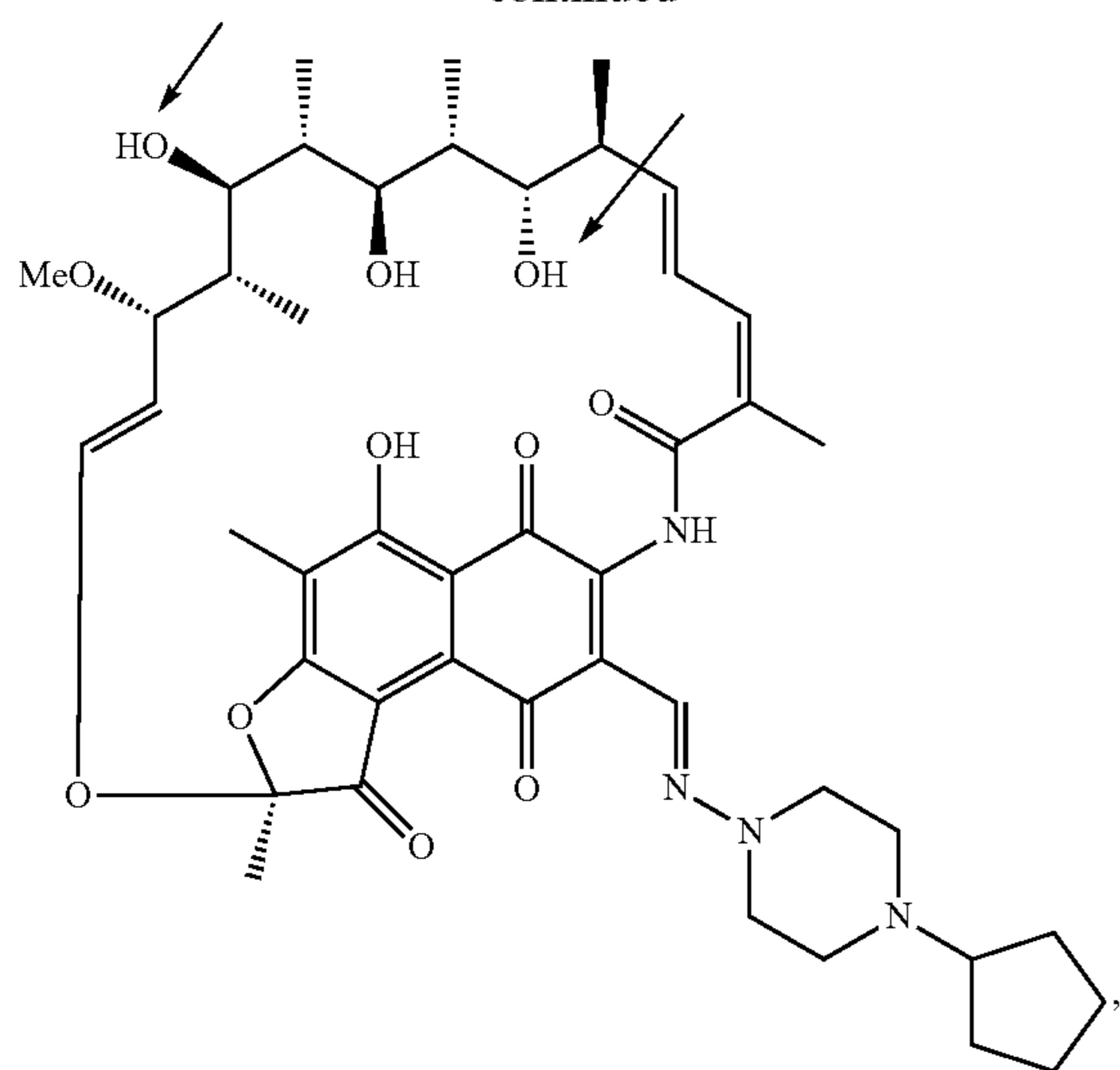
Deacetylated quinone form of rifapentin
