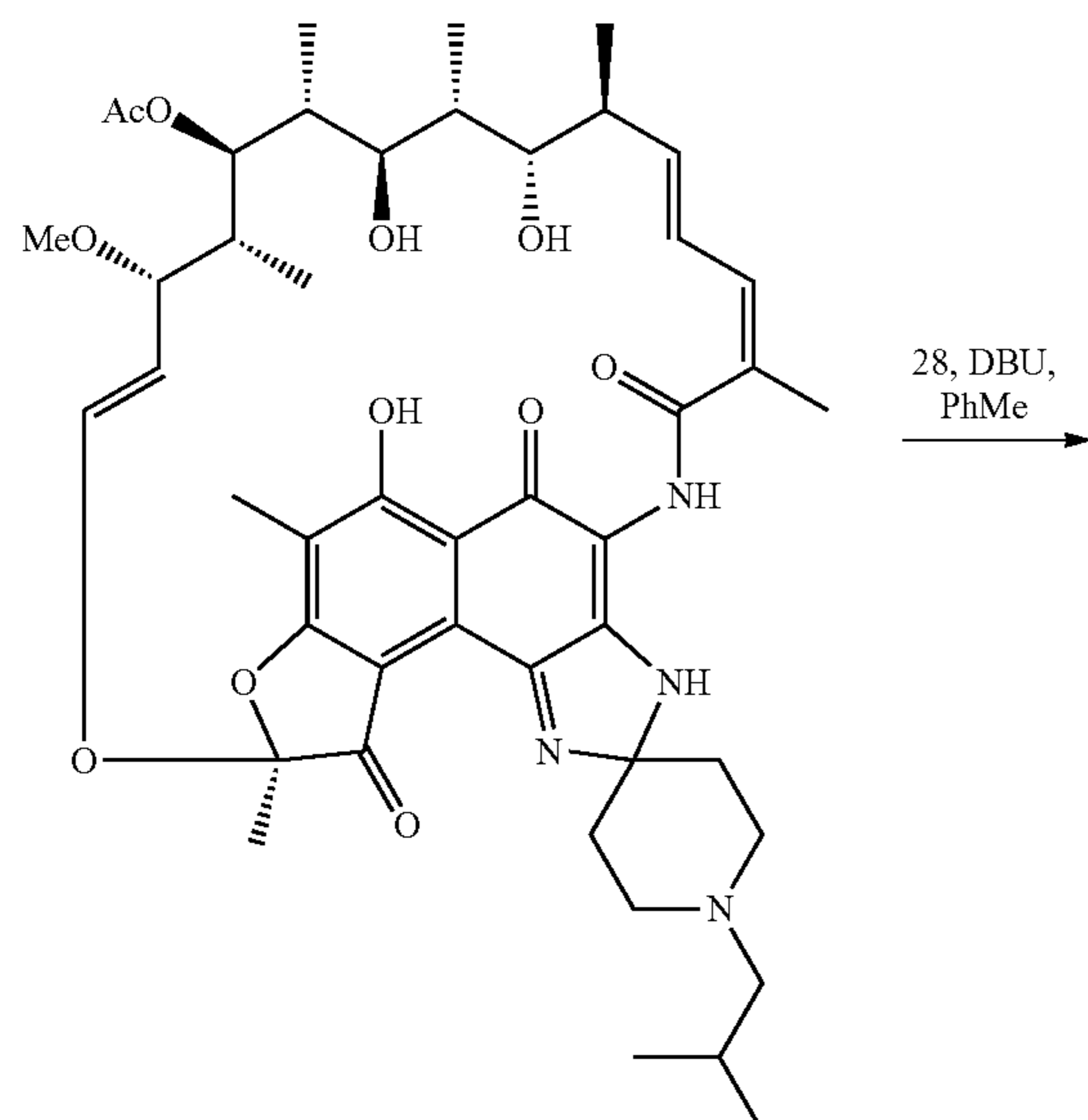
Scheme 7. Preparation of Rifabutin bisphosphonate conjugate 30
