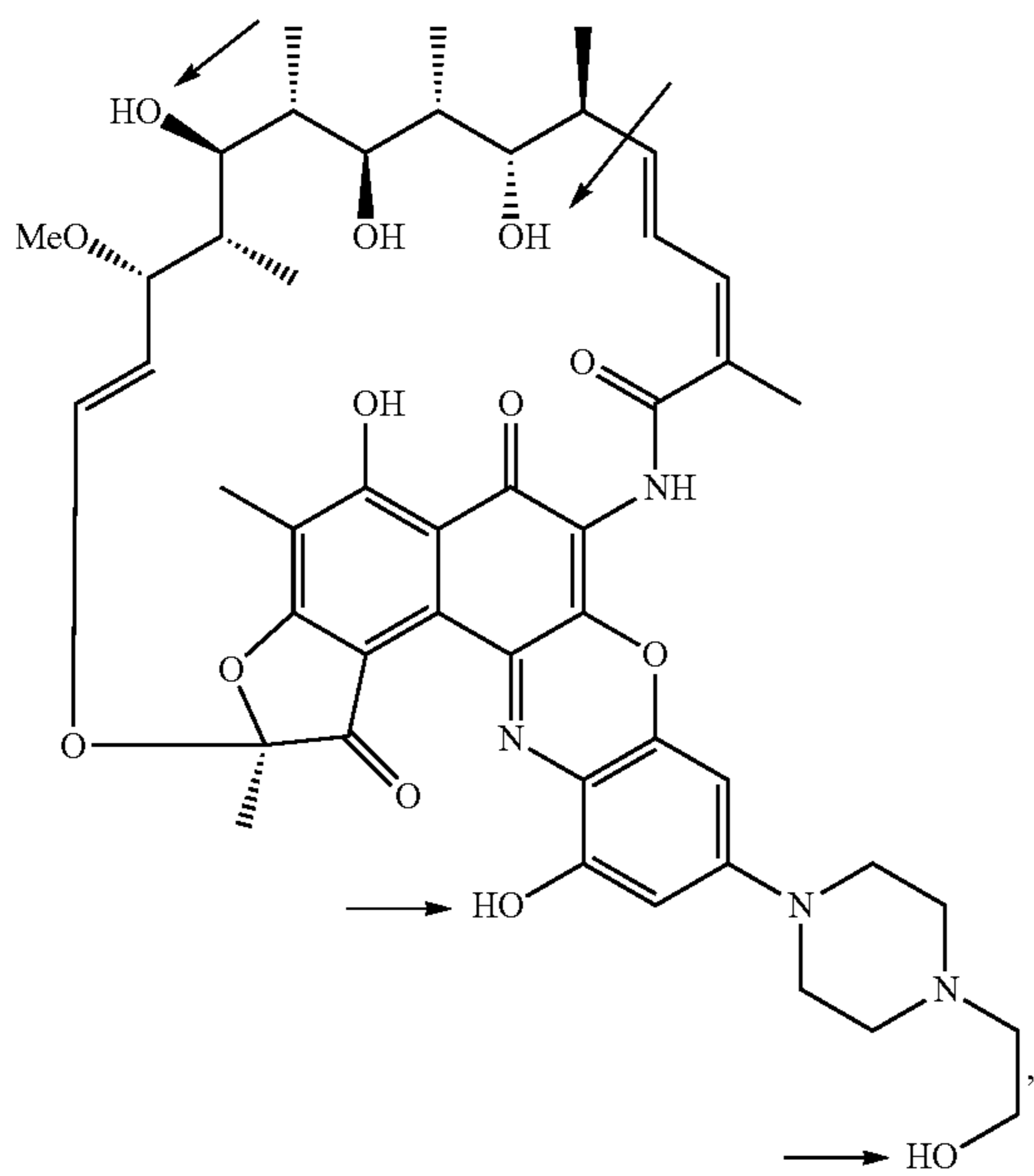
Deacetylated compound 56
