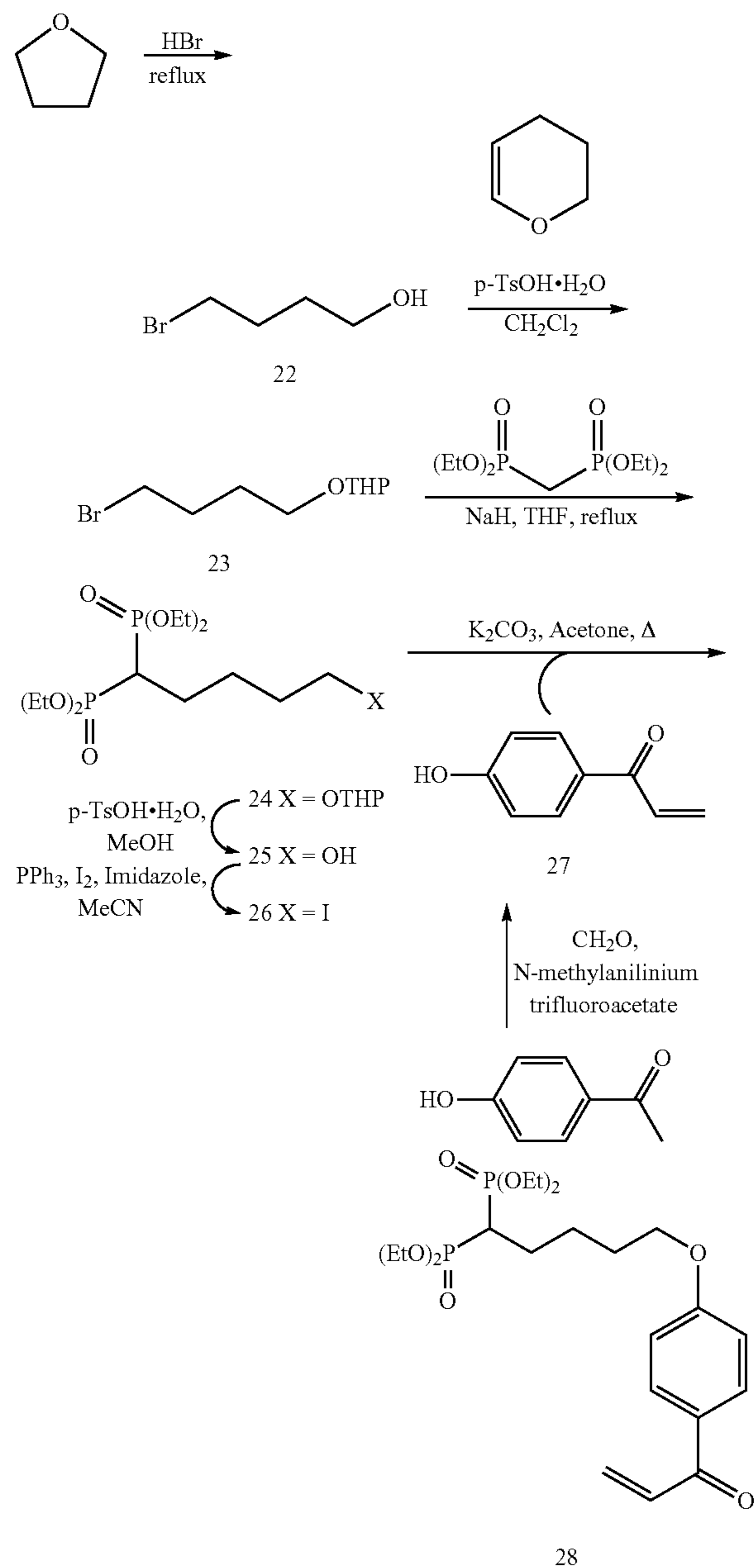
Scheme 6. Synthesis of 1-(4-(5,5-bis(diethylphosphono)pentyl)oxy)phenyl)prop-2-en-1-one.
