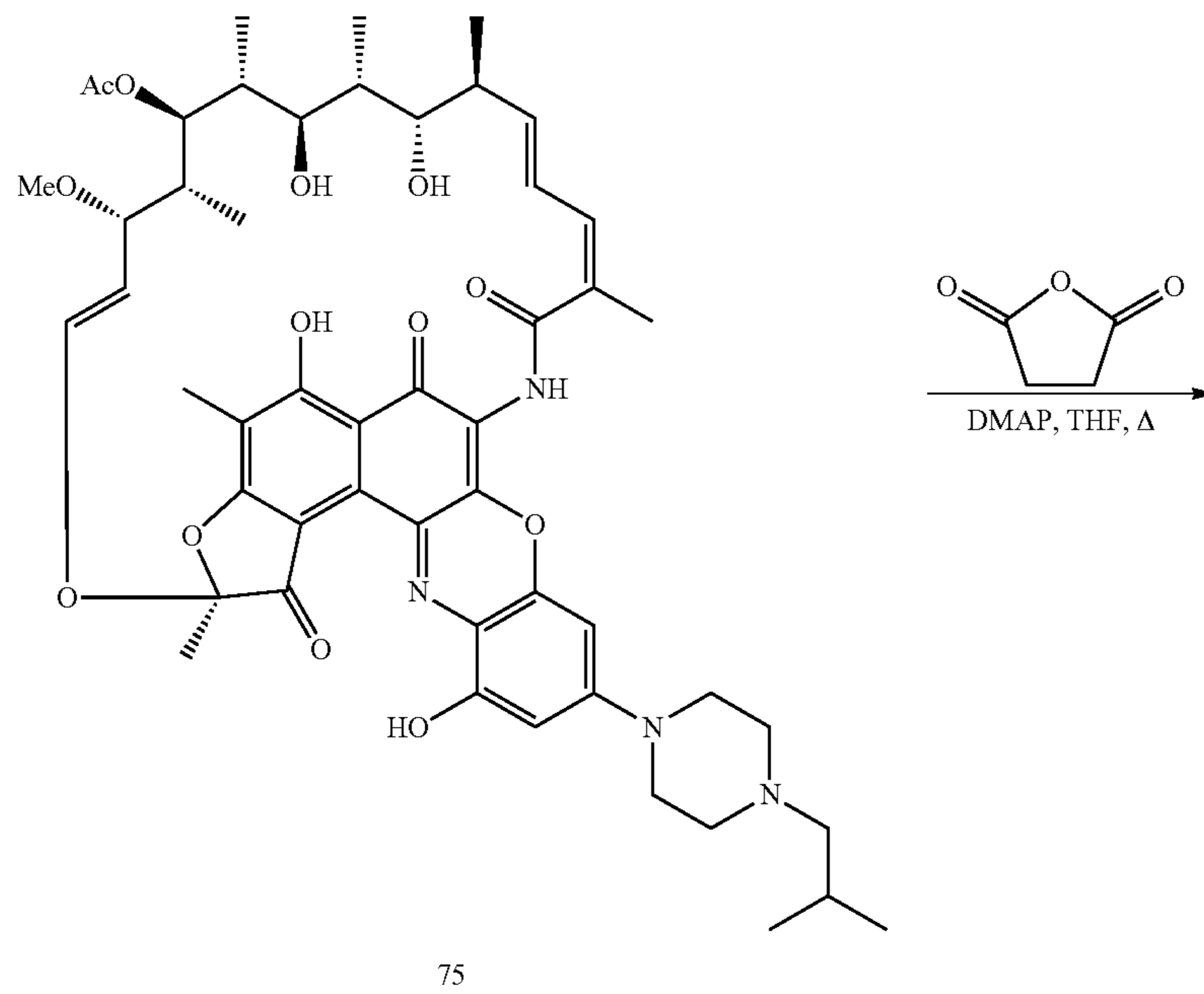
Scheme 26. Preparation of rifalazil bisphosphonate conjugate 78
