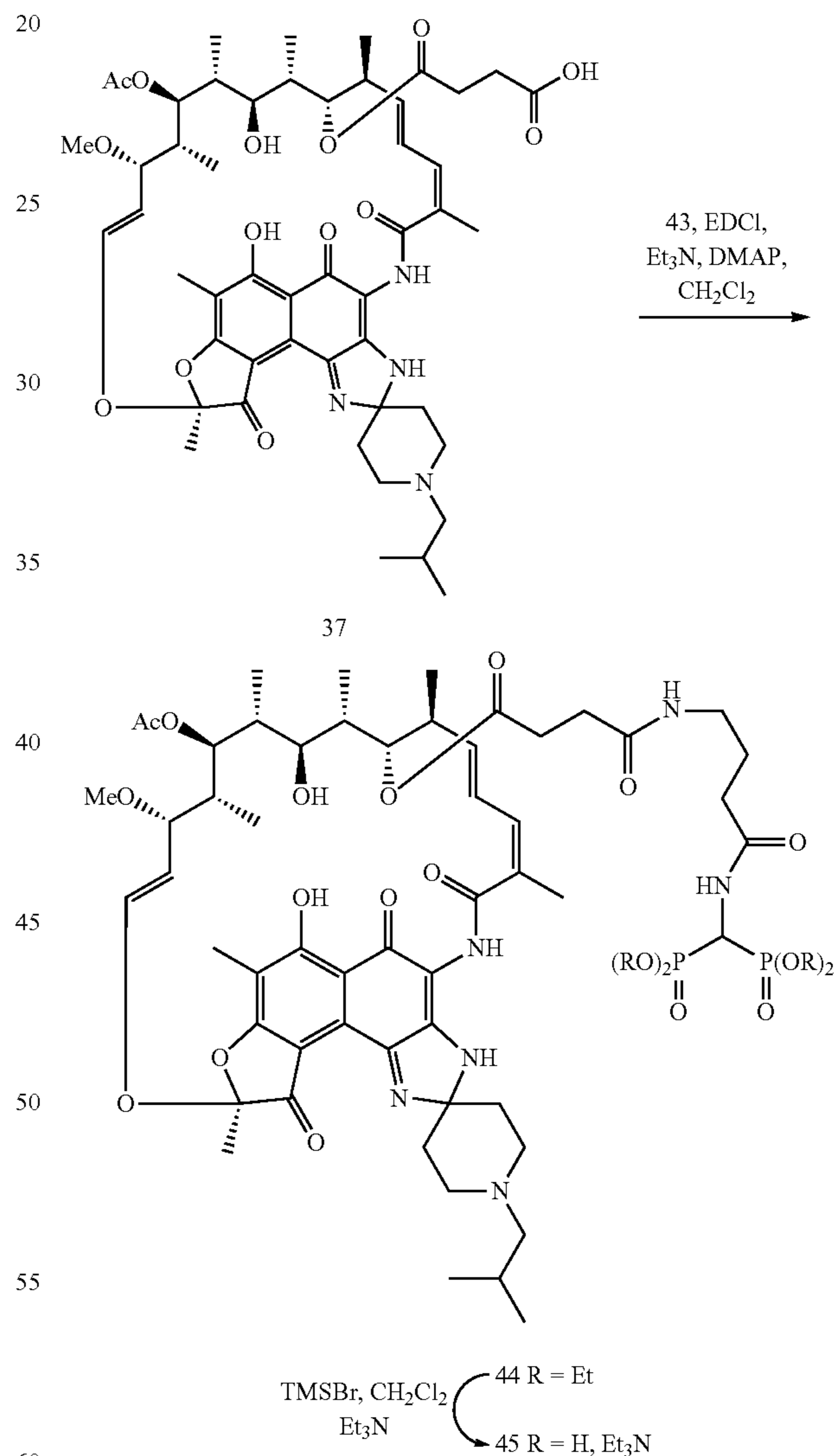
Scheme 12. Preparation of Rifabutin-bisphosphonate conjugate 45.
