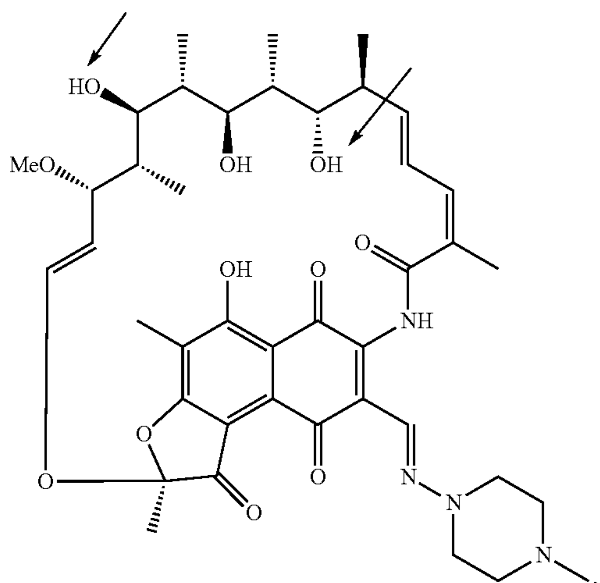
Decacetylated quinone form of Rifampicin
