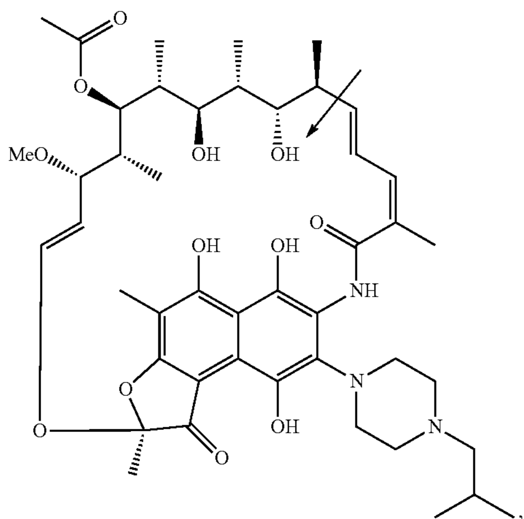
Rifandin
