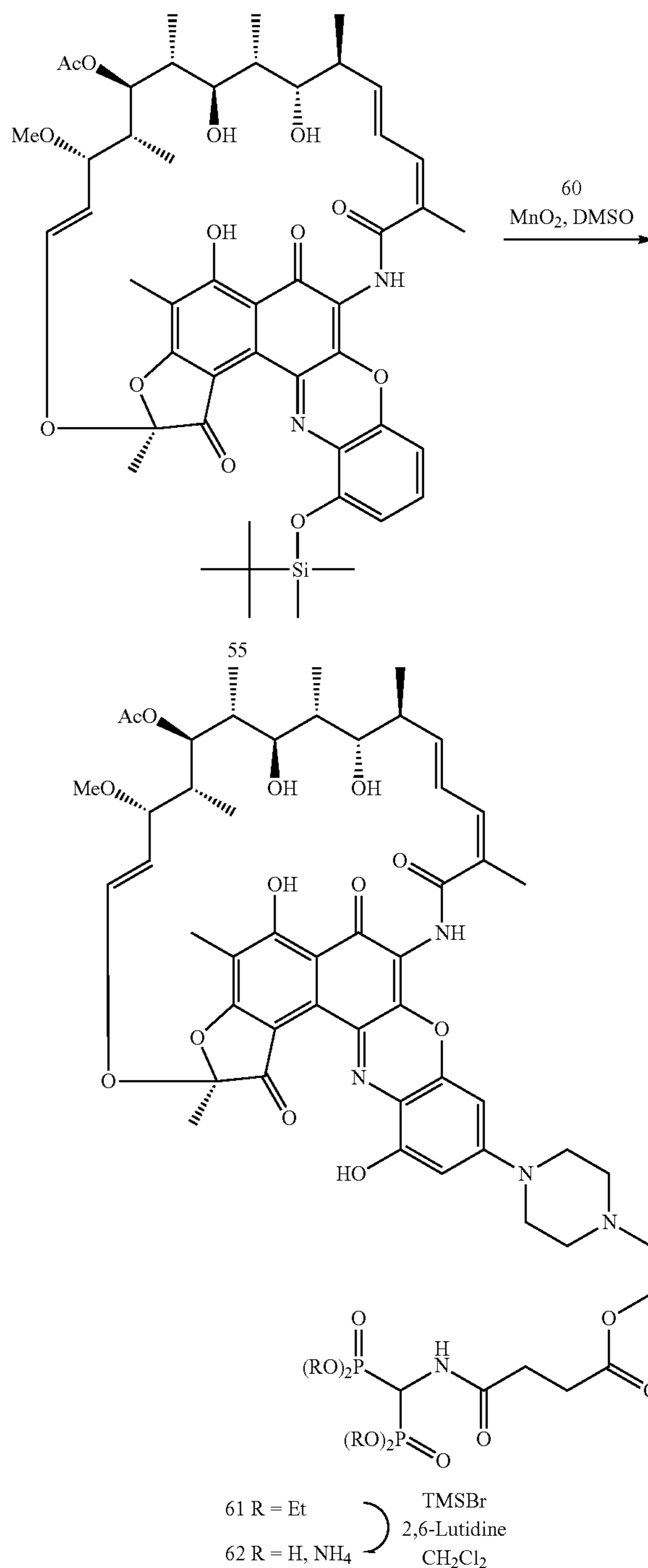
Scheme 19. Preparation of 3'-hydroxybenzoxazinorifamycin bisphosphonate conjugate 62.
