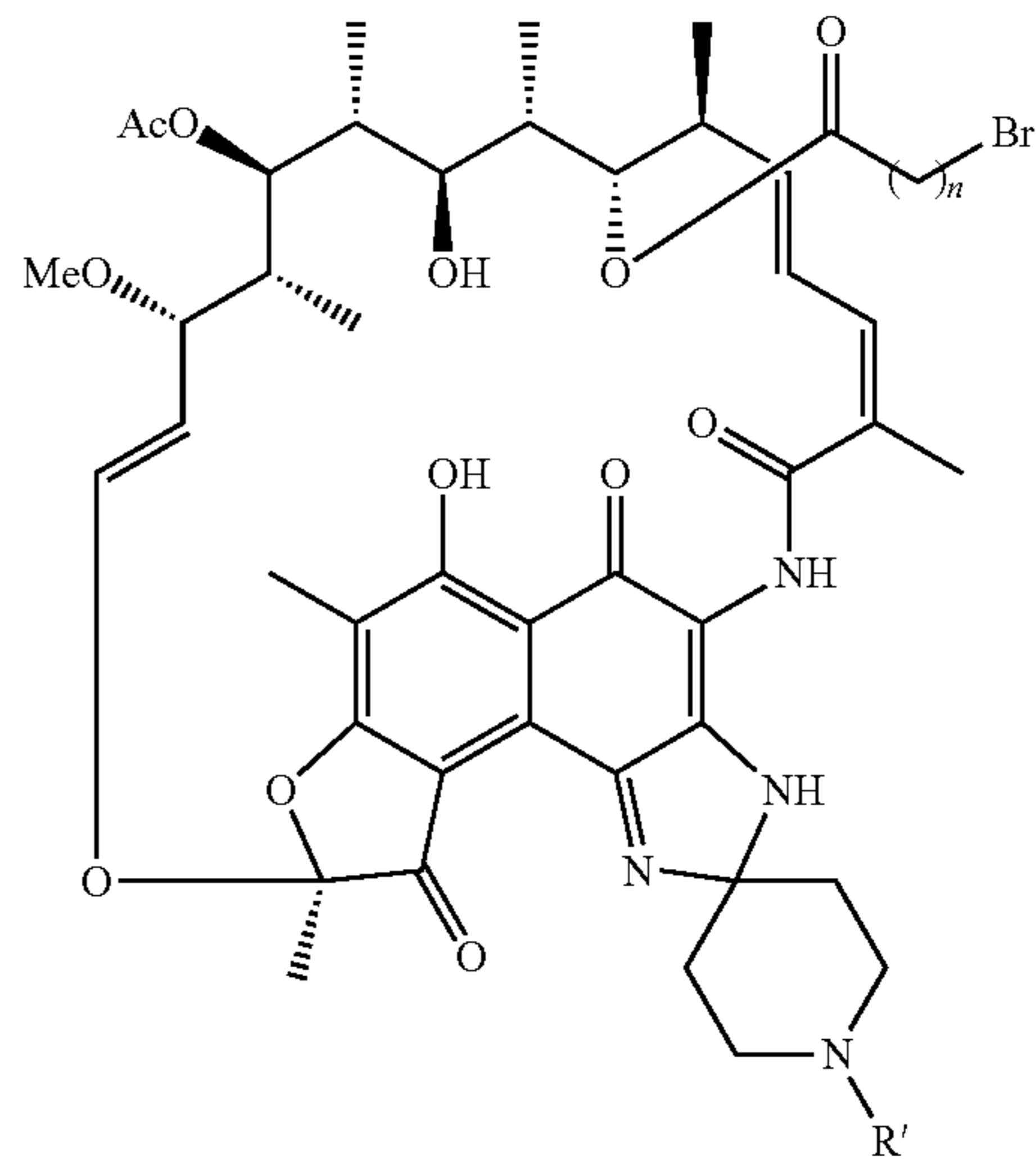
LXIIIa n = 1 LXIIIb n = 3 LXIIIc n = 4
