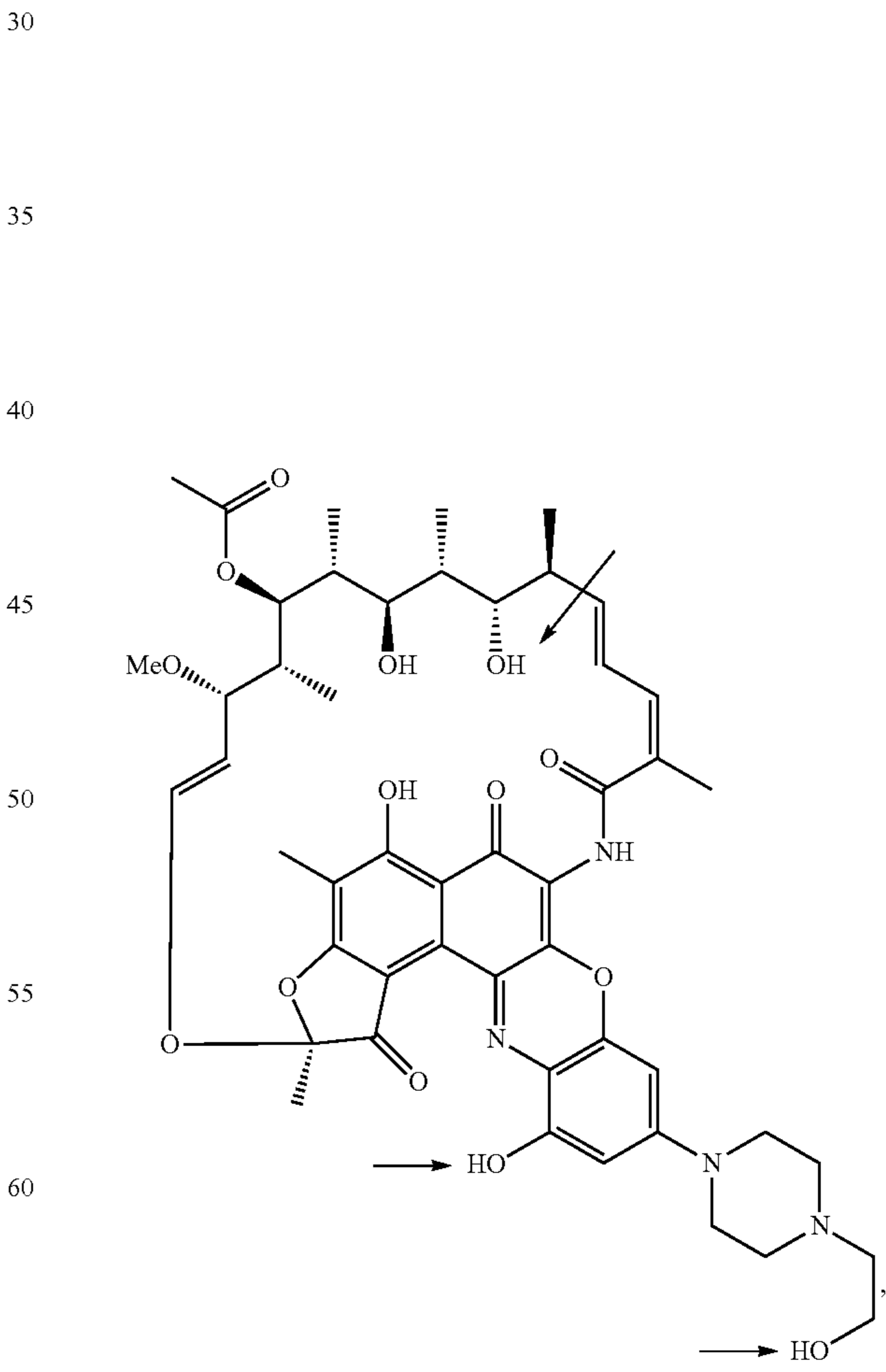
Compound 56
