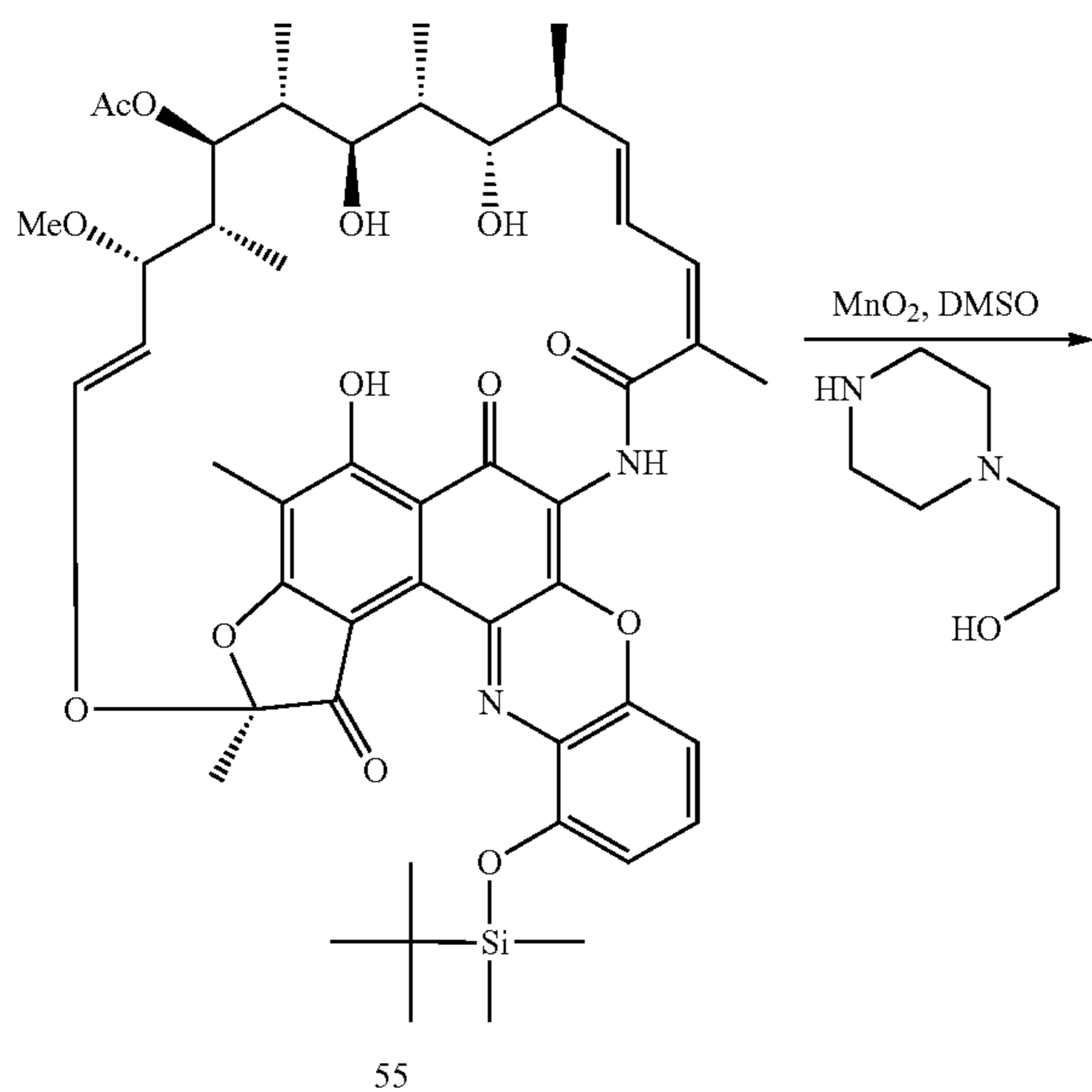
Scheme 17. Preparation of 3'-hydroxybenzoxazinorifamycin derivative 56.
