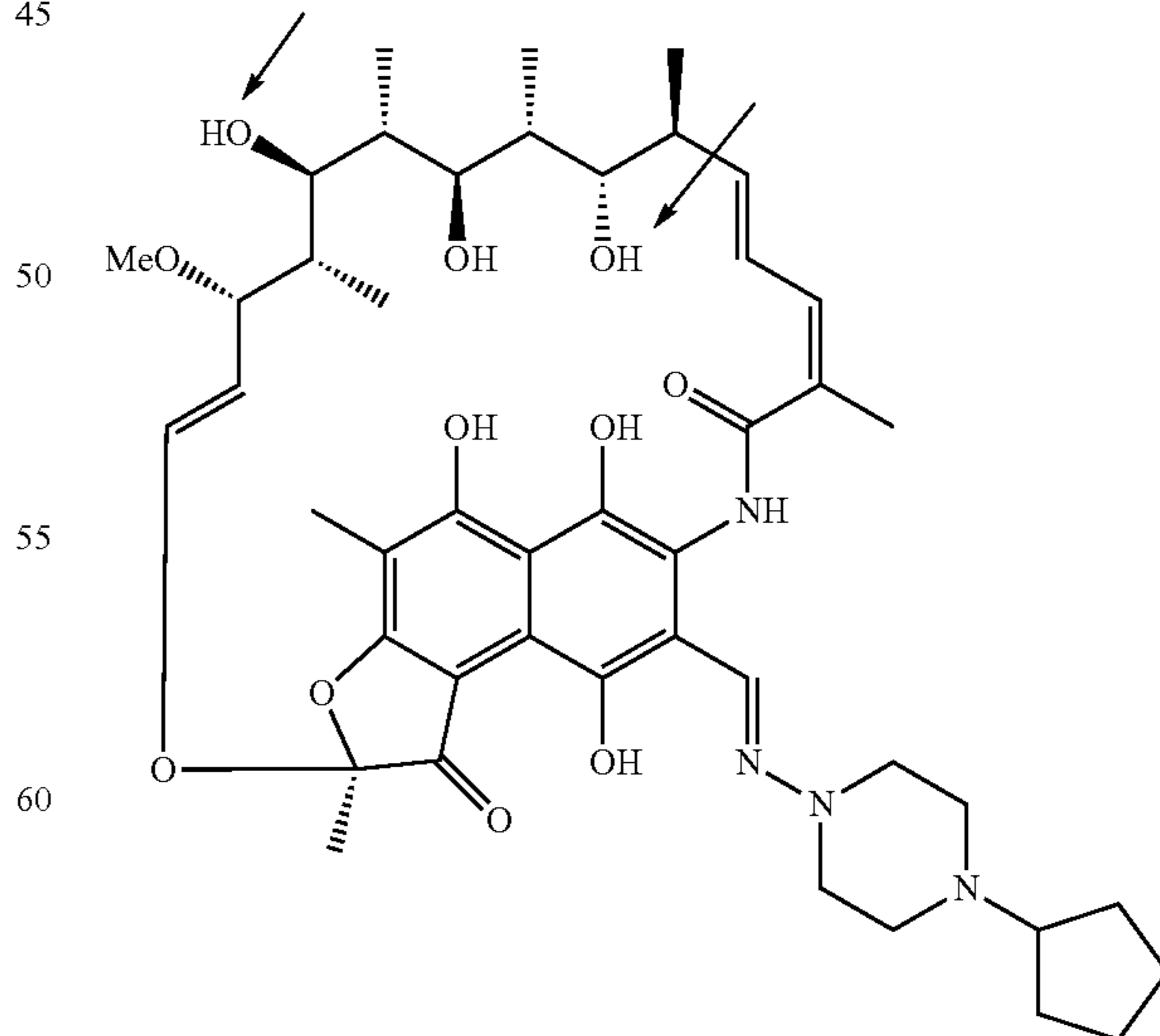
Decacetylated rifapentin
