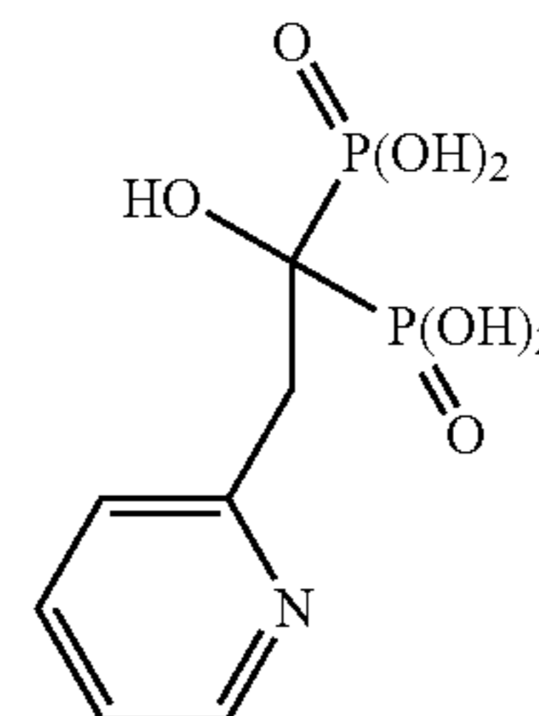
Risedronate
