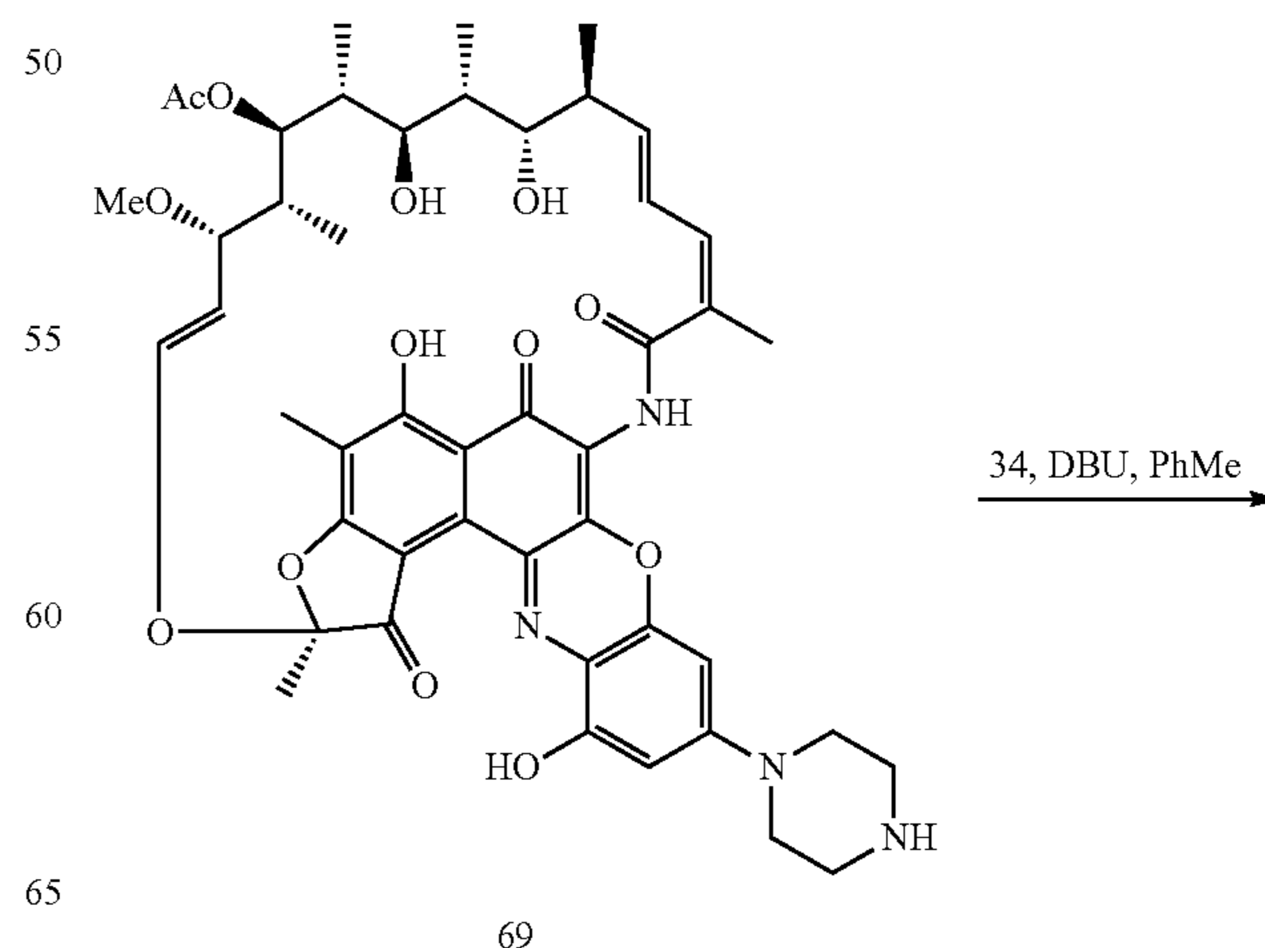
Scheme 24. Preparation of 3'-hydroxybenzoxazinorifamycin bisphosphonate conjugate 71
