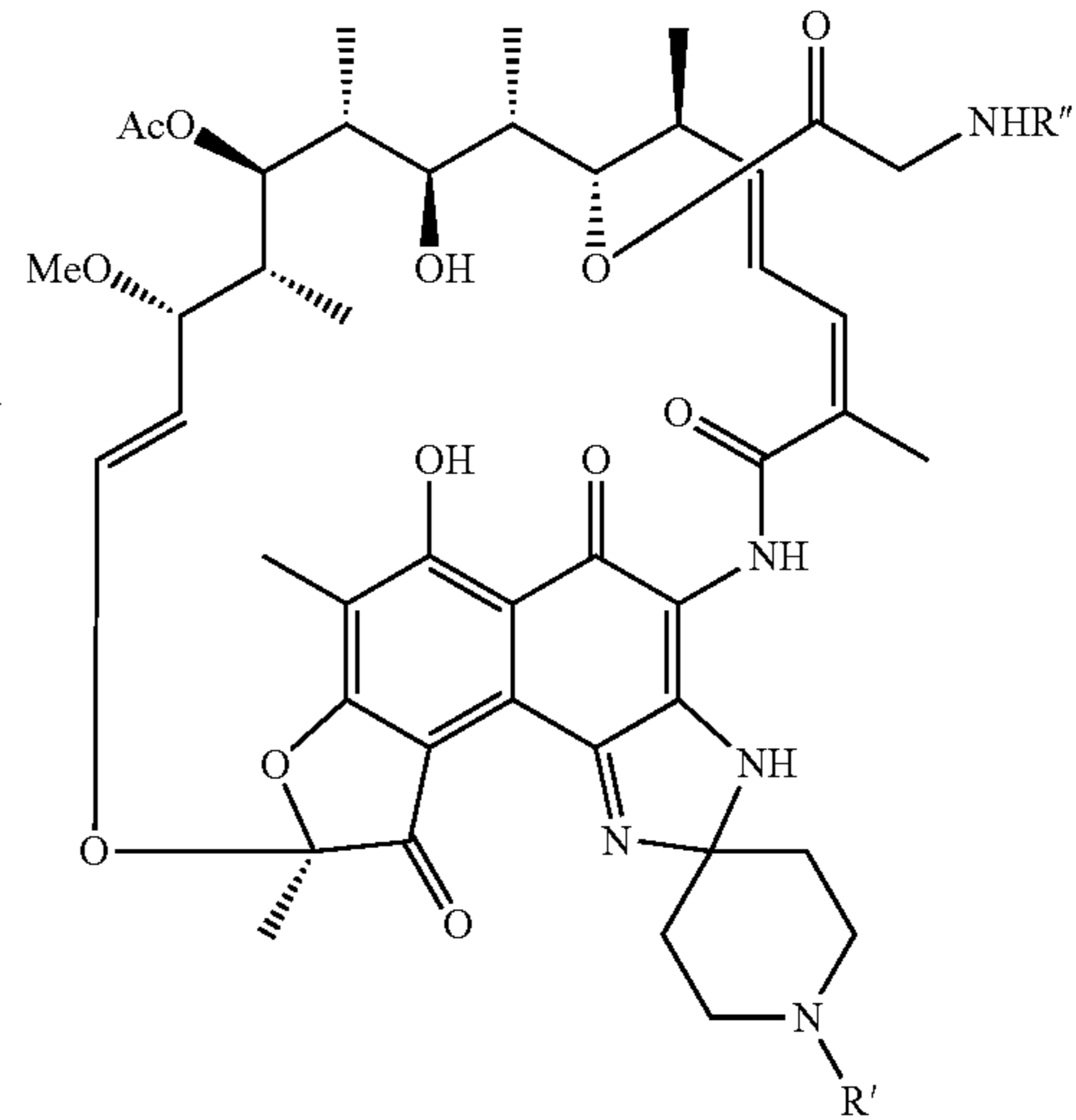
XLIIa R'' = PG XLIIb R'' = H
