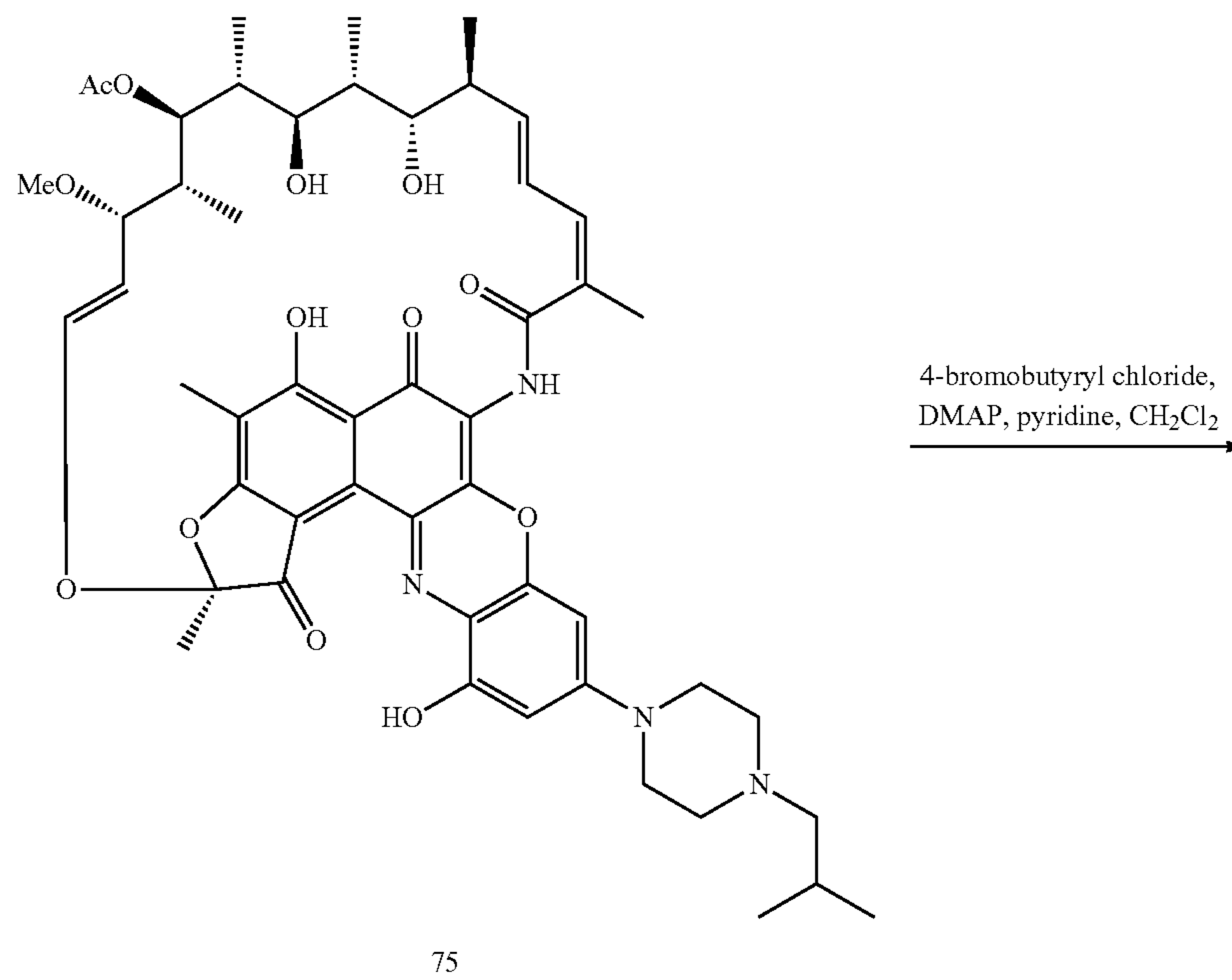
Scheme 27. Preparation of rifalazil bisphosphonate conjugate 81
