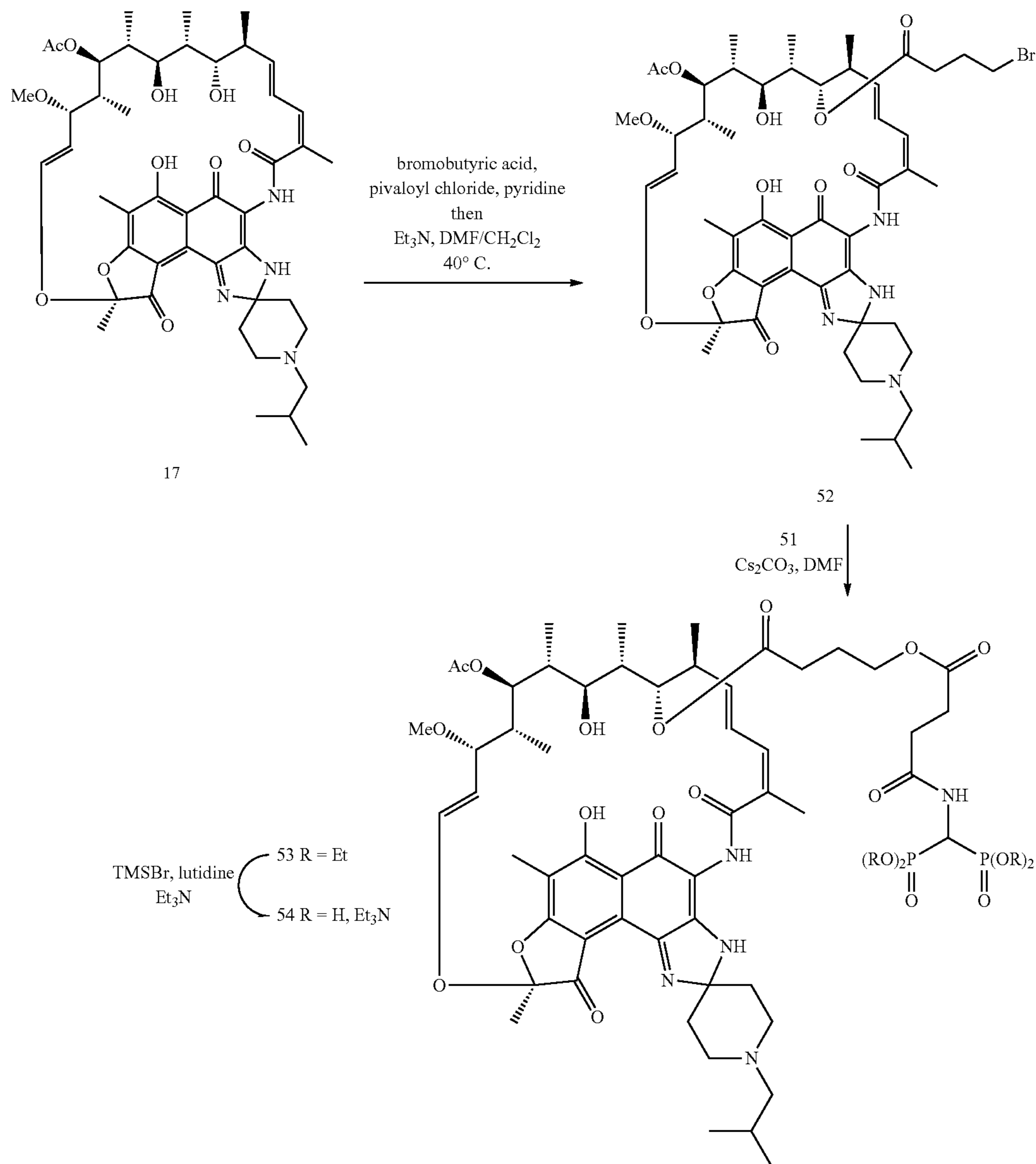
Scheme 16. Preparation of rifabutin-bisphosphonate conjugate 54
