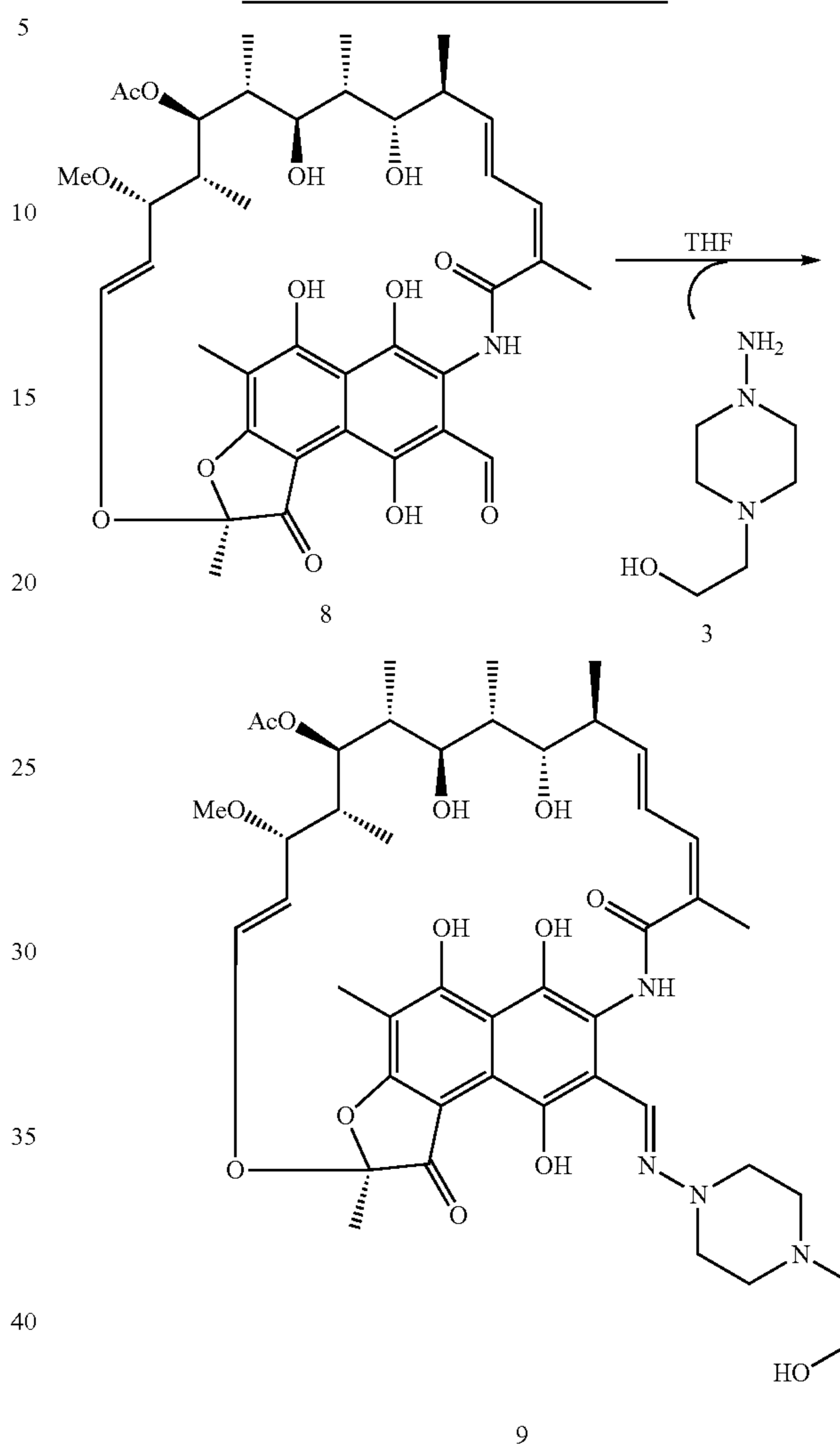
Scheme 2. Synthesis of 3-(((4-(2-hydroxyethyl)-1-piperazinyl)imino)methyl)rifamycin (9)
