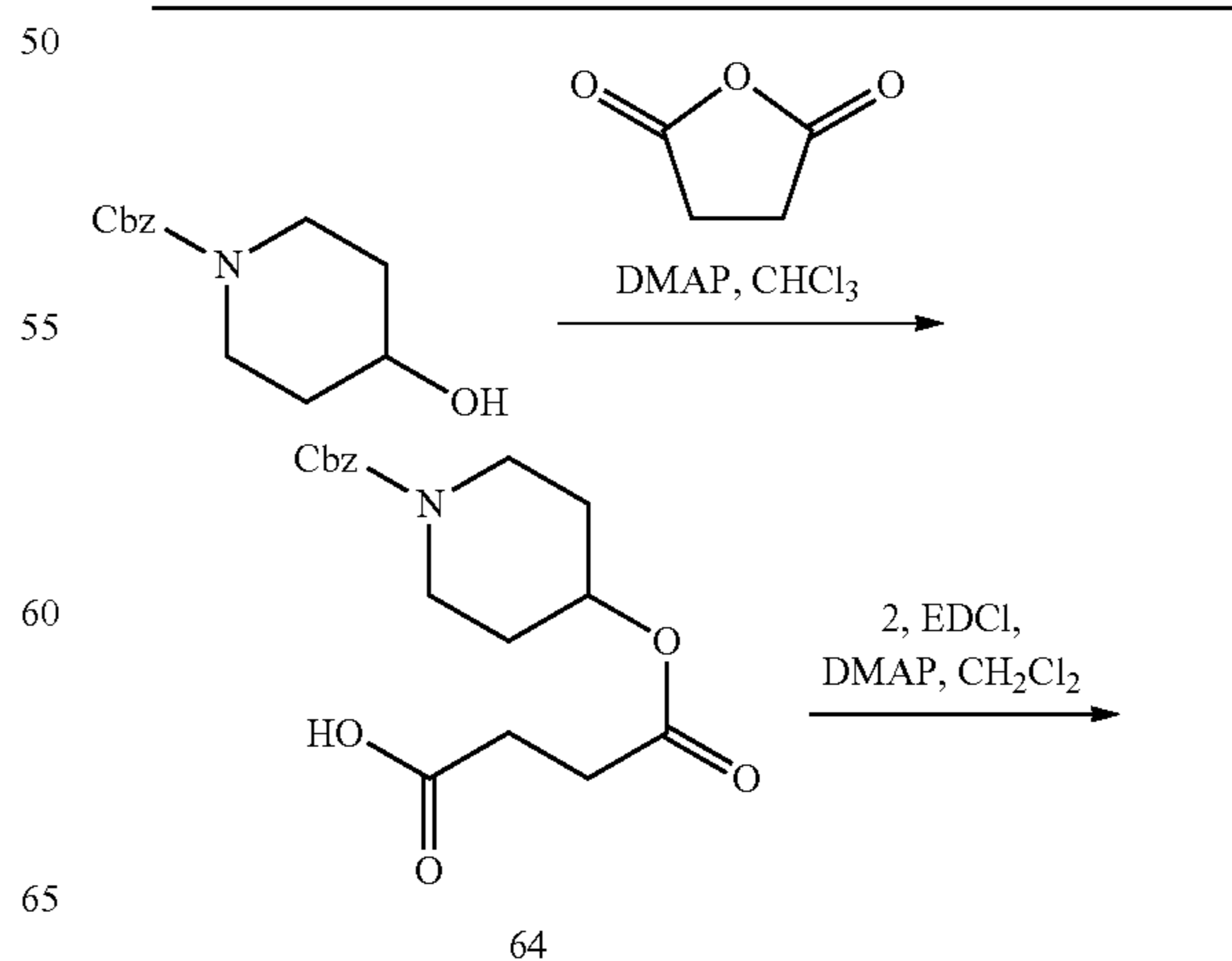
Scheme 21. Preparation of Tetraethyl (4-(2-(1-benzyloxycarbonyl)-piperidin-4-yl)ethoxy)-4-oxo-butanoyl-amino)methylene-1,1-bisphosphonate
