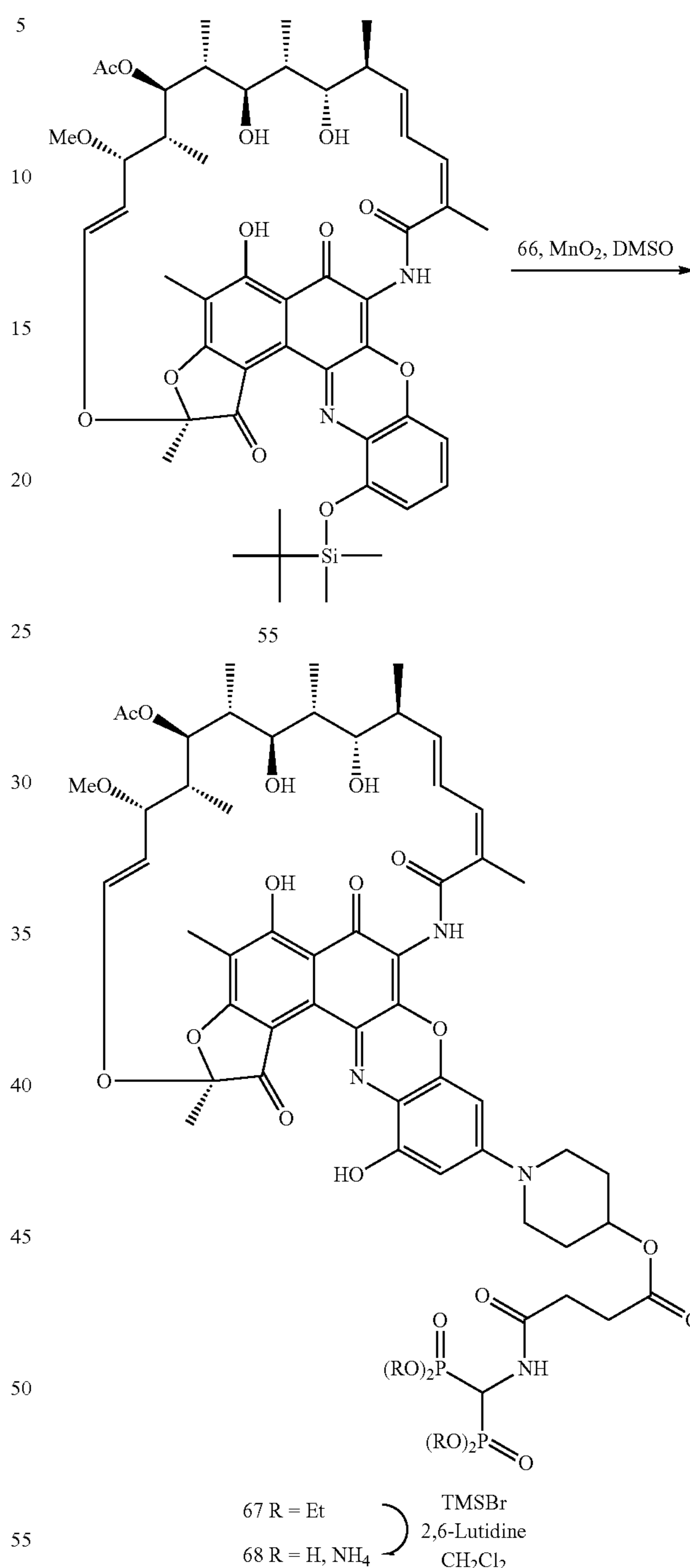
Scheme 22. Preparation of 3'-hydroxybenzoxazinorifamycin bisphosphonate conjugate 68.
