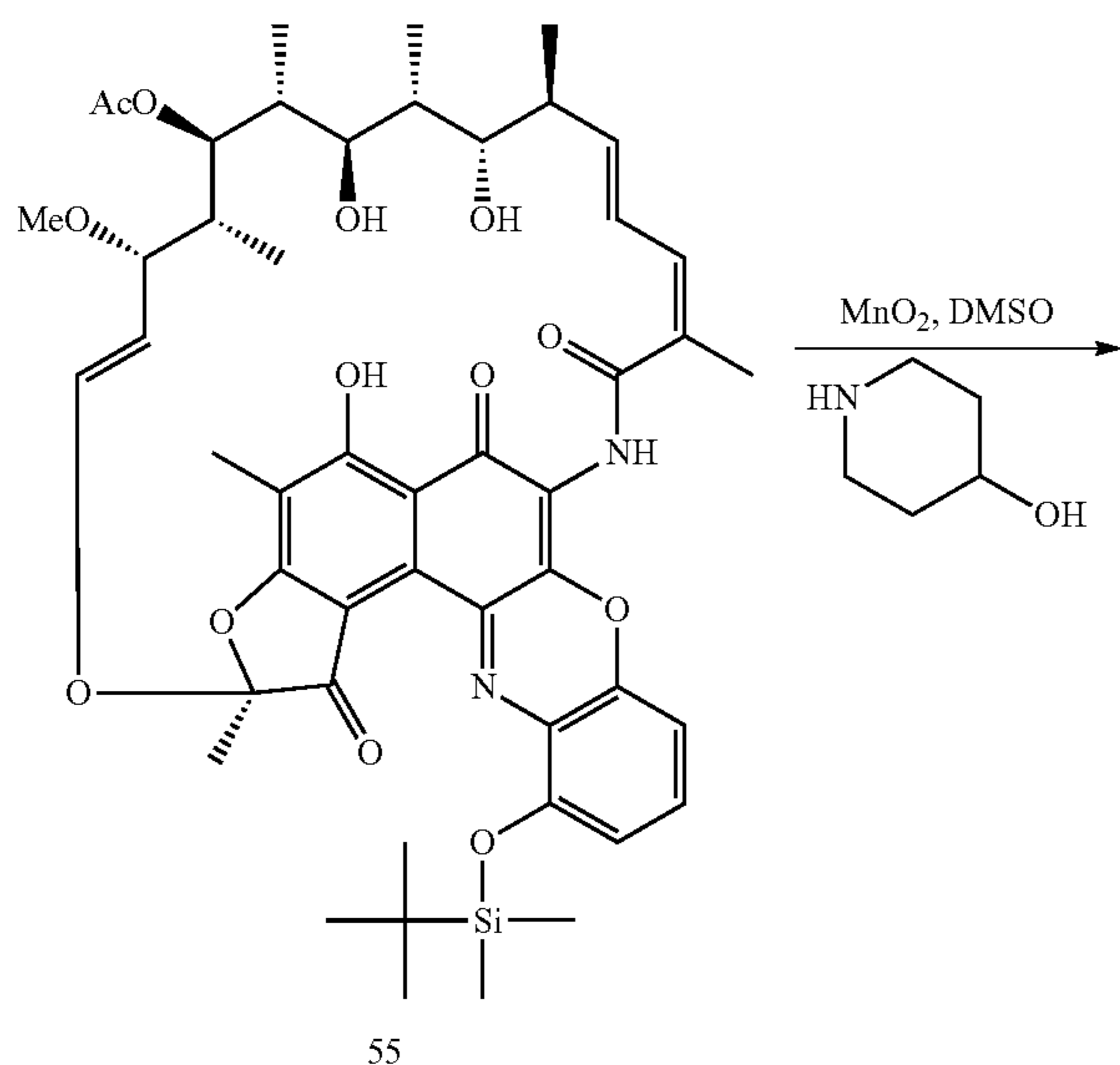
Scheme 20. Preparation of 3'-hydroxybenzoxazinorifamycin derivative 63.
