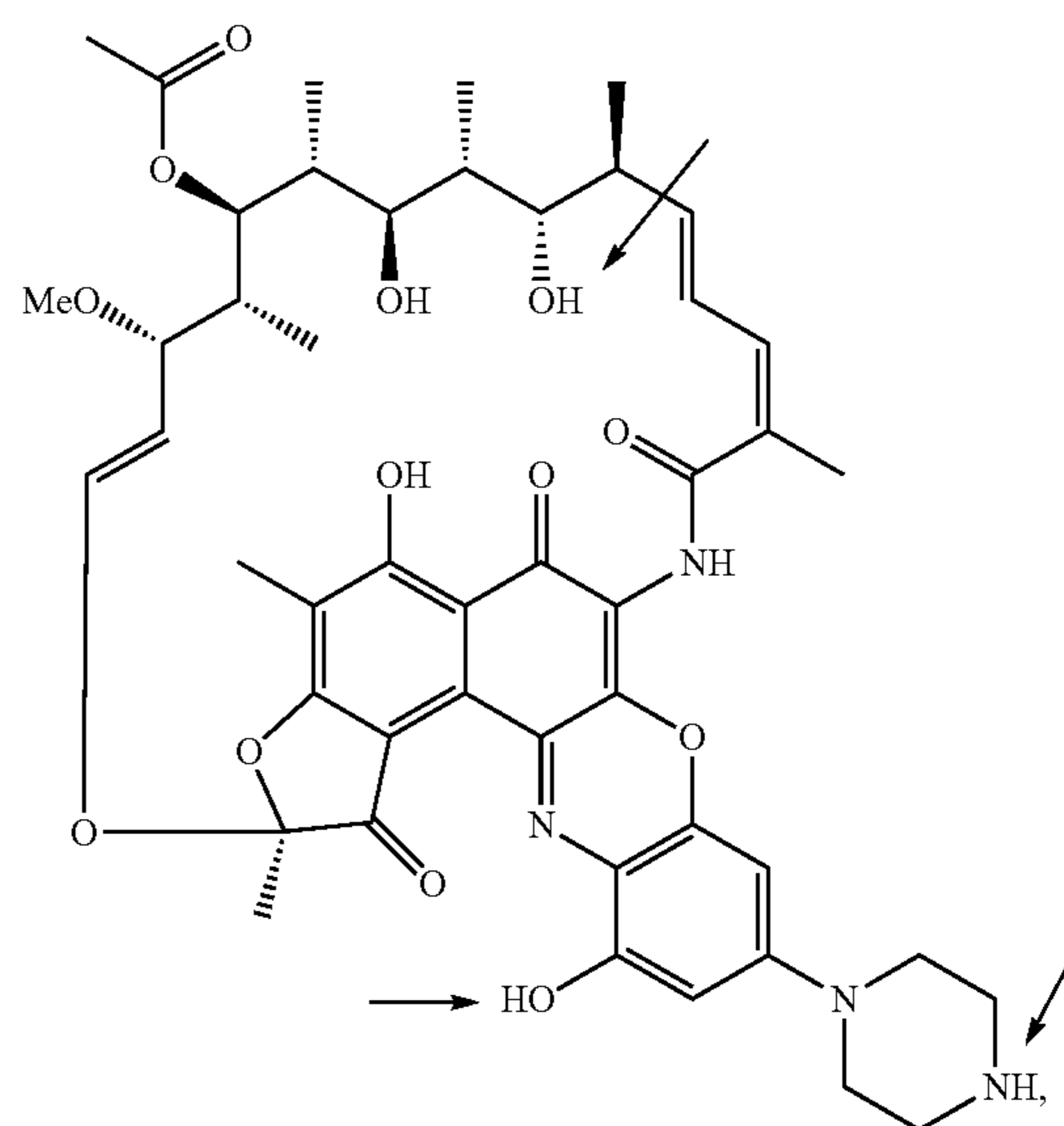
Compound 69
