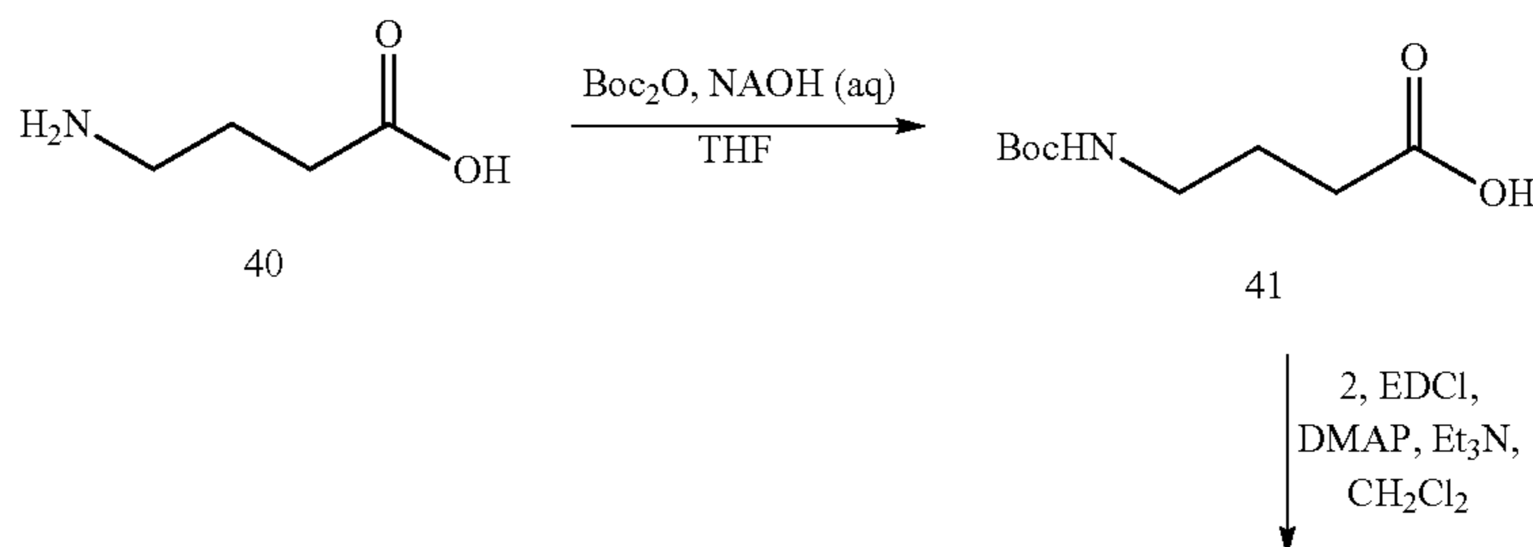
Scheme 11. Preparation of tetraethyl (4-aminobutanoylamino)methylene-1,1-bisphosphonate
