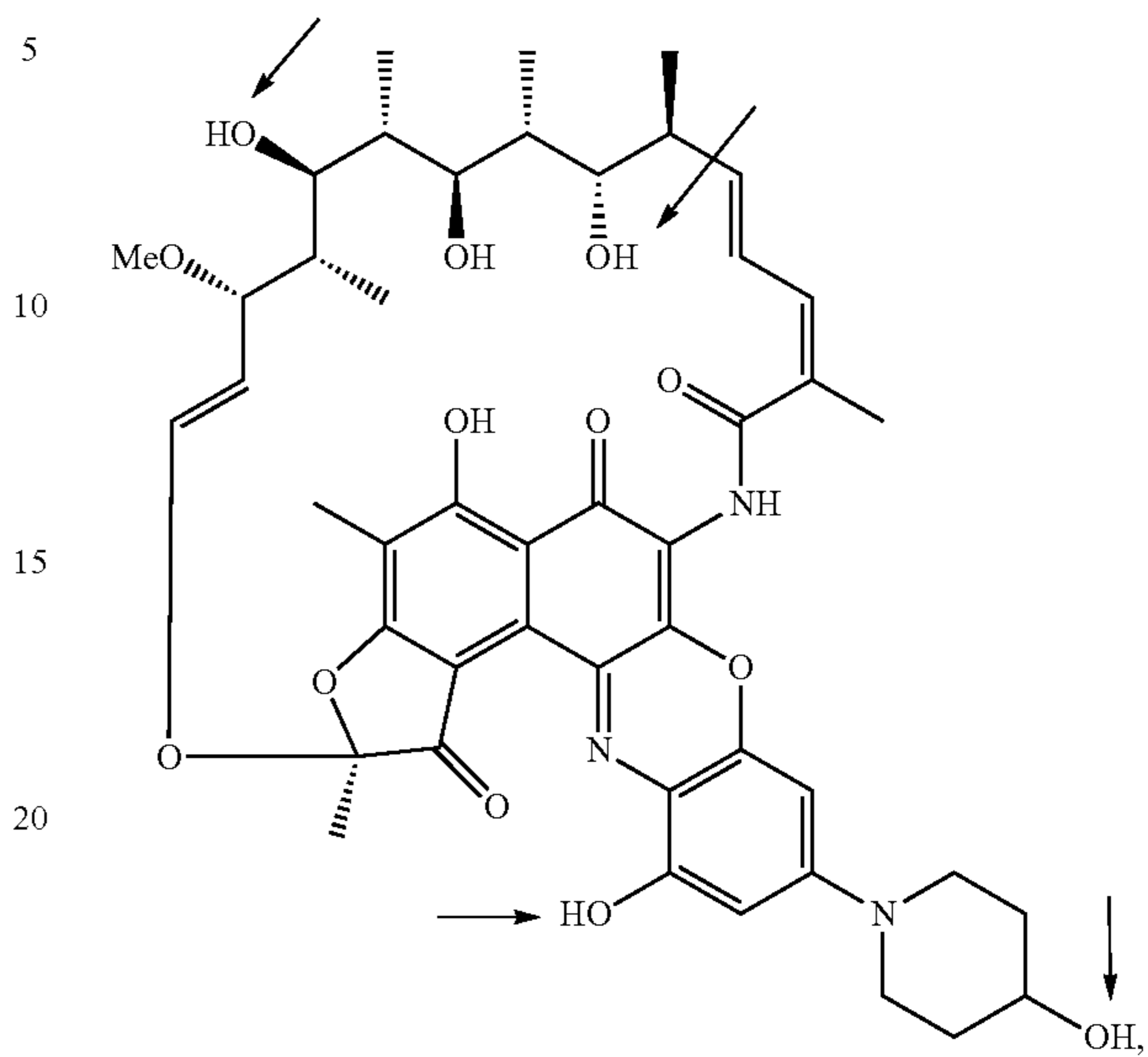
Deacetylated compound 63
