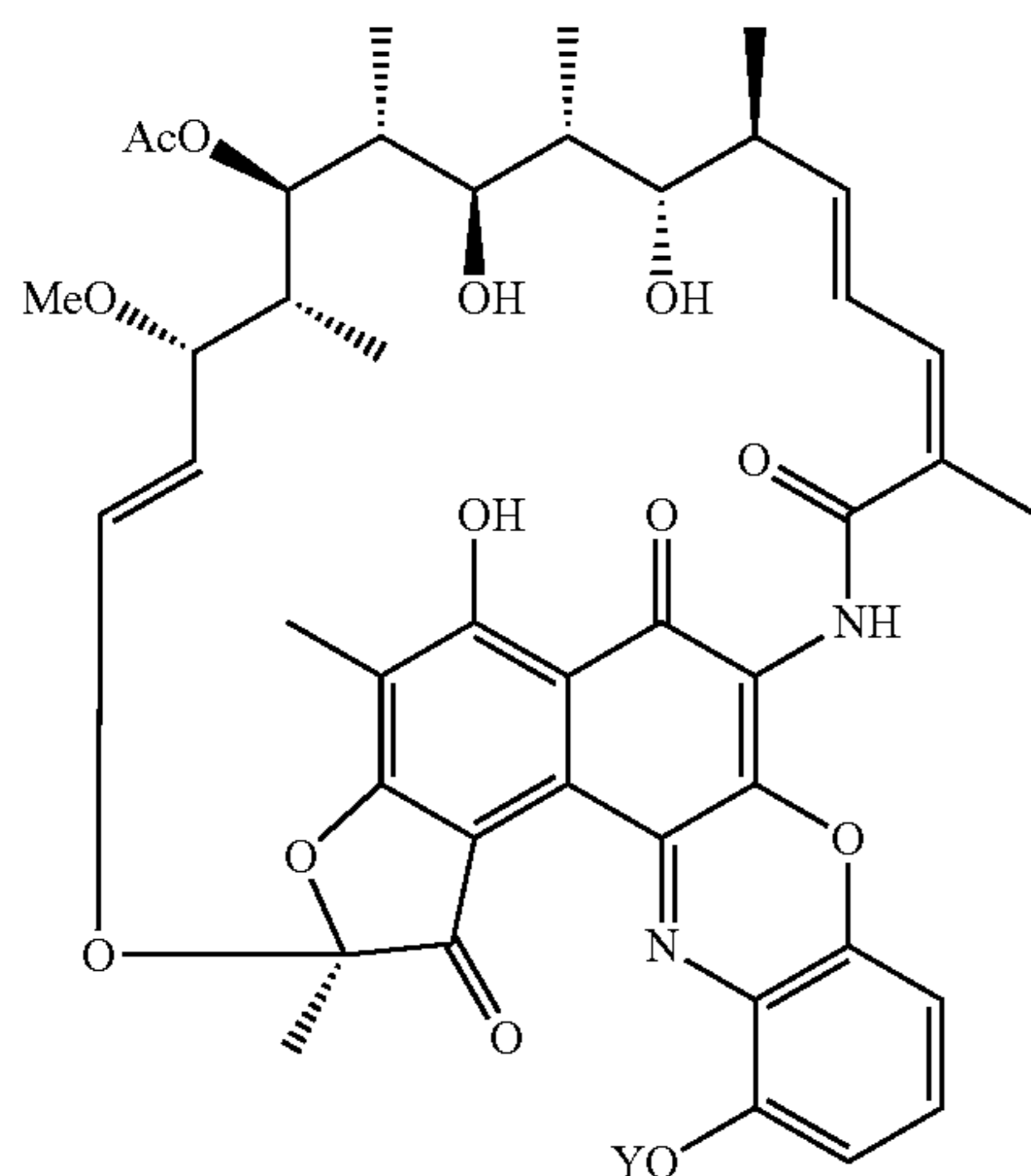
XLVa Y = H XLVb Y = Trialkylsilyl
