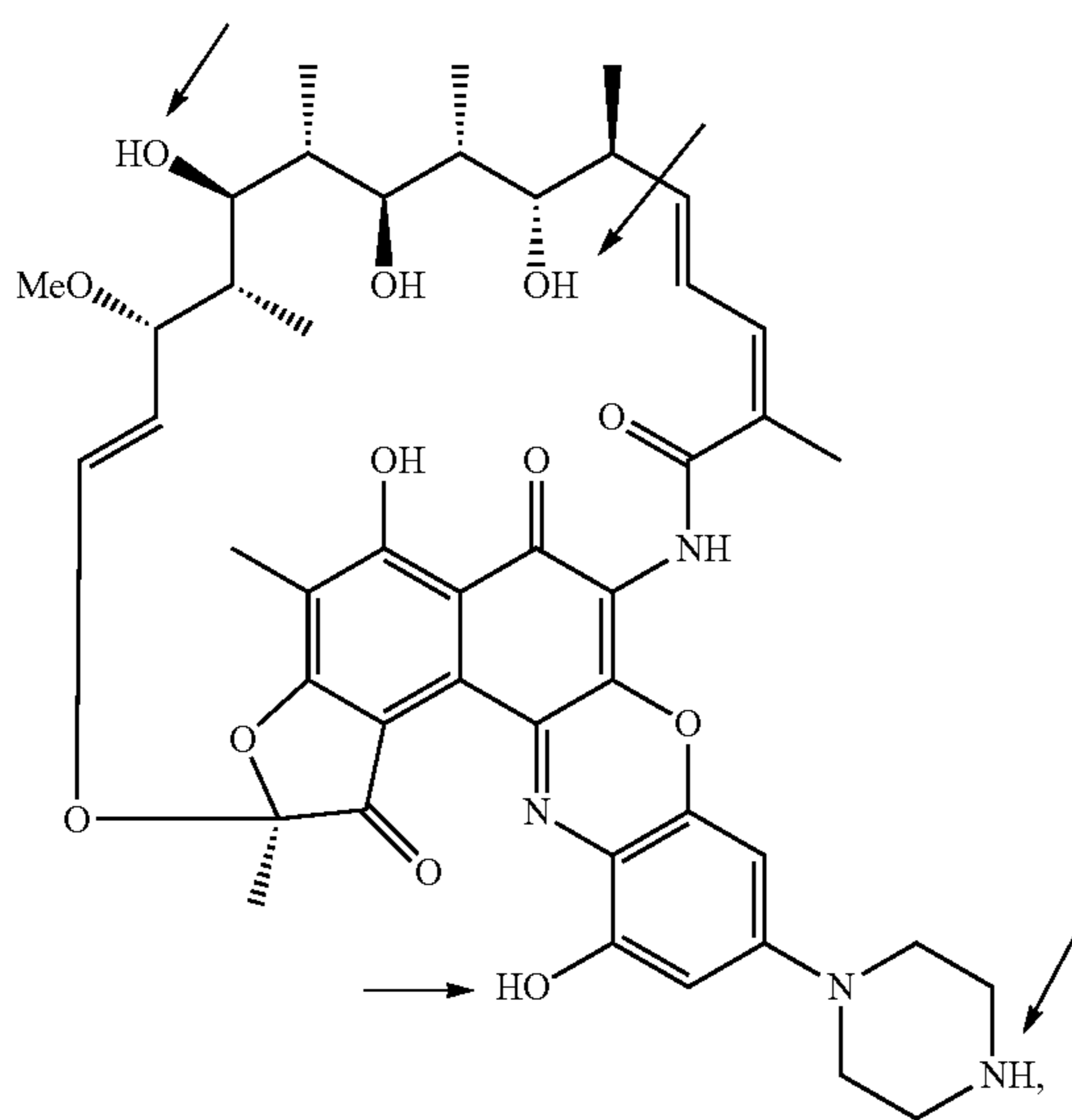
Deacetylated compound 69
